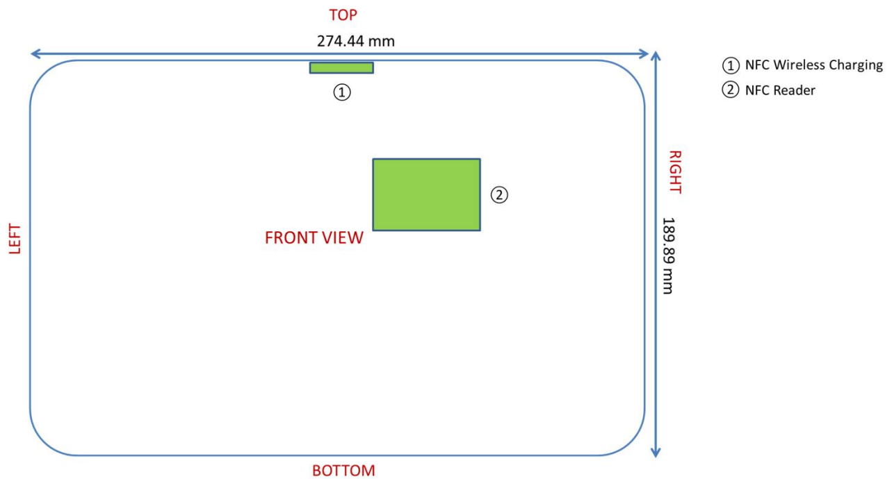
Figure G-1 DUT Antenna Locations
