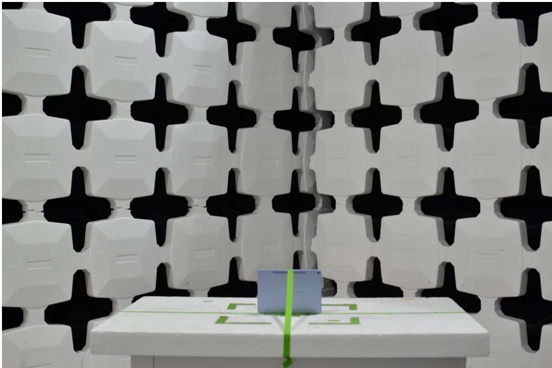
Figure 6. Test Setup – Z Position – 30MHz-1GHz – NFC
