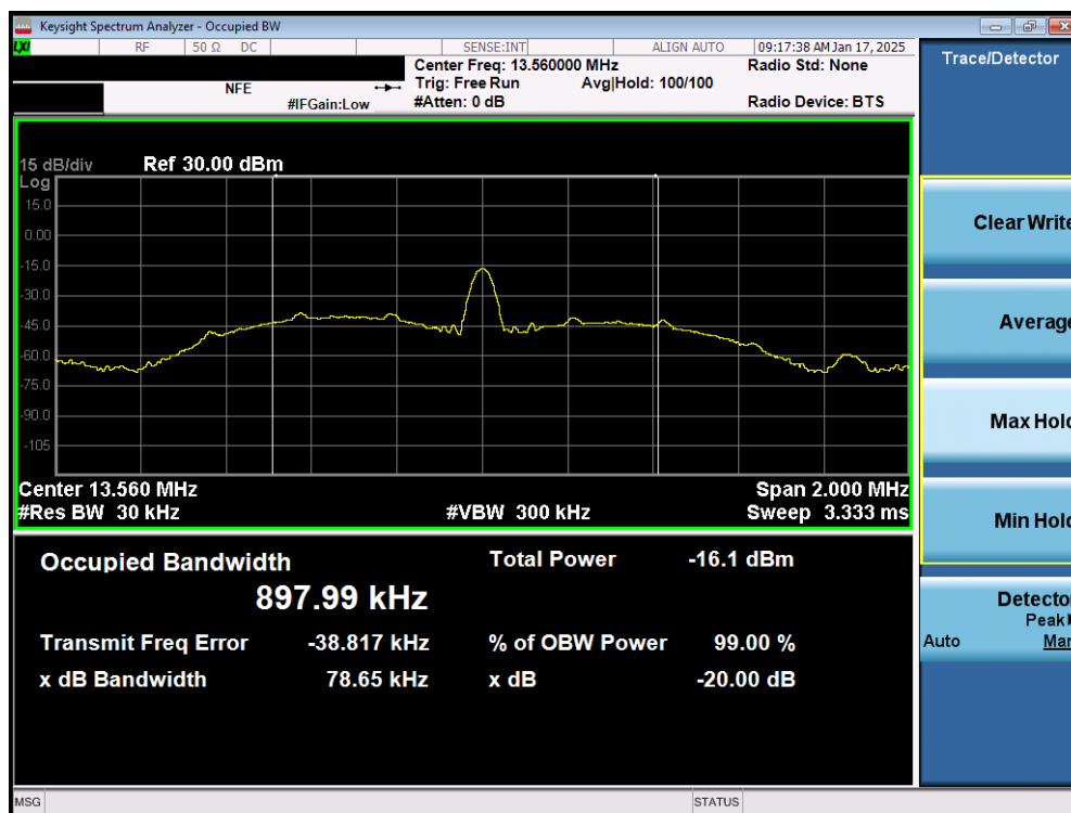
Figure 7-4. Occupied Bandwidth Plot – NFC F
