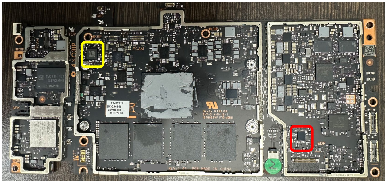
Figure 4: PCB top side, with covers removed
