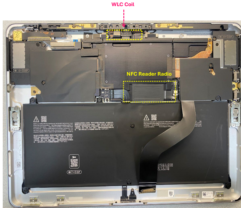
Figure 1: Behind the display
