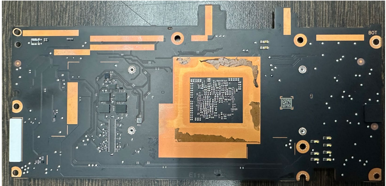
Figure 5: PCB bottom side, with covers removed
