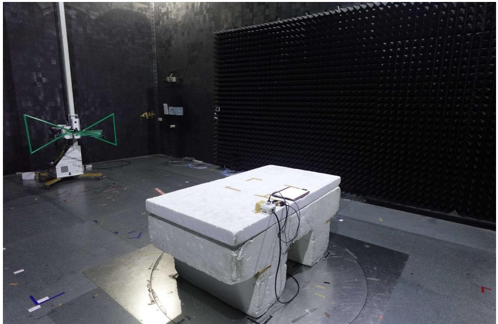
Rear view
