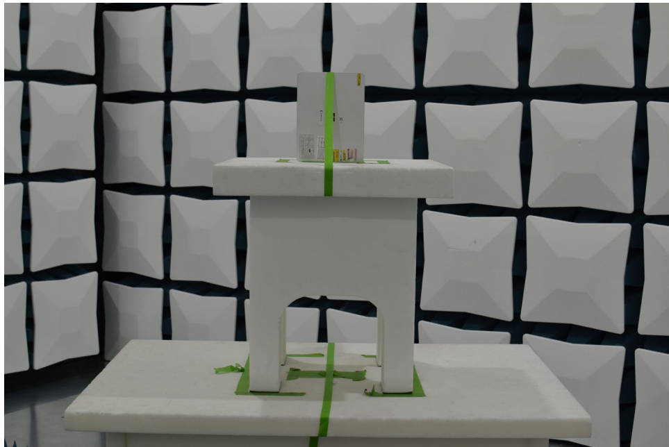
Figure 4. Test Setup – Y Position – 1GHz-40GHz – Closed
