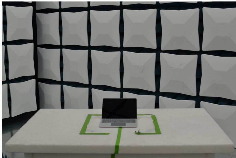
Figure 12. Test Setup – X Position – 30MHz-1GHz – Open
