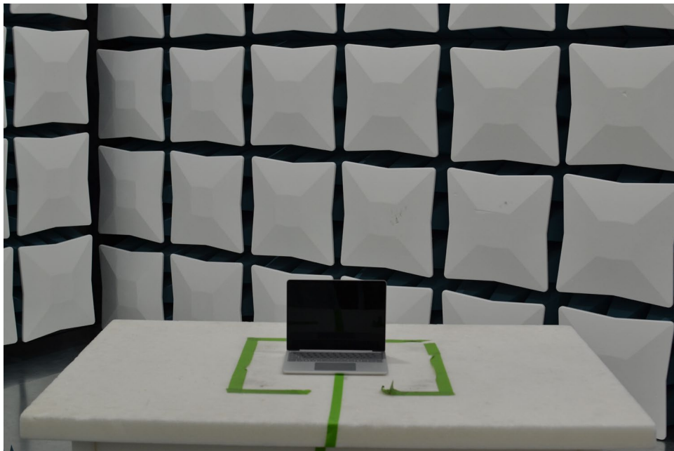
Figure 18. Test Setup – X Position – 30MHz-1GHz – Half Open
