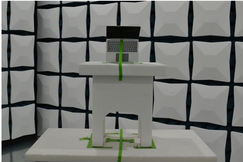
Figure 11. Test Setup – Z Position – 1GHz-40GHz – Open
