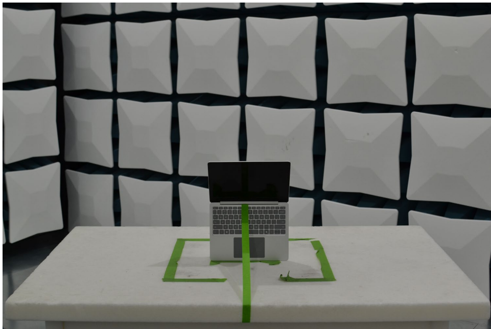
Figure 14. Test Setup – Z Position – 30MHz-1GHz – Open
