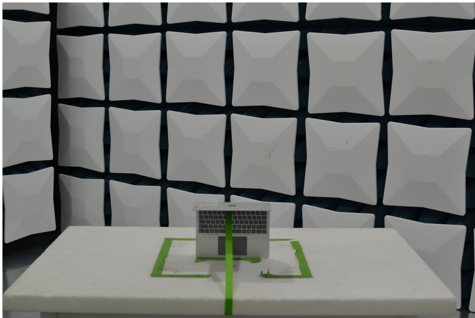
Figure 20. Test Setup – Z Position – 30MHz-1GHz – Half Open
