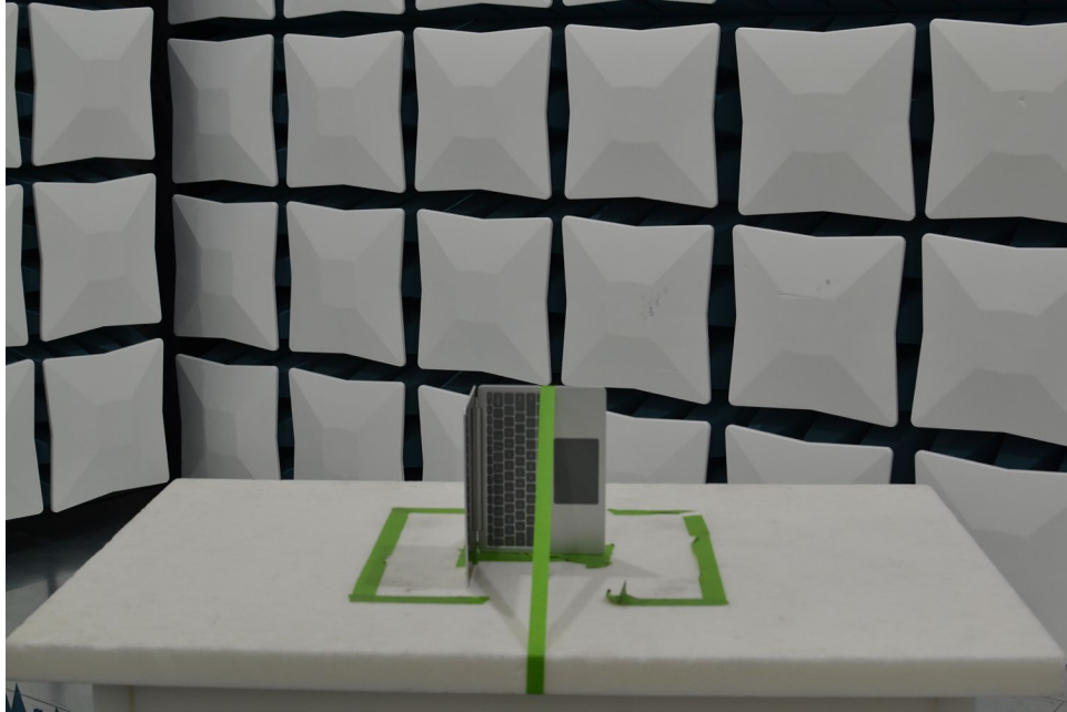
Figure 19. Test Setup – Y Position – 30MHz-1GHz – Half Open
