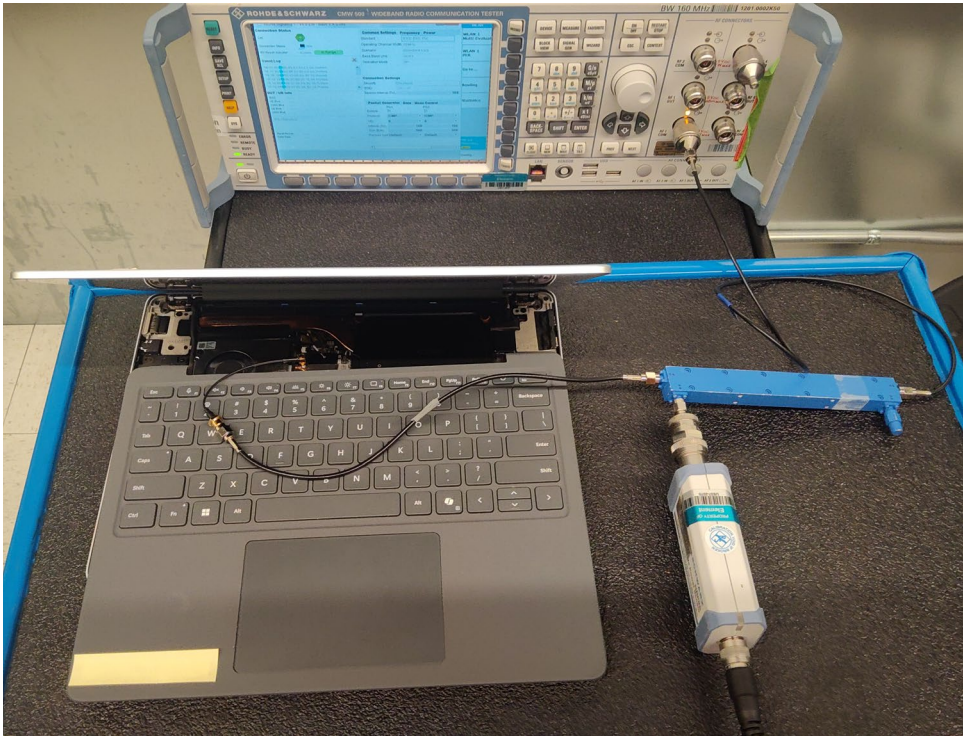
Test Setup Photo 2 – Conducted Test Setup (Figure 6-1a)
