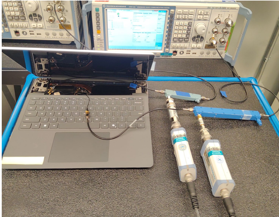
Test Setup Photo 3 – Conducted Test Setup (Figure 6-1b)
