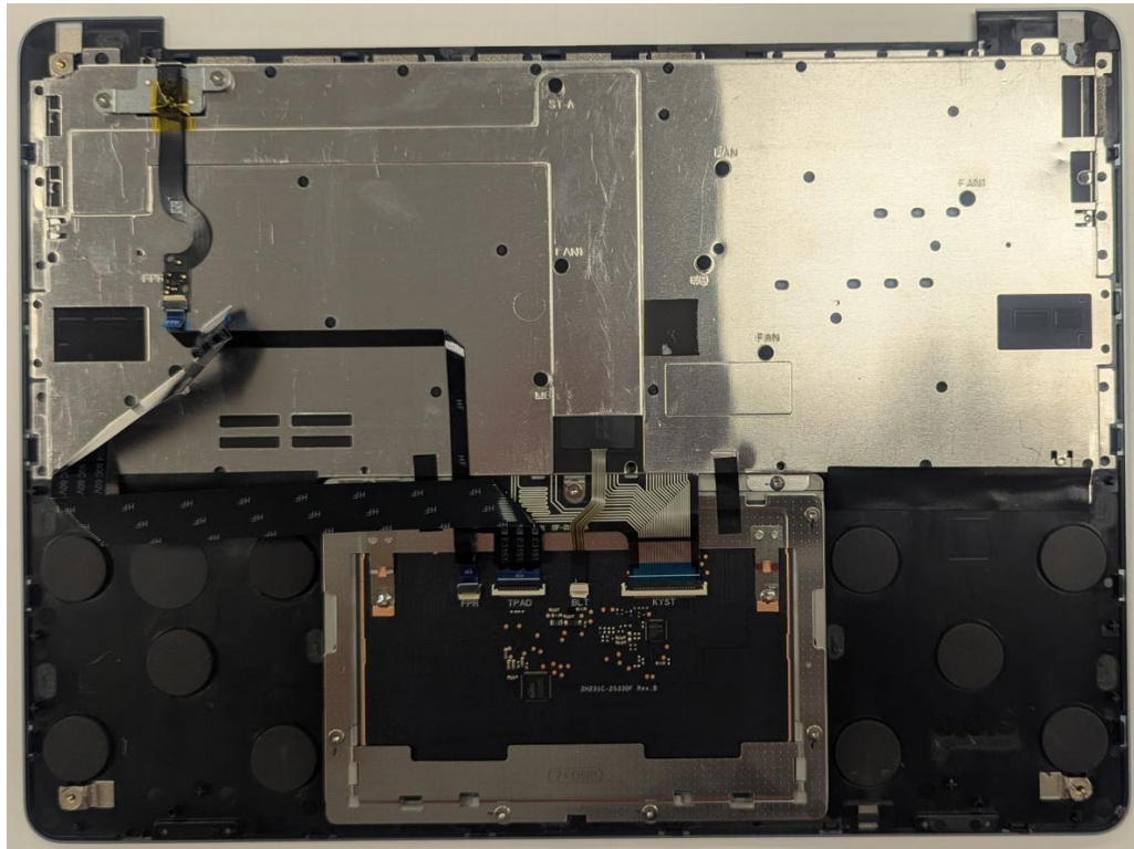
Figure 4: Behind the keyboard
