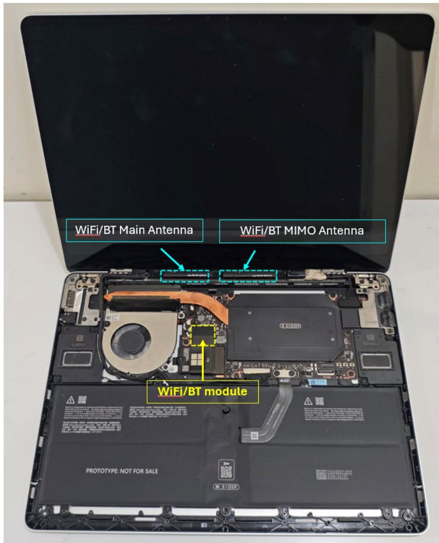
Figure 1: Front View with keyboard removed
