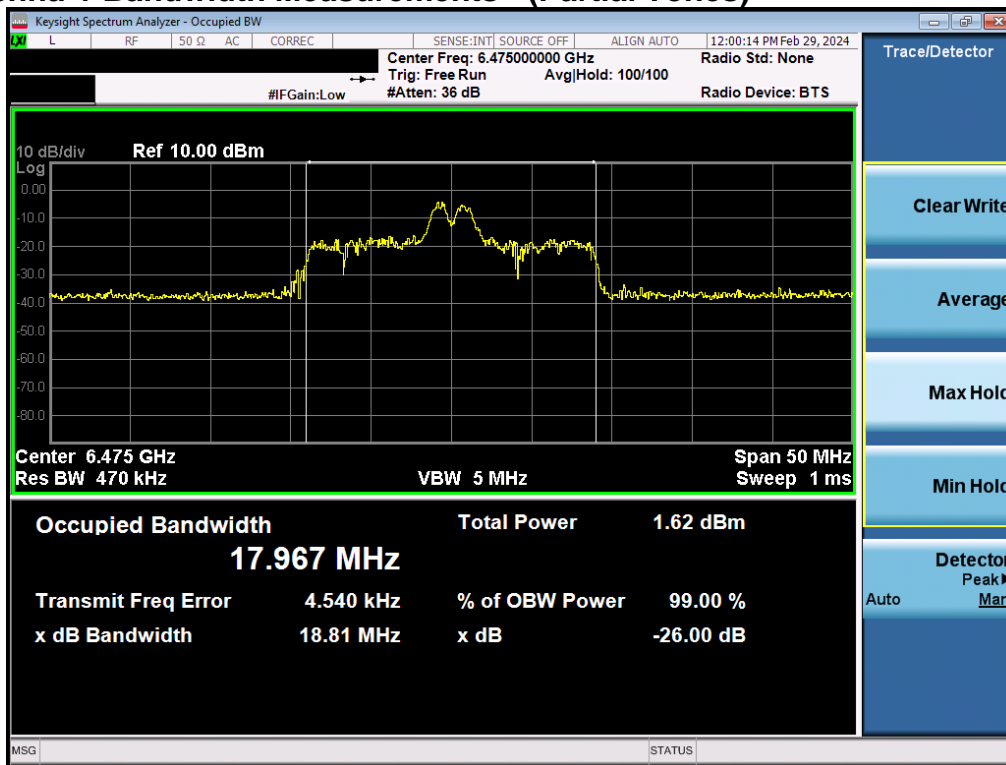
Plot 7-6. Occupied Bandwidth Plot MIMO ANT1 (20MHz BW 802.11be (26 Tones) (UNII Band 6) – Ch. 105)
