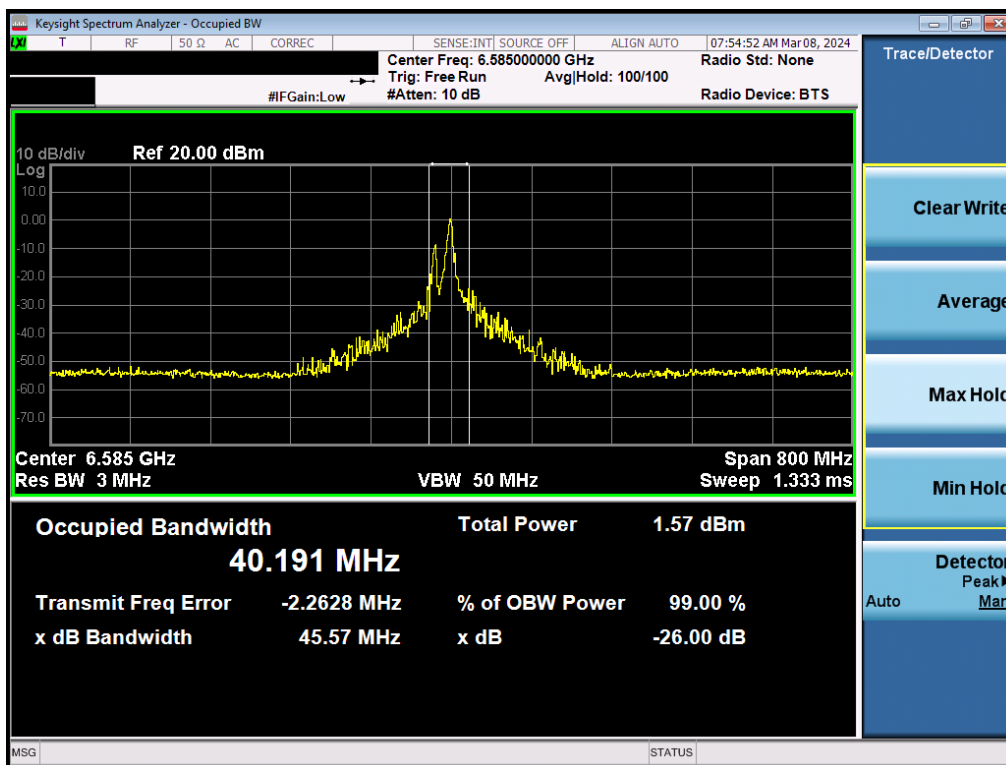
Plot 7-15. Occupied Bandwidth Plot MIMO ANT1 (320MHz BW 802. 11be (26 Tones) (UNII Band 7) – Ch. 127)
