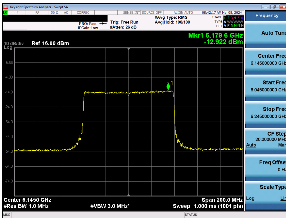
Plot 7-103. Power Spectral Density Plot MIMO ANT1 (80MHz BW 802.11be (Full Tone) (UNII Band 5) – Ch. 39)
