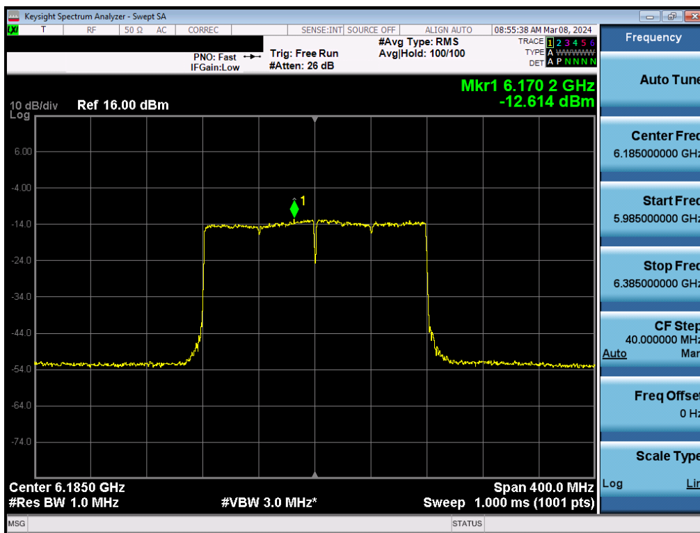
Plot 7-104. Power Spectral Density Plot MIMO ANT1 (160MHz BW 802.11be (Full Tone) (UNII Band 5) – Ch. 47)
