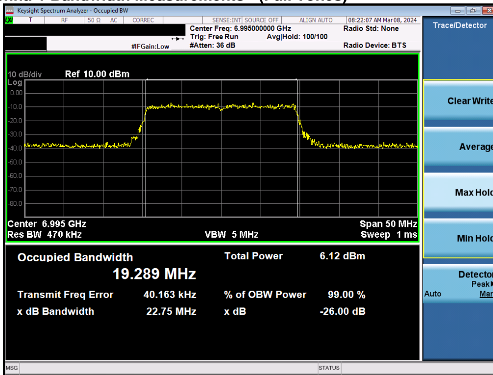
Plot 7-36. Occupied Bandwidth Plot MIMO ANT1 (20MHz BW 802.11be (Full Tone) (UNII Band 8) – Ch. 209)
