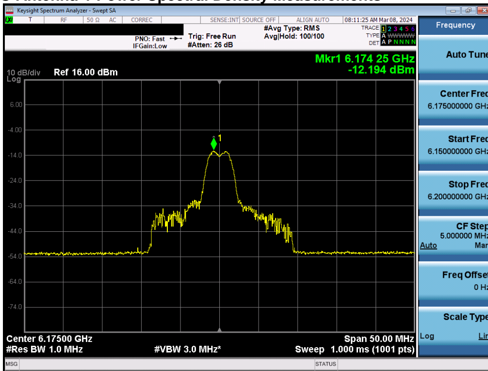
Plot 7-81. Power Spectral Density Plot MIMO ANT1 (20MHz BW 802.11be (26 Tones) (UNII Band 5) – Ch. 45)
