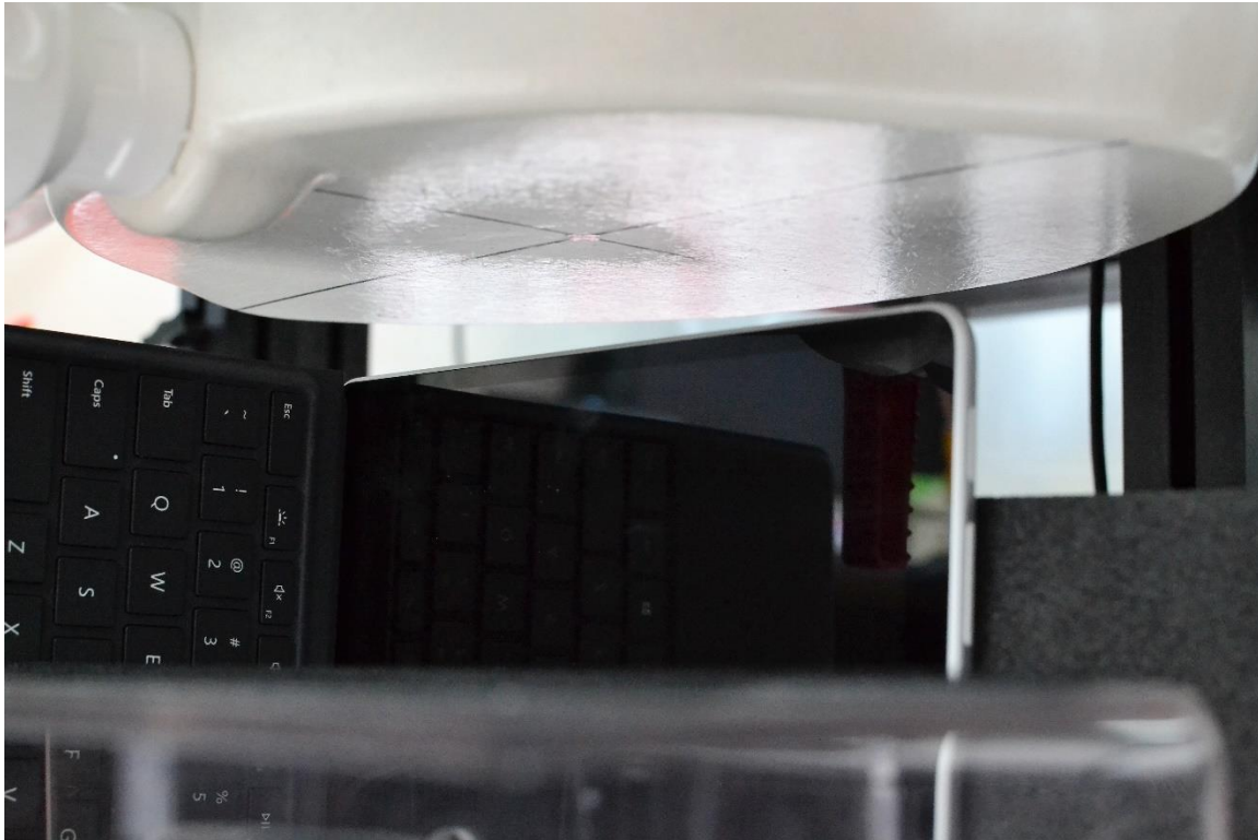
SAR Test Setup Photo 37 – Laptop, Left Edge at 25mm – All Antennas
