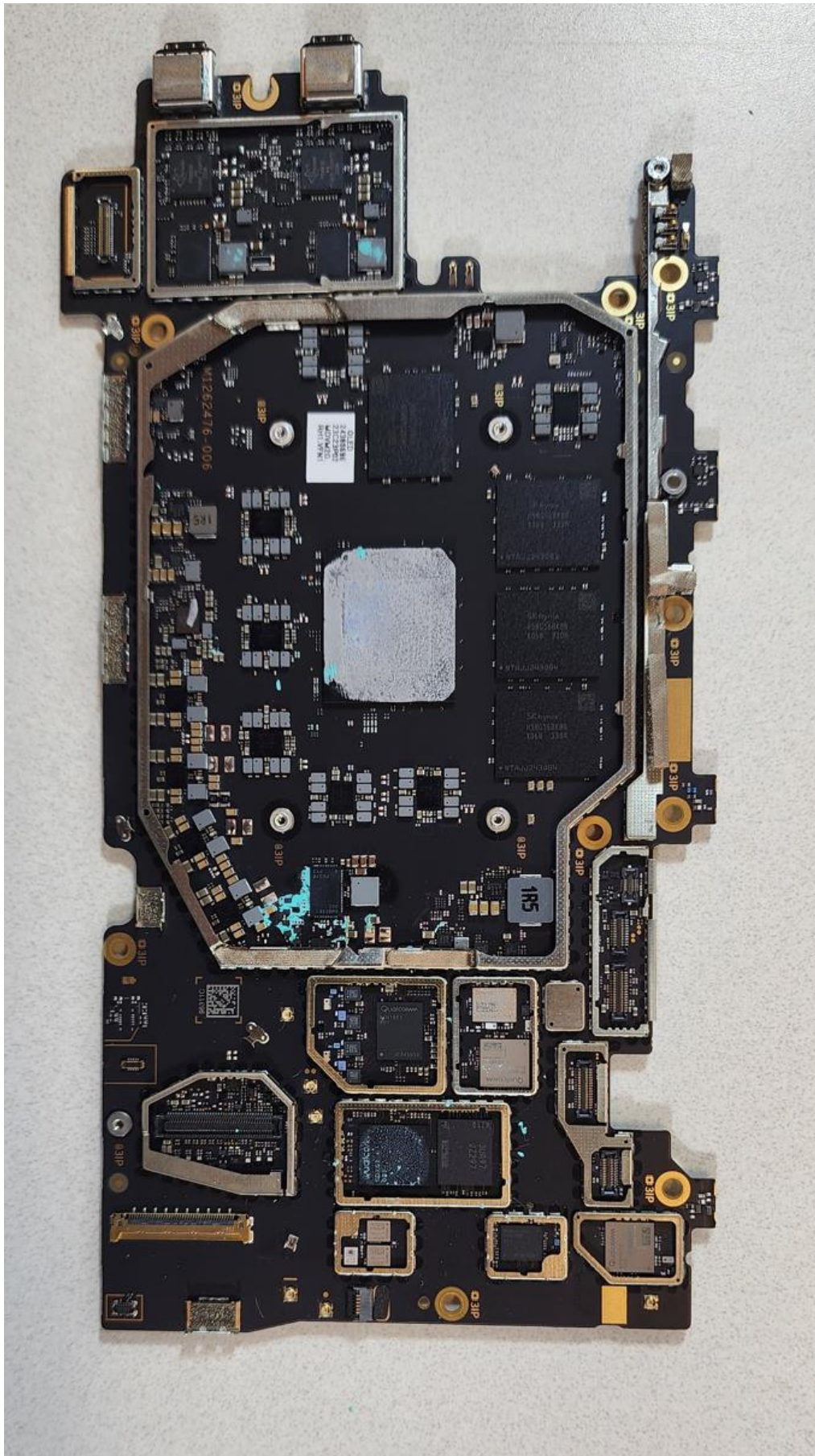
Model 2077 Internal Photographs
