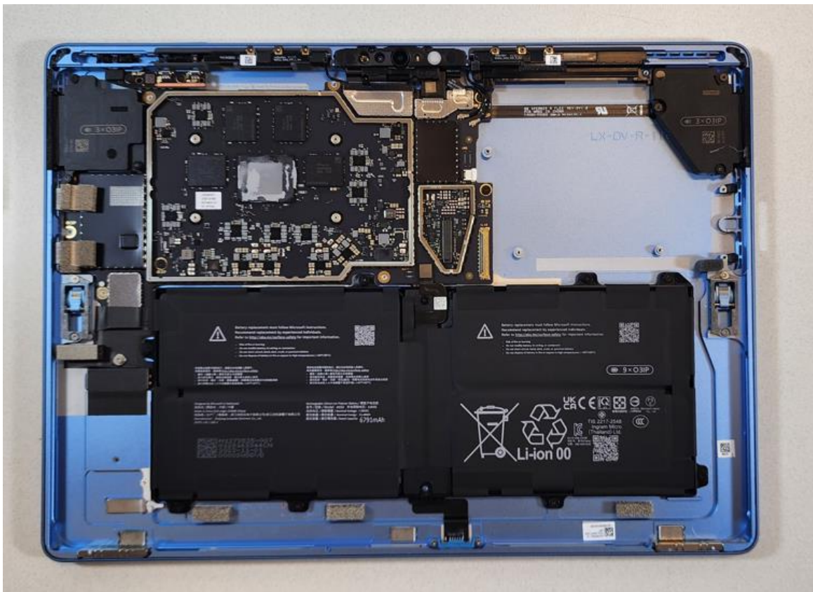
Model 2076 Internal Photographs
