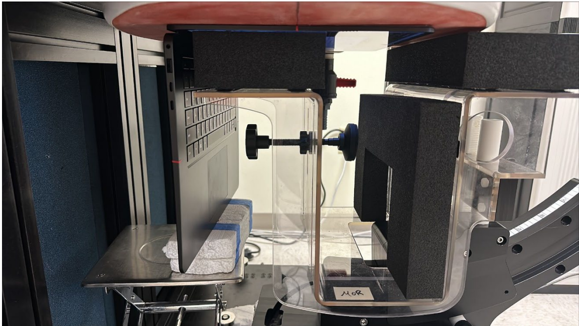
Photograph 5: Standalone, Rear of Display, 0 mm, screen at 90°
