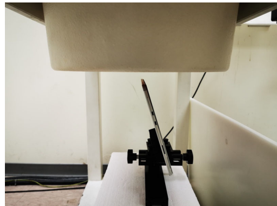
Photograph 20. Body, Top Curve, 30mm
