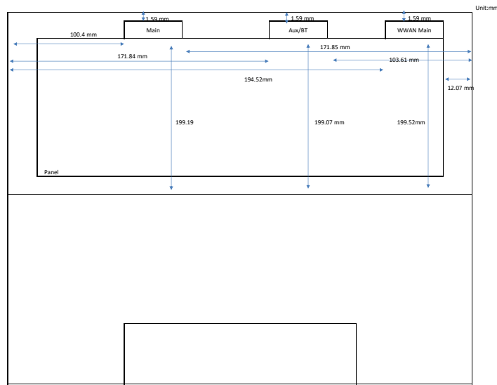
Photograph 25. Antenna position of EUT (Tablet mode)
