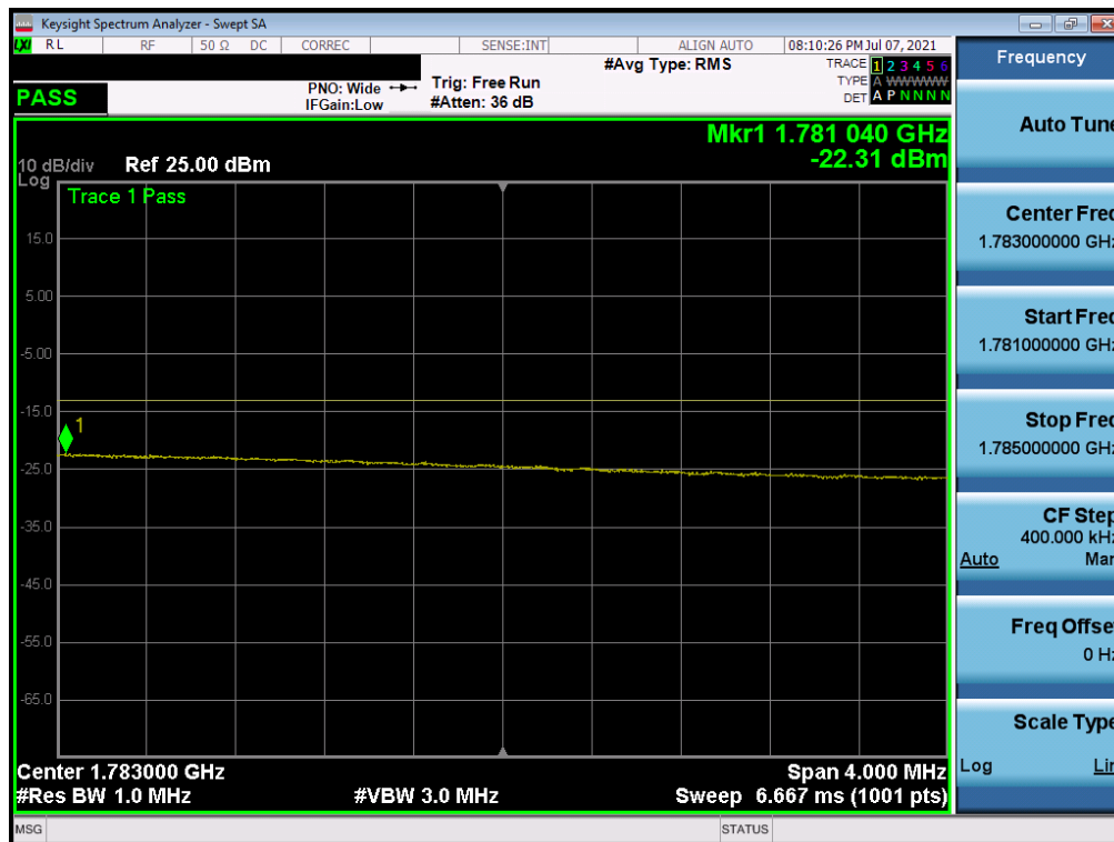
Plot 7-186. Upper Extended Band Edge Plot (NR Band n66 – 30.0MHz - Full RB)
