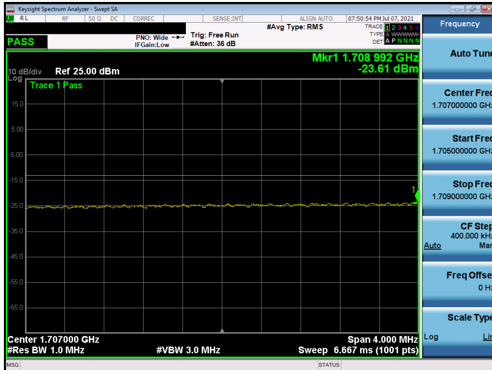
Plot 7-180. Lower Extended Band Edge Plot (NR Band n66 – 40.0MHz - Full RB)
