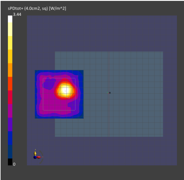
Figure 12-2 4cm 2 psPD distribution measured at input.power.limit of 5.7 dBm on the flat, back side for n260 beam 5
