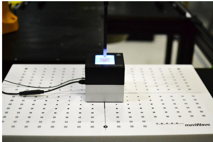
Figure 14-1 System Verification Setup Photo
