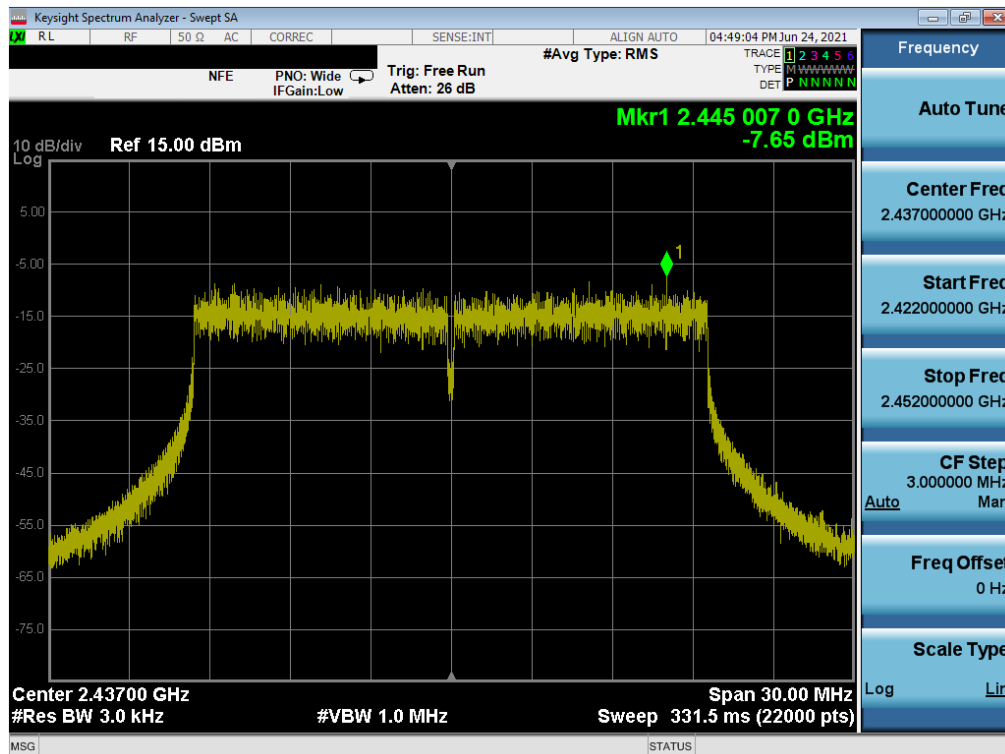
Plot 7-53. Power Spectral Density Plot MIMO SOUTH (802.11ax 20MHz BW OFDMA – 242 Tones – Ch. 6)
