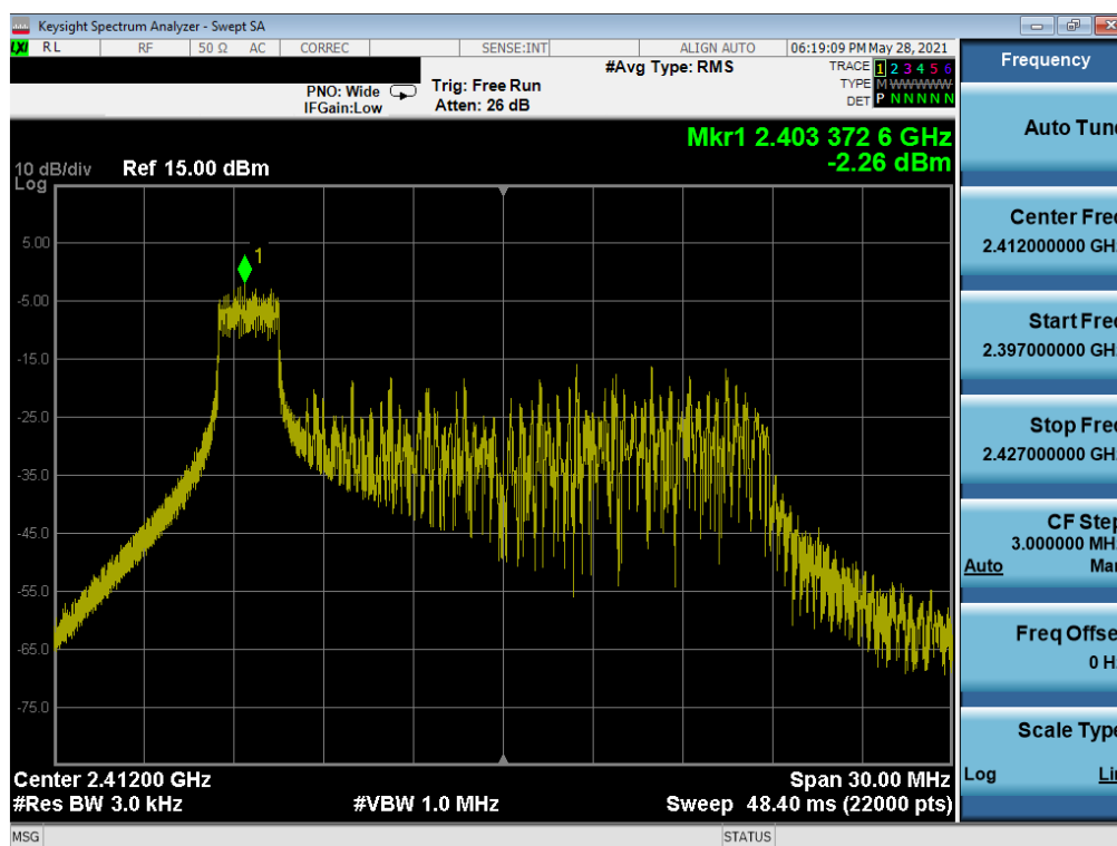
Plot 7-37. Power Spectral Density Plot SISO NORTH (802.11ax 20MHz BW OFDMA - 26 Tones - Ch. 1)
