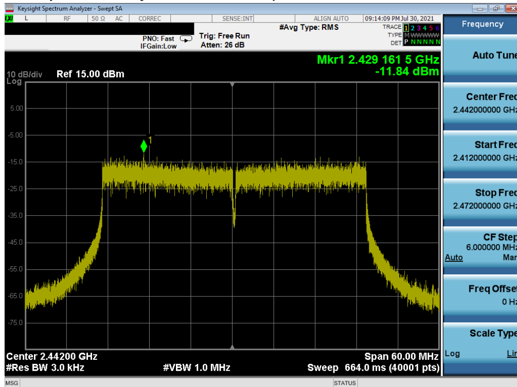
Plot 7-47. Power Spectral Density Plot SISO NORTH (802.11ax 40MHz BW OFDMA – 484 Tones – Ch. 7)
