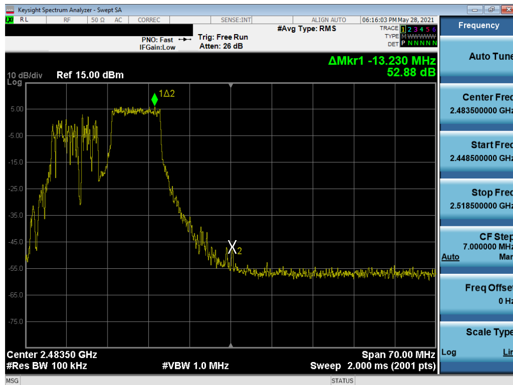
Plot 7-76. Band Edge Plot SISO SOUTH (802.11ax 20MHz BW OFDMA - 106 Tones - Ch. 11)
