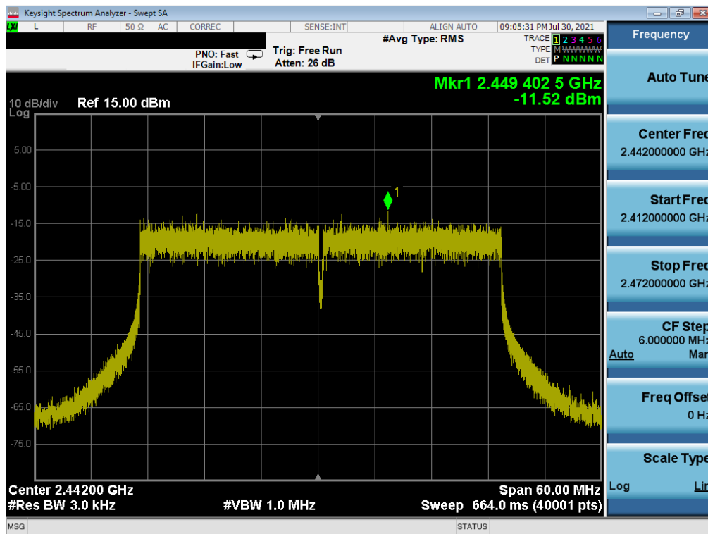
Plot 7-35. Power Spectral Density Plot SISO SOUTH (802.11ax 40MHz BW OFDMA – 484 Tones – Ch. 7)
