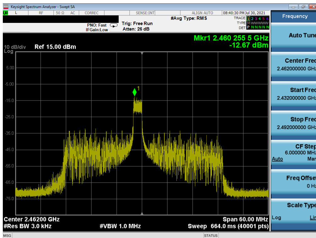
Plot 7-45. Power Spectral Density Plot SISO NORTH (802.11ax 40MHz BW OFDMA – 26 Tones – Ch. 11)
