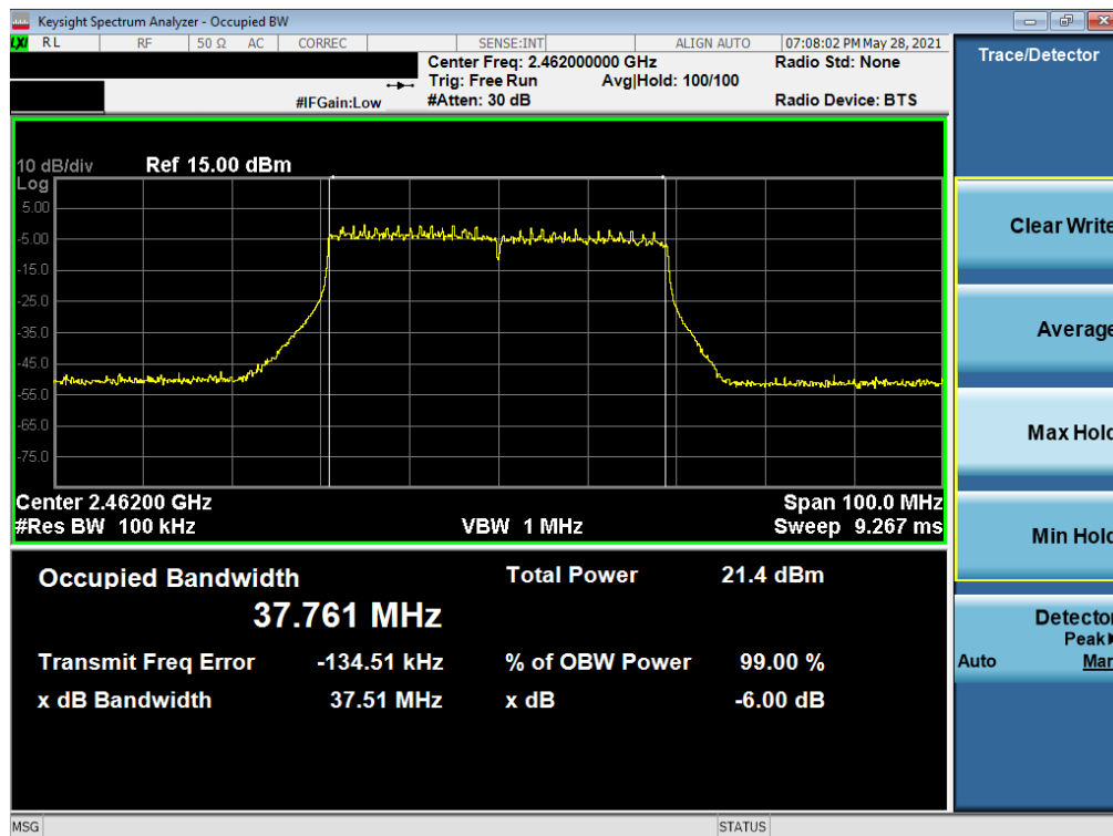
Plot 7-12. 6dB Bandwidth Plot SISO SOUTH (802.11ax 40MHz BW OFDMA – 484 Tones – Ch. 11)
