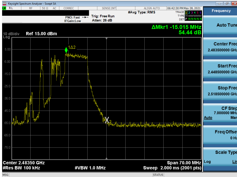
Plot 7-101. Band Edge Plot SISO NORTH (802.11ax 20MHz BW OFDMA – 106 Tones – Ch. 12)
