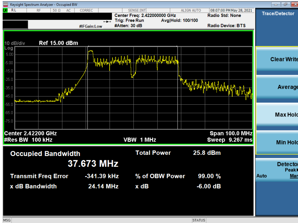
Plot 7-19. 6dB Bandwidth Plot SISO SOUTH (802.11ax 40MHz BW OFDMA – 26 Tones – Ch. 3)
