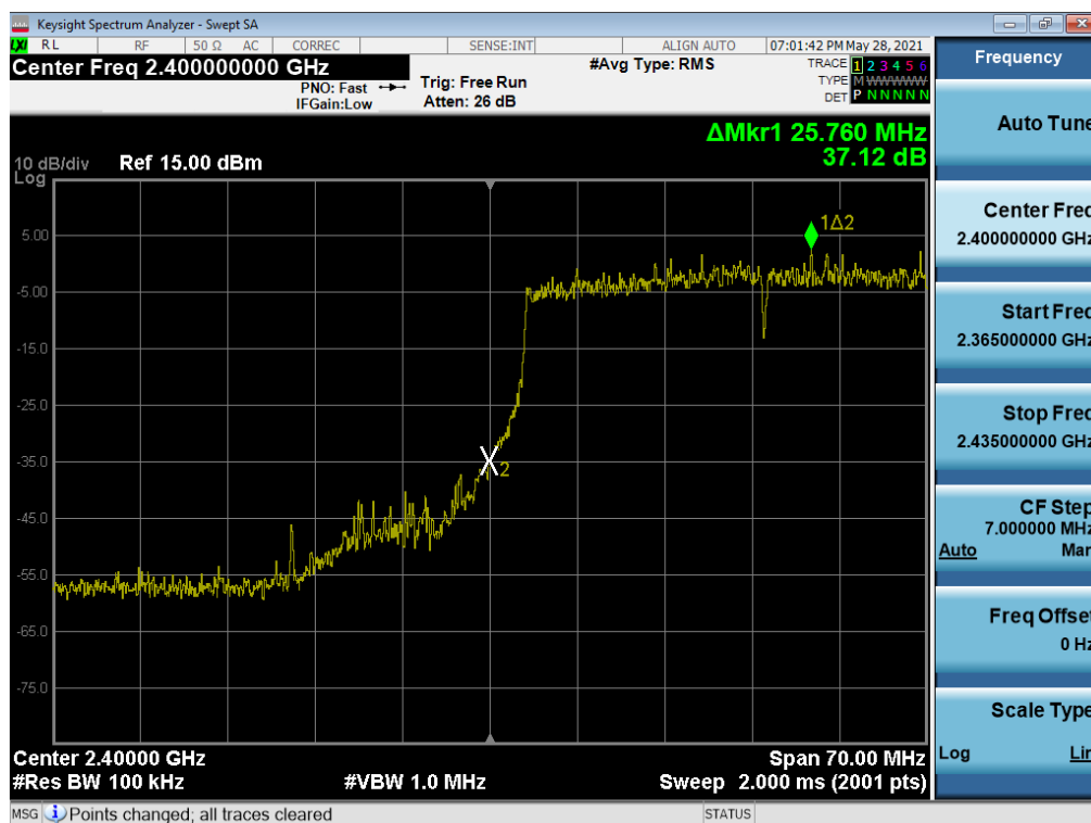
Plot 7-92. Band Edge Plot SISO SOUTH (802.11ax 40MHz BW OFDMA – 484 Tones – Ch. 3)
