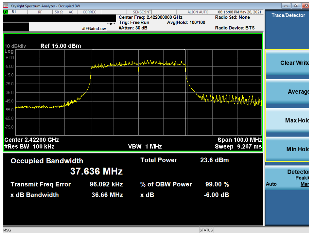
Plot 7-22. 6dB Bandwidth Plot SISO SOUTH (802.11ax 40MHz BW OFDMA – 484 Tones – Ch. 3)
