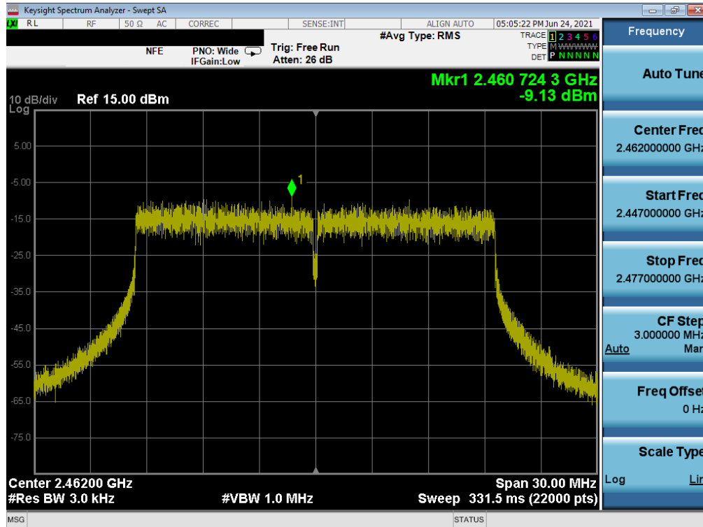
Plot 7-60. Power Spectral Density Plot MIMO NORTH (802.11ax 20MHz BW OFDMA – 484 Tones – Ch. 11)
