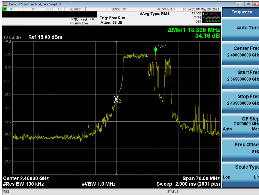
Plot 7-73. Band Edge Plot SISO SOUTH (802.11ax 20MHz BW OFDMA – 106 Tones – Ch. 1)
