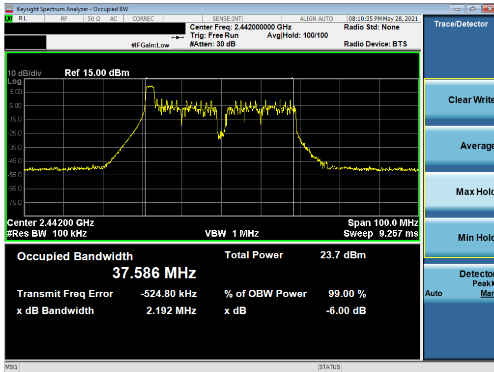
Plot 7-20. 6dB Bandwidth Plot SISO SOUTH (802.11ax 40MHz BW OFDMA – 26 Tones – Ch. 7)
