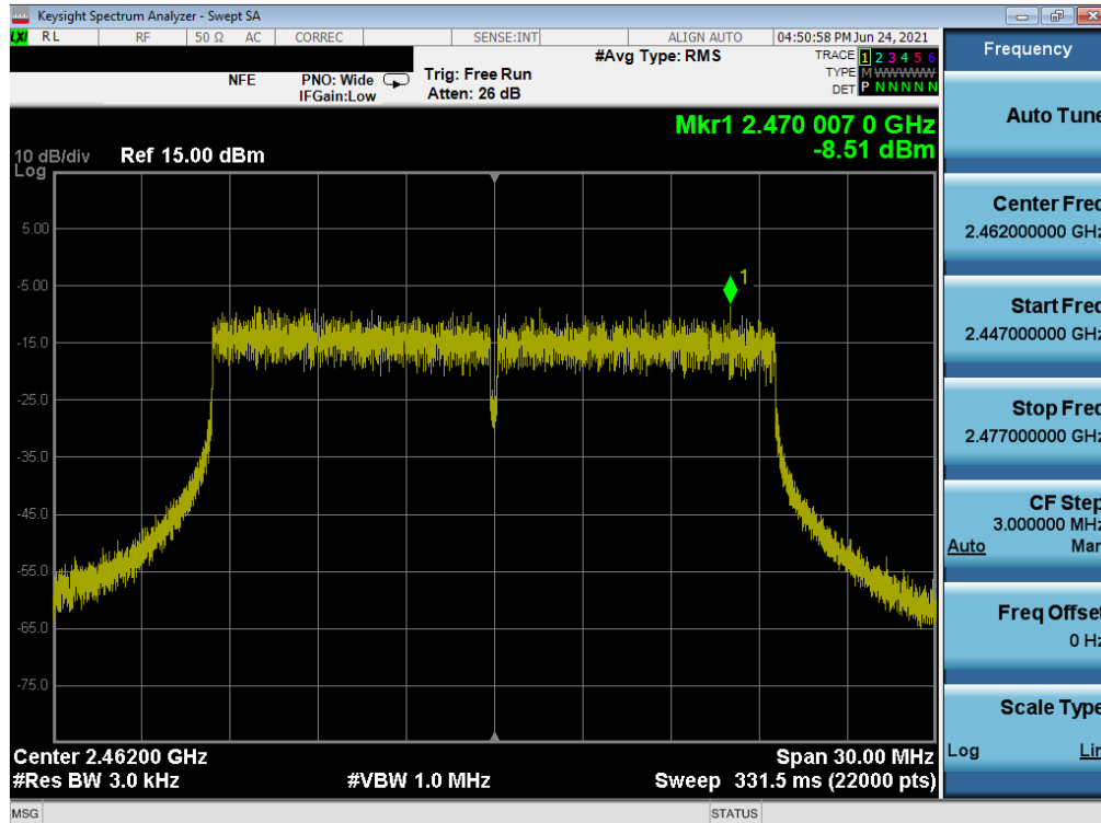
Plot 7-54. Power Spectral Density Plot MIMO SOUTH (802.11ax 20MHz BW OFDMA – 242 Tones – Ch. 11)
