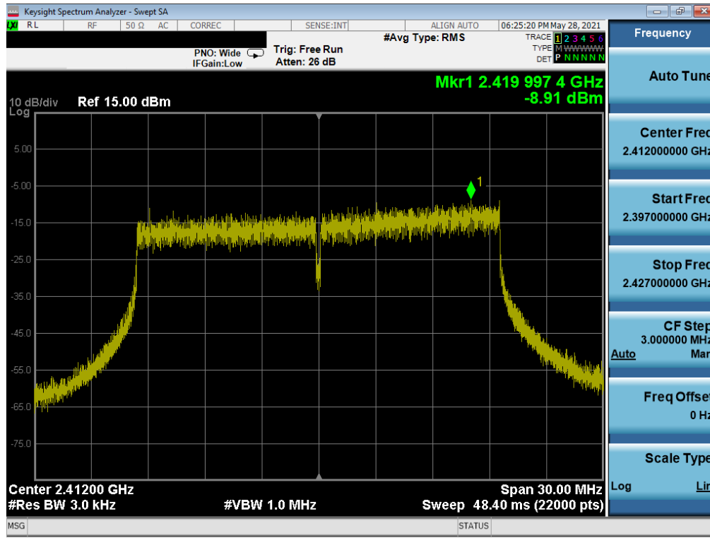
Plot 7-40. Power Spectral Density Plot SISO NORTH (802.11ax 20MHz BW OFDMA – 242 Tones – Ch. 1)
