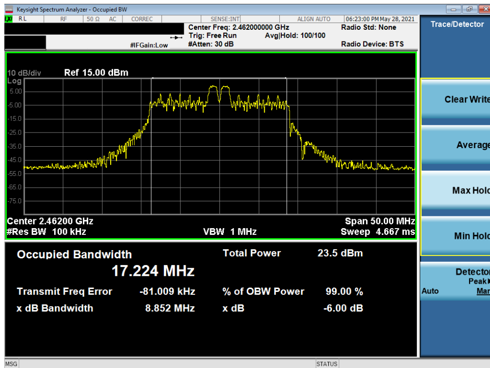
Plot 7-15. 6dB Bandwidth Plot SISO SOUTH (802.11ax 20MHz BW OFDMA – 26 Tones – Ch. 11)
