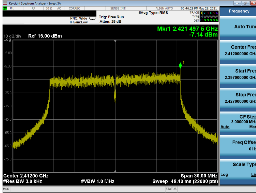
Plot 7-28. Power Spectral Density Plot SISO SOUTH (802.11ax 20MHz BW OFDMA – 242 Tones – Ch. 1)
