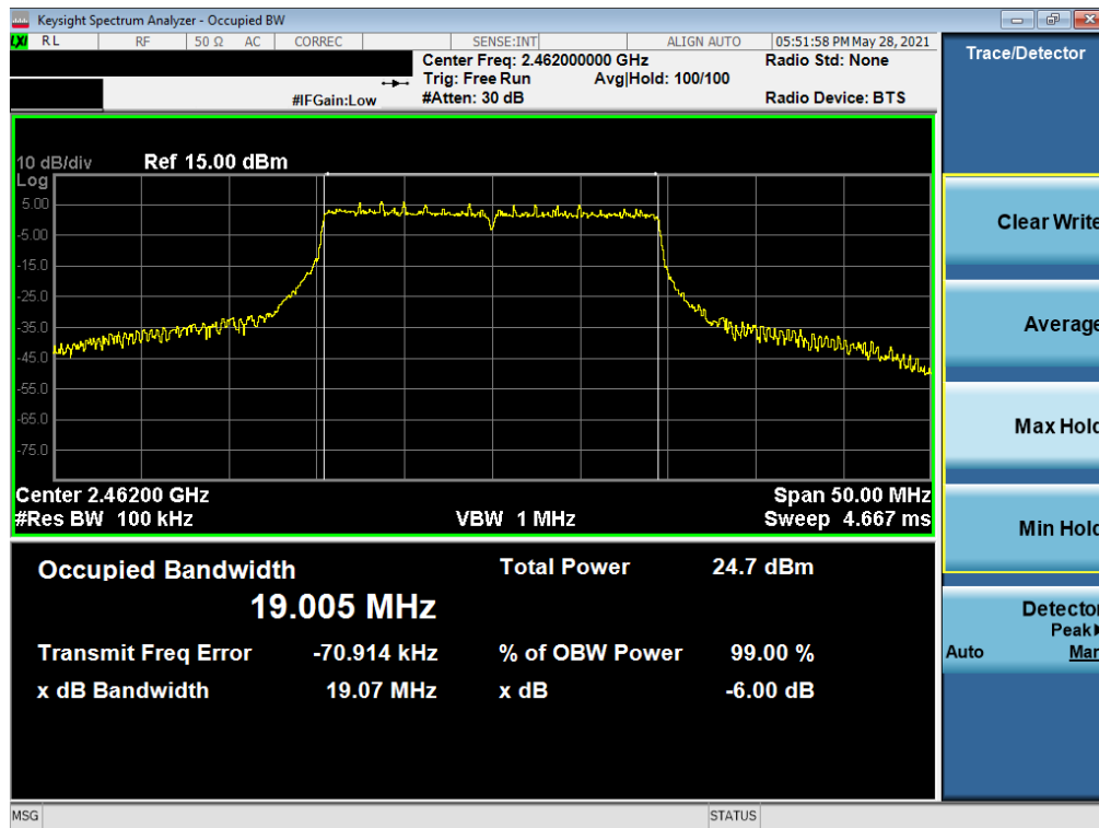
Plot 7-6. 6dB Bandwidth Plot SISO SOUTH (802.11ax 20MHz BW OFDMA – 242 Tones – Ch. 11)
