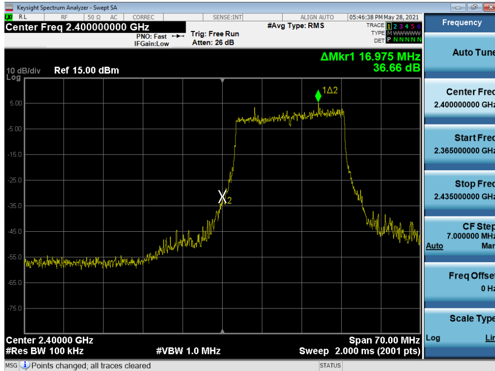
Plot 7-79. Band Edge Plot SISO SOUTH (802.11ax 20MHz BW OFDMA – 242 Tones – Ch. 1)
