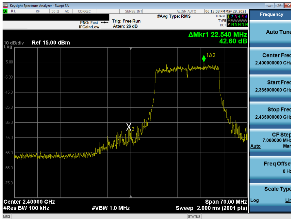
Plot 7-80. Band Edge Plot SISO SOUTH (802.11ax 20MHz BW OFDMA – 242 Tones – Ch. 2)
