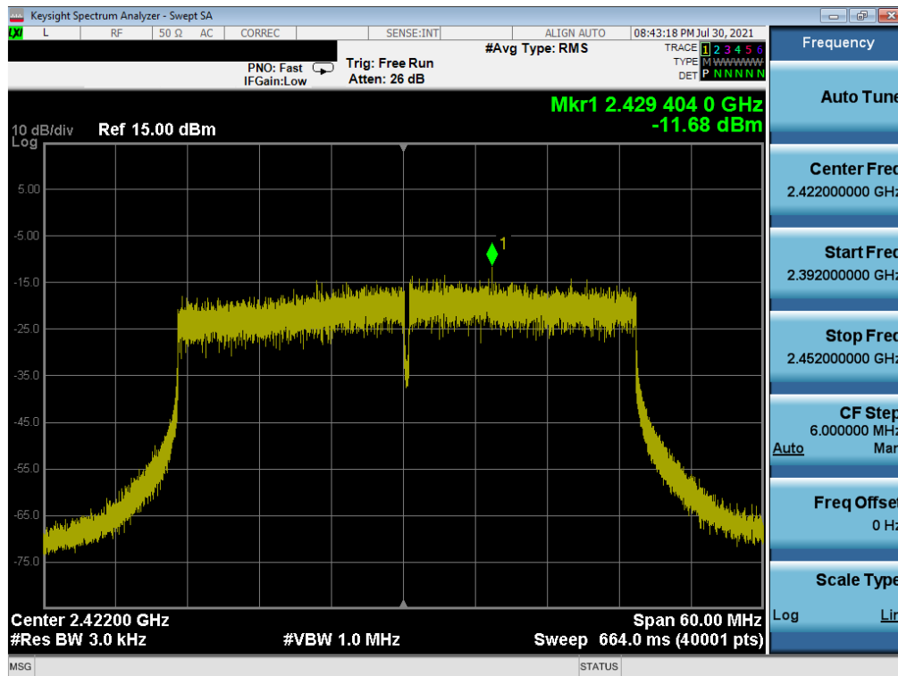
Plot 7-70. Power Spectral Density Plot MIMO NORTH (802.11ax 40MHz BW OFDMA – 484 Tones – Ch. 3)
