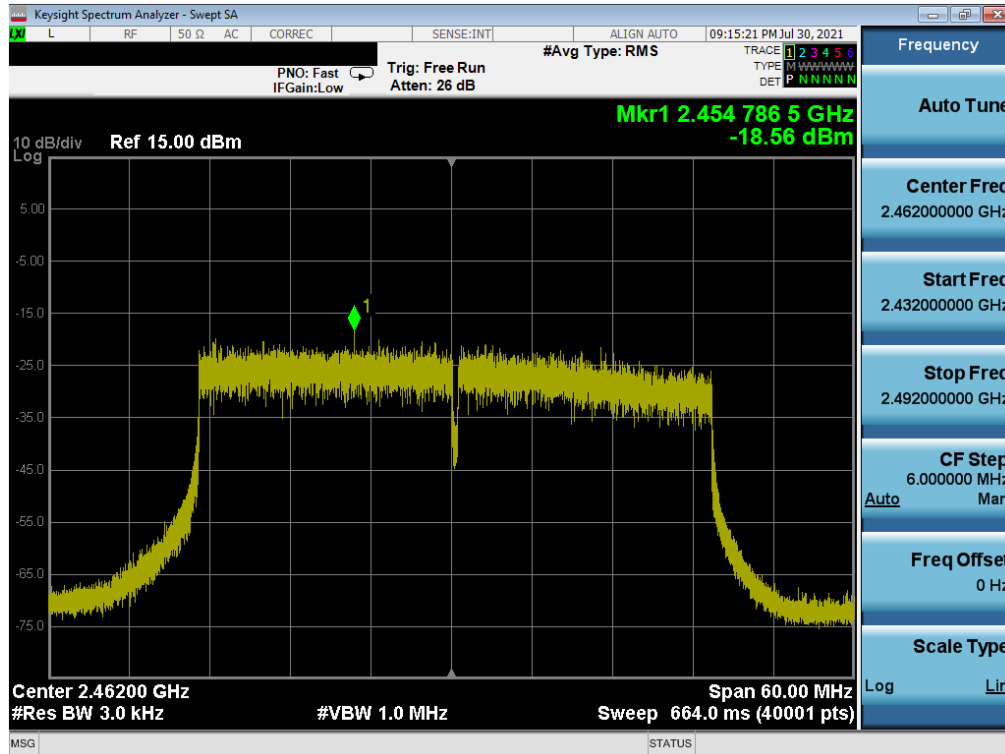
Plot 7-48. Power Spectral Density Plot SISO NORTH (802.11ax 40MHz BW OFDMA – 484 Tones – Ch. 11)
