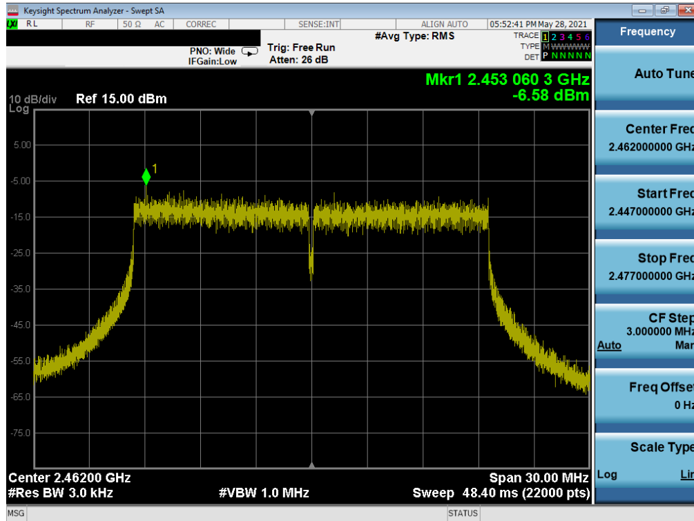
Plot 7-30. Power Spectral Density Plot SISO SOUTH (802.11ax 20MHz BW OFDMA – 242 Tones – Ch. 11)
