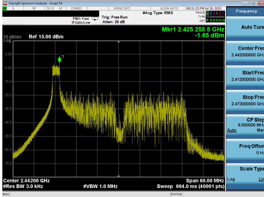
Plot 7-68. Power Spectral Density Plot MIMO NORTH (802.11ax 40MHz BW OFDMA – 26 Tones – Ch. 7)
