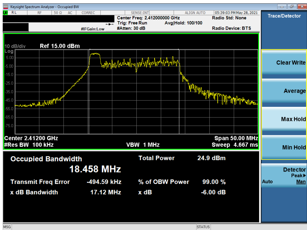
Plot 7-1. 6dB Bandwidth Plot SISO SOUTH (802.11ax 20MHz BW OFDMA – 26 Tones – Ch. 1)
