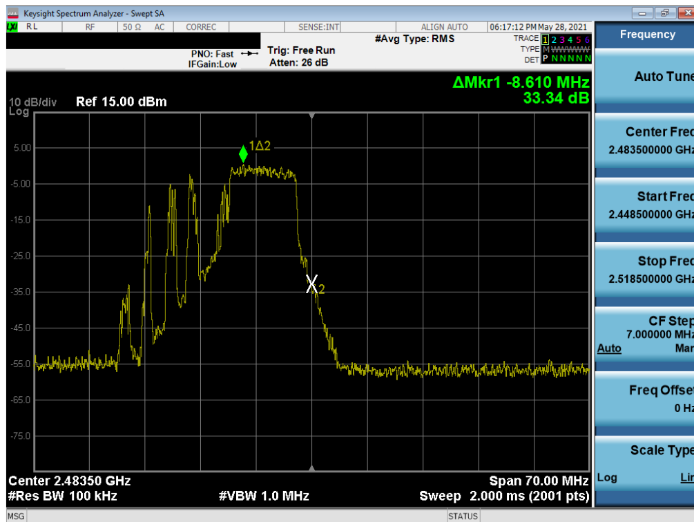
Plot 7-78. Band Edge Plot SISO SOUTH (802.11ax 20MHz BW OFDMA – 106 Tones – Ch. 13)
