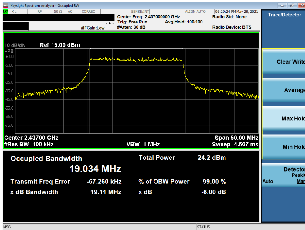
Plot 7-17. 6dB Bandwidth Plot SISO SOUTH (802.11ax 20MHz BW OFDMA – 242 Tones – Ch. 6)
