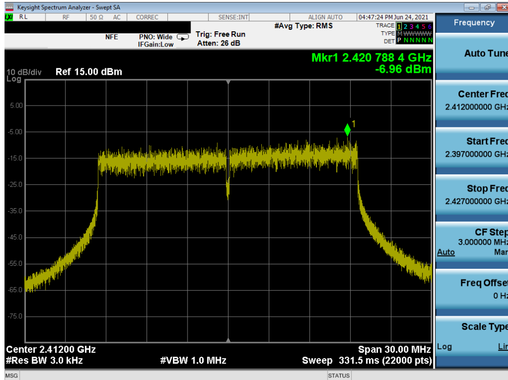
Plot 7-52. Power Spectral Density Plot MIMO SOUTH (802.11ax 20MHz BW OFDMA – 242 Tones – Ch. 1)
