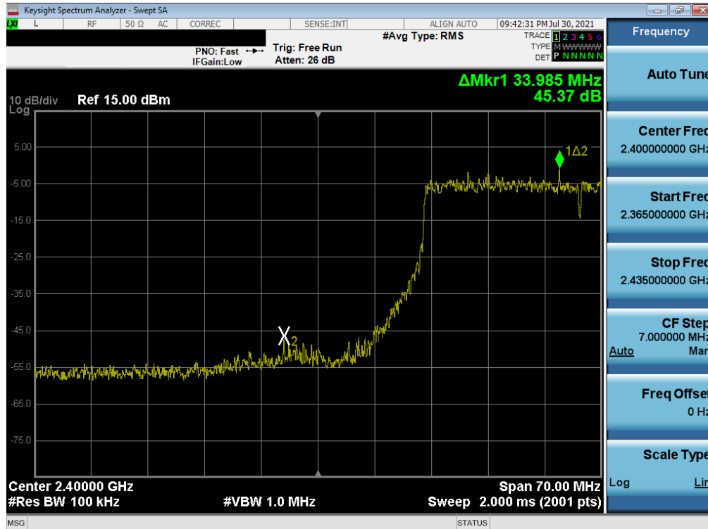
Plot 7-93. Band Edge Plot SISO SOUTH (802.11ax 40MHz BW OFDMA – 484 Tones – Ch. 5)
