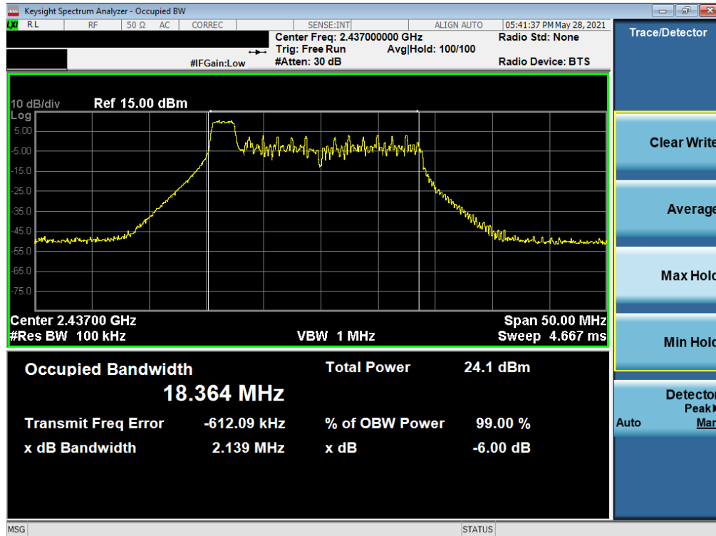
Plot 7-2. 6dB Bandwidth Plot SISO SOUTH (802.11ax 20MHz BW OFDMA – 26 Tones – Ch. 6)
