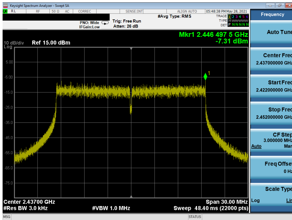
Plot 7-29. Power Spectral Density Plot SISO SOUTH (802.11ax 20MHz BW OFDMA – 242 Tones – Ch. 6)
