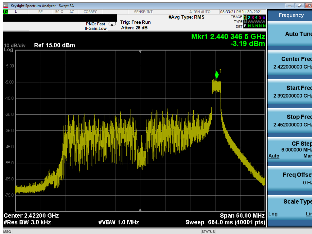
Plot 7-67. Power Spectral Density Plot MIMO NORTH (802.11ax 40MHz BW OFDMA – 26 Tones – Ch. 3)
