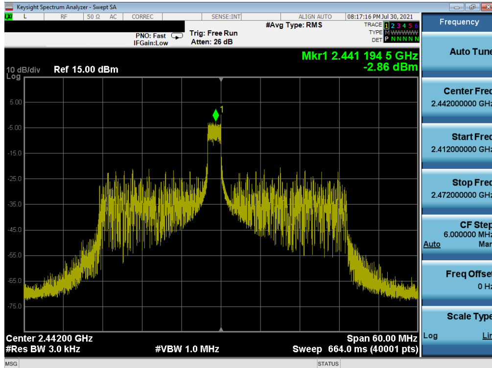
Plot 7-32. Power Spectral Density Plot SISO SOUTH (802.11ax 40MHz BW OFDMA – 26 Tones – Ch. 7)
