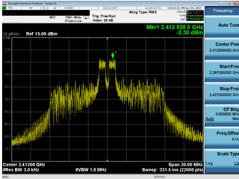
Plot 7-49. Power Spectral Density Plot MIMO SOUTH (802.11ax 20MHz BW OFDMA – 26 Tones – Ch. 1)
