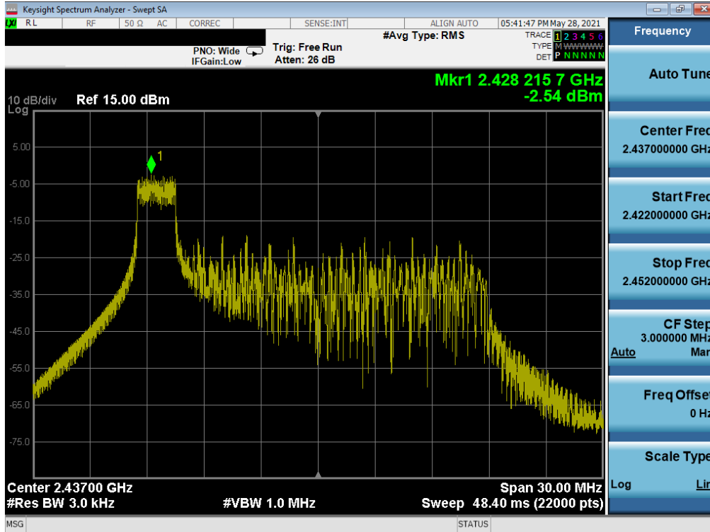
Plot 7-26. Power Spectral Density Plot SISO SOUTH (802.11ax 20MHz BW OFDMA – 26 Tones – Ch. 6)
