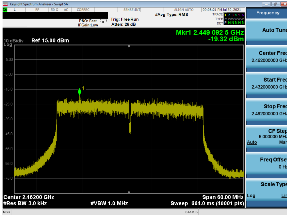
Plot 7-36. Power Spectral Density Plot SISO SOUTH (802.11ax 40MHz BW OFDMA – 484 Tones – Ch. 11)
