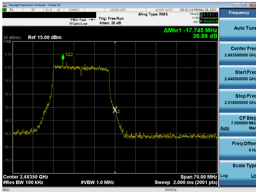
Plot 7-86. Band Edge Plot SISO SOUTH (802.11ax 20MHz BW OFDMA – 242 Tones – Ch. 13)
