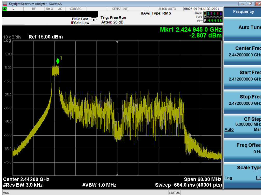
Plot 7-62. Power Spectral Density Plot MIMO SOUTH (802.11ax 40MHz BW OFDMA – 26 Tones – Ch. 7)
