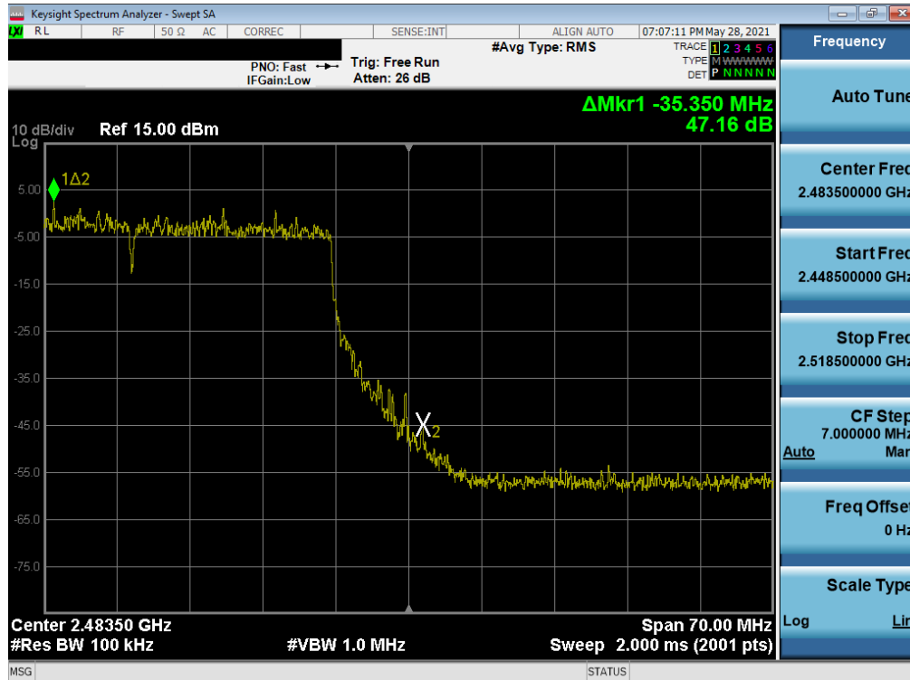
Plot 7-95. Band Edge Plot SISO SOUTH (802.11ax 40MHz BW OFDMA - 484 Tones - Ch. 10)
