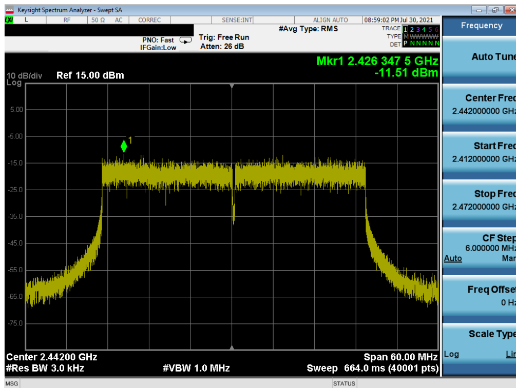
Plot 7-65. Power Spectral Density Plot MIMO SOUTH (802.11ax 40MHz BW OFDMA – 242 Tones – Ch. 7)
