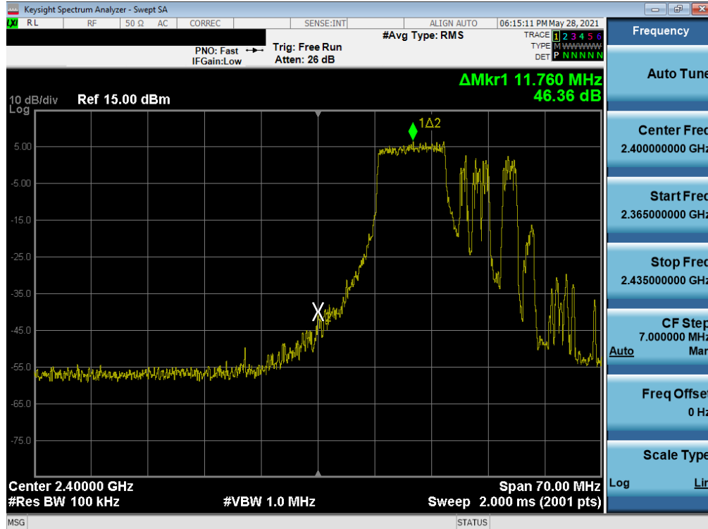
Plot 7-74. Band Edge Plot SISO SOUTH (802.11ax 20MHz BW OFDMA – 106 Tones – Ch. 2)
