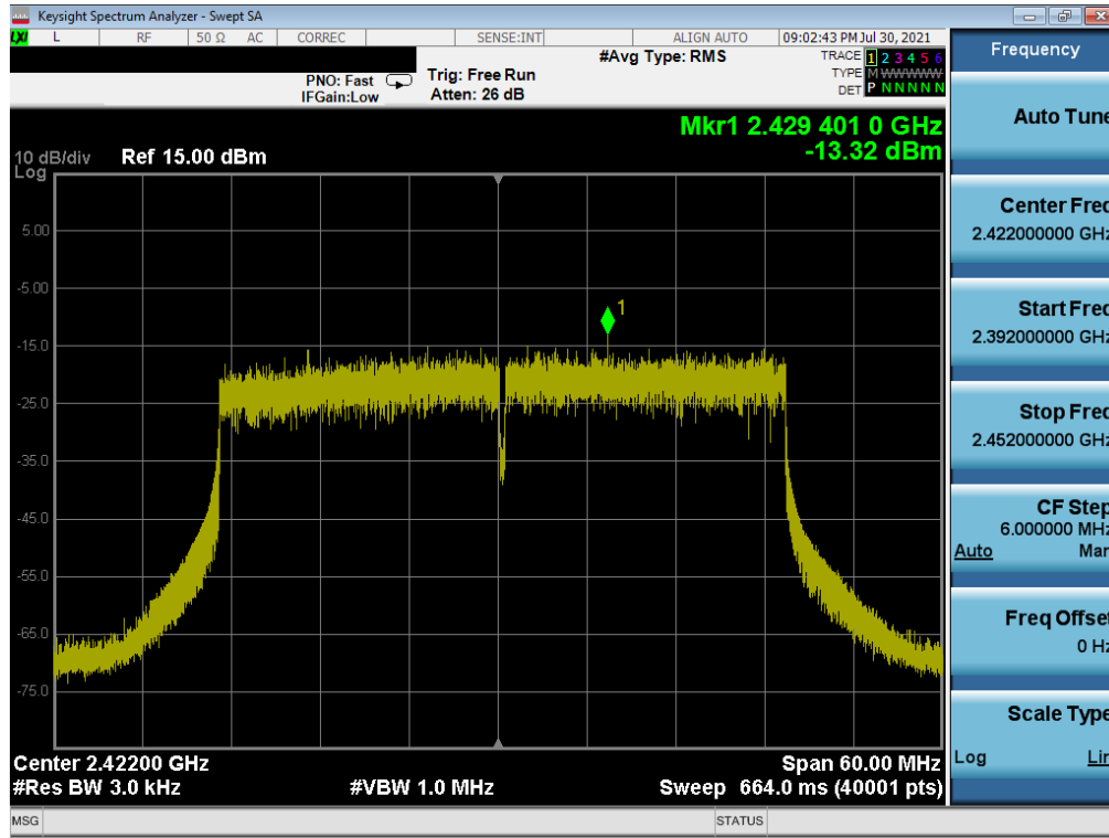
Plot 7-34. Power Spectral Density Plot SISO SOUTH (802.11ax 40MHz BW OFDMA – 484 Tones – Ch. 3)
