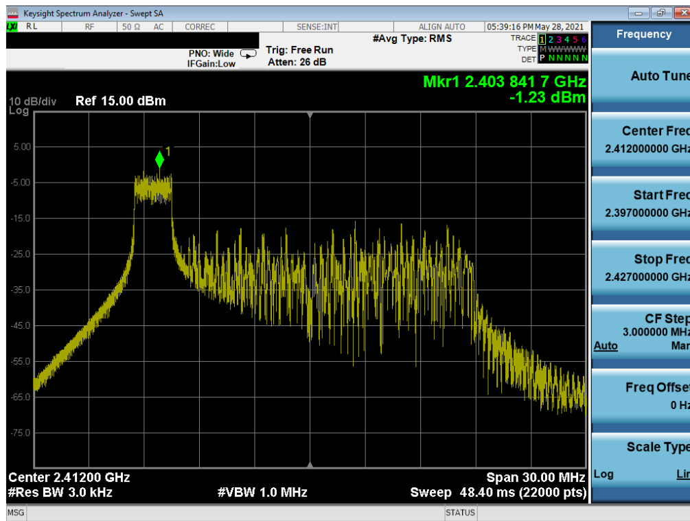
Plot 7-25. Power Spectral Density Plot SISO SOUTH (802.11ax 20MHz BW OFDMA – 26 Tones – Ch. 1)
