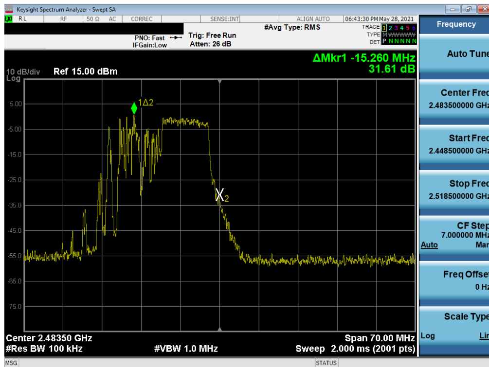
Plot 7-102. Band Edge Plot SISO NORTH (802.11ax 20MHz BW OFDMA – 106 Tones – Ch. 13)
