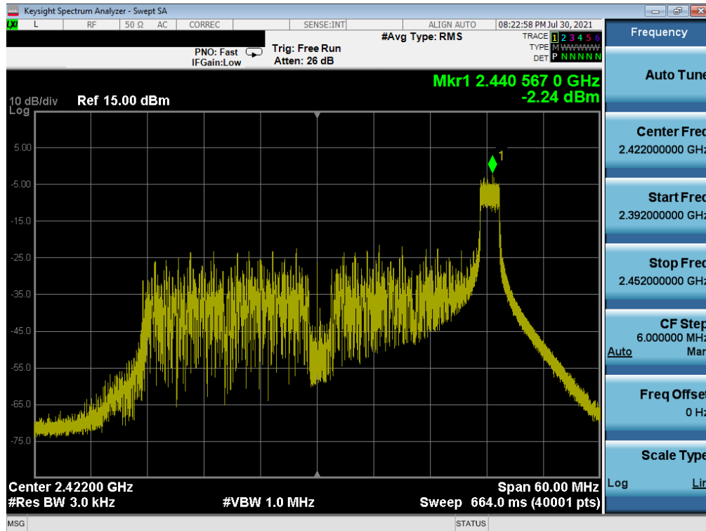
Plot 7-61. Power Spectral Density Plot MIMO SOUTH (802.11ax 40MHz BW OFDMA – 26 Tones – Ch. 3)
