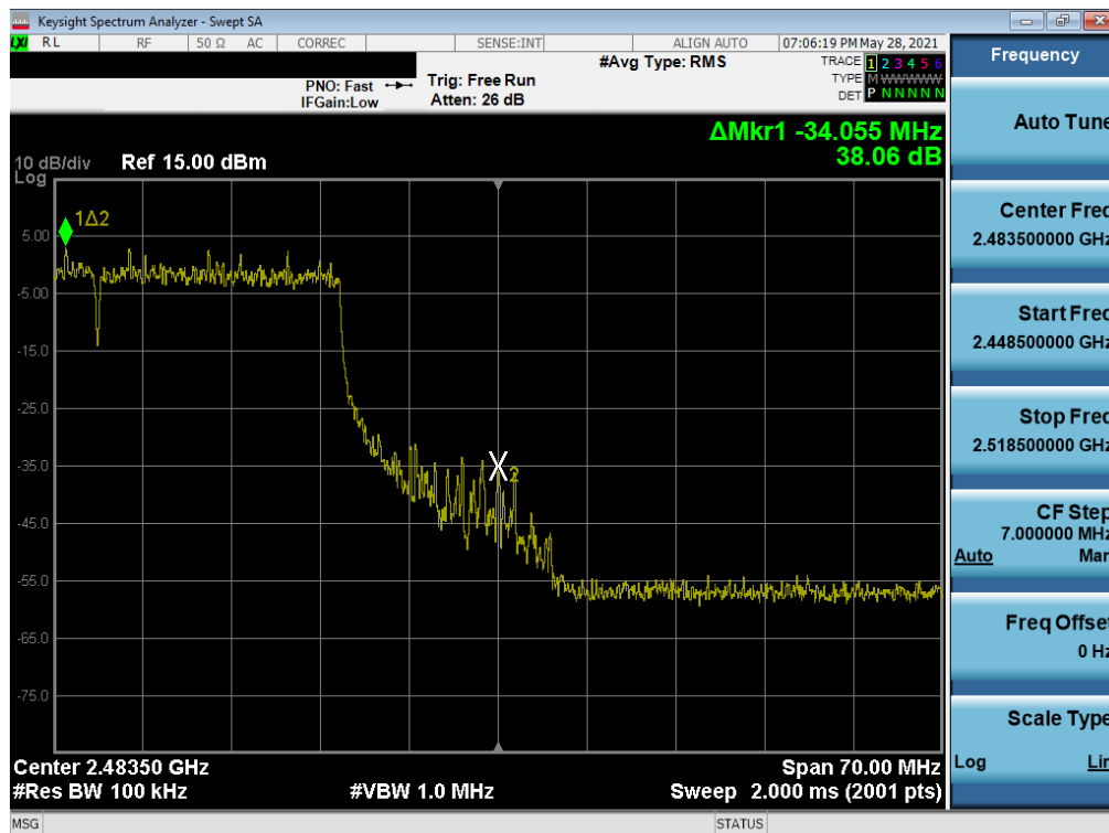
Plot 7-94. Band Edge Plot SISO SOUTH (802.11ax 40MHz BW OFDMA – 484 Tones – Ch. 9)
