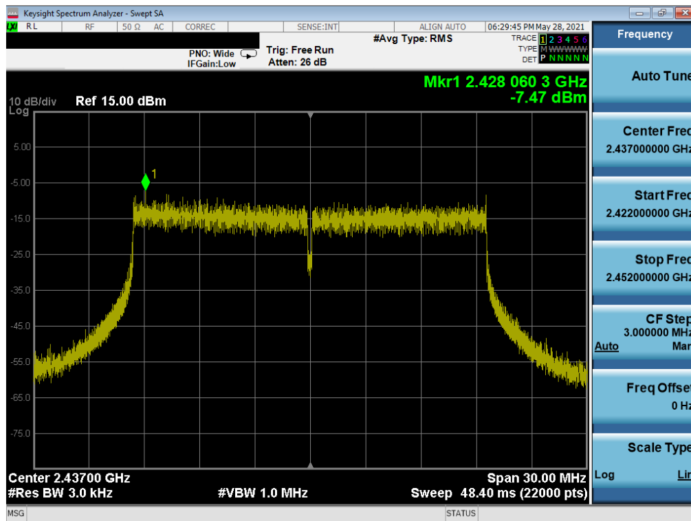
Plot 7-41. Power Spectral Density Plot SISO NORTH (802.11ax 20MHz BW OFDMA – 242 Tones – Ch. 6)
