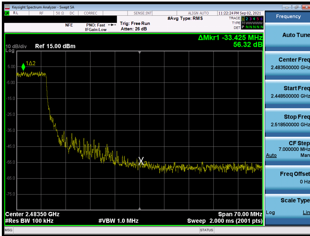
Plot 7-81. Band Edge Plot SISO SOUTH (802.11ax 20MHz BW OFDMA – 242 Tones – Ch. 8)
