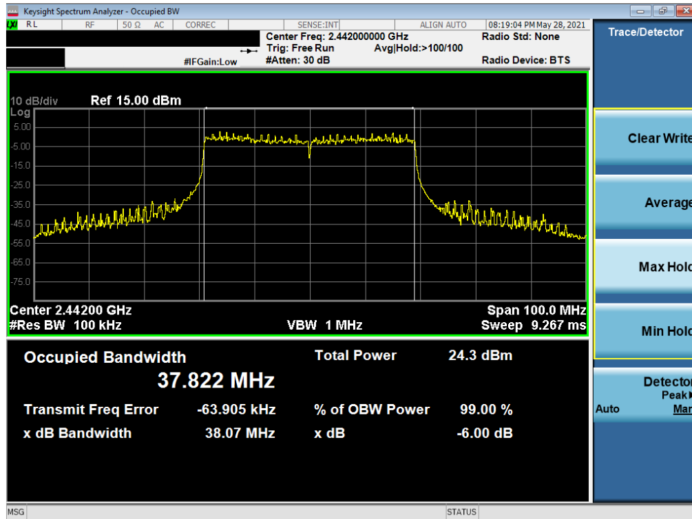
Plot 7-23. 6dB Bandwidth Plot SISO SOUTH (802.11ax 40MHz BW OFDMA – 484 Tones – Ch. 7)
