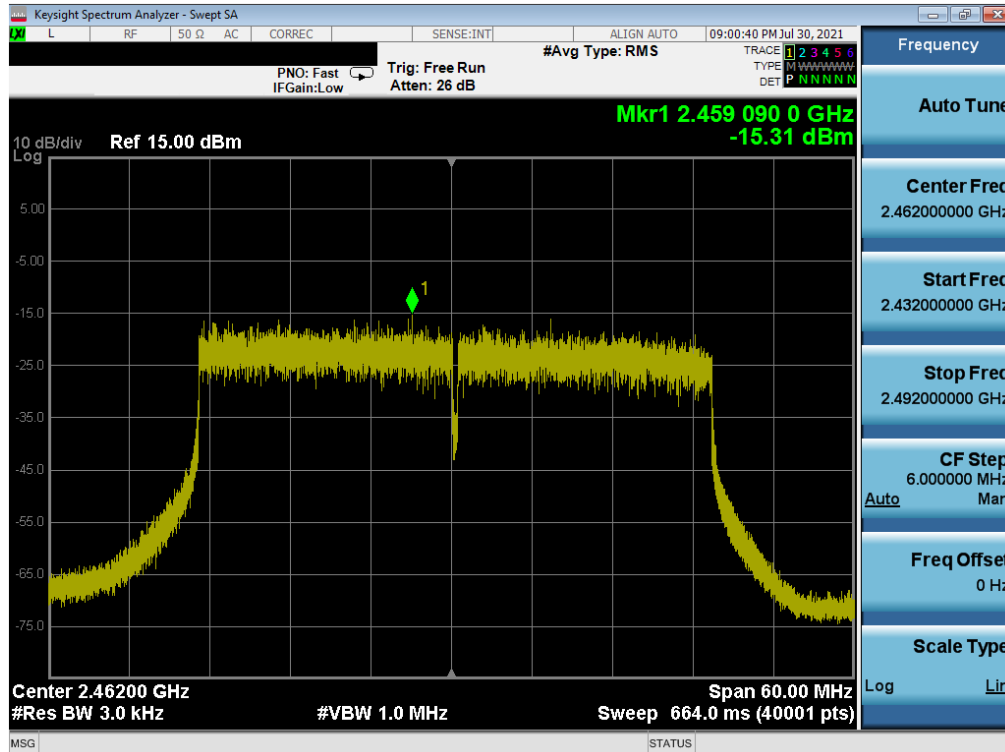
Plot 7-66. Power Spectral Density Plot MIMO SOUTH (802.11ax 40MHz BW OFDMA – 242 Tones – Ch. 11)
