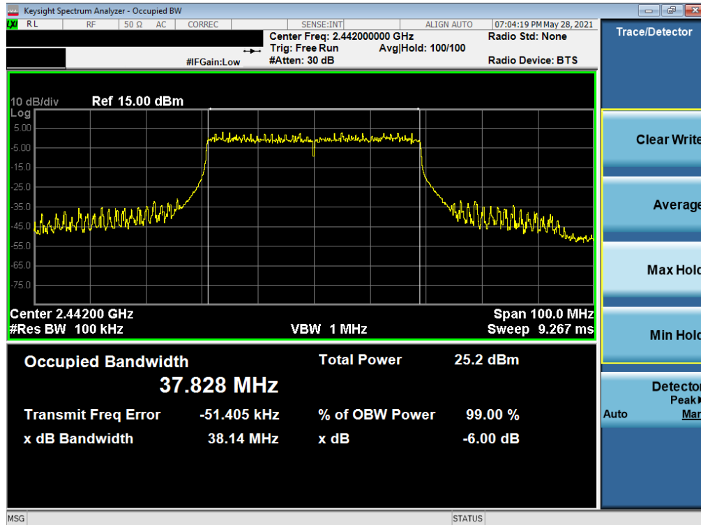
Plot 7-11. 6dB Bandwidth Plot SISO SOUTH (802.11ax 40MHz BW OFDMA – 484 Tones – Ch. 7)
