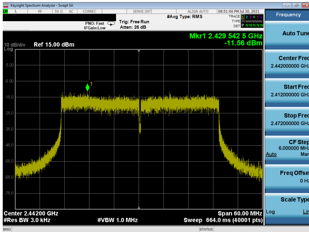
Plot 7-71. Power Spectral Density Plot MIMO NORTH (802.11ax 40MHz BW OFDMA – 484 Tones – Ch. 7)
