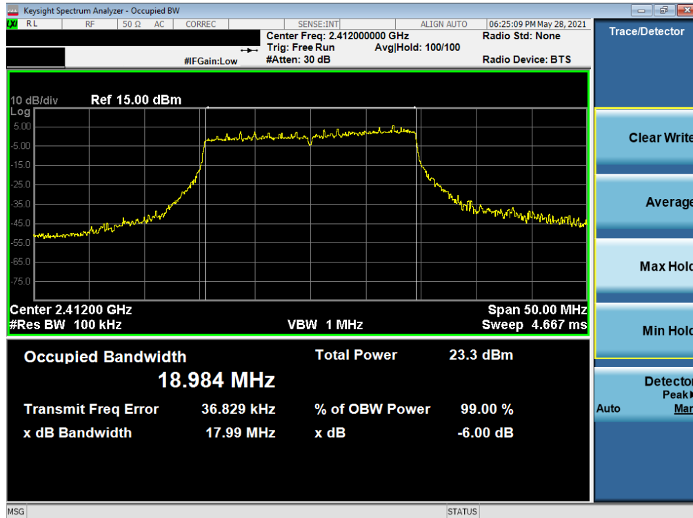
Plot 7-16. 6dB Bandwidth Plot SISO SOUTH (802.11ax 20MHz BW OFDMA – 242 Tones – Ch. 1)
