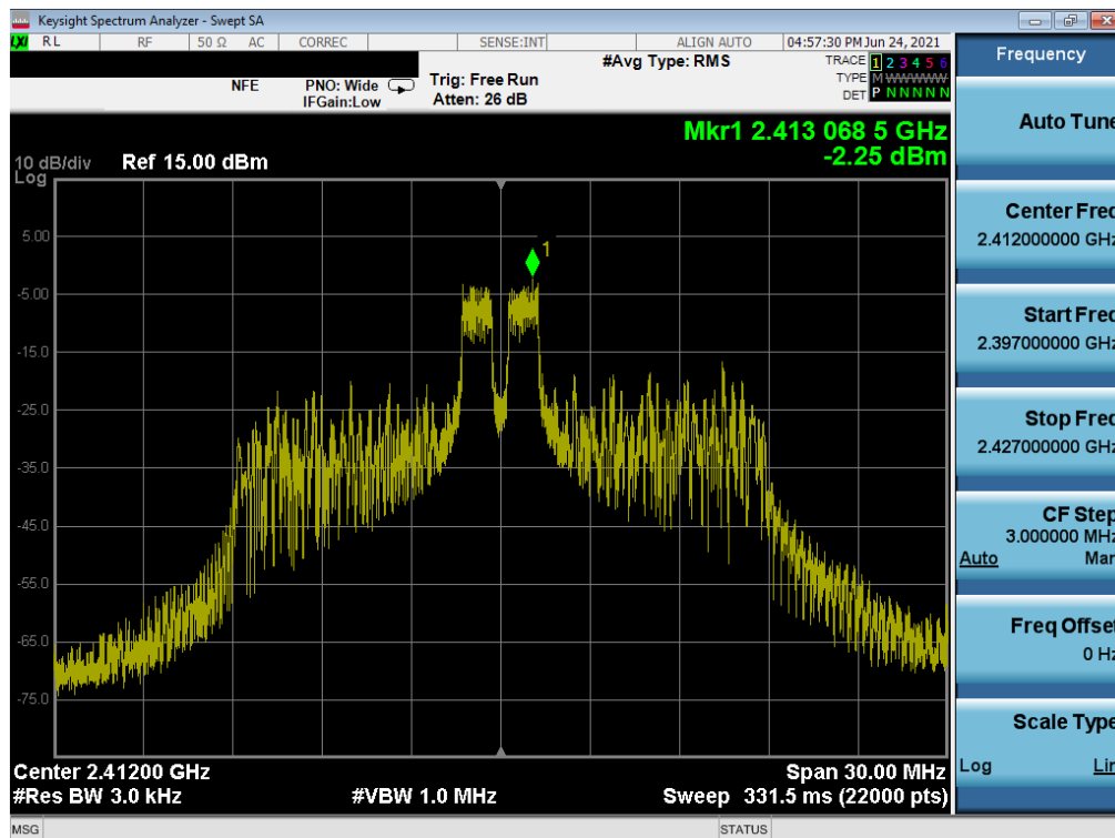
Plot 7-55. Power Spectral Density Plot MIMO NORTH (802.11ax 20MHz BW OFDMA – 26 Tones – Ch. 1)
