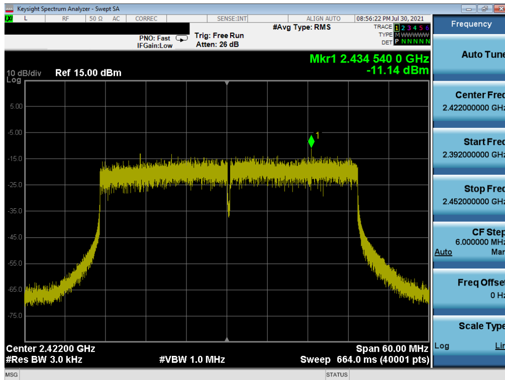
Plot 7-64. Power Spectral Density Plot MIMO SOUTH (802.11ax 40MHz BW OFDMA – 484 Tones – Ch. 3)
