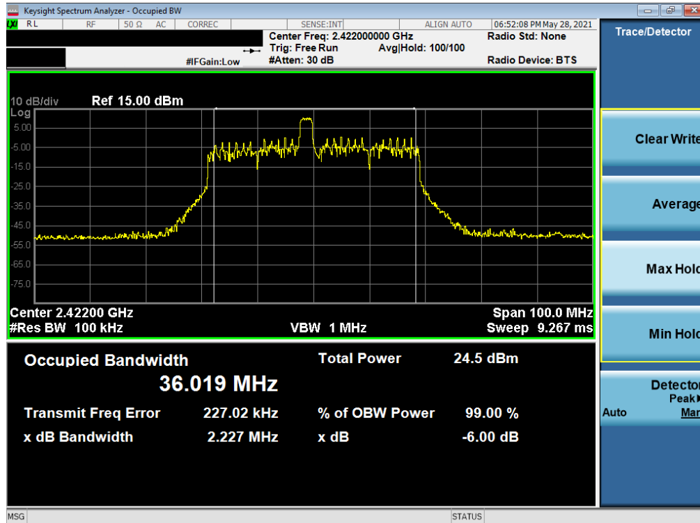
Plot 7-7. 6dB Bandwidth Plot SISO SOUTH (802.11ax 40MHz BW OFDMA – 26 Tones – Ch. 3)
