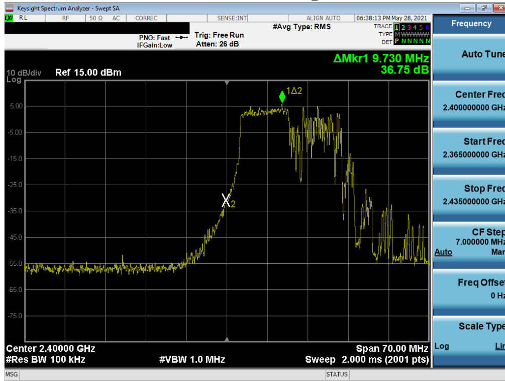
Plot 7-97. Band Edge Plot SISO NORTH (802.11ax 20MHz BW OFDMA – 106 Tones – Ch. 1)
