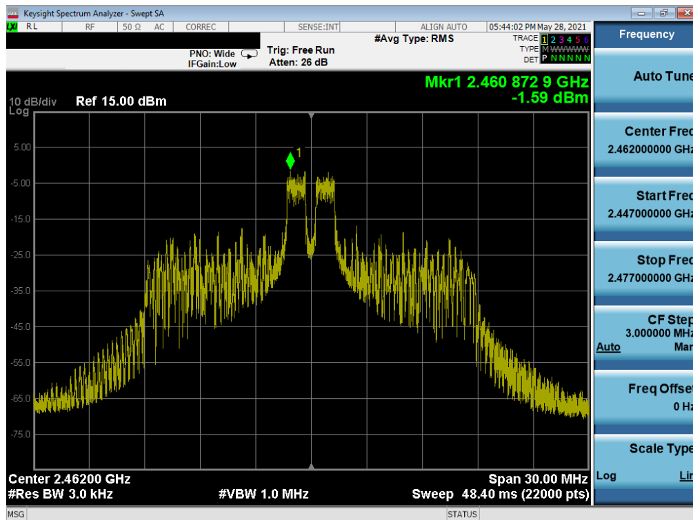
Plot 7-27. Power Spectral Density Plot SISO SOUTH (802.11ax 20MHz BW OFDMA – 26 Tones – Ch. 11)
