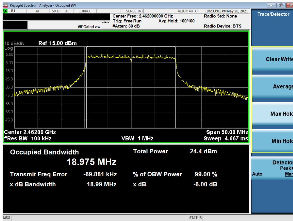
Plot 7-18. 6dB Bandwidth Plot SISO SOUTH (802.11ax 20MHz BW OFDMA – 242 Tones – Ch. 11)
