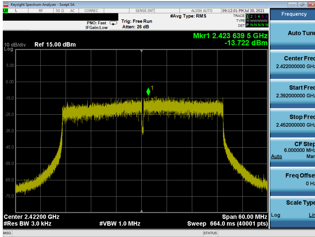
Plot 7-46. Power Spectral Density Plot SISO NORTH (802.11ax 40MHz BW OFDMA – 484 Tones – Ch. 3)
