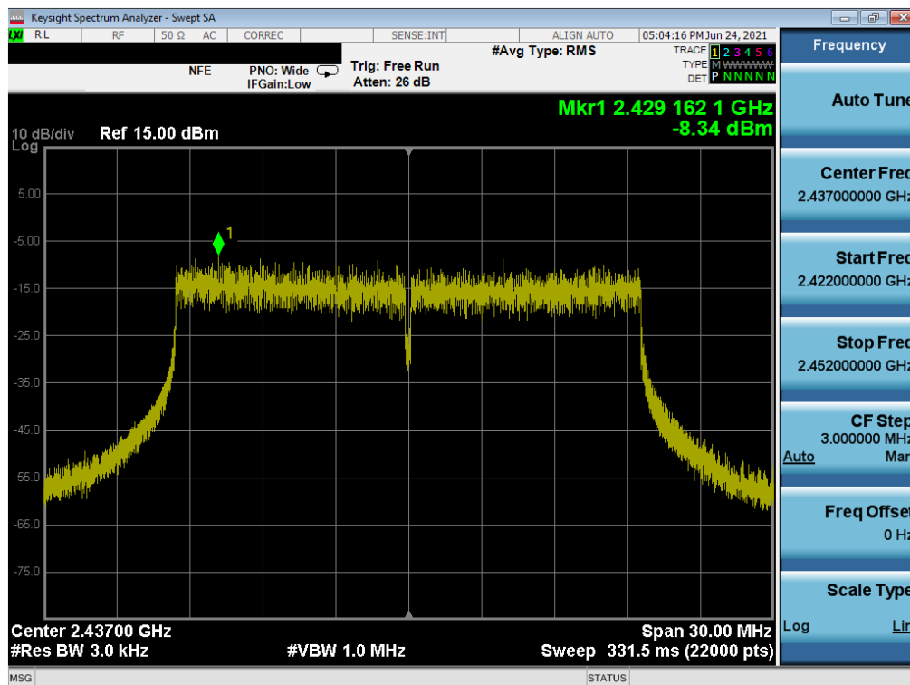
Plot 7-59. Power Spectral Density Plot MIMO NORTH (802.11ax 20MHz BW OFDMA – 484 Tones – Ch. 6)
