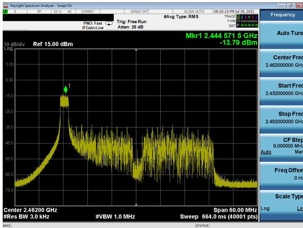
Plot 7-33. Power Spectral Density Plot SISO SOUTH (802.11ax 40MHz BW OFDMA – 26 Tones – Ch. 11)
