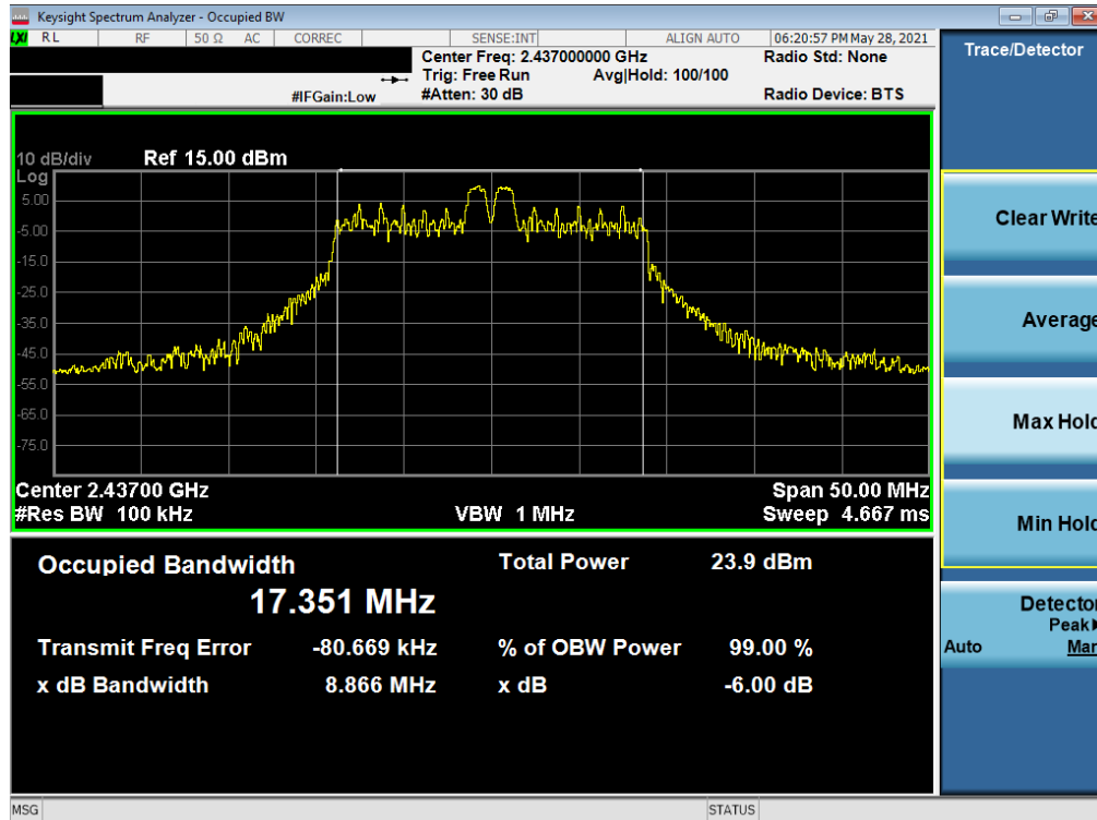
Plot 7-14. 6dB Bandwidth Plot SISO SOUTH (802.11ax 20MHz BW OFDMA – 26 Tones – Ch. 6)
