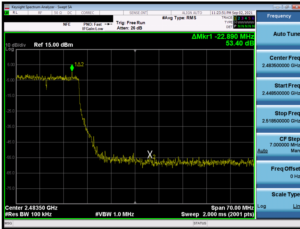
Plot 7-83. Band Edge Plot SISO SOUTH (802.11ax 20MHz BW OFDMA - 242 Tones - Ch. 10)
