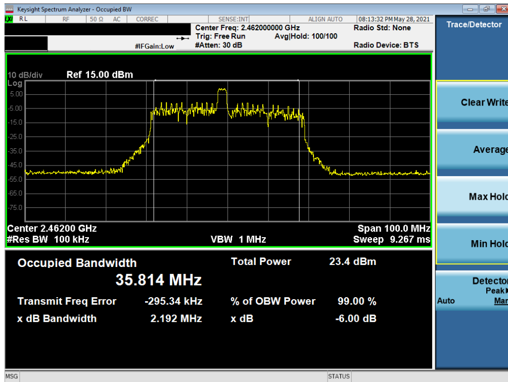
Plot 7-21. 6dB Bandwidth Plot SISO SOUTH (802.11ax 40MHz BW OFDMA – 26 Tones – Ch. 11)
