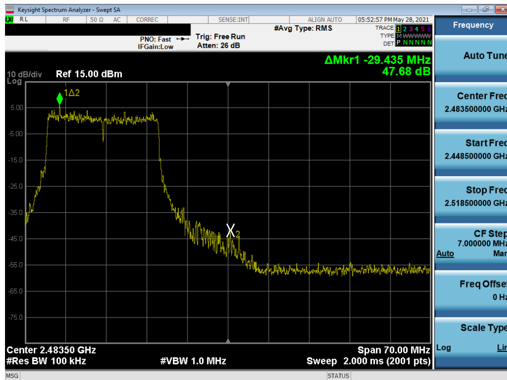
Plot 7-84. Band Edge Plot SISO SOUTH (802.11ax 20MHz BW OFDMA - 242 Tones - Ch. 11)
