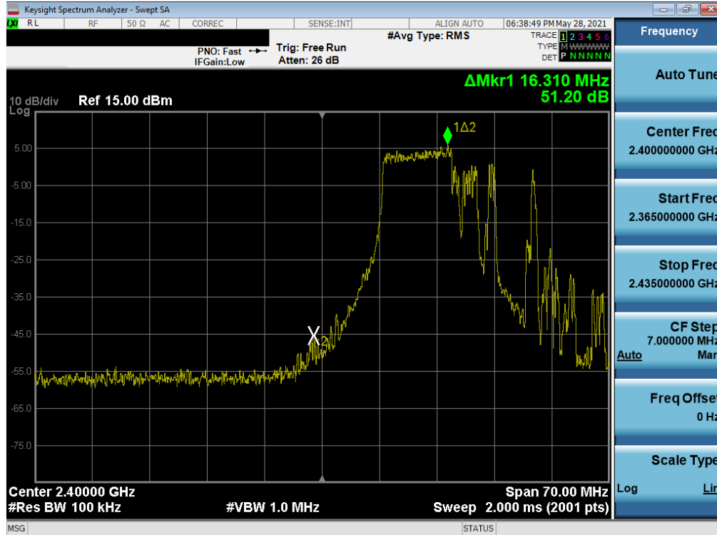
Plot 7-98. Band Edge Plot SISO NORTH (802.11ax 20MHz BW OFDMA – 106 Tones – Ch. 2)
