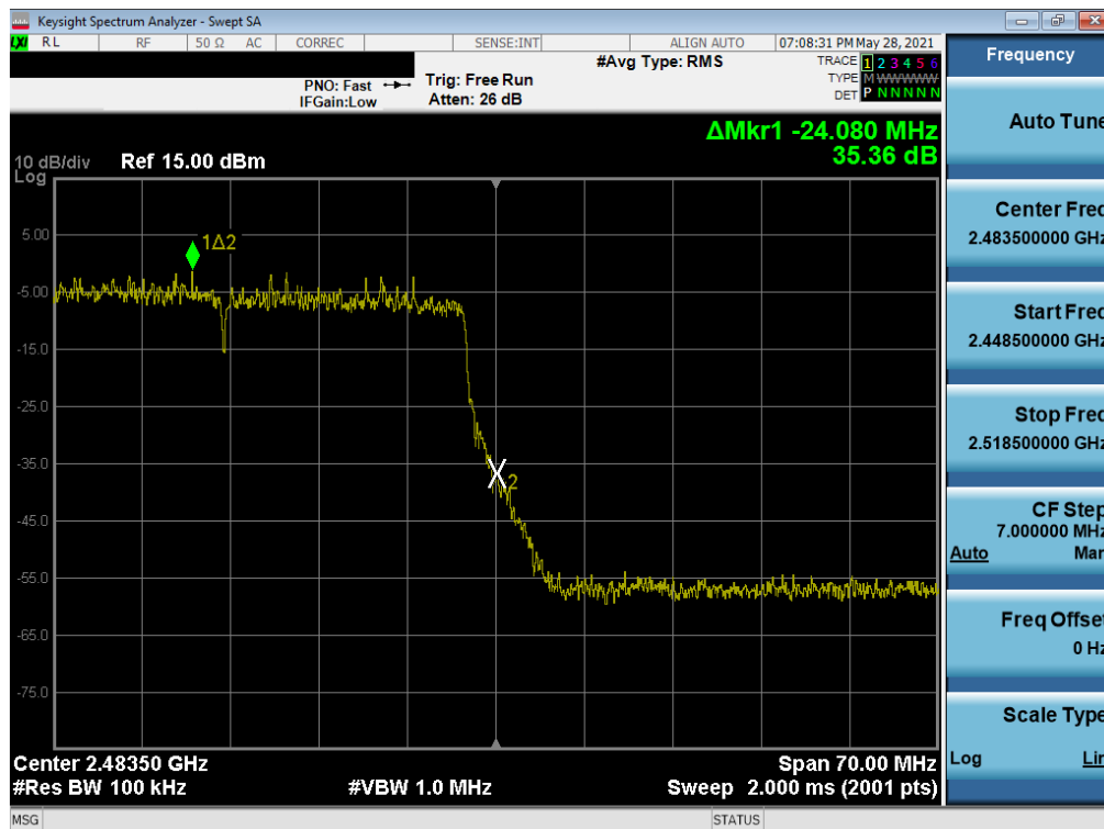
Plot 7-96. Band Edge Plot SISO SOUTH (802.11ax 40MHz BW OFDMA - 484 Tones - Ch. 11)
