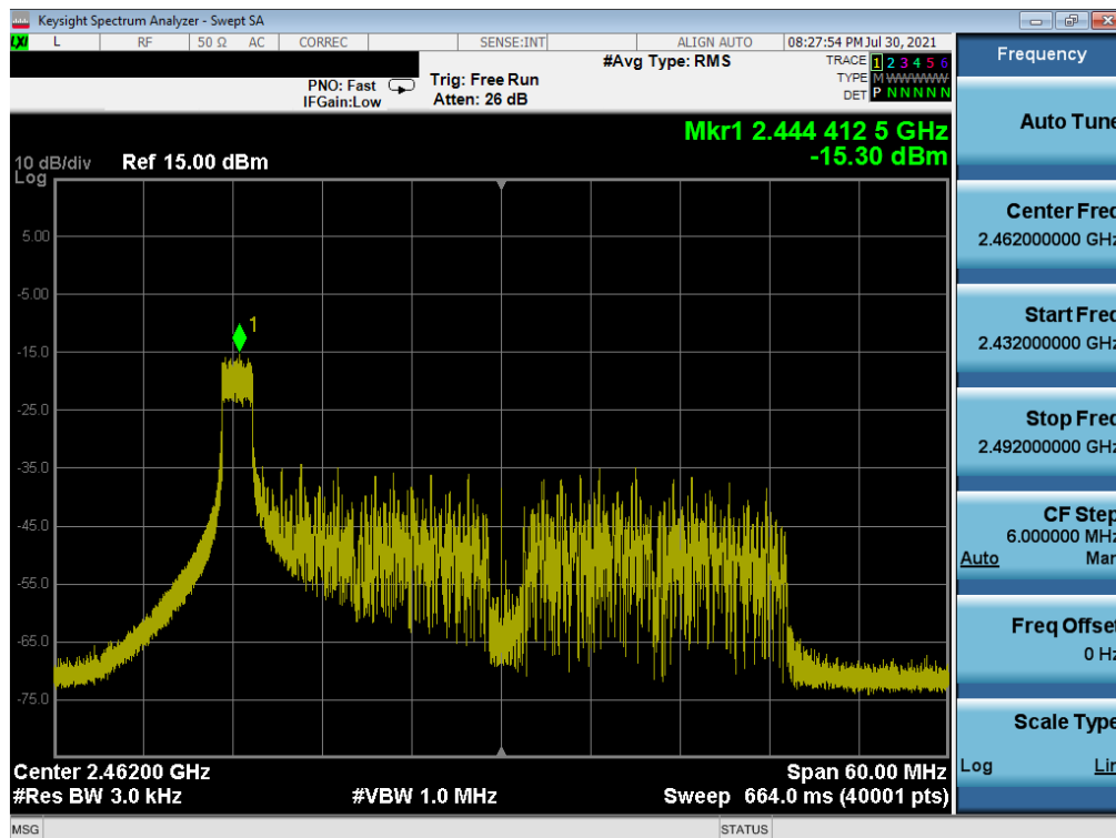
Plot 7-63. Power Spectral Density Plot MIMO SOUTH (802.11ax 40MHz BW OFDMA – 26 Tones – Ch. 11)
