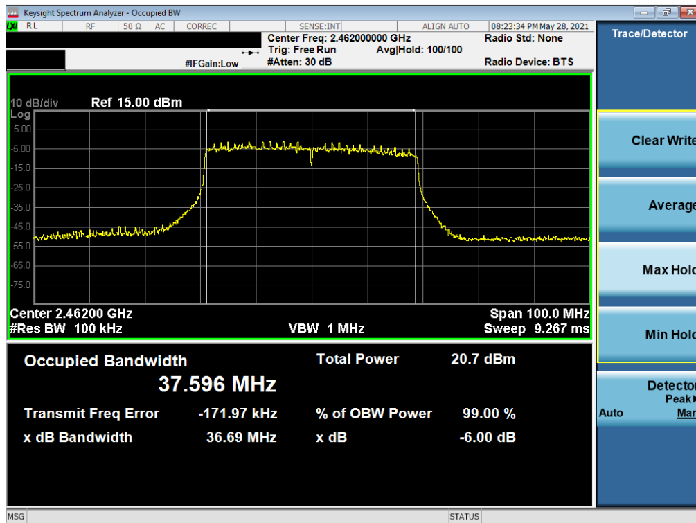
Plot 7-24. 6dB Bandwidth Plot SISO SOUTH (802.11ax 40MHz BW OFDMA – 484 Tones – Ch. 11)
