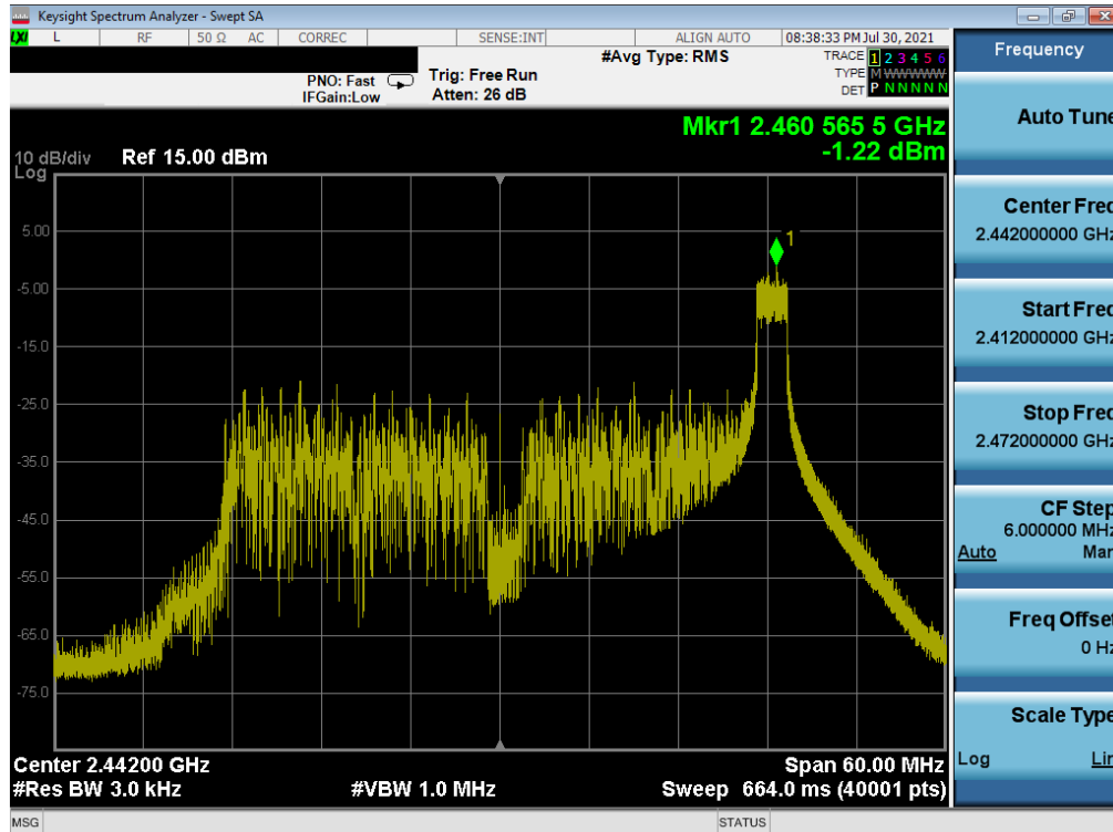
Plot 7-44. Power Spectral Density Plot SISO NORTH (802.11ax 40MHz BW OFDMA – 26 Tones – Ch. 7)
