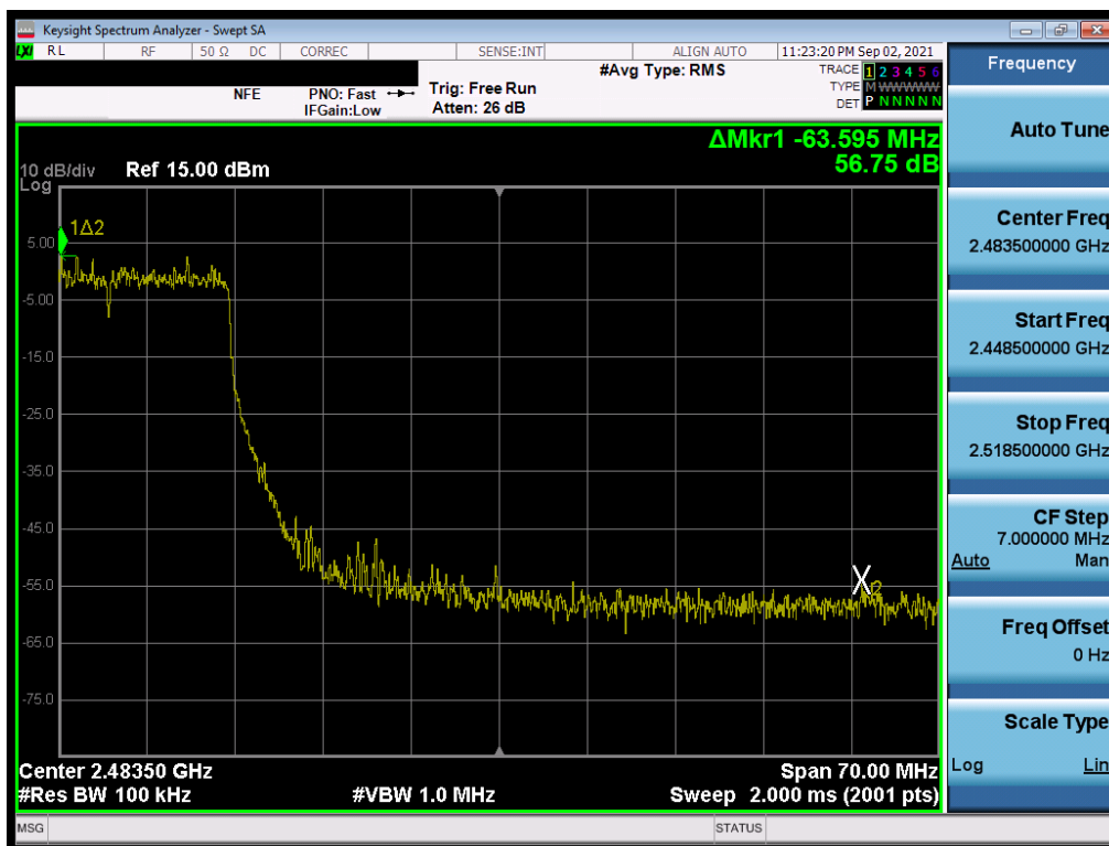
Plot 7-82. Band Edge Plot SISO SOUTH (802.11ax 20MHz BW OFDMA – 242 Tones – Ch. 9)
