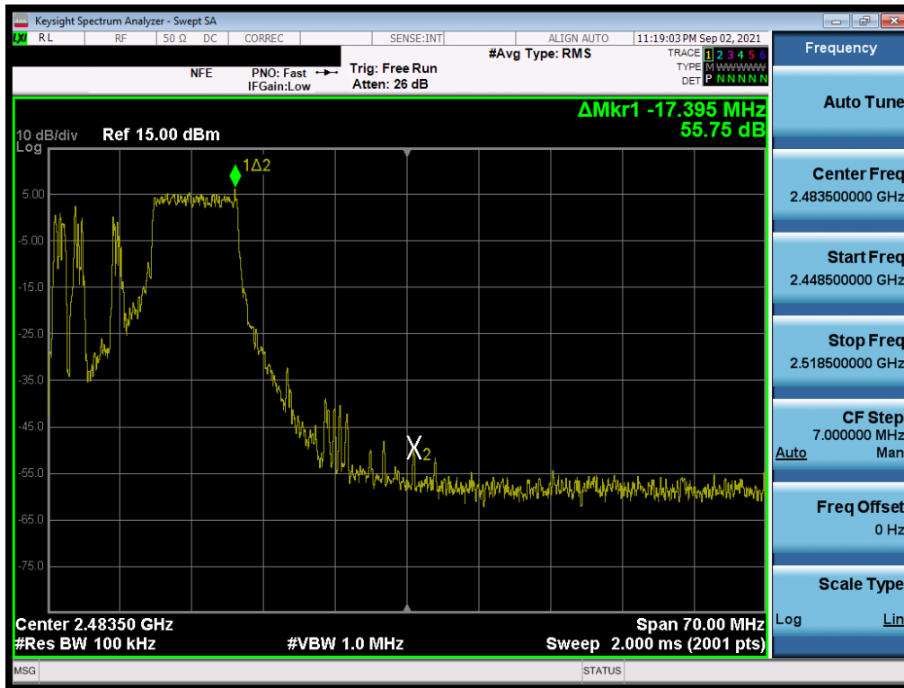
Plot 7-75. Band Edge Plot SISO SOUTH (802.11ax 20MHz BW OFDMA - 106 Tones - Ch. 10)
