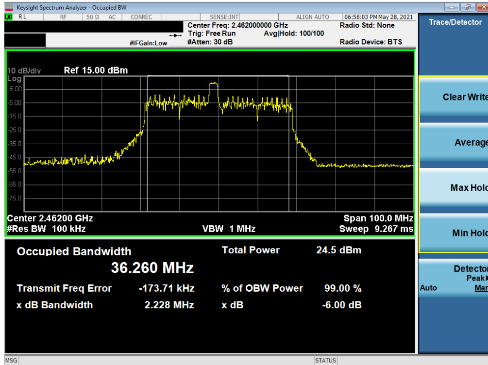
Plot 7-9. 6dB Bandwidth Plot SISO SOUTH (802.11ax 40MHz BW OFDMA – 26 Tones – Ch. 11)
