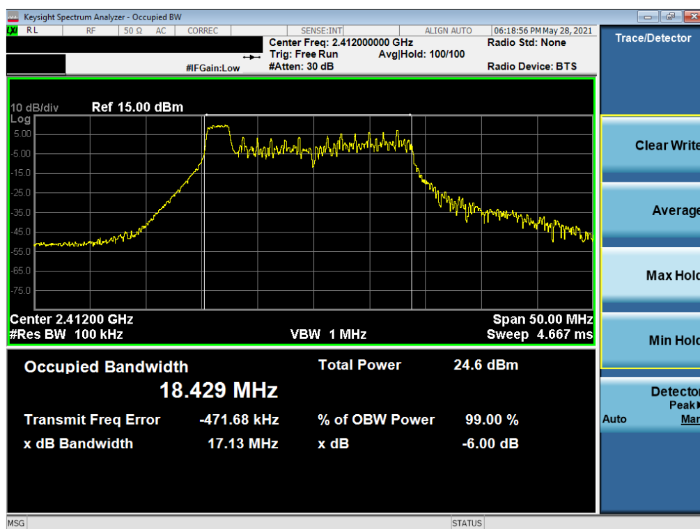
Plot 7-13. 6dB Bandwidth Plot SISO SOUTH (802.11ax 20MHz BW OFDMA – 26 Tones – Ch. 1)
