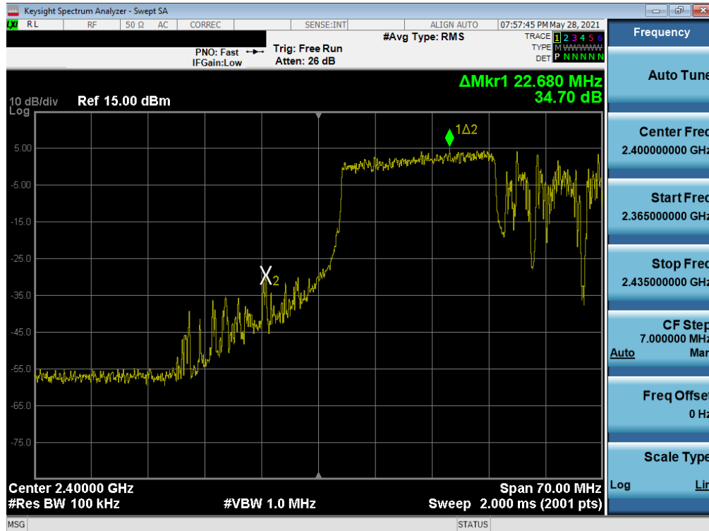
Plot 7-87. Band Edge Plot SISO SOUTH (802.11ax 40MHz BW OFDMA – 242 Tones – Ch. 3)
