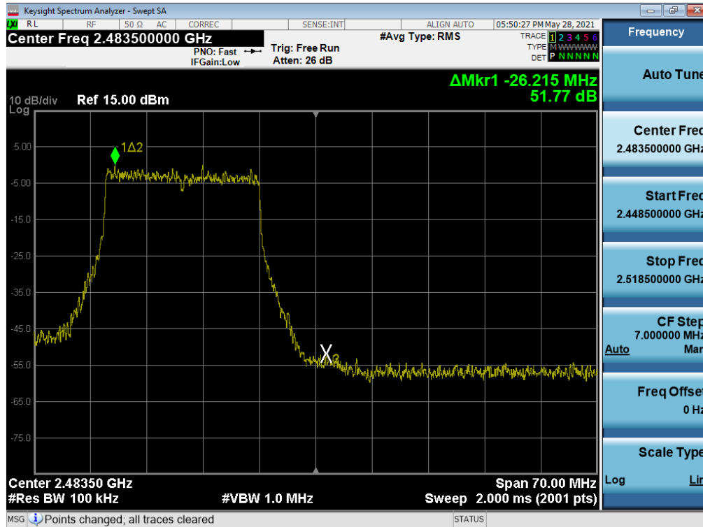
Plot 7-85. Band Edge Plot SISO SOUTH (802.11ax 20MHz BW OFDMA – 242 Tones – Ch. 12)
