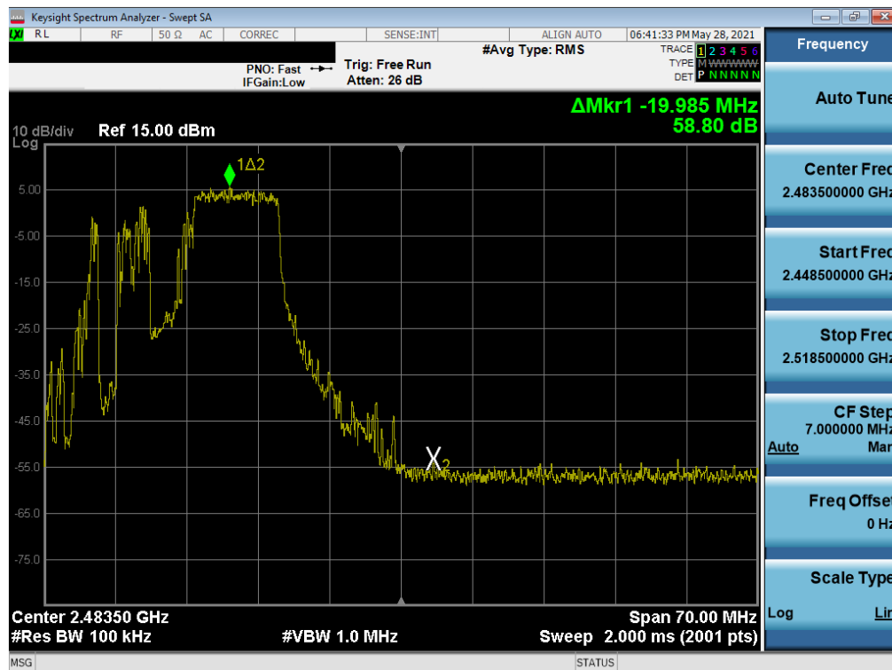
Plot 7-100. Band Edge Plot SISO NORTH (802.11ax 20MHz BW OFDMA – 106 Tones – Ch. 11)
