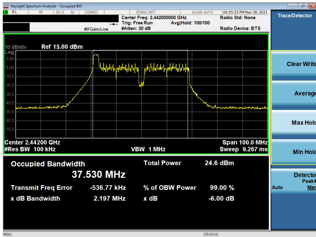
Plot 7-8. 6dB Bandwidth Plot SISO SOUTH (802.11ax 40MHz BW OFDMA – 26 Tones – Ch. 7)
