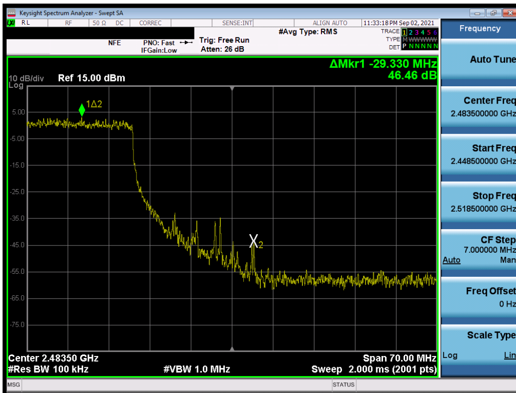
Plot 7-88. Band Edge Plot SISO SOUTH (802.11ax 40MHz BW OFDMA – 242 Tones – Ch. 8)
