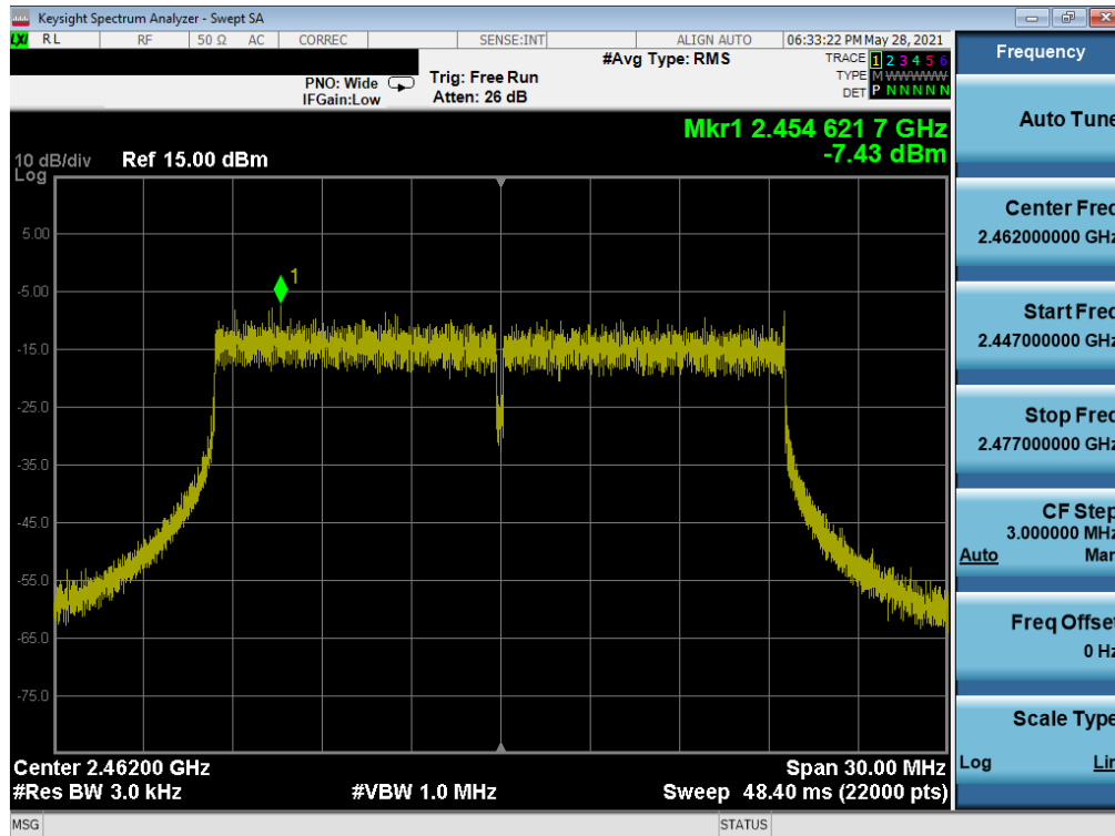
Plot 7-42. Power Spectral Density Plot SISO NORTH (802.11ax 20MHz BW OFDMA – 242 Tones – Ch. 11)
