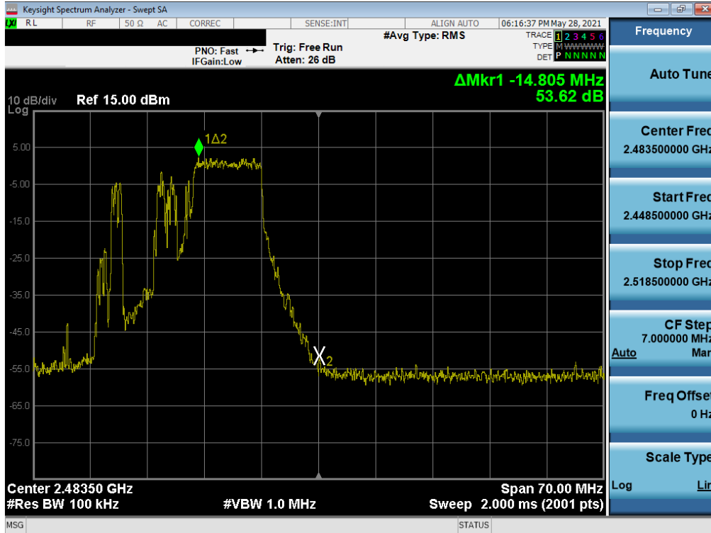
Plot 7-77. Band Edge Plot SISO SOUTH (802.11ax 20MHz BW OFDMA – 106 Tones – Ch. 12)
