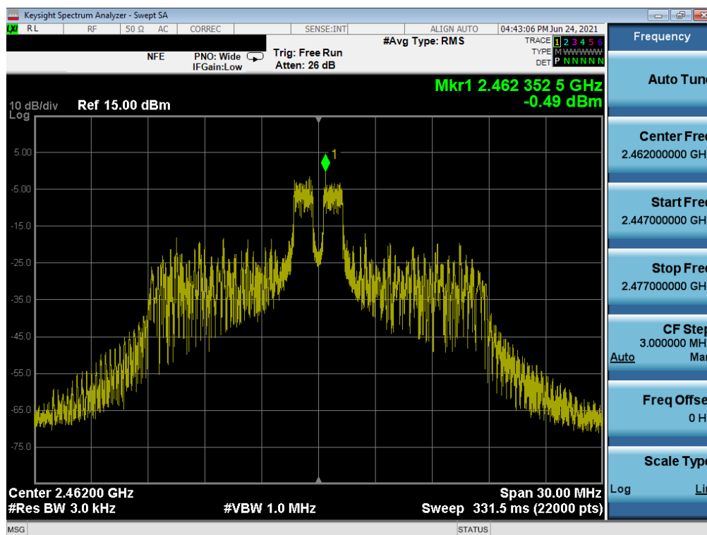
Plot 7-51. Power Spectral Density Plot MIMO SOUTH (802.11ax 20MHz BW OFDMA – 26 Tones – Ch. 11)
