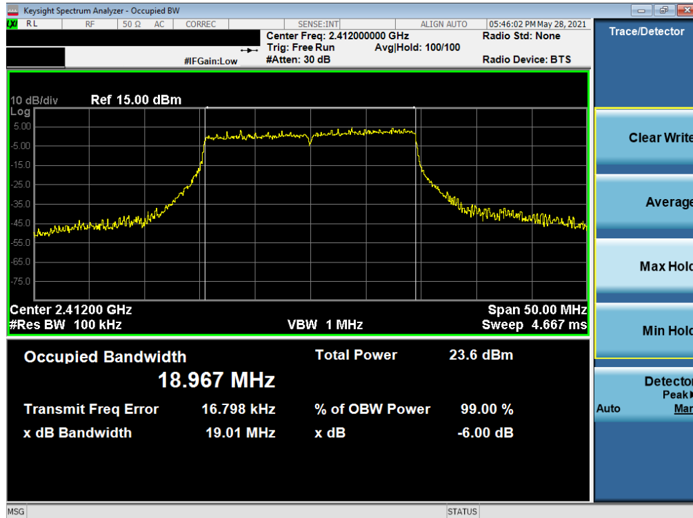
Plot 7-4. 6dB Bandwidth Plot SISO SOUTH (802.11ax 20MHz BW OFDMA – 242 Tones – Ch. 1)
