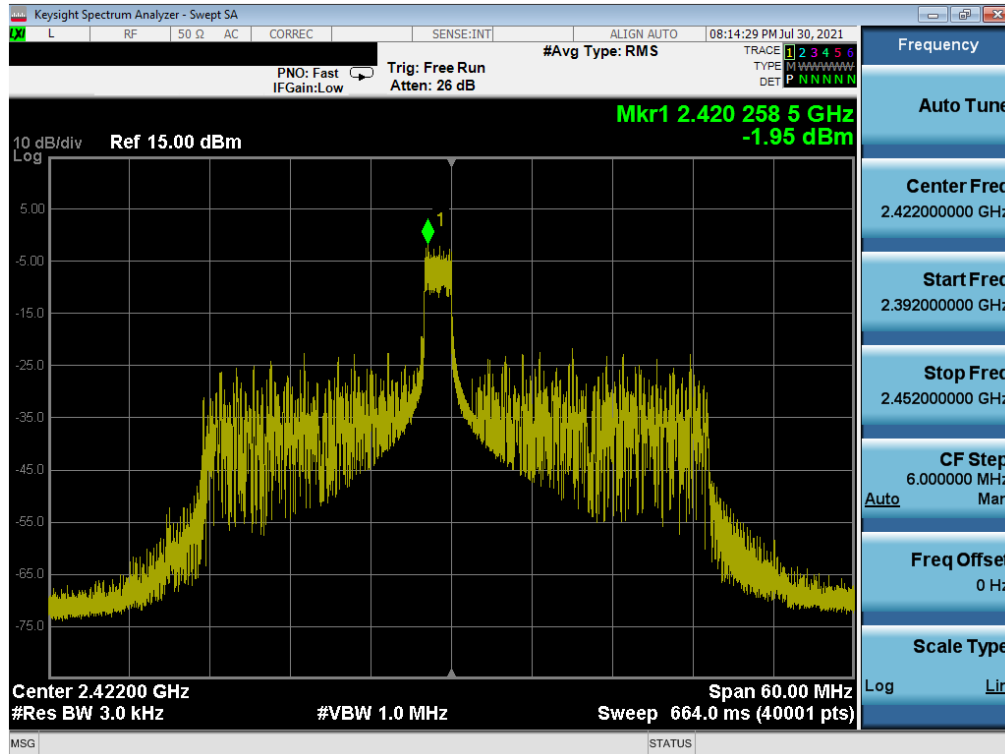
Plot 7-31. Power Spectral Density Plot SISO SOUTH (802.11ax 40MHz BW OFDMA – 26 Tones – Ch. 3)
