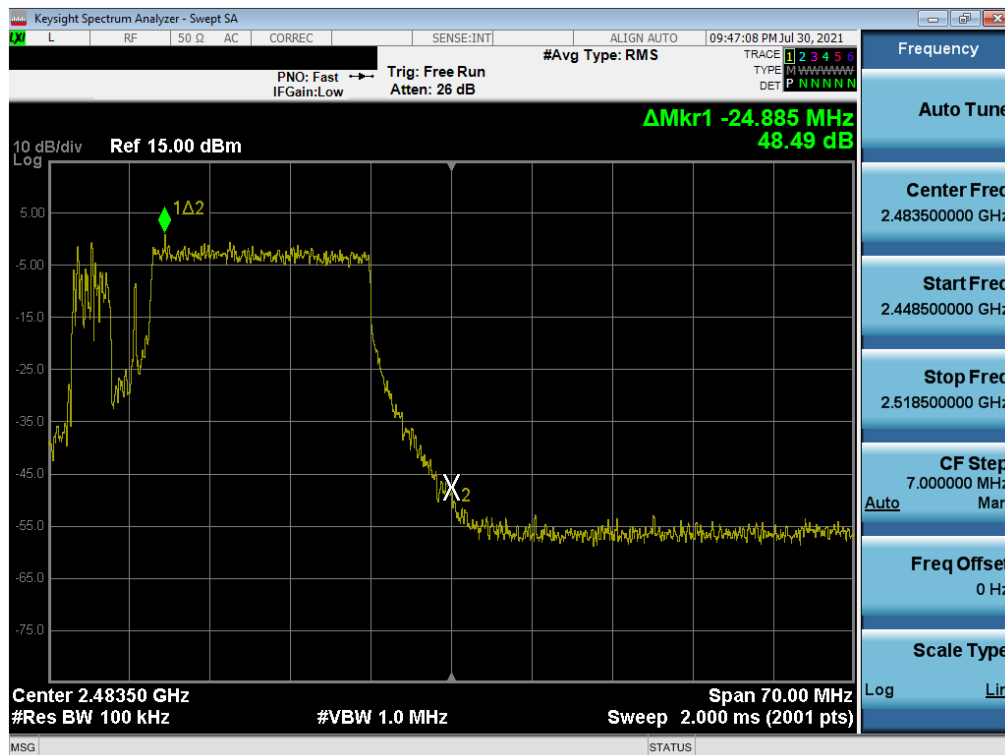
Plot 7-90. Band Edge Plot SISO SOUTH (802.11ax 40MHz BW OFDMA – 242 Tones – Ch. 10)
