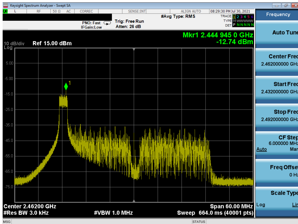
Plot 7-69. Power Spectral Density Plot MIMO NORTH (802.11ax 40MHz BW OFDMA – 26 Tones – Ch. 11)
