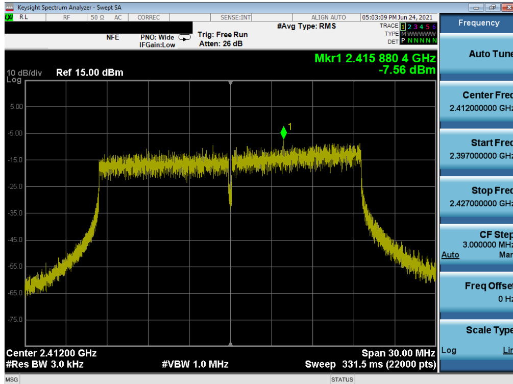
Plot 7-58. Power Spectral Density Plot MIMO NORTH (802.11ax 20MHz BW OFDMA – 484 Tones – Ch. 1)
