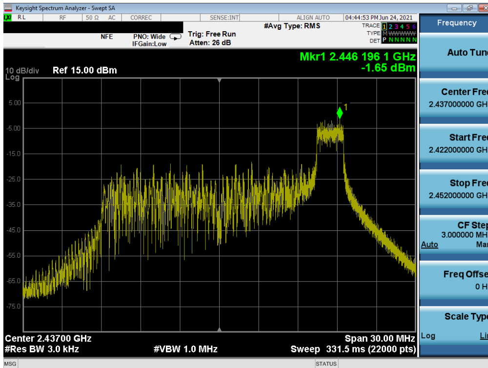
Plot 7-50. Power Spectral Density Plot MIMO SOUTH (802.11ax 20MHz BW OFDMA – 26 Tones – Ch. 6)
