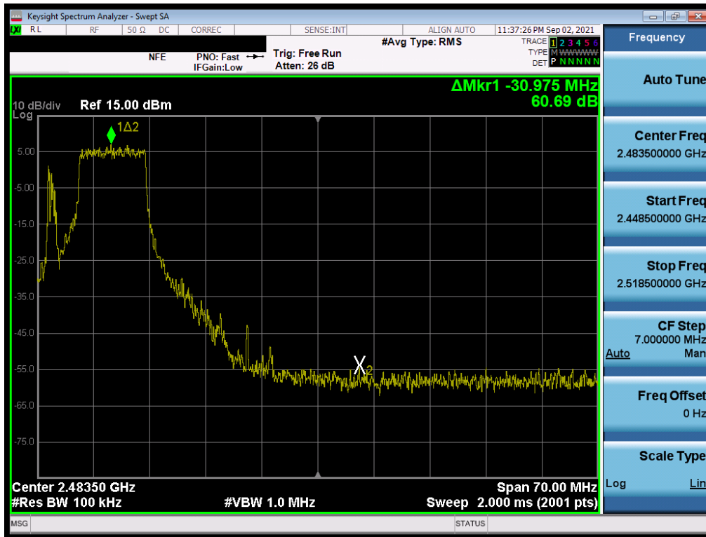
Plot 7-99. Band Edge Plot SISO NORTH (802.11ax 20MHz BW OFDMA – 106 Tones – Ch. 10)
