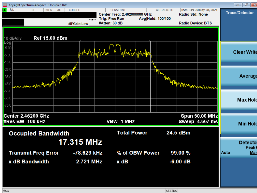
Plot 7-3. 6dB Bandwidth Plot SISO SOUTH (802.11ax 20MHz BW OFDMA – 26 Tones – Ch. 11)
