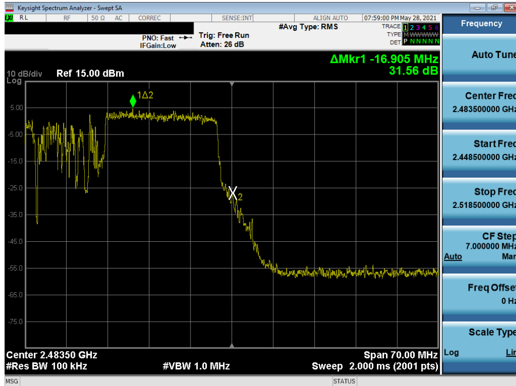
Plot 7-91. Band Edge Plot SISO SOUTH (802.11ax 40MHz BW OFDMA – 242 Tones – Ch. 11)
