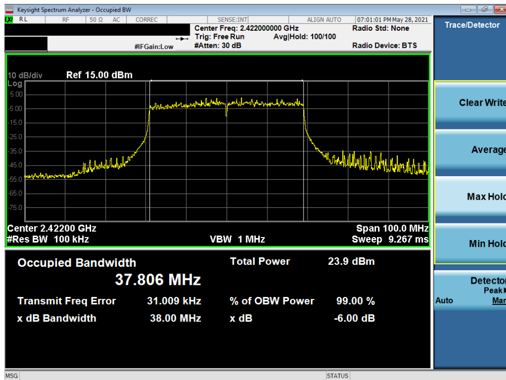
Plot 7-10. 6dB Bandwidth Plot SISO SOUTH (802.11ax 40MHz BW OFDMA – 484 Tones – Ch. 3)
