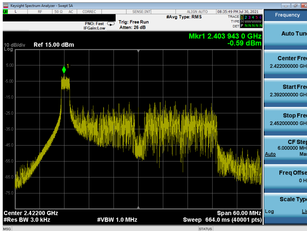
Plot 7-43. Power Spectral Density Plot SISO NORTH (802.11ax 40MHz BW OFDMA – 26 Tones – Ch. 3)
