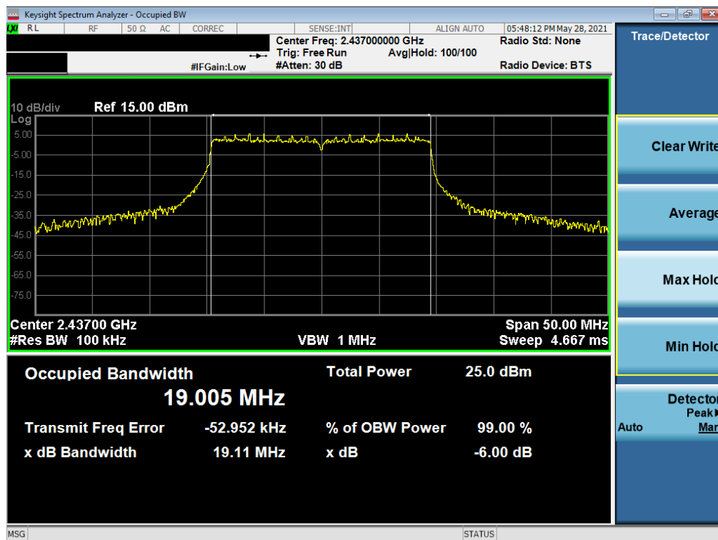
Plot 7-5. 6dB Bandwidth Plot SISO SOUTH (802.11ax 20MHz BW OFDMA – 242 Tones – Ch. 6)
