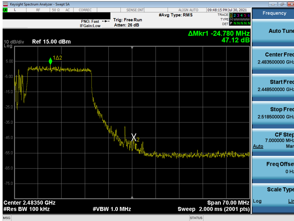
Plot 7-89. Band Edge Plot SISO SOUTH (802.11ax 40MHz BW OFDMA – 242 Tones – Ch. 9)
