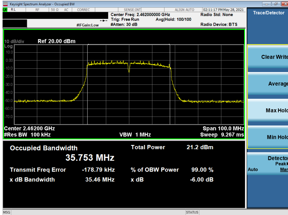
Plot 7-33. 6dB Bandwidth Plot SISO NORTH (802.11n 40MHz BW (2.4GHz) – Ch. 11)
