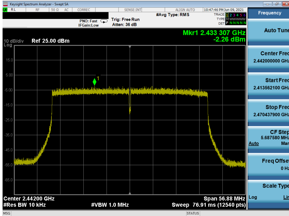
Plot 7-53. Power Spectral Density Plot SISO SOUTH (802.11ax 40MHz BW (2.4GHz) – Ch. 7)
