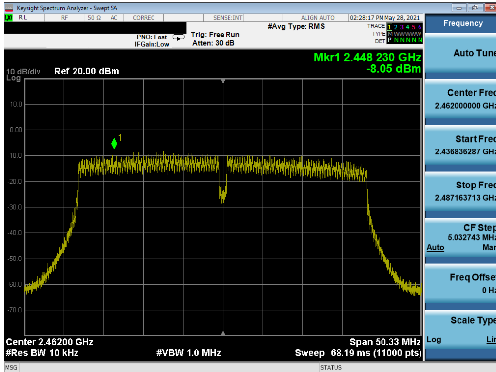
Plot 7-51. Power Spectral Density Plot SISO SOUTH (802.11n 40MHz BW (2.4GHz) – Ch. 11)
