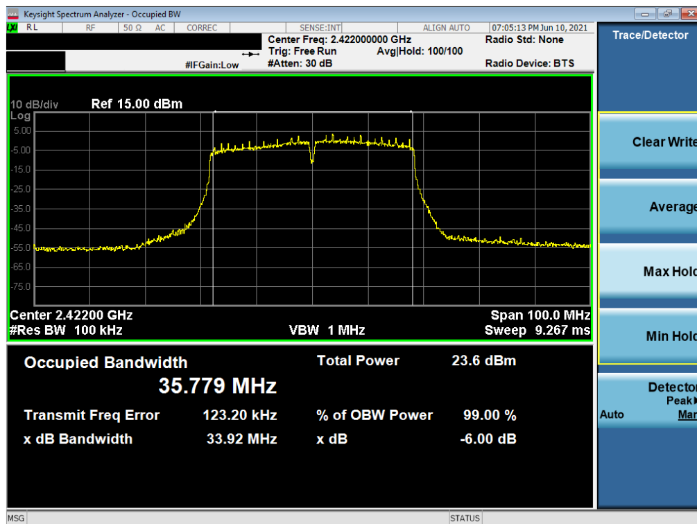
Plot 7-34. 6dB Bandwidth Plot SISO NORTH (802.11ax 40MHz BW (2.4GHz) – Ch. 3)
