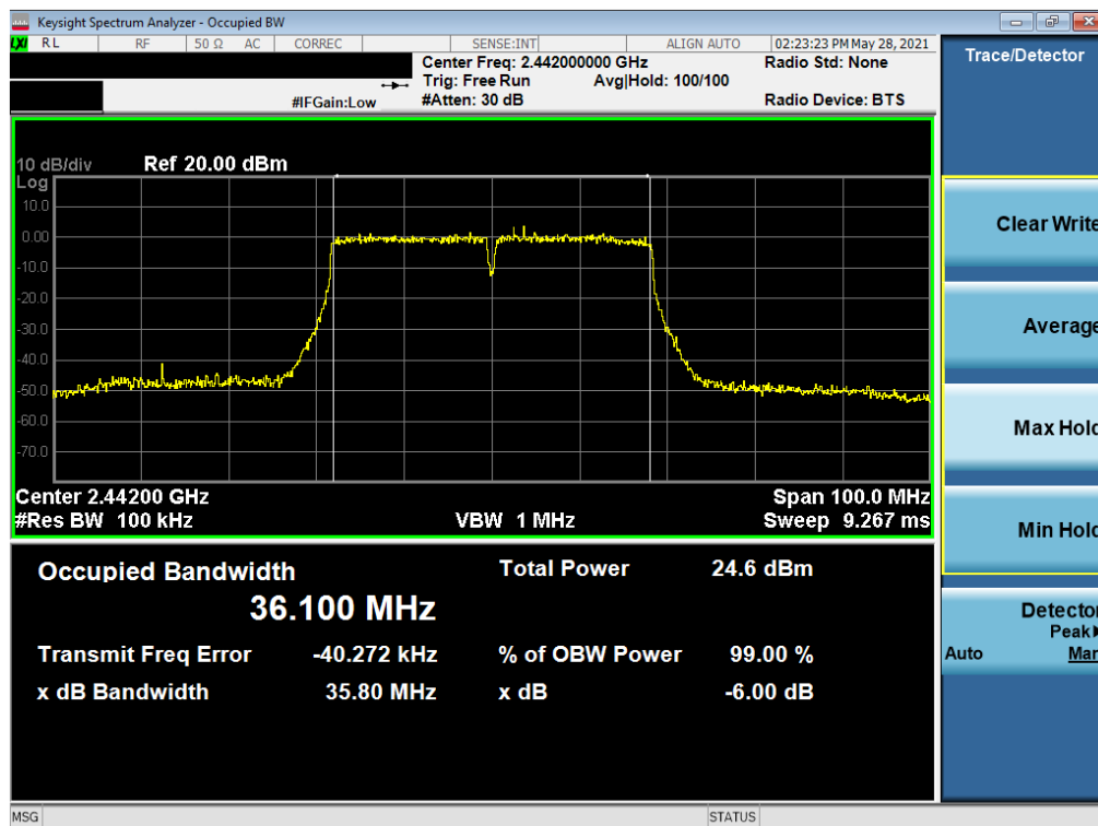
Plot 7-14. 6dB Bandwidth Plot SISO SOUTH (802.11n 40MHz BW (2.4GHz) – Ch. 7)
