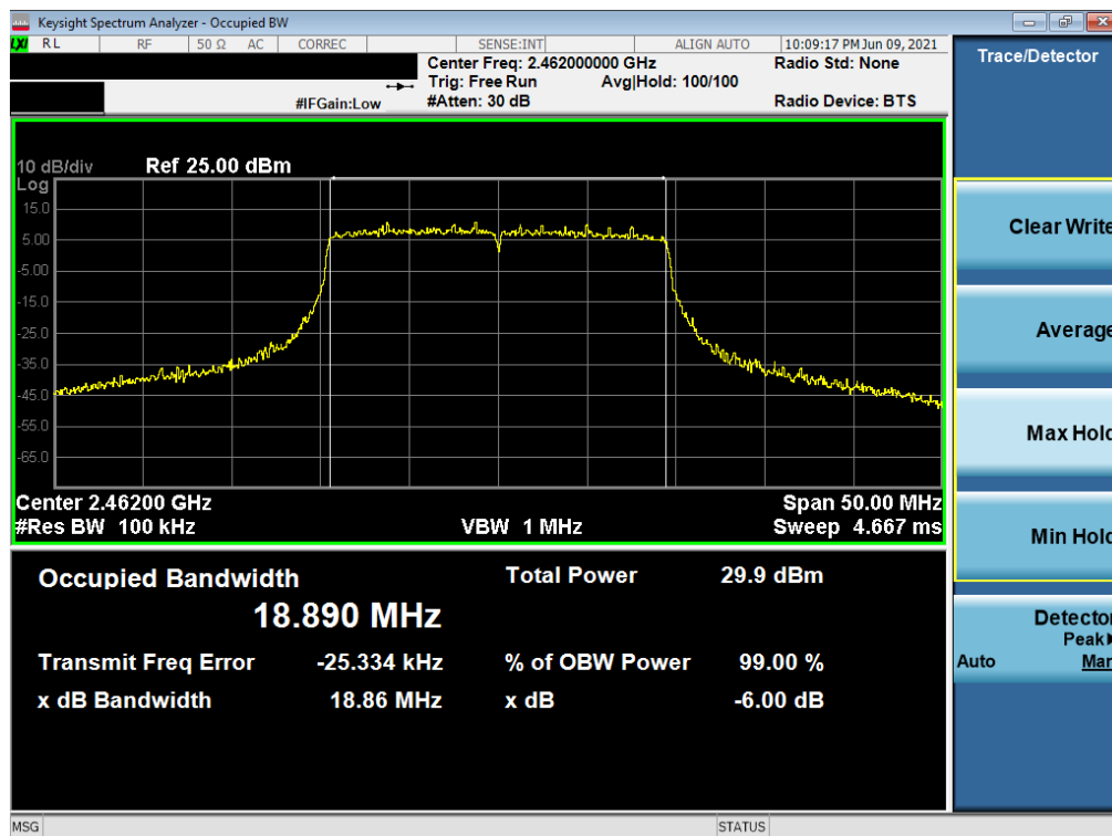
Plot 7-12. 6dB Bandwidth Plot SISO SOUTH (802.11ax 20MHz BW (2.4GHz) – Ch. 11)
