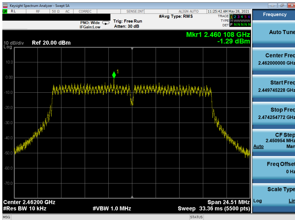
Plot 7-42. Power Spectral Density Plot SISO SOUTH (802.11g – Ch. 11)
