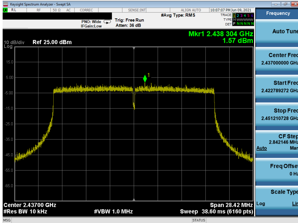
Plot 7-47. Power Spectral Density Plot SISO SOUTH (802.11ax 20MHz BW (2.4GHz) – Ch. 6)
