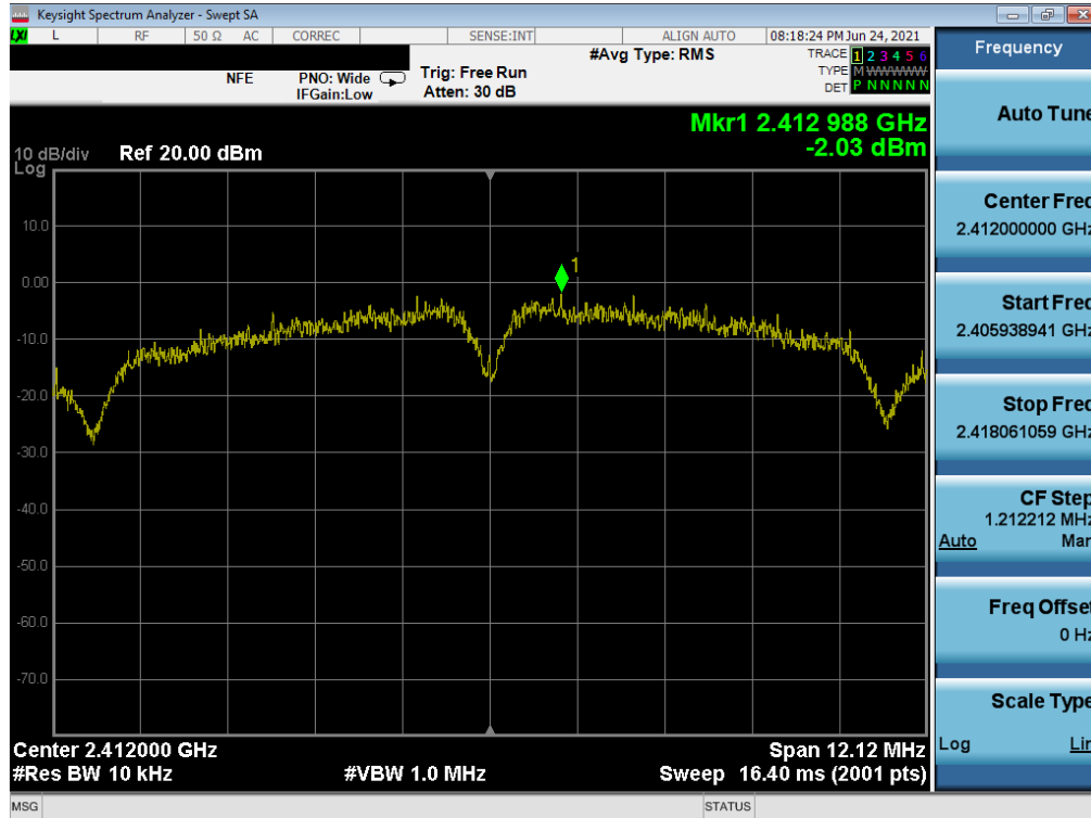
Plot 7-91. Power Spectral Density Plot MIMO NORTH (802.11b – Ch. 1)
