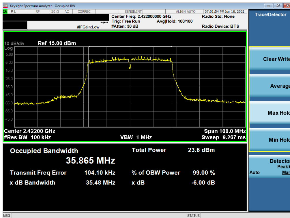
Plot 7-16. 6dB Bandwidth Plot SISO SOUTH (802.11ax 40MHz BW (2.4GHz) – Ch. 3)
