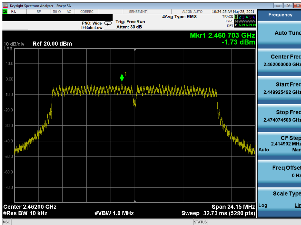
Plot 7-60. Power Spectral Density Plot SISO NORTH (802.11g – Ch. 11)
