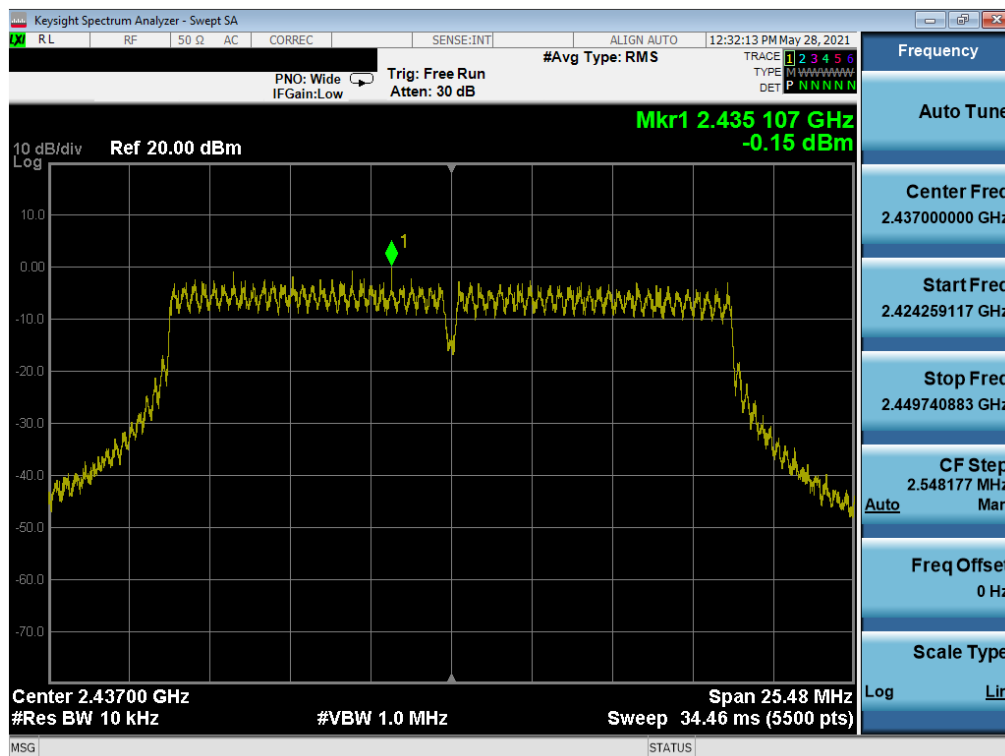
Plot 7-62. Power Spectral Density Plot SISO NORTH (802.11n 20MHz BW (2.4GHz) – Ch. 6)
