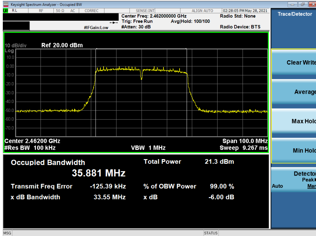
Plot 7-15. 6dB Bandwidth Plot SISO SOUTH (802.11n 40MHz BW (2.4GHz) – Ch. 11)
