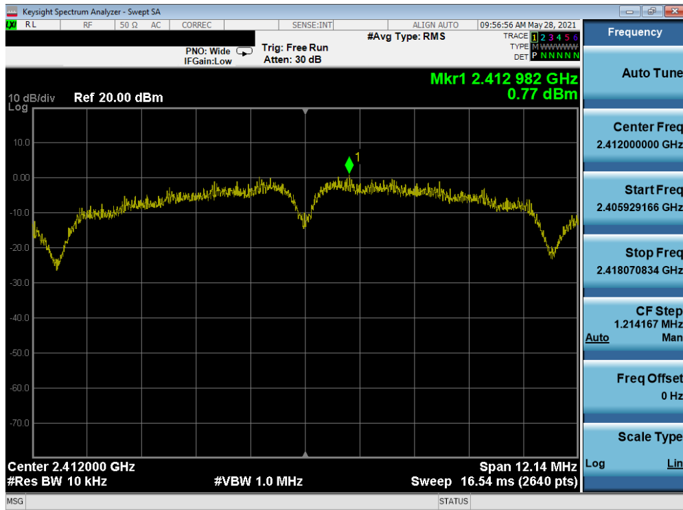
Plot 7-55. Power Spectral Density Plot SISO NORTH (802.11b – Ch. 1)
