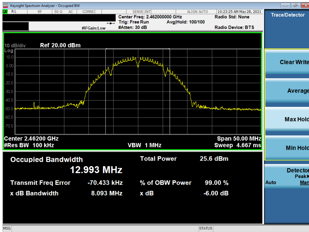
Plot 7-21. 6dB Bandwidth Plot SISO NORTH (802.11b – Ch. 11)
