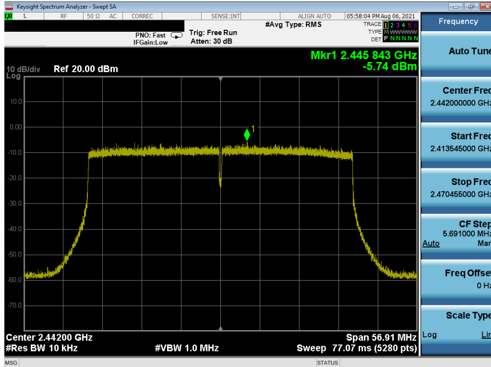
Plot 7-89. Power Spectral Density Plot MIMO SOUTH (802.11ax 40MHz BW (2.4GHz) – Ch. 7)
