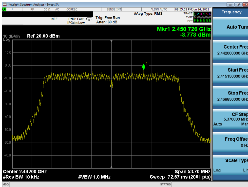
Plot 7-86. Power Spectral Density Plot MIMO SOUTH (802.11n 40MHz BW (2.4GHz) – Ch. 7)
