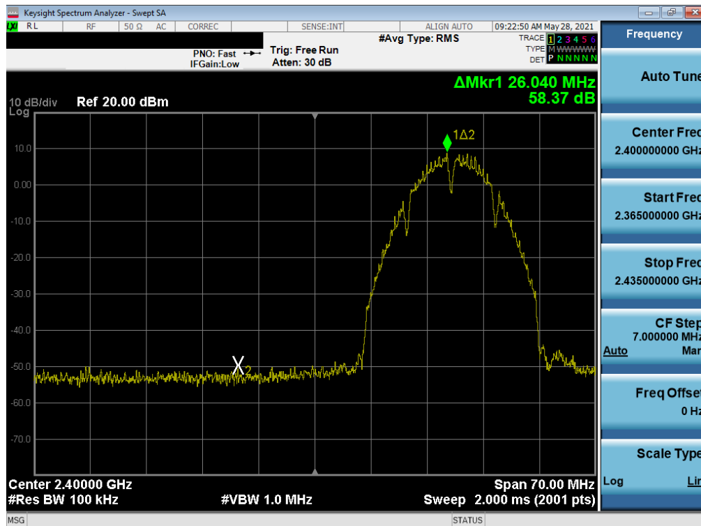
Plot 7-110. Band Edge Plot SISO SOUTH (802.11b – Ch. 2)
