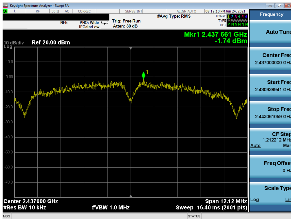
Plot 7-92. Power Spectral Density Plot MIMO NORTH (802.11b – Ch. 6)
