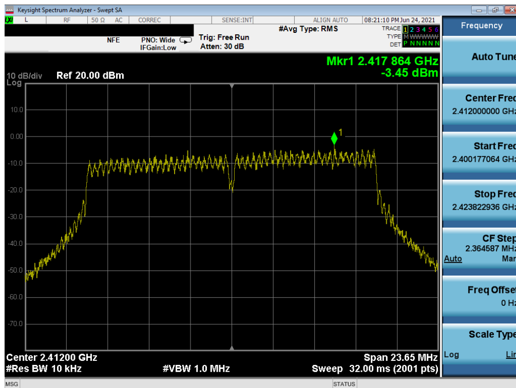
Plot 7-94. Power Spectral Density Plot MIMO NORTH (802.11g – Ch. 1)
