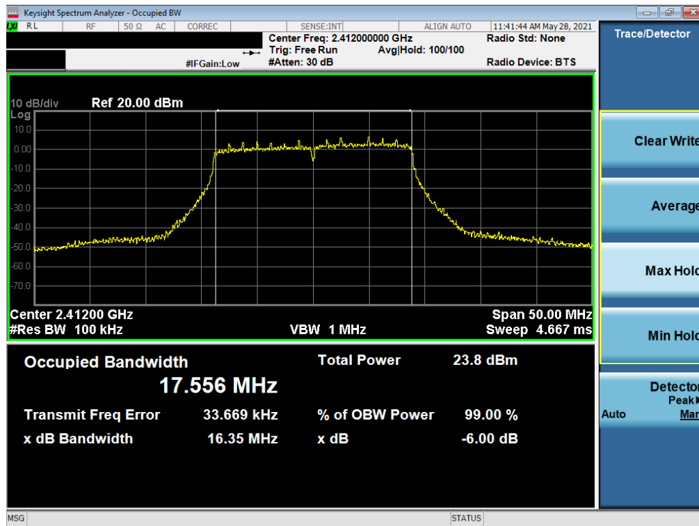
Plot 7-7. 6dB Bandwidth Plot SISO SOUTH (802.11n 20MHz BW (2.4GHz) – Ch. 1)
