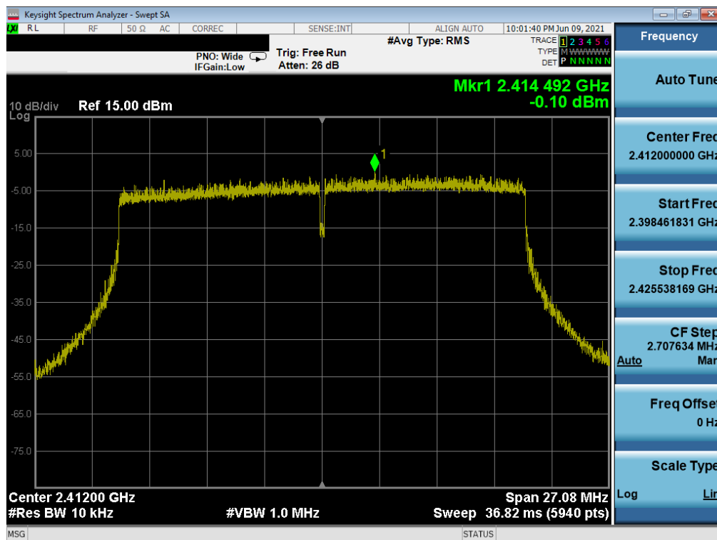
Plot 7-46. Power Spectral Density Plot SISO SOUTH (802.11ax 20MHz BW (2.4GHz) – Ch. 1)
