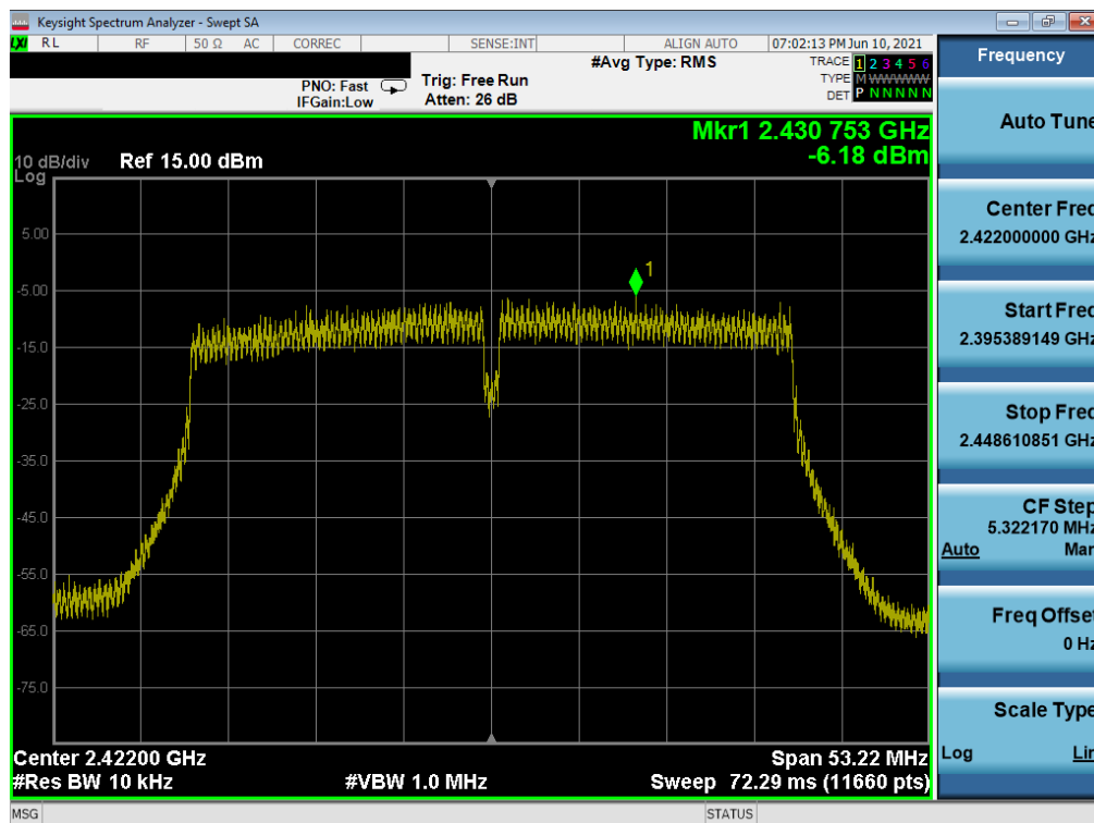
Plot 7-52. Power Spectral Density Plot SISO SOUTH (802.11ax 40MHz BW (2.4GHz) – Ch. 3)
