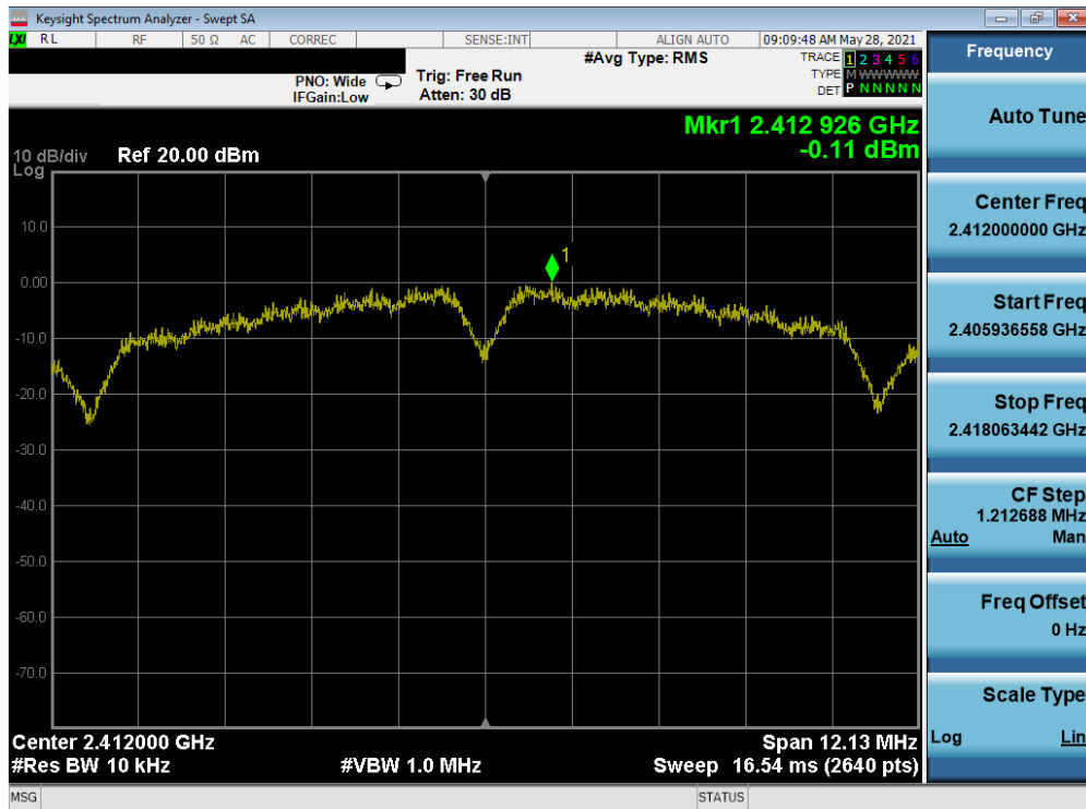
Plot 7-37. Power Spectral Density Plot SISO SOUTH (802.11b – Ch. 1)
