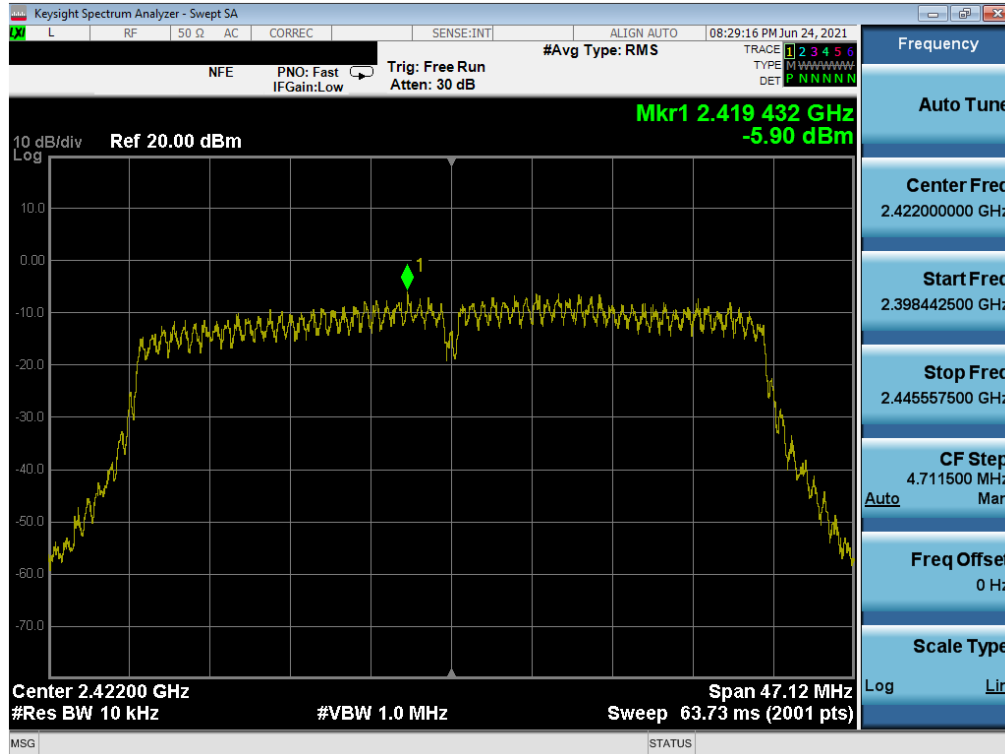
Plot 7-103. Power Spectral Density Plot MIMO NORTH (802.11n 40MHz BW (2.4GHz) – Ch. 3)
