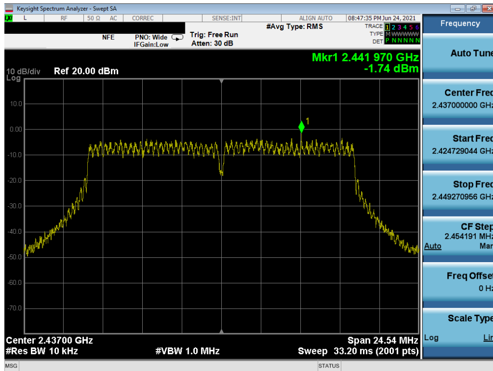
Plot 7-77. Power Spectral Density Plot MIMO SOUTH (802.11g – Ch. 6)
