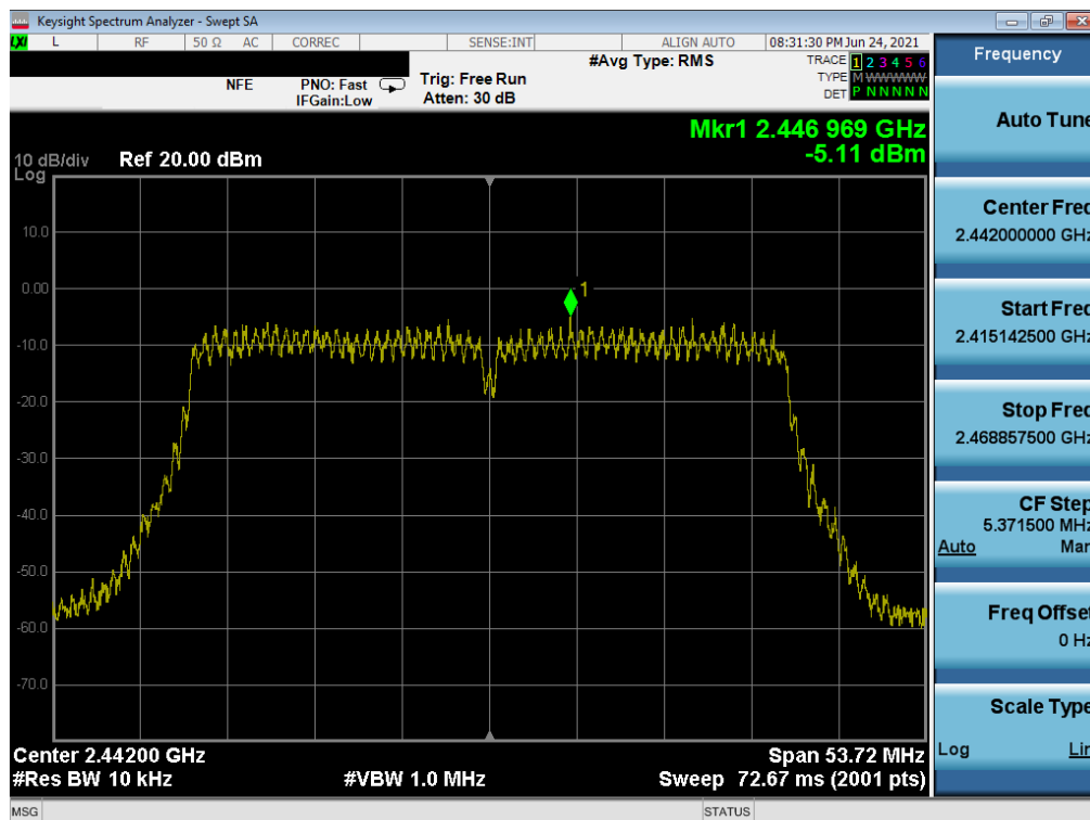
Plot 7-104. Power Spectral Density Plot MIMO NORTH (802.11n 40MHz BW (2.4GHz) – Ch. 7)
