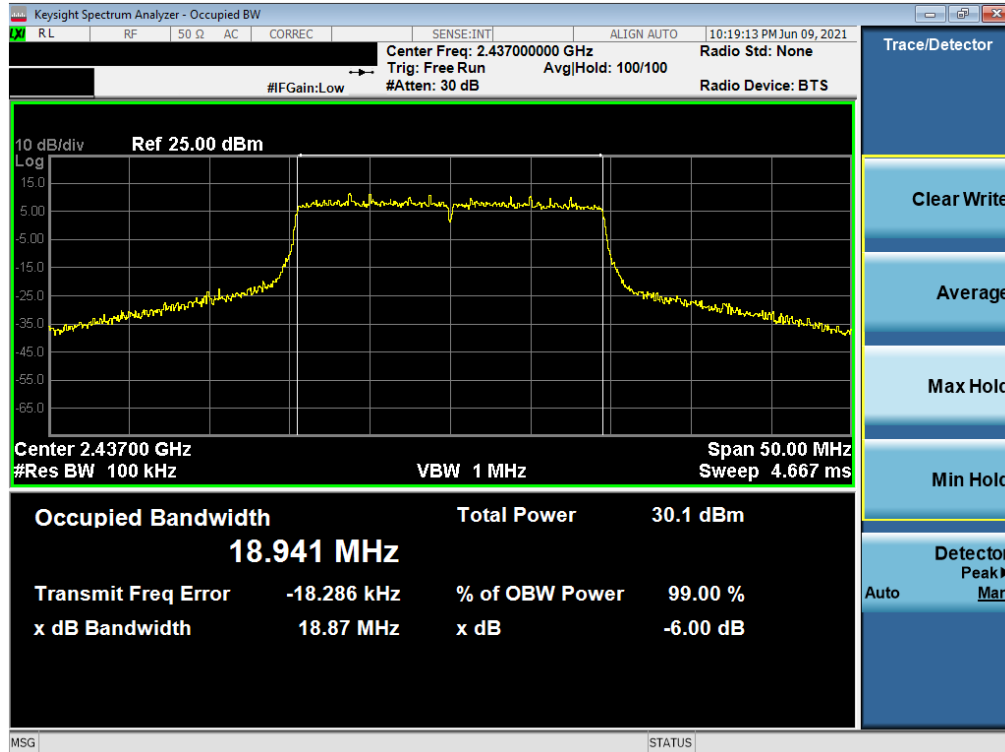
Plot 7-29. 6dB Bandwidth Plot SISO NORTH (802.11ax 20MHz BW (2.4GHz) – Ch. 6)
