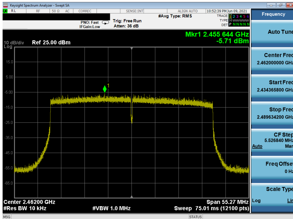
Plot 7-54. Power Spectral Density Plot SISO SOUTH (802.11ax 40MHz BW (2.4GHz) – Ch. 11)
