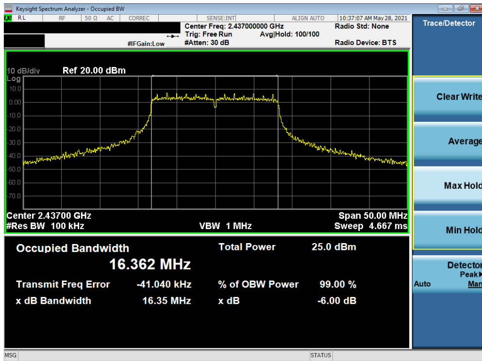
Plot 7-23. 6dB Bandwidth Plot SISO NORTH (802.11g – Ch. 6)
