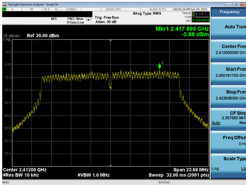
Plot 7-76. Power Spectral Density Plot MIMO SOUTH (802.11g – Ch. 1)
