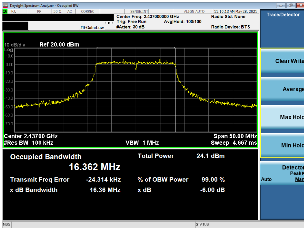
Plot 7-5. 6dB Bandwidth Plot SISO SOUTH (802.11g – Ch. 6)
