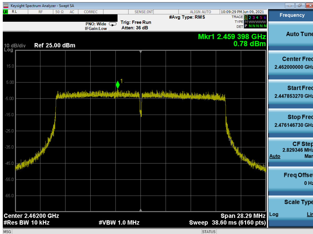
Plot 7-48. Power Spectral Density Plot SISO SOUTH (802.11ax 20MHz BW (2.4GHz) – Ch. 11)
