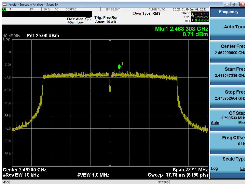
Plot 7-66. Power Spectral Density Plot SISO NORTH (802.11ax 20MHz BW (2.4GHz) – Ch. 11)
