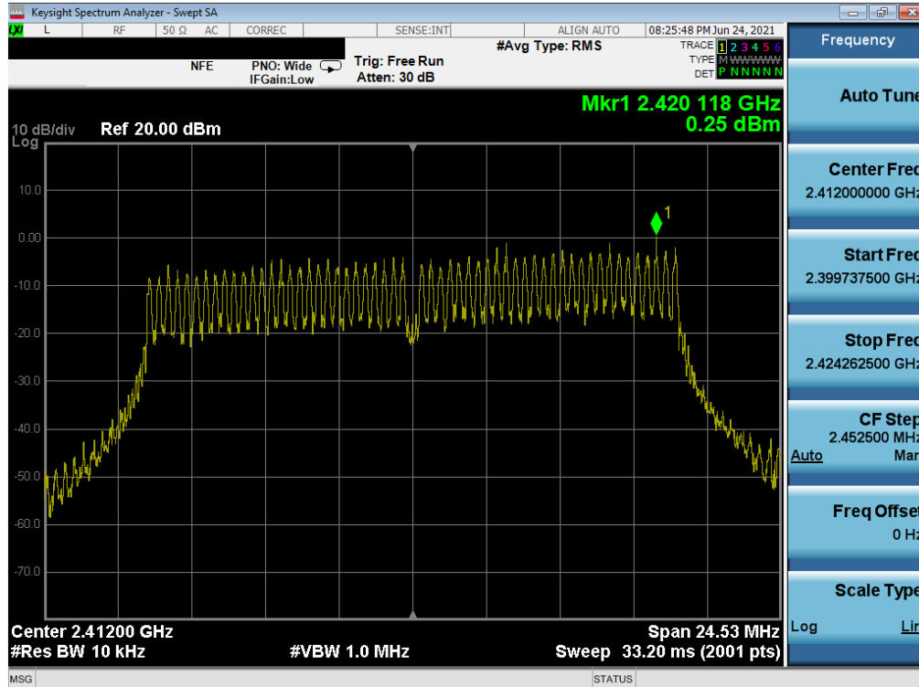
Plot 7-97. Power Spectral Density Plot MIMO NORTH (802.11n 20MHz BW (2.4GHz) – Ch. 1)
