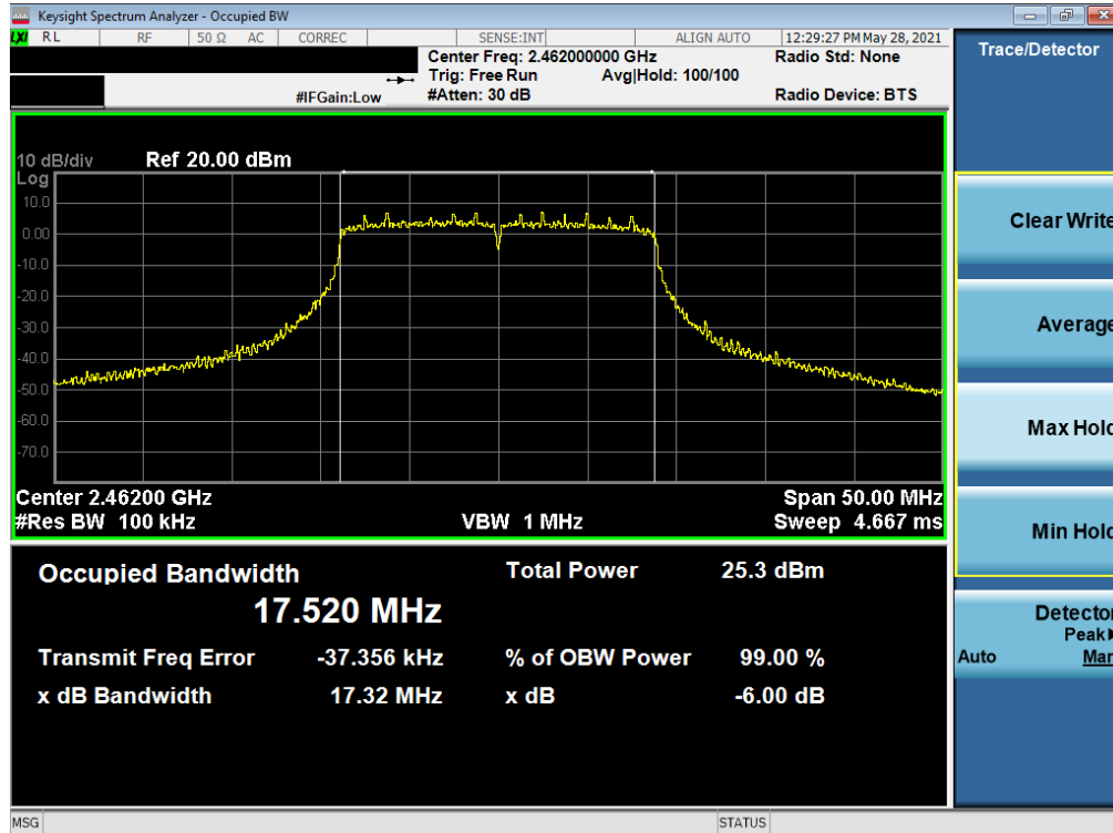
Plot 7-27. 6dB Bandwidth Plot SISO NORTH (802.11n 20MHz BW (2.4GHz) – Ch. 11)
