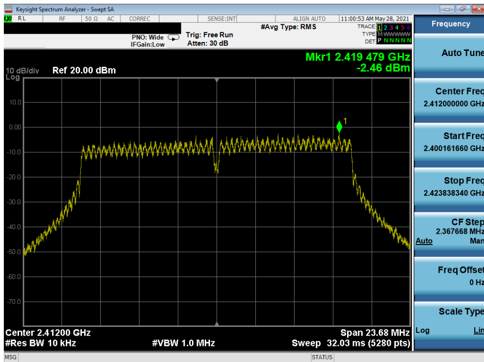
Plot 7-40. Power Spectral Density Plot SISO SOUTH (802.11g – Ch. 1)
