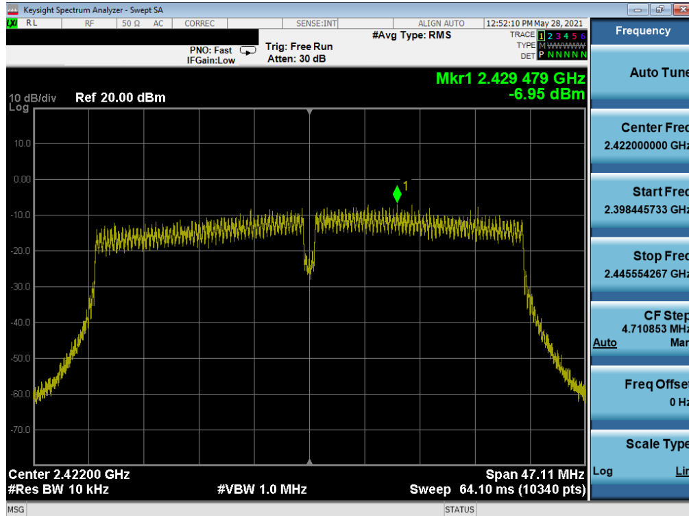
Plot 7-67. Power Spectral Density Plot SISO NORTH (802.11n 40MHz BW (2.4GHz) – Ch. 3)
