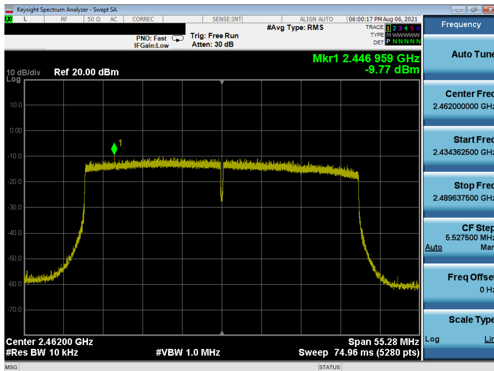
Plot 7-90. Power Spectral Density Plot MIMO SOUTH (802.11ax 40MHz BW (2.4GHz) – Ch. 11)
