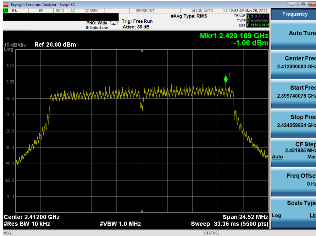
Plot 7-43. Power Spectral Density Plot SISO SOUTH (802.11n 20MHz BW (2.4GHz) – Ch. 1)
