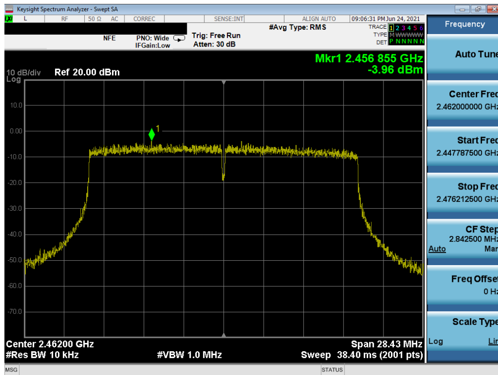
Plot 7-84. Power Spectral Density Plot MIMO SOUTH (802.11ax 20MHz BW (2.4GHz) – Ch. 11)
