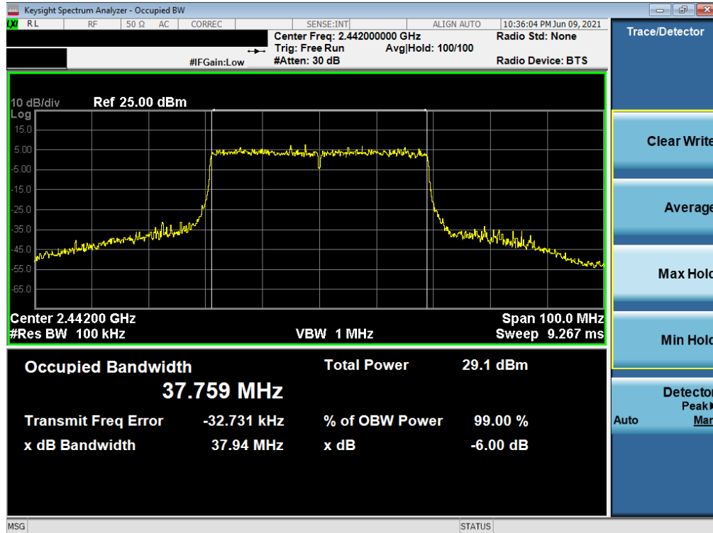
Plot 7-35. 6dB Bandwidth Plot SISO NORTH (802.11ax 40MHz BW (2.4GHz) – Ch. 7)
