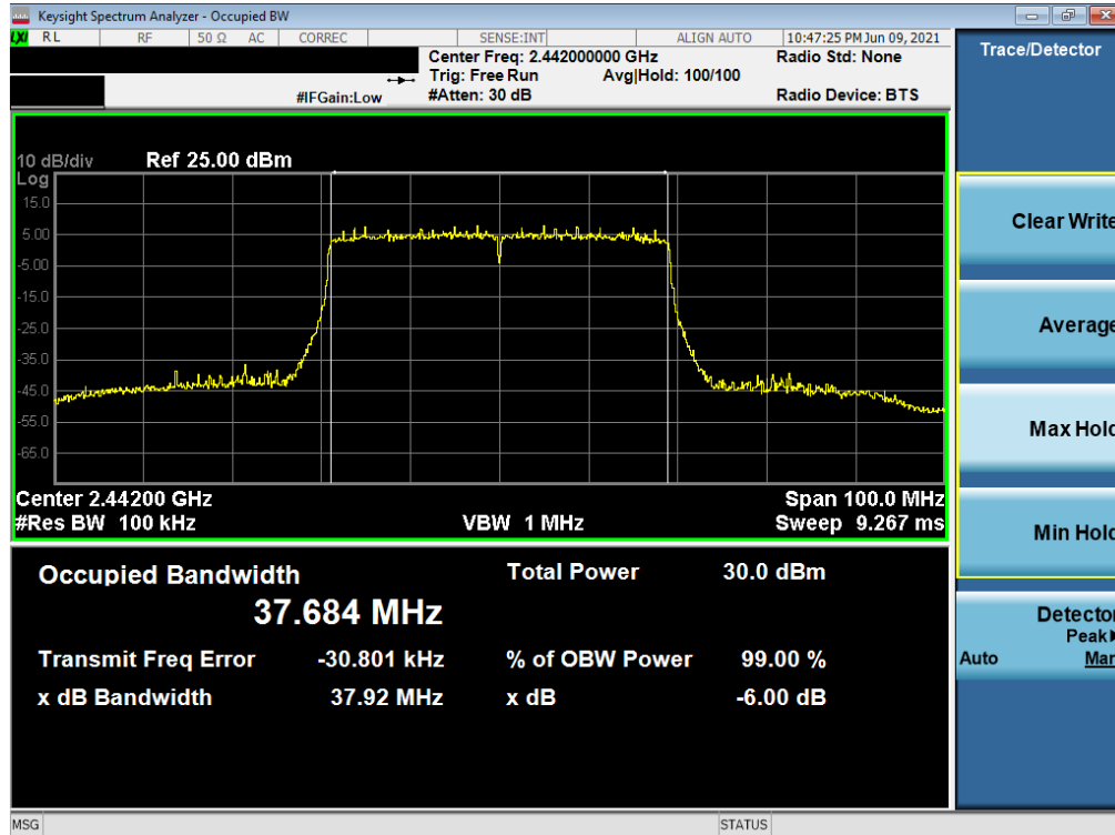
Plot 7-17. 6dB Bandwidth Plot SISO SOUTH (802.11ax 40MHz BW (2.4GHz) – Ch. 7)
