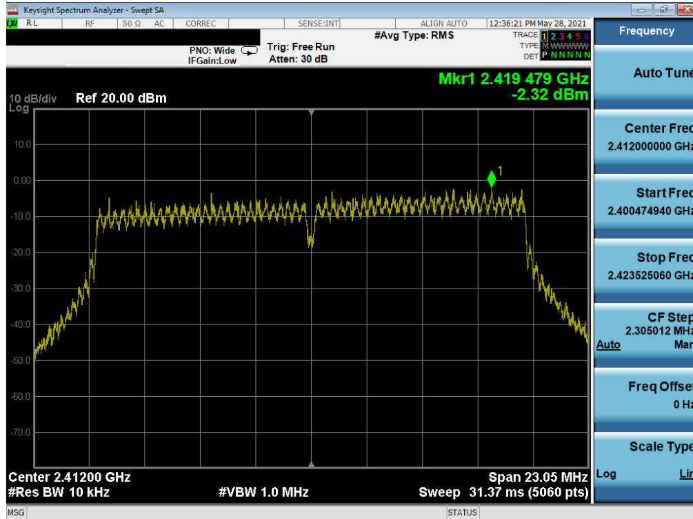
Plot 7-61. Power Spectral Density Plot SISO NORTH (802.11n 20MHz BW (2.4GHz) – Ch. 1)
