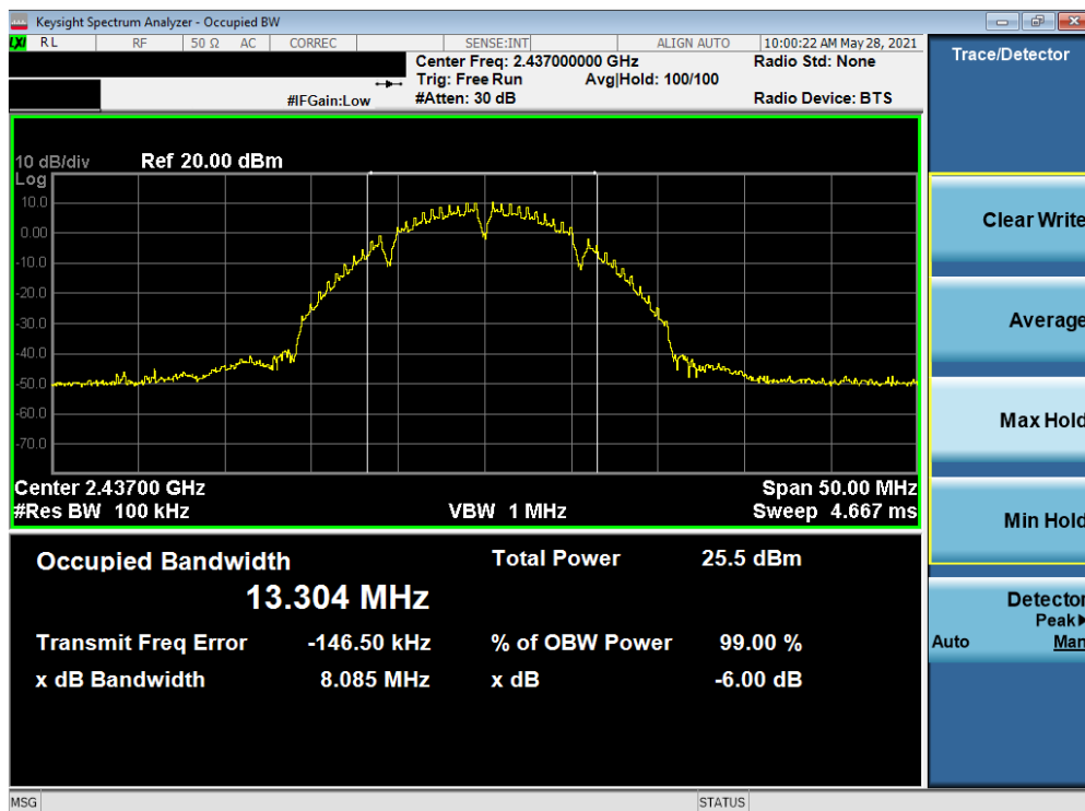
Plot 7-20. 6dB Bandwidth Plot SISO NORTH (802.11b – Ch. 6)
