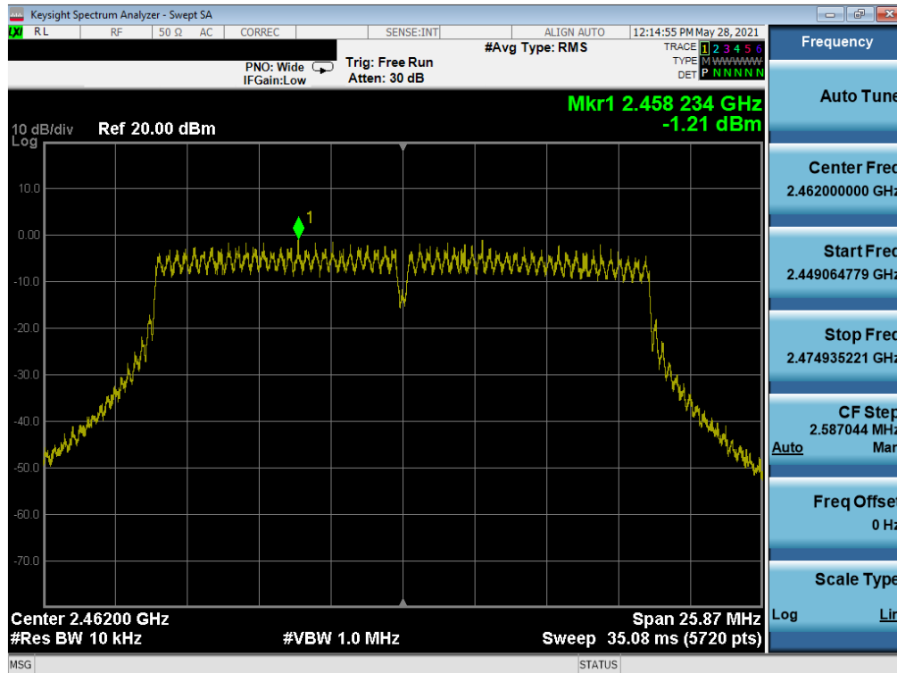
Plot 7-45. Power Spectral Density Plot SISO SOUTH (802.11n 20MHz BW (2.4GHz) – Ch. 11)
