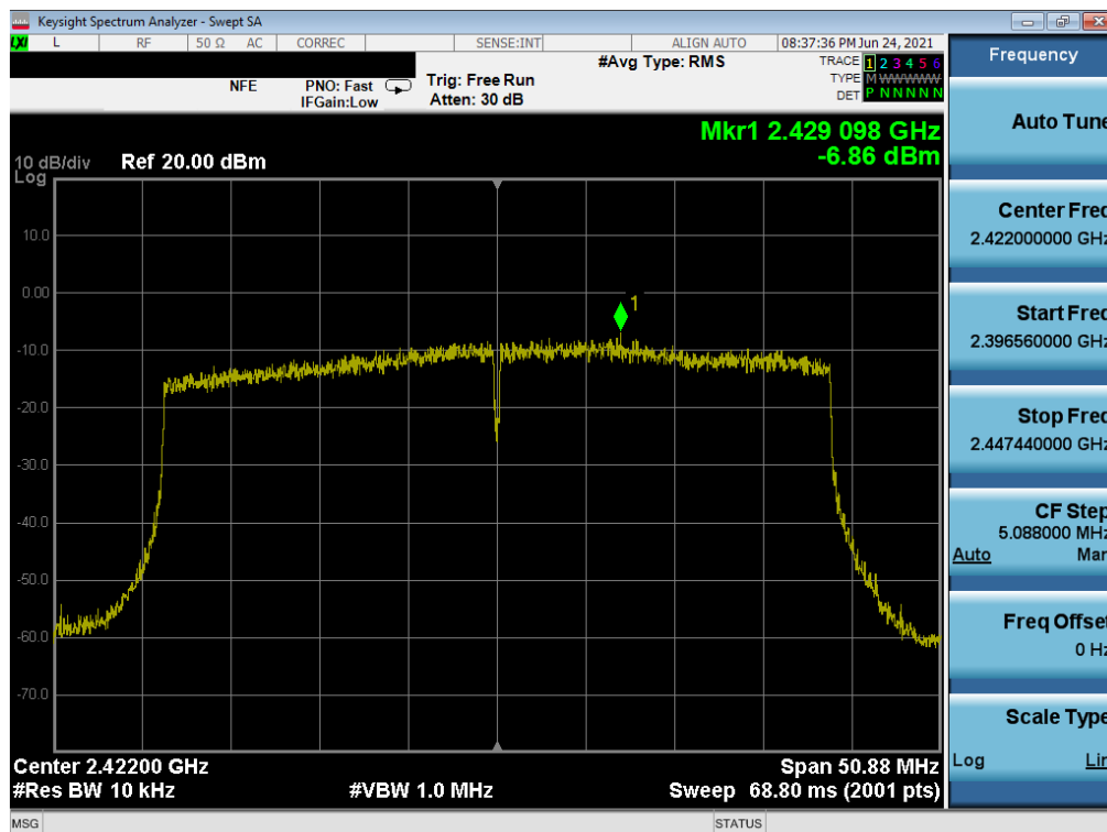
Plot 7-106. Power Spectral Density Plot MIMO NORTH (802.11ax 40MHz BW (2.4GHz) – Ch. 3)
