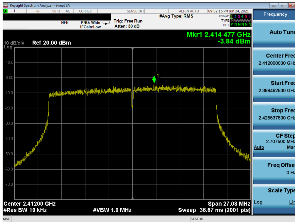
Plot 7-82. Power Spectral Density Plot MIMO SOUTH (802.11ax 20MHz BW (2.4GHz) – Ch. 1)
