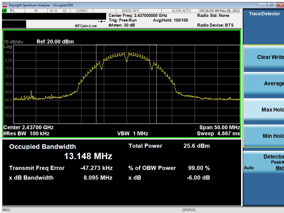
Plot 7-2. 6dB Bandwidth Plot SISO SOUTH (802.11b – Ch. 6)
