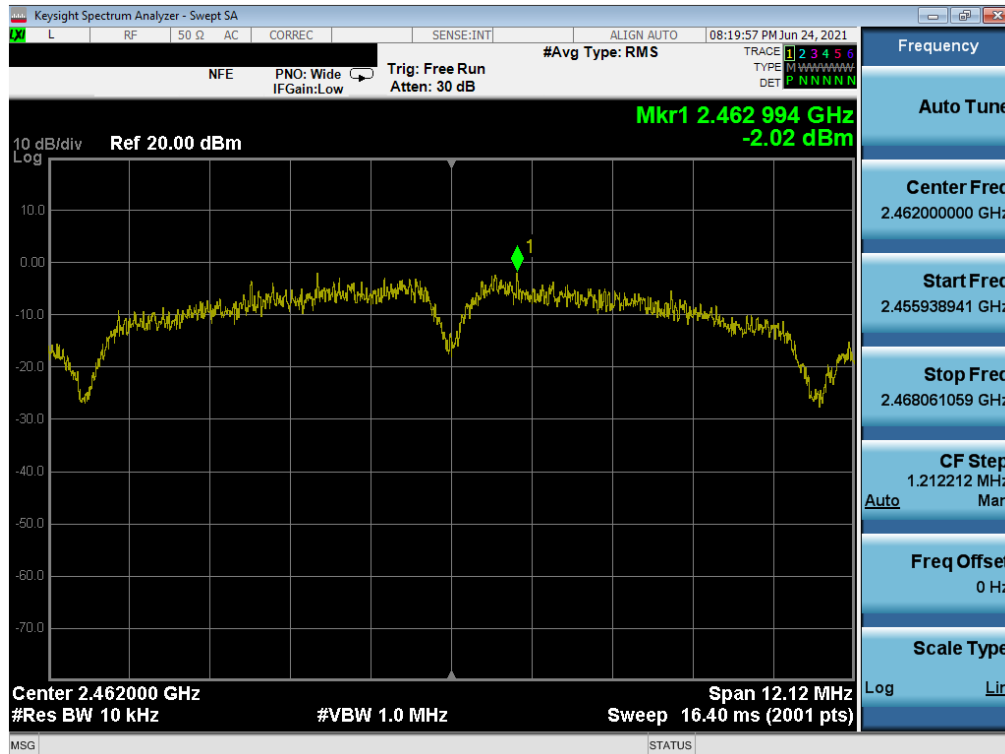
Plot 7-93. Power Spectral Density Plot MIMO NORTH (802.11b – Ch. 11)
