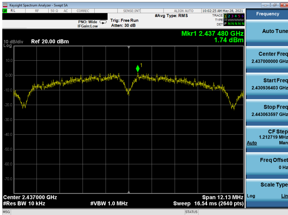
Plot 7-56. Power Spectral Density Plot SISO NORTH (802.11b – Ch. 6)
