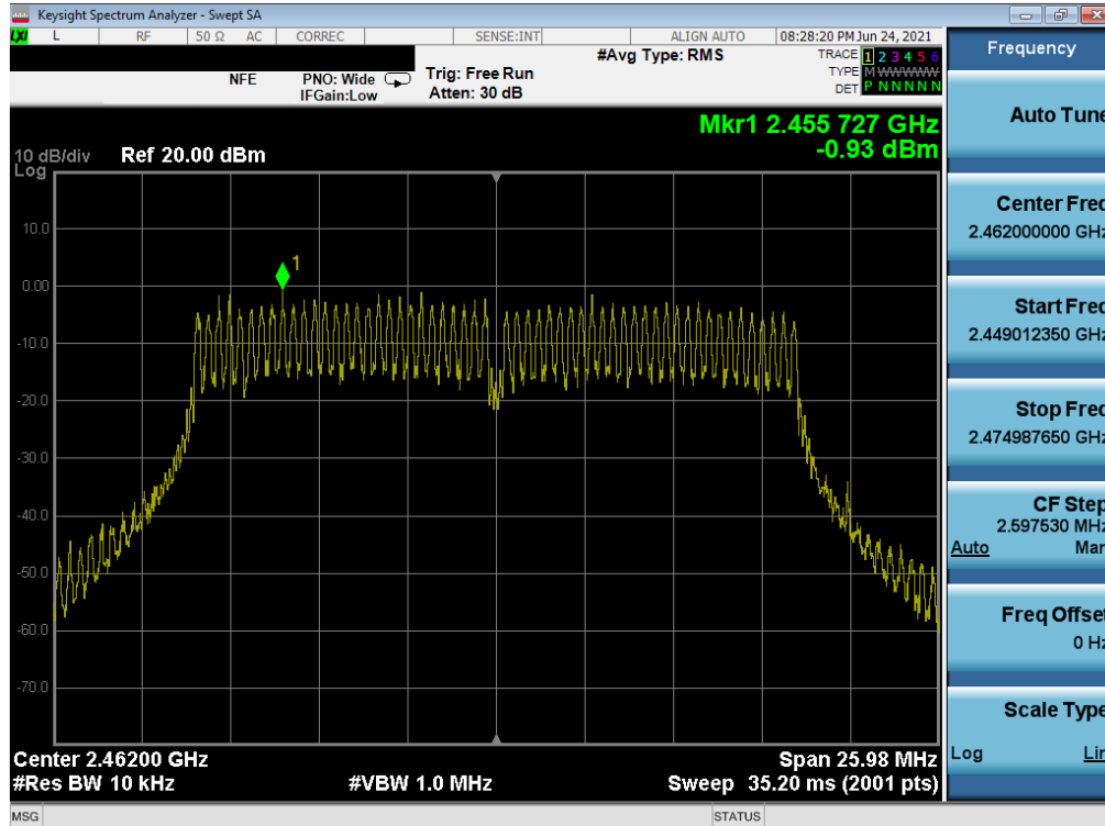
Plot 7-99. Power Spectral Density Plot MIMO NORTH (802.11n 20MHz BW (2.4GHz) – Ch. 11)
