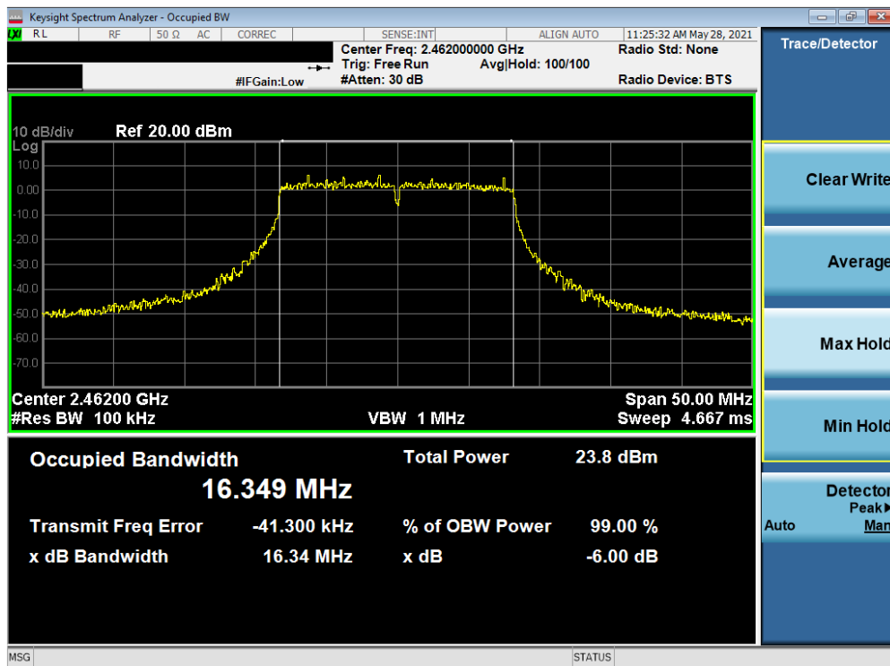
Plot 7-6. 6dB Bandwidth Plot SISO SOUTH (802.11g – Ch. 11)
