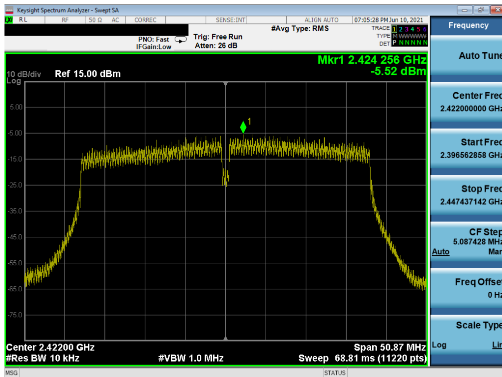
Plot 7-70. Power Spectral Density Plot SISO NORTH (802.11ax 40MHz BW (2.4GHz) – Ch. 3)
