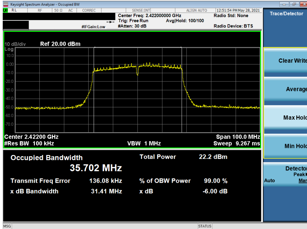
Plot 7-31. 6dB Bandwidth Plot SISO NORTH (802.11n 40MHz BW (2.4GHz) – Ch. 3)
