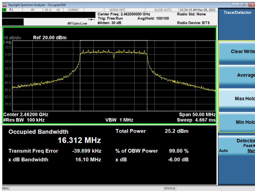
Plot 7-24. 6dB Bandwidth Plot SISO NORTH (802.11g – Ch. 11)
