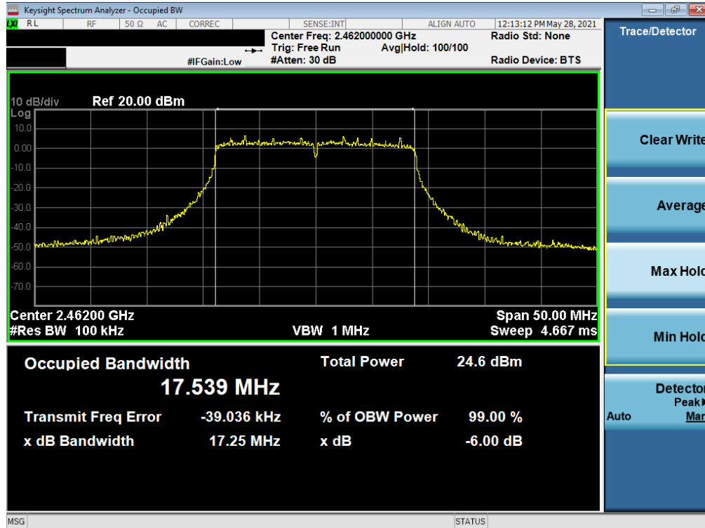
Plot 7-9. 6dB Bandwidth Plot SISO SOUTH (802.11n 20MHz BW (2.4GHz) – Ch. 11)
