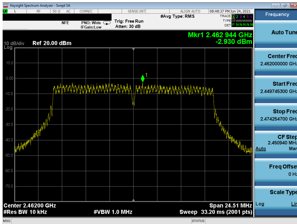
Plot 7-78. Power Spectral Density Plot MIMO SOUTH (802.11g– Ch. 11)
