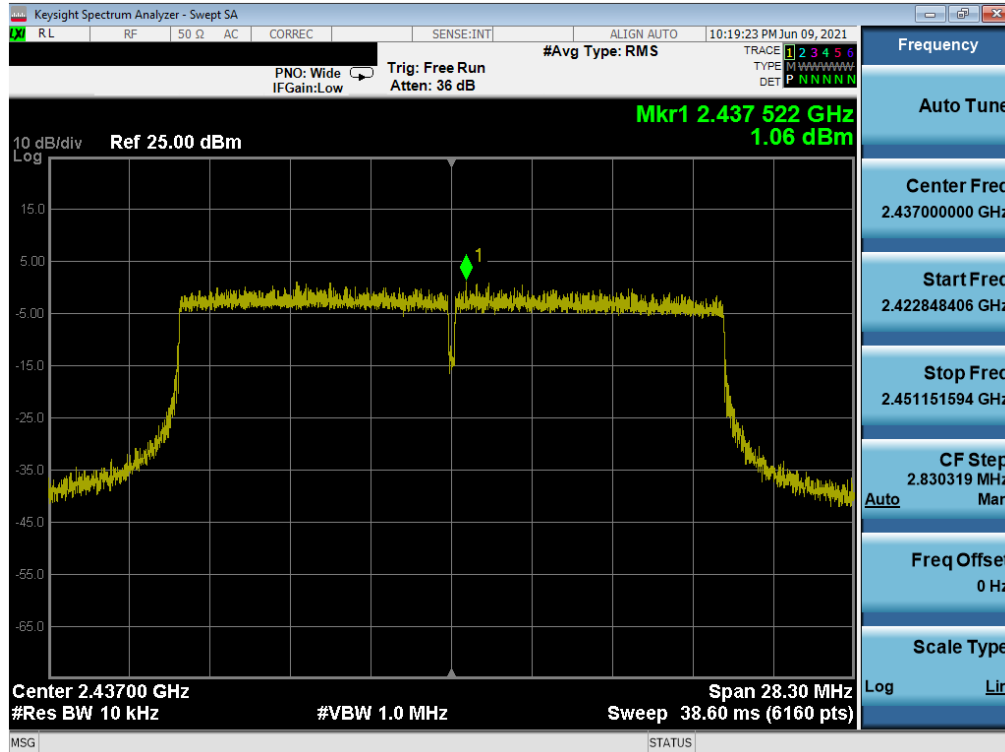
Plot 7-65. Power Spectral Density Plot SISO NORTH (802.11ax 20MHz BW (2.4GHz) – Ch. 6)
