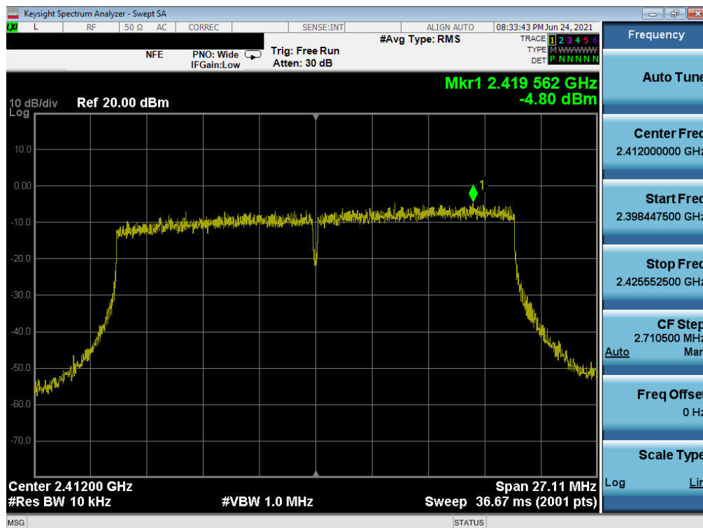
Plot 7-100. Power Spectral Density Plot MIMO NORTH (802.11ax 20MHz BW (2.4GHz) – Ch. 1)
