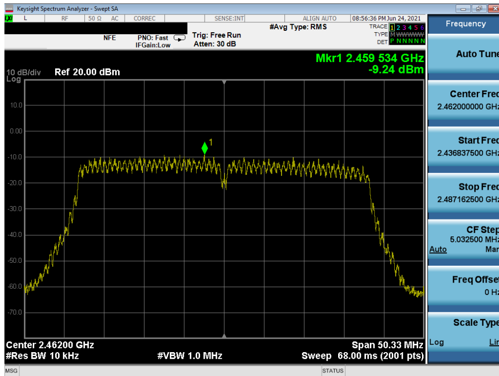
Plot 7-87. Power Spectral Density Plot MIMO SOUTH (802.11n 40MHz BW (2.4GHz) – Ch. 11)
