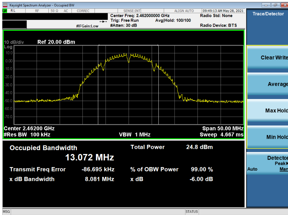
Plot 7-3. 6dB Bandwidth Plot SISO SOUTH (802.11b – Ch. 11)
