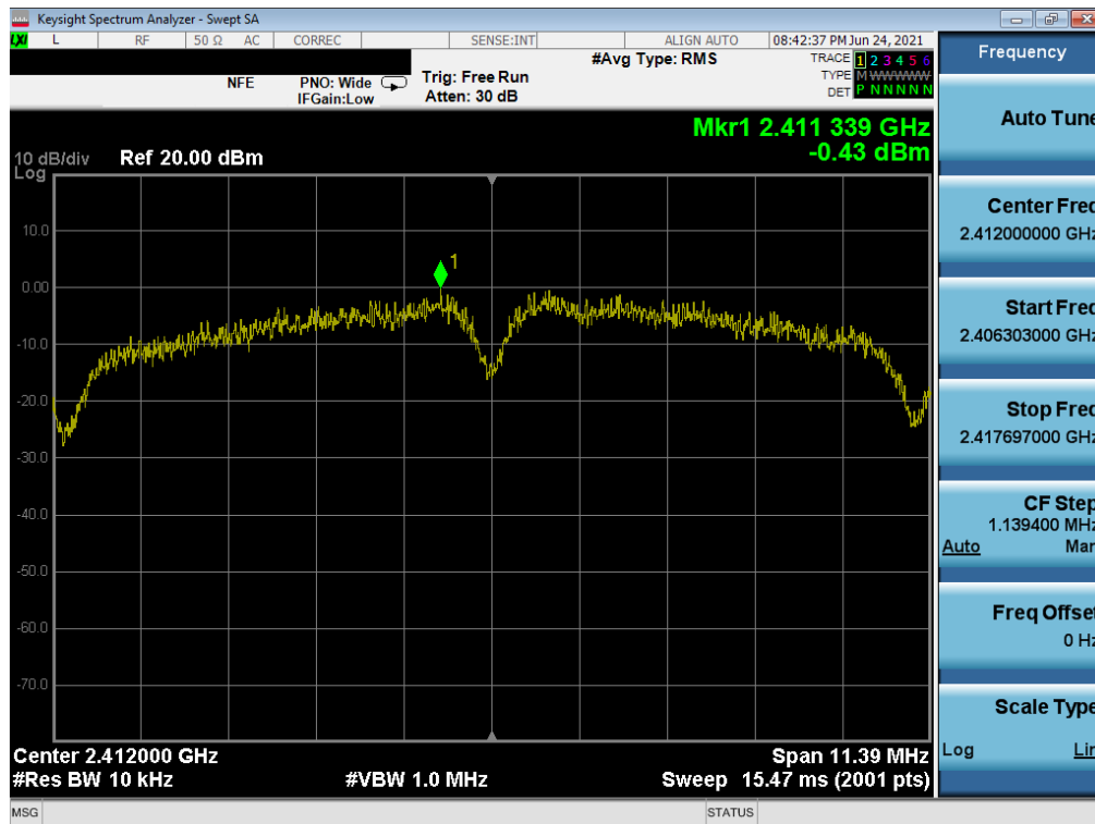
Plot 7-73. Power Spectral Density Plot MIMO SOUTH (802.11b – Ch. 1)
