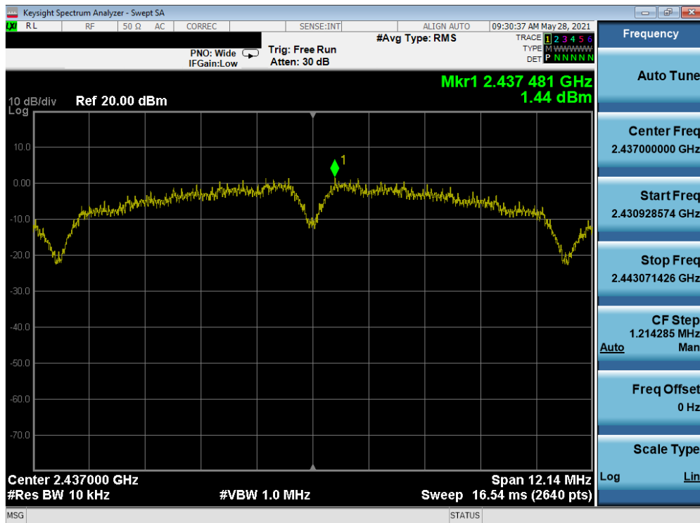
Plot 7-38. Power Spectral Density Plot SISO SOUTH (802.11b – Ch. 6)
