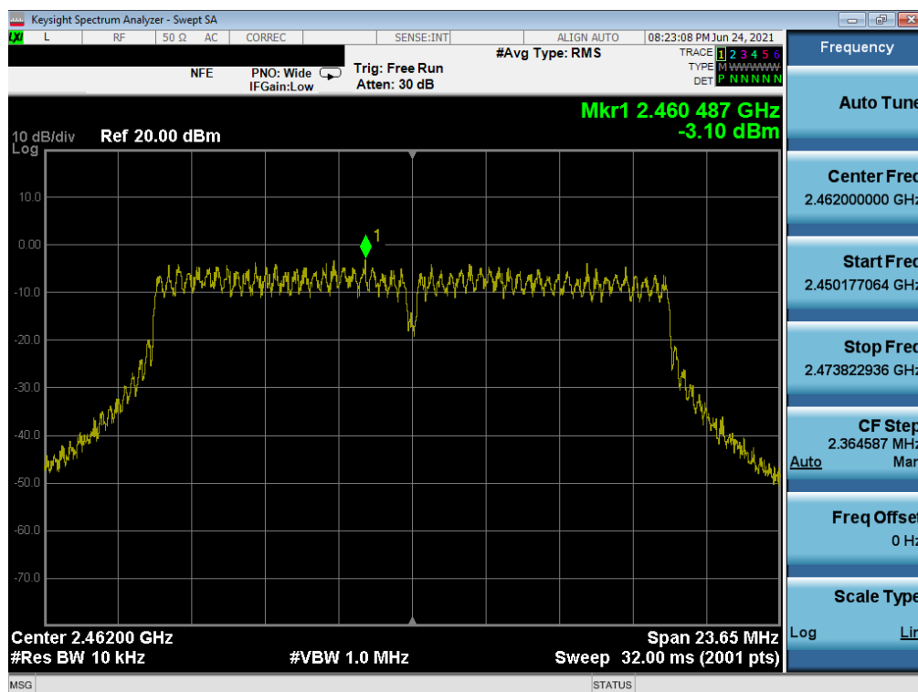
Plot 7-96. Power Spectral Density Plot MIMO NORTH (802.11g– Ch. 11)
