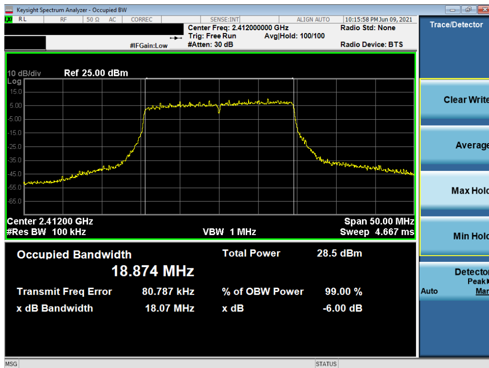
Plot 7-28. 6dB Bandwidth Plot SISO NORTH (802.11ax 20MHz BW (2.4GHz) – Ch. 1)
