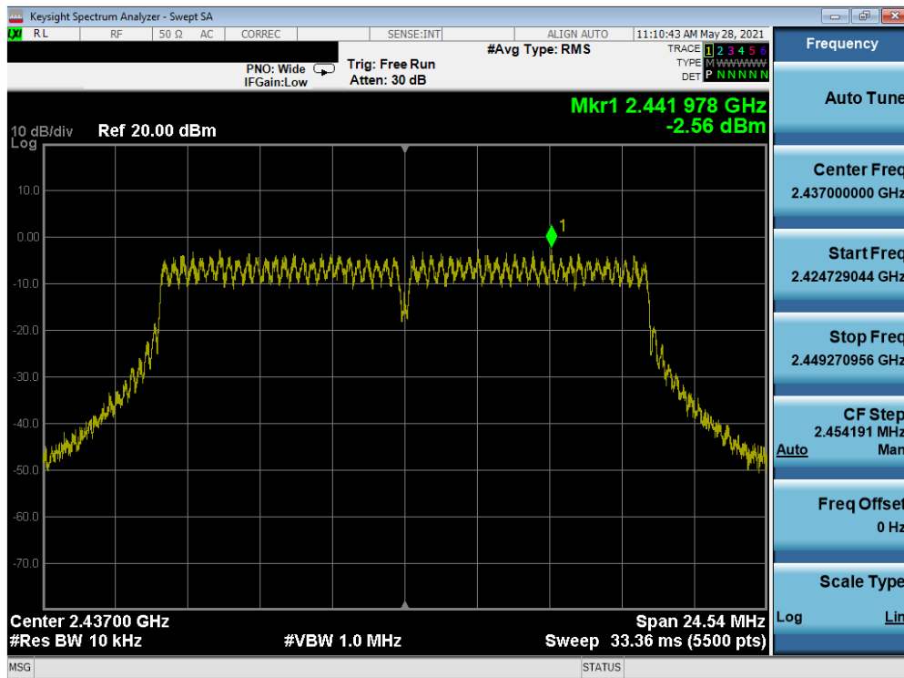
Plot 7-41. Power Spectral Density Plot SISO SOUTH (802.11g – Ch. 6)
