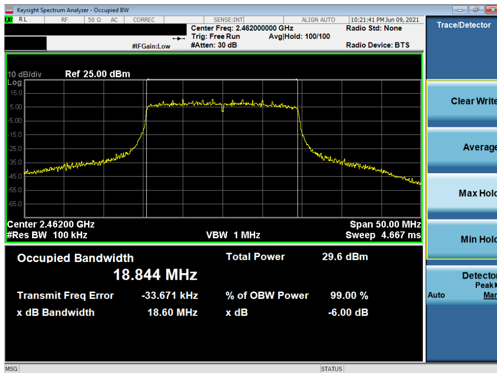
Plot 7-30. 6dB Bandwidth Plot SISO NORTH (802.11ax 20MHz BW (2.4GHz) – Ch. 11)
