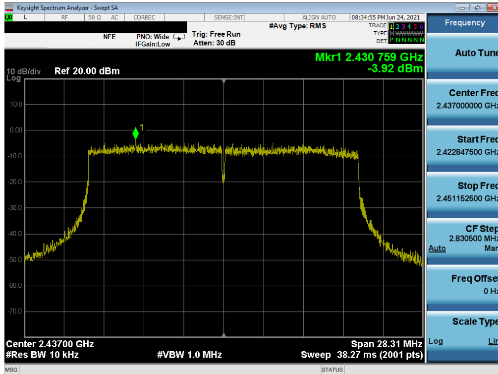
Plot 7-101. Power Spectral Density Plot MIMO NORTH (802.11ax 20MHz BW (2.4GHz) – Ch. 6)
