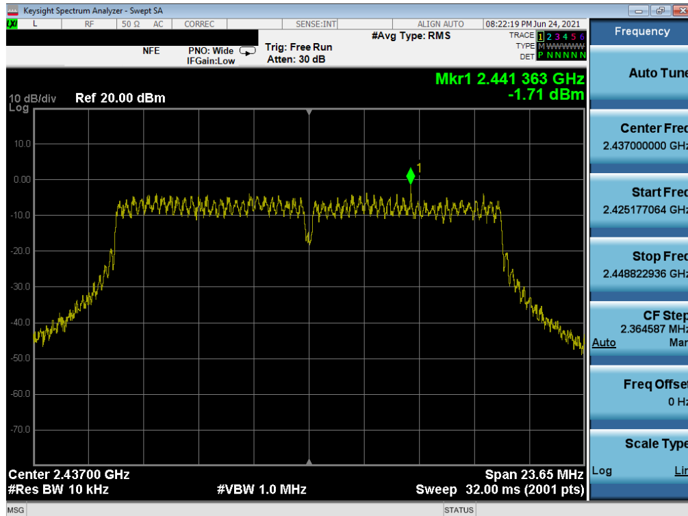
Plot 7-95. Power Spectral Density Plot MIMO NORTH (802.11g – Ch. 6)
