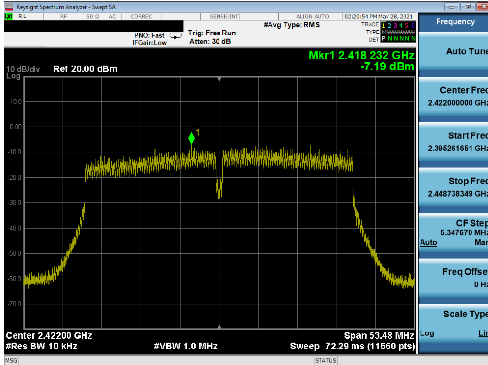
Plot 7-49. Power Spectral Density Plot SISO SOUTH (802.11n 40MHz BW (2.4GHz) – Ch. 3)
