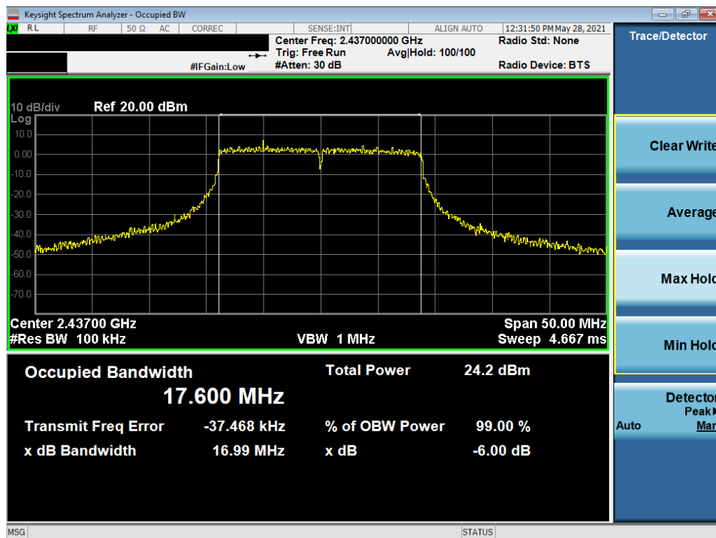
Plot 7-26. 6dB Bandwidth Plot SISO NORTH (802.11n 20MHz BW (2.4GHz) – Ch. 6)
