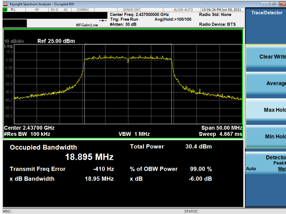
Plot 7-11. 6dB Bandwidth Plot SISO SOUTH (802.11ax 20MHz BW (2.4GHz) – Ch. 6)
