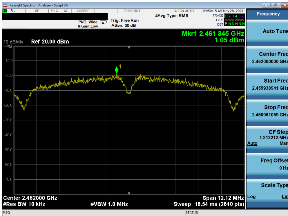
Plot 7-39. Power Spectral Density Plot SISO SOUTH (802.11b – Ch. 11)
