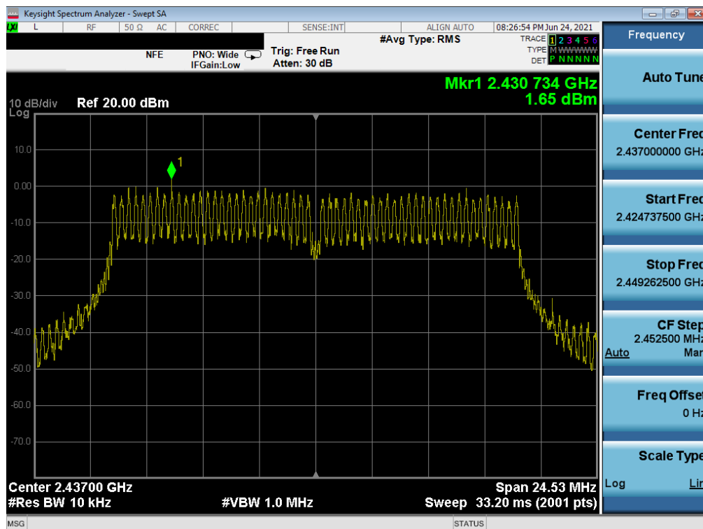
Plot 7-98. Power Spectral Density Plot MIMO NORTH (802.11n 20MHz BW (2.4GHz) – Ch. 6)
