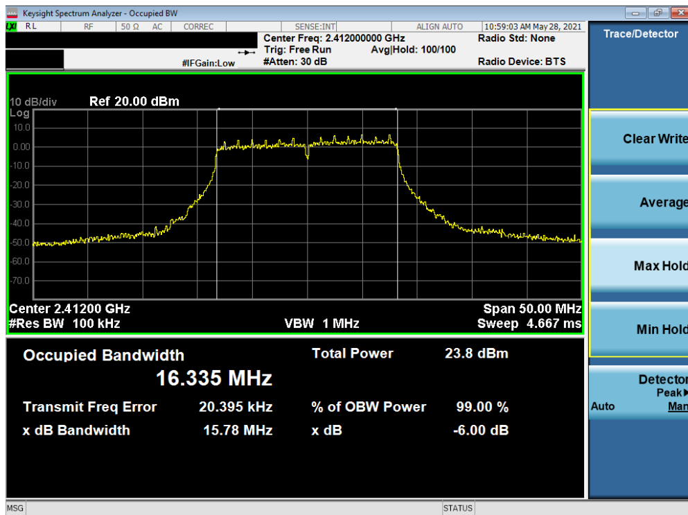
Plot 7-4. 6dB Bandwidth Plot SISO SOUTH (802.11g – Ch. 1)
