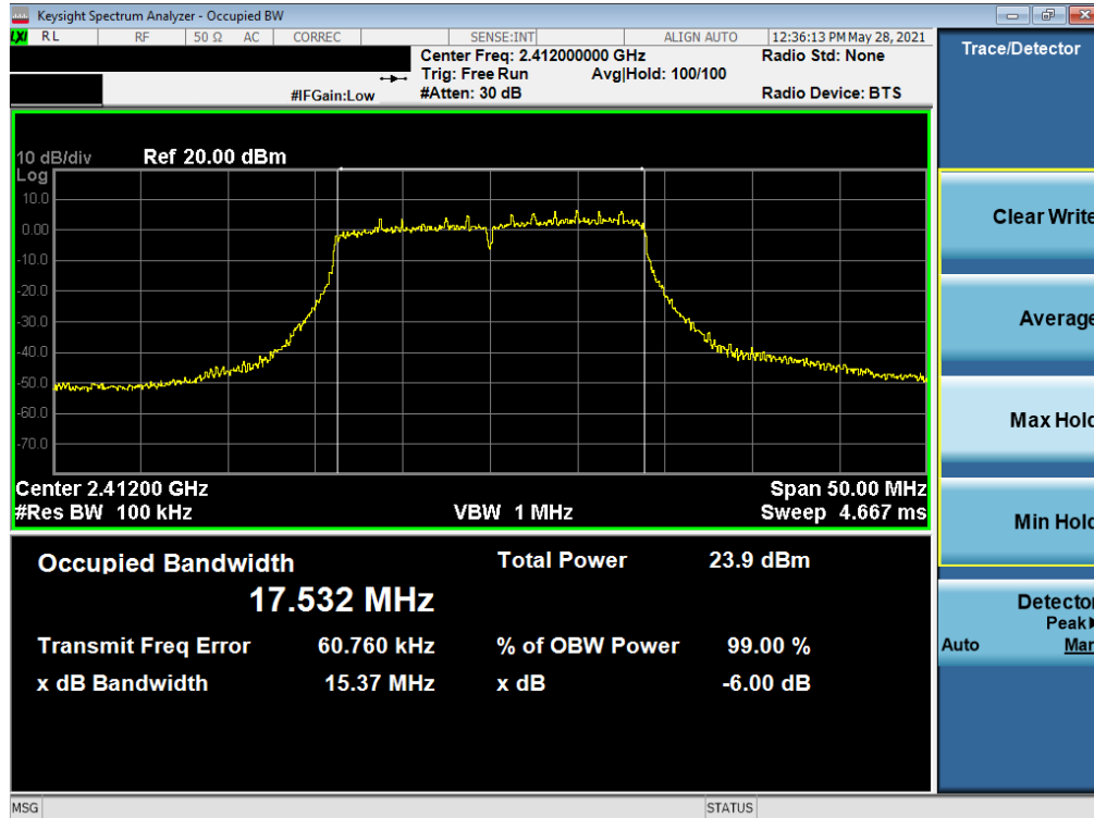
Plot 7-25. 6dB Bandwidth Plot SISO NORTH (802.11n 20MHz BW (2.4GHz) – Ch. 1)
