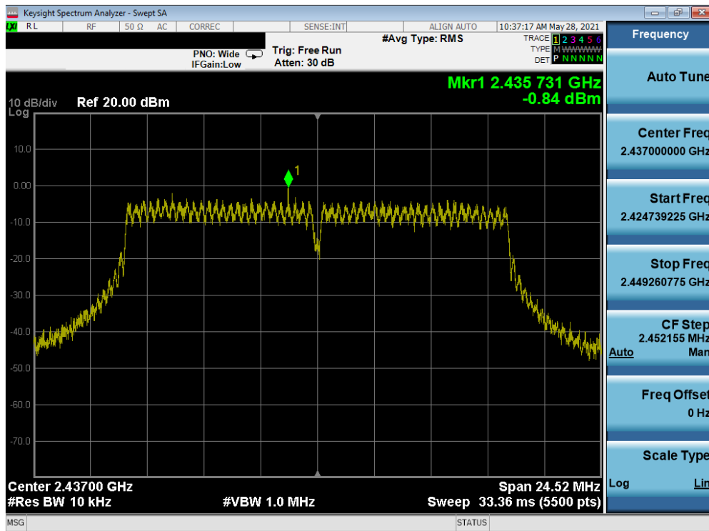
Plot 7-59. Power Spectral Density Plot SISO NORTH (802.11g – Ch. 6)
