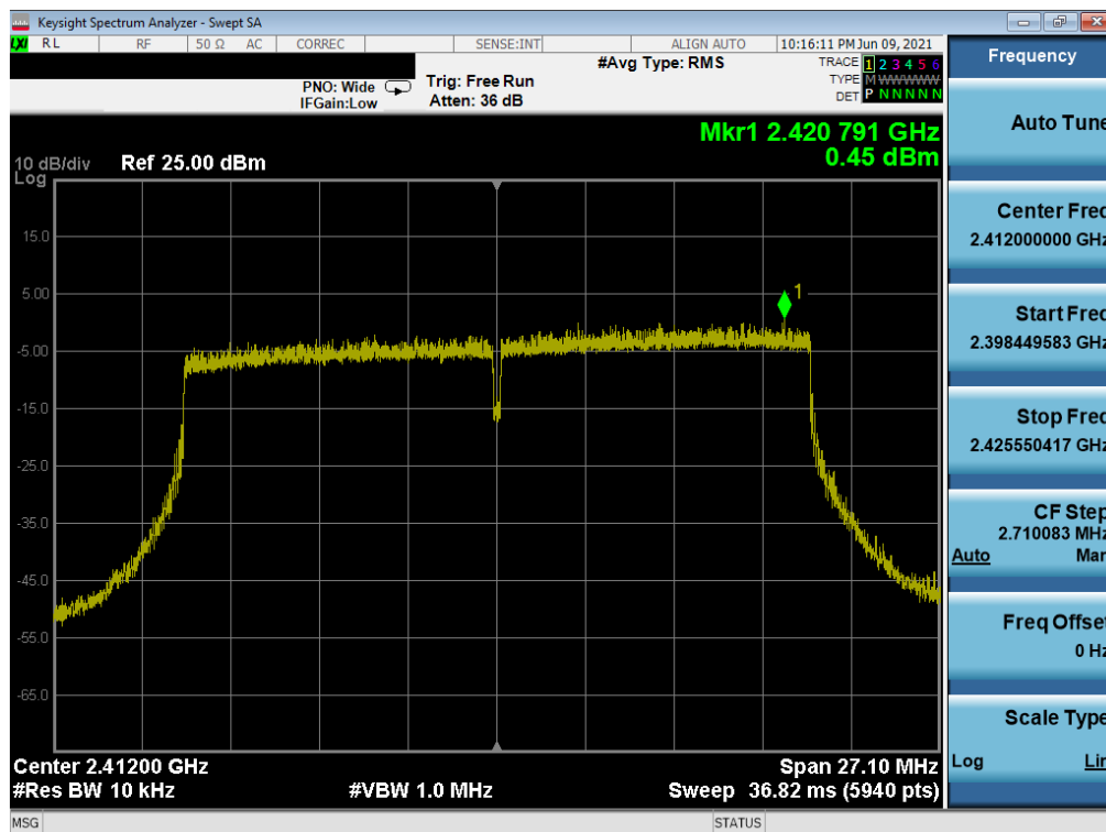
Plot 7-64. Power Spectral Density Plot SISO NORTH (802.11ax 20MHz BW (2.4GHz) – Ch. 1)
