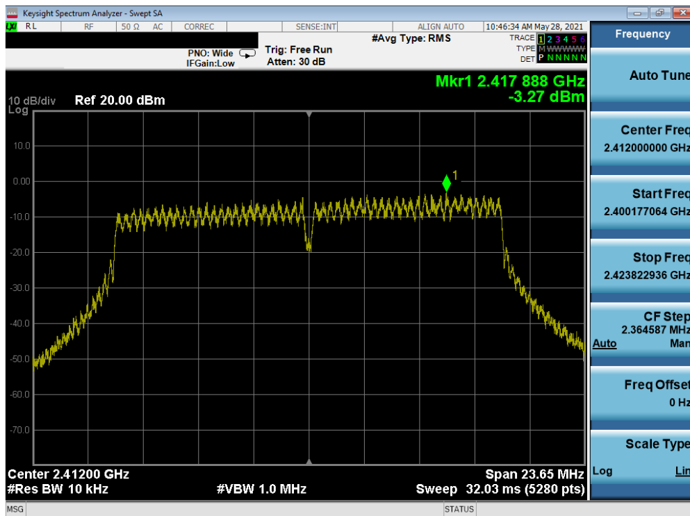
Plot 7-58. Power Spectral Density Plot SISO NORTH (802.11g – Ch. 1)
