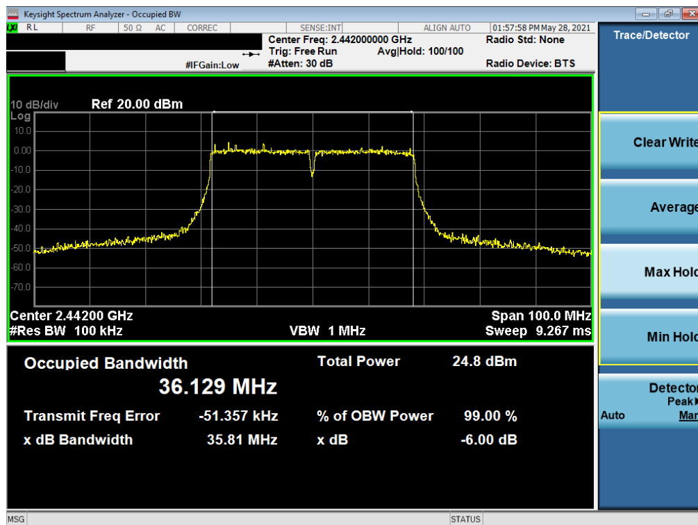
Plot 7-32. 6dB Bandwidth Plot SISO NORTH (802.11n 40MHz BW (2.4GHz) – Ch. 7)
