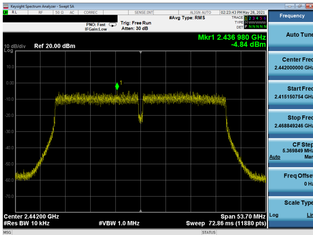
Plot 7-50. Power Spectral Density Plot SISO SOUTH (802.11n 40MHz BW (2.4GHz) – Ch. 7)
