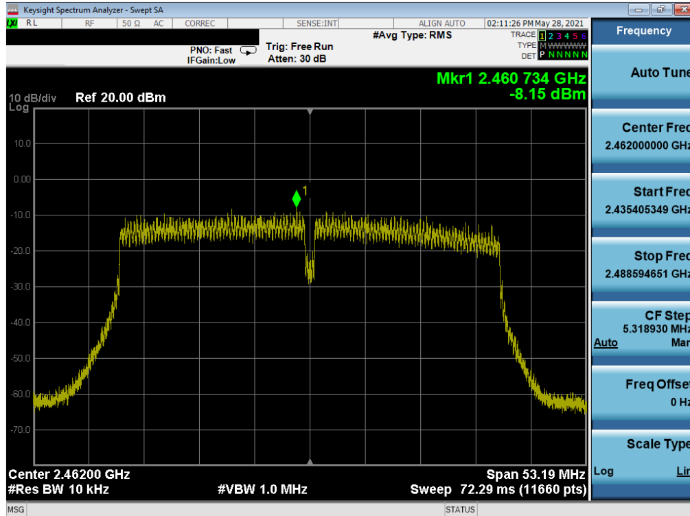
Plot 7-69. Power Spectral Density Plot SISO NORTH (802.11n 40MHz BW (2.4GHz) – Ch. 11)
