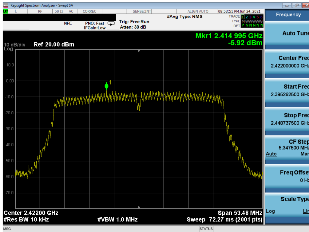
Plot 7-85. Power Spectral Density Plot MIMO SOUTH (802.11n 40MHz BW (2.4GHz) – Ch. 3)
