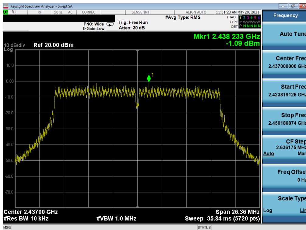
Plot 7-44. Power Spectral Density Plot SISO SOUTH (802.11n 20MHz BW (2.4GHz) – Ch. 6)
