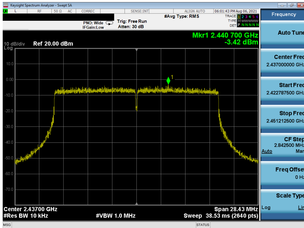
Plot 7-83. Power Spectral Density Plot MIMO SOUTH (802.11ax 20MHz BW (2.4GHz) – Ch. 6)
