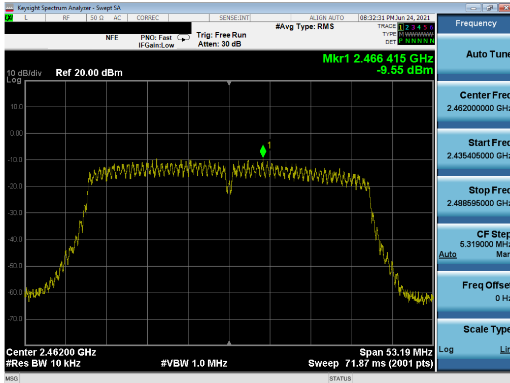
Plot 7-105. Power Spectral Density Plot MIMO NORTH (802.11n 40MHz BW (2.4GHz) – Ch. 11)
