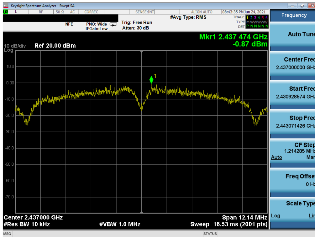
Plot 7-74. Power Spectral Density Plot MIMO SOUTH (802.11b – Ch. 6)
