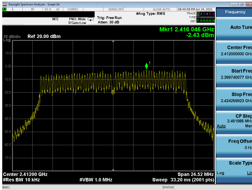
Plot 7-79. Power Spectral Density Plot MIMO SOUTH (802.11n 20MHz BW (2.4GHz) – Ch. 1)
