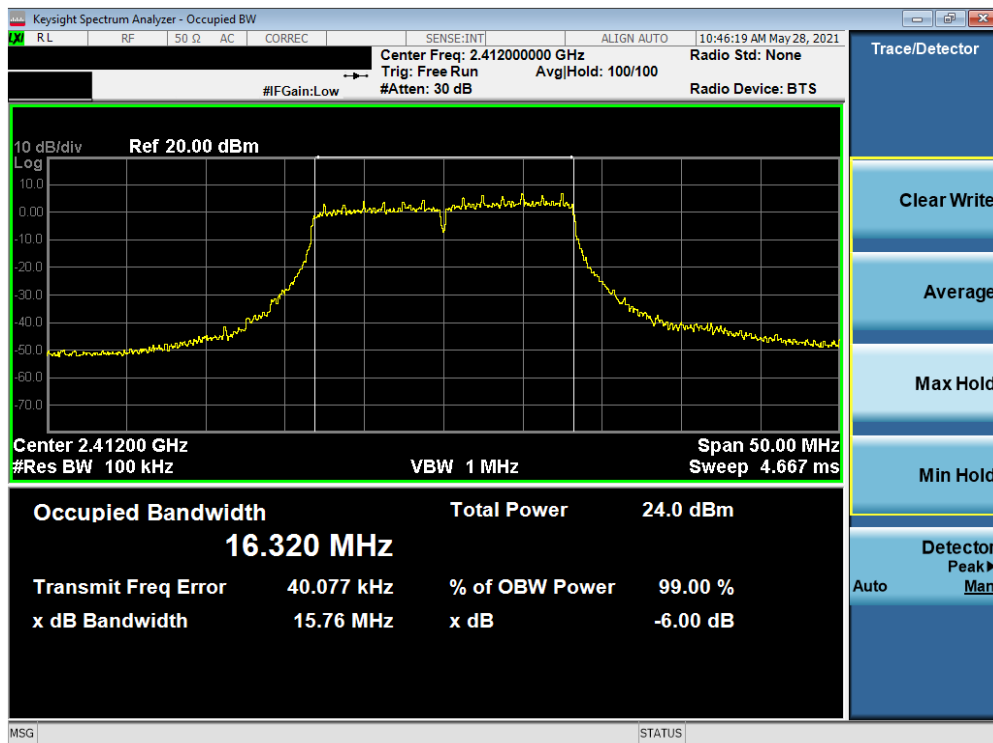
Plot 7-22. 6dB Bandwidth Plot SISO NORTH (802.11g – Ch. 1)
