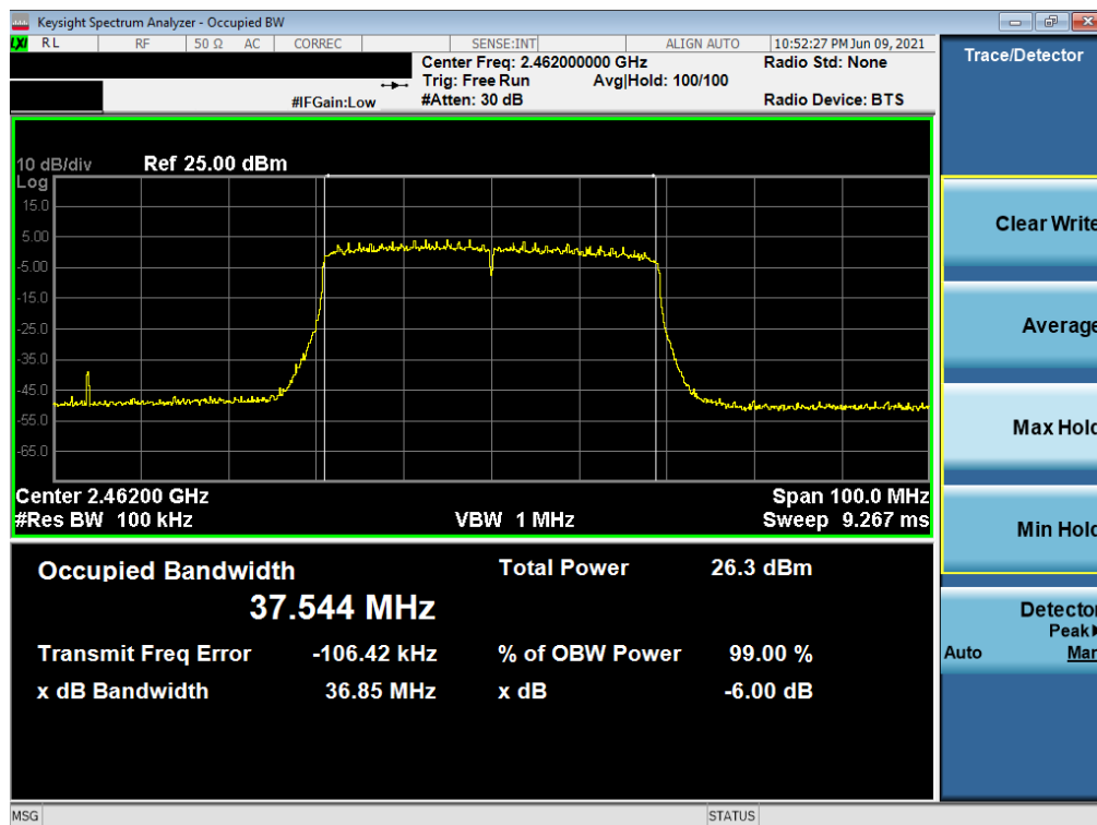
Plot 7-18. 6dB Bandwidth Plot SISO SOUTH (802.11ax 40MHz BW (2.4GHz) – Ch. 11)
