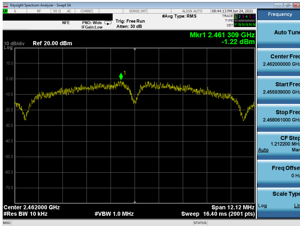
Plot 7-75. Power Spectral Density Plot MIMO SOUTH (802.11b – Ch. 11)
