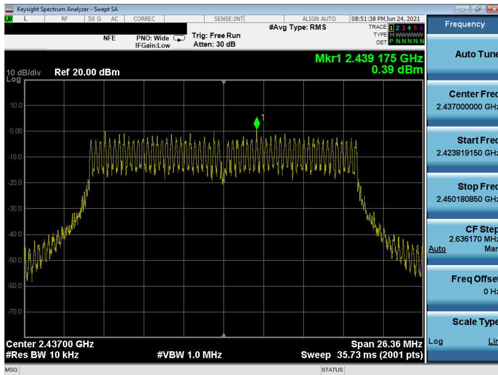
Plot 7-80. Power Spectral Density Plot MIMO SOUTH (802.11n 20MHz BW (2.4GHz) – Ch. 6)
