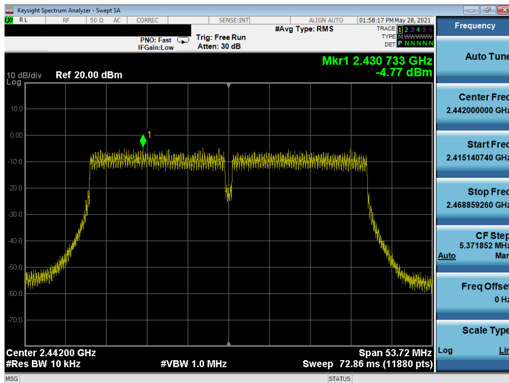
Plot 7-68. Power Spectral Density Plot SISO NORTH (802.11n 40MHz BW (2.4GHz) – Ch. 7)
