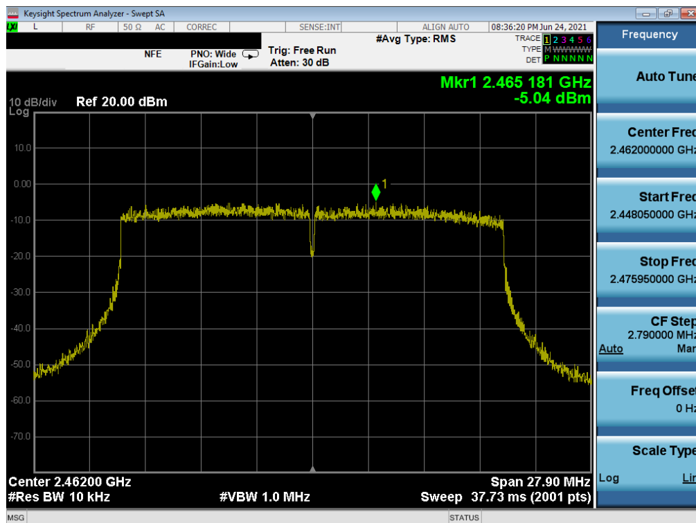
Plot 7-102. Power Spectral Density Plot MIMO NORTH (802.11ax 20MHz BW (2.4GHz) – Ch. 11)
