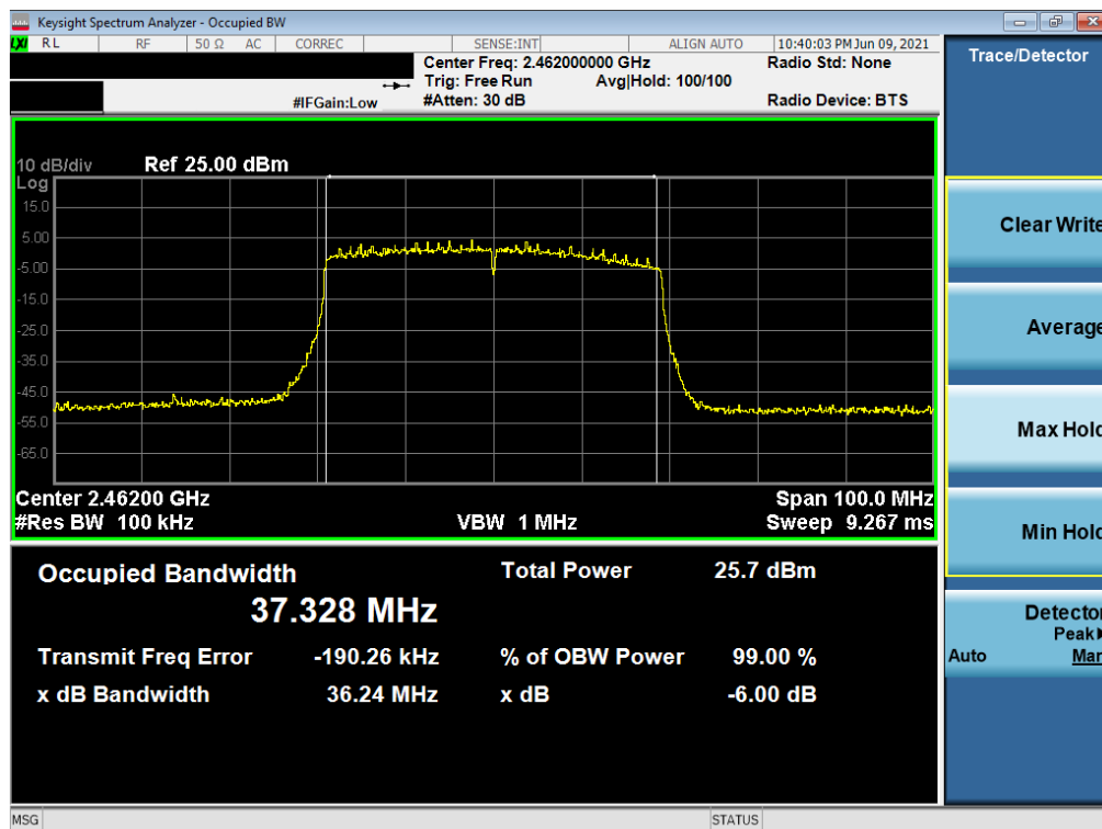
Plot 7-36. 6dB Bandwidth Plot SISO NORTH (802.11ax 40MHz BW (2.4GHz) – Ch. 11)
