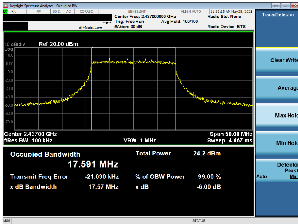
Plot 7-8. 6dB Bandwidth Plot SISO SOUTH (802.11n 20MHz BW (2.4GHz) – Ch. 6)
