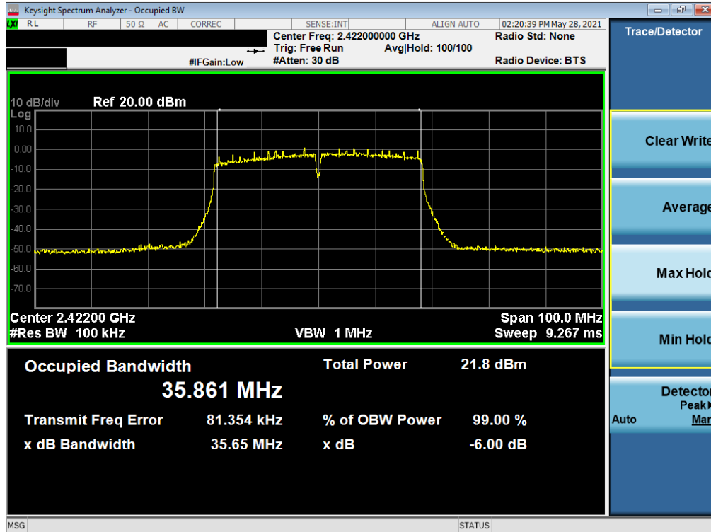
Plot 7-13. 6dB Bandwidth Plot SISO SOUTH (802.11n 40MHz BW (2.4GHz) – Ch. 3)
