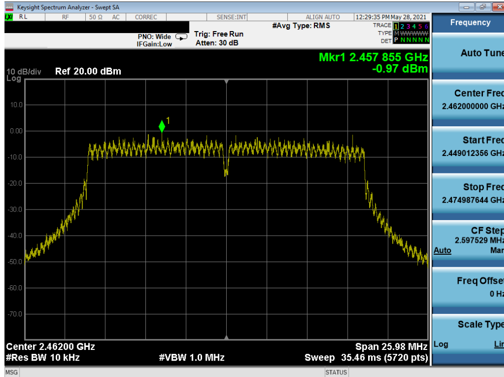
Plot 7-63. Power Spectral Density Plot SISO NORTH (802.11n 20MHz BW (2.4GHz) – Ch. 11)
