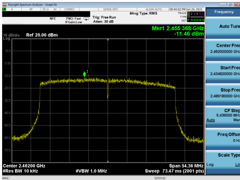
Plot 7-108. Power Spectral Density Plot MIMO NORTH (802.11ax 40MHz BW (2.4GHz) – Ch. 11)
