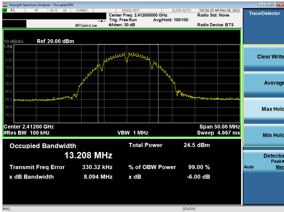
Plot 7-19. 6dB Bandwidth Plot SISO NORTH (802.11b – Ch. 1)
