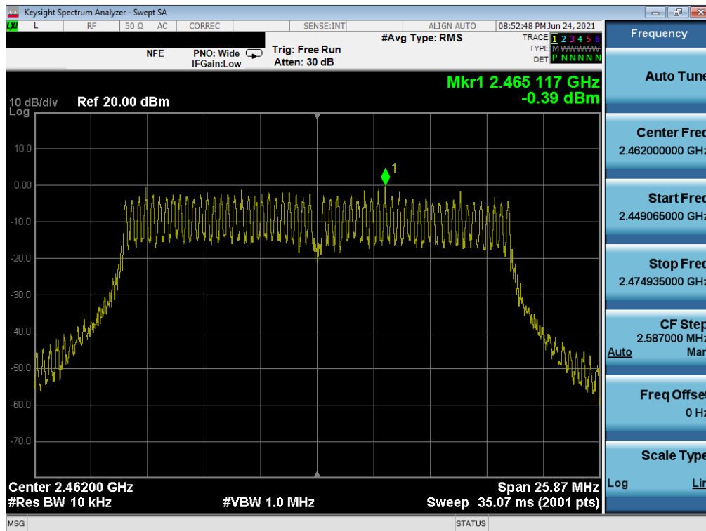
Plot 7-81. Power Spectral Density Plot MIMO SOUTH (802.11n 20MHz BW (2.4GHz) – Ch. 11)
