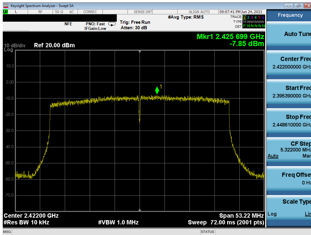
Plot 7-88. Power Spectral Density Plot MIMO SOUTH (802.11ax 40MHz BW (2.4GHz) – Ch. 3)
