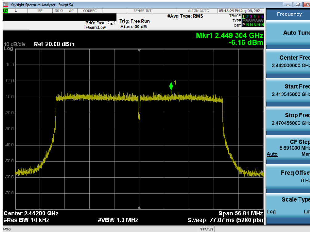
Plot 7-107. Power Spectral Density Plot MIMO NORTH (802.11ax 40MHz BW (2.4GHz) – Ch. 7)
