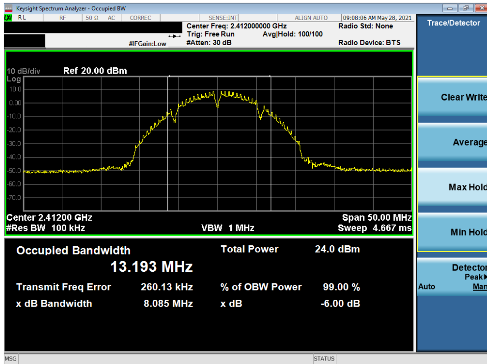
Plot 7-1. 6dB Bandwidth Plot SISO SOUTH (802.11b – Ch. 1)
