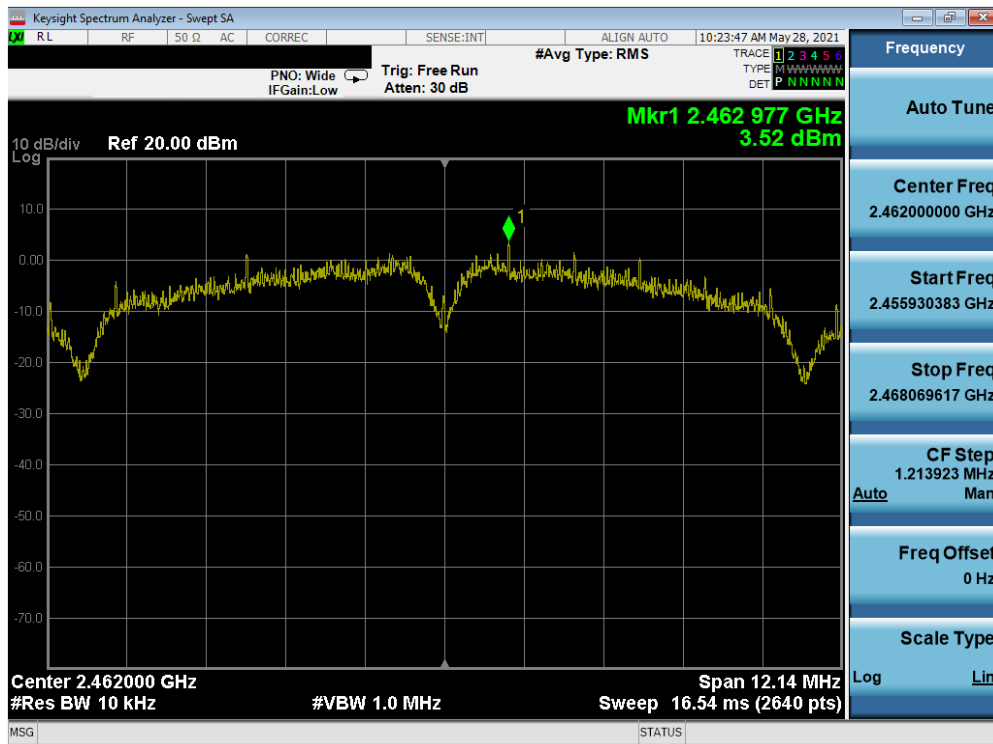
Plot 7-57. Power Spectral Density Plot SISO NORTH (802.11b – Ch. 11)
