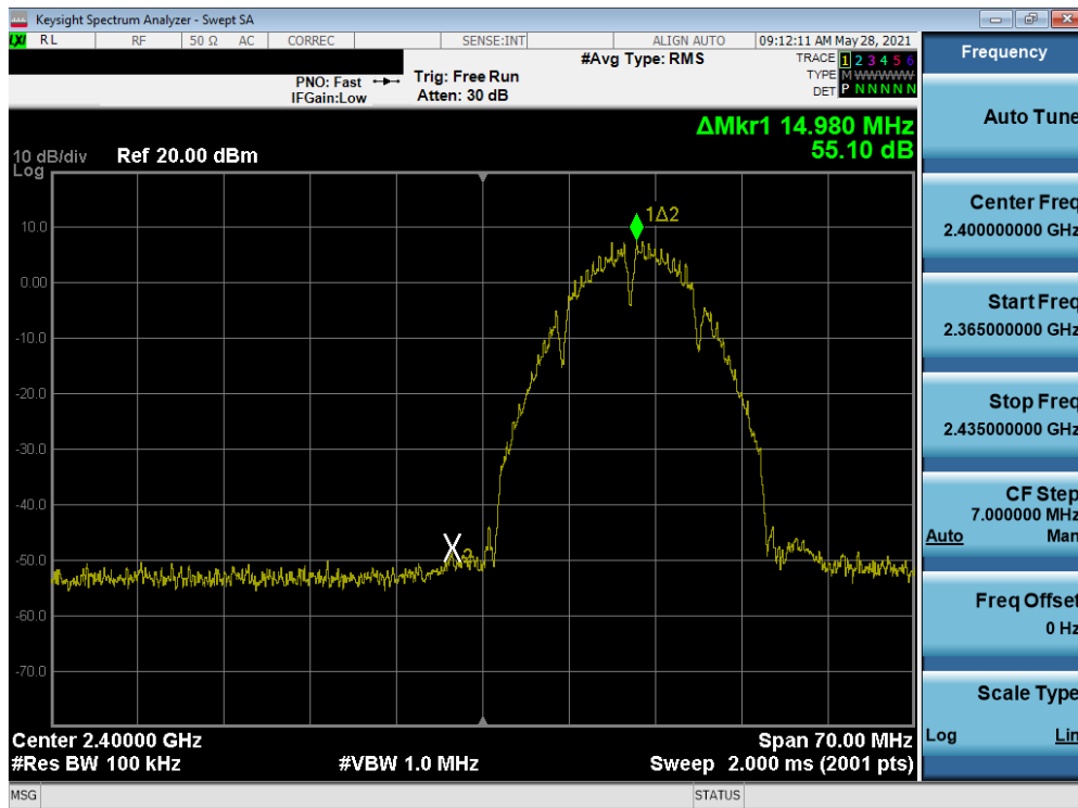
Plot 7-109. Band Edge Plot SISO SOUTH (802.11b – Ch. 1)
