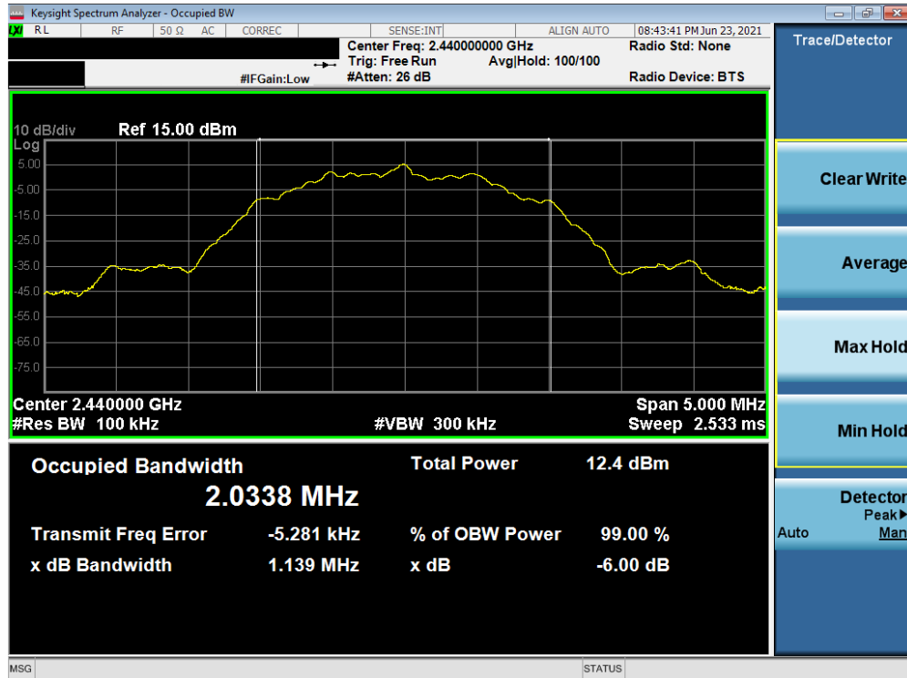
Plot 7-23. 6dB Bandwidth Plot (Bluetooth (LE), 2Mbps – Ch. 19) – North Antenna
