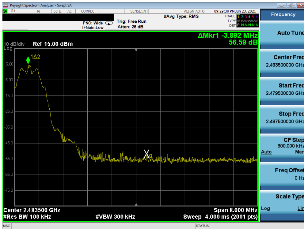
Plot 7-74. Band Edge Plot (Bluetooth (LE), 125kbps – Ch. 39) – South Antenna
