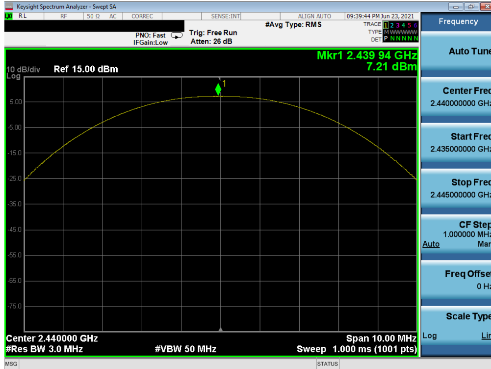
Plot 7-29. Peak Power Plot (Bluetooth (LE), 500kbps – Ch. 19) – South Antenna
