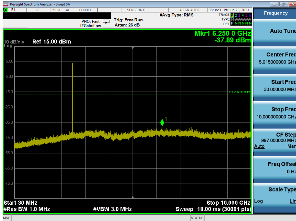
Plot 7-99. Conducted Spurious Plot (Bluetooth (LE), 1Mbps - Ch. 39) - North Antenna
