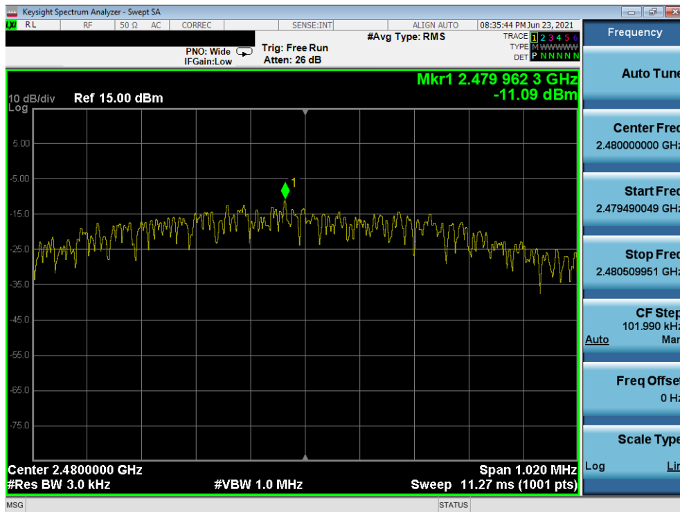
Plot 7-69. Power Spectral Density Plot (Bluetooth (LE), 1Mbps – Ch. 39) – North Antenna
