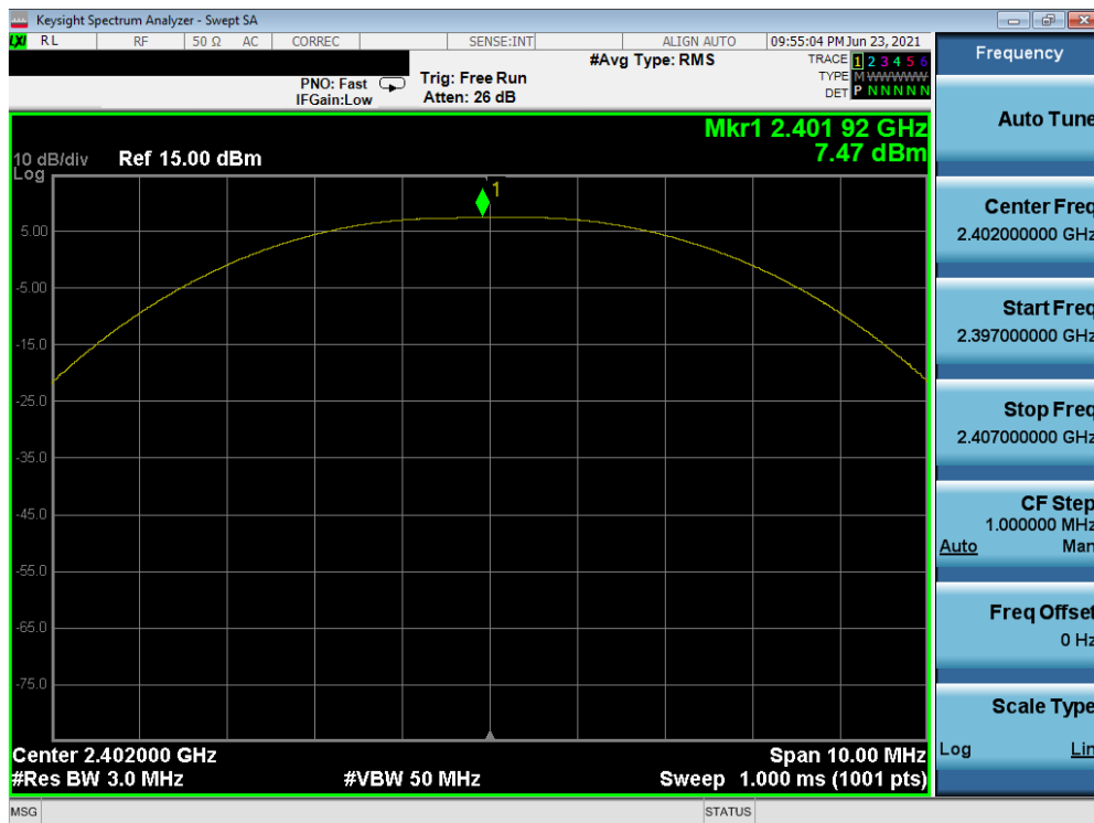
Plot 7-34. Peak Power Plot (Bluetooth (LE), 2Mbps - Ch. 0) - South Antenna
