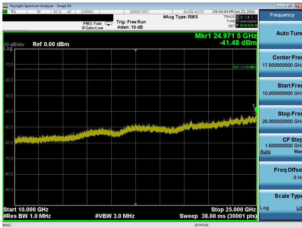
Plot 7-90. Conducted Spurious Plot (Bluetooth (LE), 1Mbps – Ch. 0) – South Antenna
