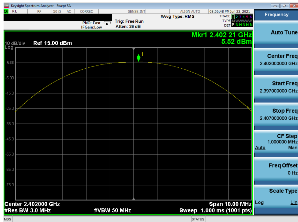
Plot 7-40. Peak Power Plot (Bluetooth (LE), 500kbps – Ch. 0) – North Antenna
