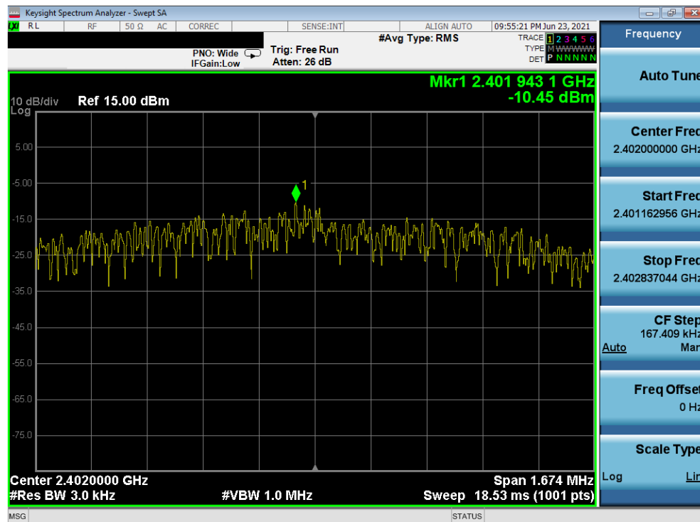
Plot 7-58. Power Spectral Density Plot (Bluetooth (LE), 2Mbps – Ch. 0) – South Antenna
