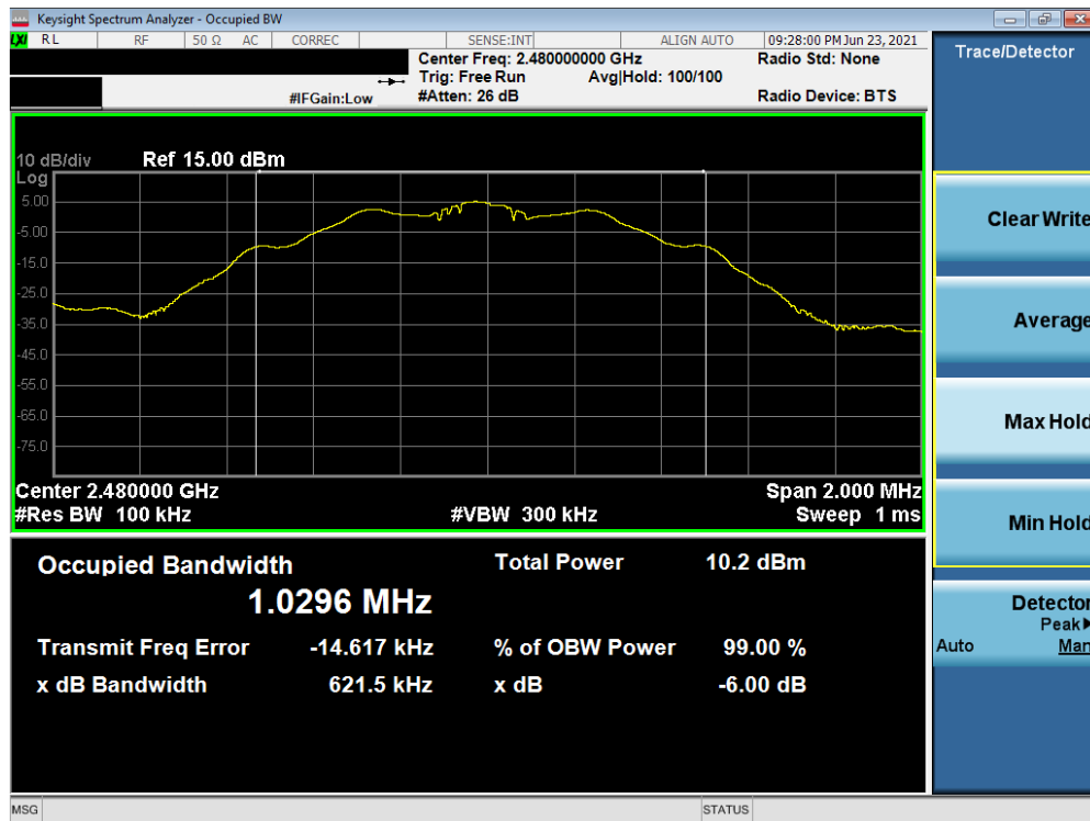
Plot 7-3. 6dB Bandwidth Plot (Bluetooth (LE), 125kbps – Ch. 39) – South Antenna
