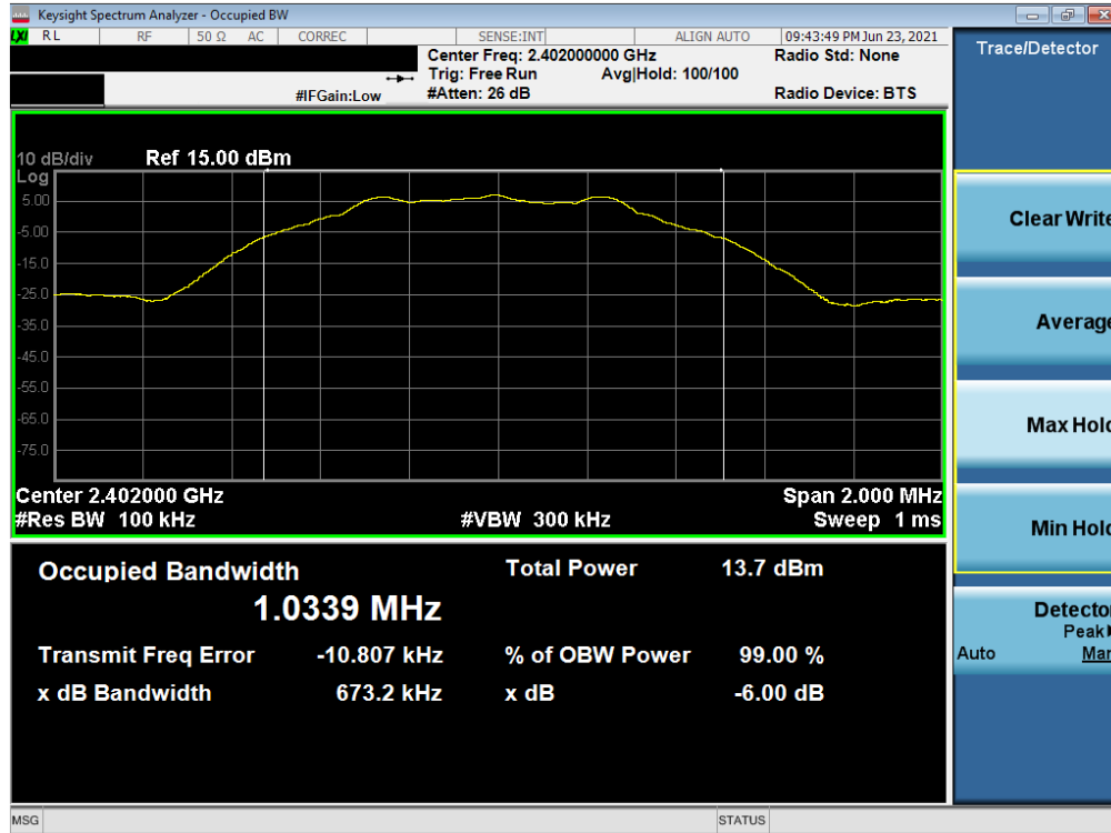
Plot 7-7. 6dB Bandwidth Plot (Bluetooth (LE), 1Mbps – Ch. 0) – South Antenna
