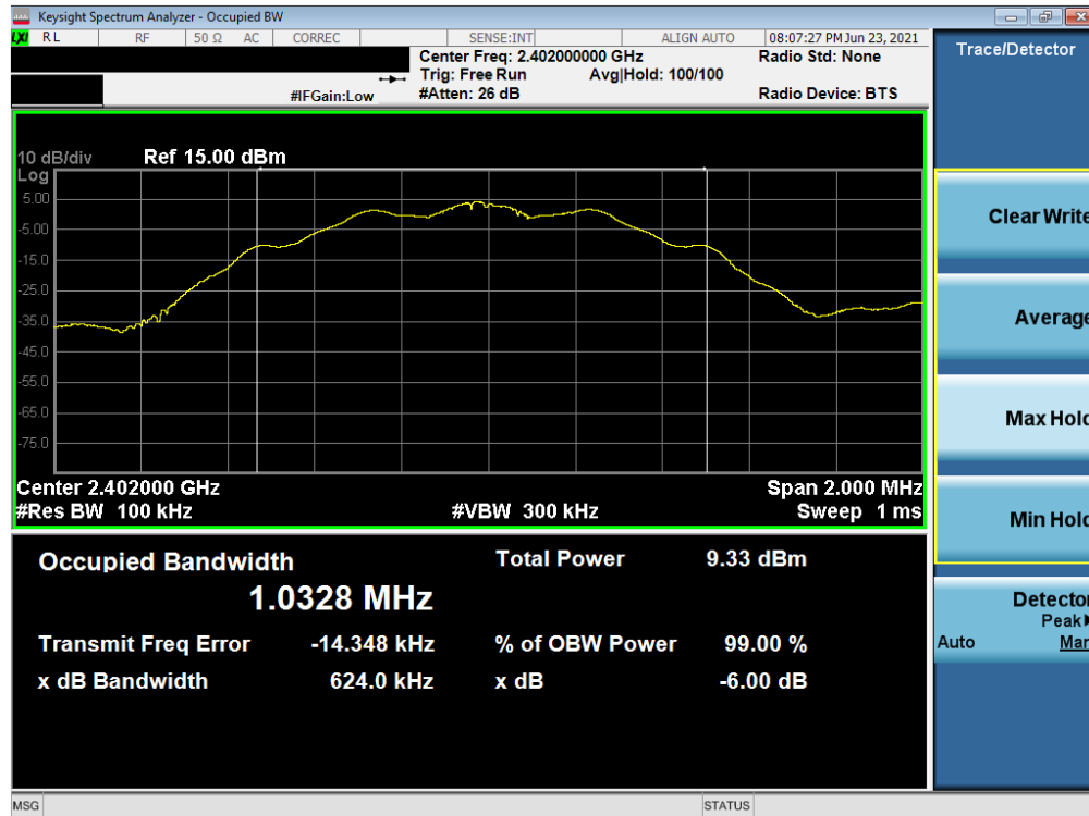
Plot 7-13. 6dB Bandwidth Plot (Bluetooth (LE), 125kbps – Ch. 0) – North Antenna
