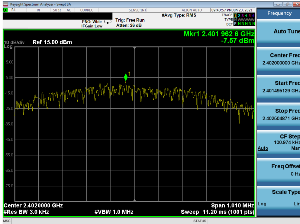
Plot 7-55. Power Spectral Density Plot (Bluetooth (LE), 1Mbps – Ch. 0) – South Antenna
