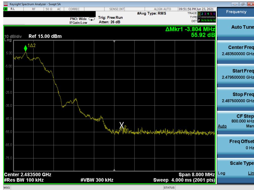
Plot 7-80. Band Edge Plot (Bluetooth (LE), 2Mbps – Ch. 39) – South Antenna
