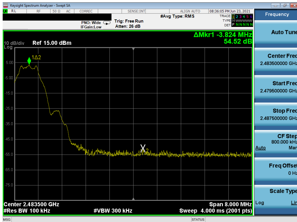
Plot 7-86. Band Edge Plot (Bluetooth (LE), 1Mbps - Ch. 39) - North Antenna
