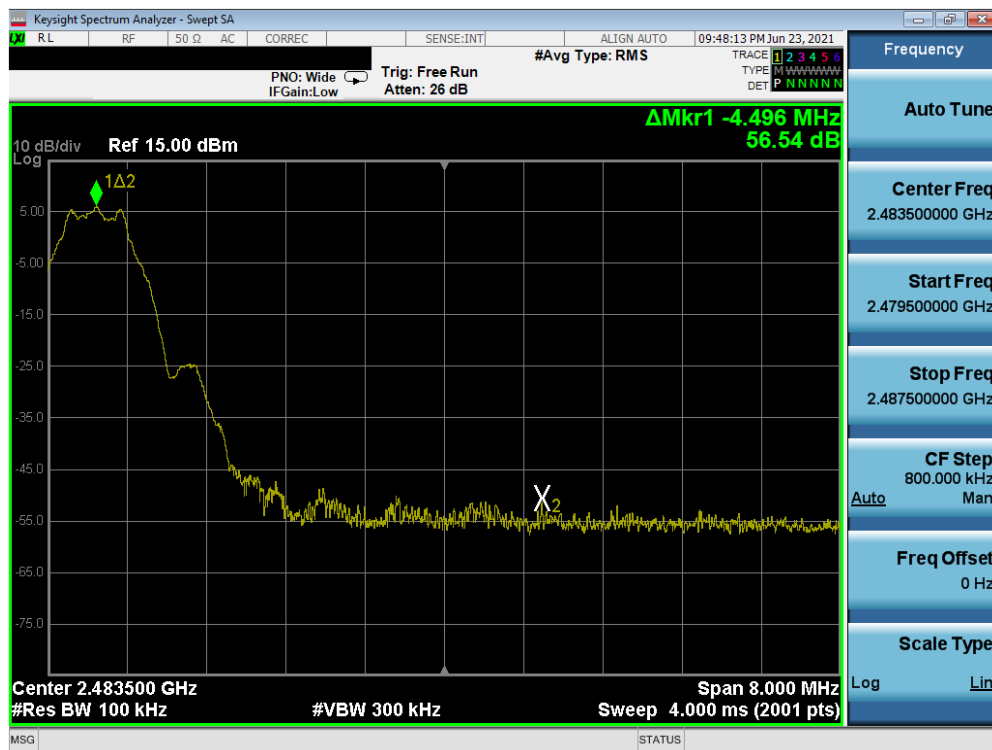
Plot 7-78. Band Edge Plot (Bluetooth (LE), 1Mbps – Ch. 39) – South Antenna
