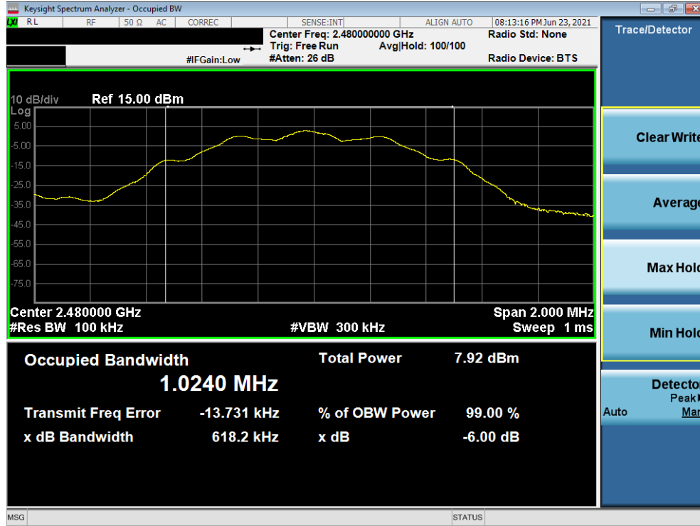
Plot 7-15. 6dB Bandwidth Plot (Bluetooth (LE), 125kbps – Ch. 39) – North Antenna
