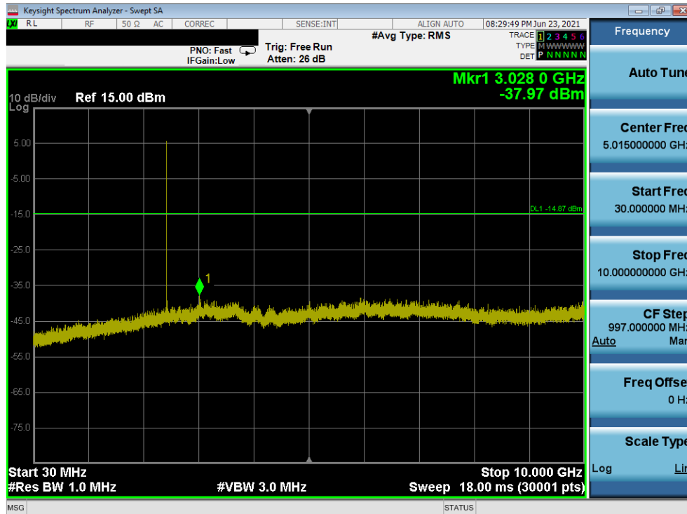
Plot 7-97. Conducted Spurious Plot (Bluetooth (LE), 1Mbps – Ch. 19) – North Antenna
