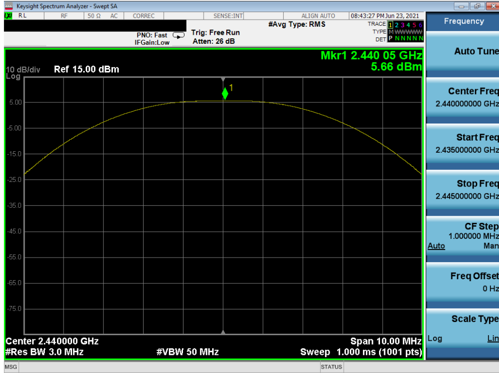
Plot 7-47. Peak Power Plot (Bluetooth (LE), 2Mbps – Ch. 19) – North Antenna
