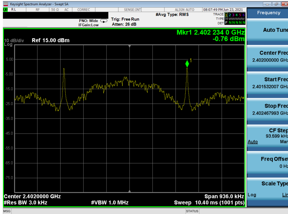
Plot 7-61. Power Spectral Density Plot (Bluetooth (LE), 125kbps – Ch. 0) – North Antenna
