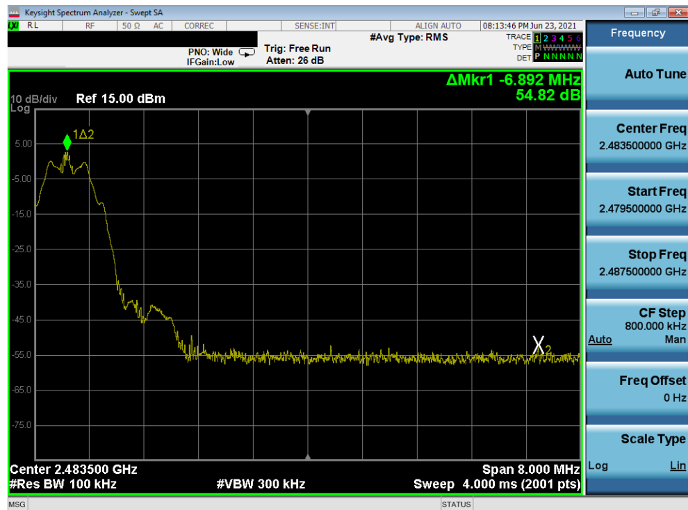
Plot 7-82. Band Edge Plot (Bluetooth (LE), 125kbps - Ch. 39) - North Antenna
