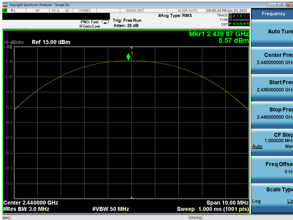
Plot 7-38. Peak Power Plot (Bluetooth (LE), 125kbps – Ch. 19) – North Antenna
