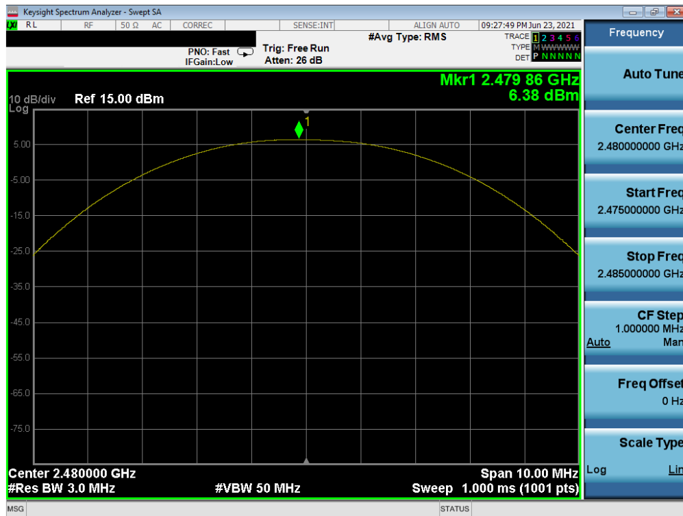
Plot 7-27. Peak Power Plot (Bluetooth (LE), 125kbps – Ch. 39) – South Antenna
