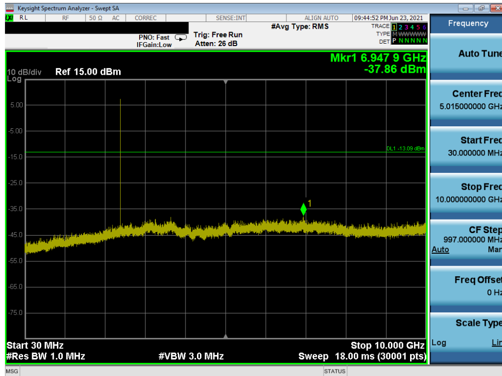
Plot 7-89. Conducted Spurious Plot (Bluetooth (LE), 1Mbps – Ch. 0) – South Antenna
