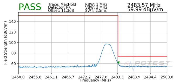
Plot 7-104. Radiated Restricted Upper Band Edge Measurement (Peak) – North Antenna
