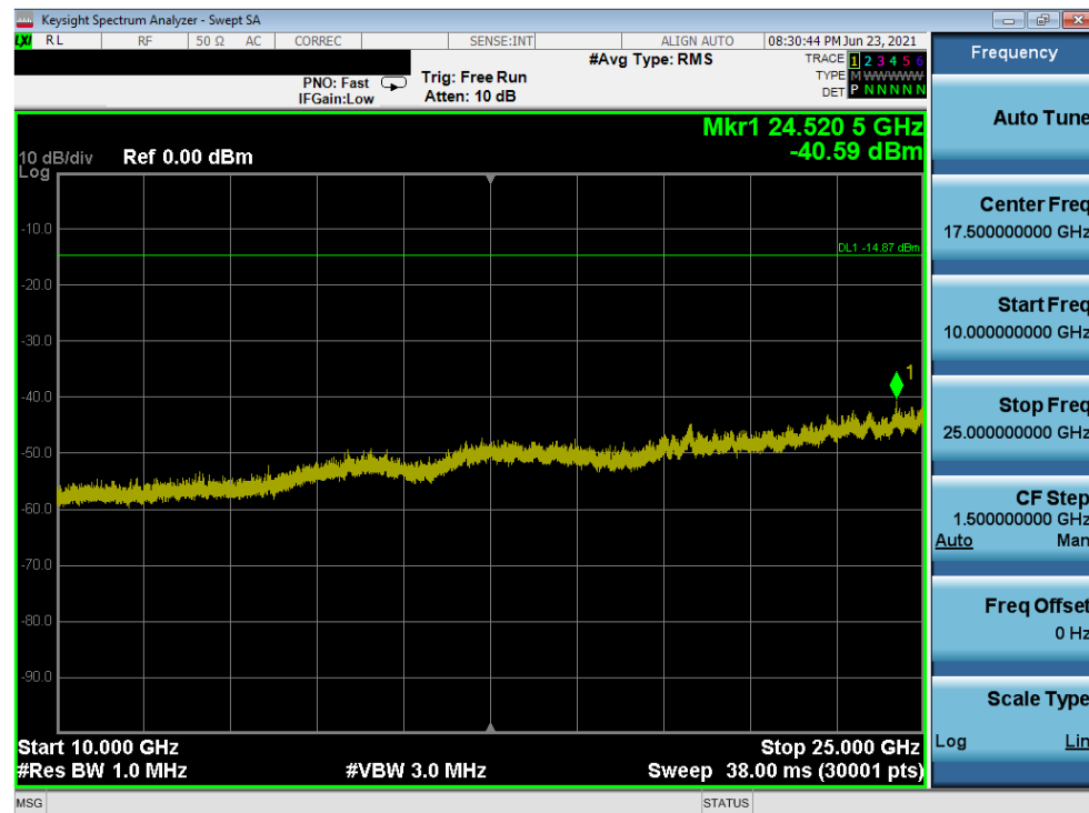
Plot 7-98. Conducted Spurious Plot (Bluetooth (LE), 1Mbps – Ch. 19) – North Antenna
