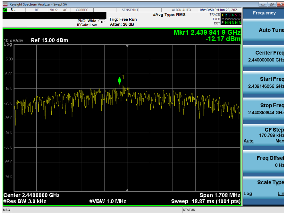
Plot 7-71. Power Spectral Density Plot (Bluetooth (LE), 2Mbps – Ch. 19) – North Antenna
