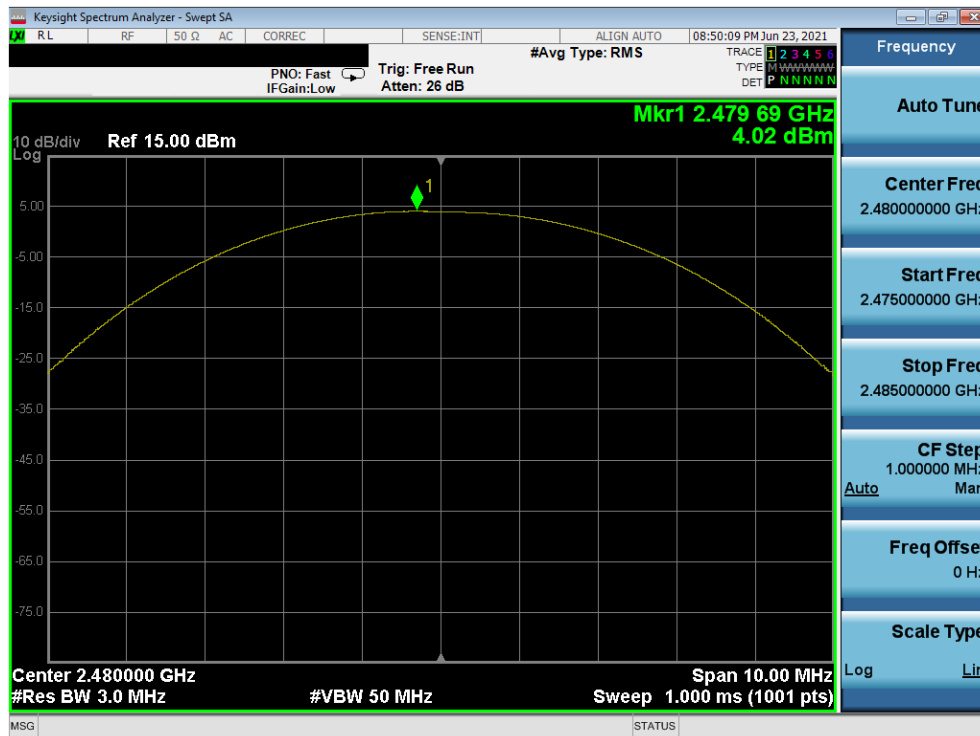
Plot 7-45. Peak Power Plot (Bluetooth (LE), 1Mbps – Ch. 39) – North Antenna
