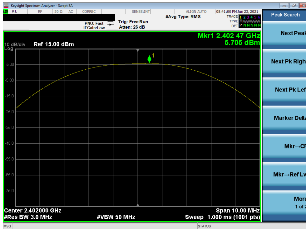
Plot 7-46. Peak Power Plot (Bluetooth (LE), 2Mbps – Ch. 0) – North Antenna
