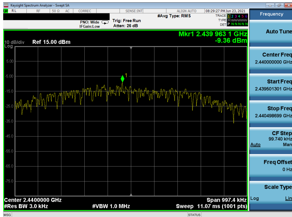
Plot 7-68. Power Spectral Density Plot (Bluetooth (LE), 1Mbps – Ch. 19) – North Antenna
