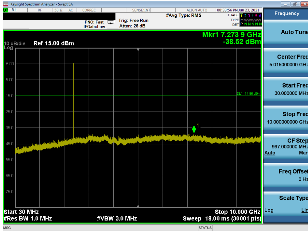
Plot 7-95. Conducted Spurious Plot (Bluetooth (LE), 1Mbps – Ch. 0) – North Antenna
