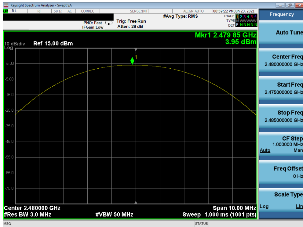
Plot 7-39. Peak Power Plot (Bluetooth (LE), 125kbps – Ch. 39) – North Antenna
