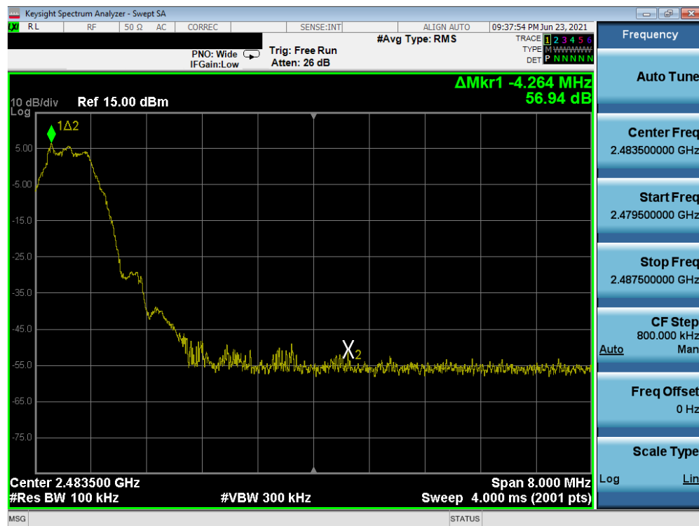
Plot 7-76. Band Edge Plot (Bluetooth (LE), 500kbps - Ch. 39) - South Antenna
