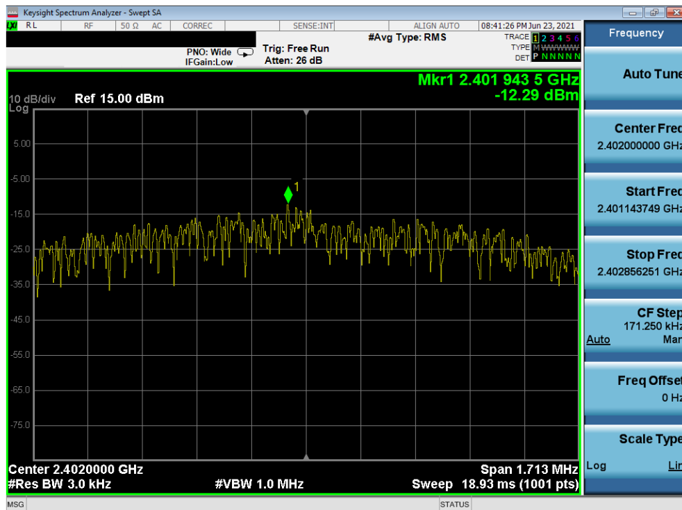
Plot 7-70. Power Spectral Density Plot (Bluetooth (LE), 2Mbps – Ch. 0) – North Antenna
