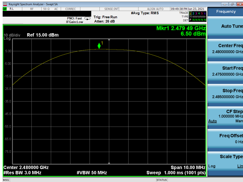
Plot 7-36. Peak Power Plot (Bluetooth (LE), 2Mbps – Ch. 39) – South Antenna
