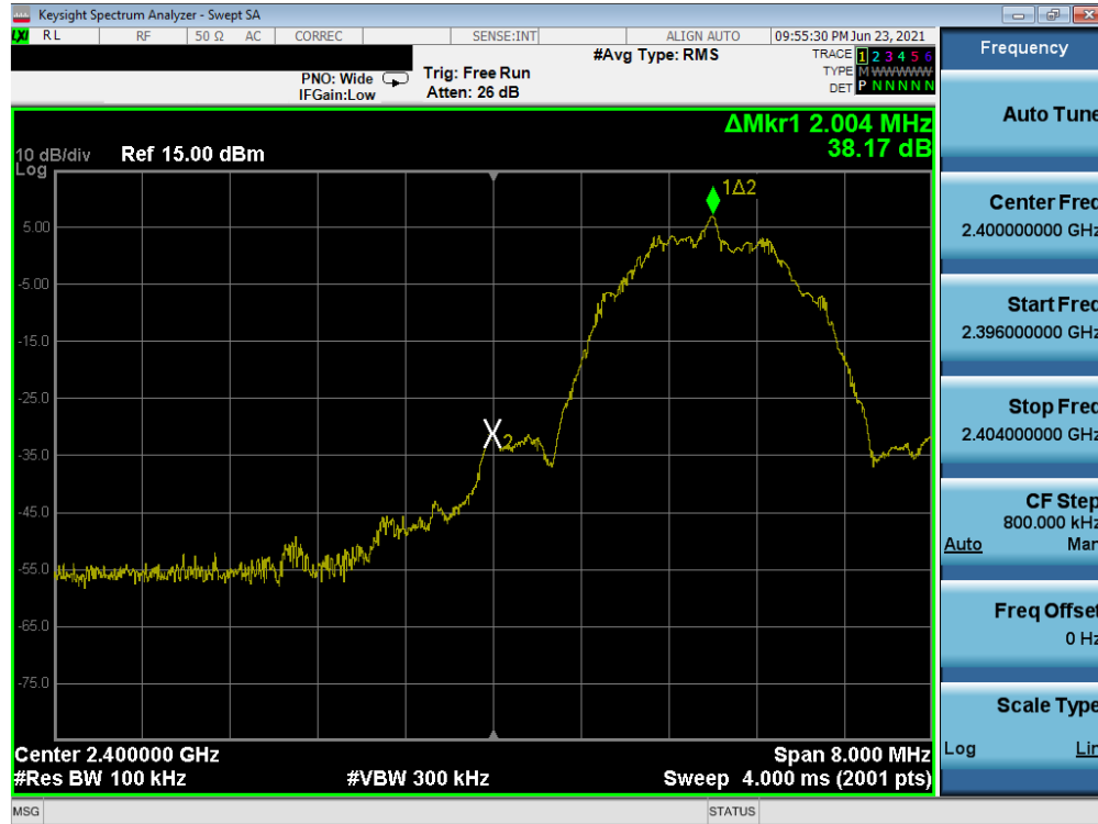
Plot 7-79. Band Edge Plot (Bluetooth (LE), 2Mbps – Ch. 0) – South Antenna
