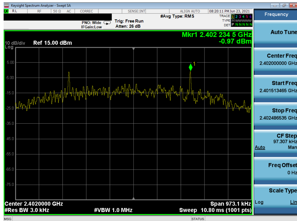
Plot 7-64. Power Spectral Density Plot (Bluetooth (LE), 500kbps – Ch. 0) – North Antenna
