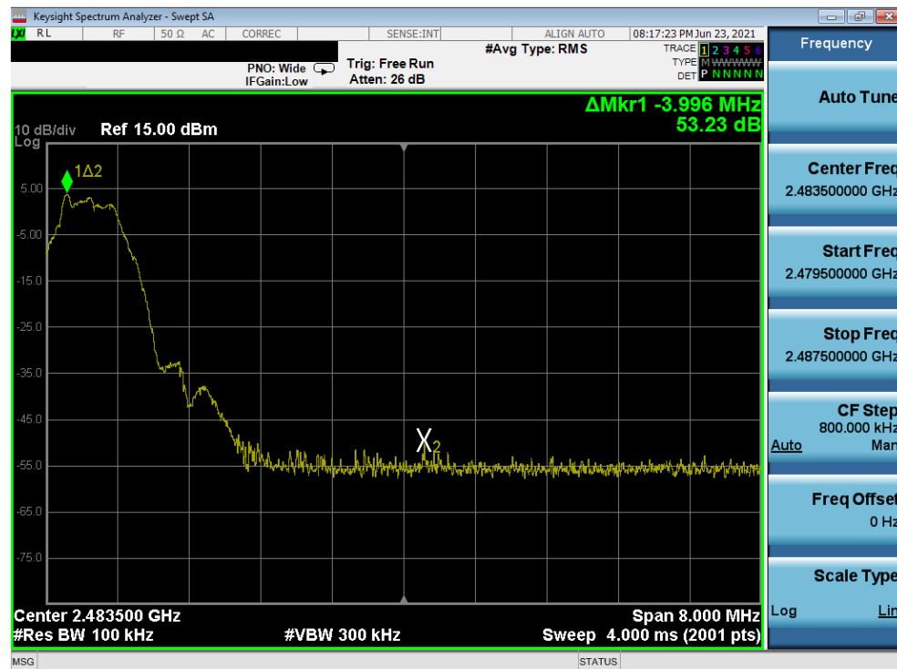
Plot 7-84. Band Edge Plot (Bluetooth (LE), 500kbps – Ch. 39) – North Antenna
