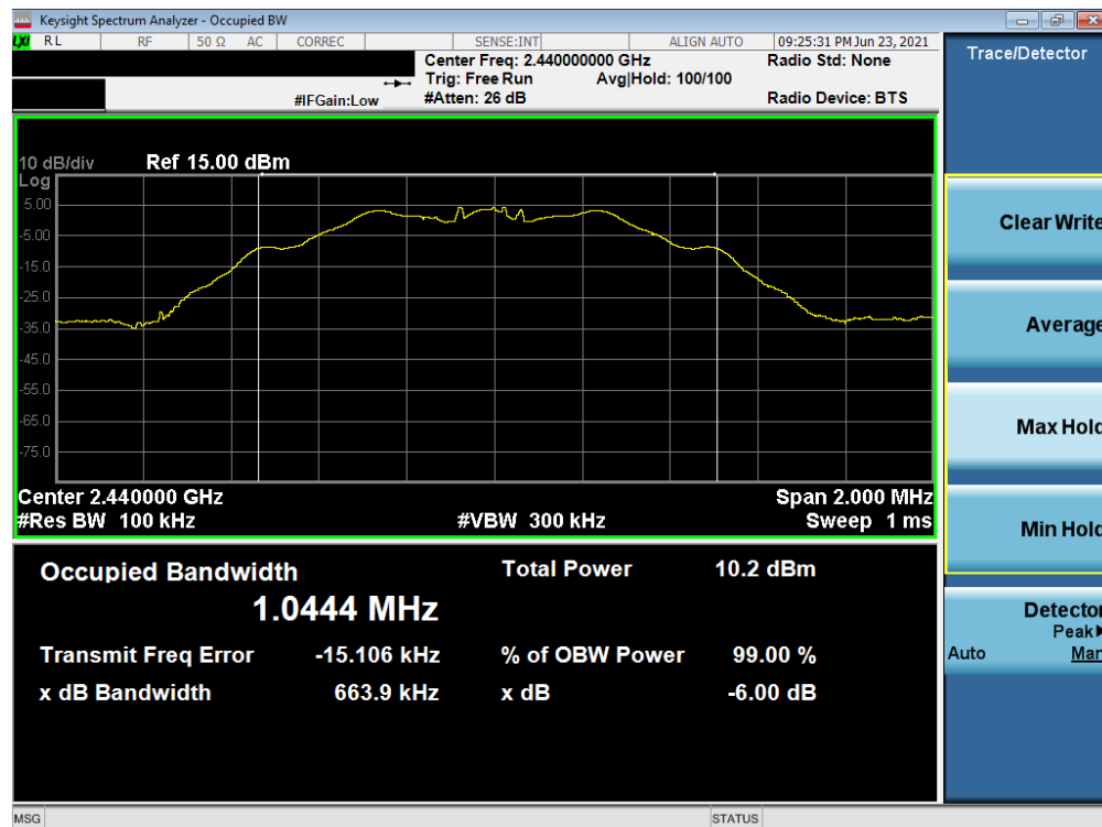
Plot 7-2. 6dB Bandwidth Plot (Bluetooth (LE), 125kbps – Ch. 19) – South Antenna
