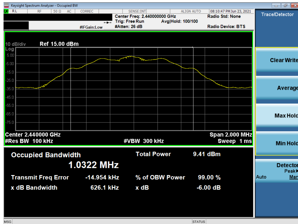
Plot 7-14. 6dB Bandwidth Plot (Bluetooth (LE), 125kbps – Ch. 19) – North Antenna
