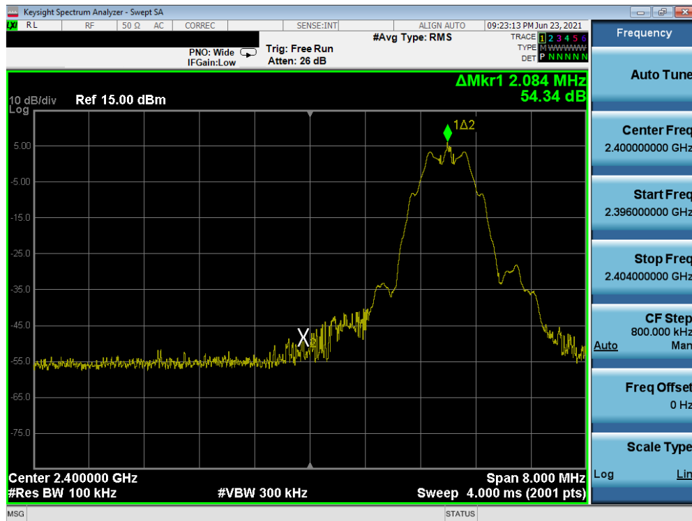
Plot 7-73. Band Edge Plot (Bluetooth (LE), 125kbps – Ch. 0) – South Antenna
