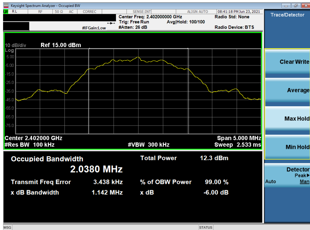
Plot 7-22. 6dB Bandwidth Plot (Bluetooth (LE), 2Mbps – Ch. 0) – North Antenna
