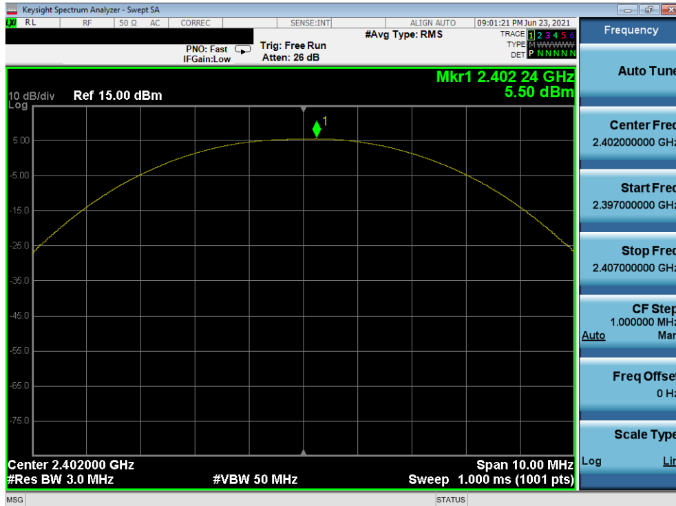
Plot 7-37. Peak Power Plot (Bluetooth (LE), 125kbps – Ch. 0) – North Antenna
