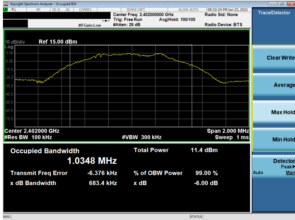
Plot 7-19. 6dB Bandwidth Plot (Bluetooth (LE), 1Mbps – Ch. 0) – North Antenna
