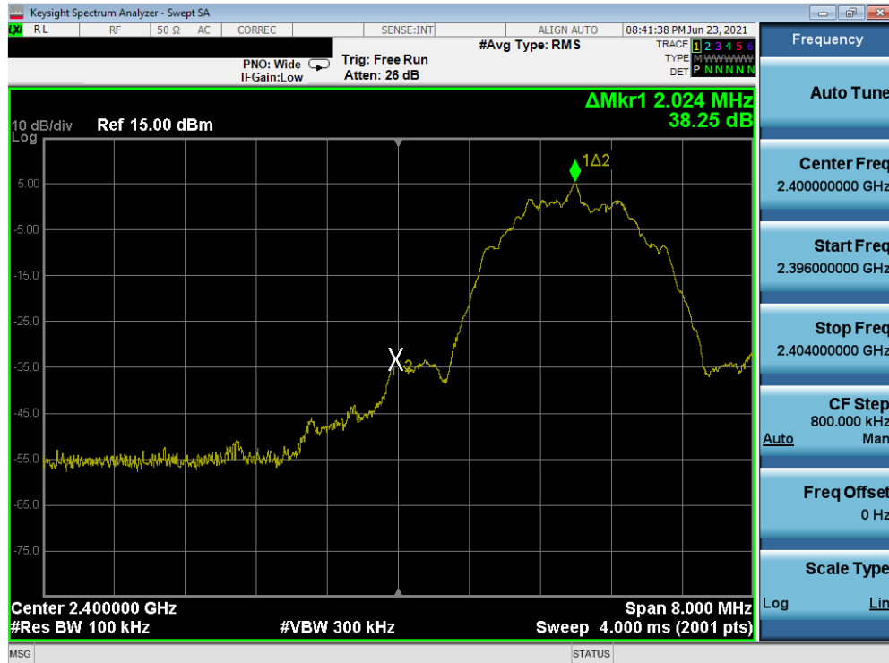
Plot 7-87. Band Edge Plot (Bluetooth (LE), 2Mbps – Ch. 0) – North Antenna
