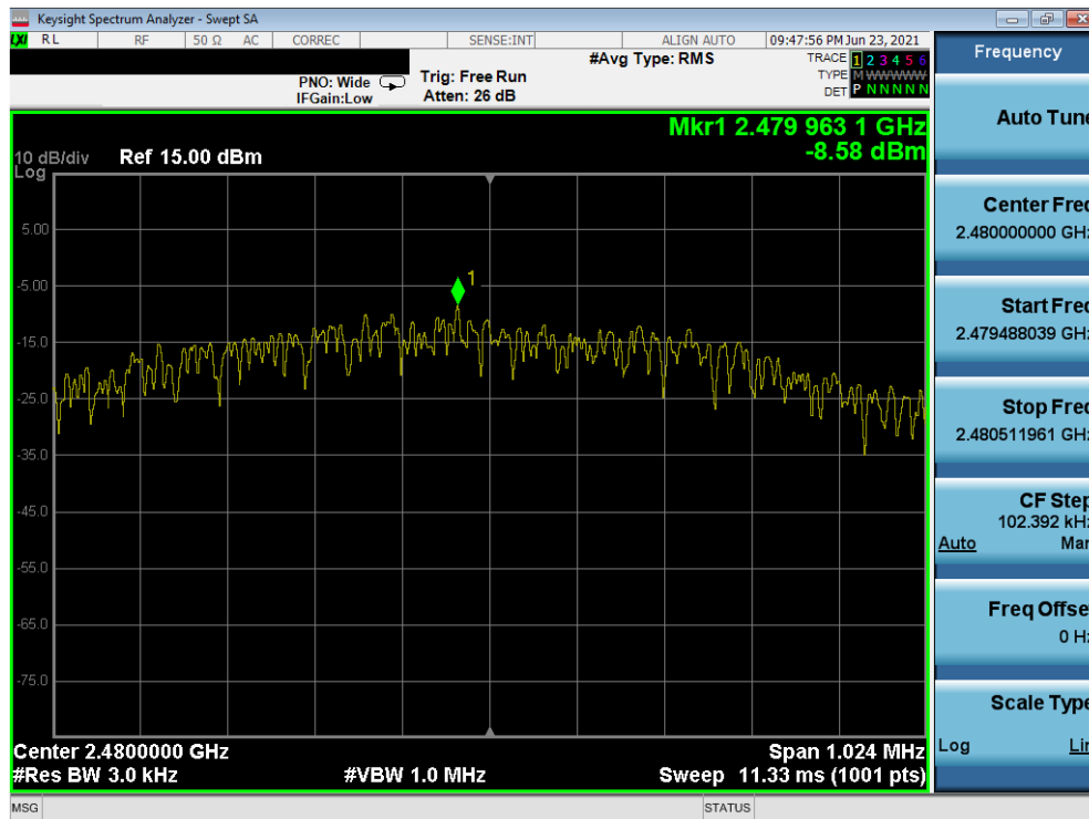
Plot 7-57. Power Spectral Density Plot (Bluetooth (LE), 1Mbps – Ch. 39) – South Antenna
