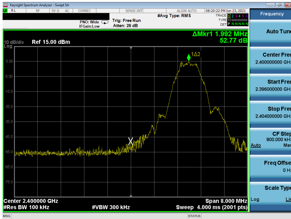
Plot 7-83. Band Edge Plot (Bluetooth (LE), 500kbps – Ch. 0) – North Antenna
