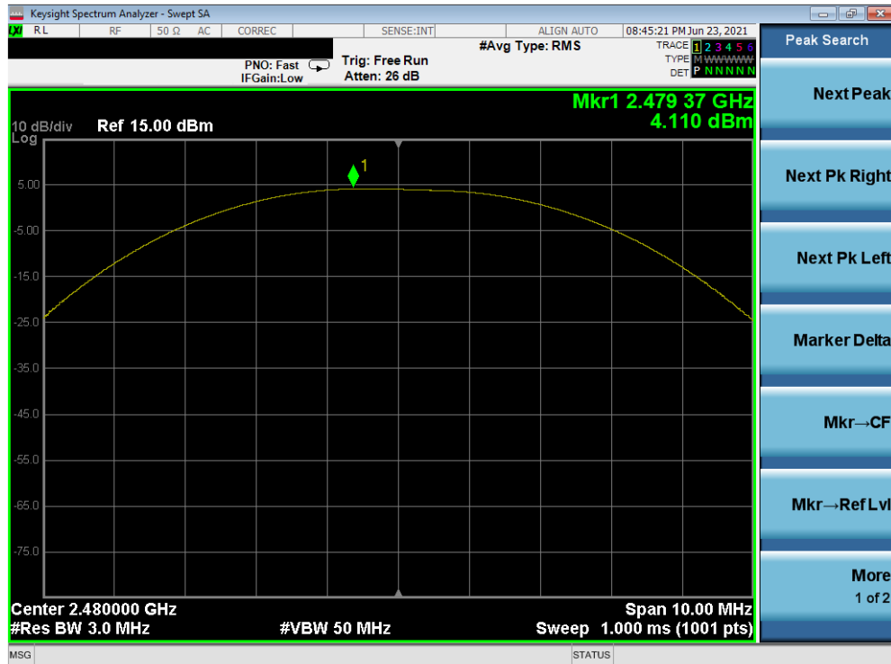
Plot 7-48. Peak Power Plot (Bluetooth (LE), 2Mbps – Ch. 39) – North Antenna
