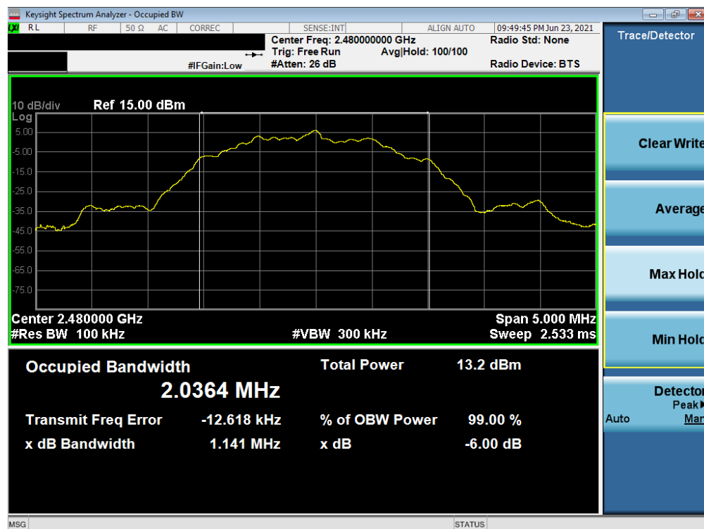
Plot 7-12. 6dB Bandwidth Plot (Bluetooth (LE), 2Mbps – Ch. 39) – South Antenna
