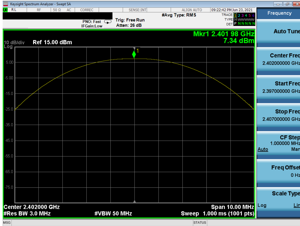
Plot 7-25. Peak Power Plot (Bluetooth (LE), 125kbps – Ch. 0) – South Antenna
