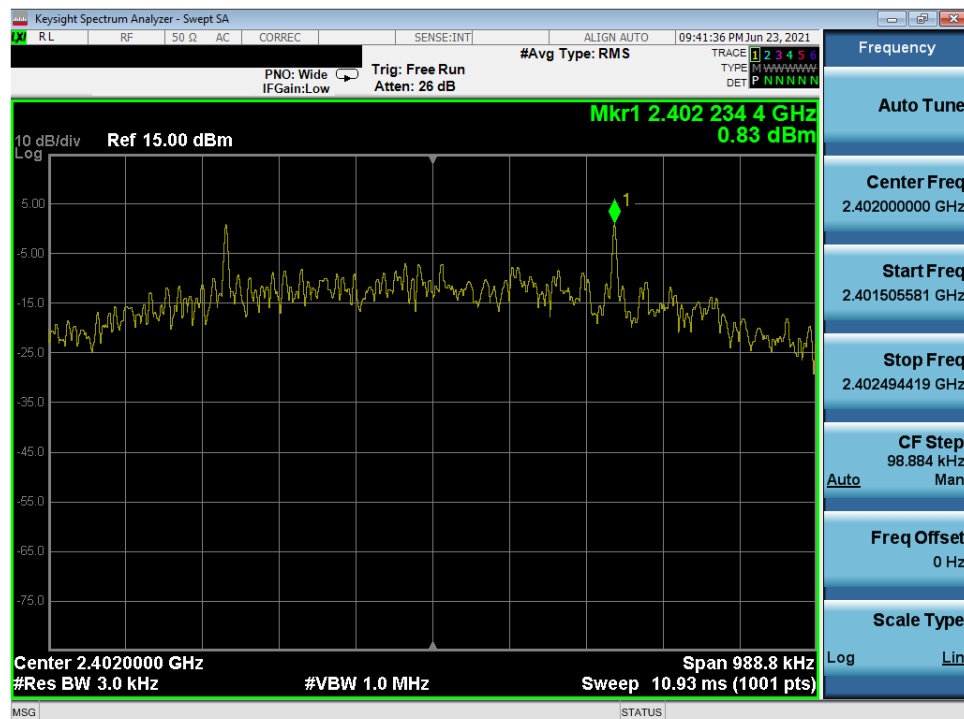
Plot 7-52. Power Spectral Density Plot (Bluetooth (LE), 500kbps – Ch. 0) – South Antenna
