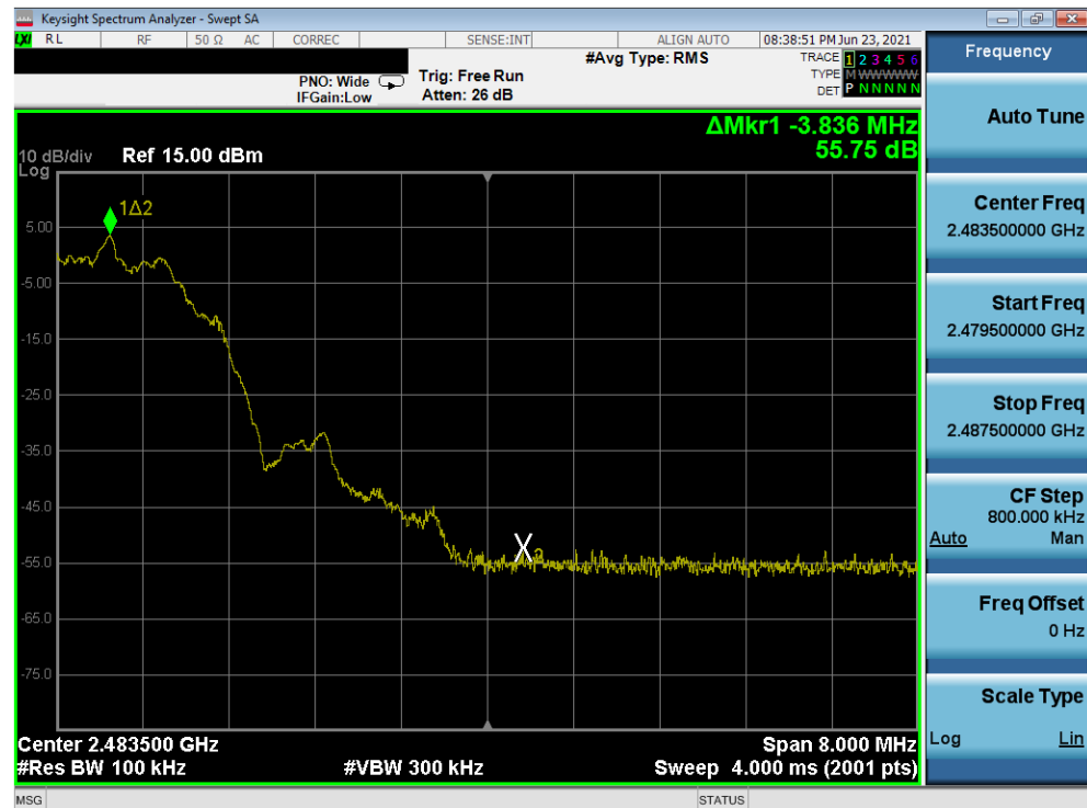
Plot 7-88. Band Edge Plot (Bluetooth (LE), 2Mbps – Ch. 39) – North Antenna
