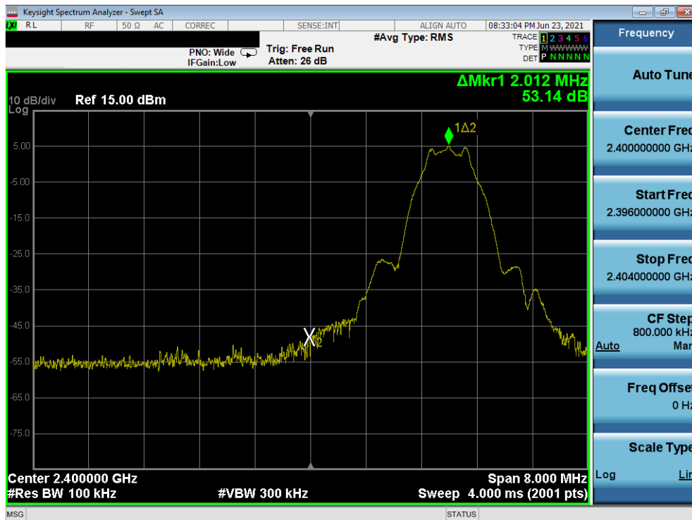
Plot 7-85. Band Edge Plot (Bluetooth (LE), 1Mbps - Ch. 0) - North Antenna
