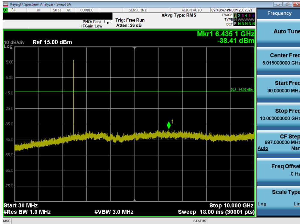
Plot 7-93. Conducted Spurious Plot (Bluetooth (LE), 1Mbps - Ch. 39) - South Antenna
