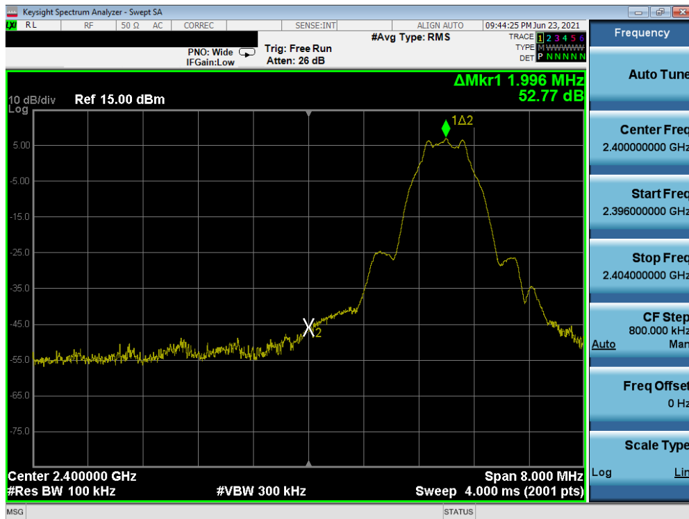
Plot 7-77. Band Edge Plot (Bluetooth (LE), 1Mbps – Ch. 0) – South Antenna
