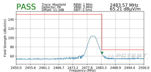
Plot 7-102. Radiated Restricted Upper Band Edge Measurement (Peak) – South Antenna
