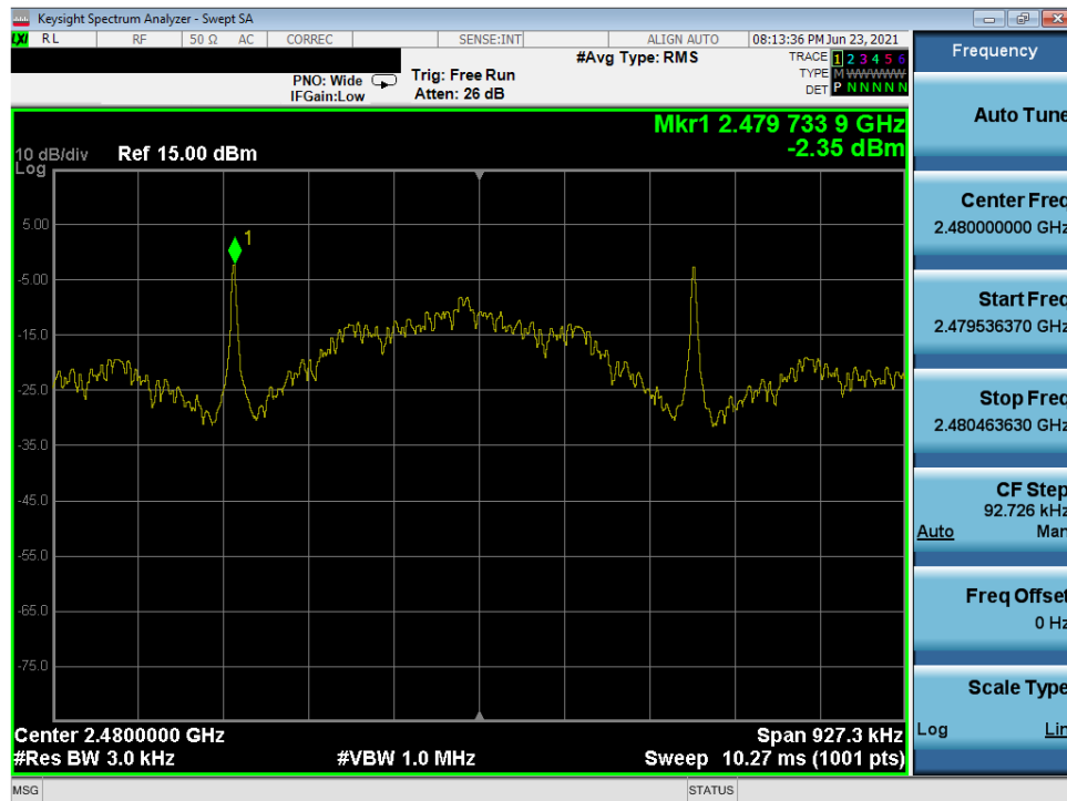
Plot 7-63. Power Spectral Density Plot (Bluetooth (LE), 125kbps – Ch. 39) – North Antenna
