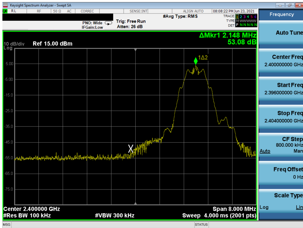
Plot 7-81. Band Edge Plot (Bluetooth (LE), 125kbps - Ch. 0) - North Antenna
