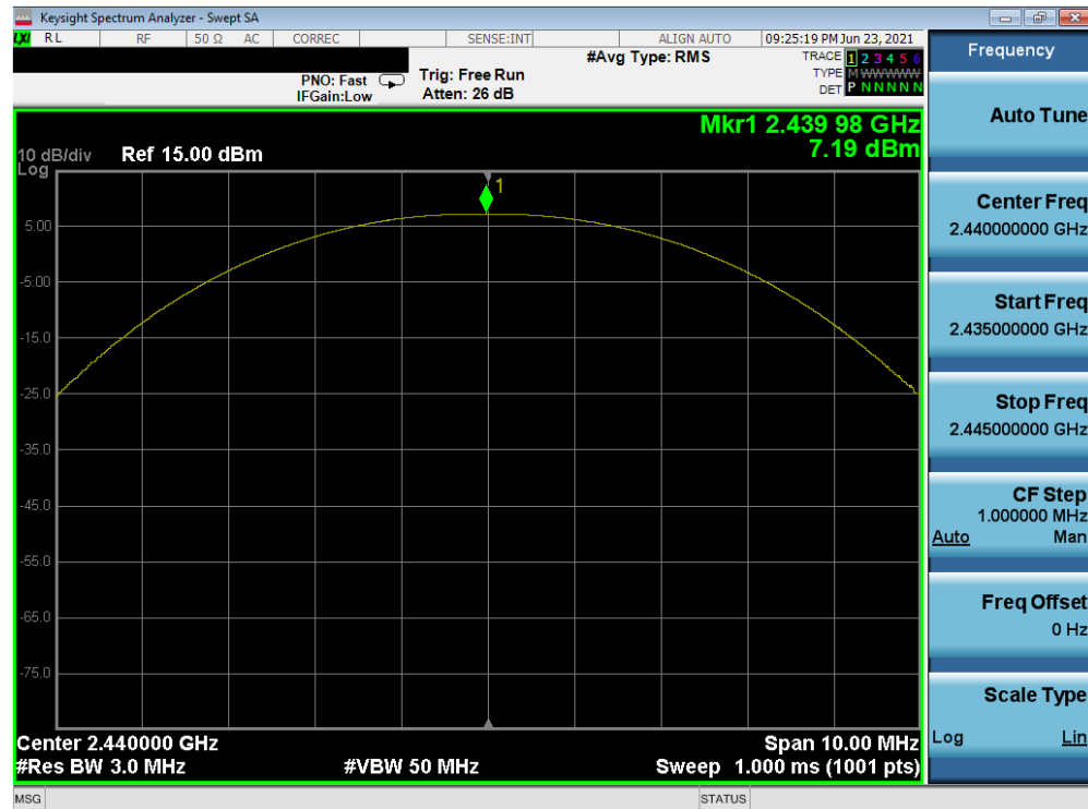
Plot 7-26. Peak Power Plot (Bluetooth (LE), 125kbps – Ch. 19) – South Antenna
