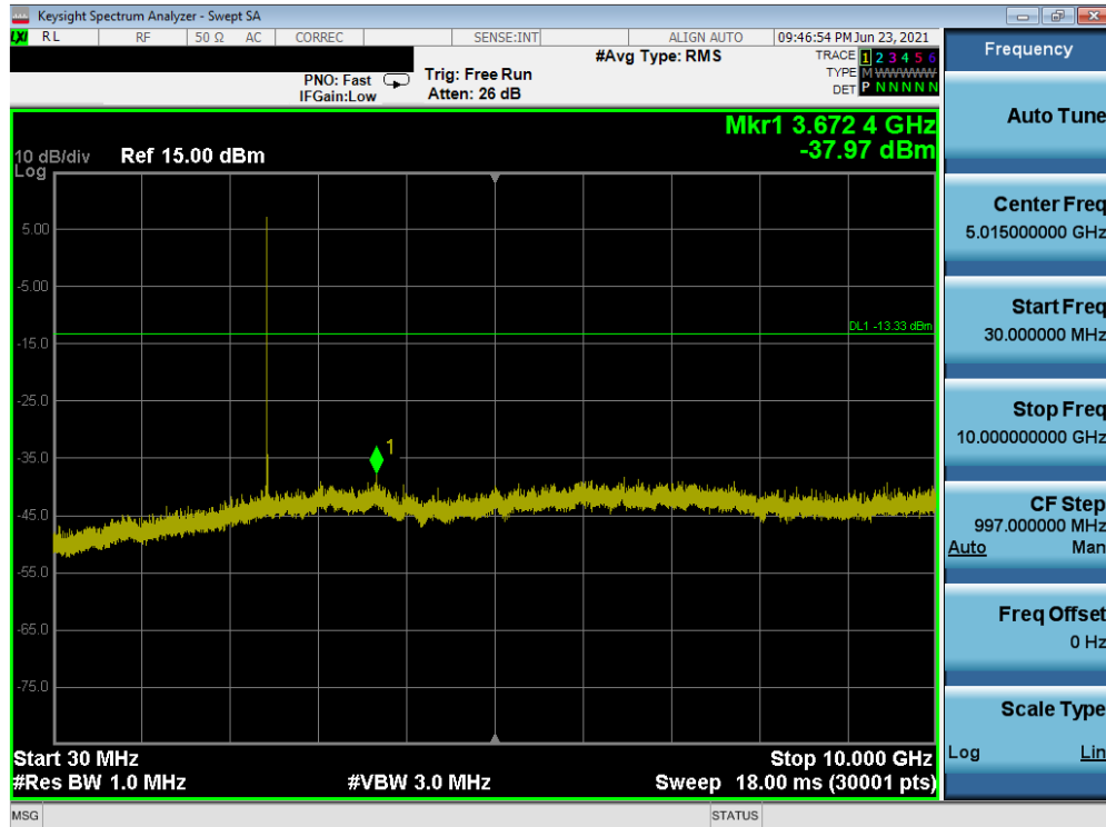
Plot 7-91. Conducted Spurious Plot (Bluetooth (LE), 1Mbps – Ch. 19) – South Antenna
