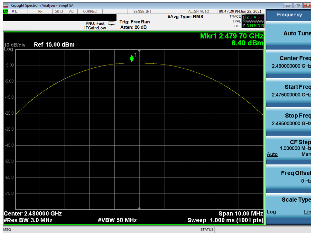
Plot 7-33. Peak Power Plot (Bluetooth (LE), 1Mbps - Ch. 39) - South Antenna
