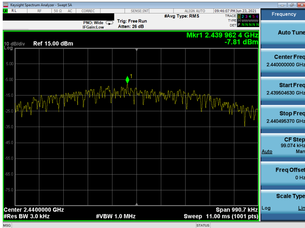
Plot 7-56. Power Spectral Density Plot (Bluetooth (LE), 1Mbps – Ch. 19) – South Antenna
