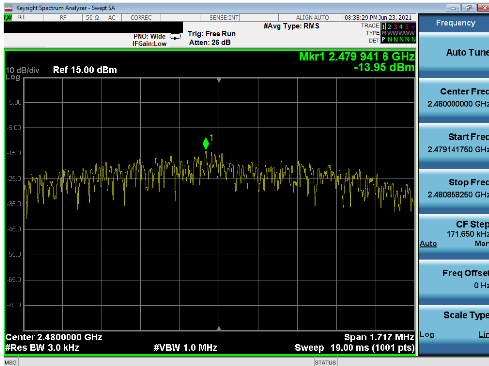
Plot 7-72. Power Spectral Density Plot (Bluetooth (LE), 2Mbps – Ch. 39) – North Antenna
