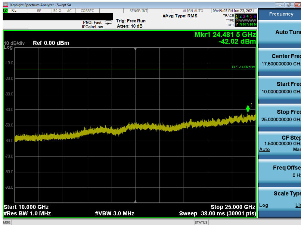
Plot 7-94. Conducted Spurious Plot (Bluetooth (LE), 1Mbps - Ch. 39) - South Antenna
