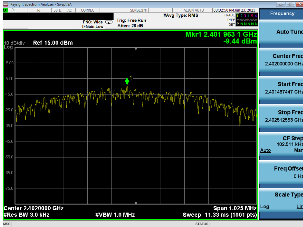
Plot 7-67. Power Spectral Density Plot (Bluetooth (LE), 1Mbps – Ch. 0) – North Antenna
