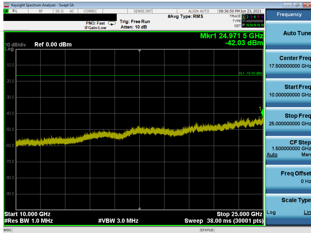
Plot 7-100. Conducted Spurious Plot (Bluetooth (LE), 1Mbps - Ch. 39) - North Antenna
