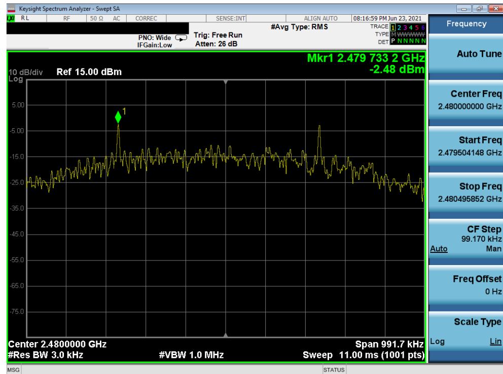
Plot 7-66. Power Spectral Density Plot (Bluetooth (LE), 500kbps – Ch. 39) – North Antenna
