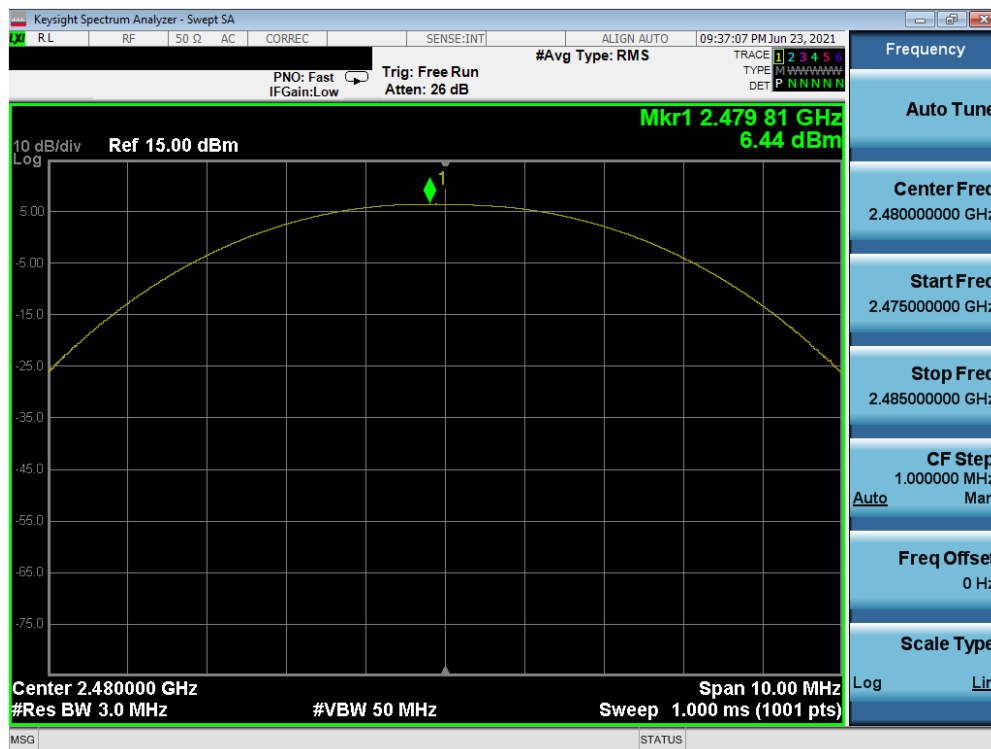
Plot 7-30. Peak Power Plot (Bluetooth (LE), 500kbps – Ch. 39) – South Antenna
