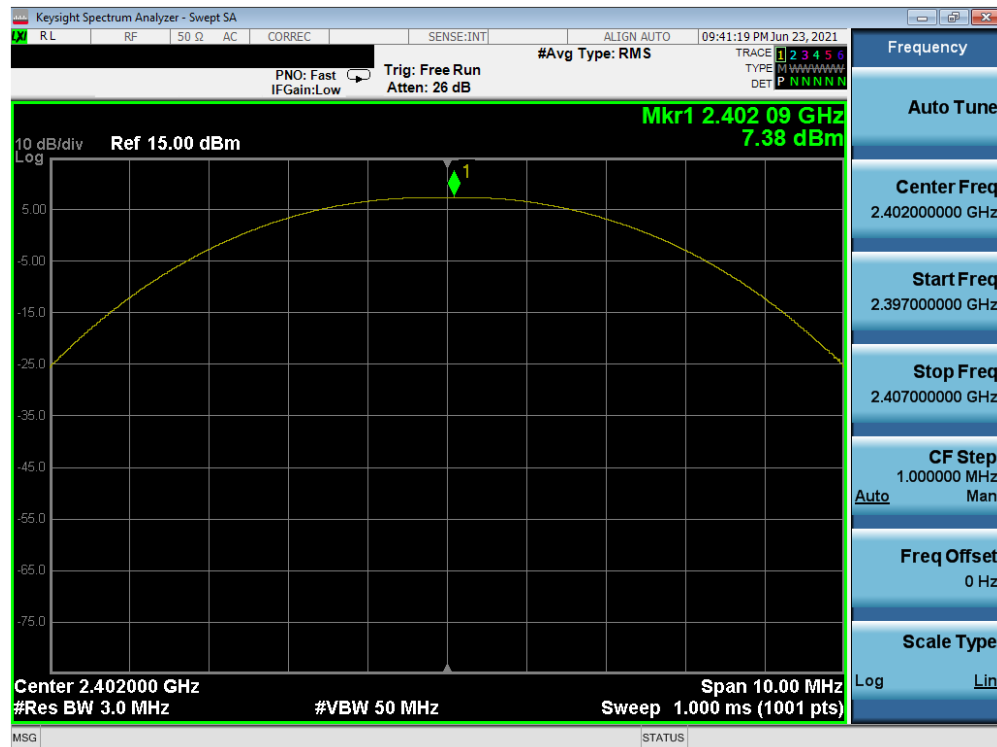
Plot 7-28. Peak Power Plot (Bluetooth (LE), 500kbps – Ch. 0) – South Antenna
