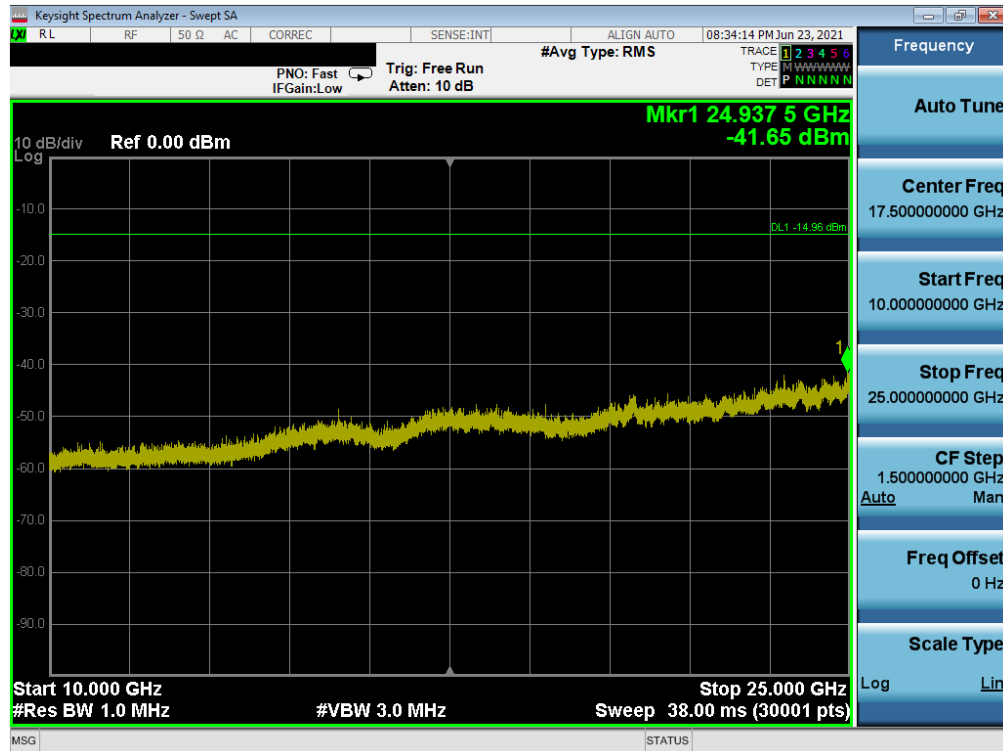
Plot 7-96. Conducted Spurious Plot (Bluetooth (LE), 1Mbps – Ch. 0) – North Antenna
