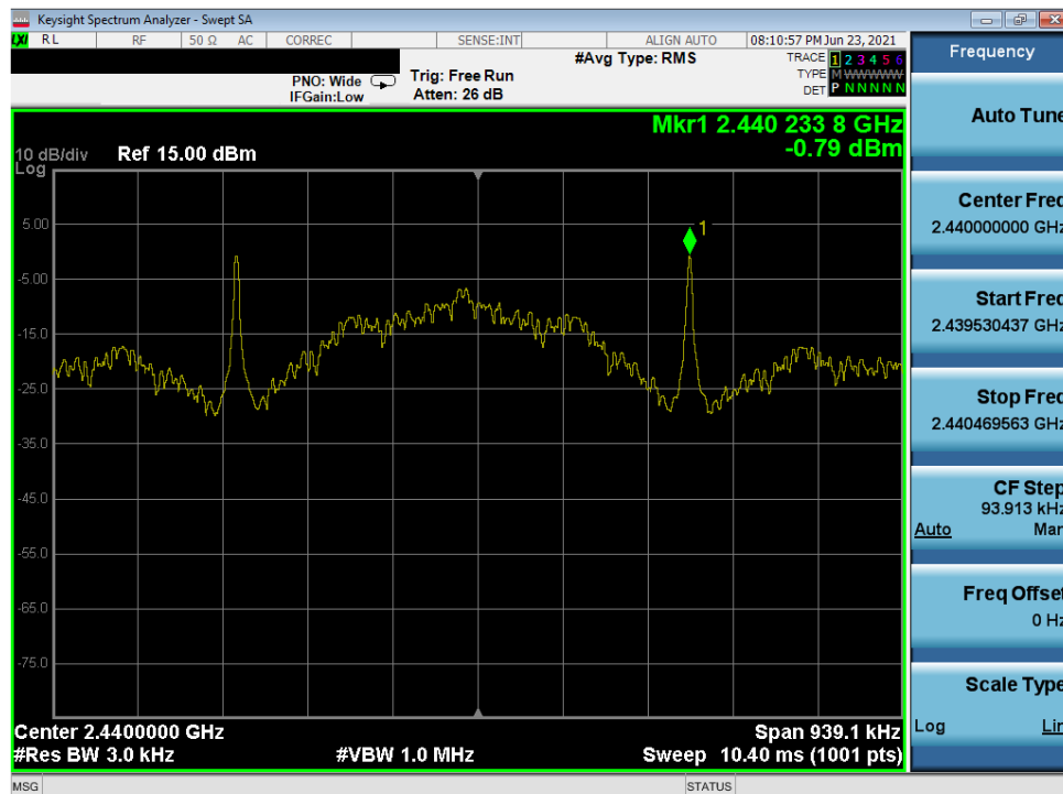
Plot 7-62. Power Spectral Density Plot (Bluetooth (LE), 125kbps – Ch. 19) – North Antenna
