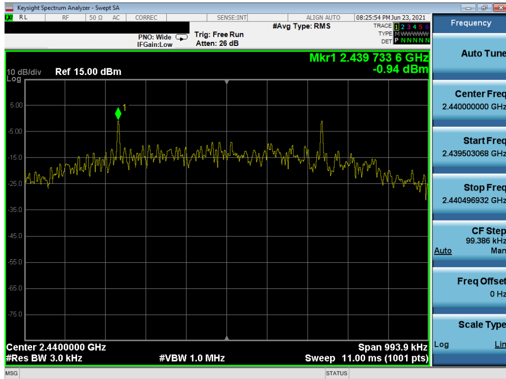
Plot 7-65. Power Spectral Density Plot (Bluetooth (LE), 500kbps – Ch. 19) – North Antenna
