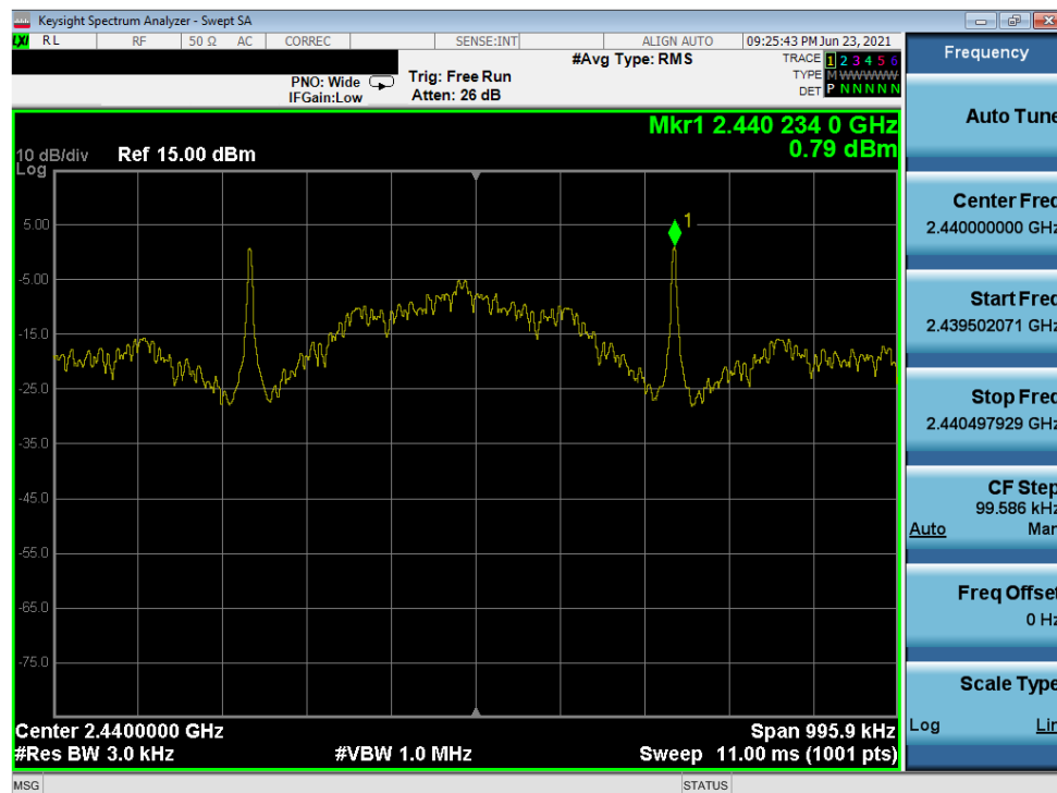
Plot 7-50. Power Spectral Density Plot (Bluetooth (LE), 125kbps – Ch. 19) – South Antenna
