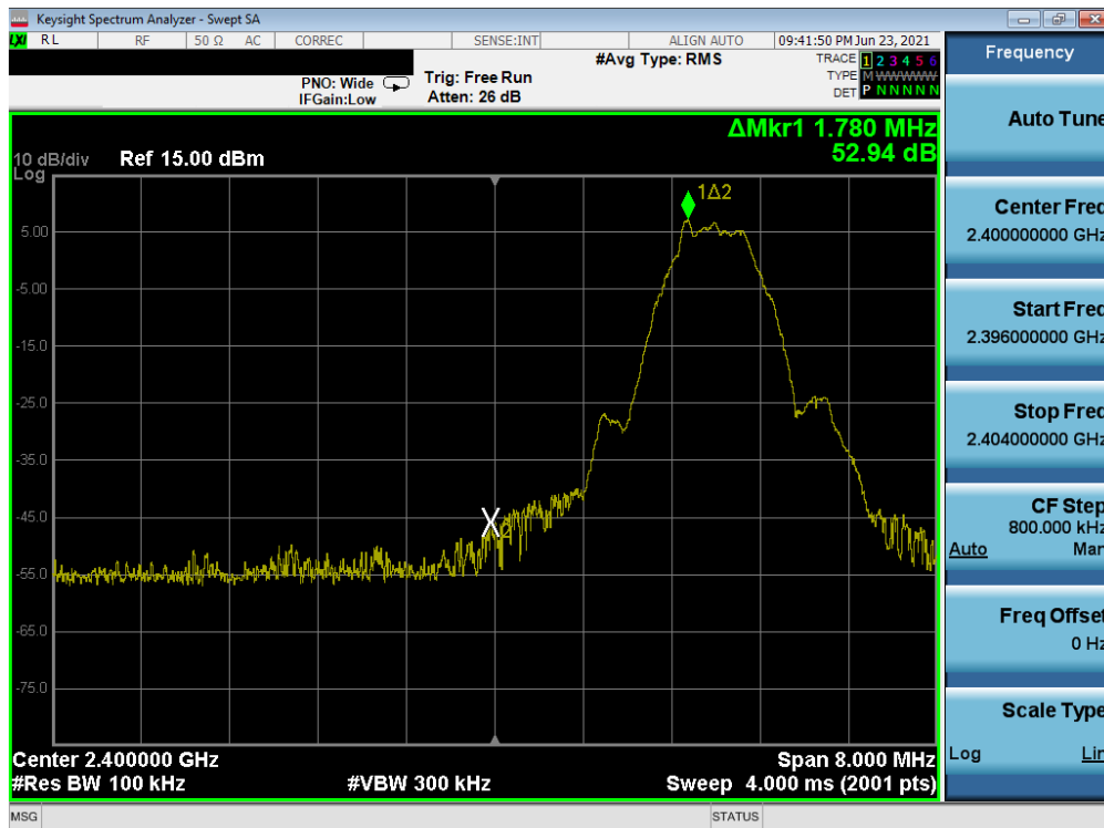
Plot 7-75. Band Edge Plot (Bluetooth (LE), 500kbps - Ch. 0) - South Antenna
