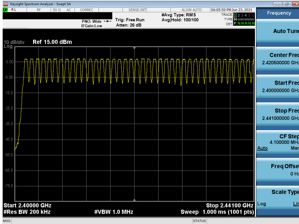
Plot 7-65. Low End Spectrum Channel Hopping Plot (Bluetooth)
