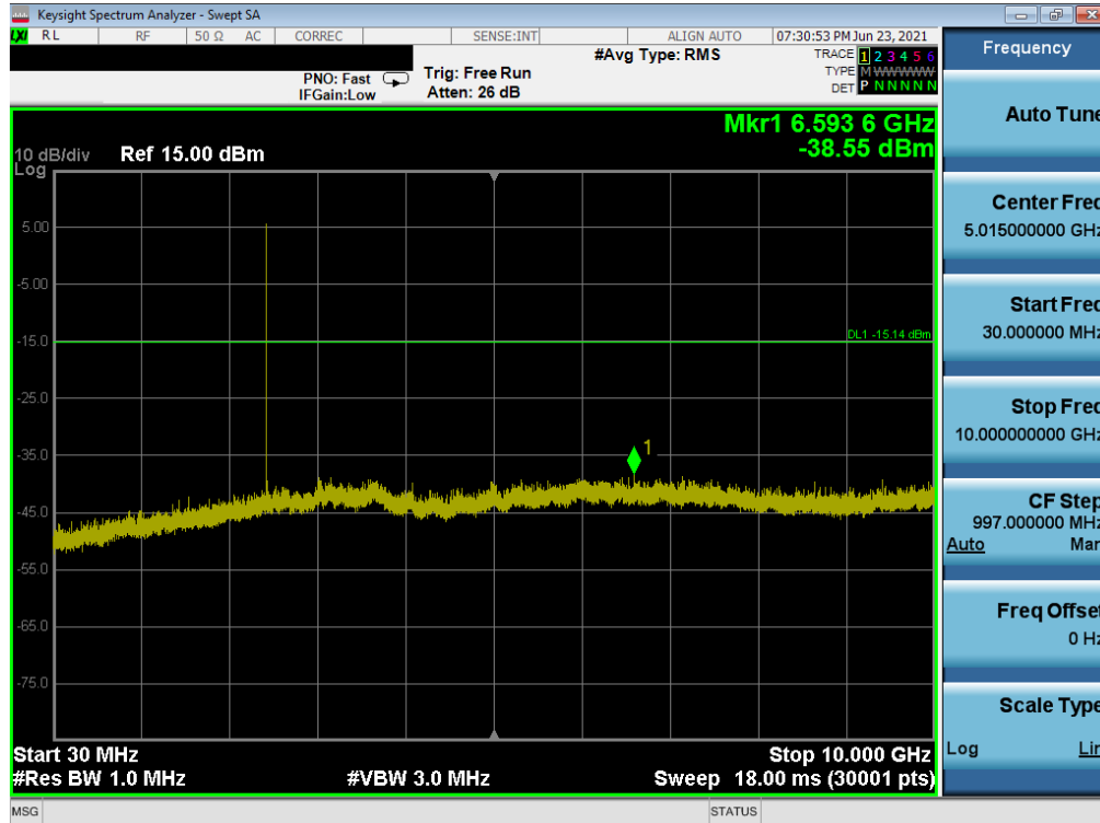
Plot 7-75. Conducted Spurious Plot (Bluetooth, 1Mbps – Ch. 39) – North Antenna
