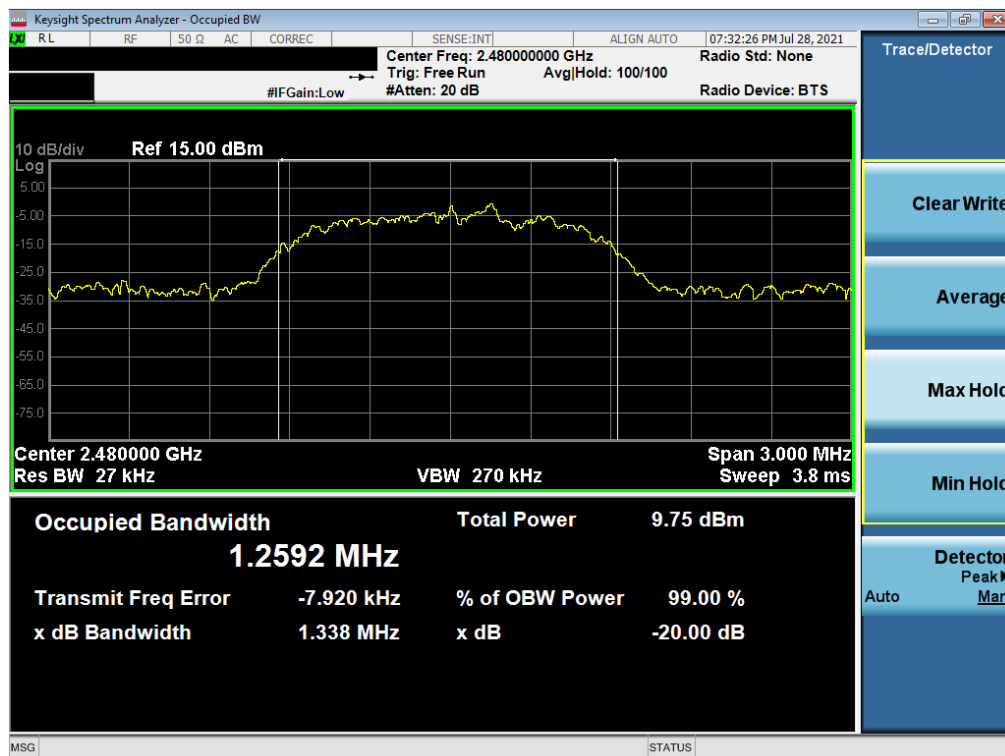
Plot 7-18. 20dB Bandwidth Plot (Bluetooth, 3Mbps – Ch. 78) – North Antenna
