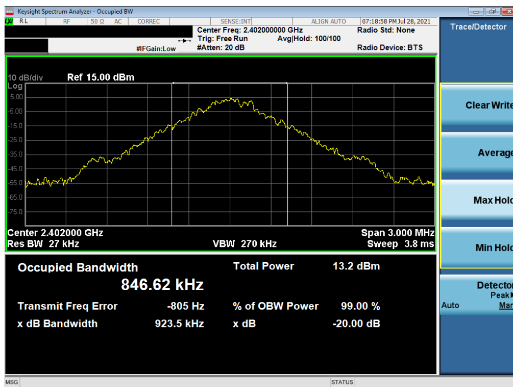
Plot 7-10. 20dB Bandwidth Plot (Bluetooth, 1Mbps – Ch. 0) – North Antenna
