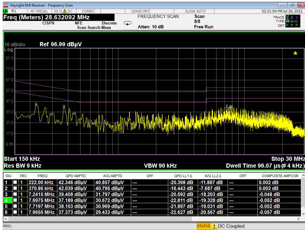
Plot 7-93. Line-Conducted Test Plot (L1)
