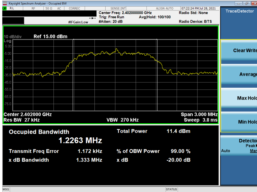
Plot 7-13. 20dB Bandwidth Plot (Bluetooth, 2Mbps – Ch. 0) – North Antenna
