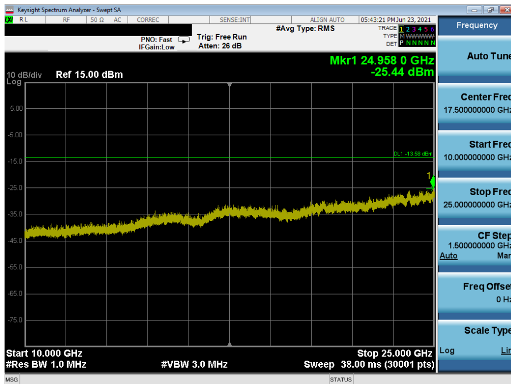
Plot 7-70. Conducted Spurious Plot (Bluetooth, 1Mbps – Ch. 39) – South Antenna
