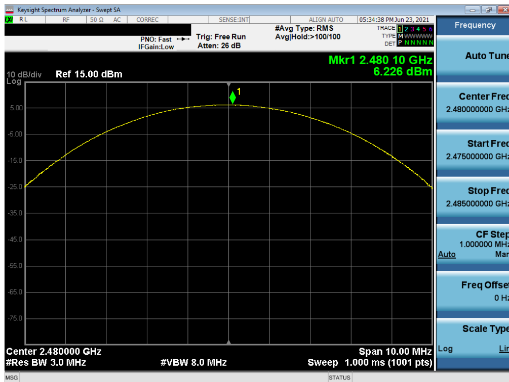
Plot 7-27. Peak Conducted Power (3Mbps - Ch. 78) - South Antenna
