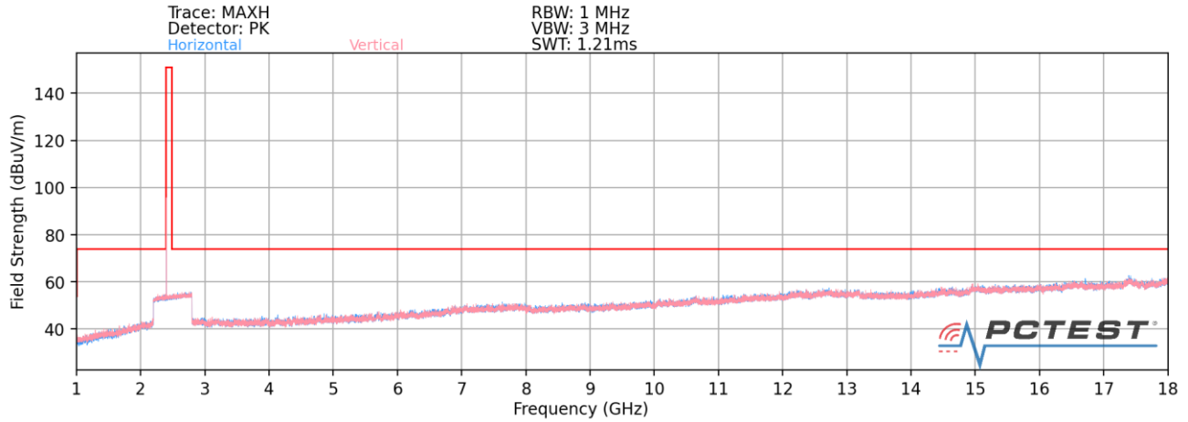
Plot 7-79. Radiated Spurious Plot above 1GHz (BT- Ch. 0) – Closed
