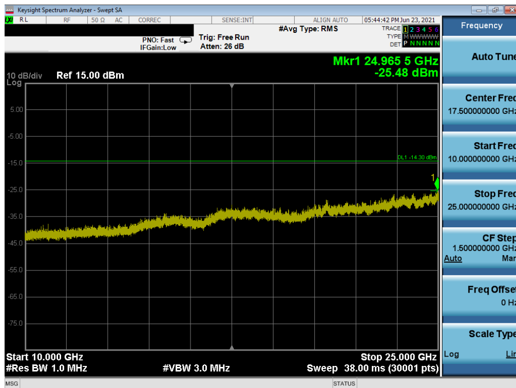
Plot 7-72. Conducted Spurious Plot (Bluetooth, 1Mbps – Ch. 78) – South Antenna
