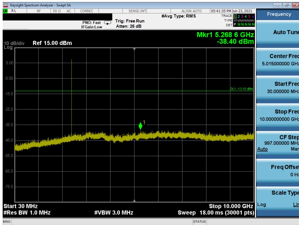
Plot 7-67. Conducted Spurious Plot (Bluetooth, 1Mbps – Ch. 0) – South Antenna
