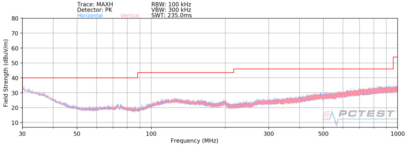
Plot 7-91. Radiated Spurious Plot below 1GHz – Closed
