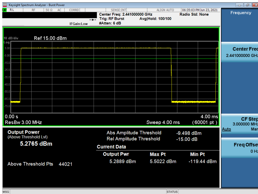
Plot 7-47. Average Conducted Power (1Mbps – Ch. 39) – North Antenna
