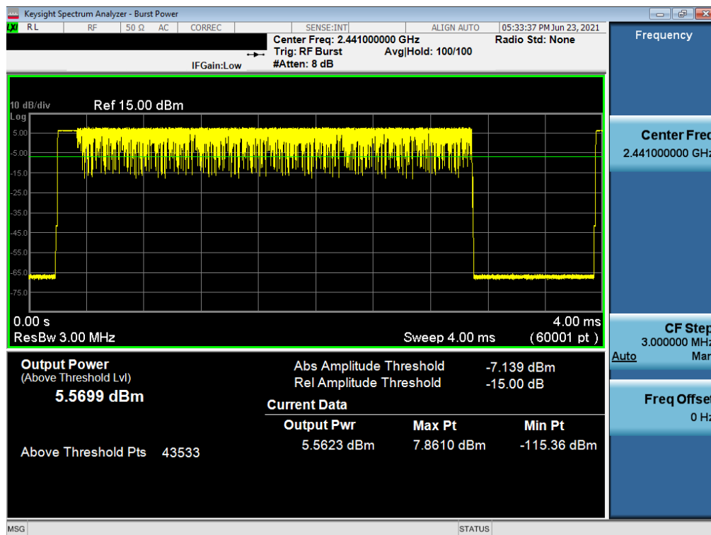
Plot 7-35. Average Conducted Power (3Mbps – Ch. 39) – South Antenna
