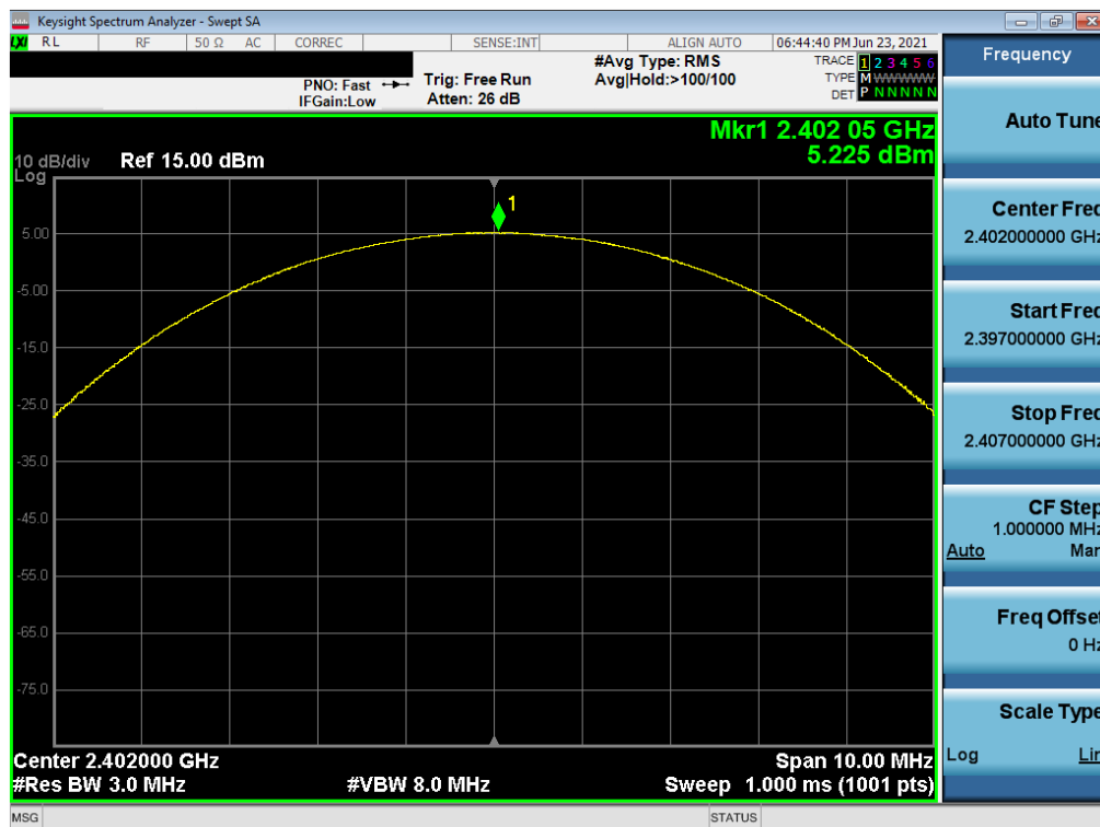
Plot 7-43. Peak Conducted Power (3Mbps – Ch. 0) – North Antenna
