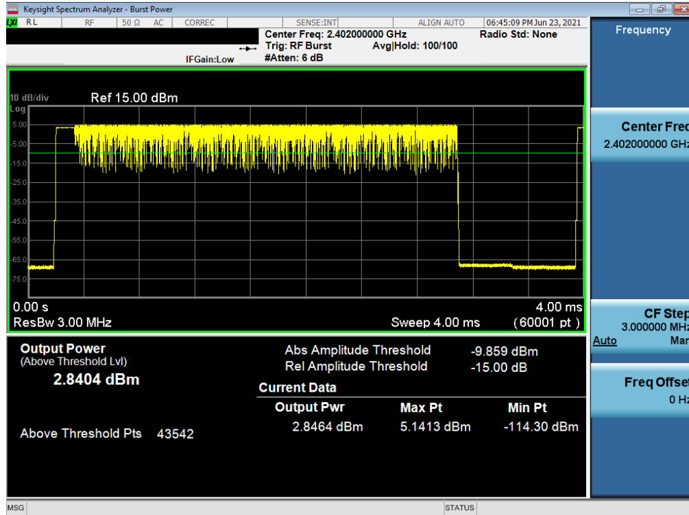
Plot 7-52. Average Conducted Power (3Mbps – Ch. 0) – North Antenna
