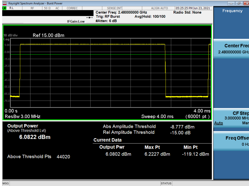
Plot 7-30. Average Conducted Power (1Mbps – Ch. 78) – South Antenna
