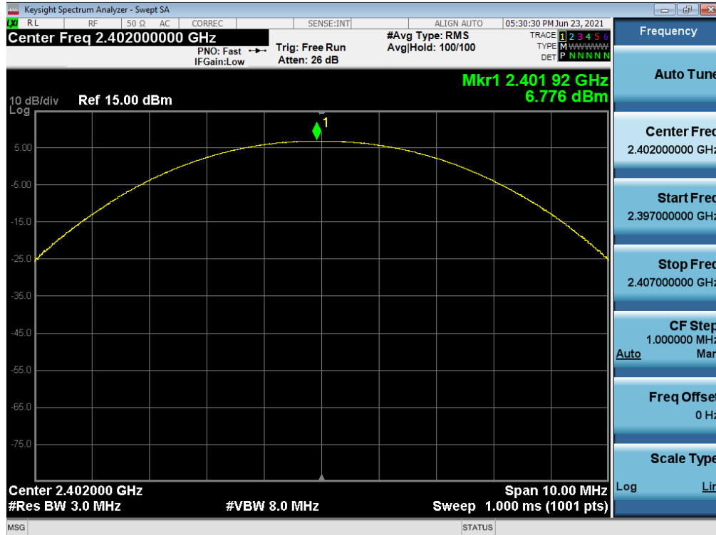
Plot 7-22. Peak Conducted Power (2Mbps - Ch. 0) - South Antenna
