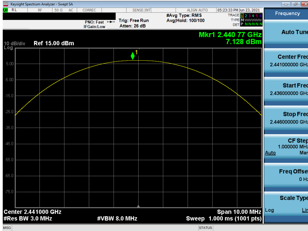
Plot 7-20. Peak Conducted Power (1Mbps – Ch. 39) – South Antenna
