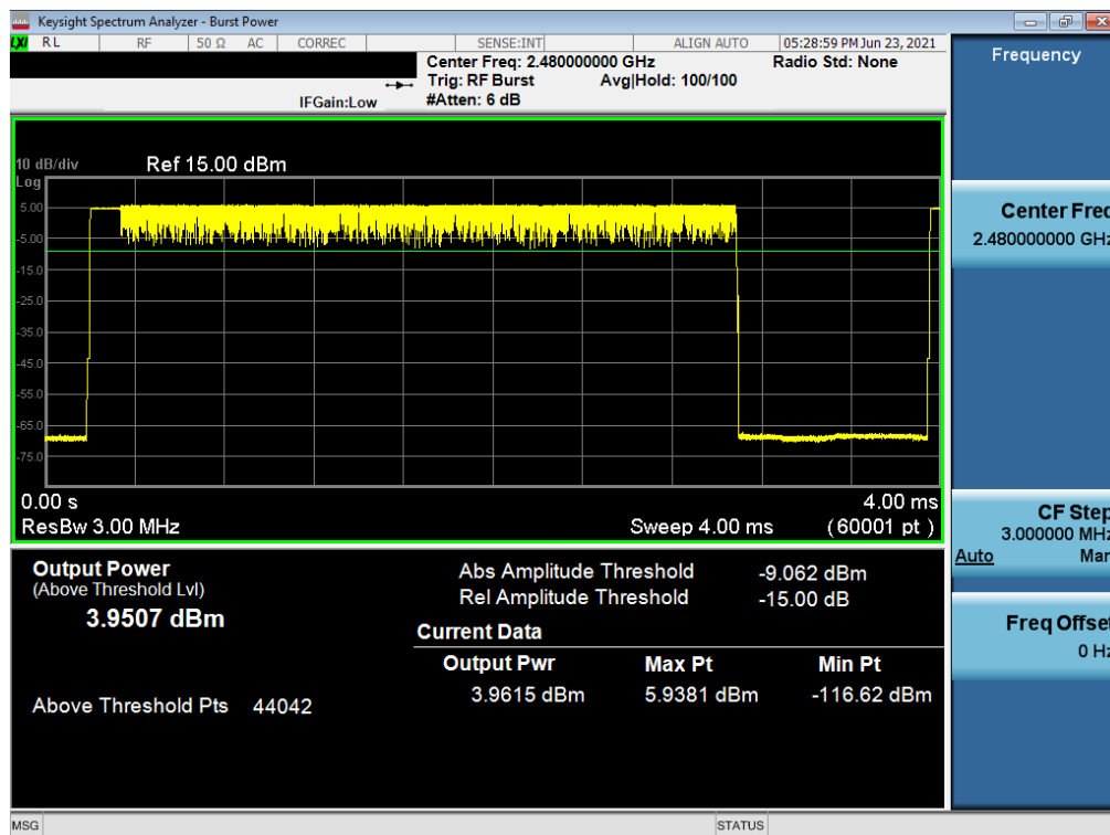
Plot 7-33. Average Conducted Power (2Mbps – Ch. 78) – South Antenna
