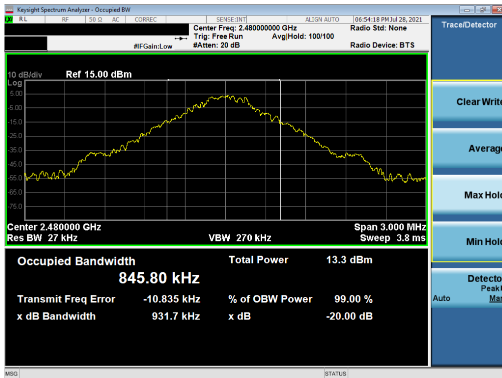
Plot 7-3. 20dB Bandwidth Plot (Bluetooth, 1Mbps – Ch. 78) – South Antenna
