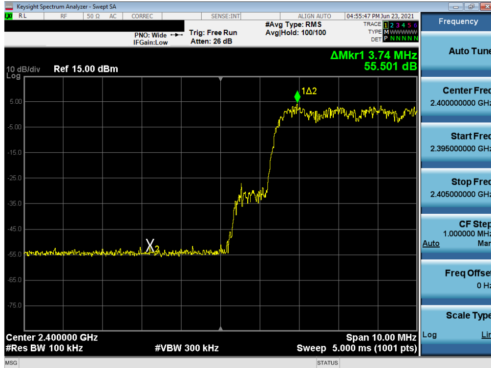
Plot 7-57. Band Edge Plot (Bluetooth with Hopping Enabled, 3 Mbps) – South Antenna
