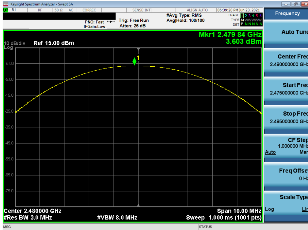
Plot 7-42. Peak Conducted Power (2Mbps – Ch. 78) – North Antenna
