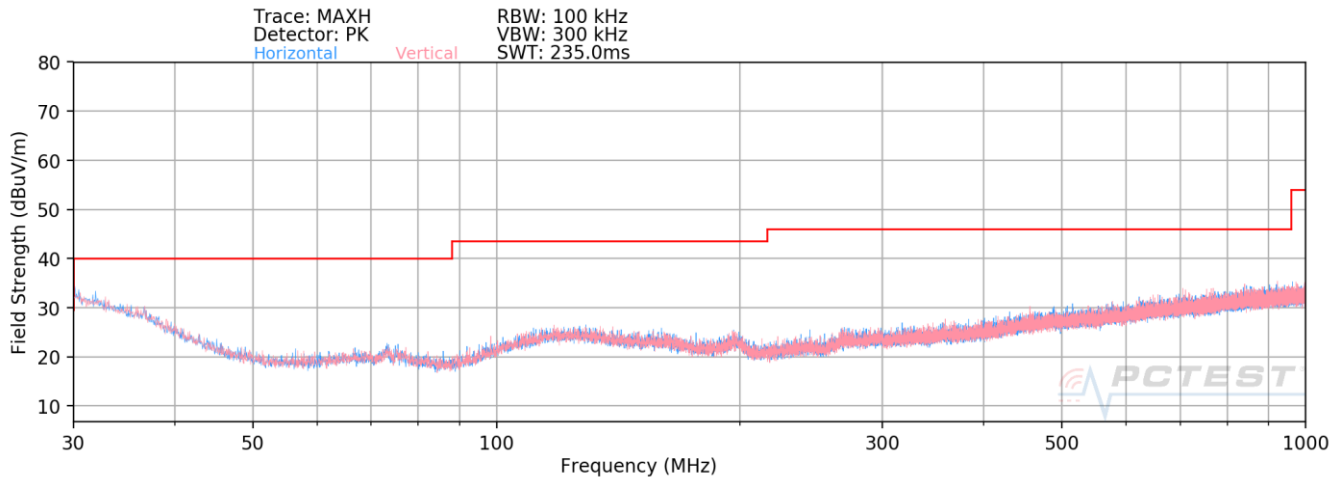
Plot 7-92. Radiated Spurious Plot below 1GHz – 300°
