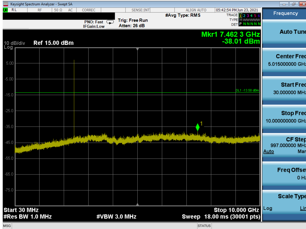
Plot 7-69. Conducted Spurious Plot (Bluetooth, 1Mbps – Ch. 39) – South Antenna
