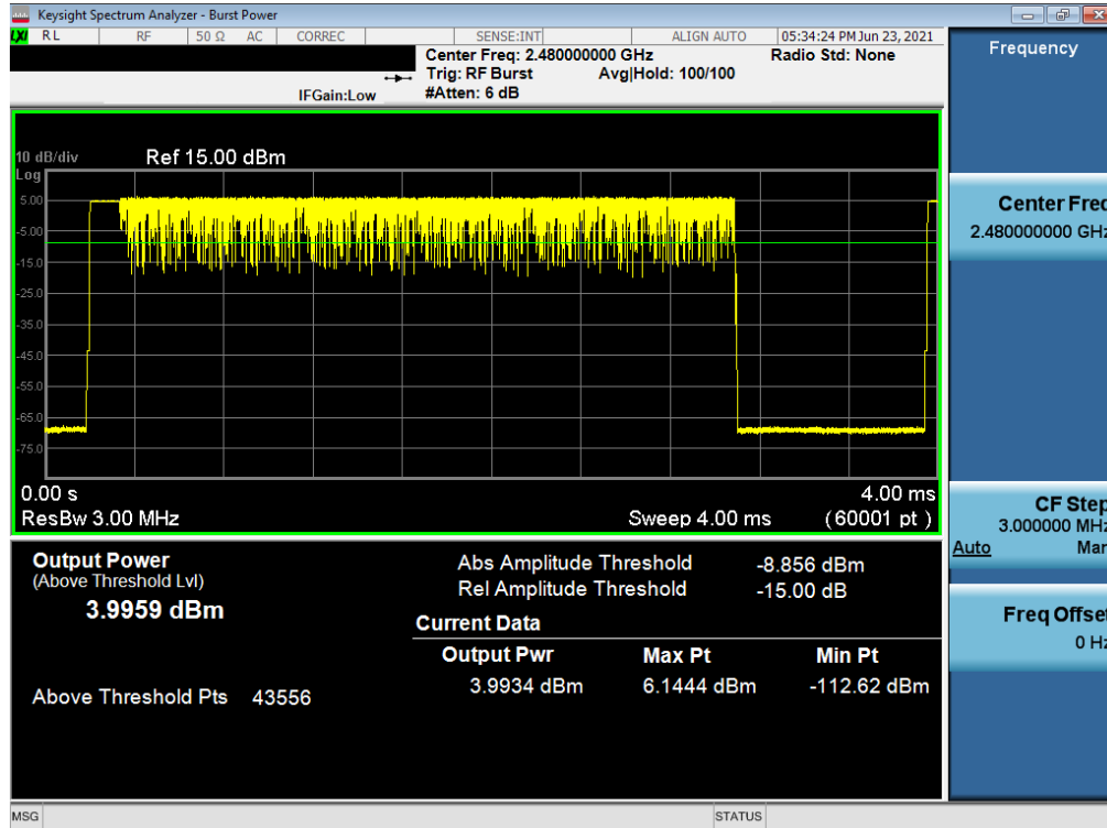
Plot 7-36. Average Conducted Power (3Mbps – Ch. 78) – South Antenna
