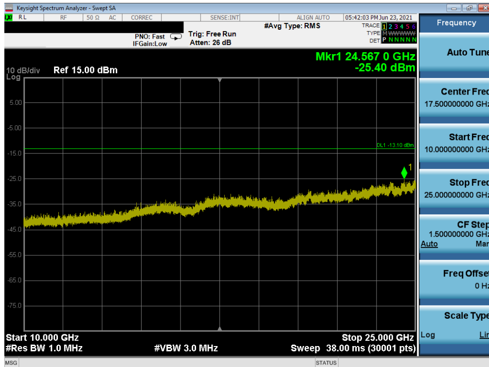
Plot 7-68. Conducted Spurious Plot (Bluetooth, 1Mbps – Ch. 0) – South Antenna
