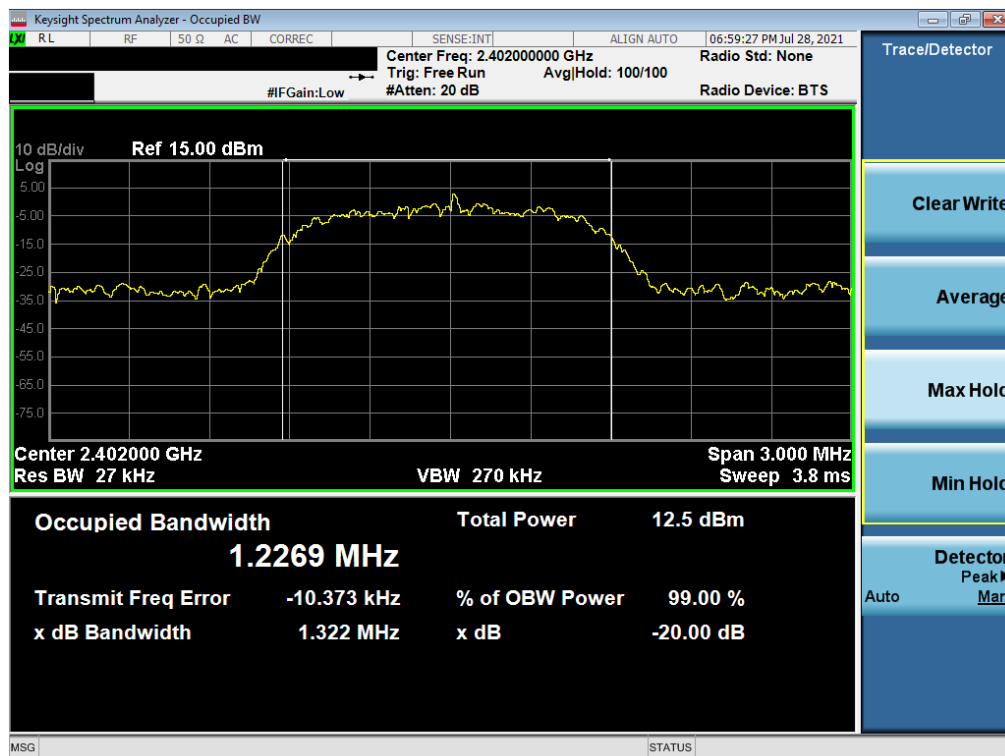
Plot 7-7. 20dB Bandwidth Plot (Bluetooth, 3Mbps – Ch. 0) – South Antenna
