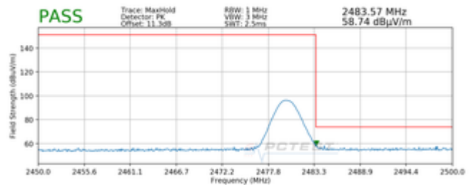
Plot 7-90. Radiated Restricted Upper Band Edge Measurement (Peak)
