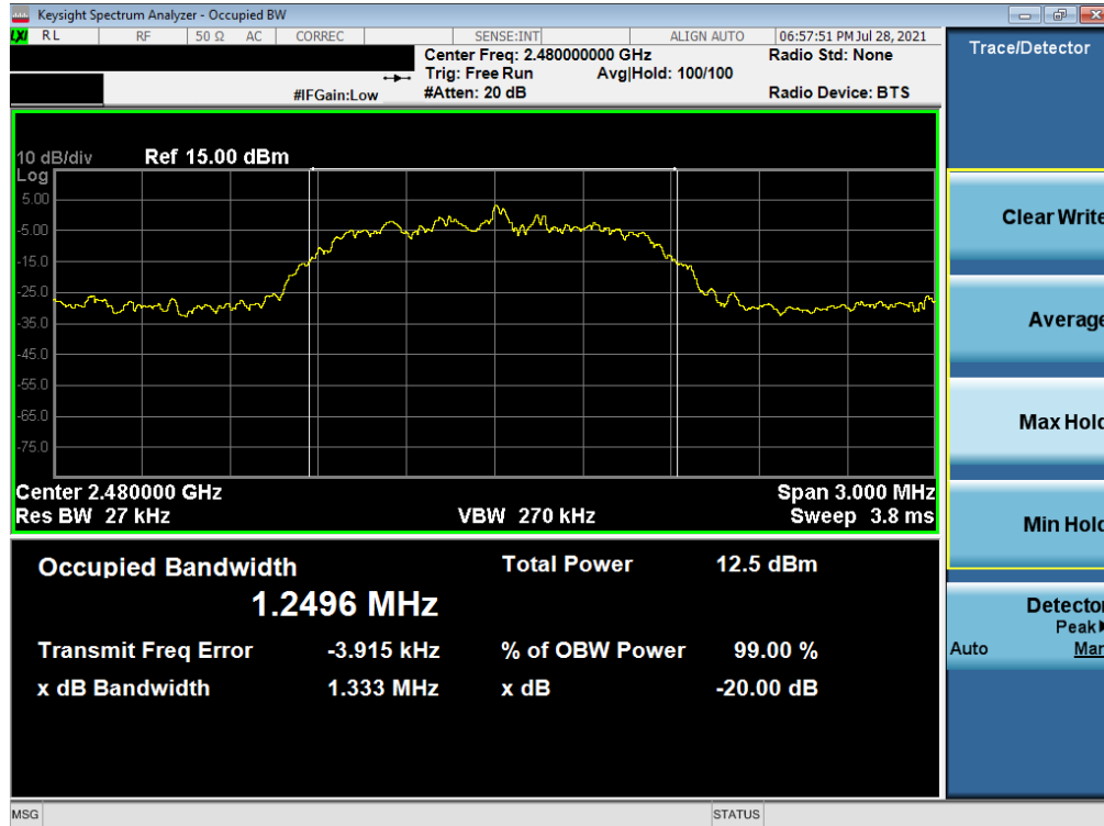
Plot 7-6. 20dB Bandwidth Plot (Bluetooth, 2Mbps – Ch. 78) – South Antenna
