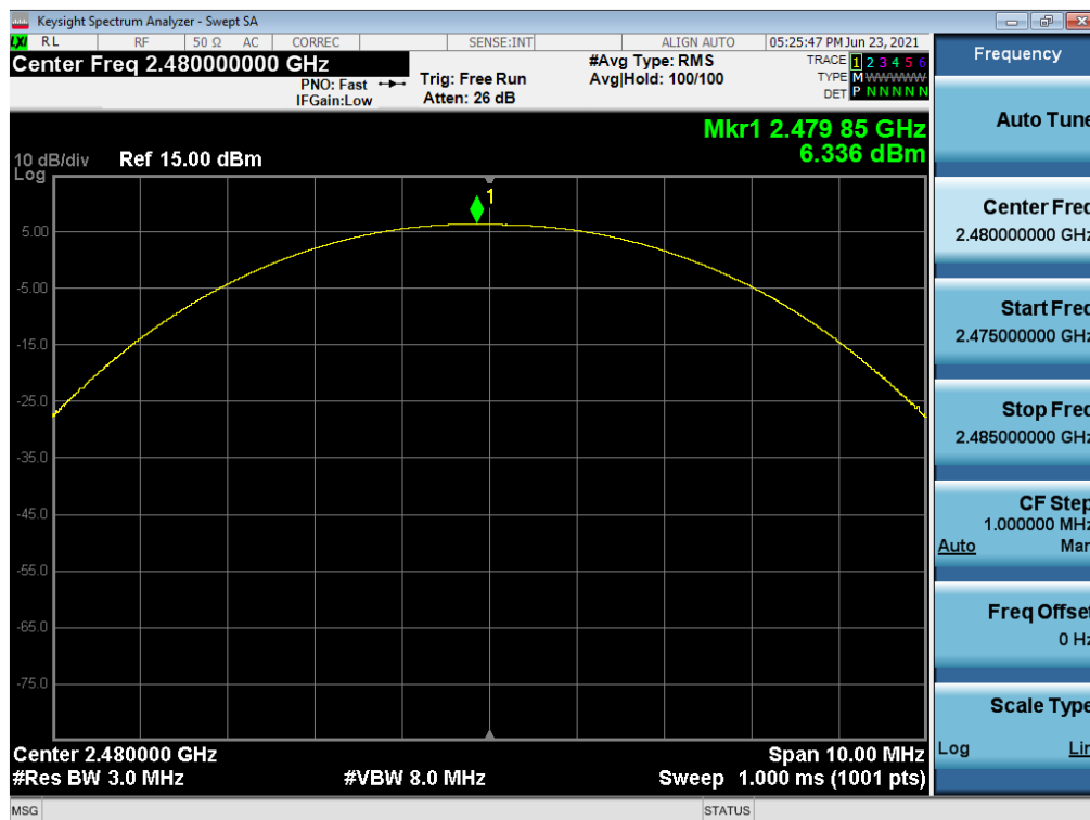
Plot 7-21. Peak Conducted Power (1Mbps – Ch. 78) – South Antenna
