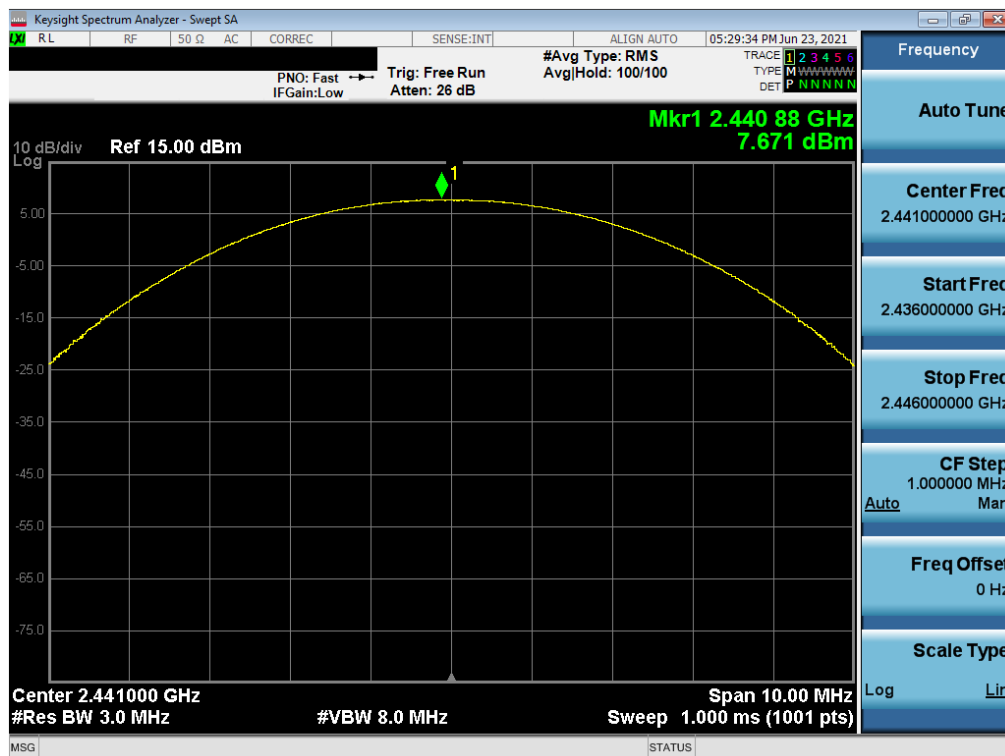
Plot 7-23. Peak Conducted Power (2Mbps - Ch. 39) - South Antenna
