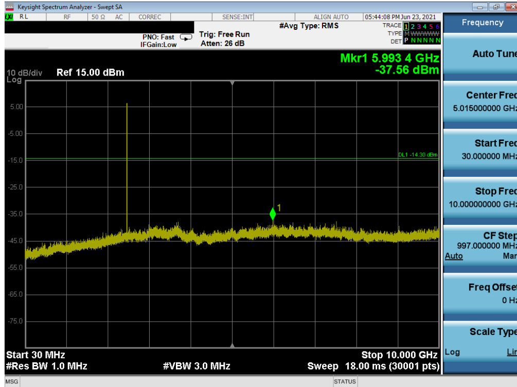
Plot 7-71. Conducted Spurious Plot (Bluetooth, 1Mbps – Ch. 78) – South Antenna
