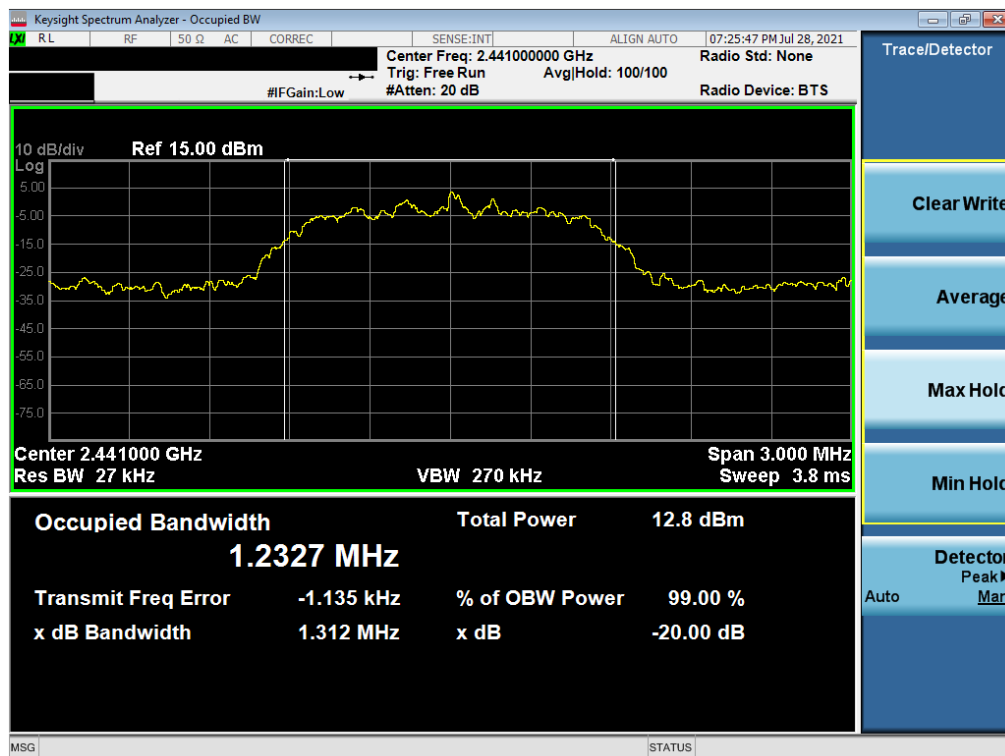
Plot 7-14. 20dB Bandwidth Plot (Bluetooth, 2Mbps – Ch. 39) – North Antenna
