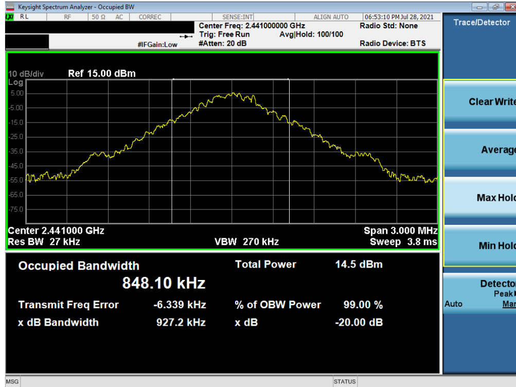
Plot 7-2. 20dB Bandwidth Plot (Bluetooth, 1Mbps – Ch. 39) – South Antenna
