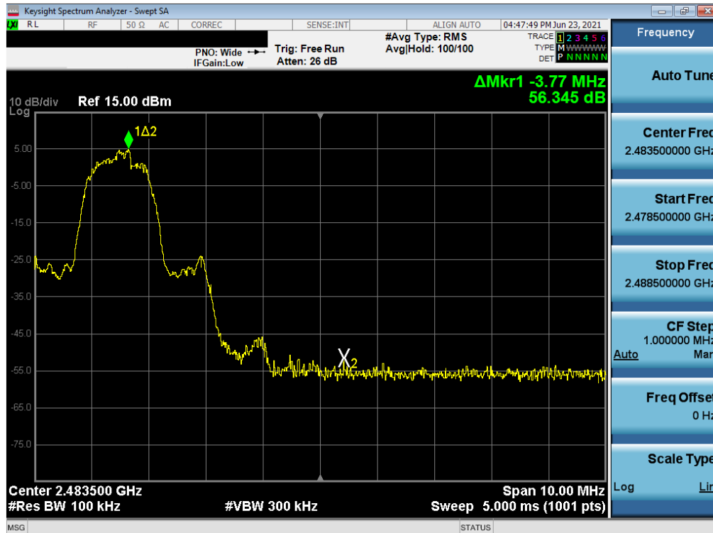
Plot 7-56. Band Edge Plot (Bluetooth with Hopping Disabled, 3 Mbps – Ch. 78) – South Antenna
