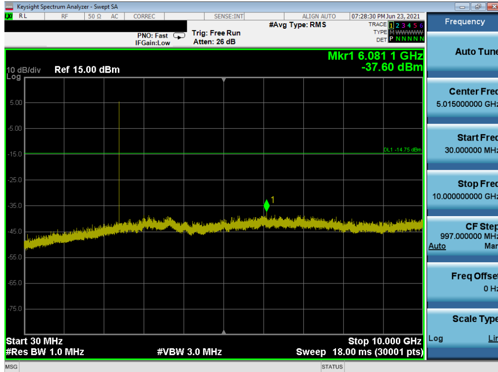
Plot 7-73. Conducted Spurious Plot (Bluetooth, 1Mbps – Ch. 0) – North Antenna
