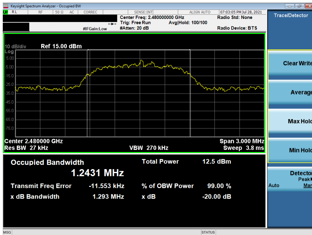
Plot 7-9. 20dB Bandwidth Plot (Bluetooth, 3Mbps – Ch. 78) – South Antenna
