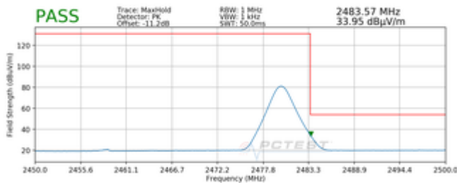
Plot 7-87. Radiated Restricted Upper Band Edge Measurement (Average)
