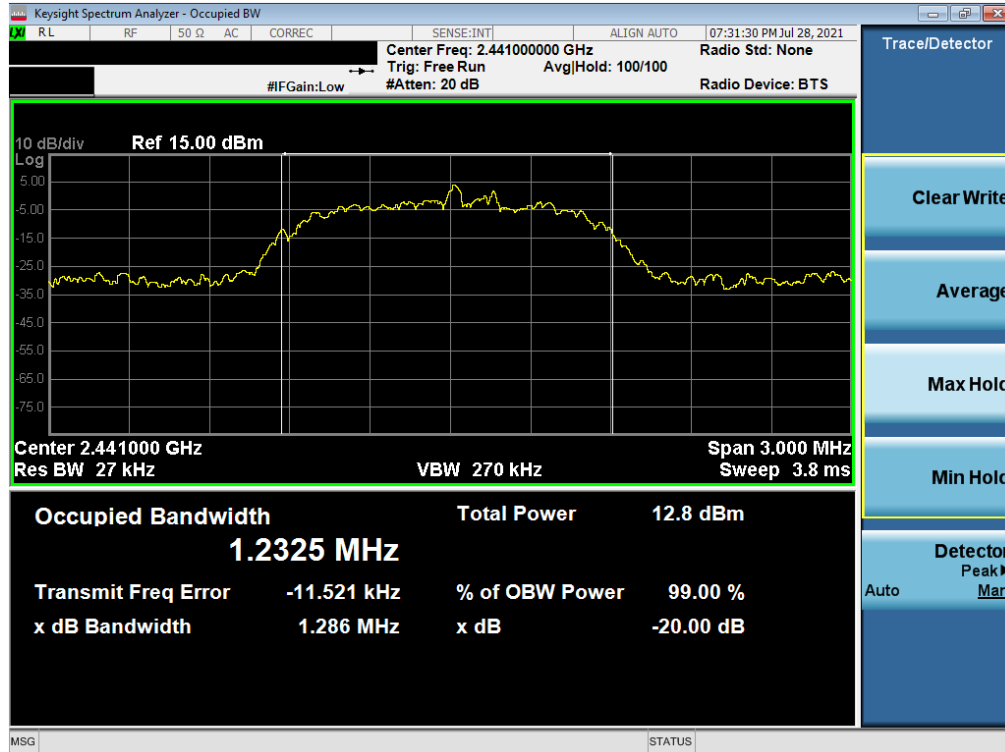
Plot 7-17. 20dB Bandwidth Plot (Bluetooth, 3Mbps – Ch. 39) – North Antenna
