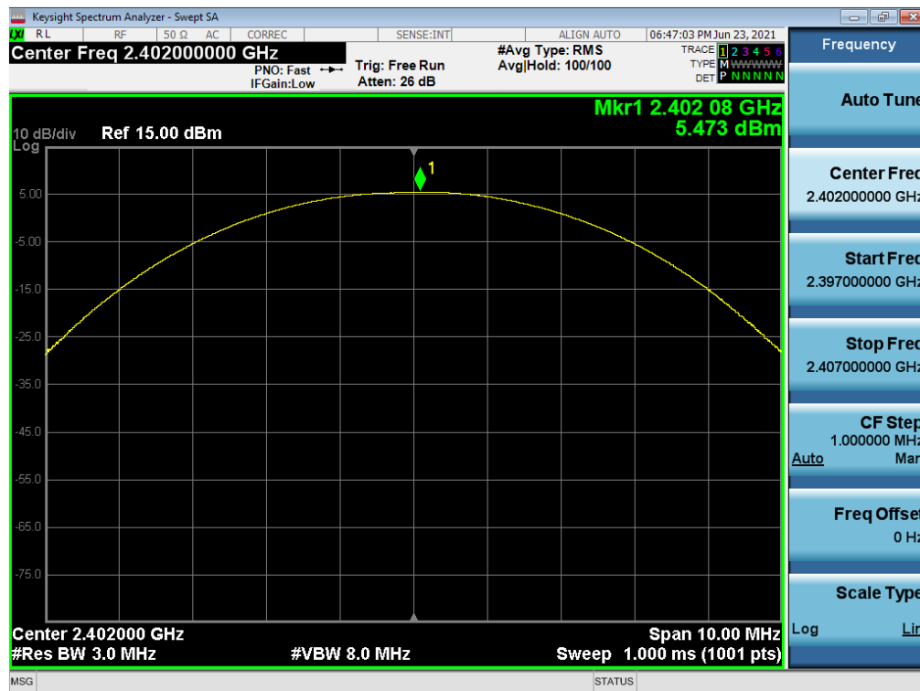
Plot 7-37. Peak Conducted Power (1Mbps – Ch. 0) – North Antenna
