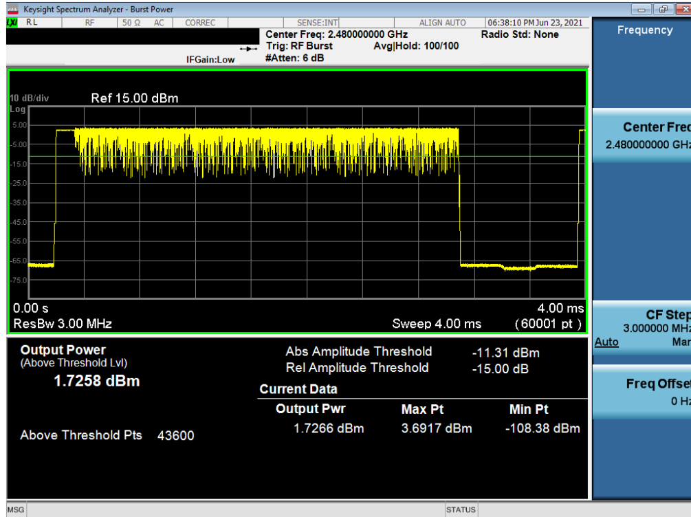
Plot 7-54. Average Conducted Power (3Mbps – Ch. 78) – North Antenna
