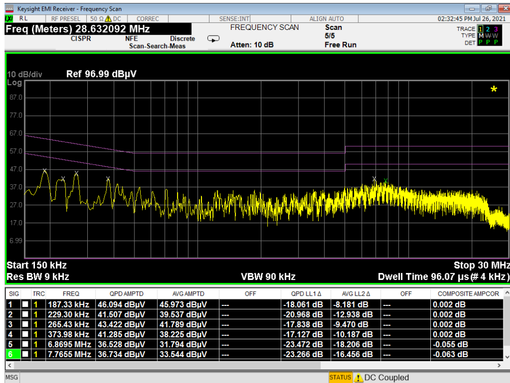
Plot 7-94. Line-Conducted Test Plot (N)
