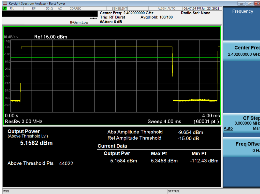
Plot 7-46. Average Conducted Power (1Mbps – Ch. 0) – North Antenna
