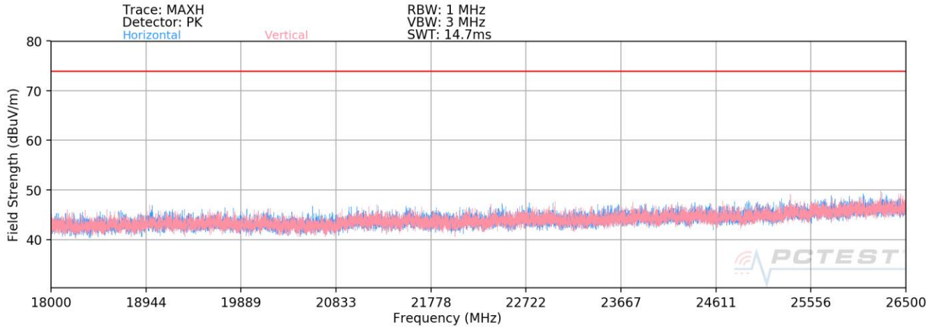
Plot 7-85. Radiated Spurious Plot above 18GHz – Closed
