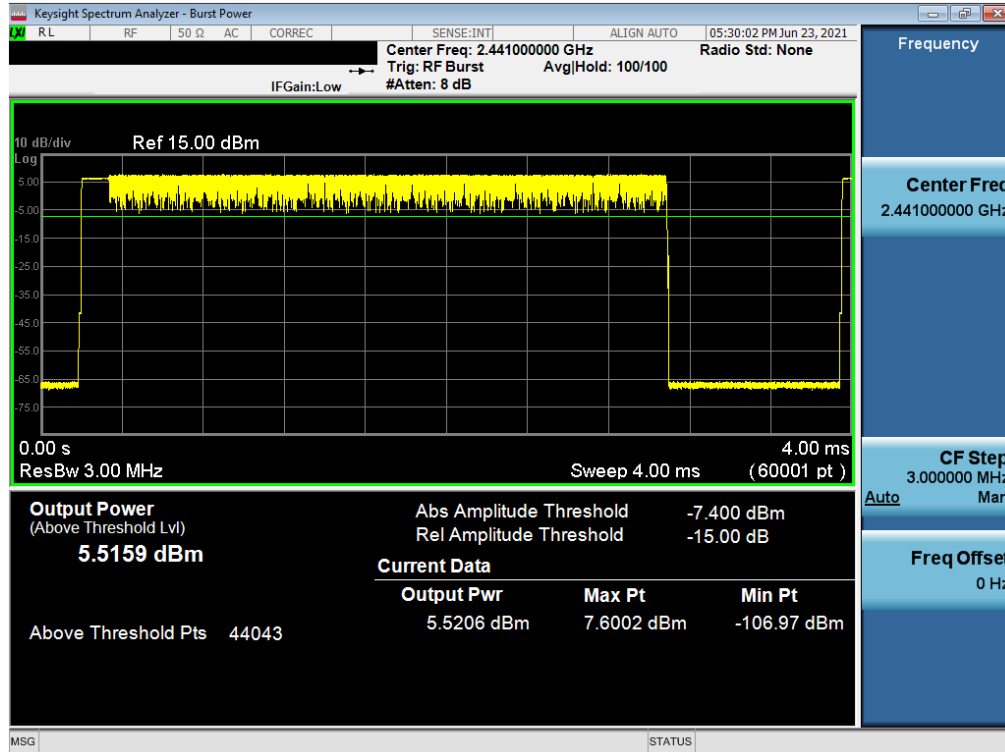
Plot 7-32. Average Conducted Power (2Mbps – Ch. 39) – South Antenna
