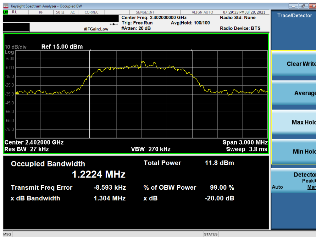
Plot 7-16. 20dB Bandwidth Plot (Bluetooth, 3Mbps – Ch. 0) – North Antenna
