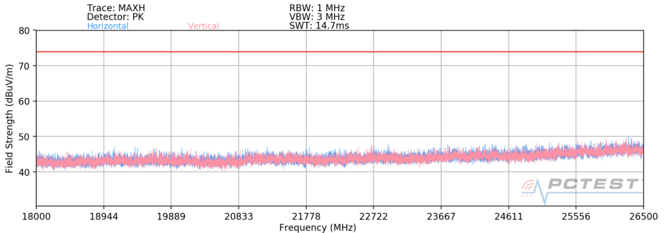
Plot 7-86. Radiated Spurious Plot above 18GHz – 300°
