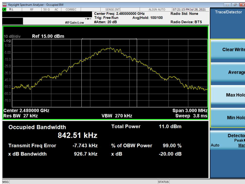
Plot 7-12. 20dB Bandwidth Plot (Bluetooth, 1Mbps – Ch. 78) – North Antenna
