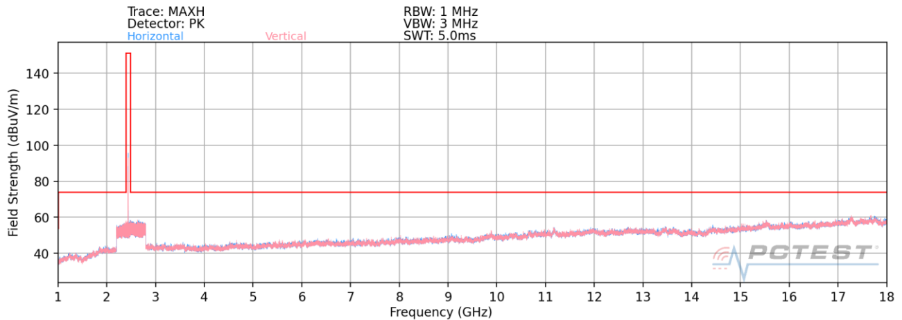
Plot 7-80. Radiated Spurious Plot above 1GHz (BT- Ch. 39) – Closed
