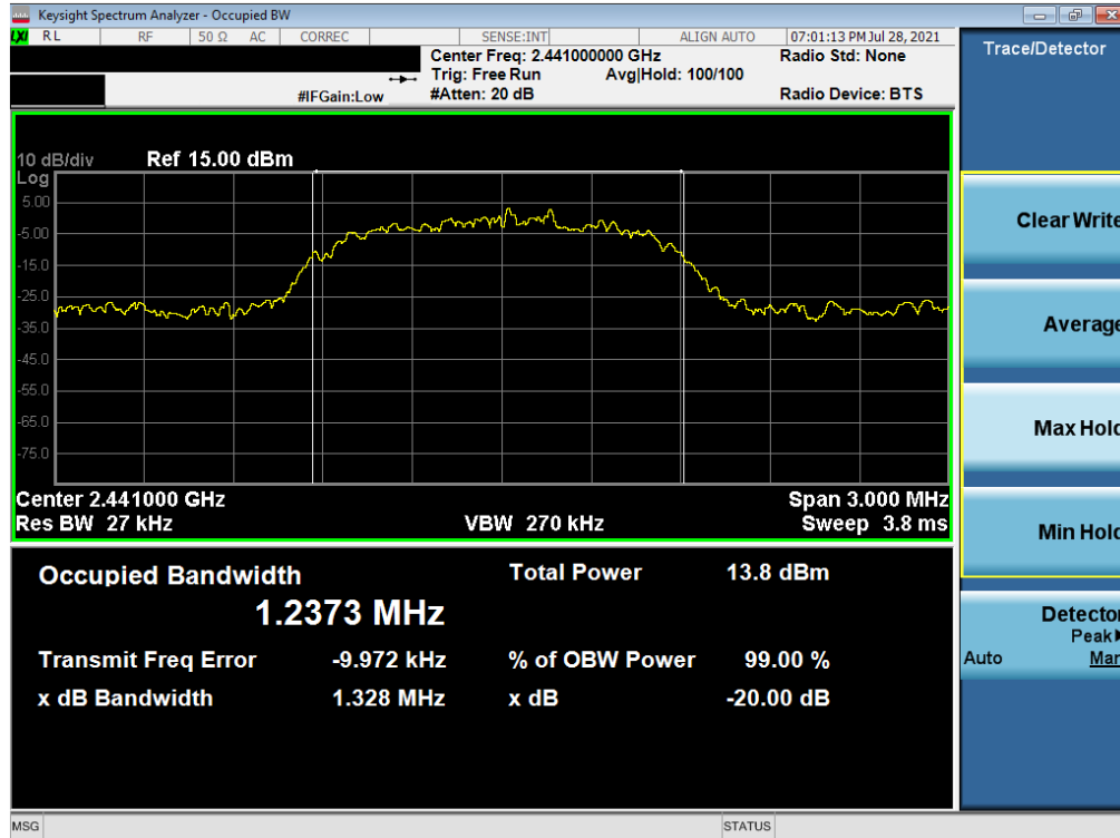
Plot 7-8. 20dB Bandwidth Plot (Bluetooth, 3Mbps – Ch. 39) – South Antenna
