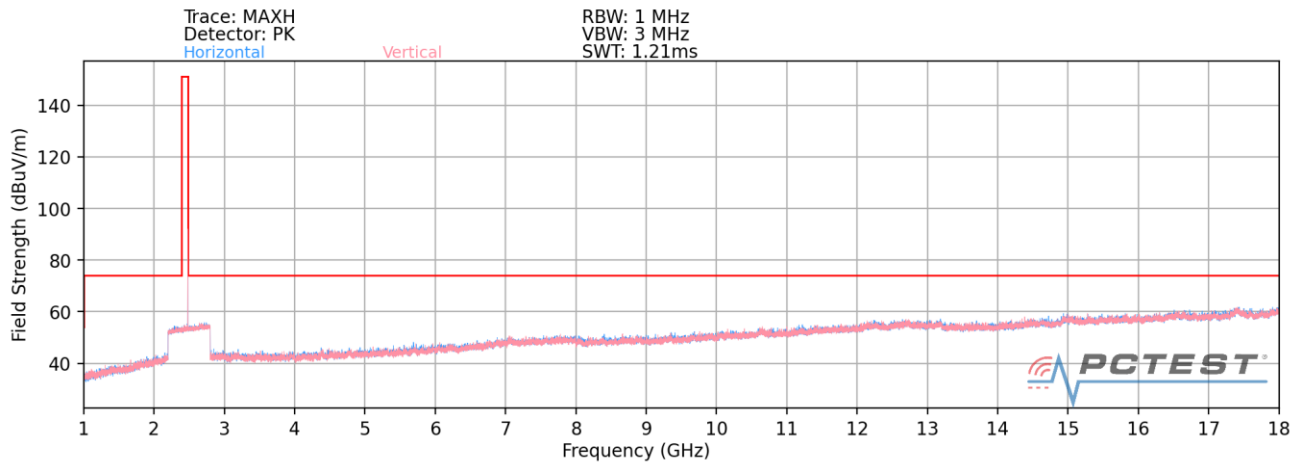
Plot 7-81. Radiated Spurious Plot above 1GHz (BT- Ch. 78) – Closed
