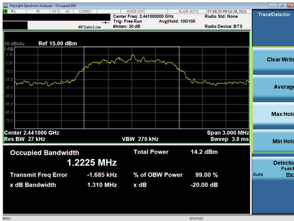
Plot 7-5. 20dB Bandwidth Plot (Bluetooth, 2Mbps – Ch. 39) – South Antenna
