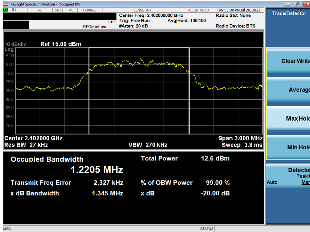
Plot 7-4. 20dB Bandwidth Plot (Bluetooth, 2Mbps – Ch. 0) – South Antenna
