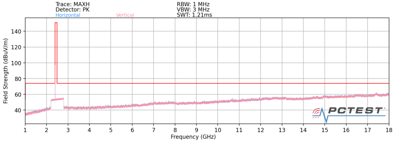
Plot 7-82. Radiated Spurious Plot above 1GHz (BT– Ch. 0) – 300°
