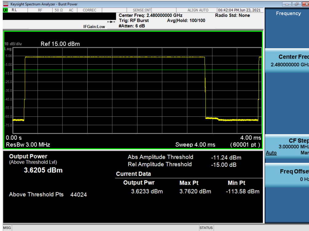
Plot 7-48. Average Conducted Power (1Mbps – Ch. 78) – North Antenna
