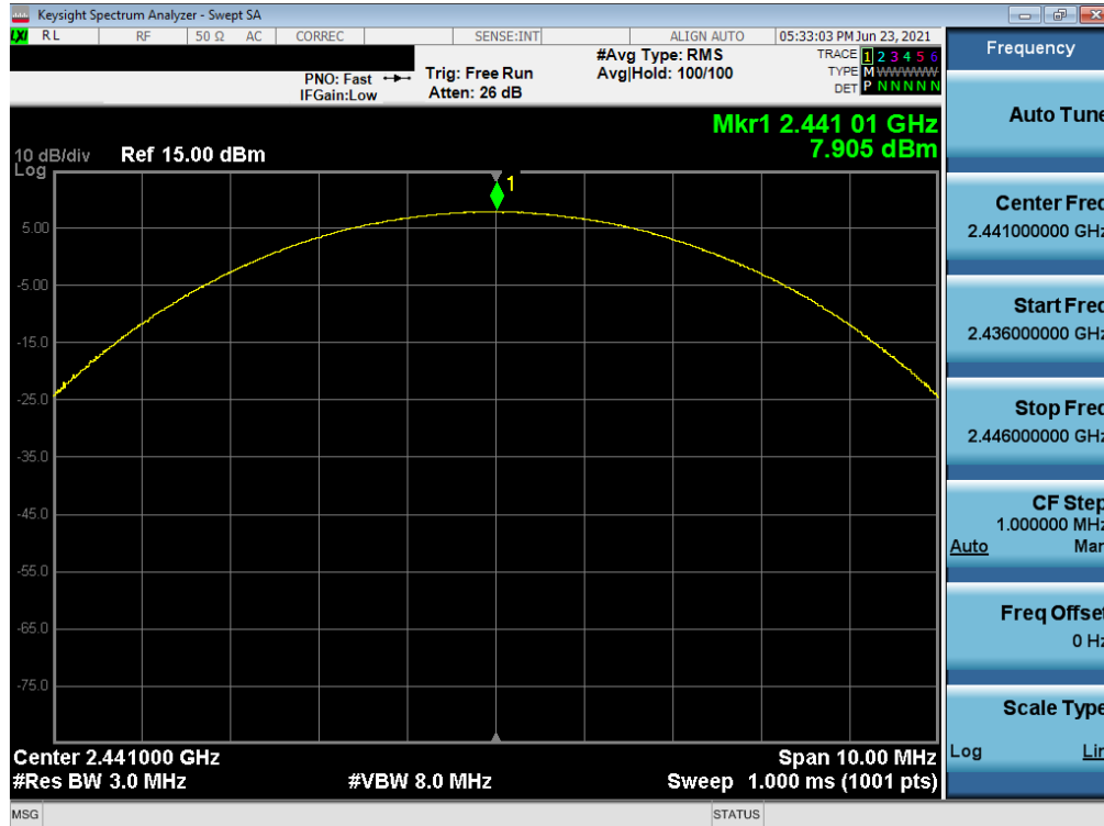
Plot 7-26. Peak Conducted Power (3Mbps - Ch. 39) - South Antenna
