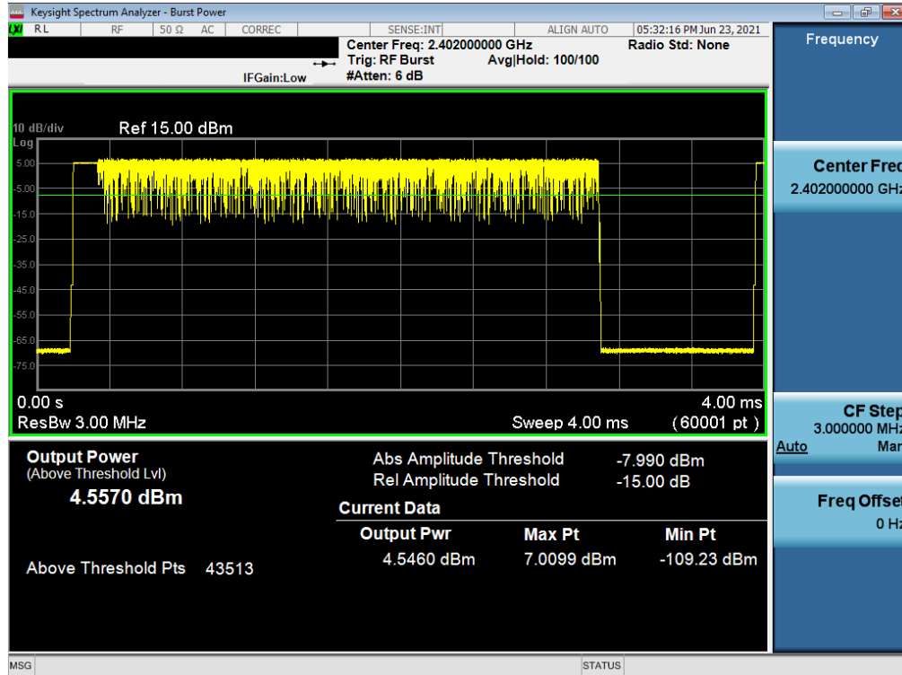
Plot 7-34. Average Conducted Power (3Mbps – Ch. 0) – South Antenna
