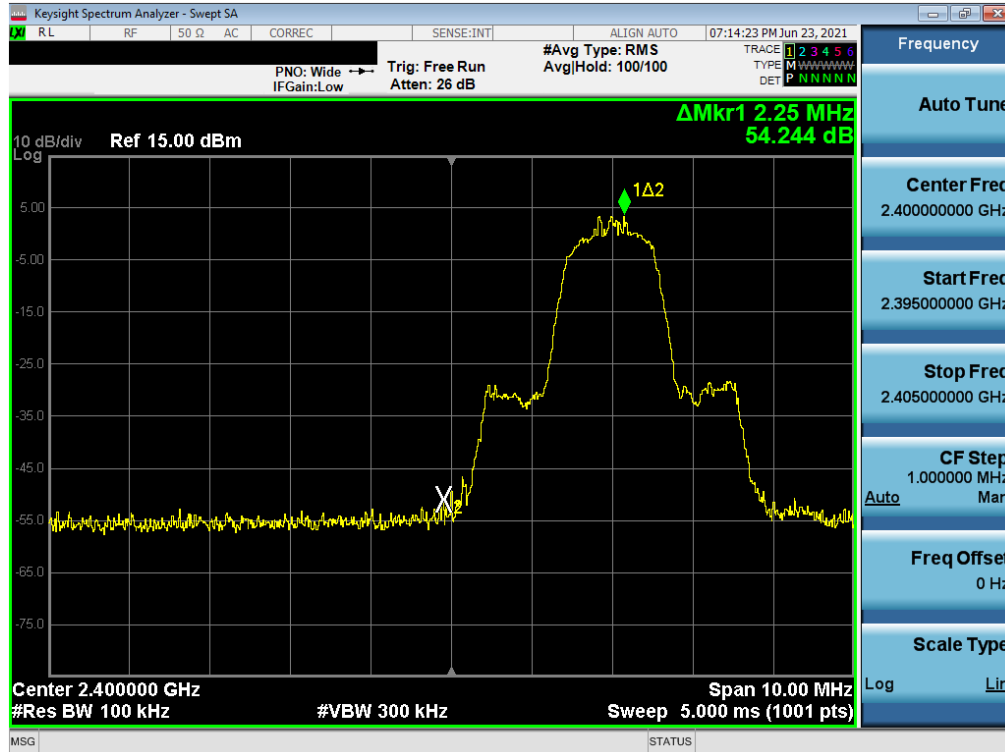
Plot 7-59. Band Edge Plot (Bluetooth with Hopping Disabled, 3 Mbps – Ch. 0) – North Antenna
