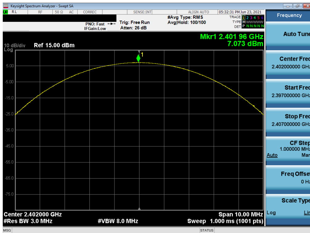
Plot 7-25. Peak Conducted Power (3Mbps – Ch. 0) – South Antenna
