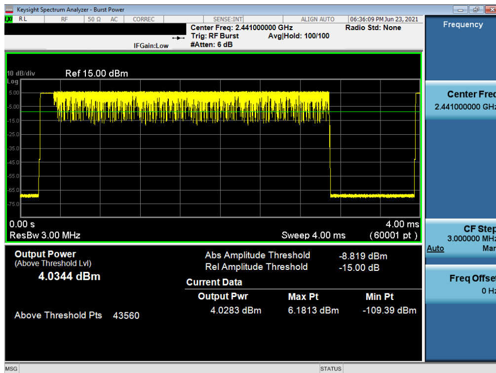
Plot 7-53. Average Conducted Power (3Mbps – Ch. 39) – North Antenna
