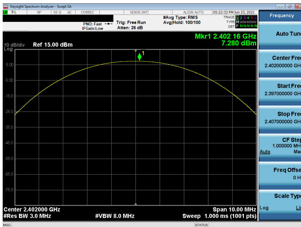
Plot 7-19. Peak Conducted Power (1Mbps – Ch. 0) – South Antenna
