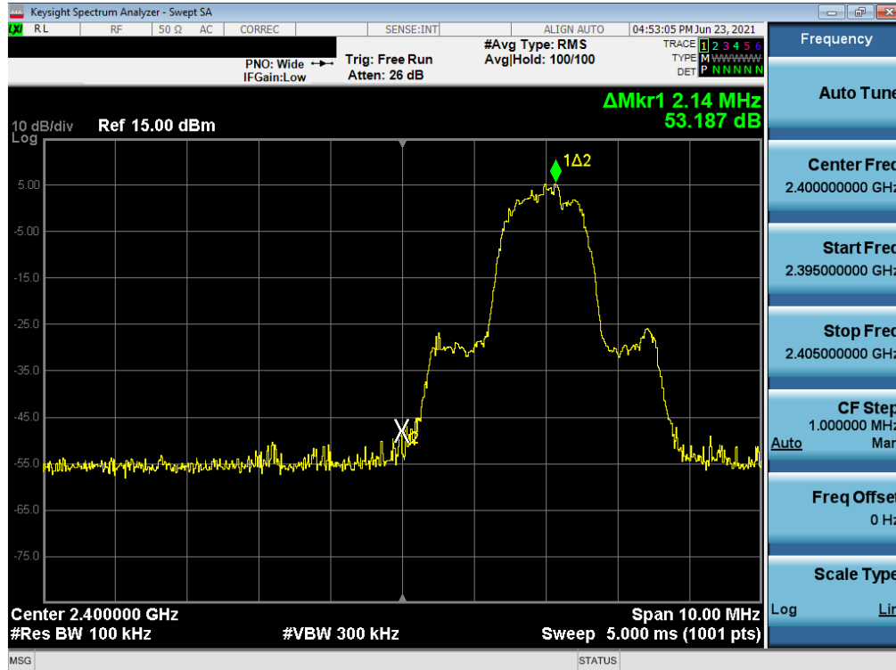
Plot 7-55. Band Edge Plot (Bluetooth with Hopping Disabled, 3 Mbps – Ch. 0) – South Antenna
