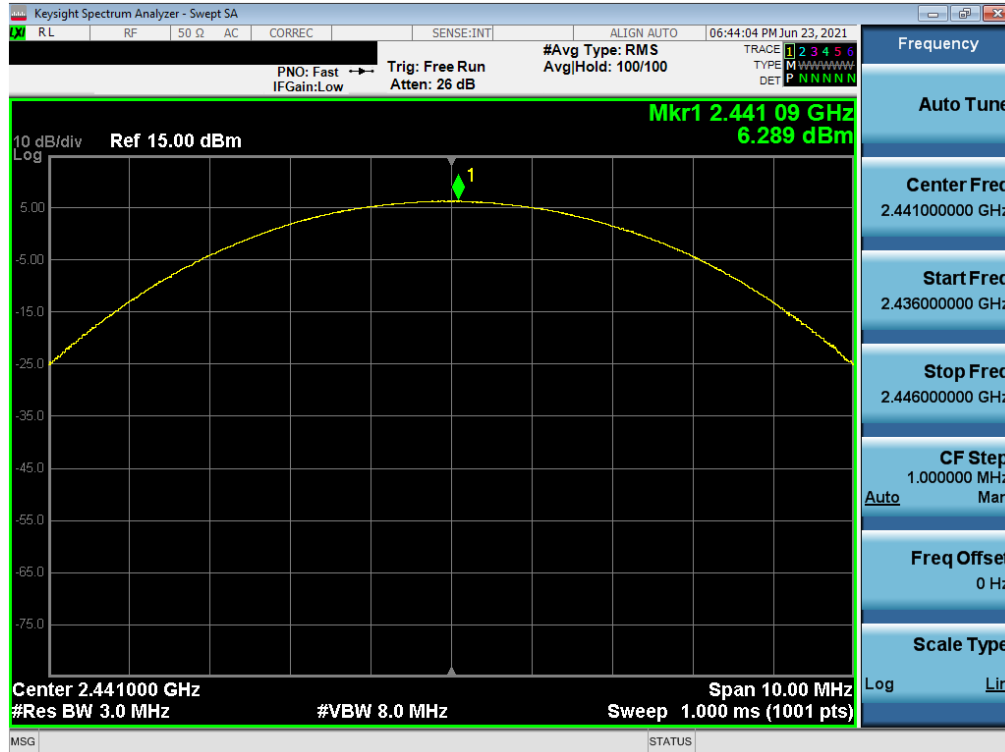
Plot 7-44. Peak Conducted Power (3Mbps – Ch. 39) – North Antenna
