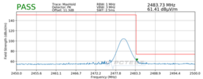
Plot 7-88. Radiated Restricted Upper Band Edge Measurement (Peak)
