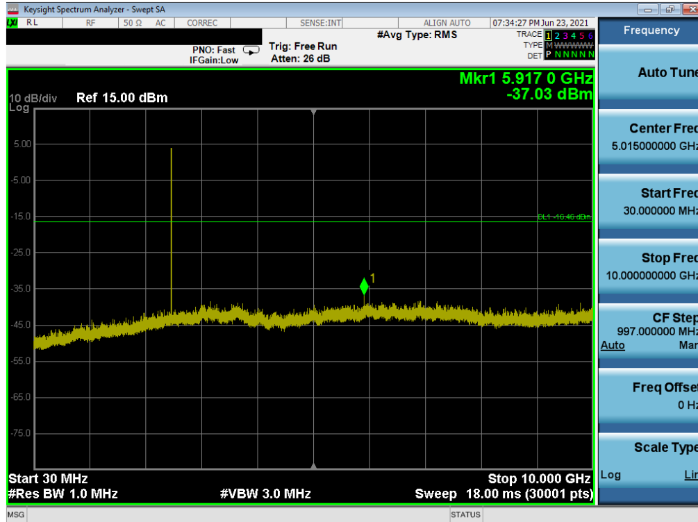
Plot 7-77. Conducted Spurious Plot (Bluetooth, 1Mbps – Ch. 78) – North Antenna
