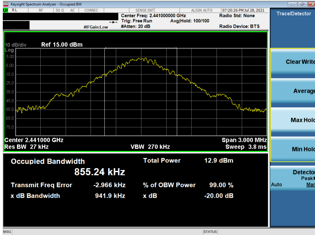
Plot 7-11. 20dB Bandwidth Plot (Bluetooth, 1Mbps – Ch. 39) – North Antenna
