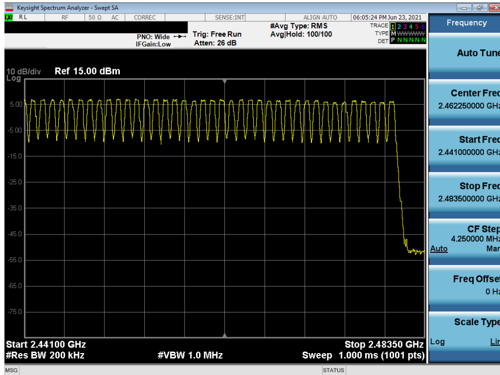
Plot 7-66. High End Spectrum Channel Hopping Plot (Bluetooth)
