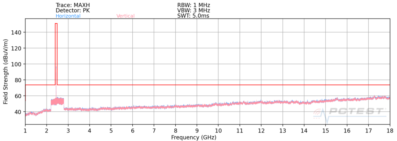
Plot 7-83. Radiated Spurious Plot above 1GHz (BT– Ch. 39) – 300°
