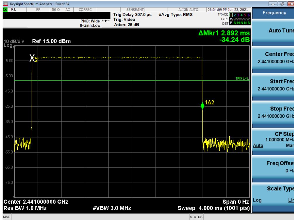
Plot 7-64. Time of Occupancy Plot (Bluetooth)
