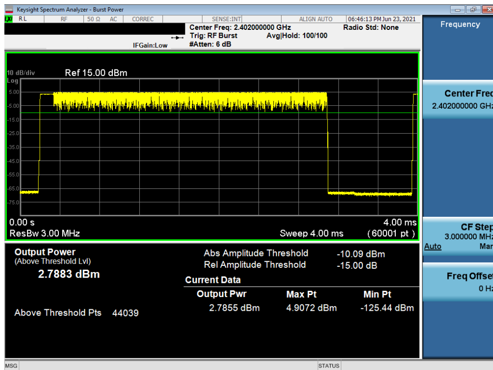
Plot 7-49. Average Conducted Power (2Mbps – Ch. 0) – North Antenna
