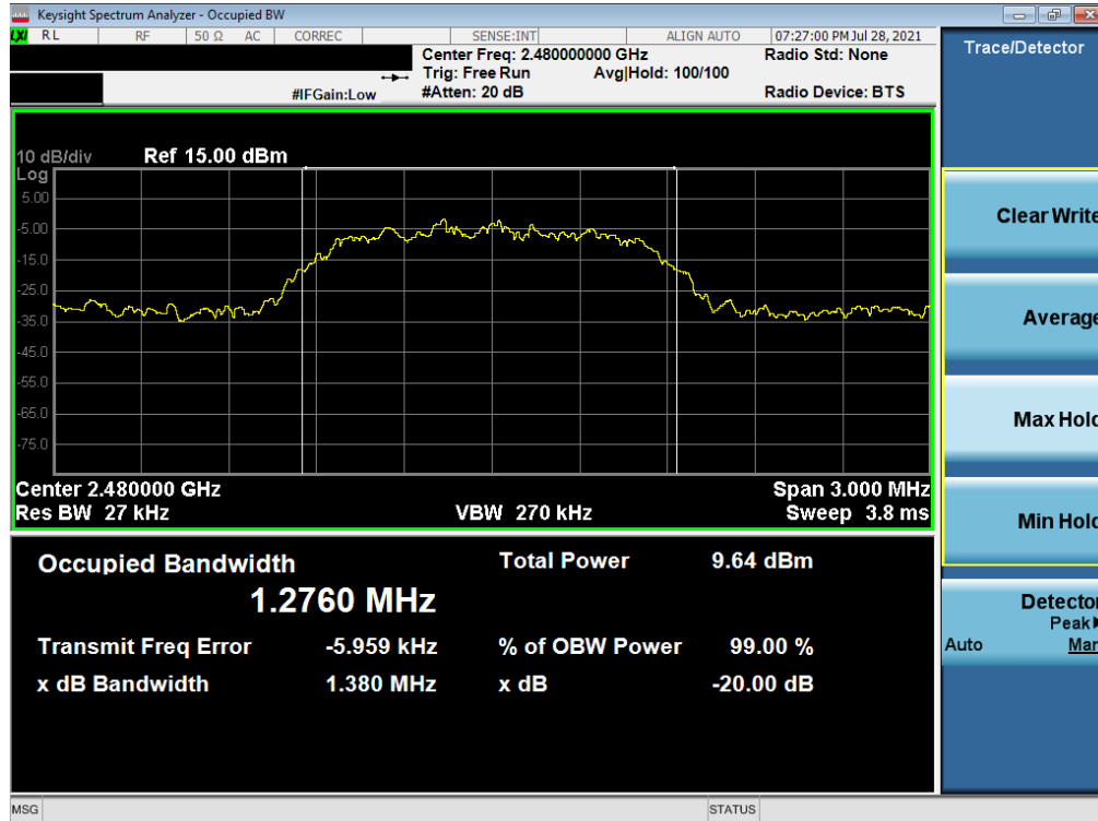
Plot 7-15. 20dB Bandwidth Plot (Bluetooth, 2Mbps – Ch. 78) – North Antenna
