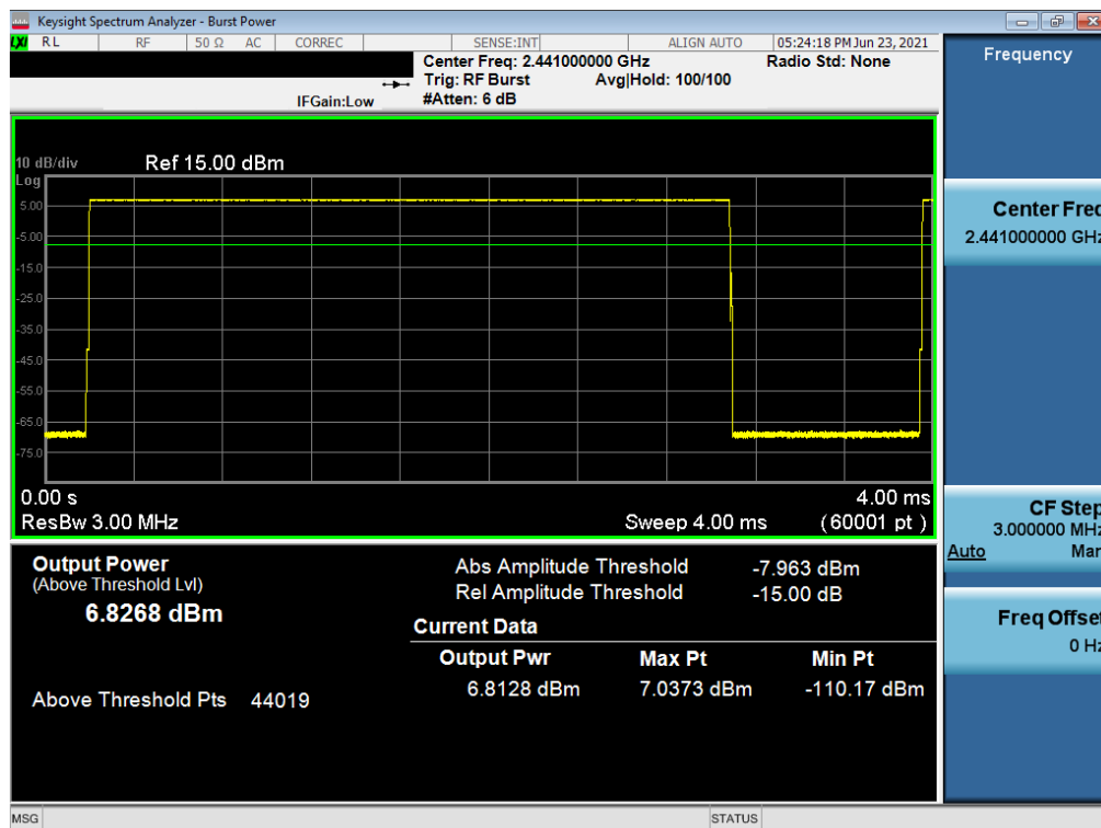
Plot 7-29. Average Conducted Power (1Mbps – Ch. 39) – South Antenna
