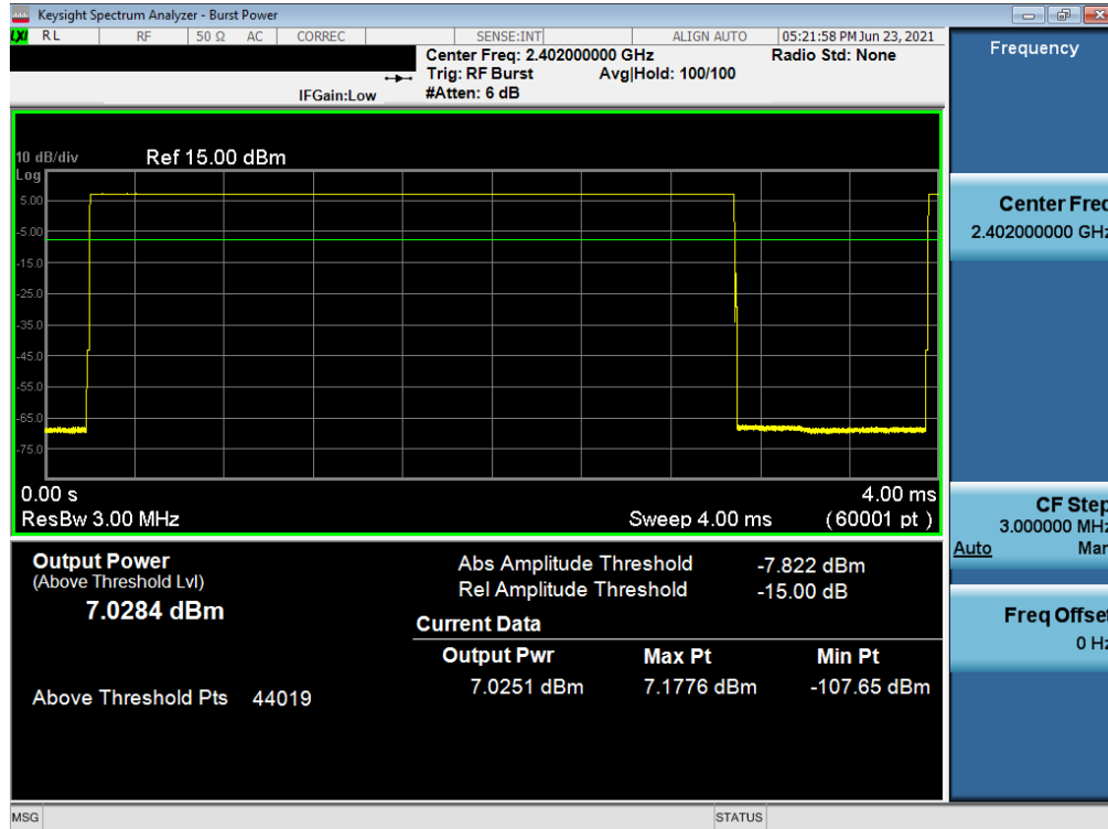
Plot 7-28. Average Conducted Power (1Mbps – Ch. 0) – South Antenna
