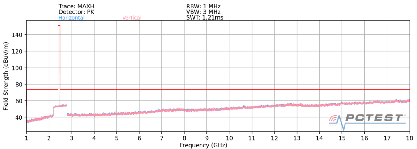
Plot 7-84. Radiated Spurious Plot above 1GHz (BT– Ch. 78) – 300°
