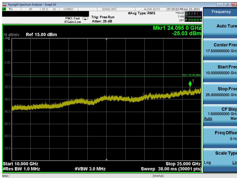
Plot 7-78. Conducted Spurious Plot (Bluetooth, 1Mbps – Ch. 78) – North Antenna
