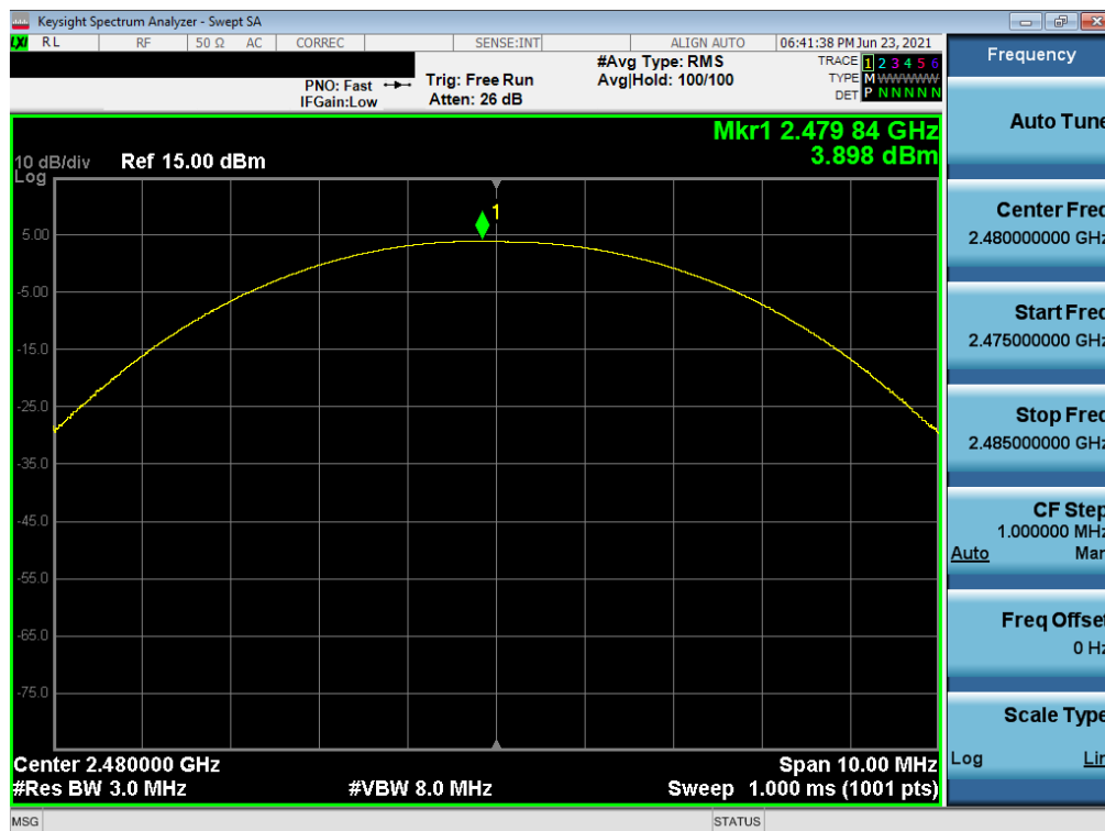
Plot 7-39. Peak Conducted Power (1Mbps – Ch. 78) – North Antenna
