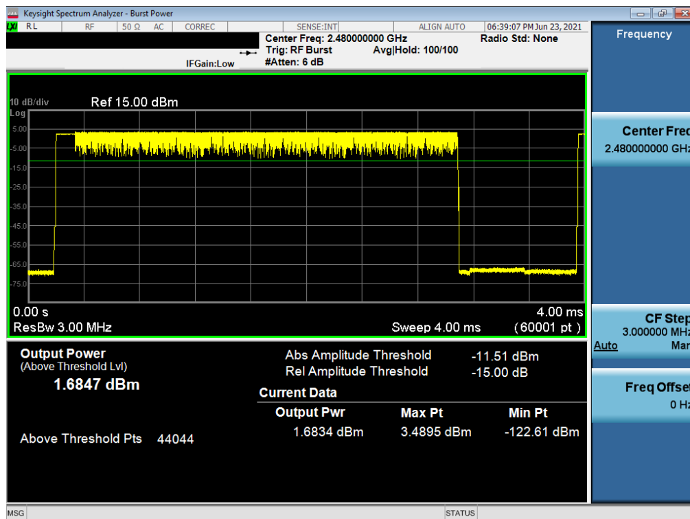
Plot 7-51. Average Conducted Power (2Mbps – Ch. 78) – North Antenna
