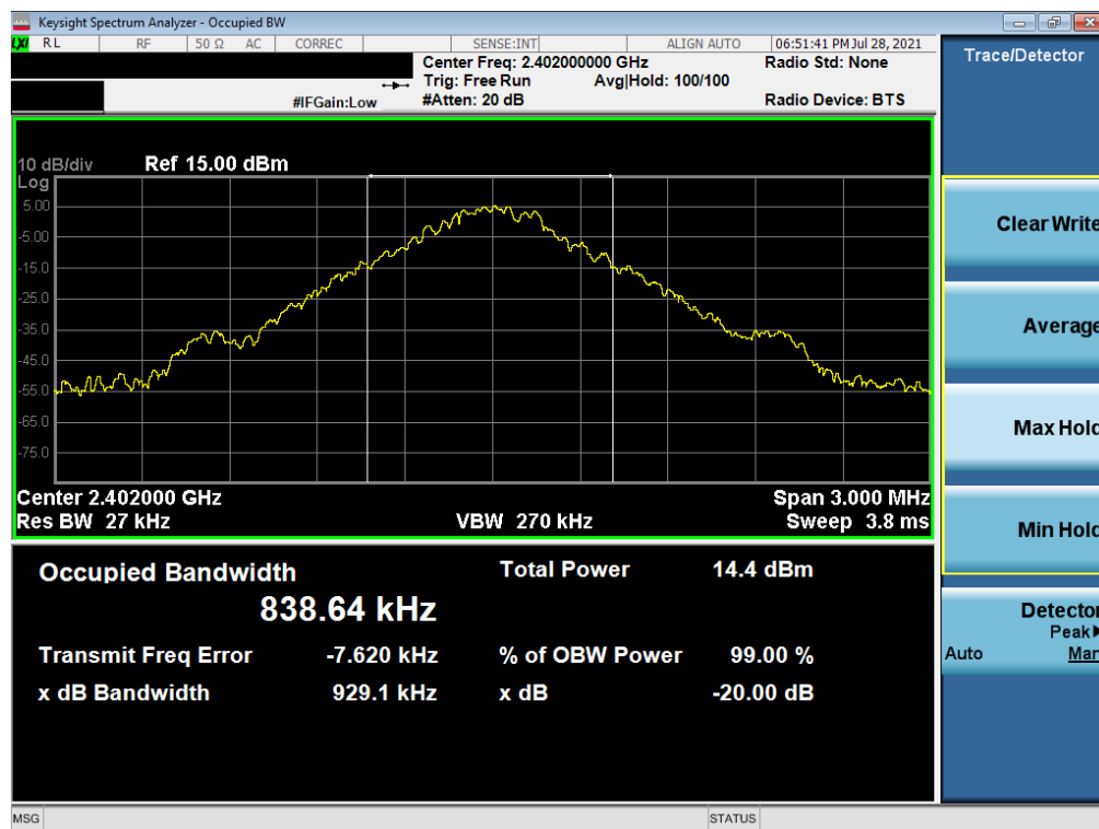
Plot 7-1. 20dB Bandwidth Plot (Bluetooth, 1Mbps – Ch. 0) – South Antenna
