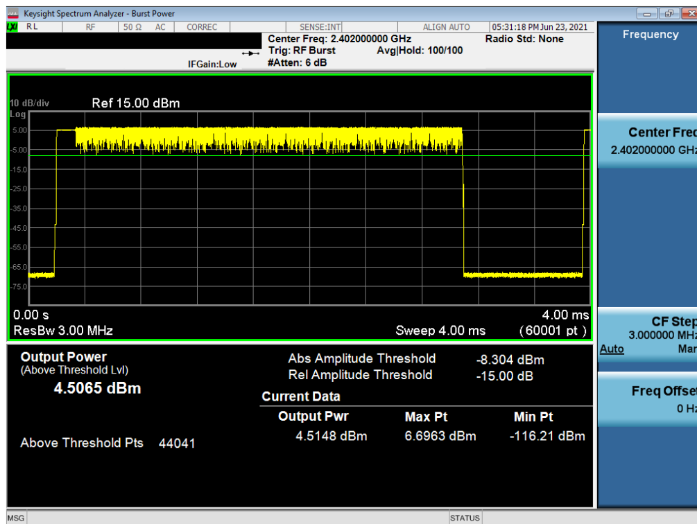
Plot 7-31. Average Conducted Power (2Mbps – Ch. 0) – South Antenna
