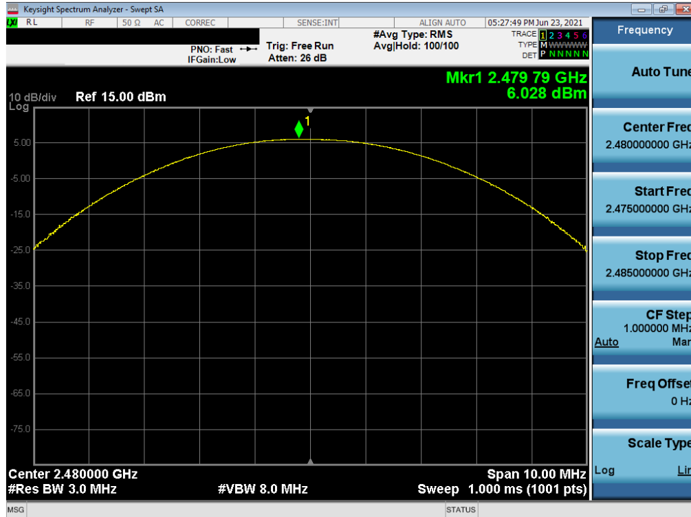
Plot 7-24. Peak Conducted Power (2Mbps – Ch. 78) – South Antenna
