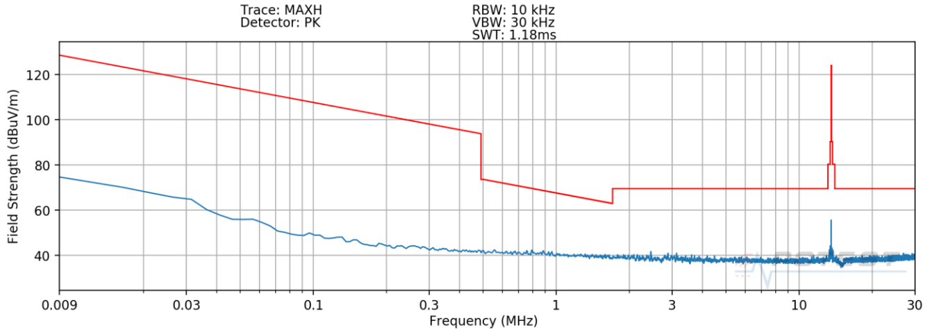
Plot 7-4. Radiated Spurious Plot 9kHz – 30MHz (Pol. X) Half
