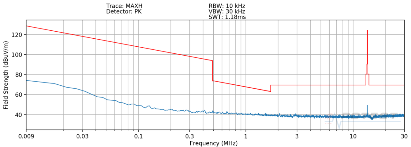
Plot 7-6. Radiated Spurious Plot 9kHz – 30MHz (Pol. Z) Half
