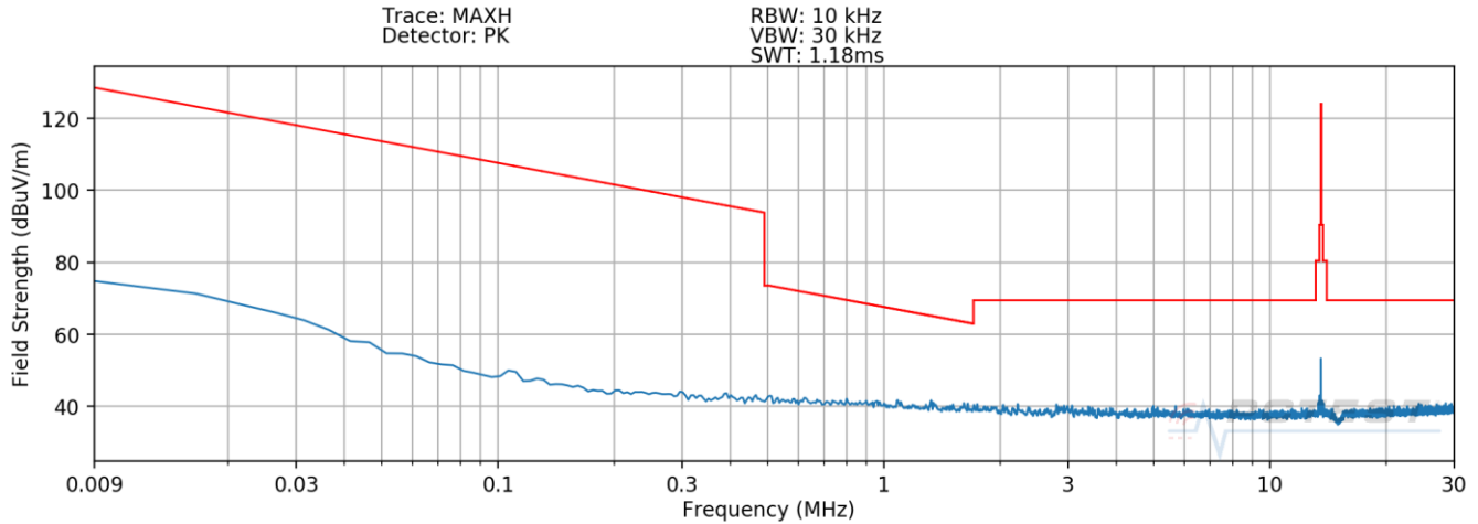
Plot 7-7. Radiated Spurious Plot 9kHz – 30MHz (Pol. X) Closed
