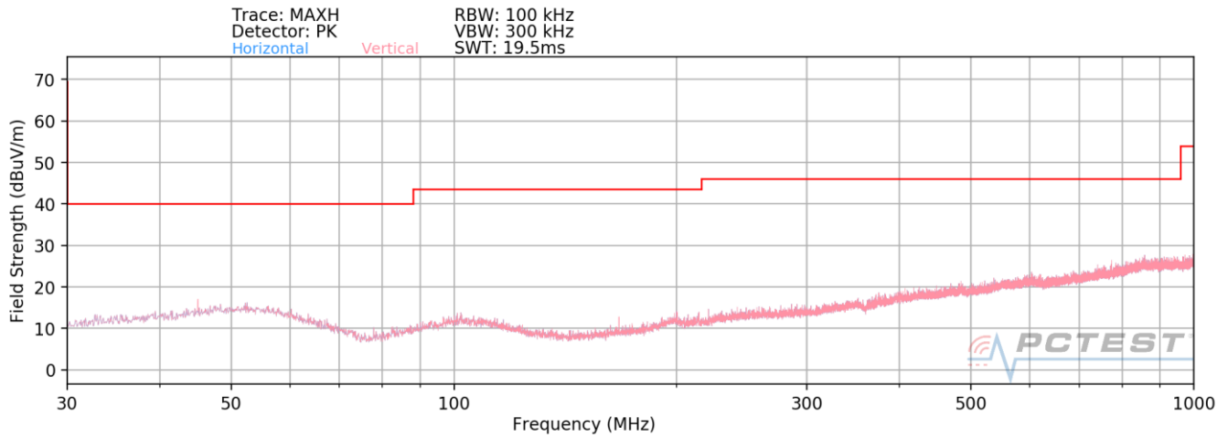
Plot 7-10. Radiated Spurious Plot 30MHz – 1GHz
