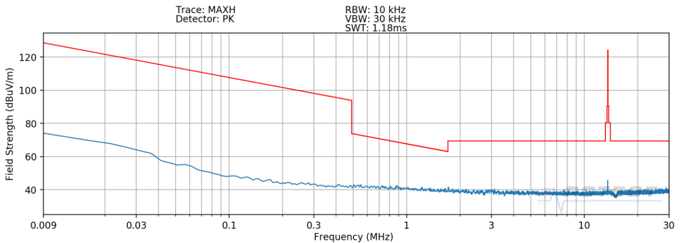
Plot 7-9. Radiated Spurious Plot 9kHz – 30MHz (Pol. Z) Closed
