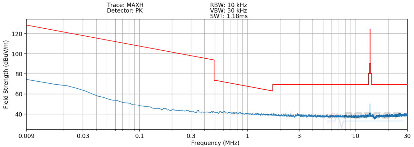
Plot 7-8. Radiated Spurious Plot 9kHz – 30MHz (Pol. Y) Closed
