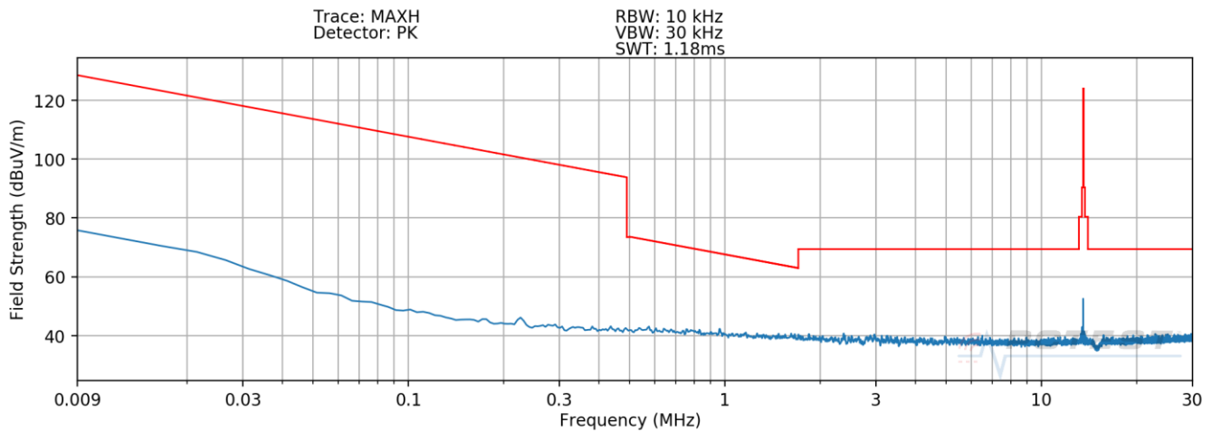
Plot 7-5. Radiated Spurious Plot 9kHz – 30MHz (Pol. Y) Half
