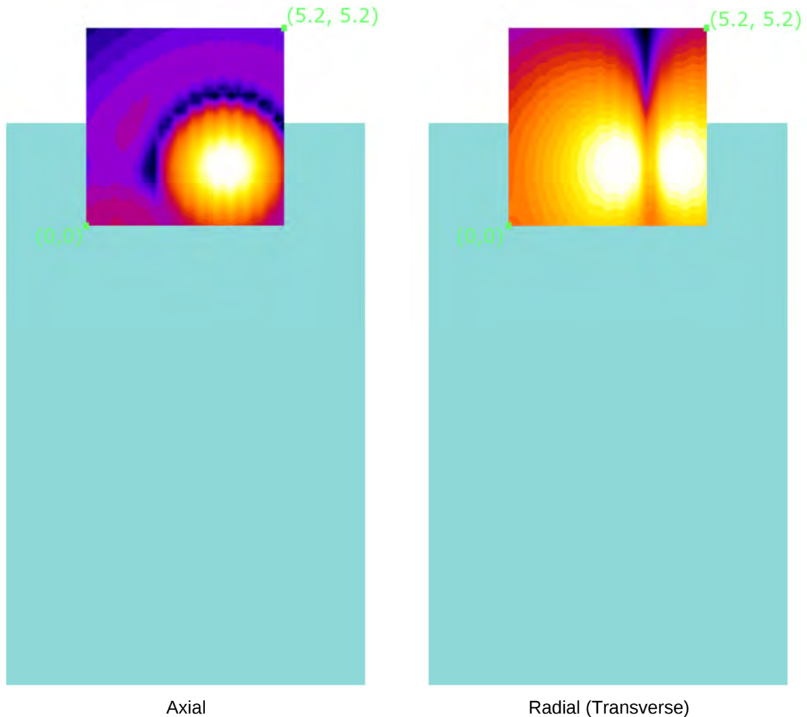
Figure 9-1 T-Coil Scan Overlay Magnetic Field Distributions
