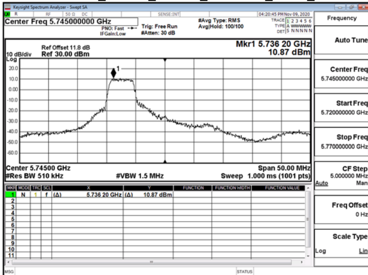
802.11ax_20MHz_ChainA_5745MHz_RU52_37
