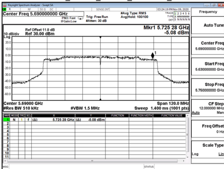
802.11ac_80MHz_ChainA_5690MHz_UNII 3
