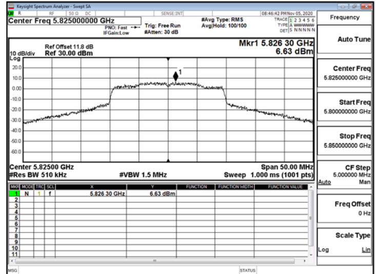
802.11ax_20MHz_ChainA_5825MHz_RU106_54
