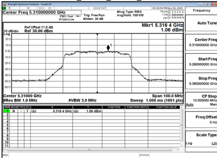
802.11ax_40MHz_ChainA_5310MHz_RU242_62
