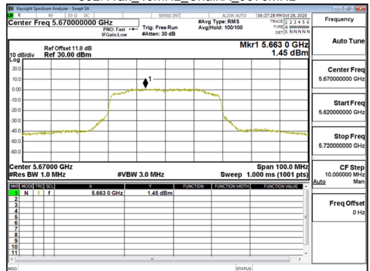
802.11ax_40MHz_ChainA_5670MHz
