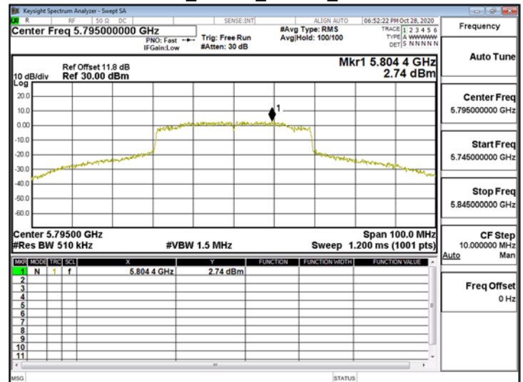
802.11ax_40MHz_ChainA_5795MHz
