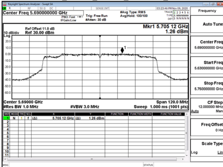
802.11ac_80MHz_ChainA_5690MHz_UNII 3
