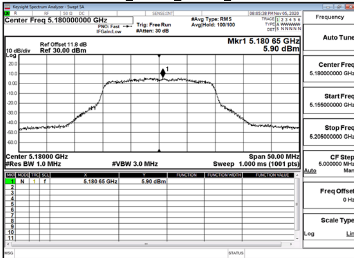
802.11ax_20MHz_ChainA_5180MHz_RU106_53
