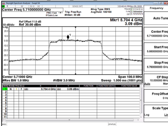
802.11ax_40MHz_ChainA_5710MHz_UNII 3
