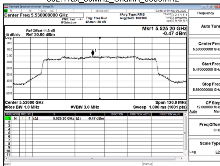
802.11ax_80MHz_ChainA_5530MHz
