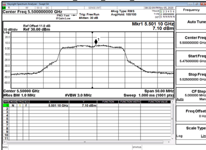
802.11ax_20MHz_ChainA_5500MHz_RU106_53
