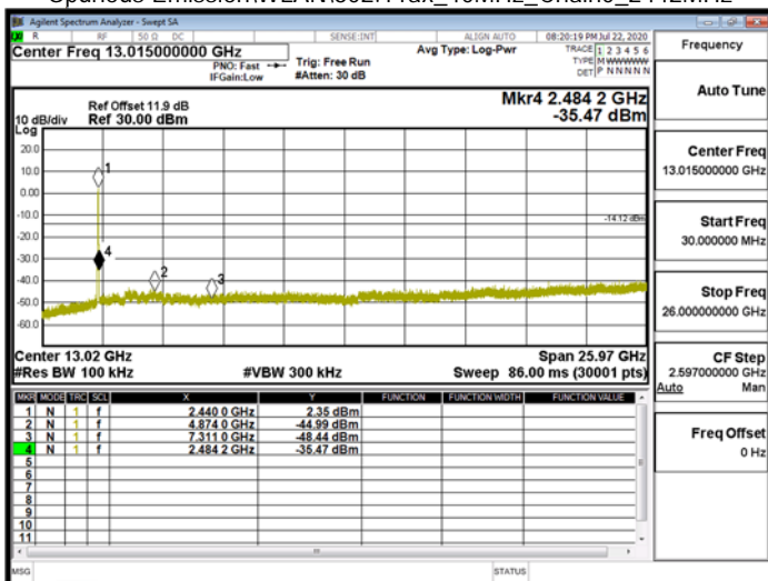
Spurious Emission\WLAN\802.11ax_40MHz_Chain0_2442MHz
