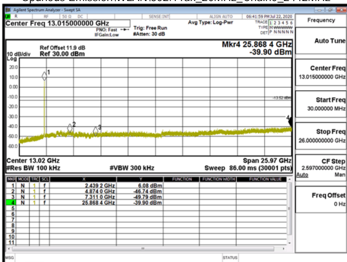
Spurious Emission\WLAN\802.11ax_20MHz_Chain0_2442MHz
