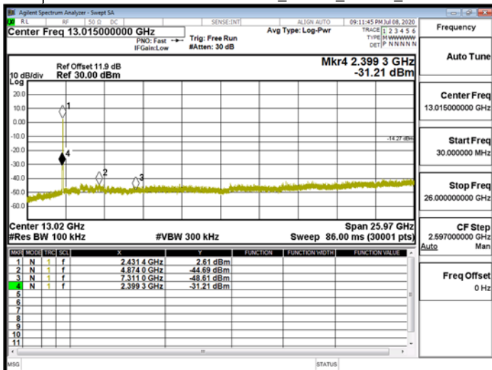
Spurious Emission\WLAN\802.11ax_40MHz_Chain0_2442MHz
