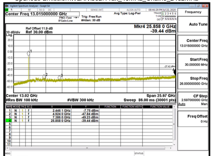
Spurious Emission\WLAN\802.11ax_40MHz_Chain0_2462MHz
