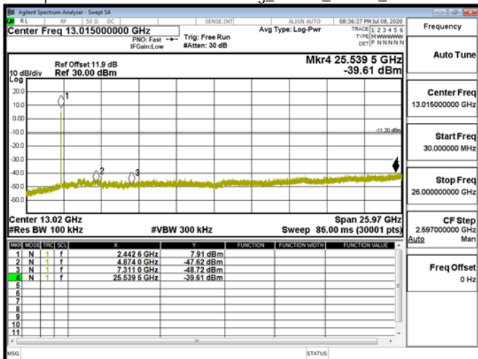
Spurious Emission\WLAN\802.11g_20MHz_Chain0_2442MHz
