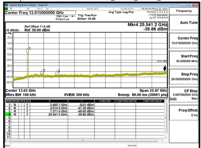
Spurious Emission\WLAN\802.11n_40MHz_Chain0_2462MHz
