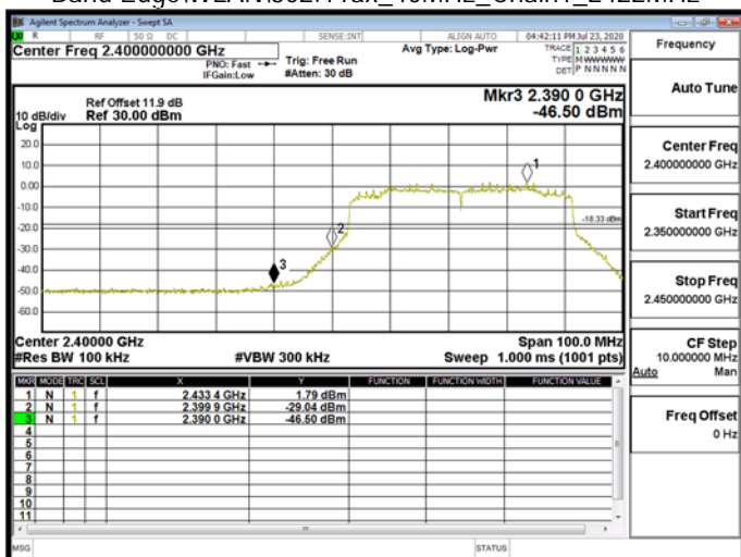
Band Edge\WLAN\802.11ax_40MHz_Chain1_2422MHz
