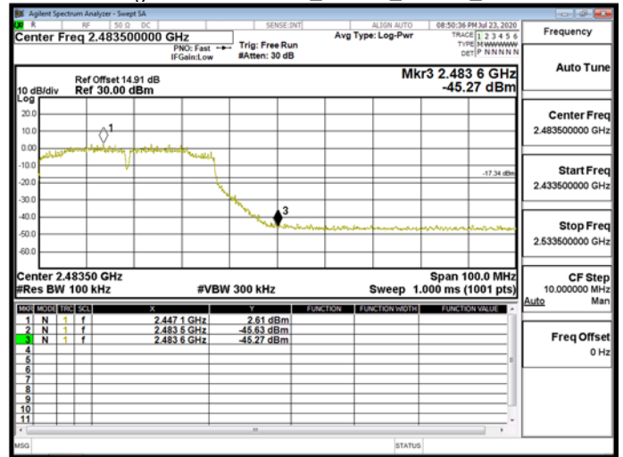
Band EdgeWLAN\802.11n_40MHz_Chain1_2457MHz
