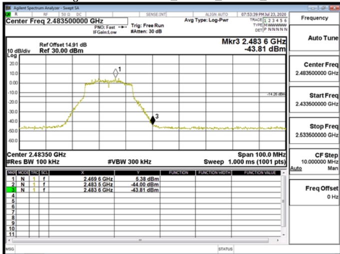
Band Edge\WLAN\802.11n_20MHz_Chain1_2467MHz
