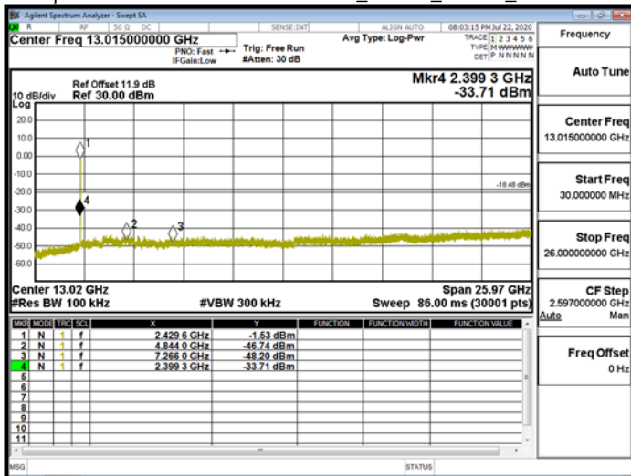
Spurious Emission\WLAN\802.11ax_40MHz_Chain0_2437MHz
