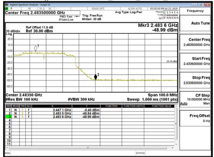
Band Edge\WLAN\802.11ax_40MHz_Chain1_2457MHz
