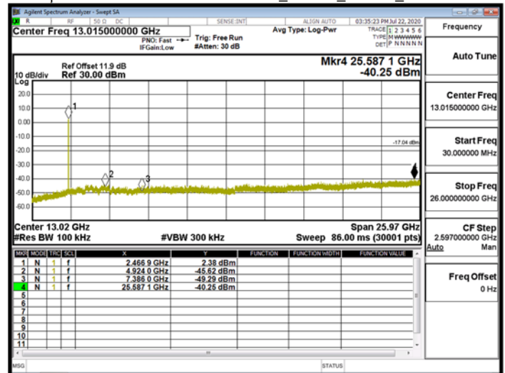
Spurious Emission\WLAN\802.11n_20MHz_Chain0_2467MHz
