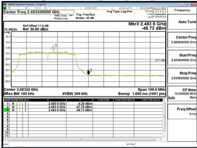
Band Edge\WLAN\802.11n_40MHz_Chain1_2462MHz
