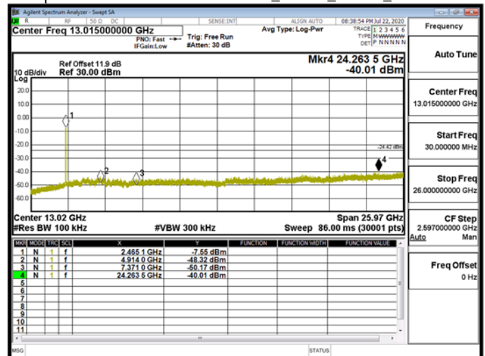
Spurious Emission\WLAN\802.11ax_40MHz_Chain0_2462MHz
