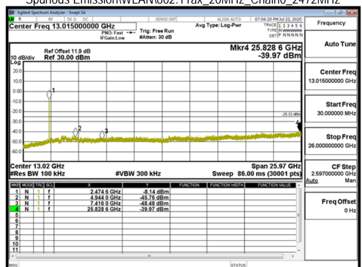
Spurious Emission\WLAN\802.11ax_20MHz_Chain0_2472MHz
