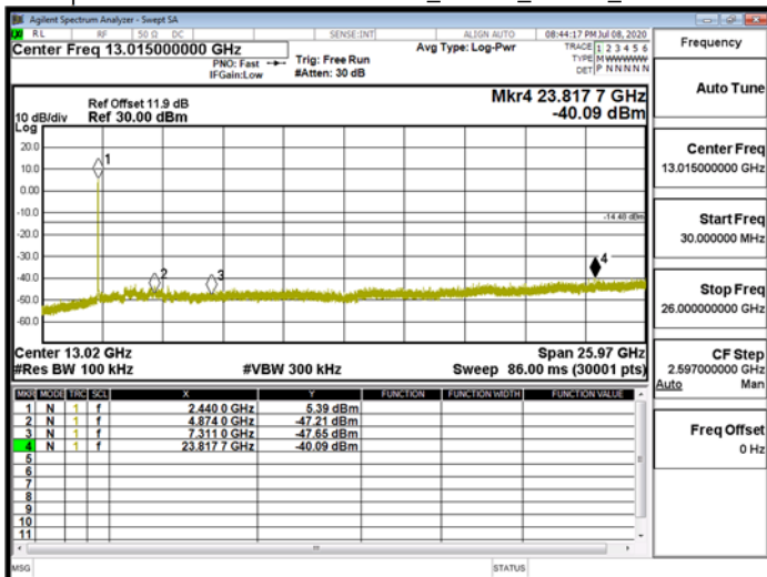
Spurious Emission\WLAN\802.11n_20MHz_Chain0_2442MHz
