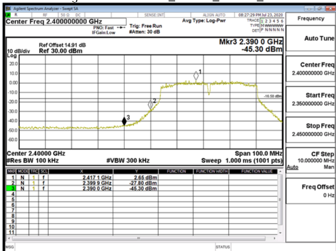
Band EdgeWLAN\802.11n_40MHz_Chain1_2422MHz
