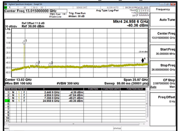
Spurious Emission\WLAN\802.11n_40MHz_Chain0_2457MHz
