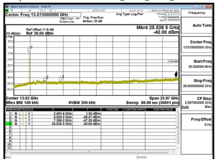
Spurious Emission\WLAN\802.11ax_20MHz_Chain0_2467MHz
