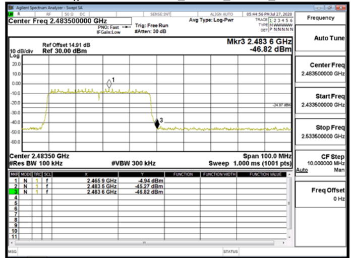
Band Edge\WLAN\802.11ax_40MHz_Chain1_2462MHz
