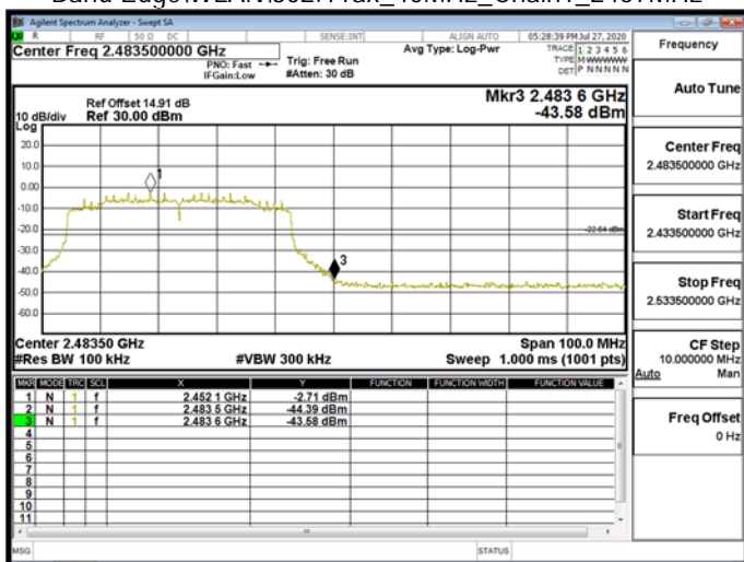
Band Edge\WLAN\802.11ax_40MHz_Chain1_2457MHz
