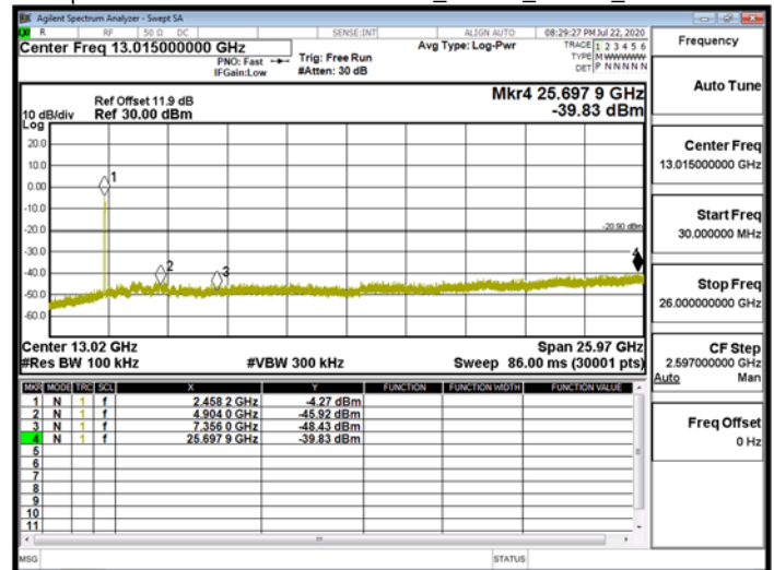
Spurious Emission\WLAN\802.11ax_40MHz_Chain0_2457MHz
