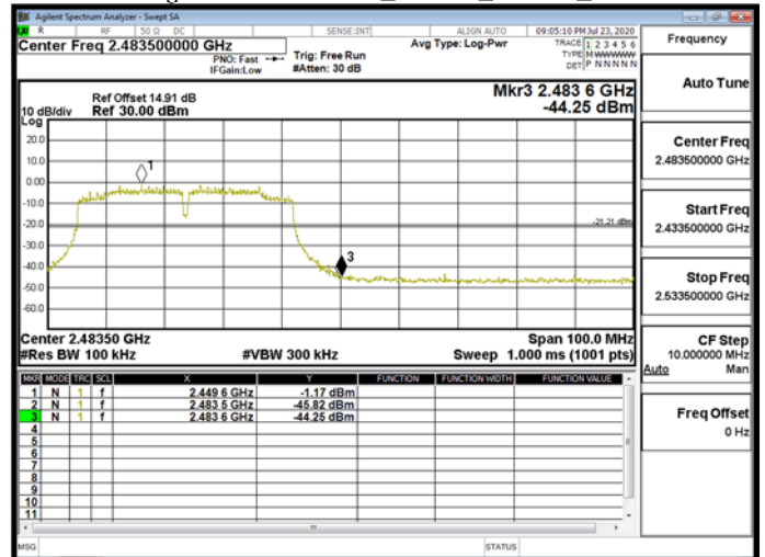
Band EdgeWLAN\802.11n_40MHz_Chain1_2462MHz
