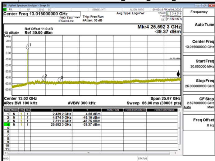
Spurious Emission\WLAN\802.11ax_20MHz_Chain0_2442MHz
