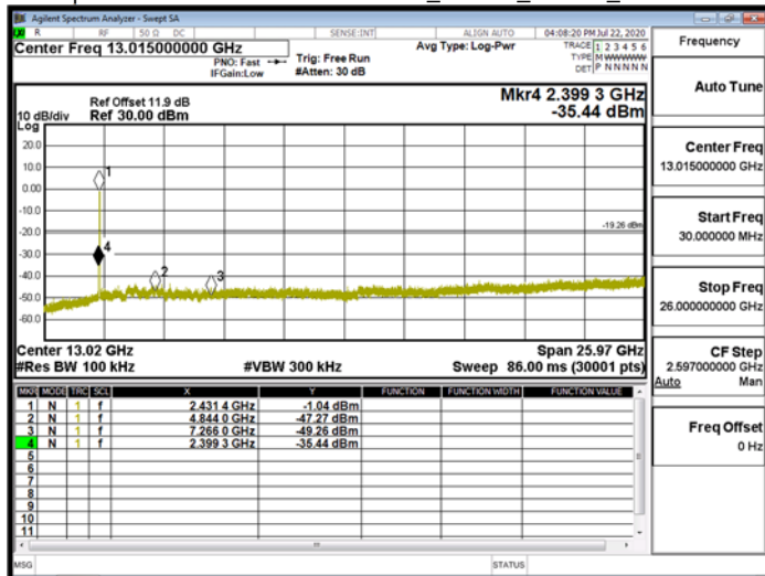
Spurious Emission\WLAN\802.11n_40MHz_Chain0_2437MHz
