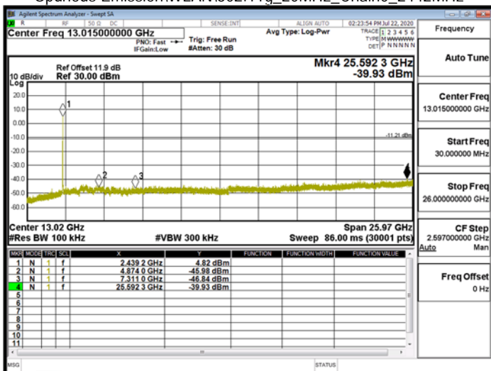
Spurious Emission\WLAN\802.11g_20MHz_Chain0_2442MHz
