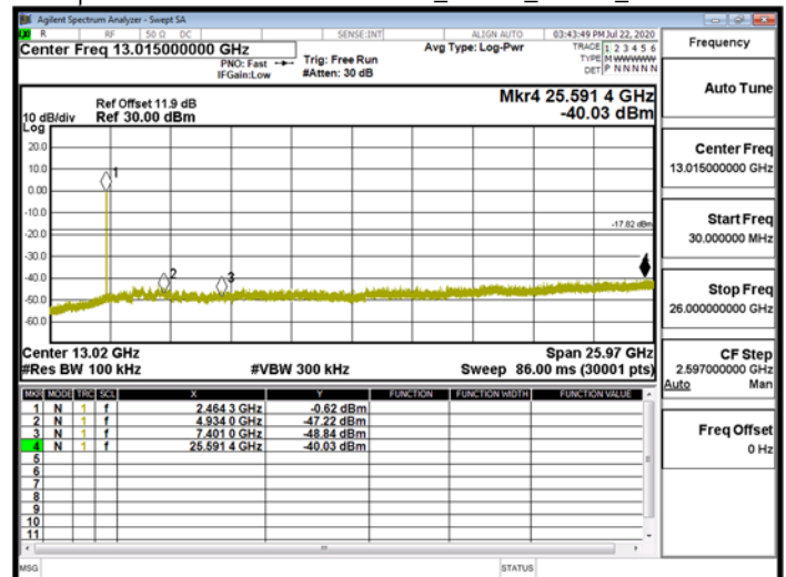
Spurious Emission\WLAN\802.11n_20MHz_Chain0_2472MHz
