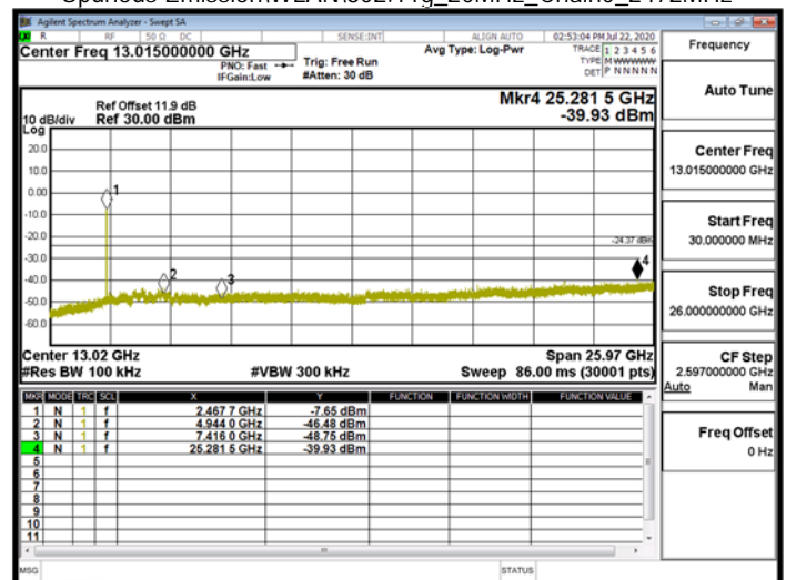
Spurious Emission\WLAN\802.11g_20MHz_Chain0_2472MHz
