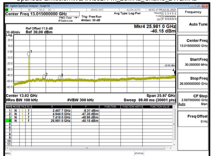
Spurious Emission\WLAN\802.11n_20MHz_Chain0_2472MHz
