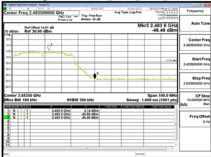
Band Edge\WLAN\802.11ax_40MHz_Chain1_2457MHz
