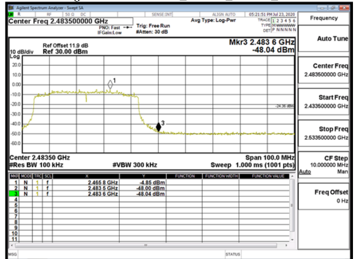
Band Edge\WLAN\802.11ax_40MHz_Chain1_2462MHz
