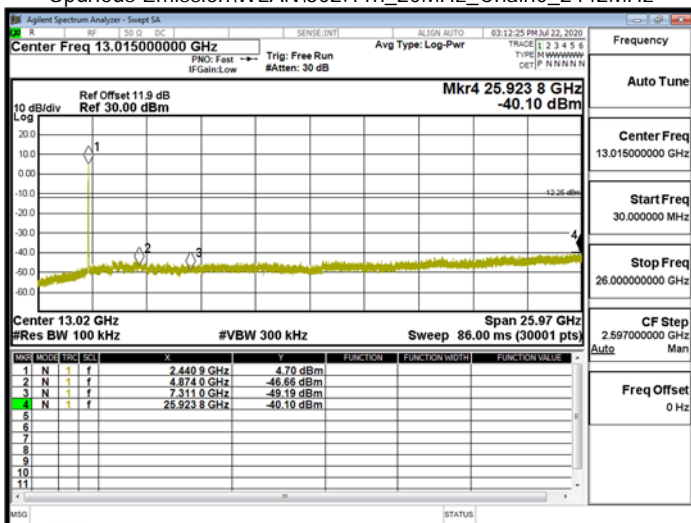
Spurious Emission\WLAN\802.11n_20MHz_Chain0_2442MHz
