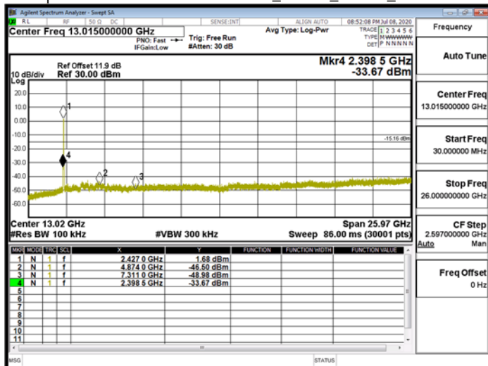
Spurious Emission\WLAN\802.11n_40MHz_Chain0_2442MHz
