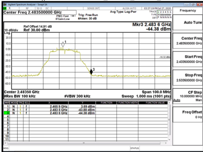
Band EdgeWLAN\802.11ax_20MHz_Chain1_2472MHz
