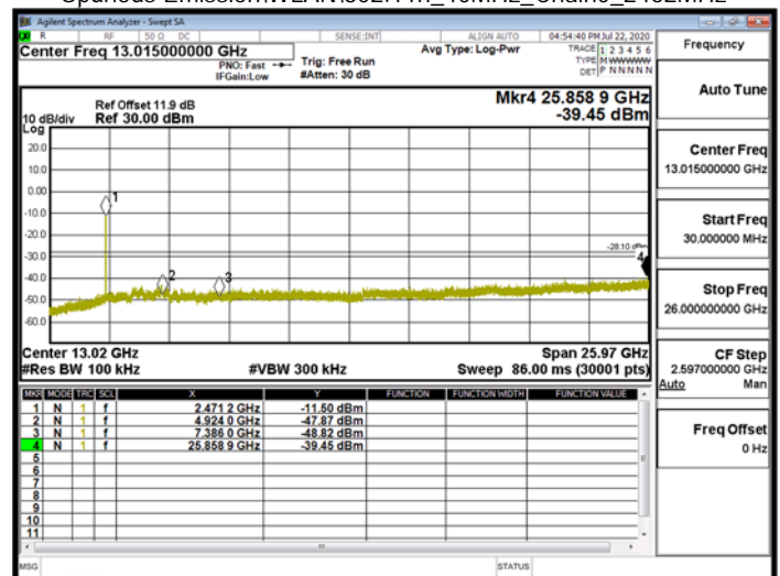
Spurious Emission\WLAN\802.11n_40MHz_Chain0_2462MHz
