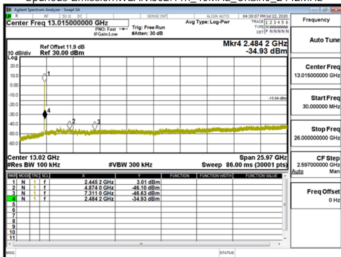
Spurious Emission\WLAN\802.11n_40MHz_Chain0_2442MHz
