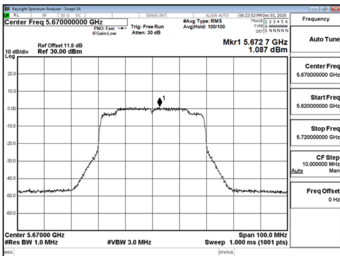
802.11ax_40MHz_5670MHz-5670
