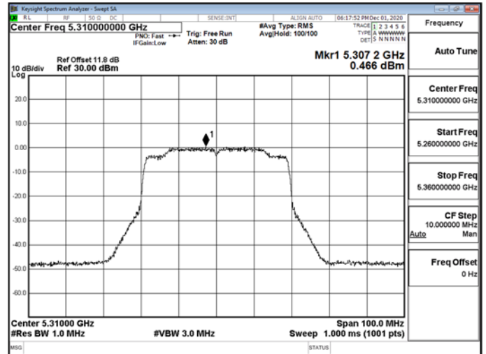
802.11ax_40MHz_RU_242_62_5310MHz-5310
