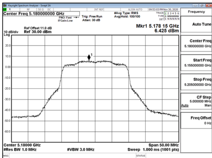
802.11ax_20MHz_RU_106_53_5180MHz-5180
