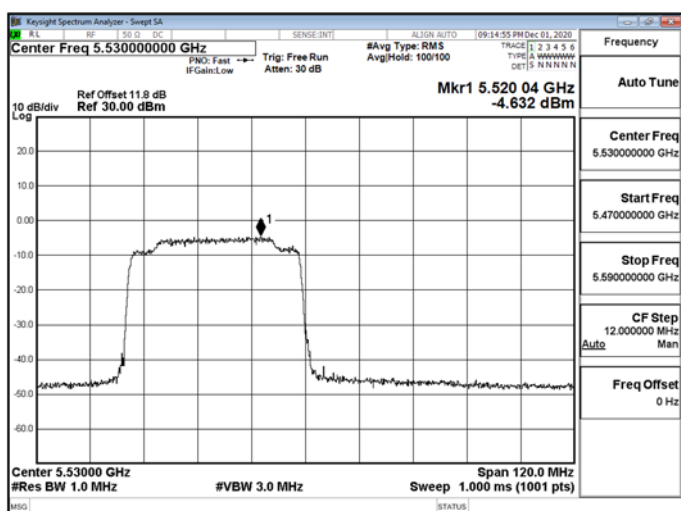
802.11ax_80MHz_RU_484_65_5530MHz-5530
