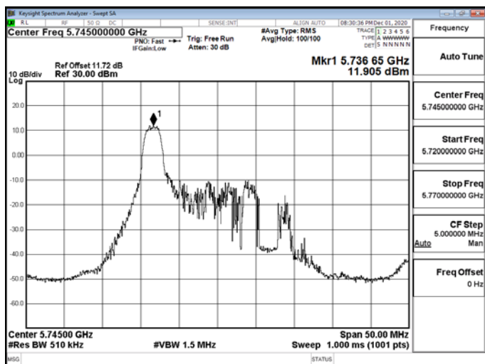
802.11ax_20MHz_RU_52_37_5745MHz-5745
