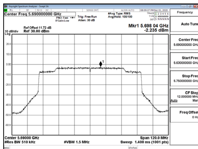
802.11ax_80MHz_5690MHz_UNII 3
