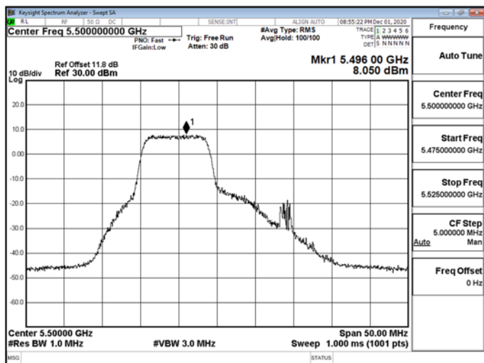
802.11ax_20MHz_RU_26_0_5500MHz-5500
