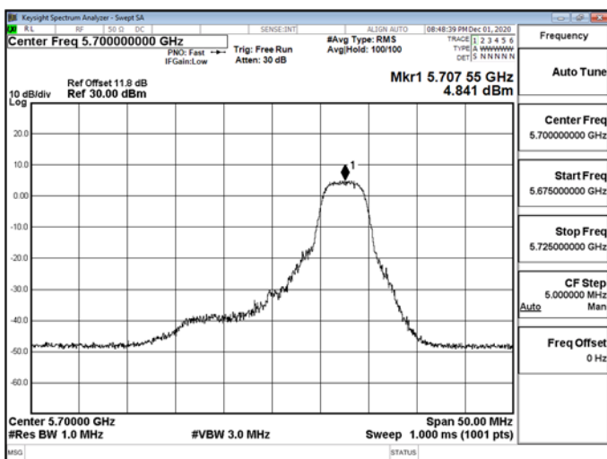
802.11ax_20MHz_RU_52_40_5700MHz-5700
