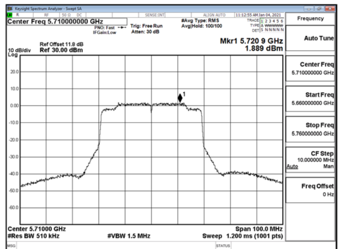
802.11ax_40MHz_5710MHz_UNII 3
