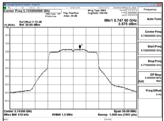
802.11ax_20MHz_5745MHz-5745
