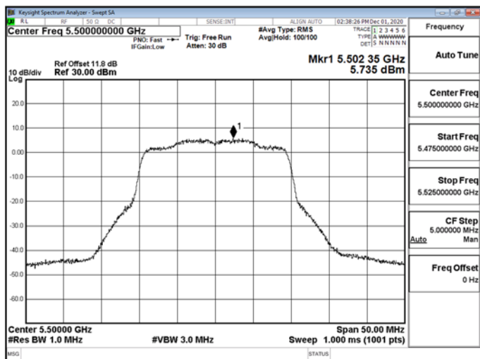
802.11ax_20MHz_RU_106_53_5500MHz-5500
