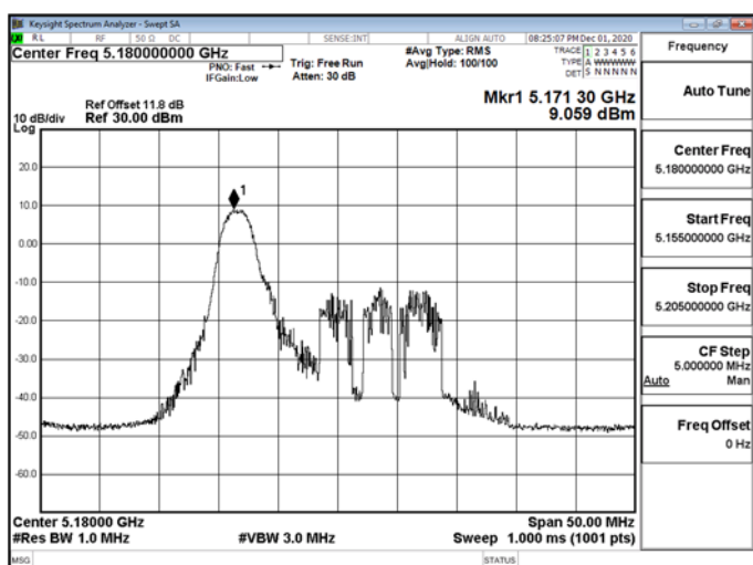
802.11ax_20MHz_RU_26_0_5180MHz-5180
