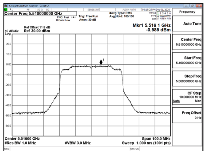
802.11ax_40MHz_5510MHz-5510
