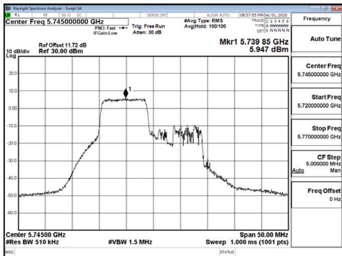
802.11ax_20MHz_RU_26_0_5745MHz-5745
