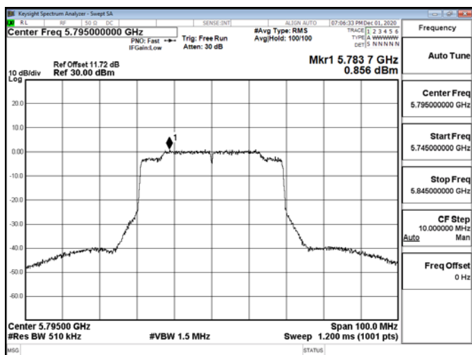
802.11ax_40MHz_5795MHz-5795
