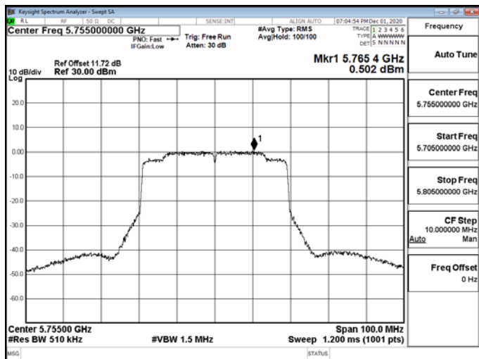
802.11ax_40MHz_RU_242_61_5755MHz-5755
