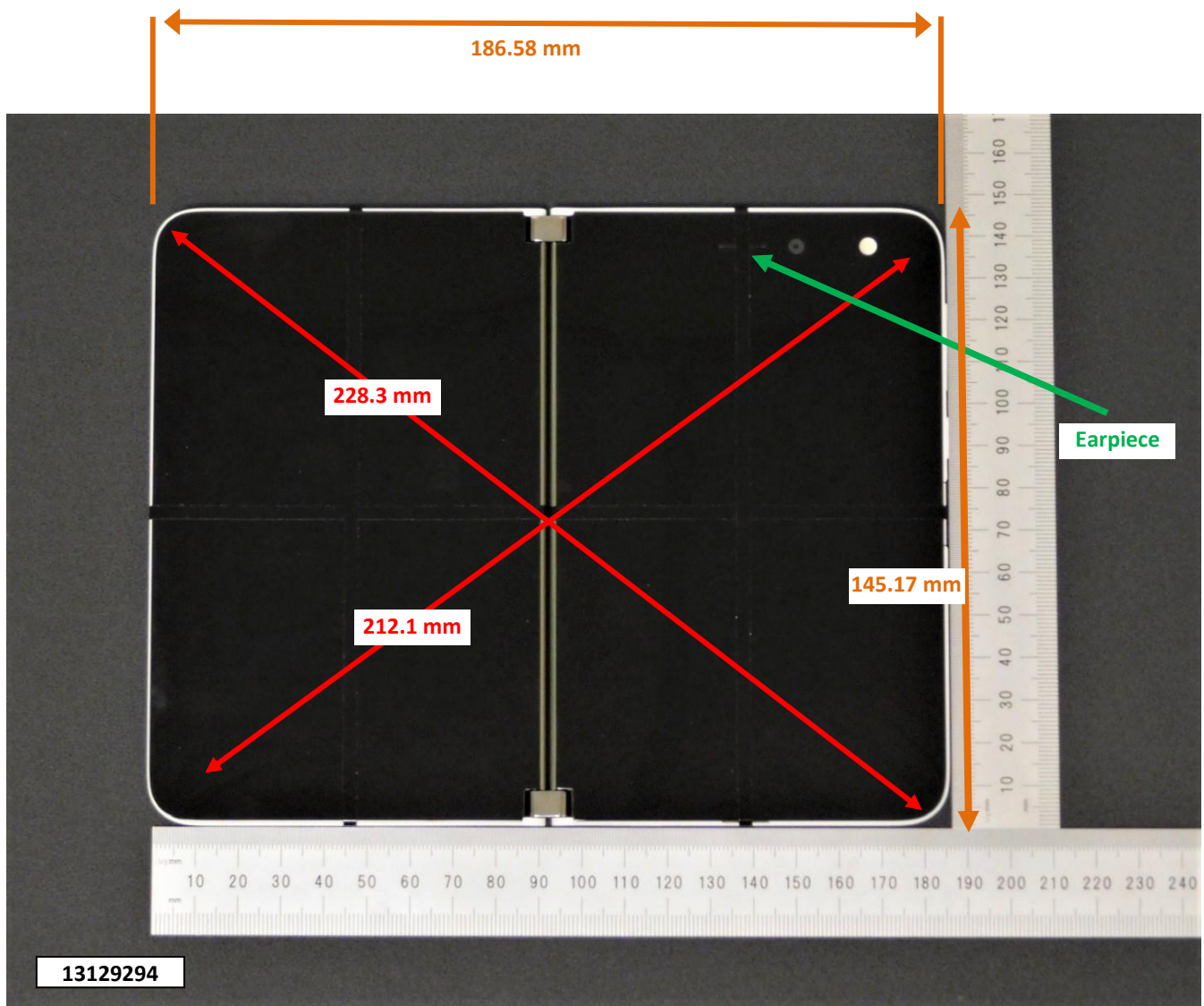
Overall Dimensions @ 180°
