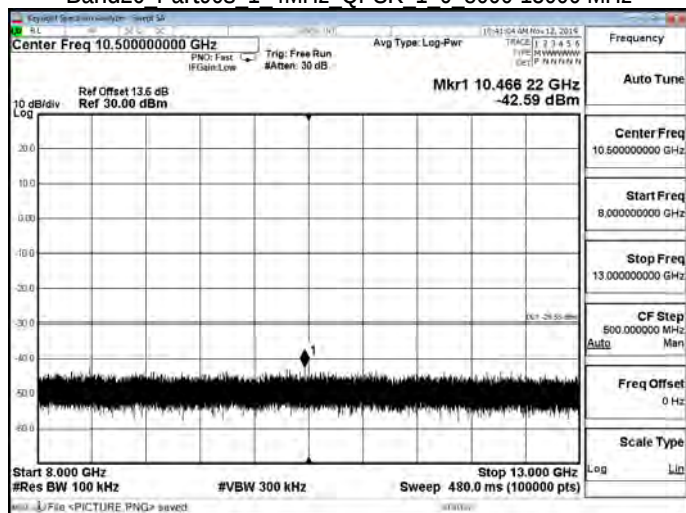
Band26 Part90s 1 4MHz QPSK 1 0 8000-13000 MHz
