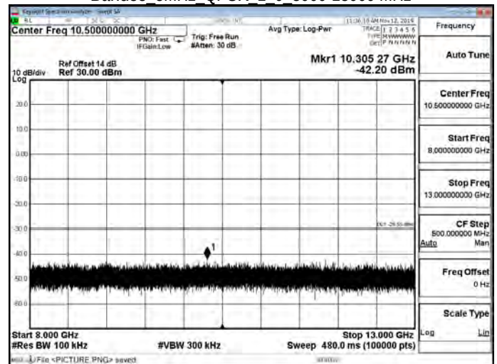
Band38 5MHz QPSK 1 0 8000-13000 MHz
