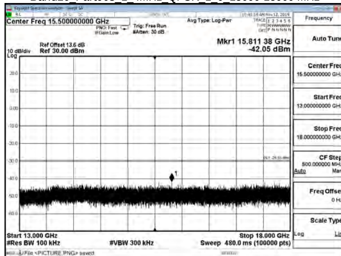
Band26 Part90s 1 4MHz QPSK 1 0 13000-18000 MHz
