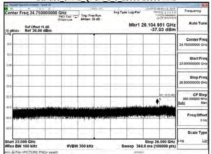
Band30 5MHz QPSK 1 0 23000-26500 MHz
