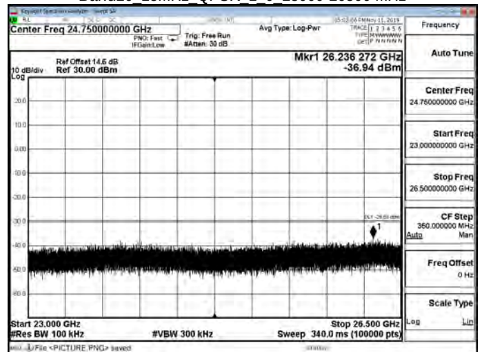
Band26 15MHz QPSK 1 0 23000-26500 MHz
