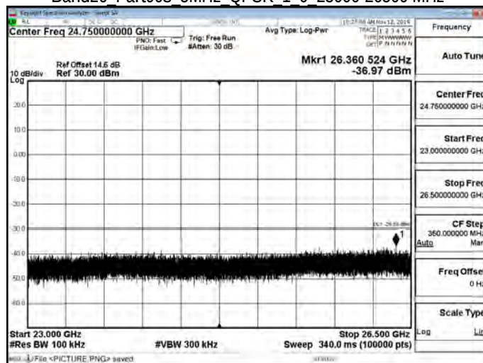
Band26 Part90s 5MHz QPSK 1 0 23000-26500 MHz
