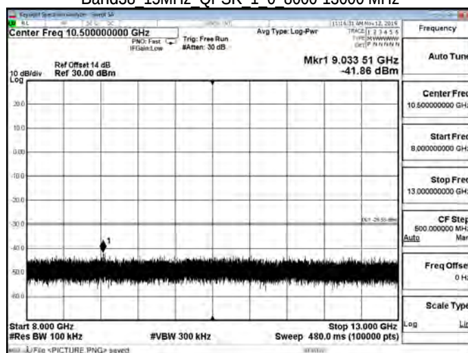
Band38 15MHz QPSK 1 0 8000-13000 MHz
