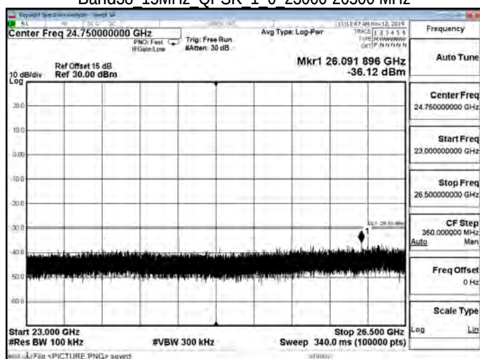
Band38 15MHz QPSK 1 0 23000-26500 MHz
