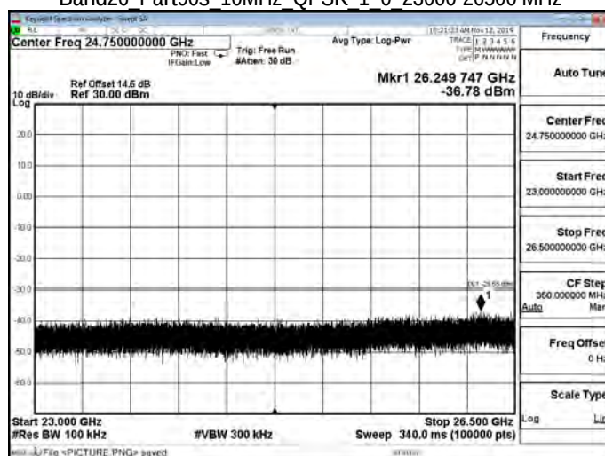
Band26 Part90s 10MHz QPSK 1 0 23000-26500 MHz
