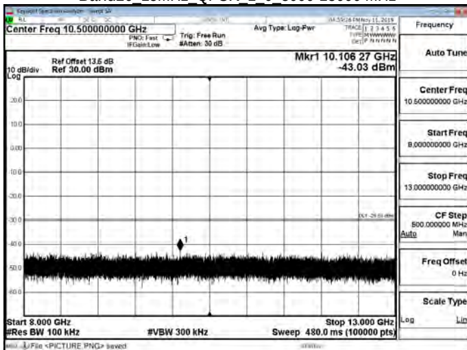
Band26 15MHz QPSK 1 0 8000-13000 MHz
