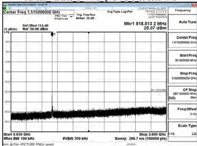
Band26 Part90s 1 4MHz QPSK 1 0 30-3000 MHz
