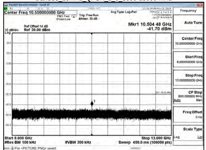
Band38 10MHz QPSK 1 0 8000-13000 MHz
