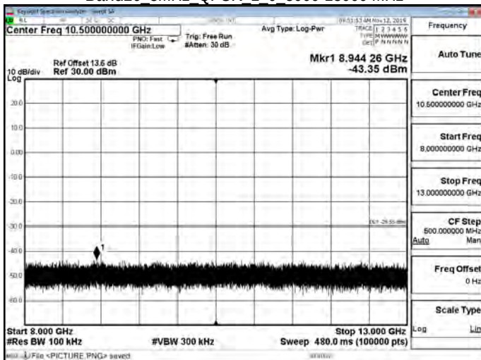
Band26 3MHz QPSK 1 0 8000-13000 MHz
