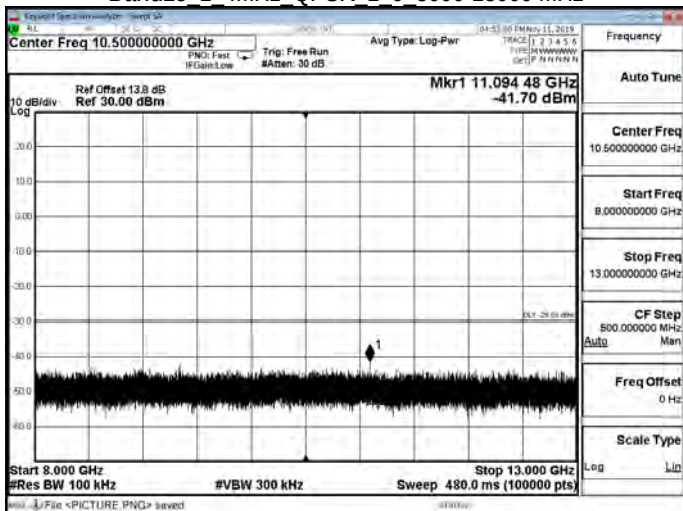
Band25 1 4MHz QPSK 1 0 8000-13000 MHz
