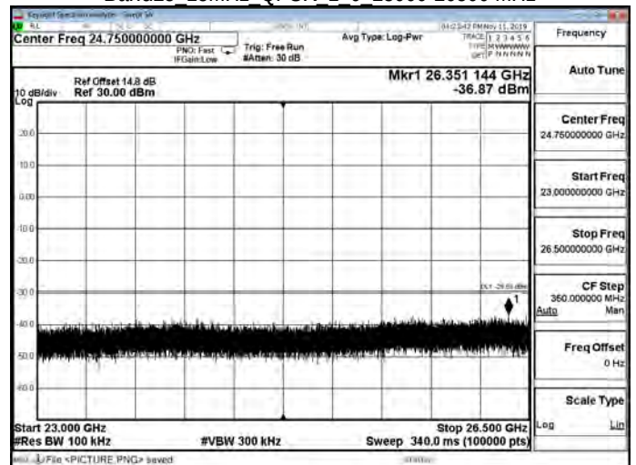
Band25 15MHz QPSK 1 0 23000-26500 MHz
