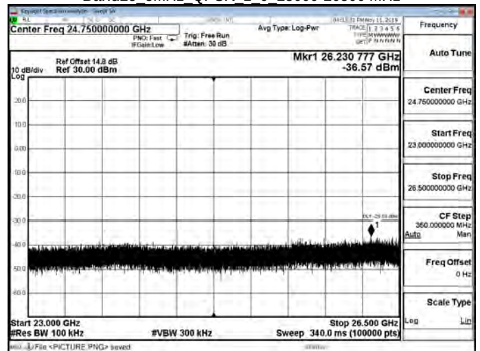
Band25 5MHz QPSK 1 0 23000-26500 MHz
