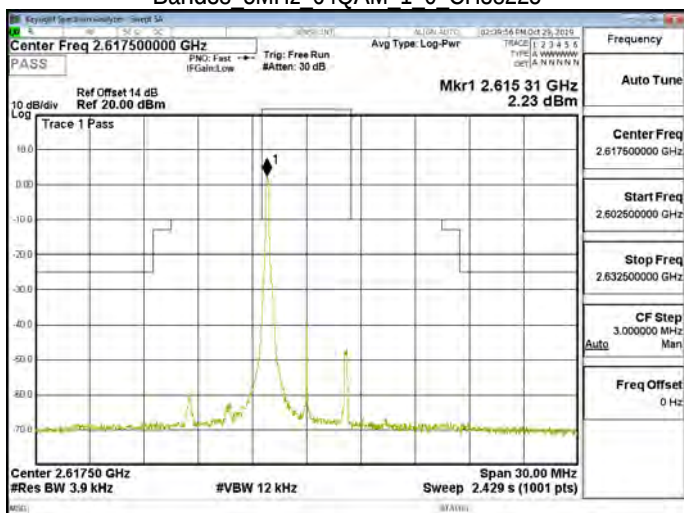
Band38 5MHz 64QAM 1 0 CH38225
