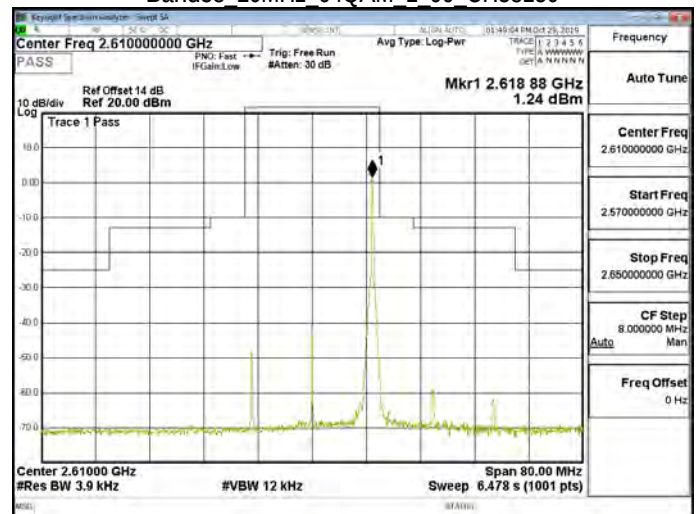
Band38 20MHz 64QAM 1 99 CH38150
