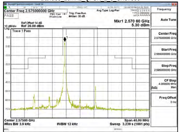
Band38 10MHz QPSK 1 0 CH37800
