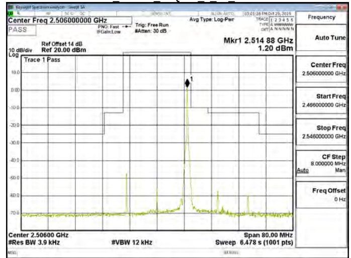
Band41 20MHz 64QAM 1 99 CH39750
