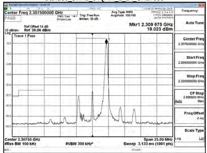
Band30 5MHz 64QAM 1 24 CH27685
