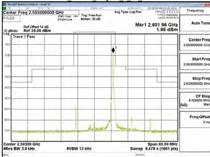
Band41 20MHz 16QAM 1 99 CH40620
