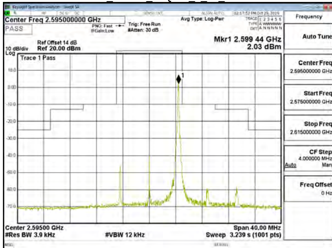
Band38 10MHz 64QAM 1 49 CH38000
