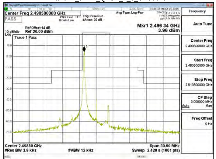
Band41 5MHz QPSK 1 0 CH39675
