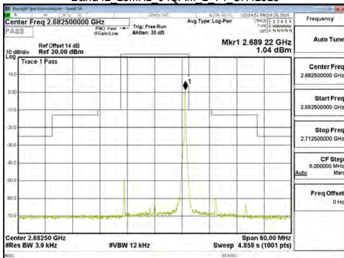
Band41 15MHz 64QAM 1 74 CH41515
