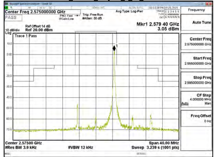
Band38 10MHz 16QAM 1 49 CH37800
