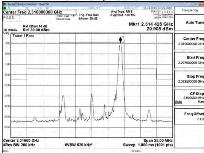
Band30 10MHz 16QAM 1 49 CH27710
