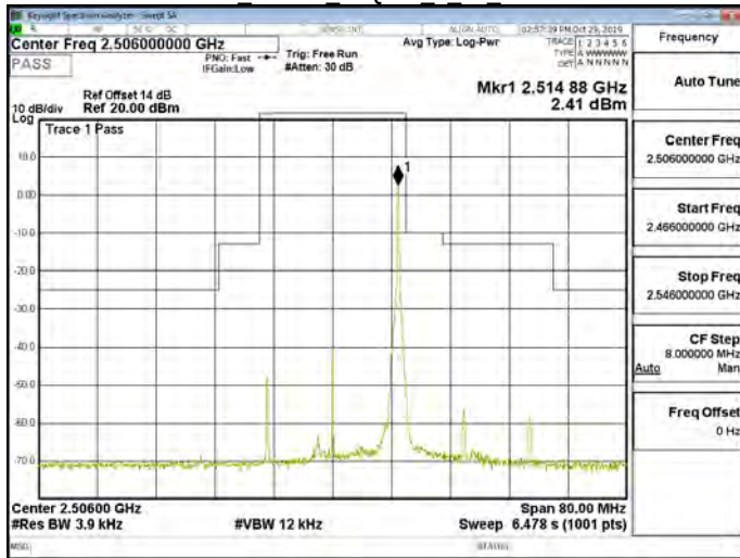
Band41 20MHz 16QAM 1 99 CH39750
