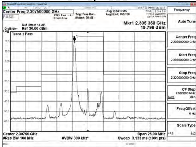
Band30 5MHz QPSK 1 0 CH27685
