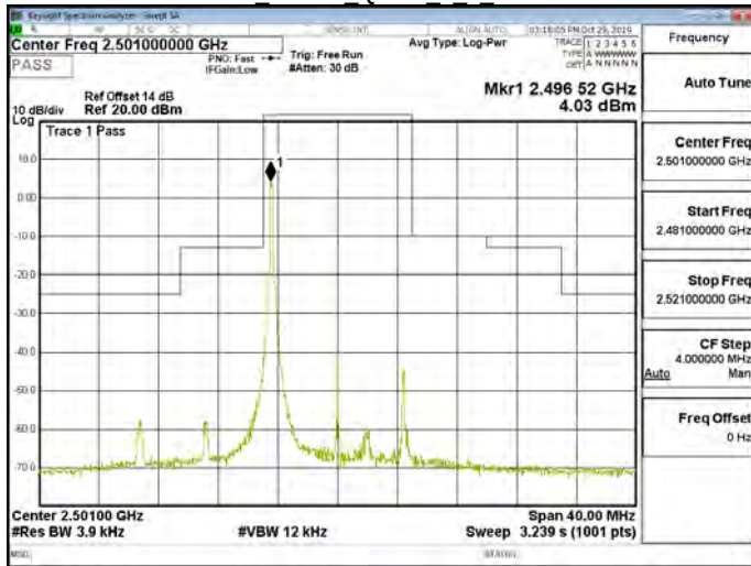
Band41 10MHz QPSK 1 0 CH39700
