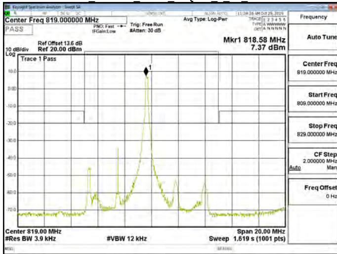
Band26 Part90s 5MHz 16QAM 1 24 CH26715
