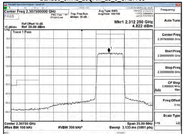
Band30 5MHz 16QAM 25 0 CH27735
