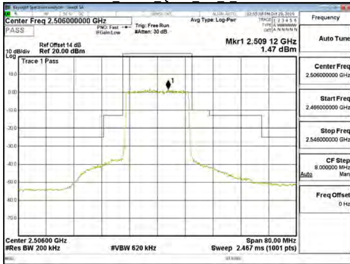
Band41 20MHz QPSK 100 0 CH39750
