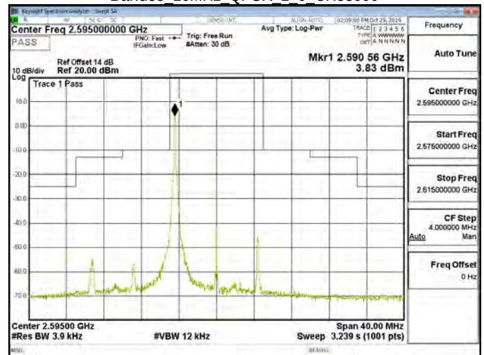
Band38 10MHz QPSK 1 0 CH38000
