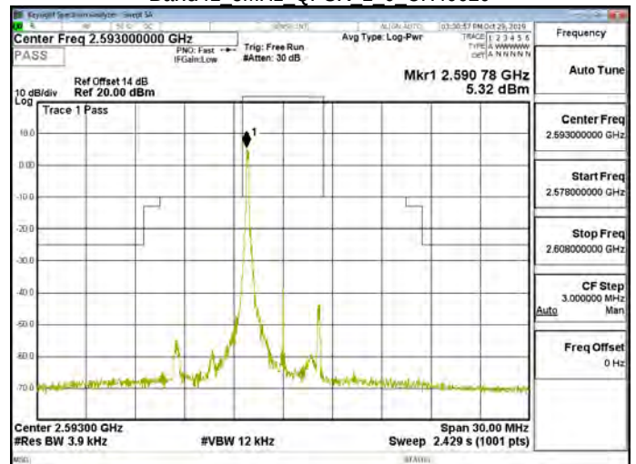
Band41 5MHz QPSK 1 0 CH40620
