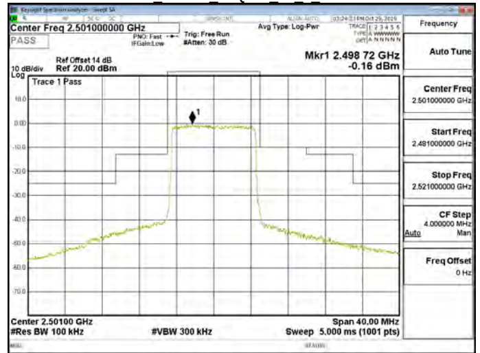
Band41 10MHz 16QAM 50 0 CH39700
