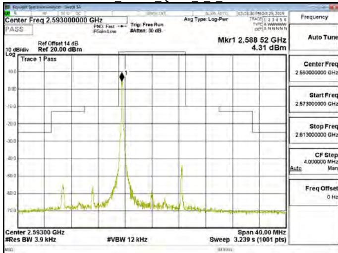
Band41 10MHz QPSK 1 0 CH40620
