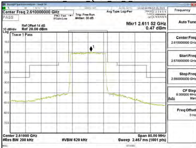
Band38 20MHz QPSK 100 0 CH38150
