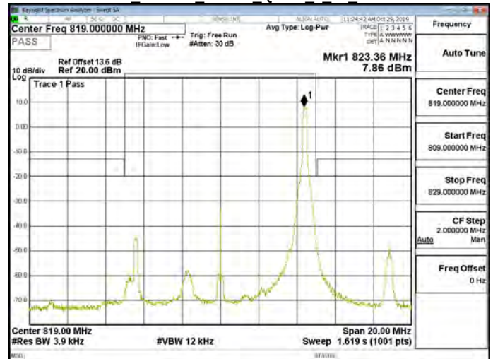
Band26 Part90s 10MHz QPSK 1 49 CH26740
