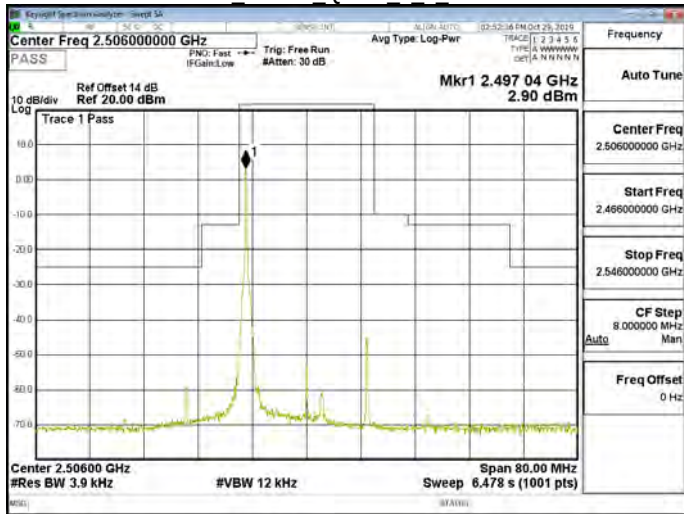
Band41 20MHz QPSK 1 0 CH39750
