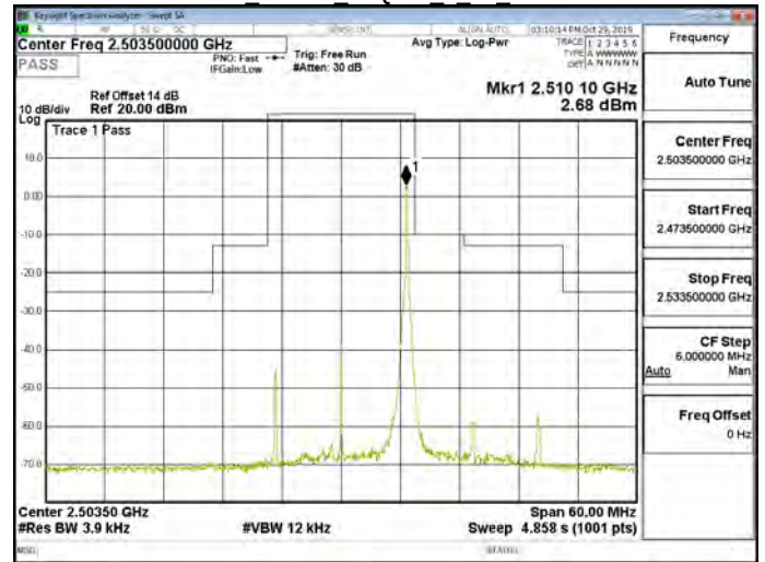
Band41 15MHz 16QAM 1 74 CH39725
