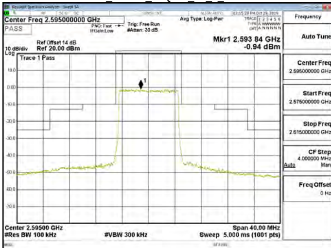
Band38 10MHz 16QAM 50 0 CH38000
