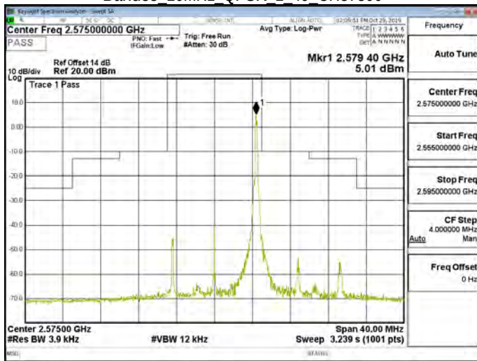
Band38 10MHz QPSK 1 49 CH37800
