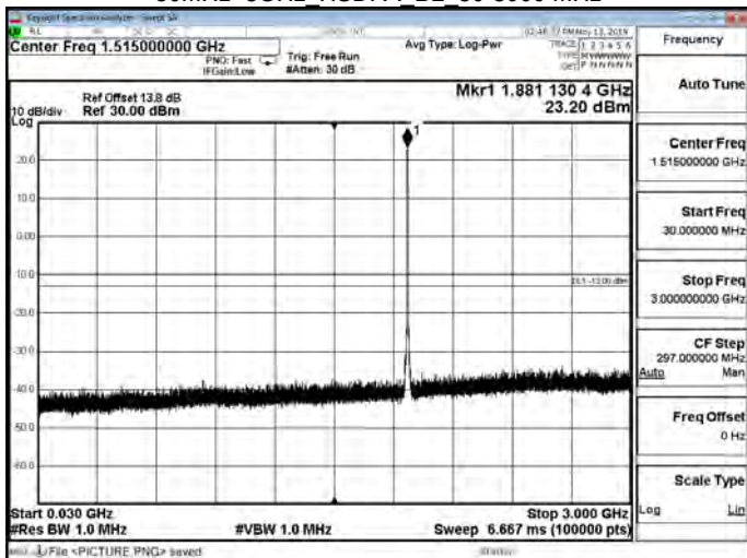
30MHz~3GHz HSDPA B2 30-3000 MHz
