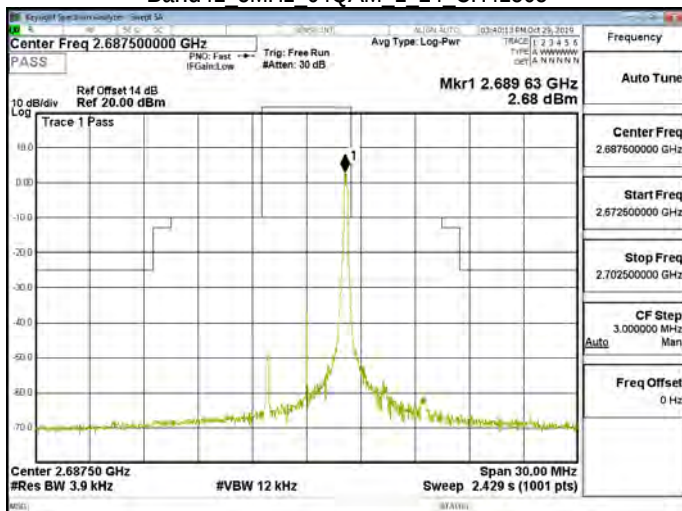
Band41 5MHz 64QAM 1 24 CH41565
