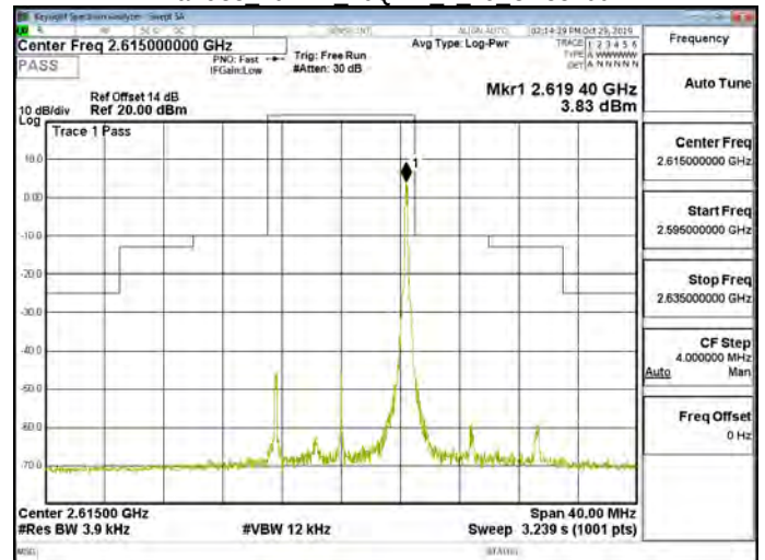
Band38 10MHz 16QAM 1 49 CH38200
