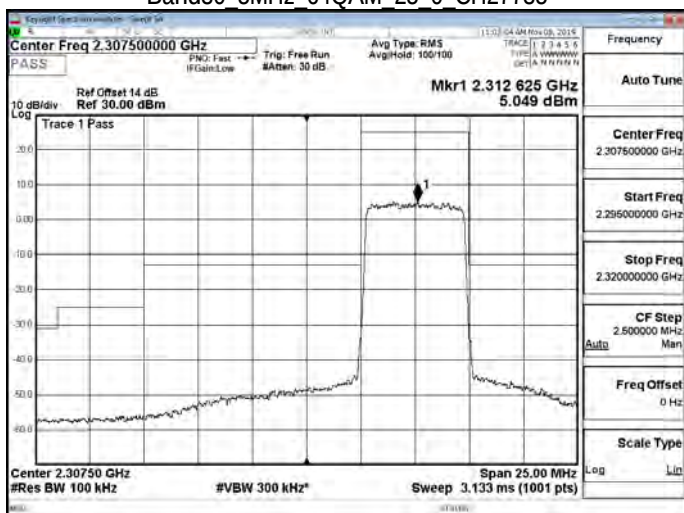
Band30 5MHz 64QAM 25 0 CH27735
