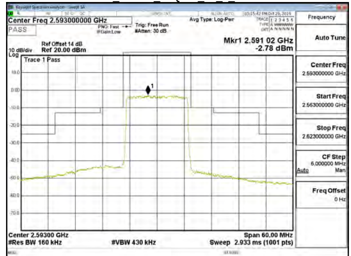
Band41 15MHz 64QAM 75 0 CH40620
