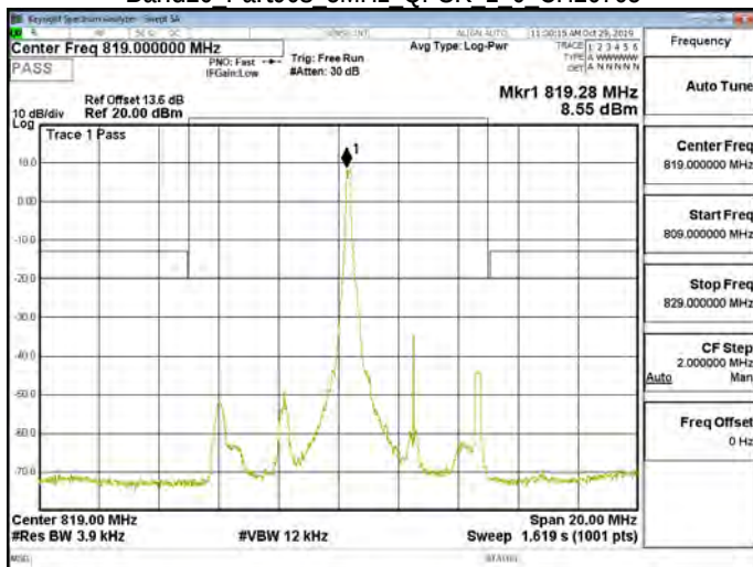
Band26 Part90s 5MHz QPSK 1 0 CH26765
