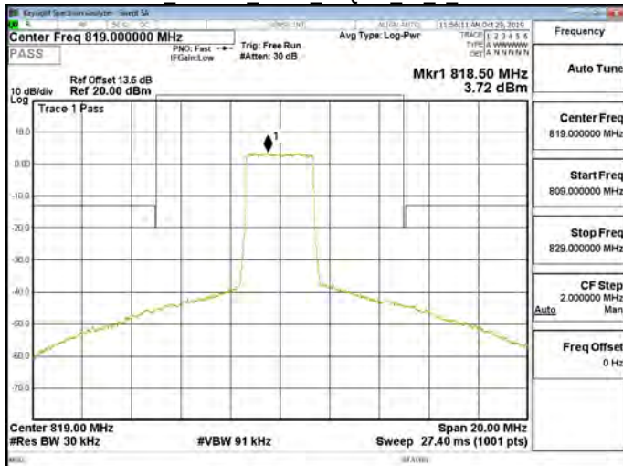
Band26 Part90s 3MHz 16QAM 15 0 CH26740
