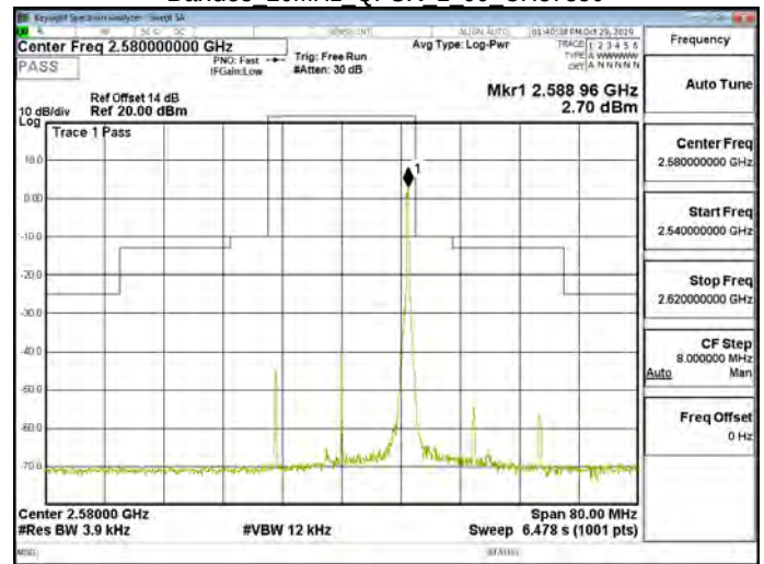
Band38 20MHz QPSK 1 99 CH37850
