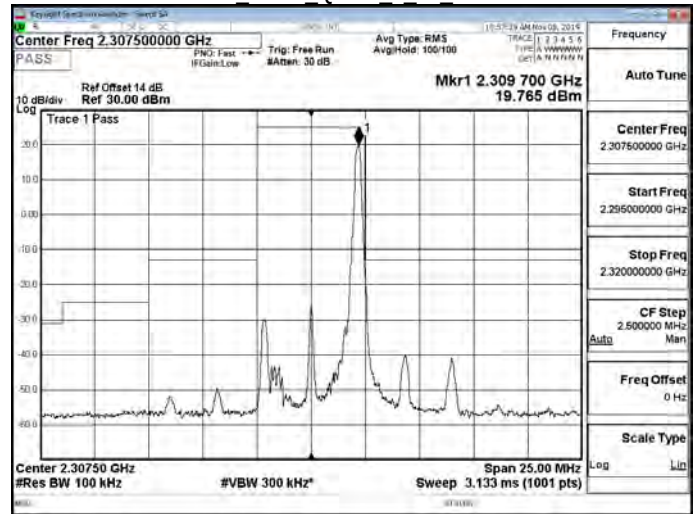
Band30 5MHz QPSK 1 24 CH27685
