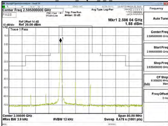
Band38 20MHz 64QAM 1 0 CH38000
