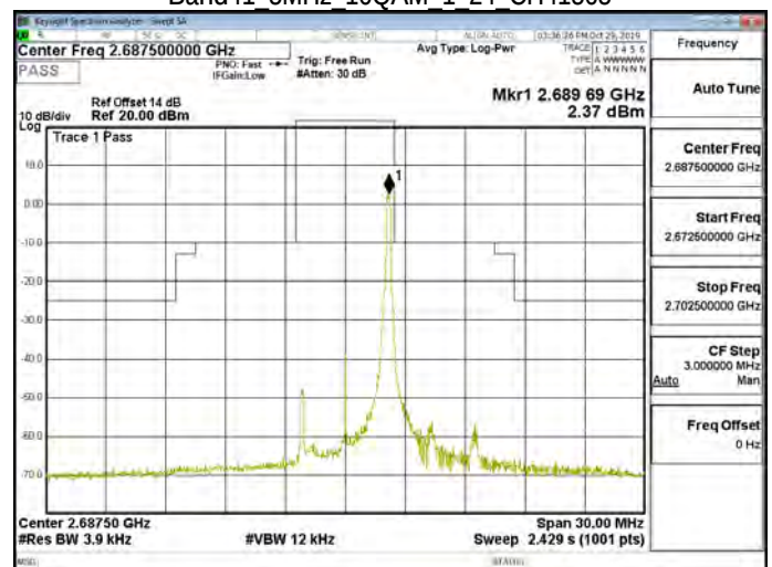
Band41 5MHz 16QAM 1 24 CH41565
