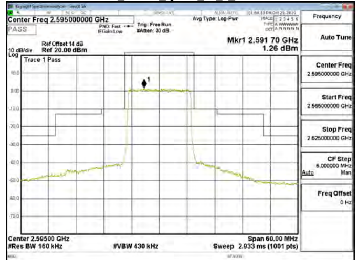
Band38 15MHz QPSK 75 0 CH38000
