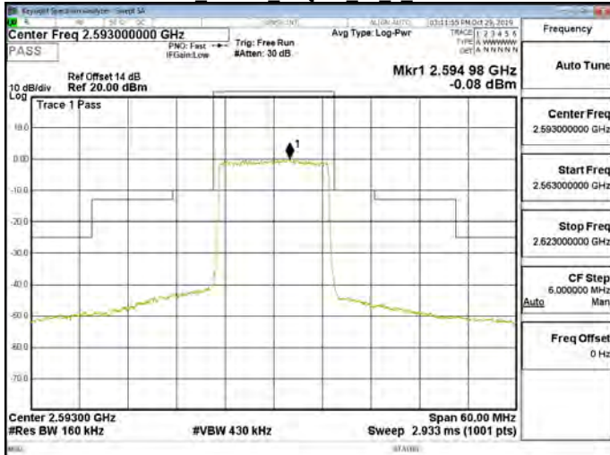
Band41 15MHz 16QAM 75 0 CH40620
