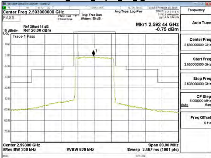
Band41 20MHz 64QAM 100 0 CH40620
