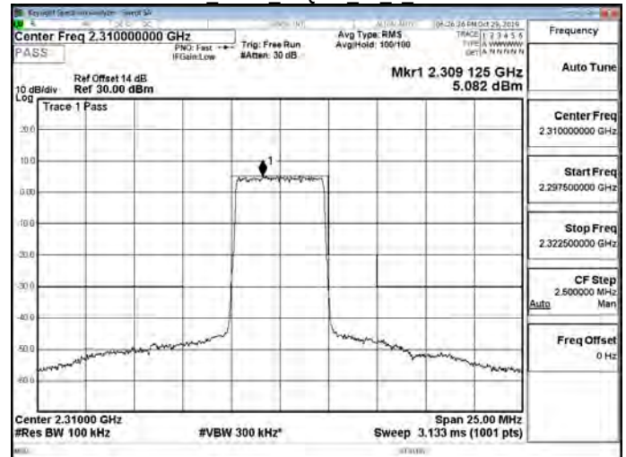
Band30 5MHz 16QAM 25 0 CH27710
