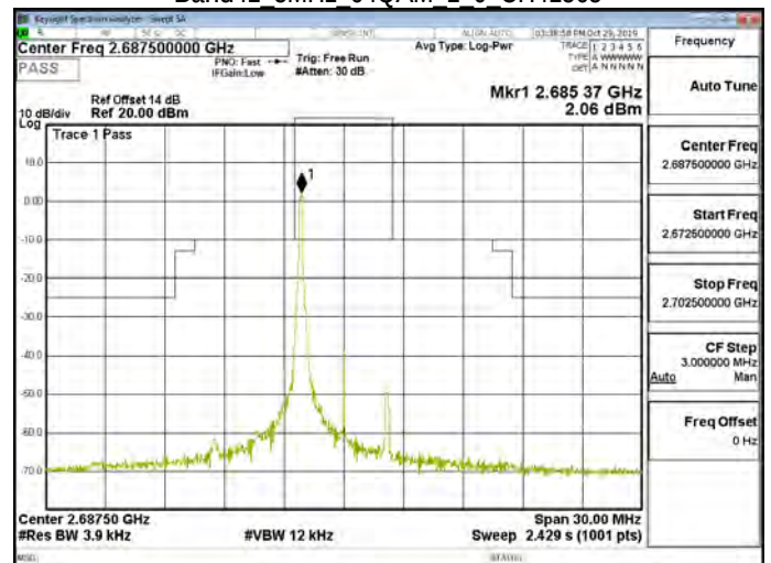
Band41 5MHz 64QAM 1 0 CH41565
