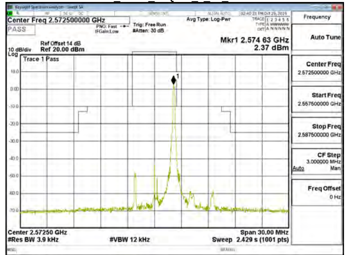
Band38 5MHz 64QAM 1 24 CH37775
