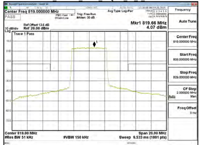
Band26 Part90s 5MHz 16QAM 25 0 CH26740
