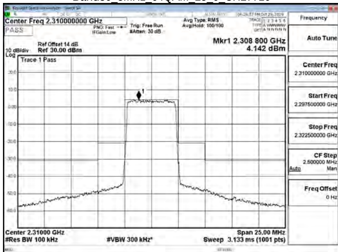
Band30 5MHz 64QAM 25 0 CH27710
