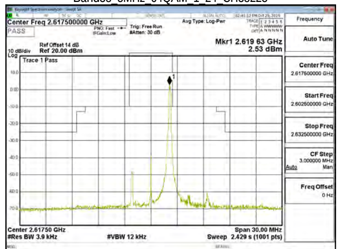
Band38 5MHz 64QAM 1 24 CH38225
