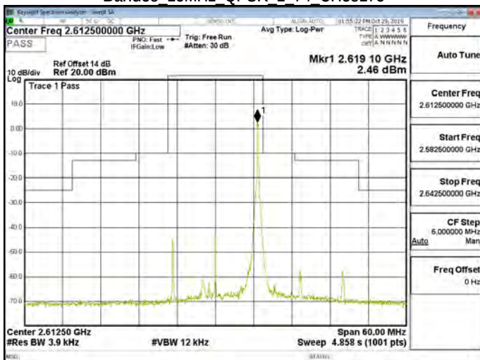
Band38 15MHz QPSK 1 74 CH38175
