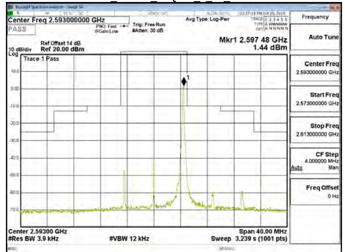
Band41 10MHz 64QAM 1 49 CH40620
