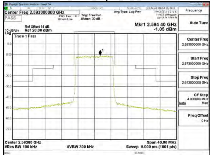
Band41 10MHz 16QAM 50 0 CH40620
