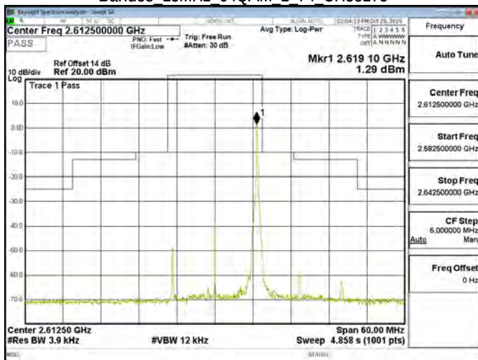
Band38 15MHz 64QAM 1 74 CH38175
