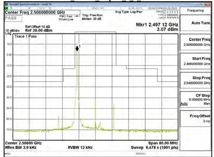
Band41 20MHz 16QAM 1 0 CH39750
