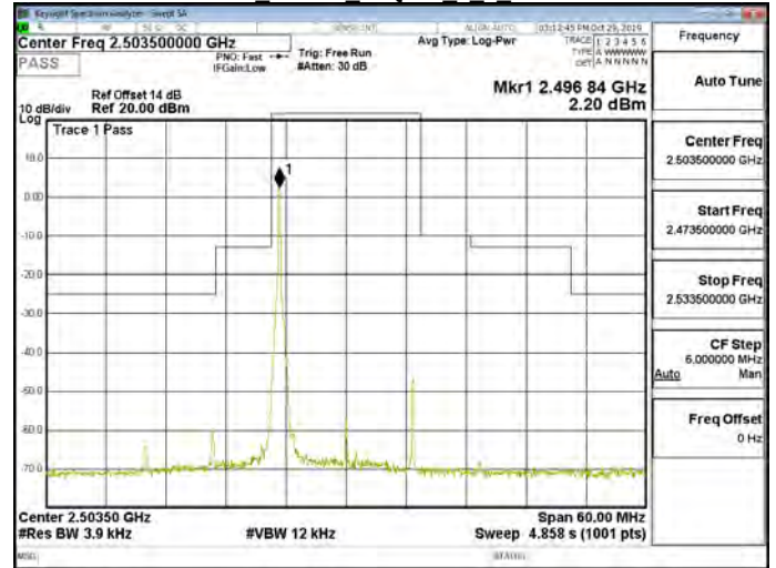
Band41 15MHz 64QAM 1 0 CH39725
