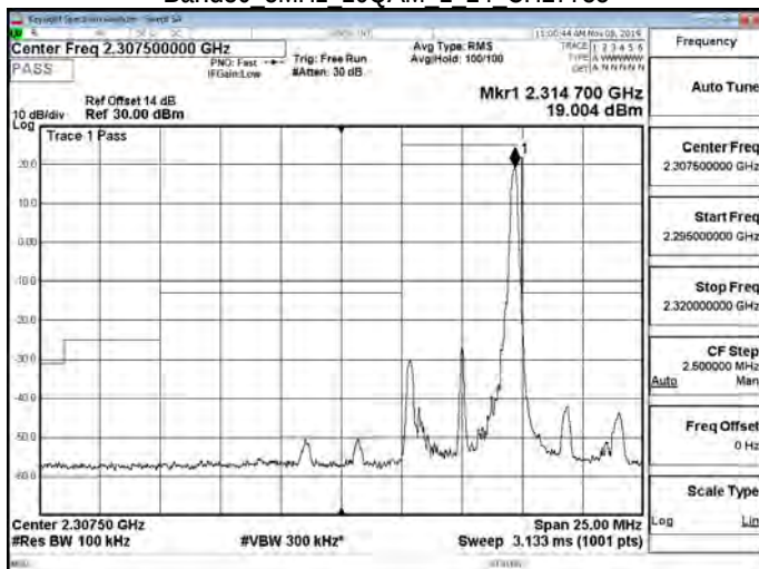
Band30 5MHz 16QAM 1 24 CH27735
