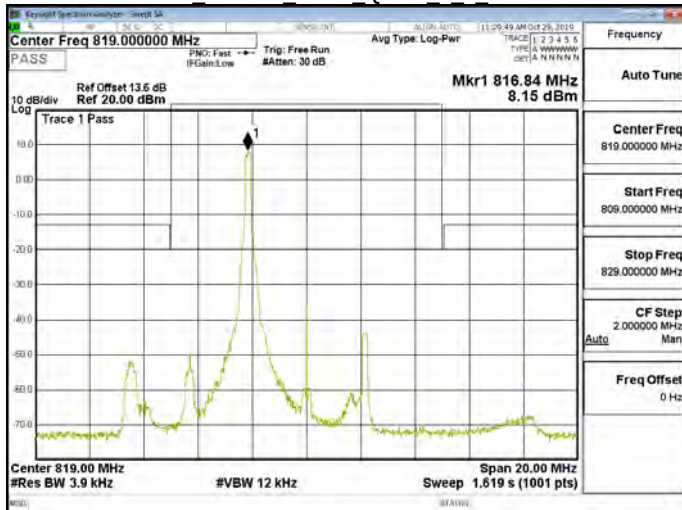
Band26 Part90s 5MHz QPSK 1 0 CH26740
