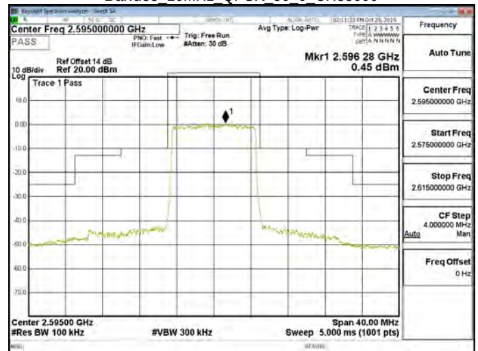
Band38 10MHz QPSK 50 0 CH38000
