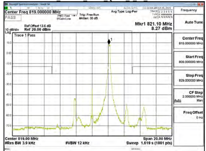
Band26 Part90s 5MHz QPSK 1 24 CH26740
