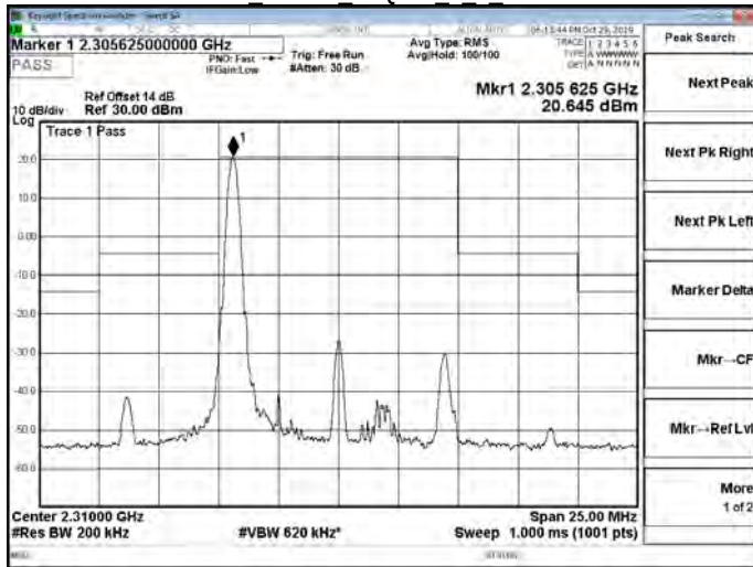
Band30 10MHz 16QAM 1 0 CH27710
