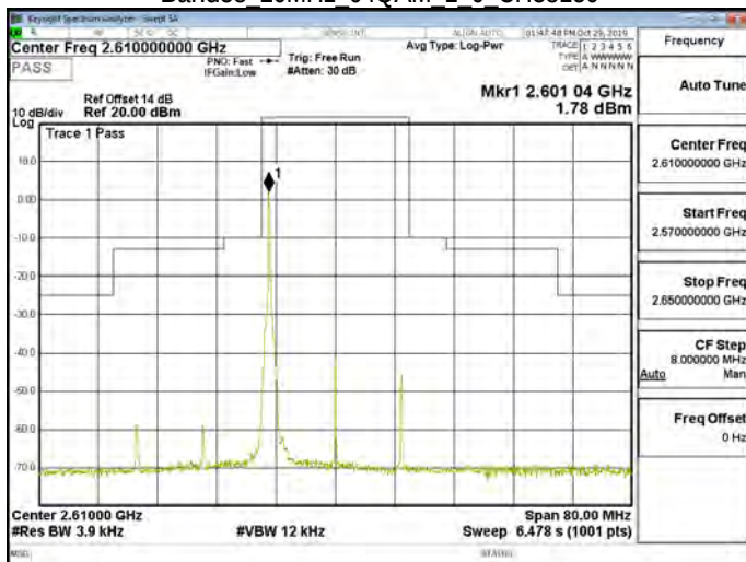
Band38 20MHz 64QAM 1 0 CH38150
