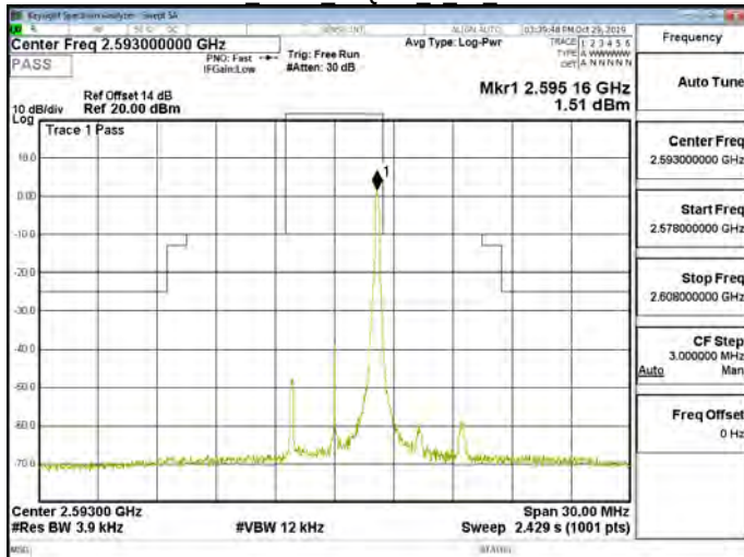
Band41 5MHz 64QAM 1 24 CH40620
