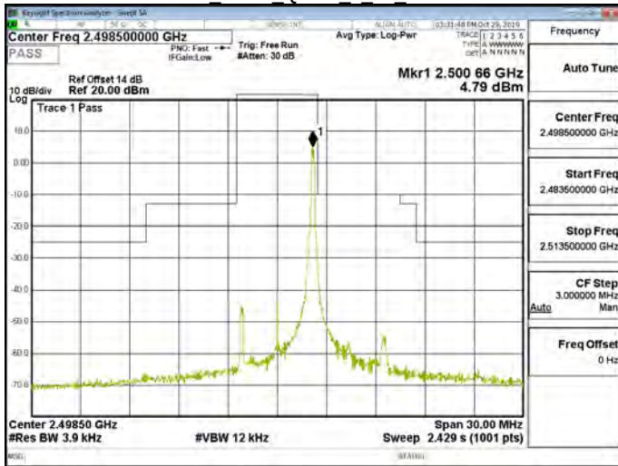
Band41 5MHz QPSK 1 24 CH39675
