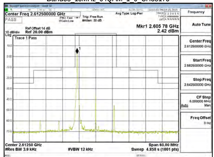
Band38 15MHz 64QAM 1 0 CH38175
