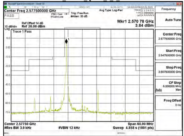
Band38 15MHz QPSK 1 0 CH37825
