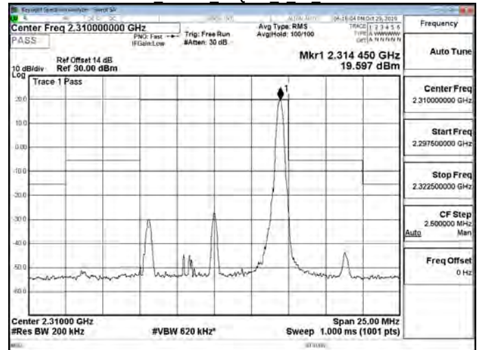
Band30 10MHz 64QAM 1 49 CH27710
