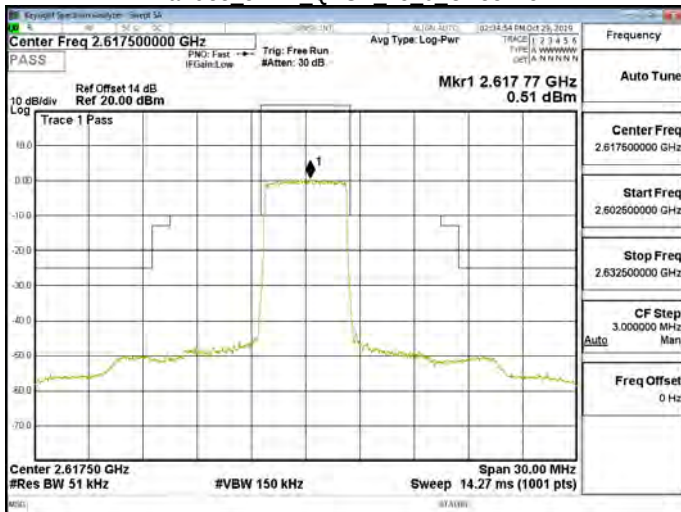
Band38 5MHz QPSK 25 0 CH38225
