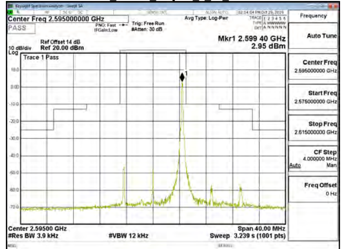
Band38 10MHz 16QAM 1 49 CH38000
