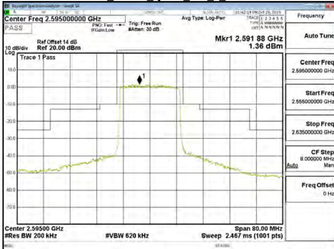
Band38 20MHz QPSK 100 0 CH38000
