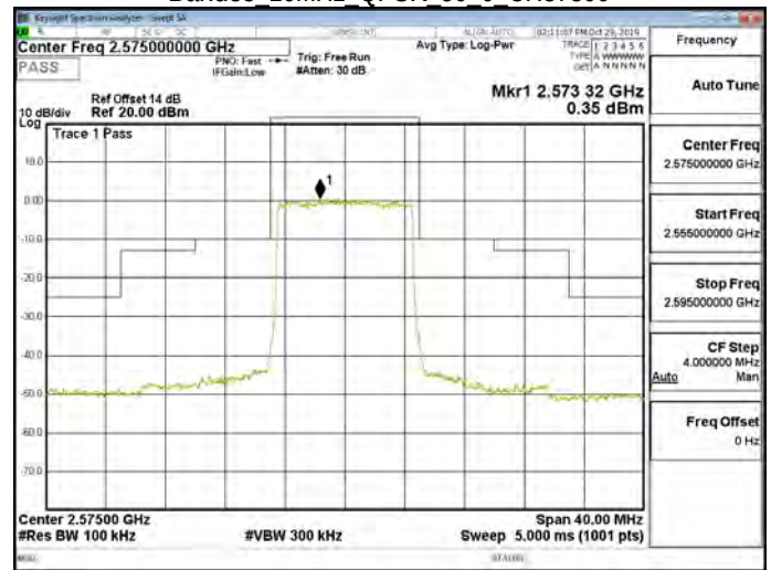
Band38 10MHz QPSK 50 0 CH37800
