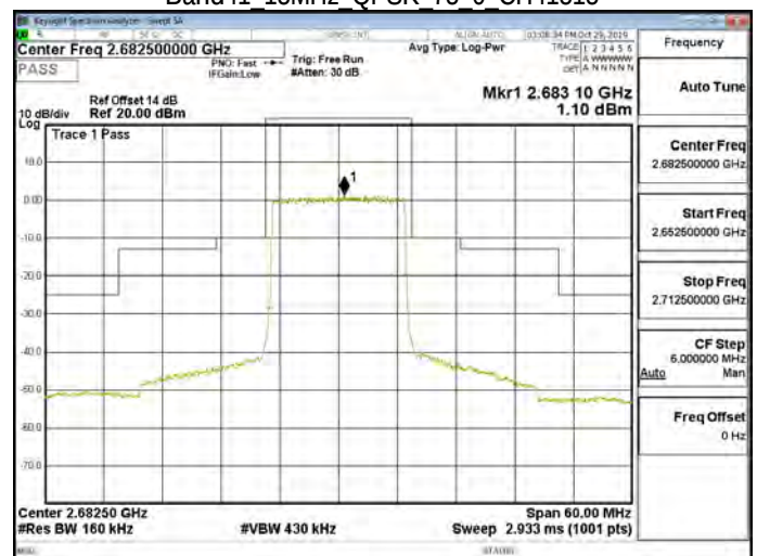
Band41 15MHz QPSK 75 0 CH41515
