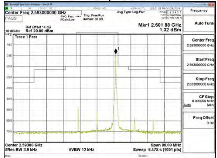
Band41 20MHz 64QAM 1 99 CH40620
