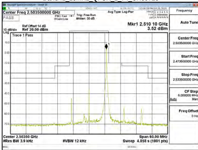
Band41 15MHz QPSK 1 74 CH39725
