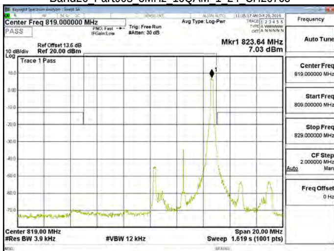
Band26 Part90s 5MHz 16QAM 1 24 CH26765
