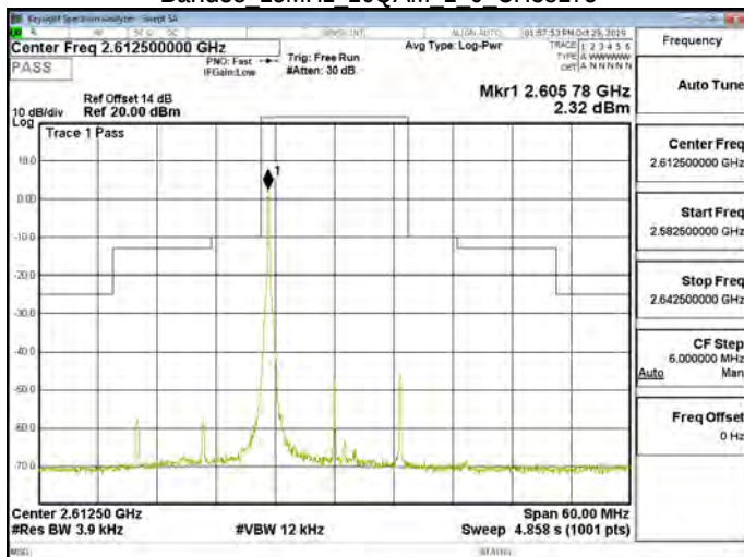
Band38 15MHz 16QAM 1 0 CH38175
