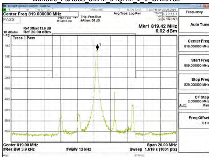
Band26 Part90s 5MHz 64QAM 1 0 CH26765
