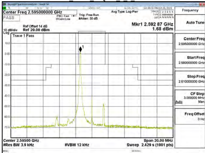
Band38 5MHz 64QAM 1 0 CH38000
