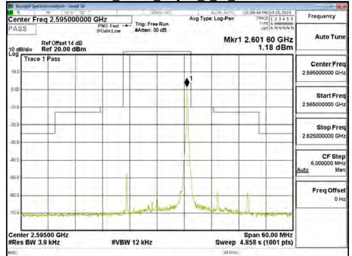
Band38 15MHz 16QAM 1 74 CH38000
