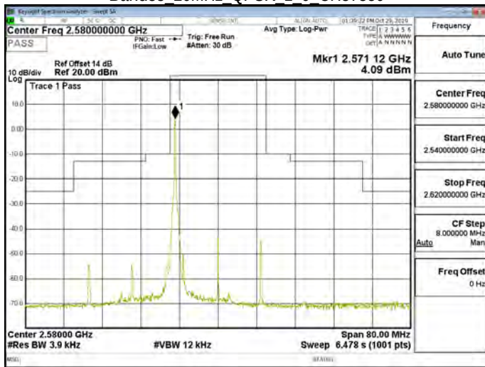
Band38 20MHz QPSK 1 0 CH37850
