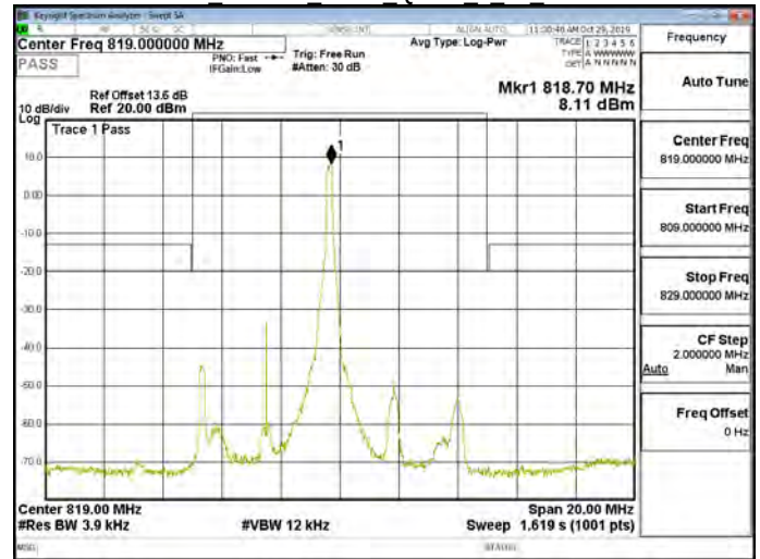
Band26 Part90s 5MHz QPSK 1 24 CH26715
