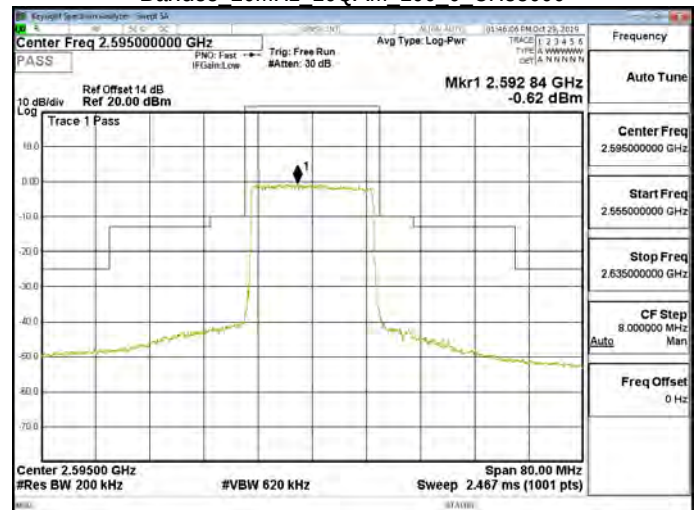
Band38 20MHz 16QAM 100 0 CH38000
