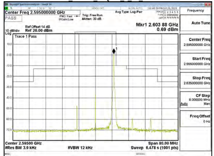
Band38 20MHz 64QAM 1 99 CH38000
