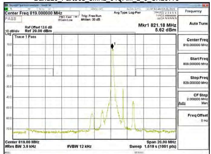
Band26 Part90s 3MHz 64QAM 1 0 CH26775
