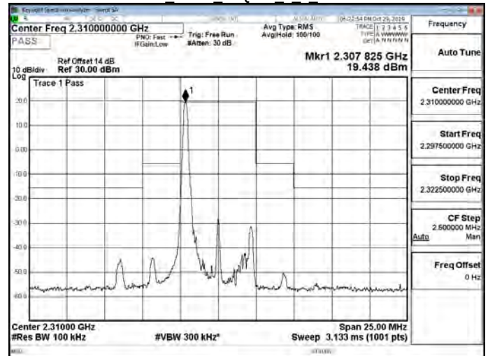
Band30 5MHz 16QAM 1 0 CH27710
