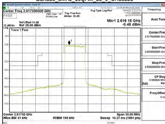
Band38 5MHz 16QAM 25 0 CH38225
