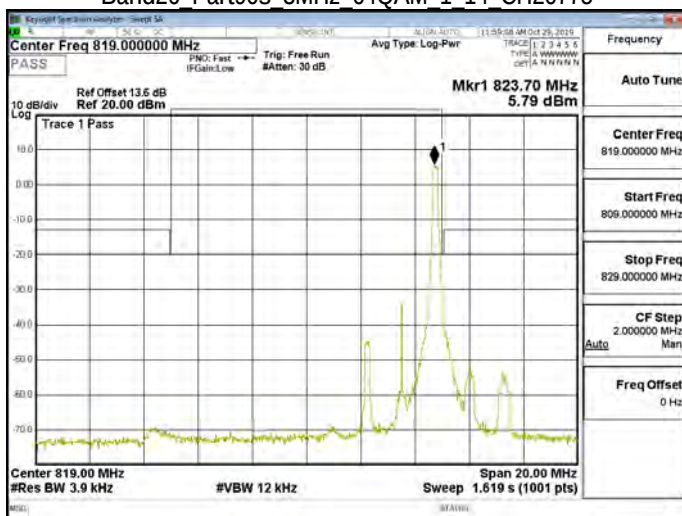
Band26 Part90s 3MHz 64QAM 1 14 CH26775
