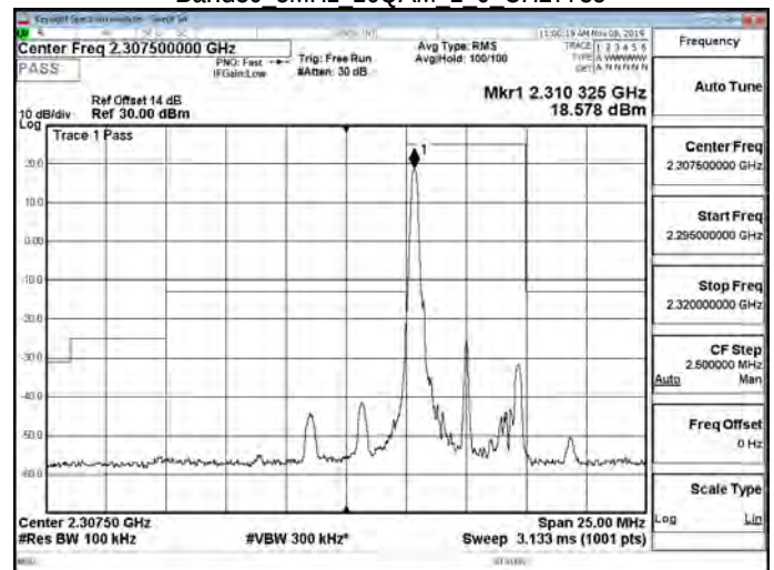
Band30 5MHz 16QAM 1 0 CH27735
