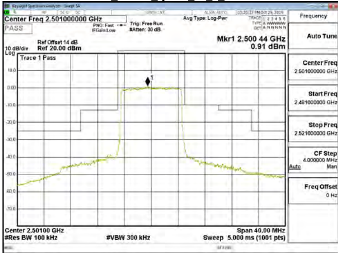
Band41 10MHz QPSK 50 0 CH39700
