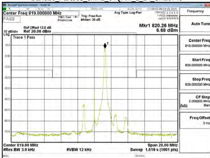
Band26 Part90s 3MHz 64QAM 1 14 CH26740
