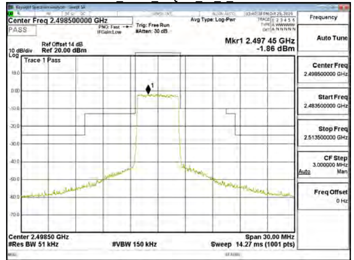
Band41 5MHz 64QAM 25 0 CH39675
