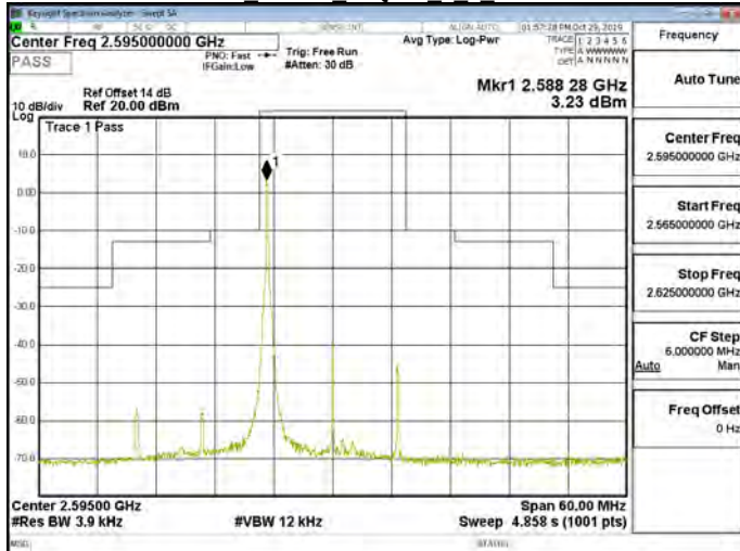
Band38 15MHz 16QAM 1 0 CH38000
