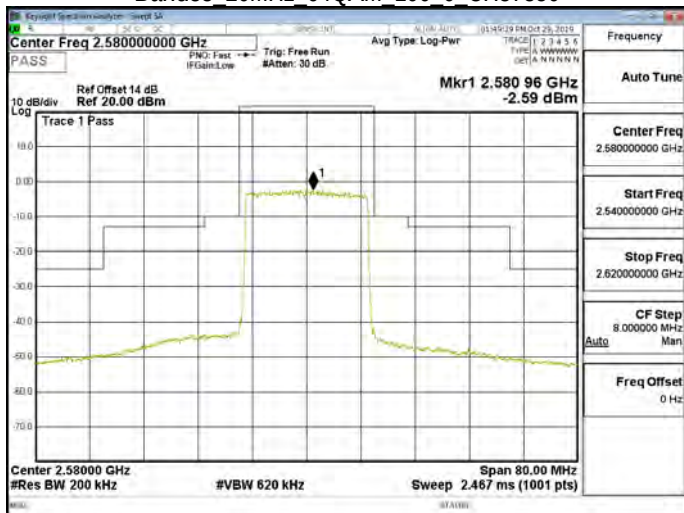
Band38 20MHz 64QAM 100 0 CH37850
