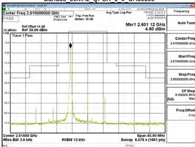
Band38 20MHz QPSK 1 0 CH38150
