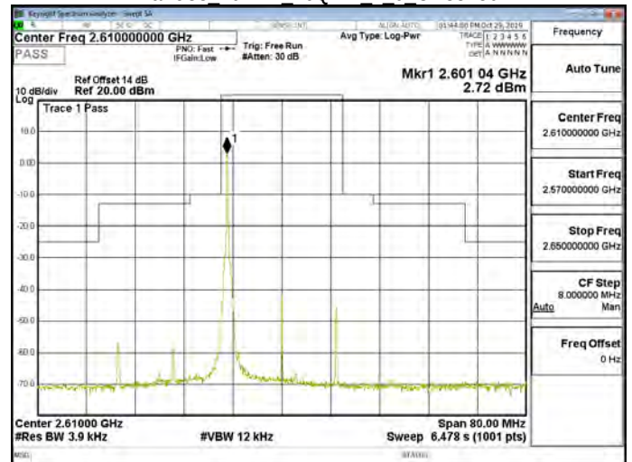
Band38 20MHz 16QAM 1 0 CH38150
