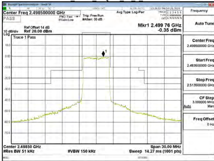
Band41 5MHz 16QAM 25 0 CH39675
