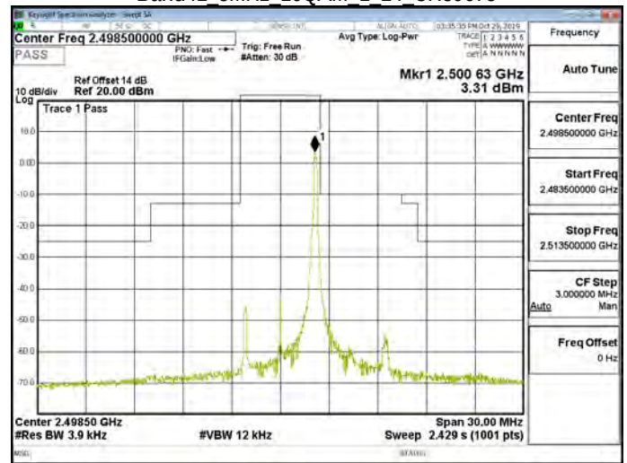
Band41 5MHz 16QAM 1 24 CH39675
