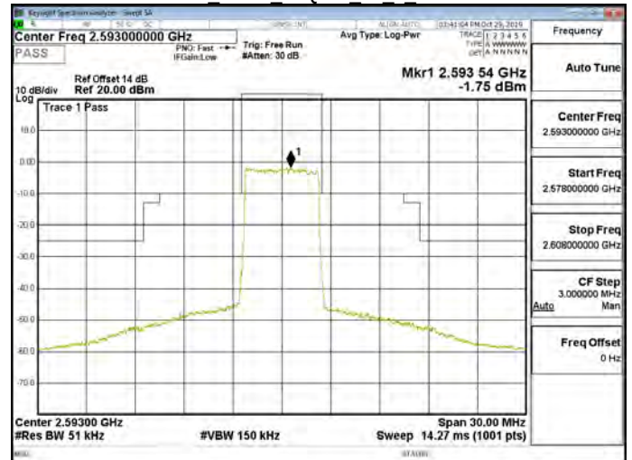
Band41 5MHz 64QAM 25 0 CH40620
