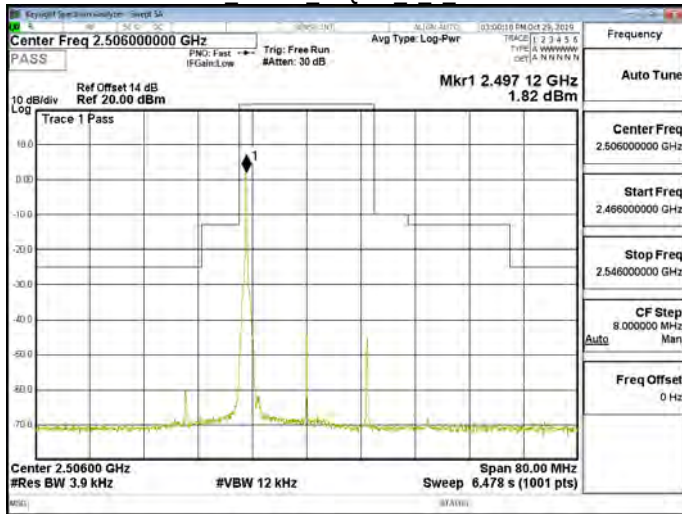
Band41 20MHz 64QAM 1 0 CH39750
