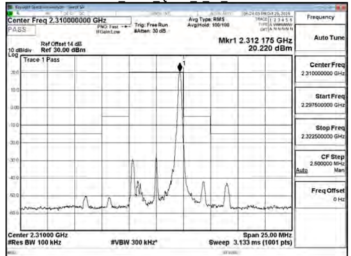
Band30 5MHz QPSK 1 24 CH27710
