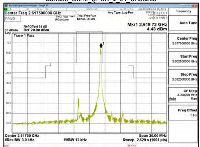
Band38 5MHz QPSK 1 24 CH38225
