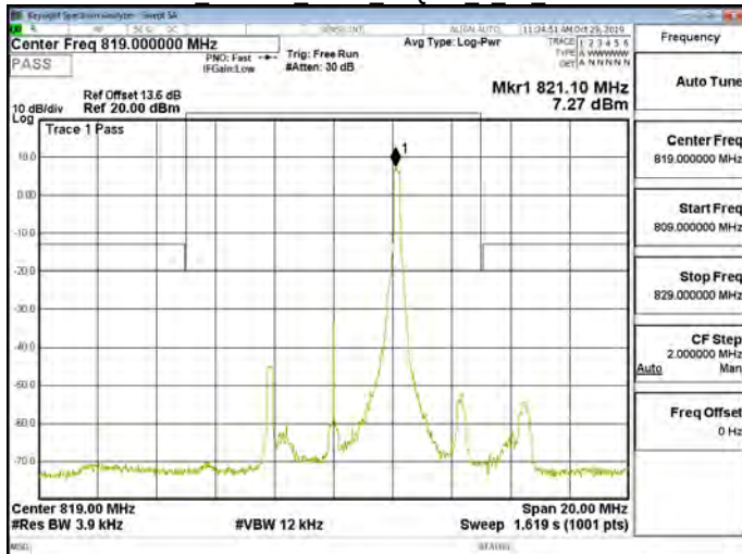
Band26 Part90s 5MHz 16QAM 1 24 CH26740
