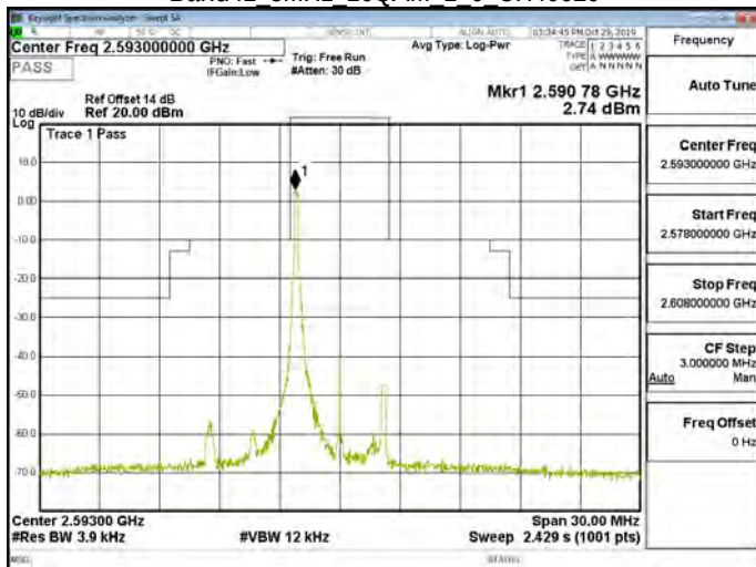
Band41 5MHz 16QAM 1 0 CH40620
