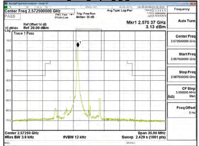
Band38 5MHz 16QAM 1 0 CH37775
