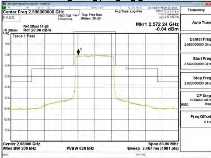
Band38 20MHz QPSK 100 0 CH37850
