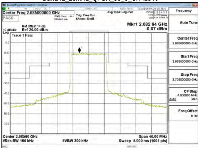
Band41 10MHz QPSK 50 0 CH41540
