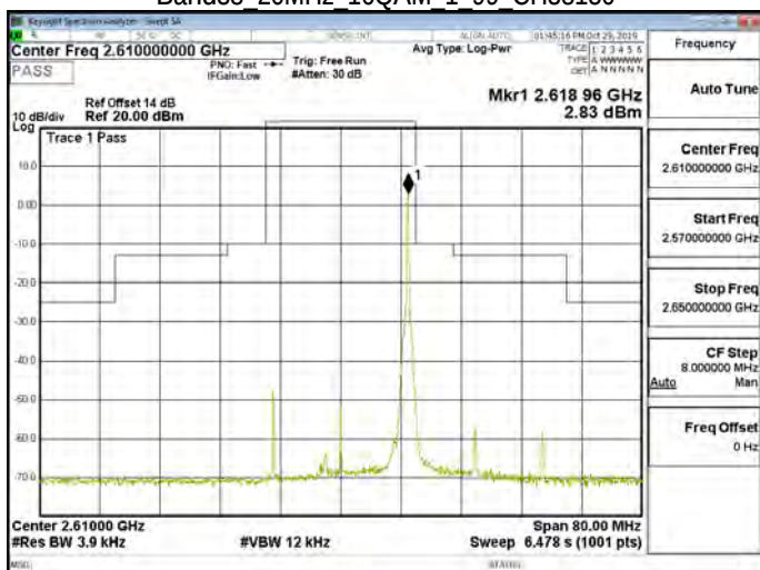
Band38 20MHz 16QAM 1 99 CH38150
