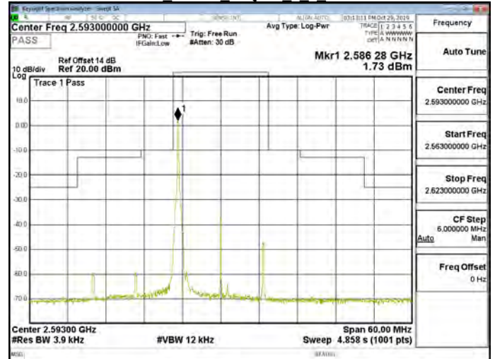
Band41 15MHz 64QAM 1 0 CH40620
