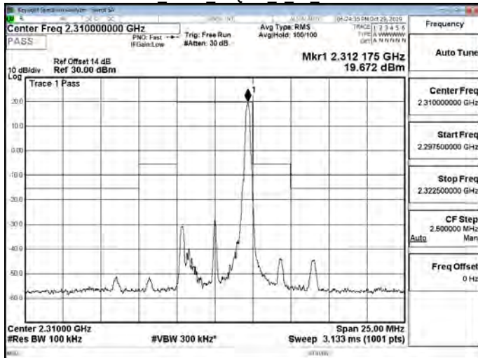
Band30 5MHz 16QAM 1 24 CH27710
