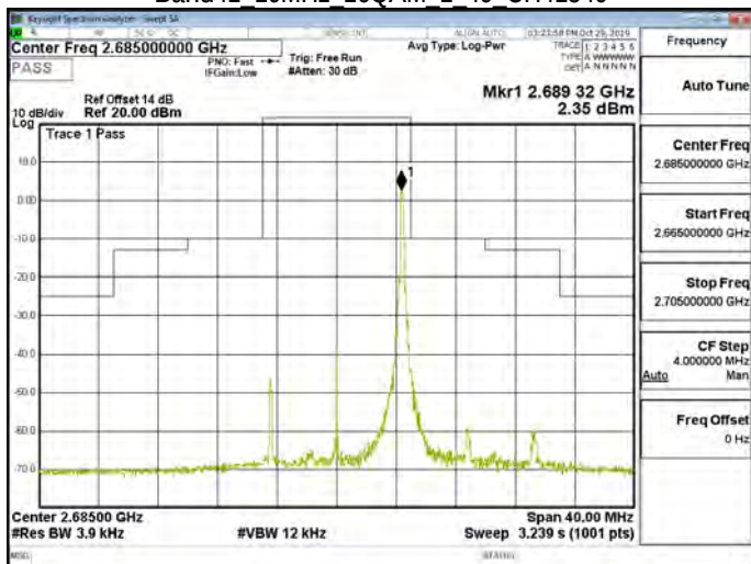
Band41 10MHz 16QAM 1 49 CH41540
