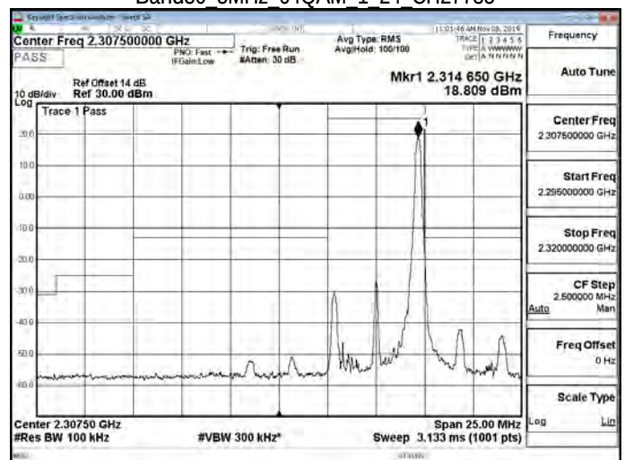
Band30 5MHz 64QAM 1 24 CH27735
