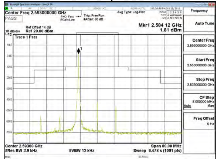
Band41 20MHz 16QAM 1 0 CH40620
