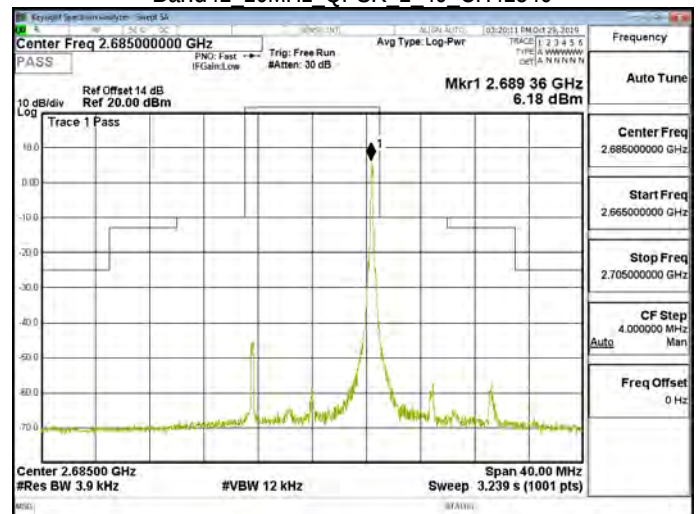
Band41 10MHz QPSK 1 49 CH41540
