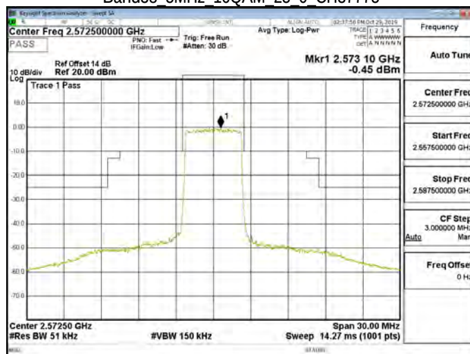
Band38 5MHz 16QAM 25 0 CH37775
