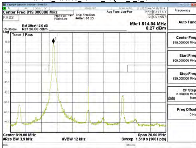
Band26 Part90s 10MHz 16QAM 1 0 CH26740
