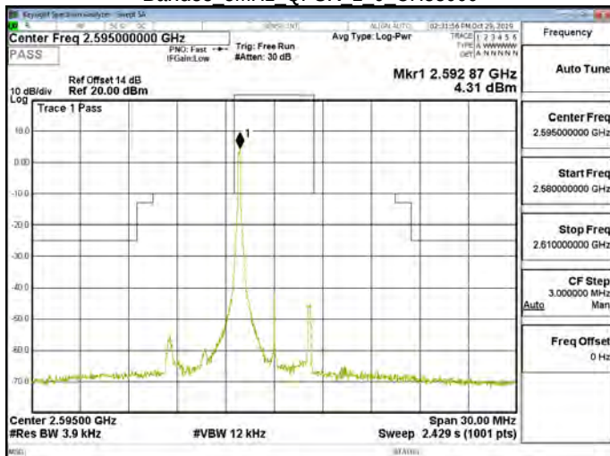
Band38 5MHz QPSK 1 0 CH38000
