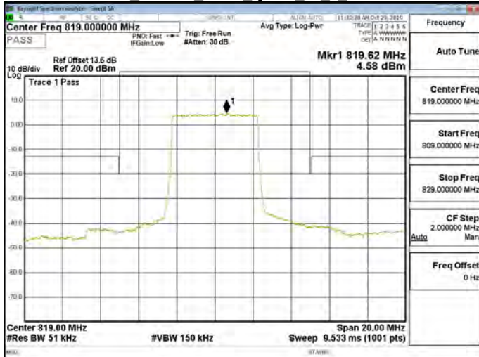
Band26 Part90s 5MHz QPSK 25 0 CH26740
