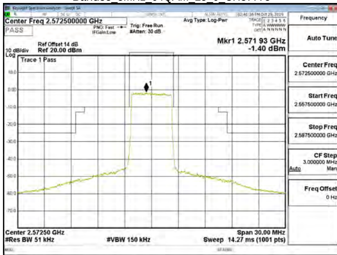
Band38 5MHz 64QAM 25 0 CH37775
