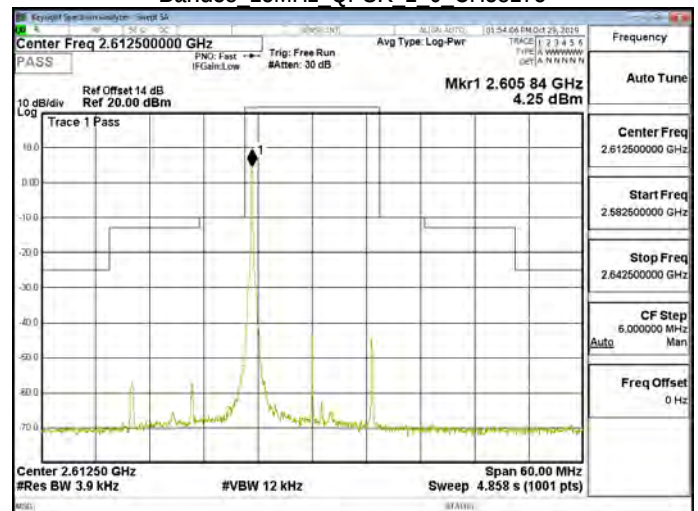
Band38 15MHz QPSK 1 0 CH38175
