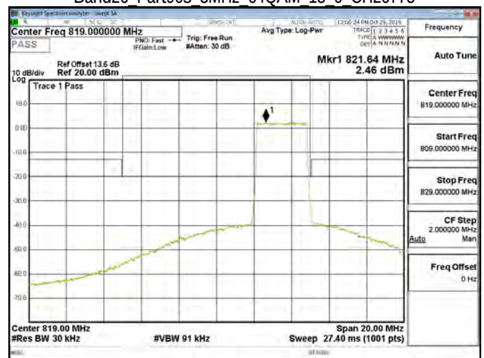
Band26 Part90s 3MHz 64QAM 15 0 CH26775
