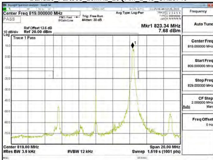
Band26 Part90s 10MHz 16QAM 1 49 CH26740
