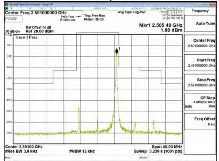
Band41 10MHz 64QAM 1 49 CH39700
