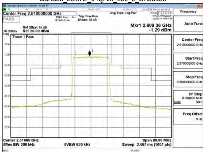
Band38 20MHz 64QAM 100 0 CH38150
