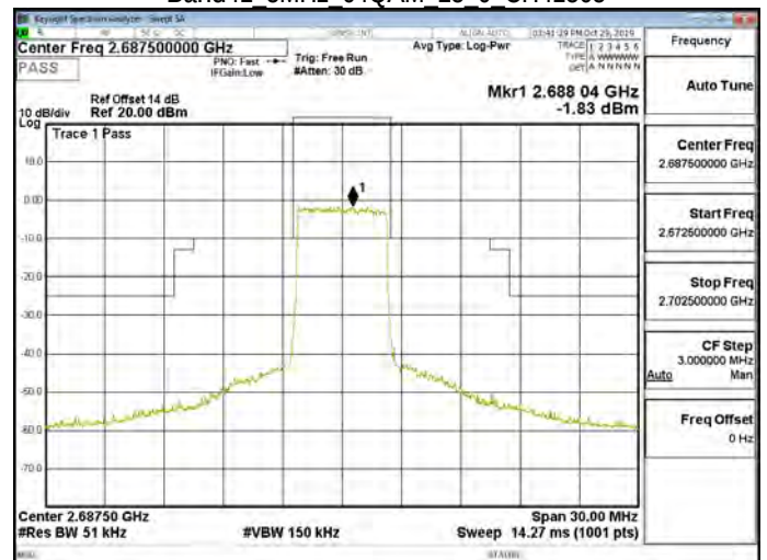
Band41 5MHz 64QAM 25 0 CH41565
