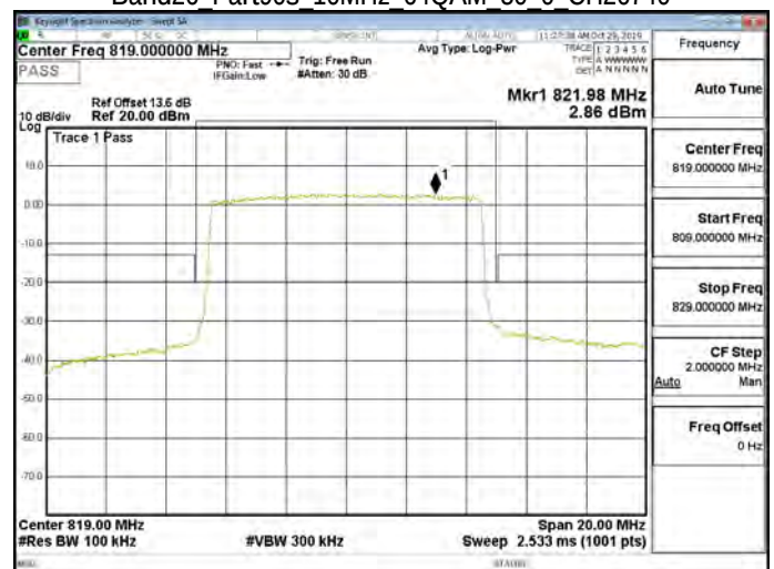
Band26 Part90s 10MHz 64QAM 50 0 CH26740
