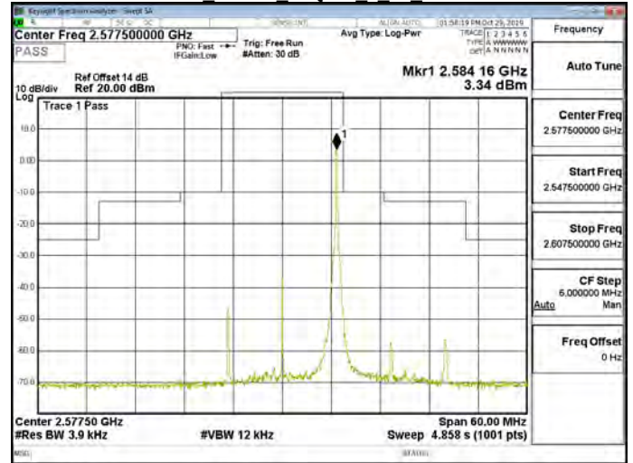
Band38 15MHz 16QAM 1 74 CH37825
