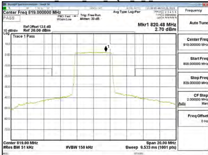
Band26 Part90s 5MHz 64QAM 25 0 CH26740
