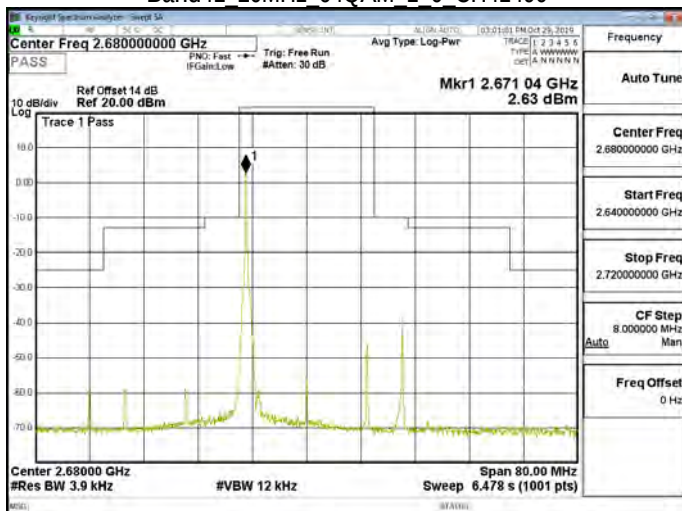
Band41 20MHz 64QAM 1 0 CH41490
