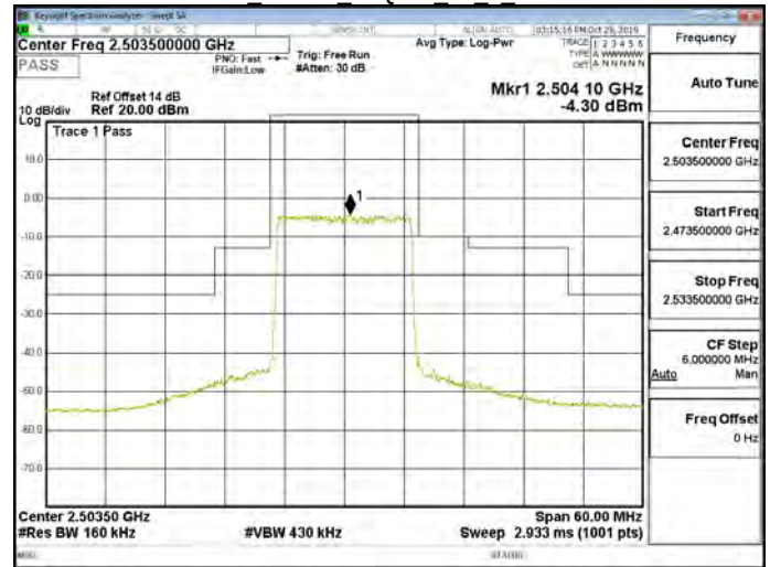
Band41 15MHz 64QAM 75 0 CH39725
