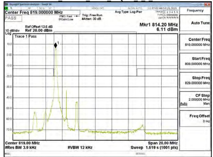
Band26 Part90s 3MHz 64QAM 1 0 CH26705
