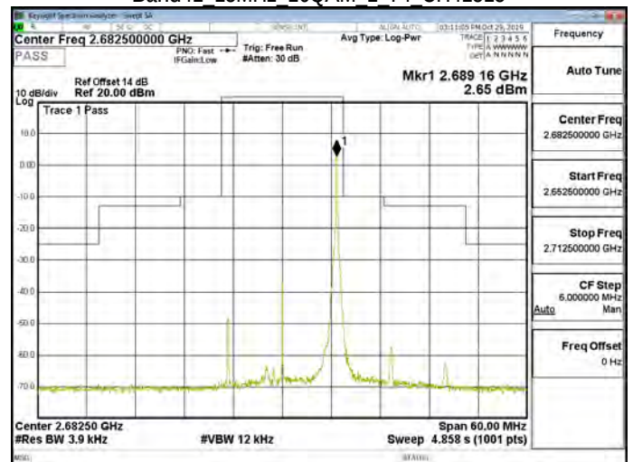
Band41 15MHz 16QAM 1 74 CH41515
