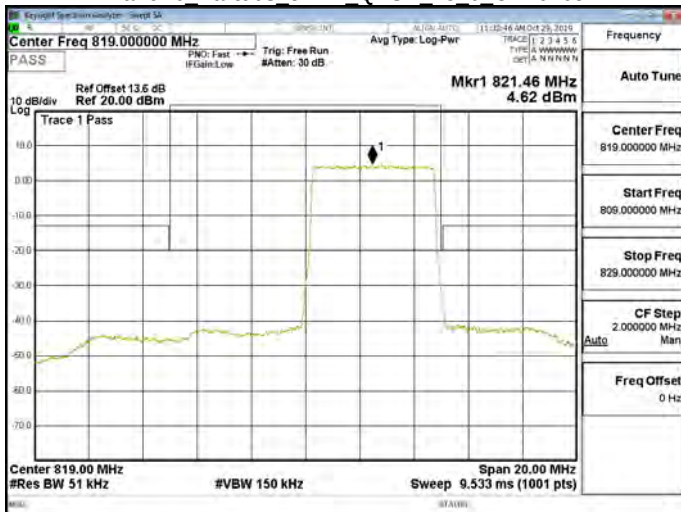
Band26 Part90s 5MHz QPSK 25 0 CH26765
