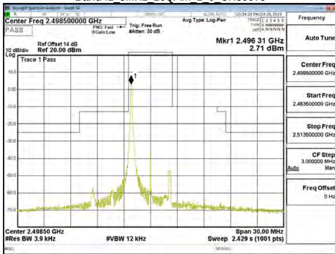
Band41 5MHz 16QAM 1 0 CH39675
