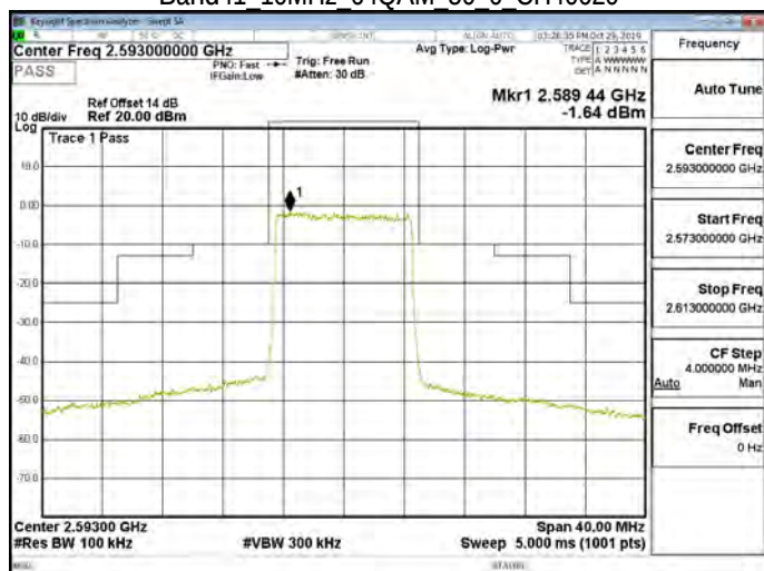
Band41 10MHz 64QAM 50 0 CH40620
