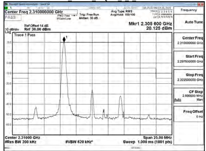
Band30 10MHz 64QAM 1 0 CH27710
