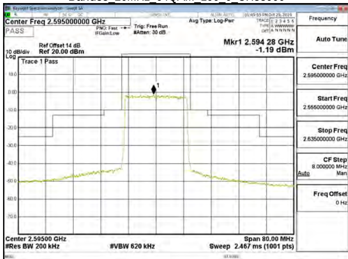
Band38 20MHz 64QAM 100 0 CH38000
