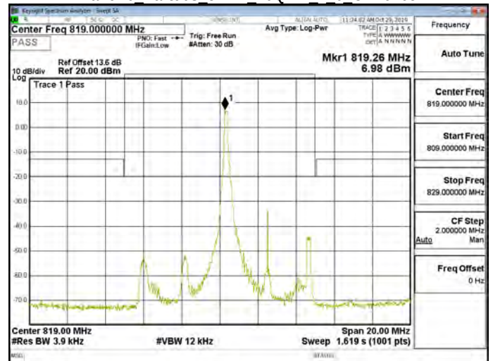
Band26 Part90s 5MHz 16QAM 1 0 CH26765
