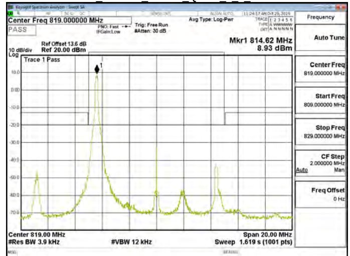
Band26 Part90s 10MHz QPSK 1 0 CH26740
