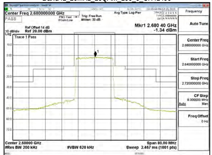
Band41 20MHz 16QAM 100 0 CH41490
