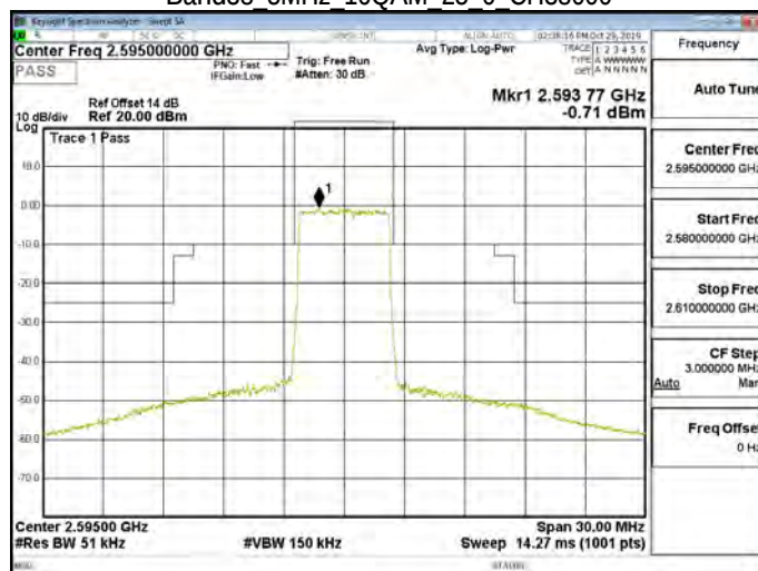
Band38 5MHz 16QAM 25 0 CH38000
