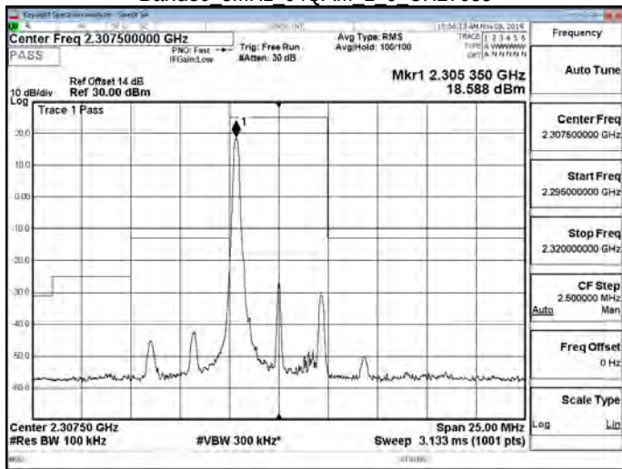
Band30 5MHz 64QAM 1 0 CH27685
