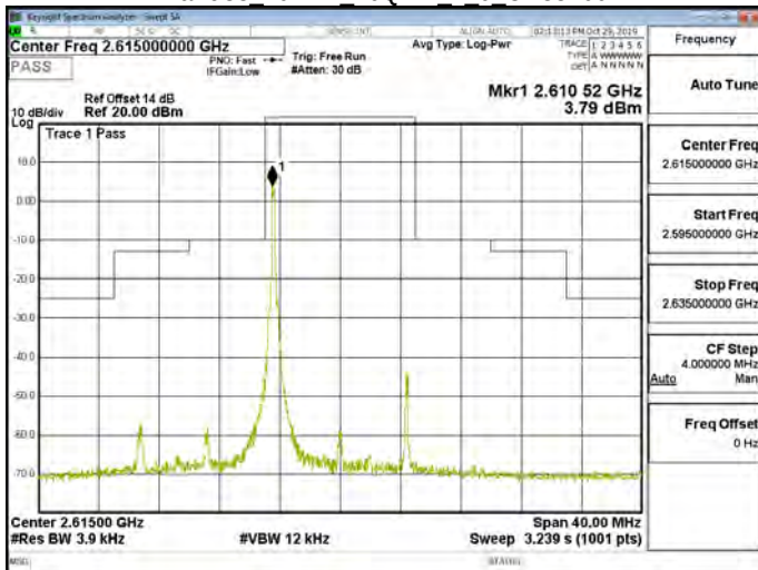
Band38 10MHz 16QAM 1 0 CH38200
