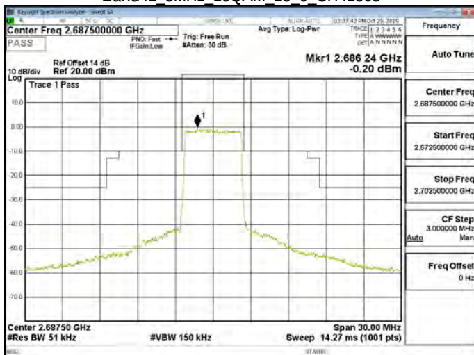
Band41 5MHz 16QAM 25 0 CH41565
