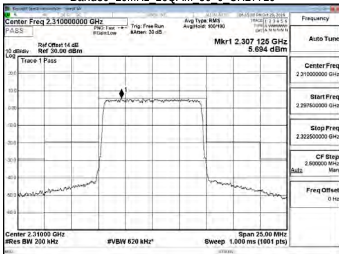
Band30 10MHz 16QAM 50 0 CH27710
