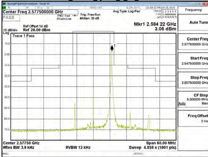
Band38 15MHz QPSK 1 74 CH37825
