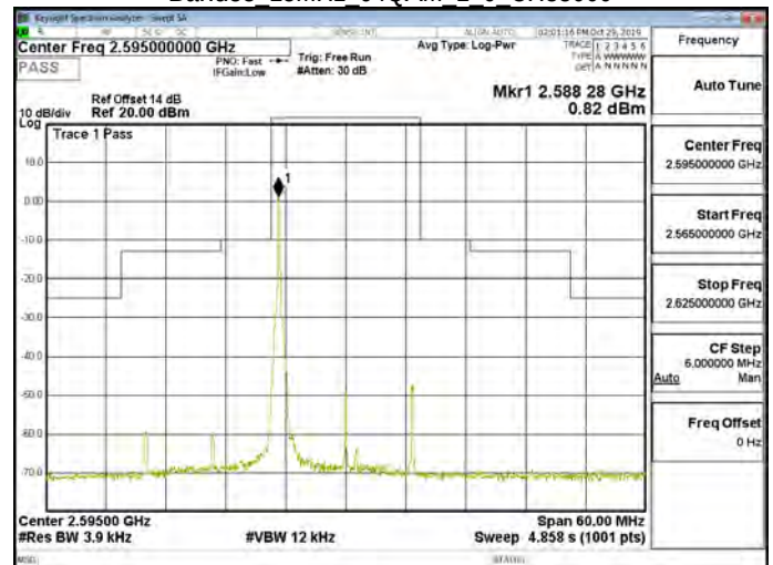
Band38 15MHz 64QAM 1 0 CH38000
