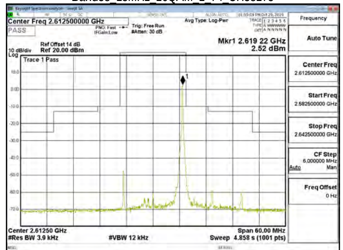
Band38 15MHz 16QAM 1 74 CH38175
