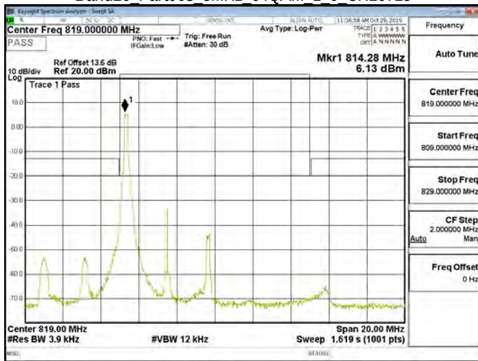
Band26 Part90s 5MHz 64QAM 1 0 CH26715
