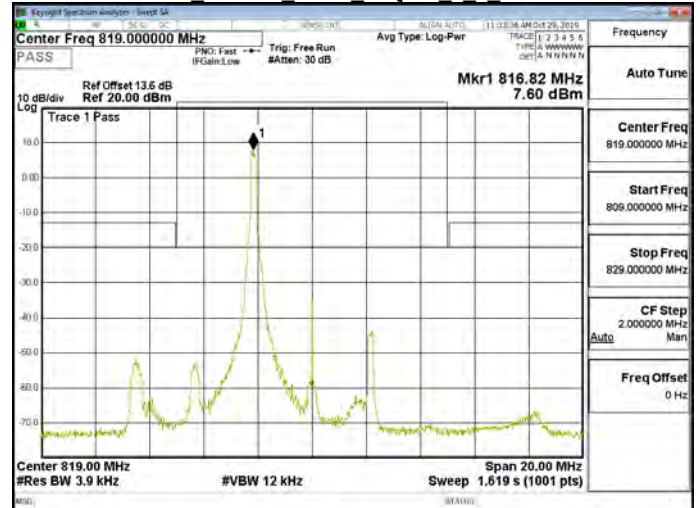
Band26 Part90s 5MHz 16QAM 1 0 CH26740
