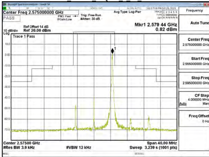
Band38 10MHz 64QAM 1 49 CH37800
