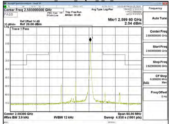
Band41 15MHz 16QAM 1 74 CH40620
