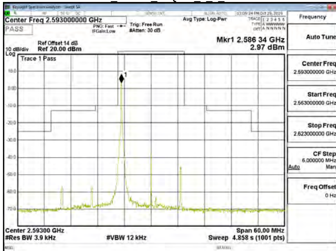
Band41 15MHz 16QAM 1 0 CH40620
