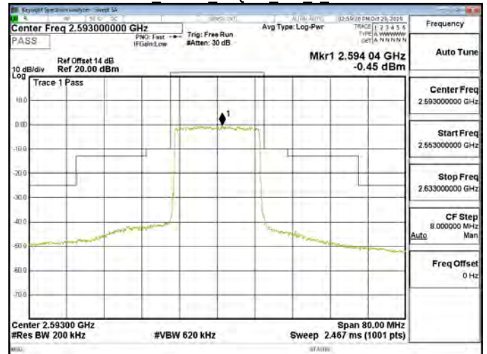
Band41 20MHz 16QAM 100 0 CH40620
