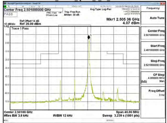
Band41 10MHz QPSK 1 49 CH39700
