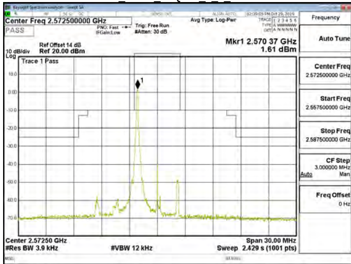
Band38 5MHz 64QAM 1 0 CH37775
