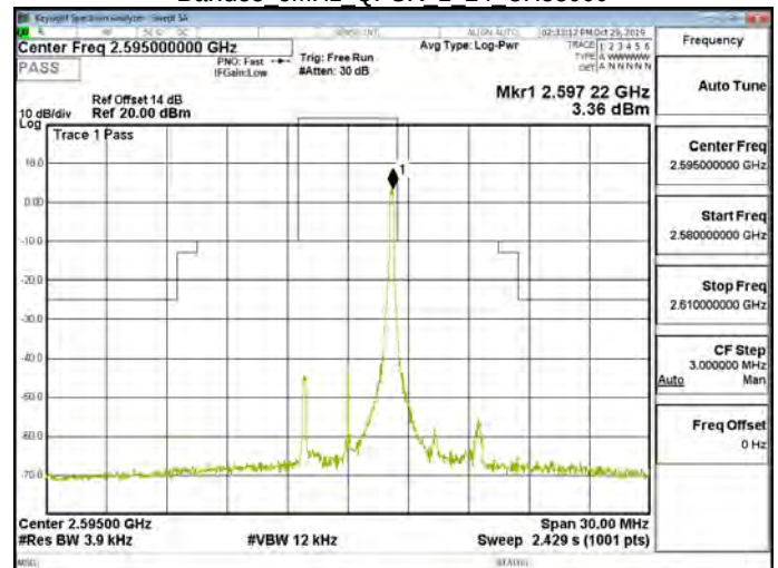
Band38 5MHz QPSK 1 24 CH38000
