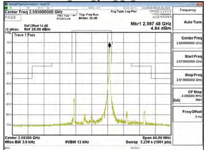
Band41 10MHz QPSK 1 49 CH40620
