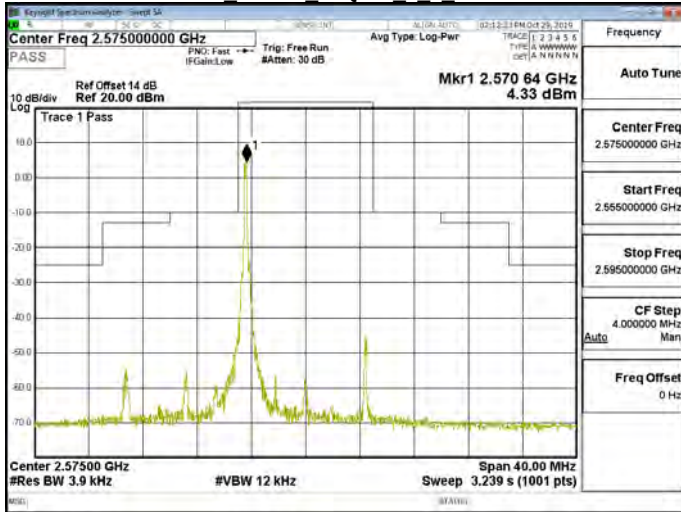
Band38 10MHz 16QAM 1 0 CH37800
