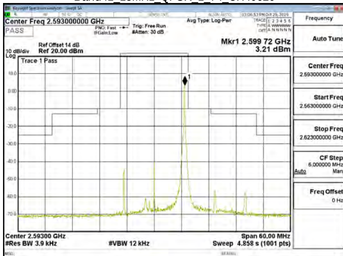
Band41 15MHz QPSK 1 74 CH40620
