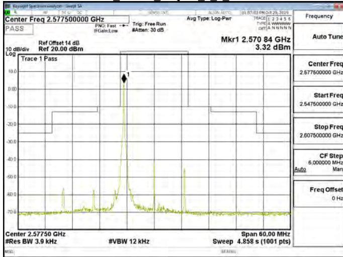
Band38 15MHz 16QAM 1 0 CH37825
