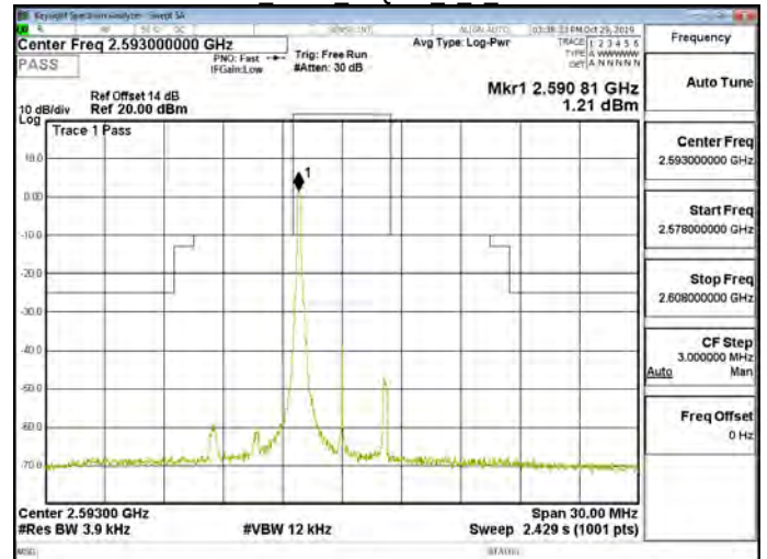
Band41 5MHz 64QAM 1 0 CH40620
