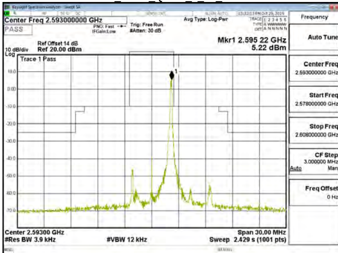
Band41 5MHz QPSK 1 24 CH40620
