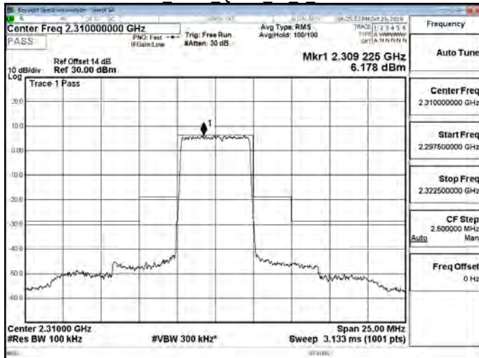
Band30 5MHz QPSK 25 0 CH27710
