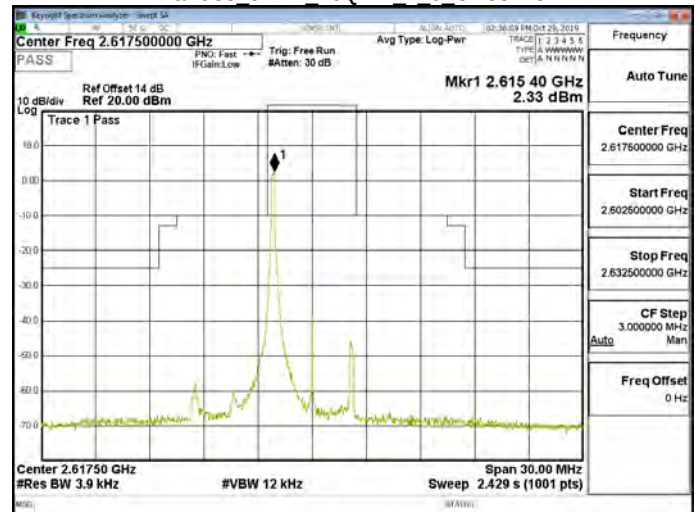
Band38 5MHz 16QAM 1 0 CH38225
