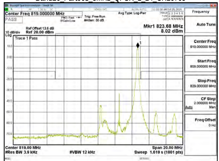
Band26 Part90s 5MHz QPSK 1 24 CH26765
