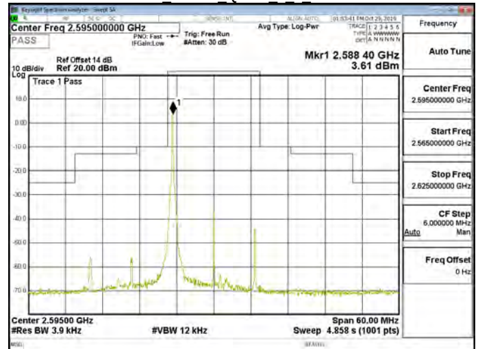
Band38 15MHz QPSK 1 0 CH38000
