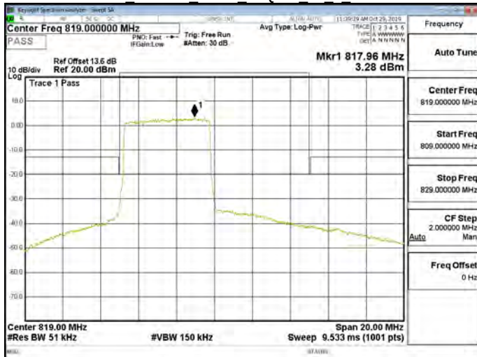
Band26 Part90s 5MHz 64QAM 25 0 CH26715
