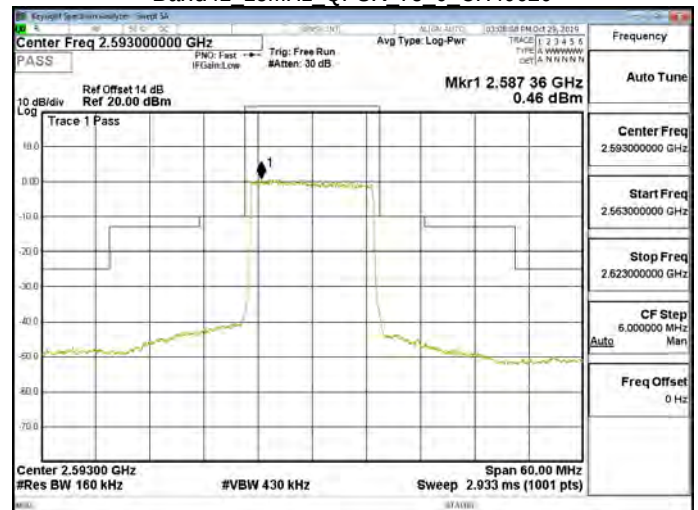
Band41 15MHz QPSK 75 0 CH40620
