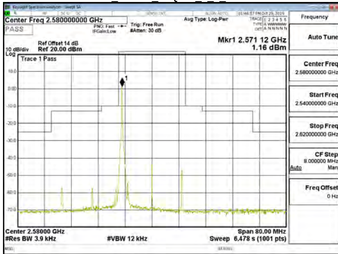
Band38 20MHz 64QAM 1 0 CH37850
