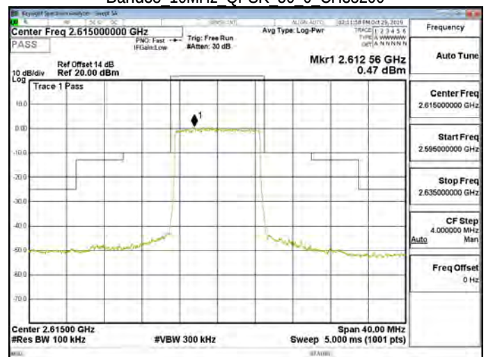
Band38 10MHz QPSK 50 0 CH38200
