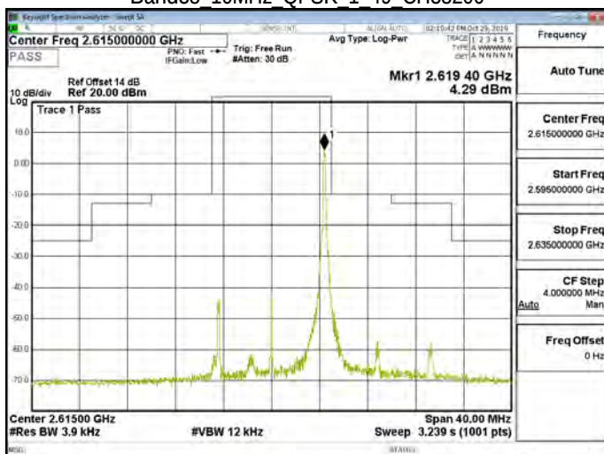
Band38 10MHz QPSK 1 49 CH38200
