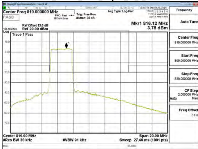
Band26 Part90s 3MHz 16QAM 15 0 CH26705
