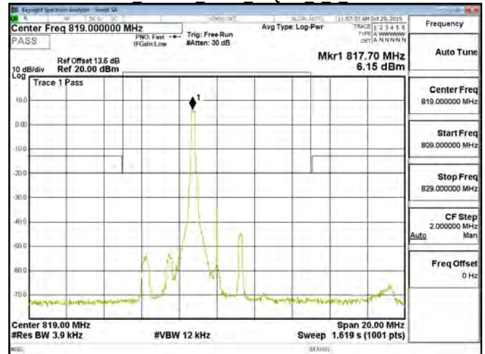
Band26 Part90s 3MHz 64QAM 1 0 CH26740
