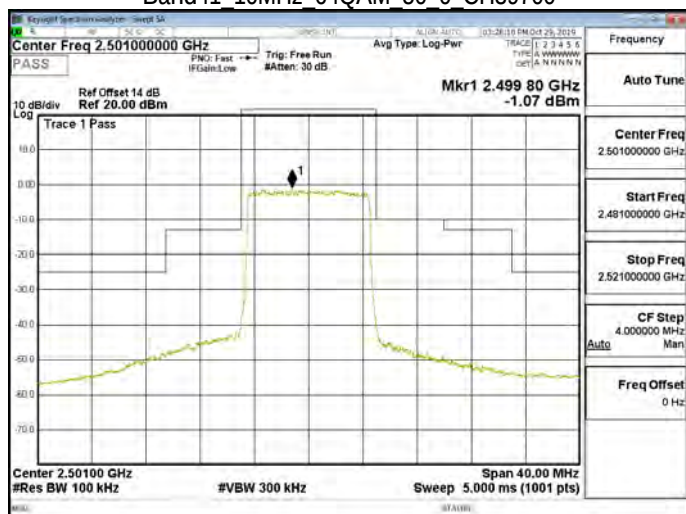
Band41 10MHz 64QAM 50 0 CH39700
