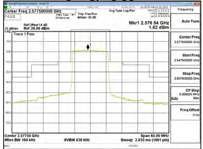
Band38 15MHz QPSK 75 0 CH37825
