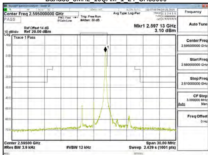
Band38 5MHz 16QAM 1 24 CH38000
