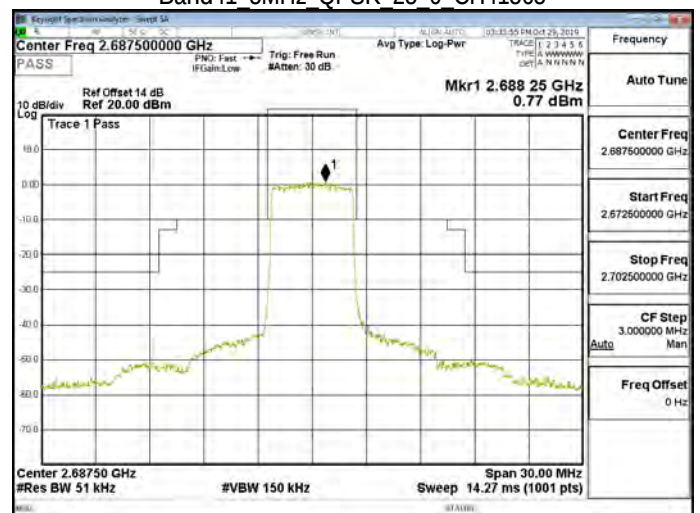
Band41 5MHz QPSK 25 0 CH41565
