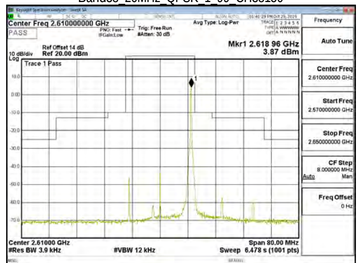
Band38 20MHz QPSK 1 99 CH38150
