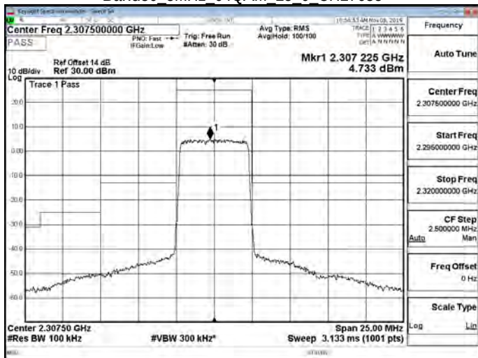
Band30 5MHz 64QAM 25 0 CH27685
