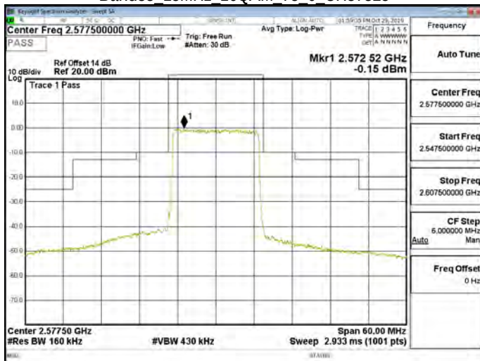
Band38 15MHz 16QAM 75 0 CH37825
