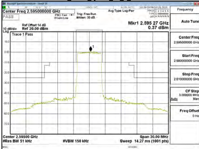
Band38 5MHz QPSK 25 0 CH38000
