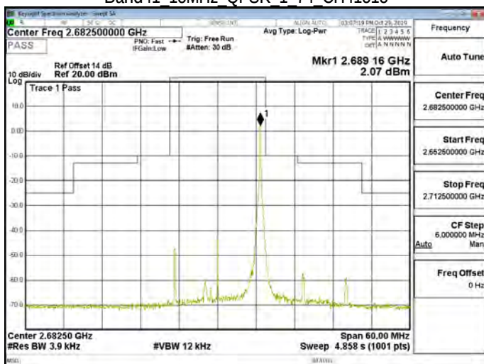
Band41 15MHz QPSK 1 74 CH41515
