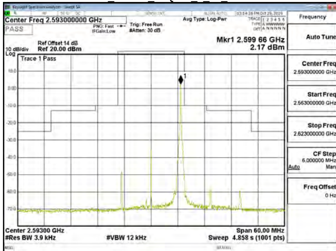
Band41 15MHz 64QAM 1 74 CH40620
