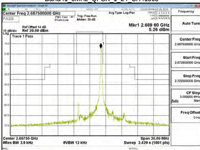
Band41 5MHz QPSK 1 24 CH41565
