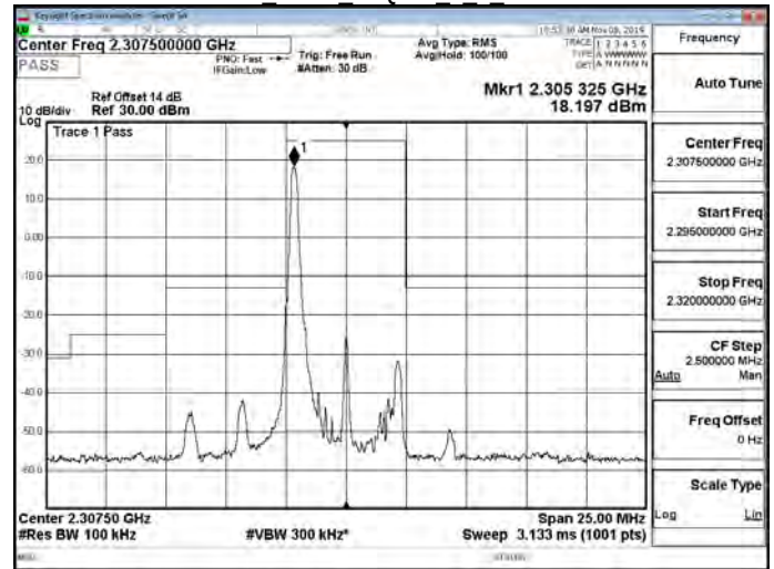
Band30 5MHz 16QAM 1 0 CH27685
