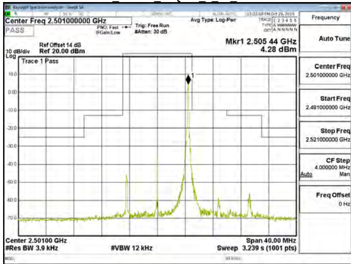
Band41 10MHz 16QAM 1 49 CH39700
