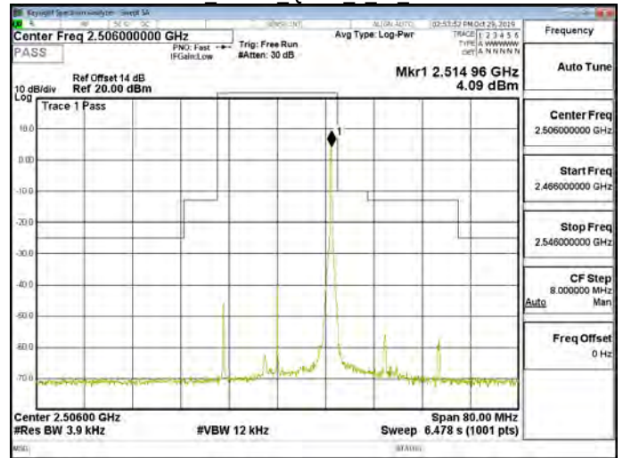
Band41 20MHz QPSK 1 99 CH39750
