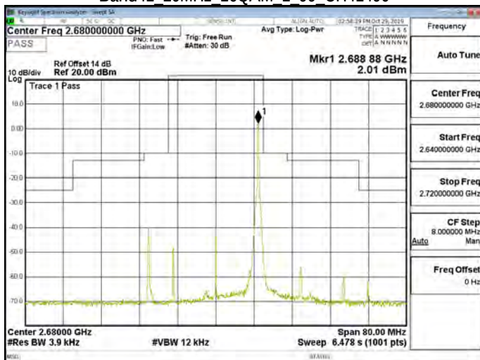
Band41 20MHz 16QAM 1 99 CH41490
