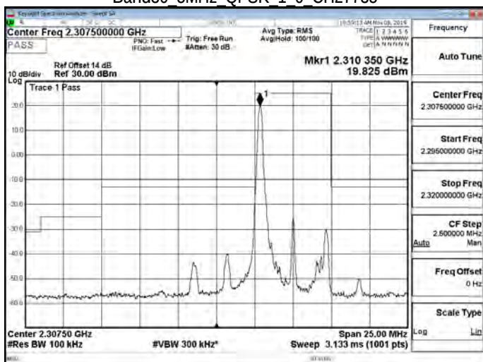
Band30 5MHz QPSK 1 0 CH27735
