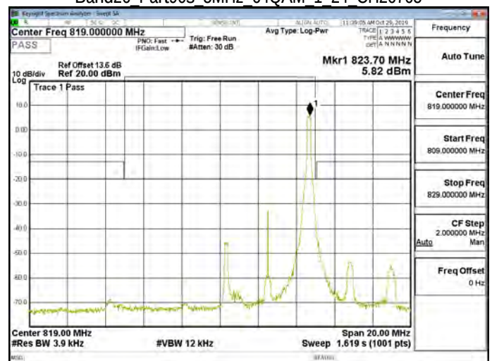
Band26 Part90s 5MHz 64QAM 1 24 CH26765
