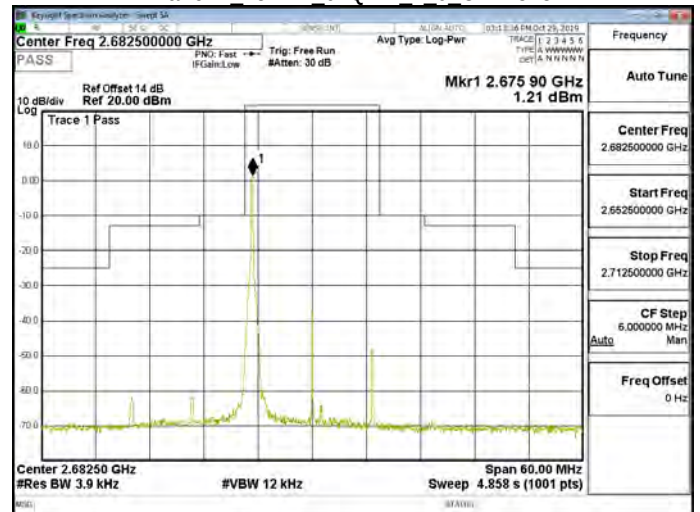
Band41 15MHz 64QAM 1 0 CH41515
