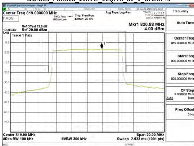
Band26 Part90s 10MHz 16QAM 50 0 CH26740
