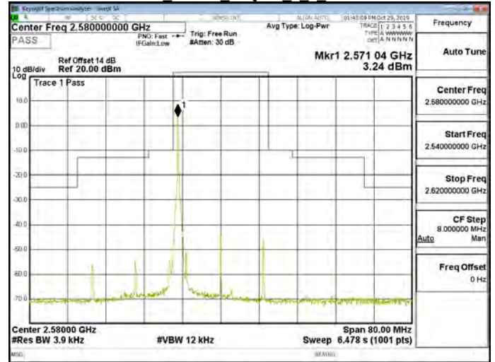
Band38 20MHz 16QAM 1 0 CH37850
