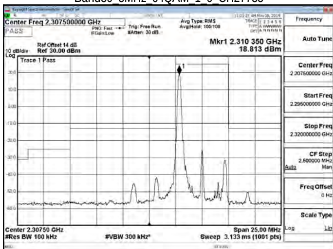
Band30 5MHz 64QAM 1 0 CH27735
