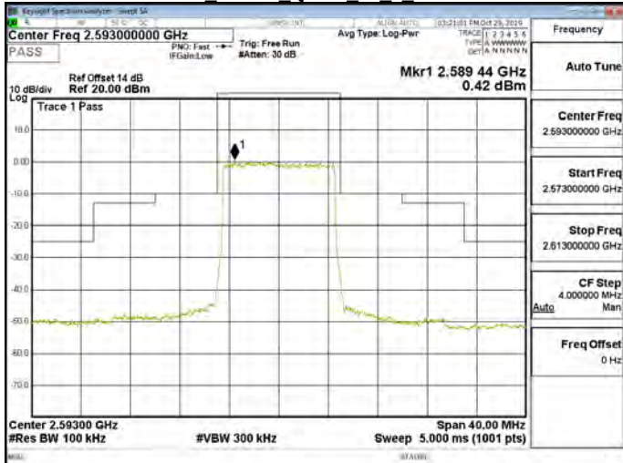
Band41 10MHz QPSK 50 0 CH40620
