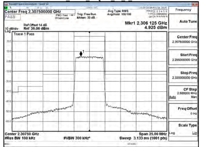
Band30 5MHz 16QAM 25 0 CH27685
