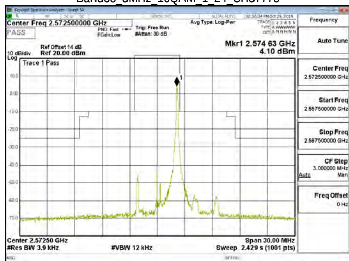
Band38 5MHz 16QAM 1 24 CH37775
