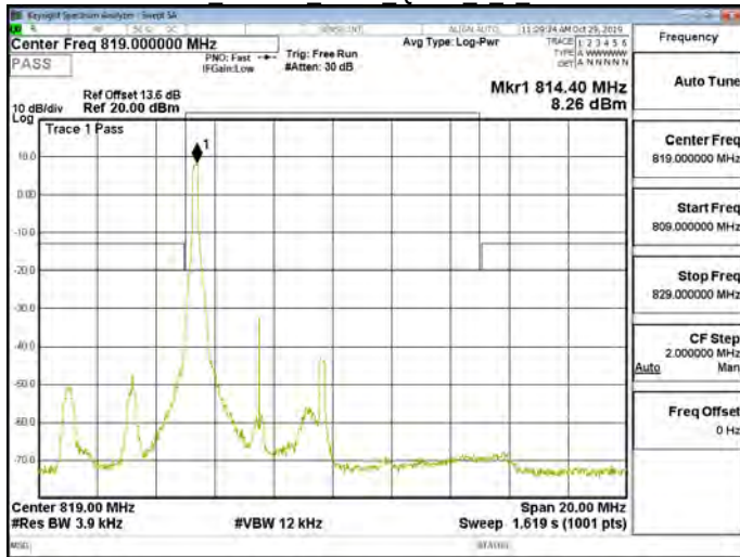
Band26 Part90s 5MHz QPSK 1 0 CH26715
