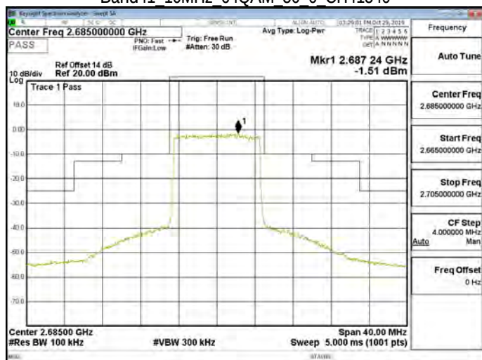
Band41 10MHz 64QAM 50 0 CH41540
