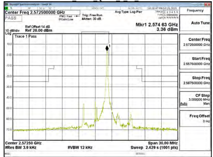
Band38 5MHz QPSK 1 24 CH37775
