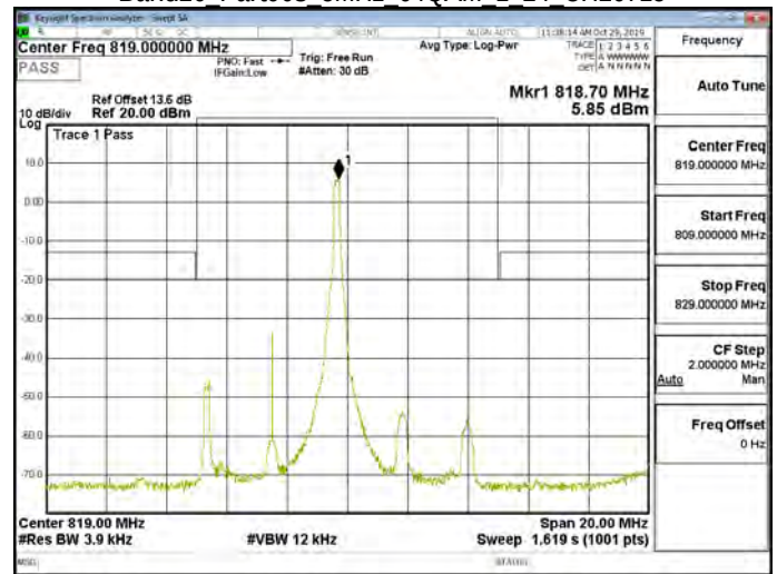
Band26 Part90s 5MHz 64QAM 1 24 CH26715
