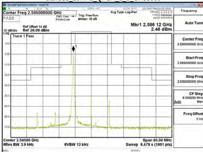
Band38 20MHz QPSK 1 0 CH38000
