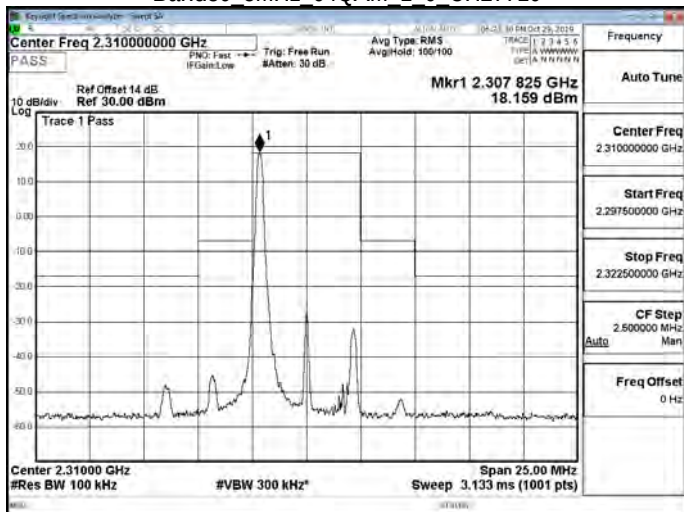
Band30 5MHz 64QAM 1 0 CH27710
