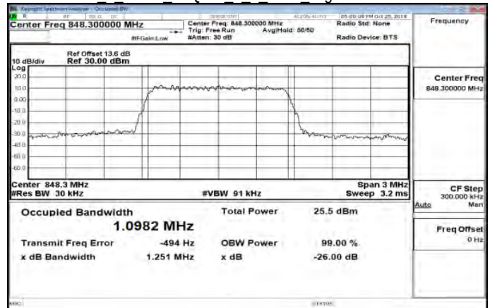
Band26 1 4MHz 16QAM 6 0 Main HighCH27033-848.3
