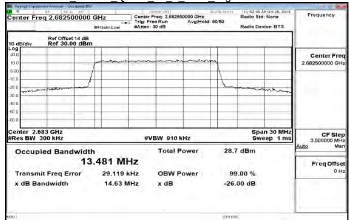
Band41 15MHz QPSK 75 0 Main HighCH41515-2682.5
