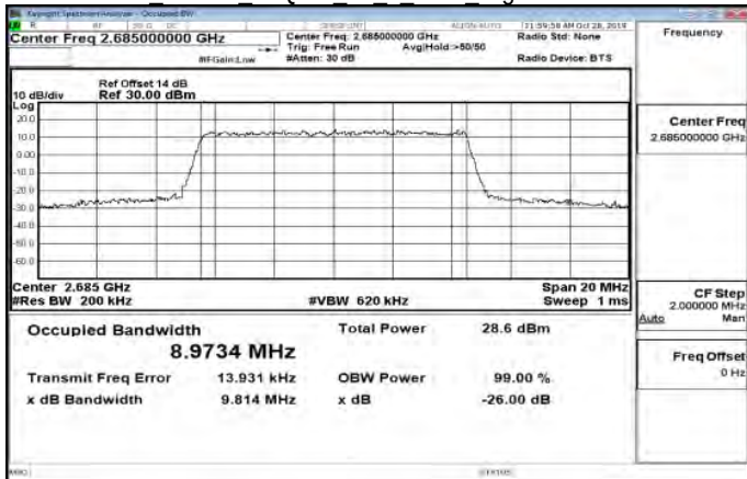
Band41 10MHz 64QAM 50 0 Main HighCH41540-2685
