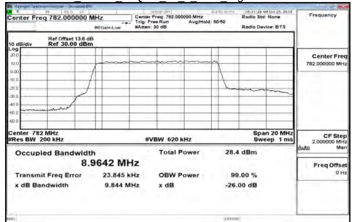
Band13 10MHz 64QAM 50 0 Main HighCH23230-782
