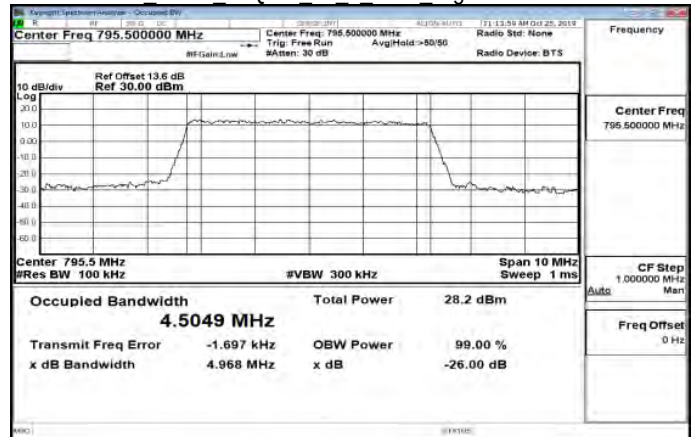
Band14 5MHz 16QAM 25 0 Main HighCH23355-795.5
