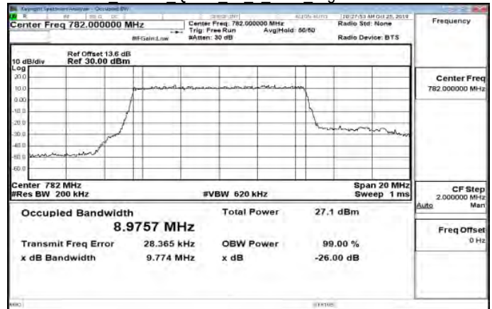
Band13 10MHz QPSK 50 0 Main HighCH23230-782
