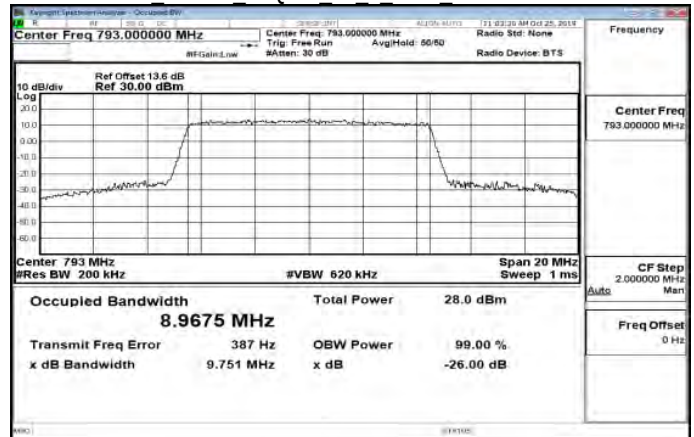
Band14 10MHz 64QAM 50 0 Main MidCH23330-793
