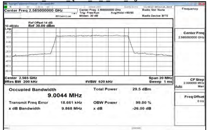
Band7 10MHz QPSK 50 0 Main HighCH21400-2565
