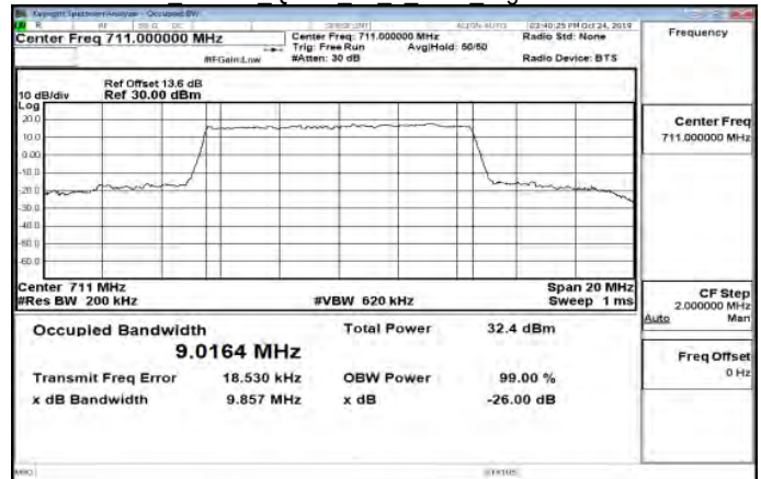
Band12 10MHz QPSK 50 0 Main HighCH23130-711
