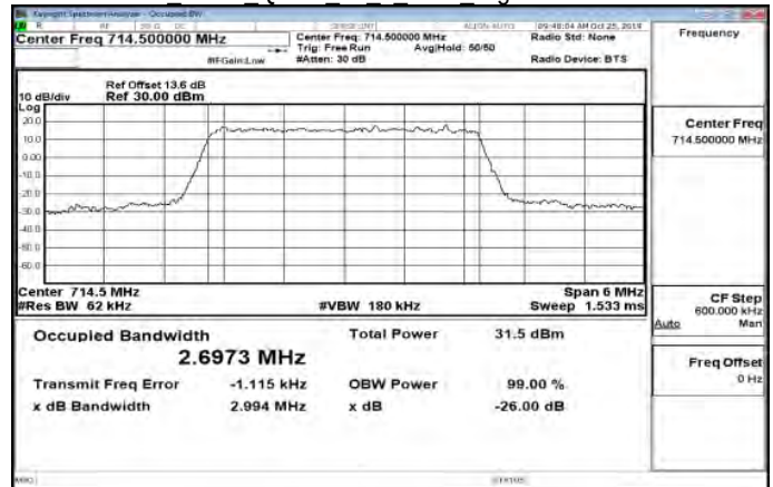
Band12 3MHz QPSK 15 0 Main HighCH23165-714.5
