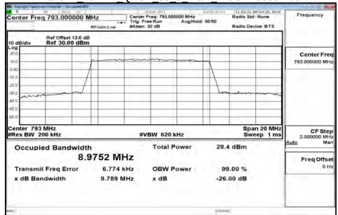
Band14 10MHz 16QAM 50 0 Main MidCH23330-793
