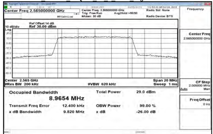
Band7 10MHz 64QAM 50 0 Main HighCH21400-2565
