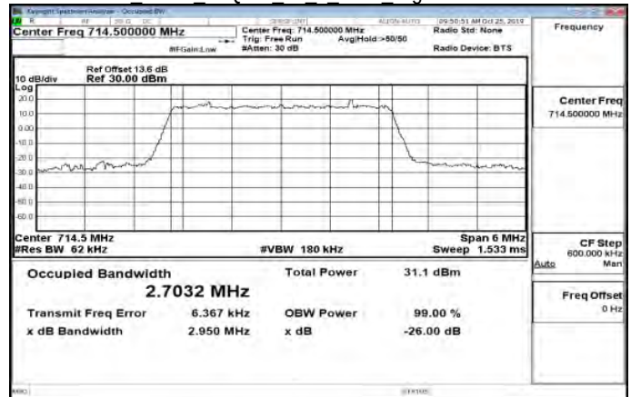
Band12 3MHz 64QAM 15 0 Main HighCH23165-714.5
