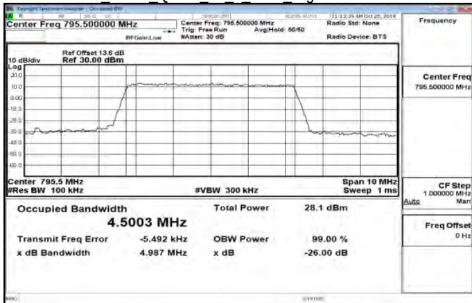
Band14 5MHz QPSK 25 0 Main HighCH23355-795.5
