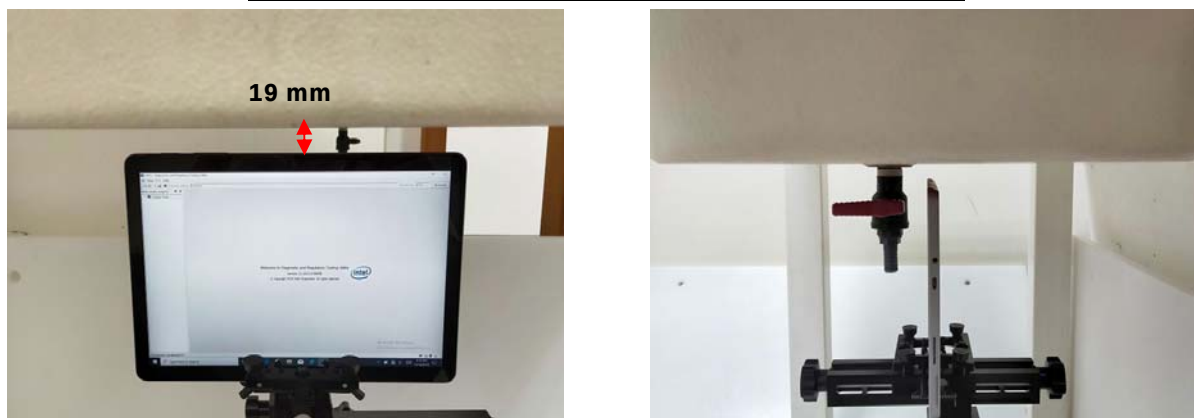
Fig.12 EUT Top side to flat phantom
