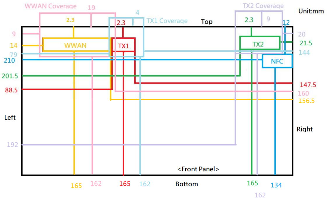
Fig.16 Antenna position of EUT
