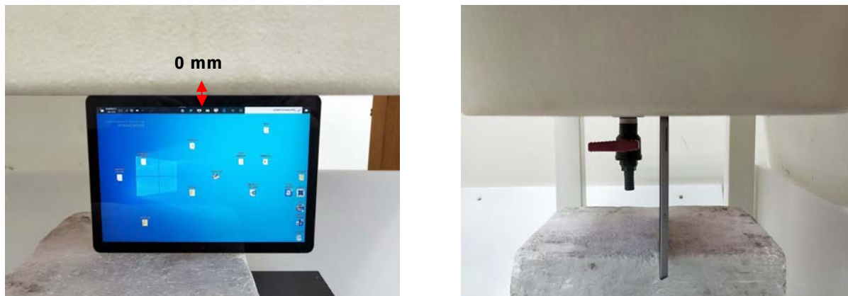
Fig.5 EUT Bottom side to flat phantom
