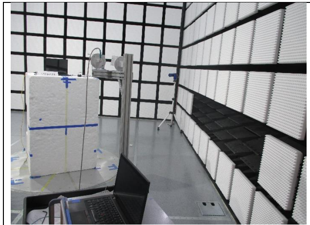
ABOVE 18GHz (FRONT)
