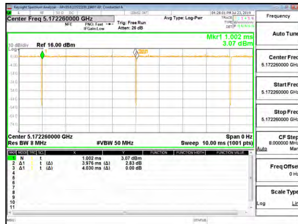
802.11ax HE80 OFDMA, RU size 106T MODE
