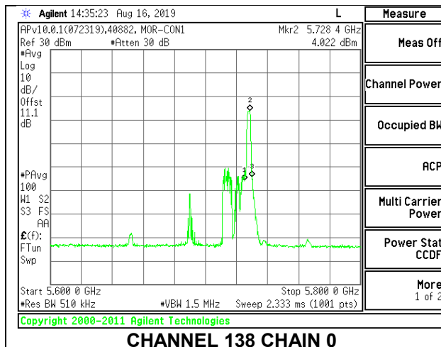
CHANNEL 138 CHAIN 0
