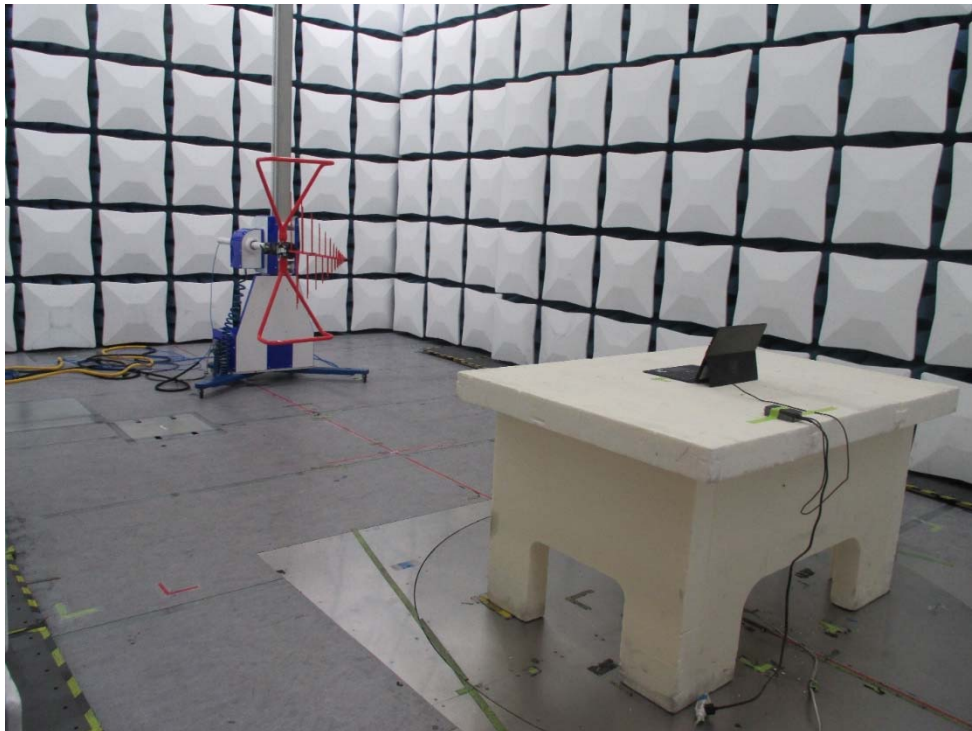
Figure 2 Radiated Spurious Emissions Test Setup (30M-1GHz)
