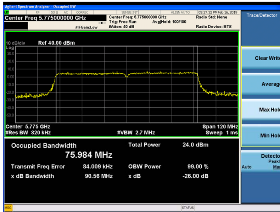
Plot 9-142. 26-dB Emission Bandwidth and 99% OBW Chain 1 802.11ac VHT80 (Ch. 155)
