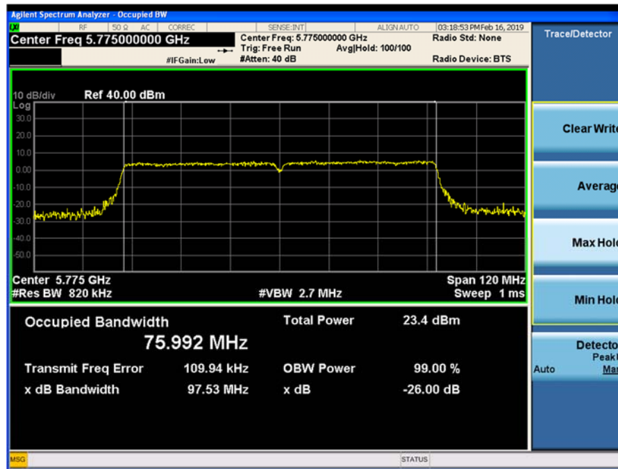
Plot 9-136. 26-dB Emission Bandwidth and 99% OBW Chain 0 802.11ac VHT80 (Ch. 155)
