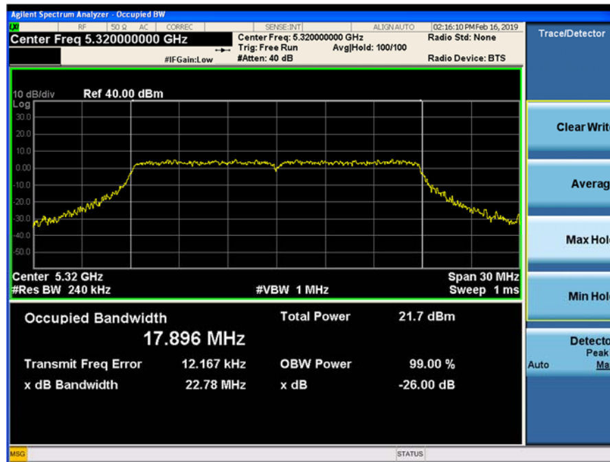
Plot 9-103. 26dB Emission Bandwidth and 99% OBW Chain 1 802.11ac VHT 20 (CH. 64)
