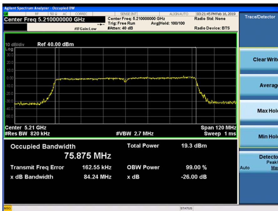
Plot 9-131. 26-dB Emission Bandwidth and 99% OBW Chain 0 802.11ac VHT80 (Ch. 42)
