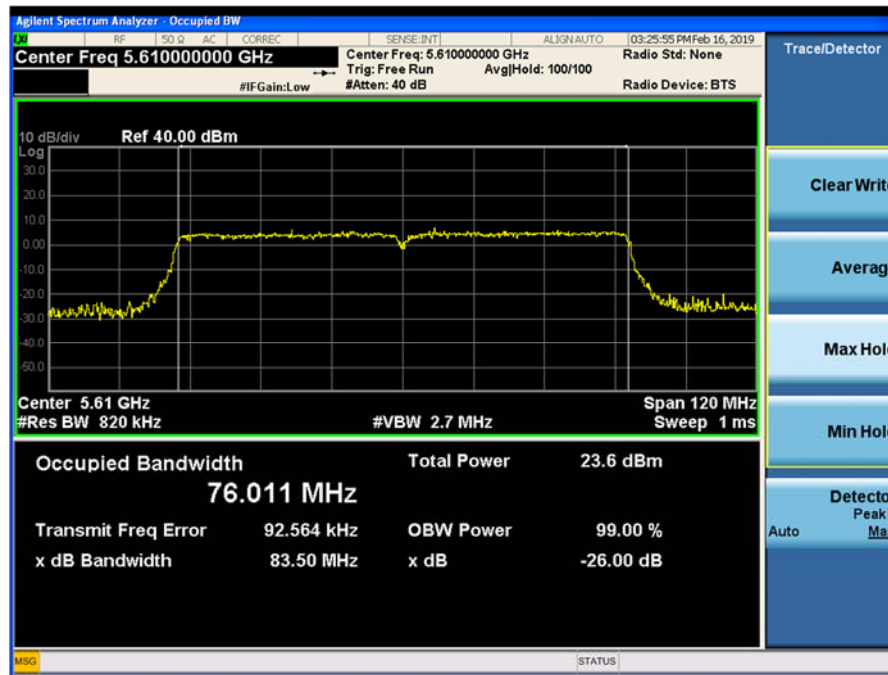
Plot 9-140. 26-dB Emission Bandwidth and 99% OBW Chain 1 802.11ac VHT80 (Ch. 122)
