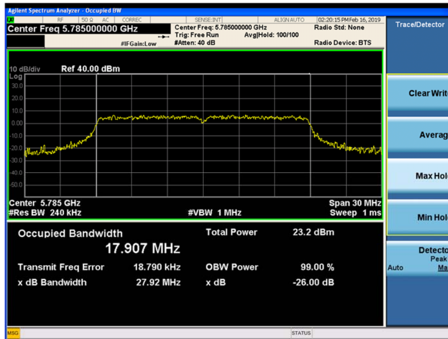
Plot 9-109. 26dB Emission Bandwidth and 99% OBW Chain 1 802.11ac VHT 20 (CH. 157)
