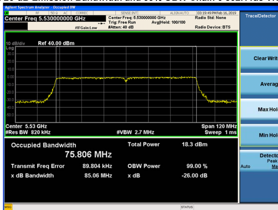
Plot 9-133. 26-dB Emission Bandwidth and 99% OBW Chain 0 802.11ac VHT80 (Ch. 106)
