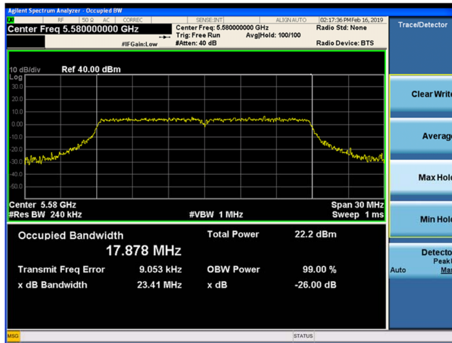
Plot 9-105. 26dB Emission Bandwidth and 99% OBW Chain 1 802.11ac VHT 20 (CH. 116)
