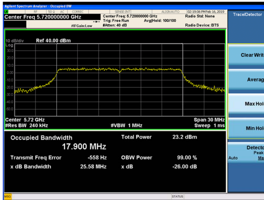
Plot 9-107. 26dB Emission Bandwidth and 99% OBW Chain 1 802.11ac VHT 20 (CH. 144)
