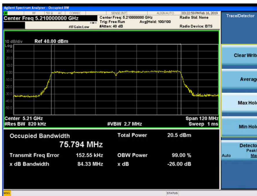
Plot 9-137. 26-dB Emission Bandwidth and 99% OBW Chain 1 802.11ac VHT80 (Ch. 42)
