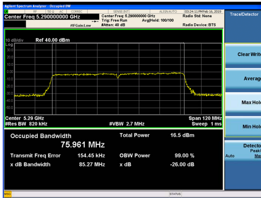
Plot 9-138. 26-dB Emission Bandwidth and 99% OBW Chain 1 802.11ac VHT80 (Ch. 58)
