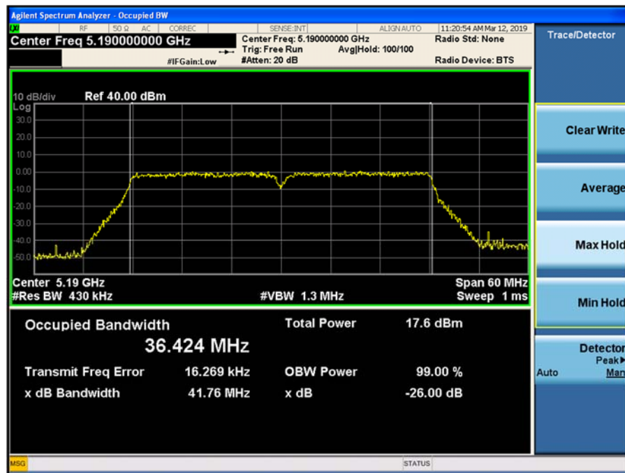
Plot 9-111. 26dB Emission Bandwidth and 99% OBW Chain 0 802.11ac VHT 40 (CH. 38)
