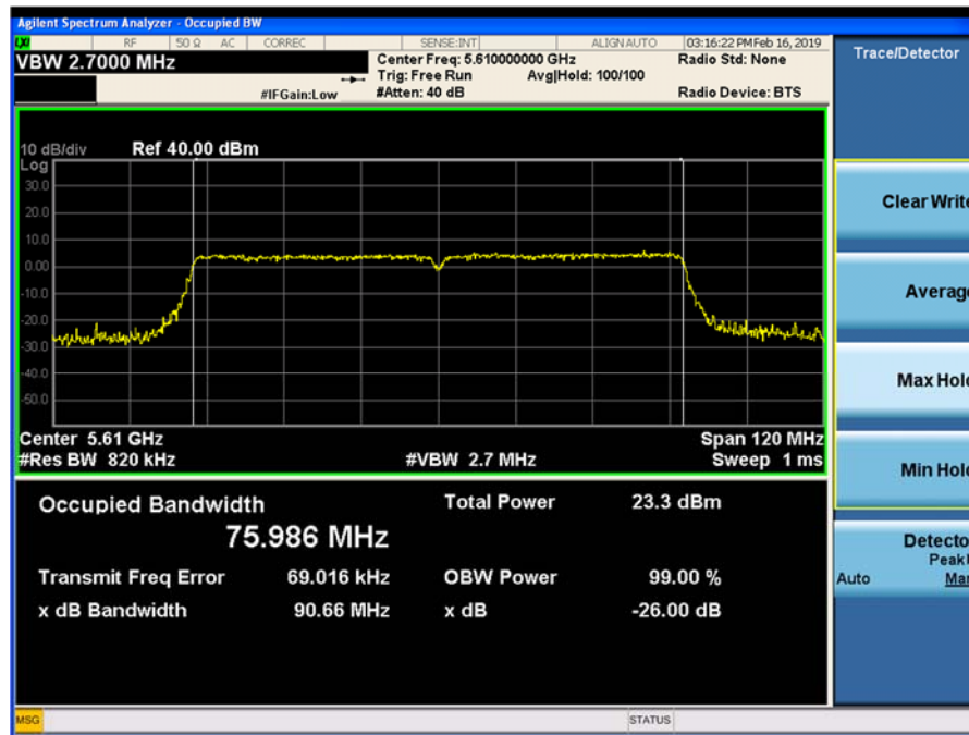
Plot 9-134. 26-dB Emission Bandwidth and 99% OBW Chain 0 802.11ac VHT80 (Ch. 122)
