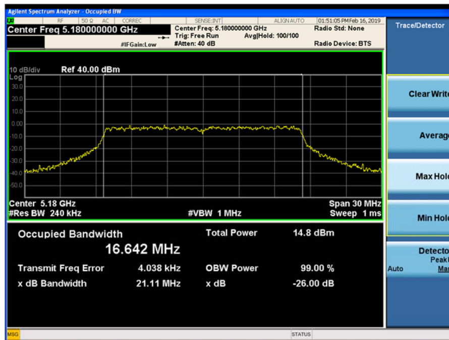
Plot 9-26. 26-dB Emission Bandwidth and 99% OBW Chain 1 802.11a (Ch. 36)
