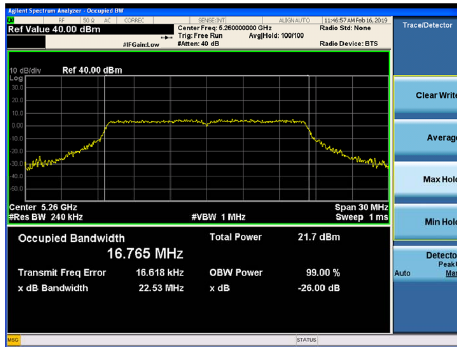
Plot 9-16. 26-dB Emission Bandwidth and 99% OBW Chain 0 802.11a (Ch. 52)
