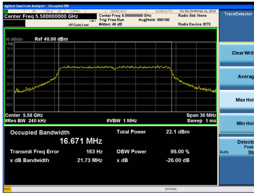
Plot 9-33. 26-dB Emission Bandwidth and 99% OBW Chain 1 802.11a (Ch. 116)
