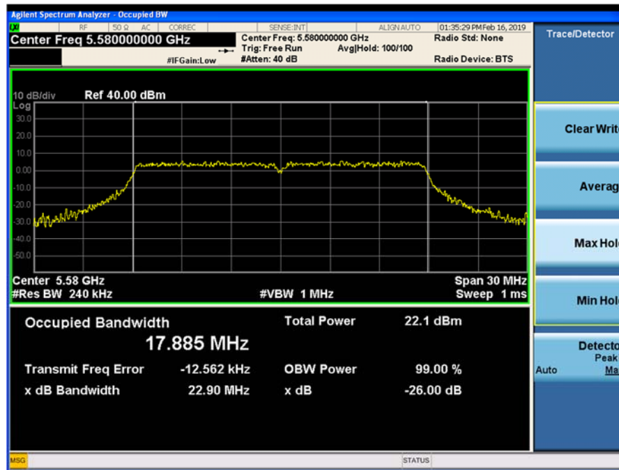
Plot 9-46. 26-dB Emission Bandwidth and 99% OBW Chain 0 802.11n HT20 (Ch. 116)
