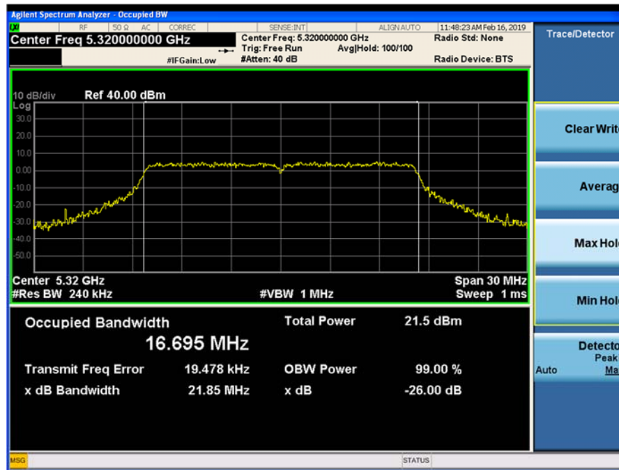
Plot 9-18. 26-dB Emission Bandwidth and 99% OBW Chain 0 802.11a (Ch. 64)
