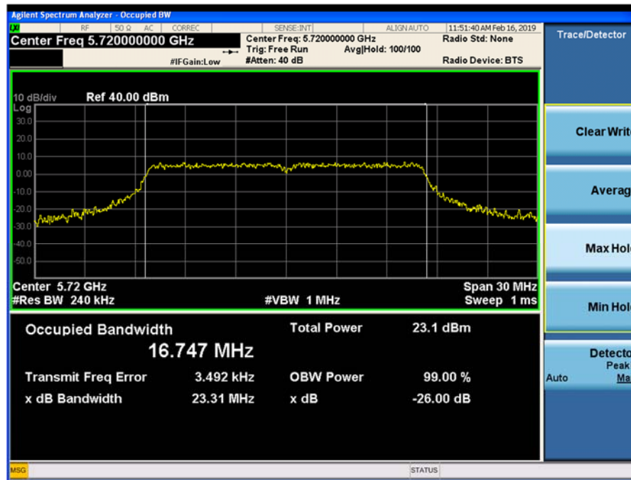
Plot 9-22 26-dB Emission Bandwidth and 99% OBW Chain 0 802.11a (Ch. 144)
