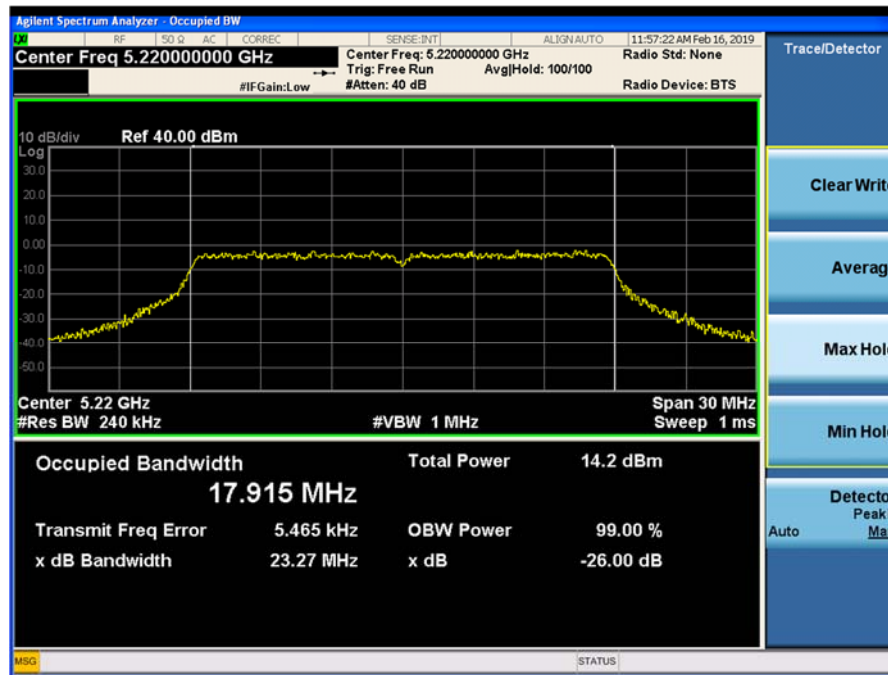
Plot 9-40. 26-dB Emission Bandwidth and 99% OBW Chain 0 802.11n HT20 (Ch. 44)
