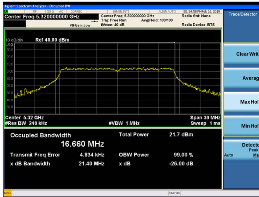
Plot 9-31. 26-dB Emission Bandwidth and 99% OBW Chain 1 802.11a (Ch. 64)
