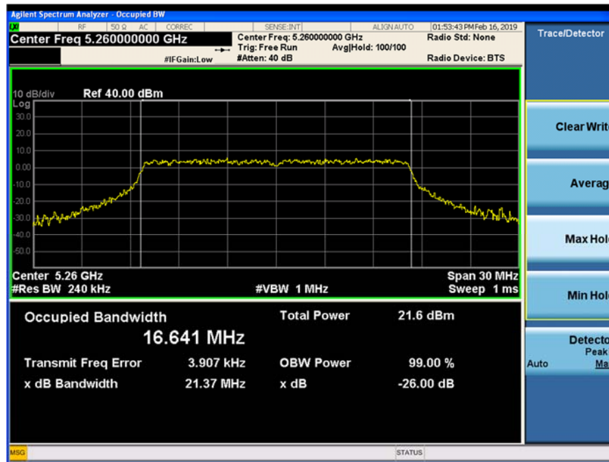
Plot 9-29. 26-dB Emission Bandwidth and 99% OBW Chain 1 802.11a (Ch. 52)
