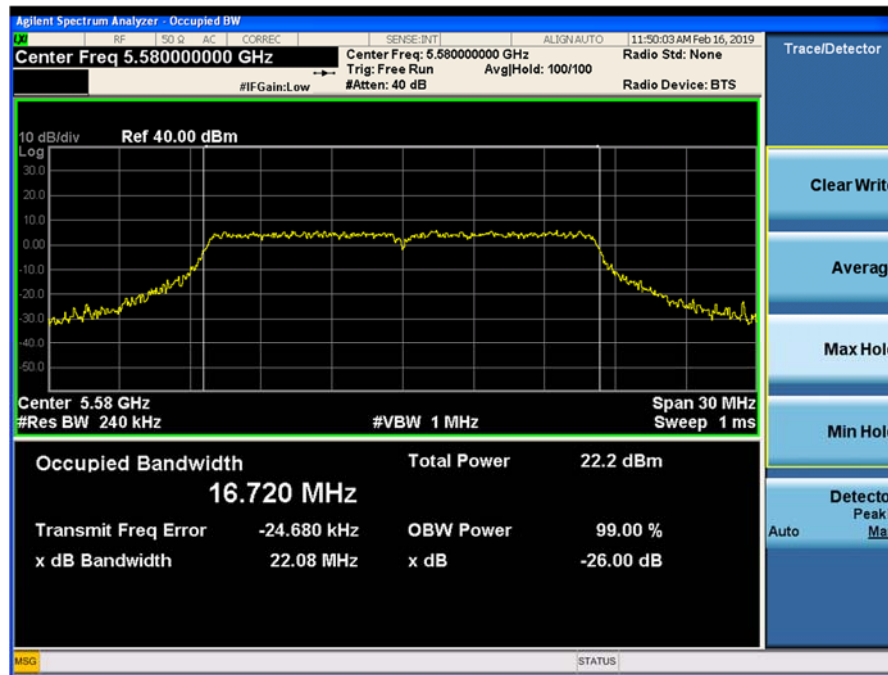
Plot 9-20. 26-dB Emission Bandwidth and 99% OBW Chain 0 802.11a (Ch. 116)
