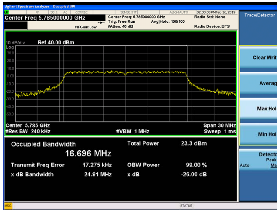
Plot 9-37. 26-dB Emission Bandwidth and 99% OBW Chain 1 802.11a (Ch. 157)
