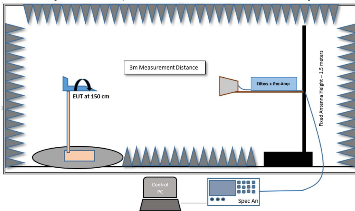
Figure 8-3. Test Setup for Radiated measurements in 1GHz- 18GHz Range
