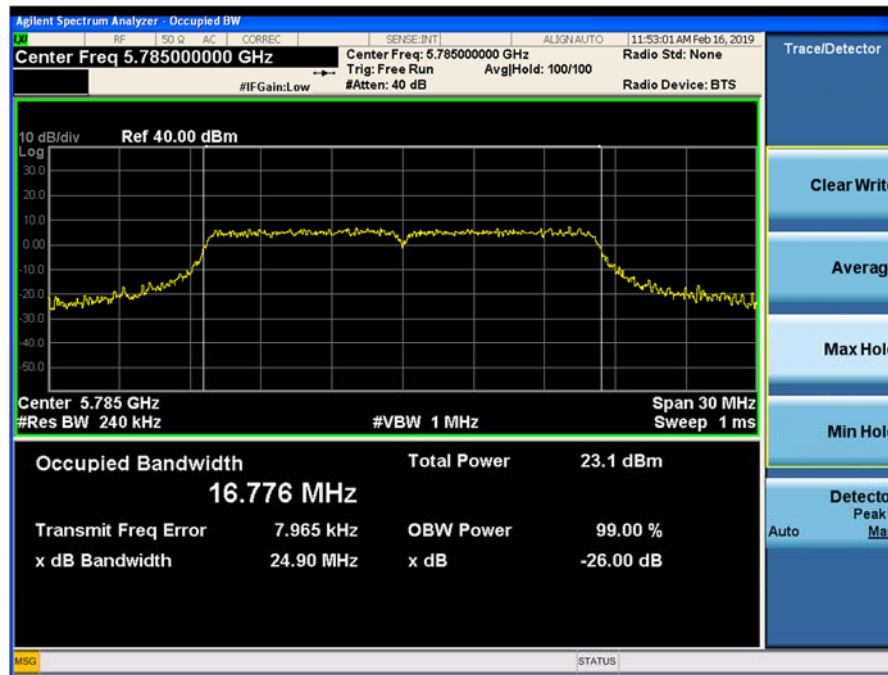
Plot 9-24. 26-dB Emission Bandwidth and 99% OBW Chain 0 802.11a (Ch. 157)
