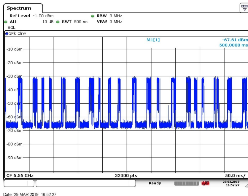
Figure 9. Channel Loading (5550 MHz 40 MHz BW)
