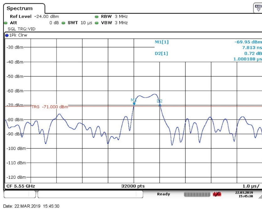
Figure 4. Radar Pulse width: Radar Type 0 (5550 MHz 40 MHz BW)
