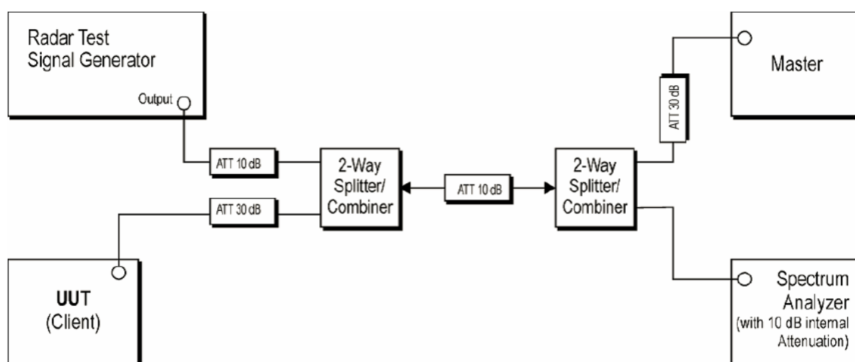
Figure 1. Test Setup for Antenna Port Conducted Measurements
