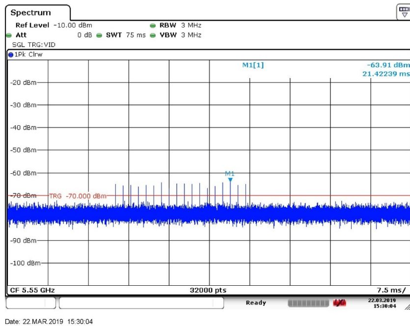
Figure 3. Radar Burst Level at -64dBm: Radar Type 0 (5550 MHz 40 MHz BW)
