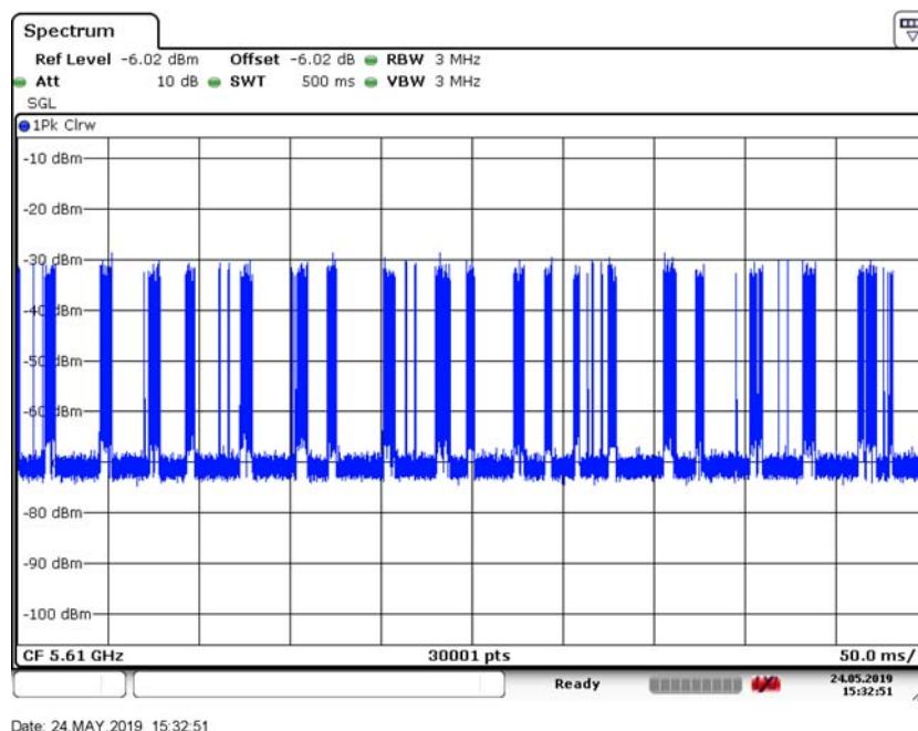
Figure 10. Channel Loading (5610 MHz 80 MHz BW)
