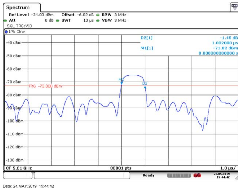
Figure 7. Radar Pulse width: Radar Type 0 (5610 MHz 80 MHz BW)
