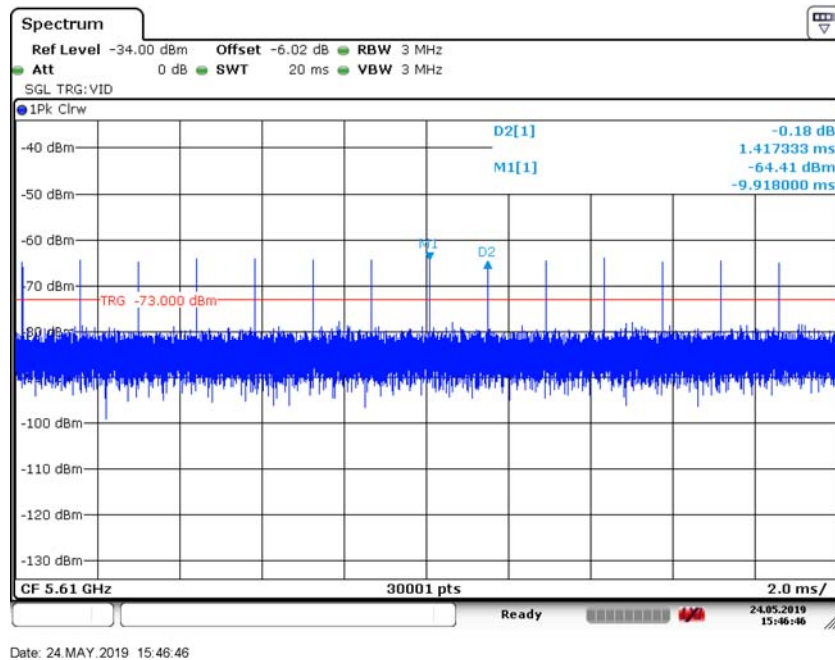
Figure 8. Radar Pulse Repetition Interval: Radar Type 0 (5610 MHz 80 MHz BW)
