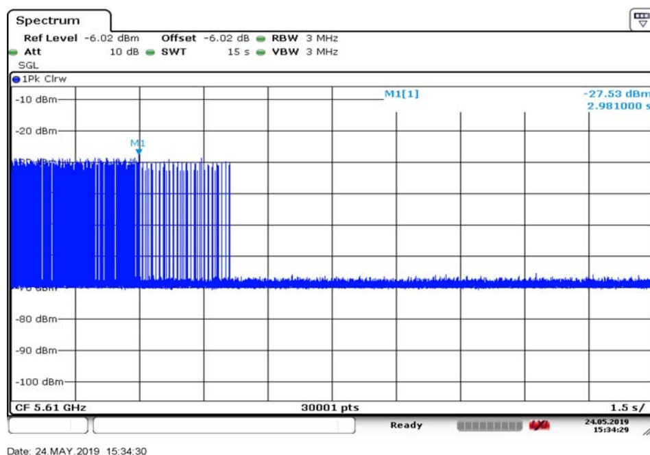
Figure 14. DFS Radar Detection Plot Channel 5610 MHz
