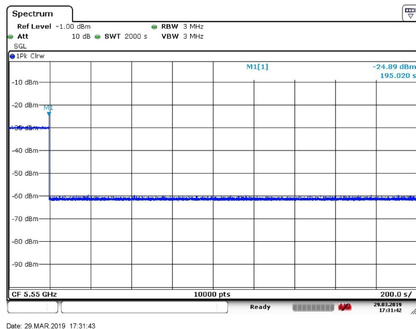
Figure 21. 30 Minute Non-Occupancy Period (5550 MHz)
