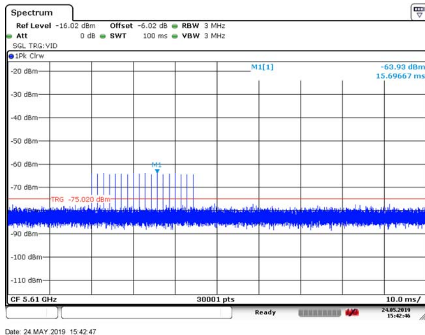
Figure 6. Radar Burst Level at -64dBm: Radar Type 0 (5610 MHz 80 MHz BW)
