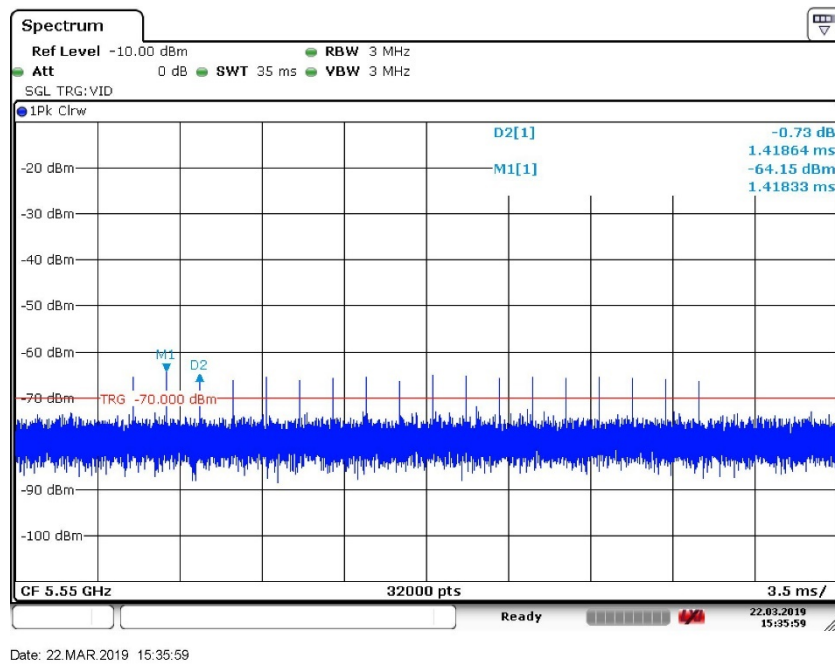
Figure 5. Radar Pulse Repetition Interval: Radar Type 0 (5550 MHz 40 MHz BW)
