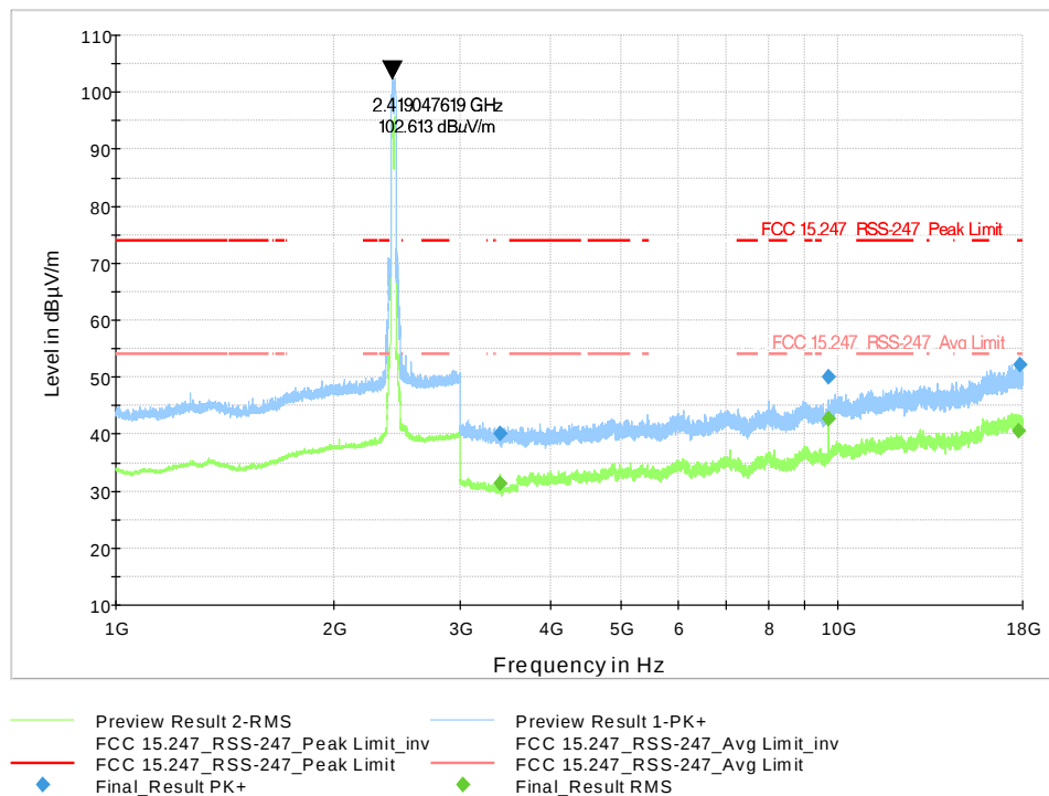
Figure 9-337 Radiated Spurious Emission 1-18GHz 802.11n40- Ch.2
