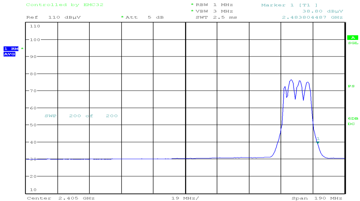
Figure 9-359 Radiated Band Edge Average 802.11g - Ch.13
