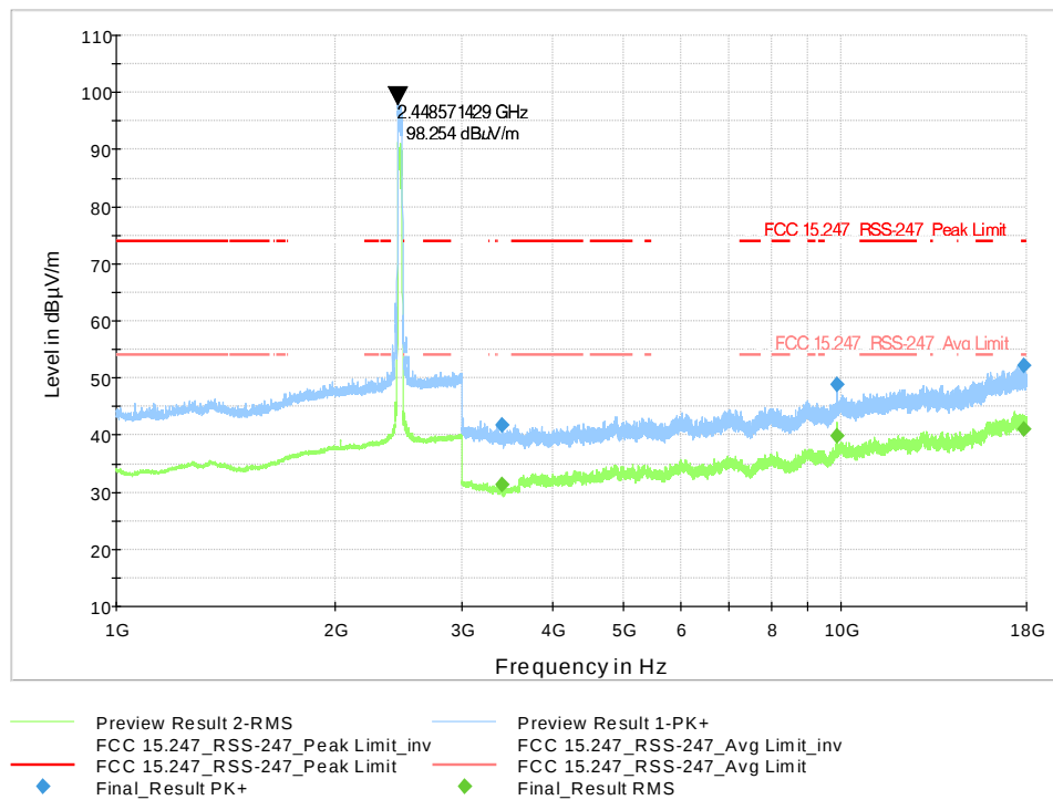
Figure 9-339 Radiated Spurious Emission 1-18GHz 802.11n40- Ch.11
