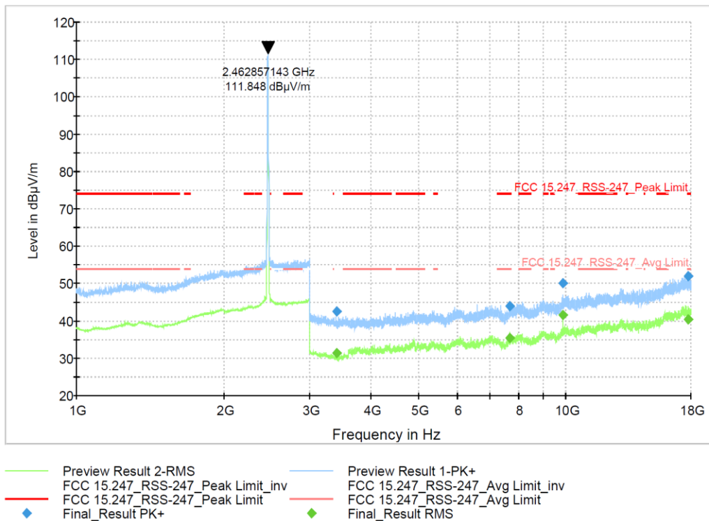
Figure 9-324 Radiated Spurious Emission 1-18GHz 802.11b - Ch.11
