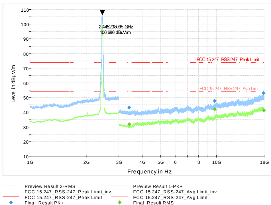
Figure 9-338 Radiated Spurious Emission 1-18GHz 802.11n40- Ch.7
