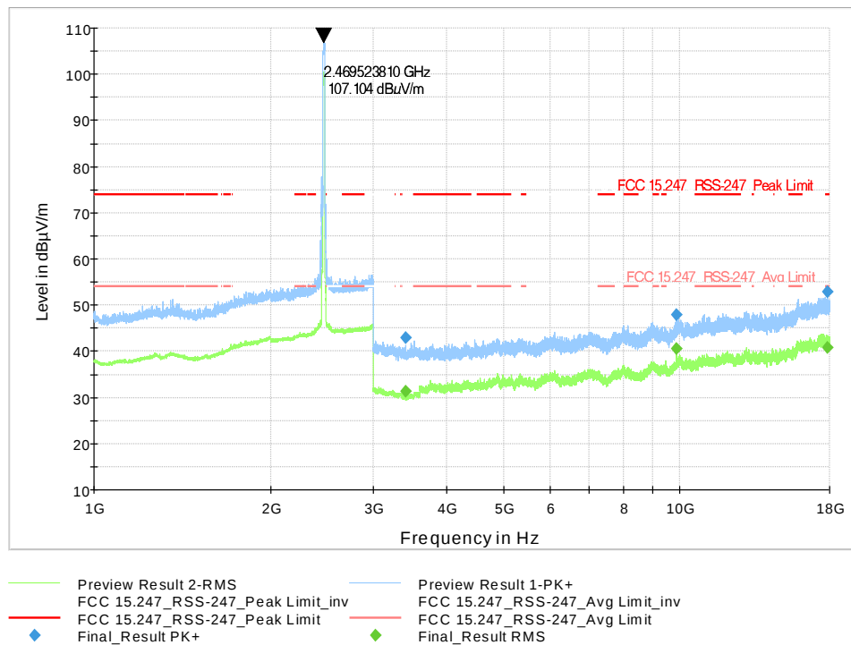
Figure 9-335 Radiated Spurious Emission 1-18GHz 802.11n20- Ch.12
