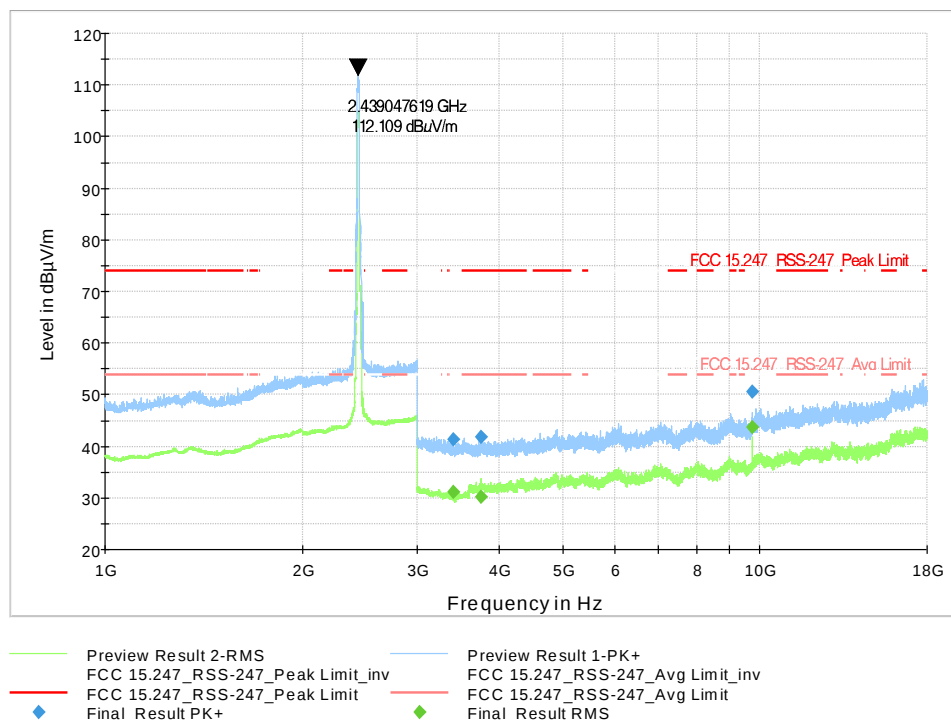
Figure 9-333 Radiated Spurious Emission 1-18GHz 802.11n20- Ch.6
