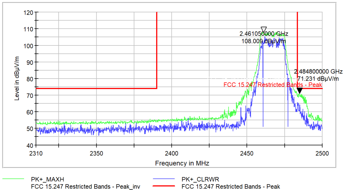
Figure 9-356 Radiated Band Edge Peak 802.11g- Ch.12
