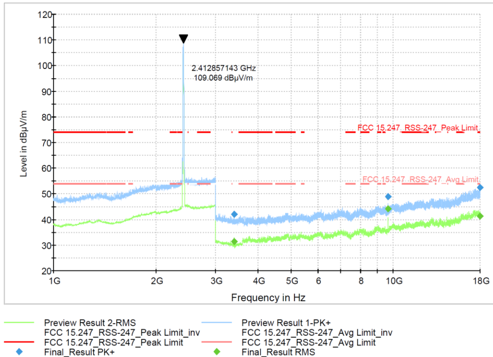
Figure 9-322 Radiated Spurious Emission 1-18GHz 802.11b - Ch.1
