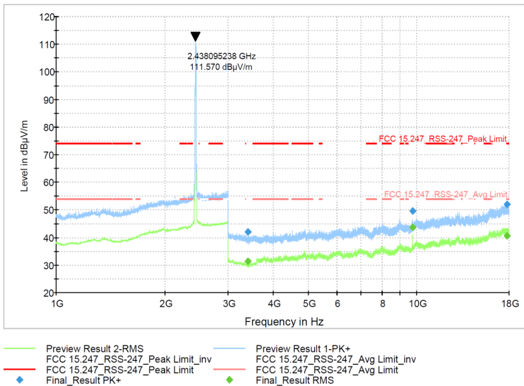
Figure 9-323 Radiated Spurious Emission 1-18GHz 802.11b - Ch.6
