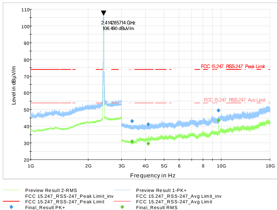
Figure 9-332 Radiated Spurious Emission 1-18GHz 802.11n20 - Ch.1
