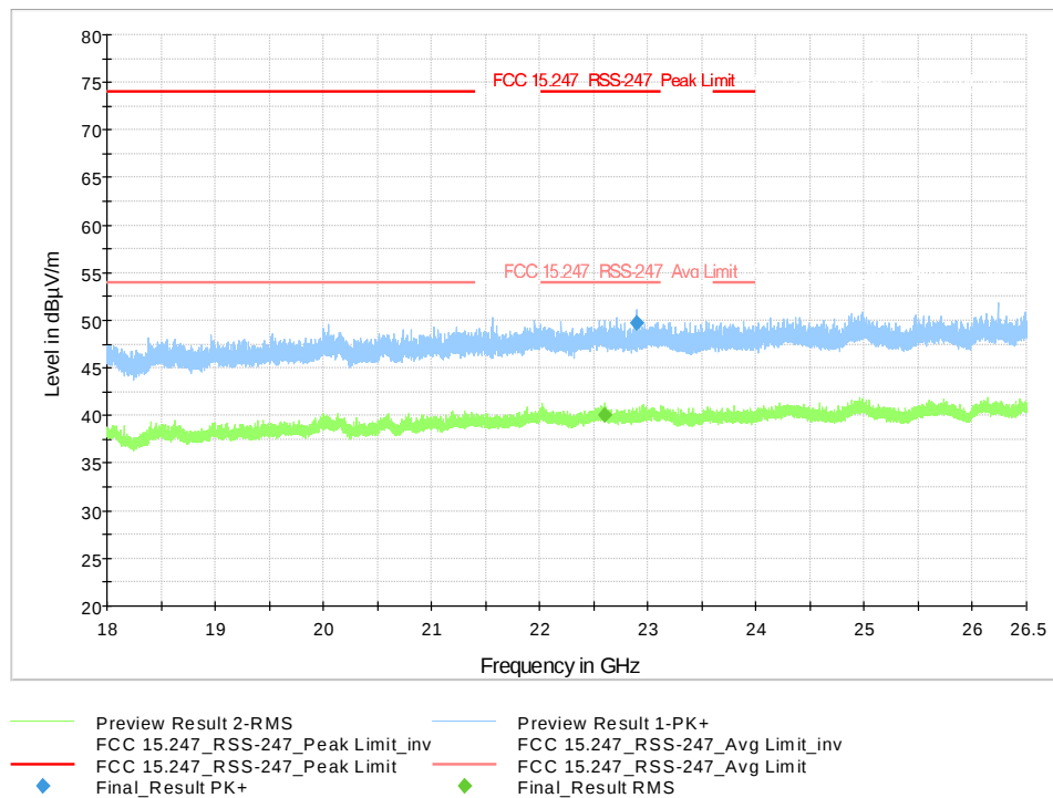
Figure 9-343 Radiated Spurious Emissions 18-26.5GHz 802.11n40 - Ch.3
