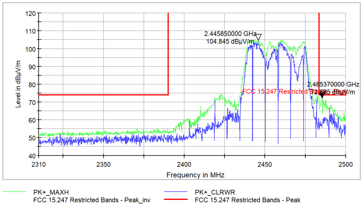
Figure 9-372 Radiated Band Edge Peak 802.11n40- Ch.10
