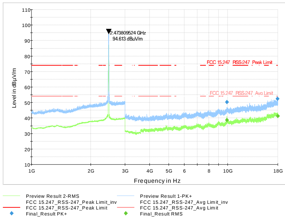
Figure 9-336 Radiated Spurious Emission 1-18GHz 802.11n20- Ch.13
