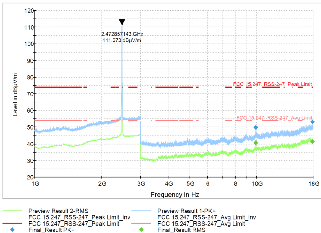
Figure 9-326 Radiated Spurious Emission 1-18GHz 802.11b - Ch.13
