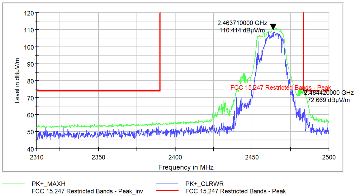
Figure 9-362 Radiated Band Edge Peak 802.11n20- Ch.11
