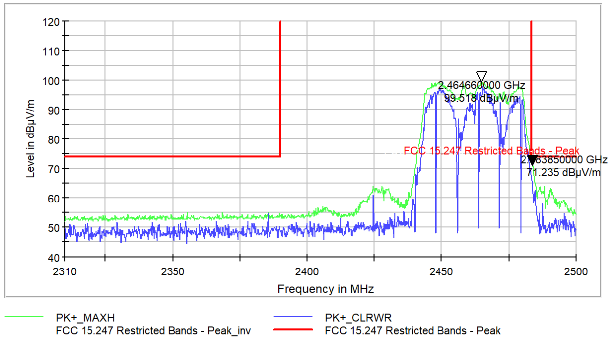
Figure 9-374 Radiated Band Edge Peak 802.11n40- Ch.11
