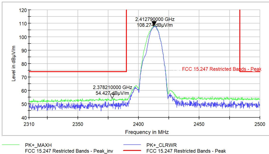
Figure 9-344 Radiated Band Edge Peak 802.11b - Ch.1
