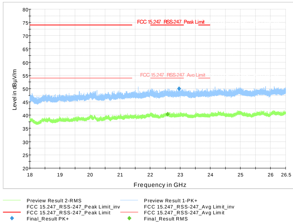
Figure 9-342 Radiated Spurious Emissions 18-26.5GHz 802.11n20 - Ch.11
