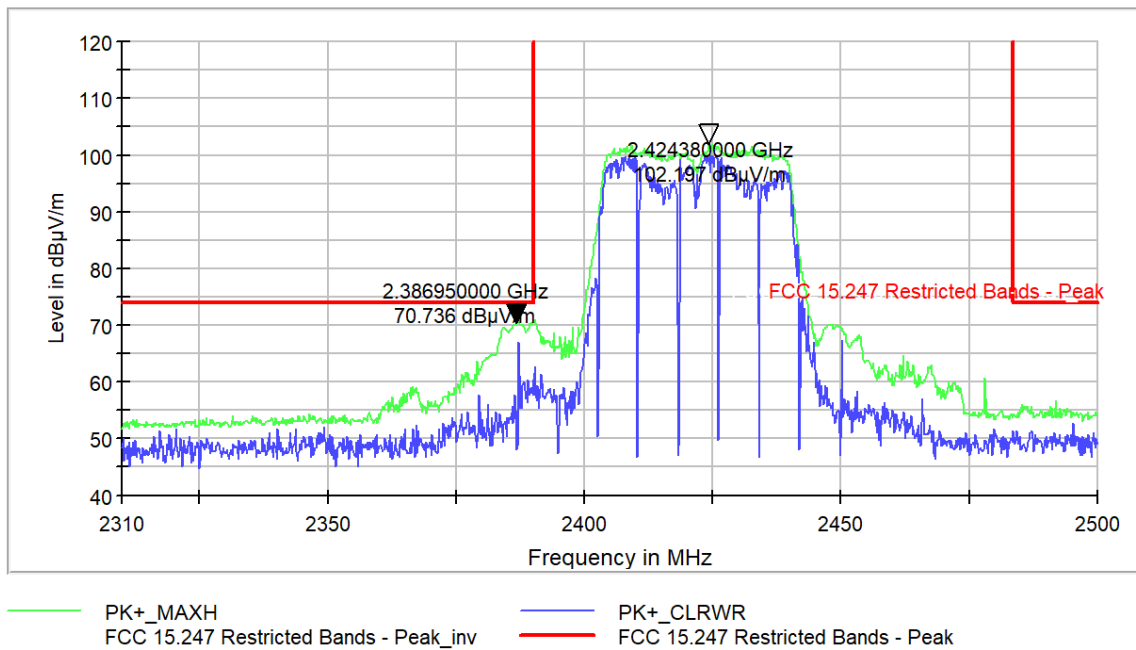
Figure 9-368 Radiated Band Edge Peak 802.11n40 – Ch3
