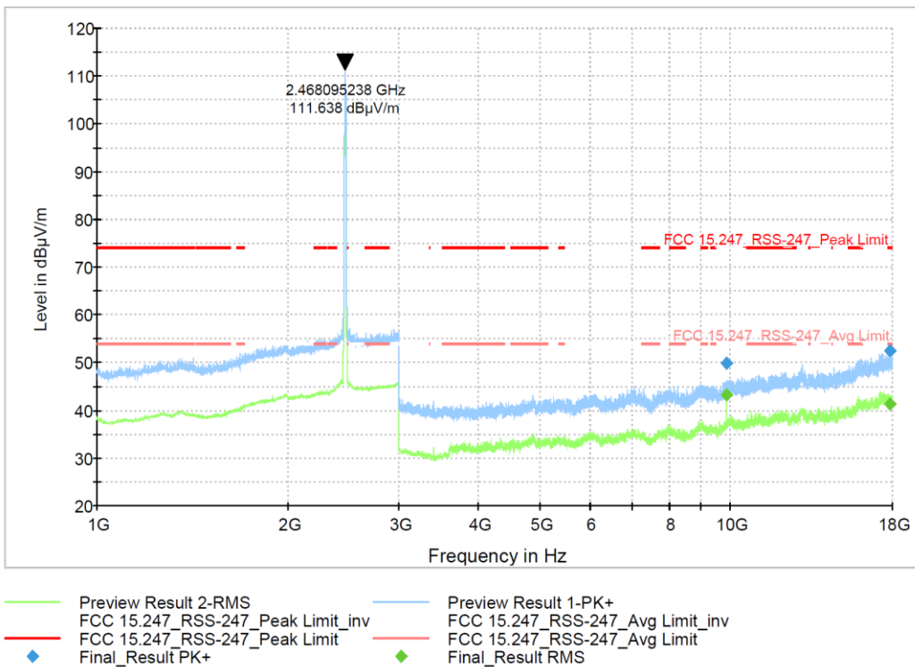
Figure 9-325 Radiated Spurious Emission 1-18GHz 802.11b - Ch.12
