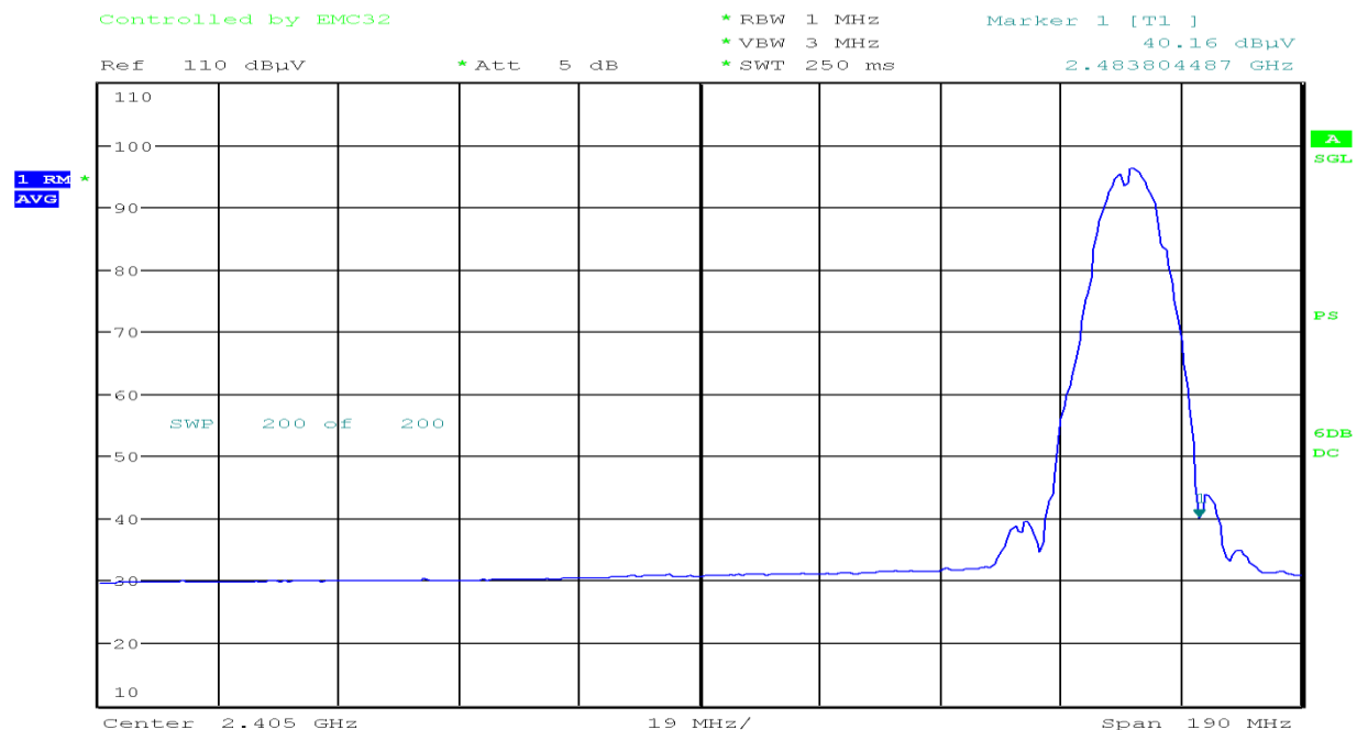
Figure 9-351 Radiated Band Edge Average 802.11b - Ch.13
