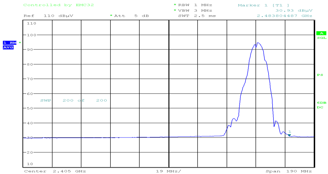
Figure 9-347 Radiated Band Edge Average 802.11b - Ch.11
