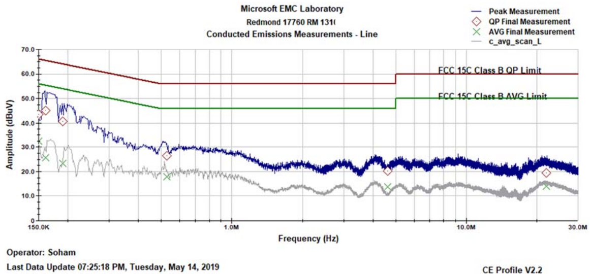
Figure 9-67 AC Line Conducted Emissions- Line (150 kHz- 30 MHz)
