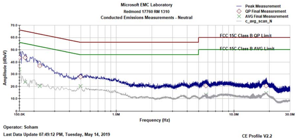
Figure 9-68 AC Line Conducted Emissions- Neutral (150 kHz- 30 MHz)
