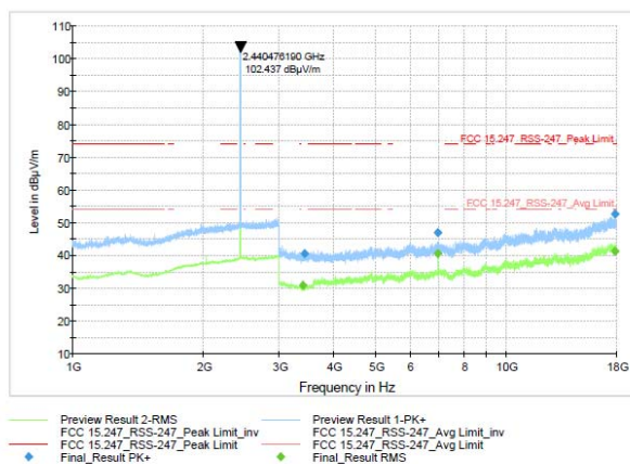
Figure 9-60 Radiated Spurious Emissions 1-18 GHz (Ch. 19) BW 2-MHz
