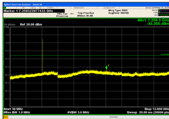
Figure 9-4321 Conducted Spurious Emissions 30-12000 MHz (Ch.39) 1MHz BW
