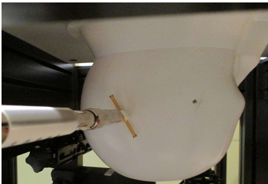
2.4 GHz Dipole Placed at Location A in 90° Orientation (10mm Spacer)
