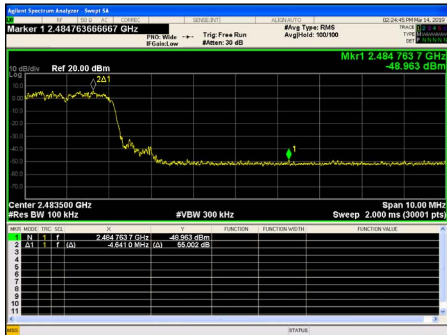
Figure 9-41 High Channel Band 3-DH5 Mode (Hopping enabled)
