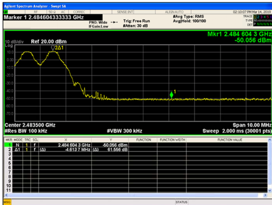
Figure 9-39 High Channel Band 1-DH5 Mode (Hopping enabled)
