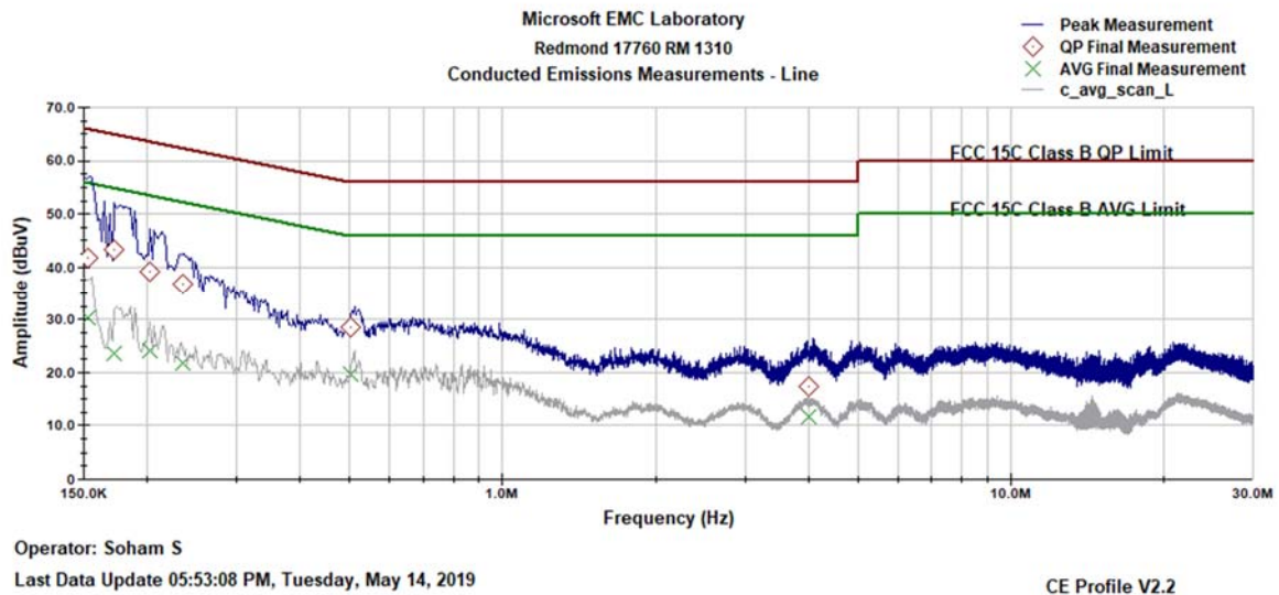
Figure 9-83 AC Line Conducted Emissions- Line (150 kHz- 30 MHz)
