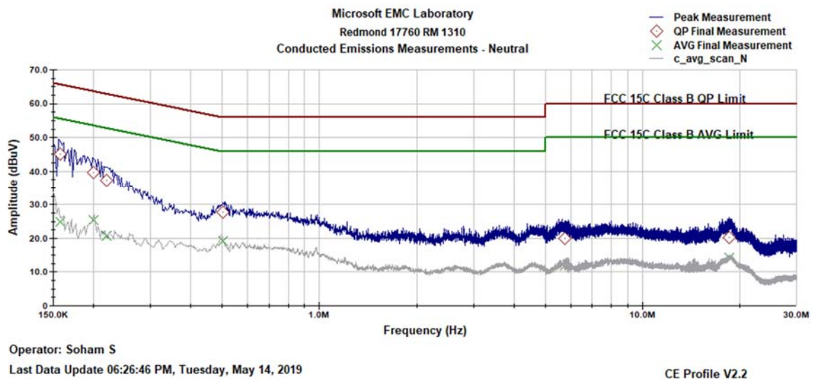
Figure 9-84 AC Line Conducted Emissions- Neutral (150 kHz- 30 MHz)
