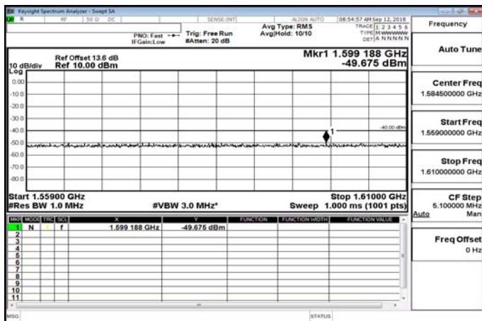
1559MHz~1610MHz_Band13_10MHz_QPSK_1_0_MidCH23230-782
