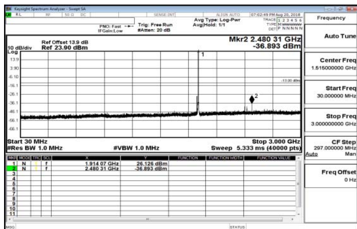
30MHz~3GHz_Band25_1_4MHz_QPSK_1_0_HighCH26683-1914.3
