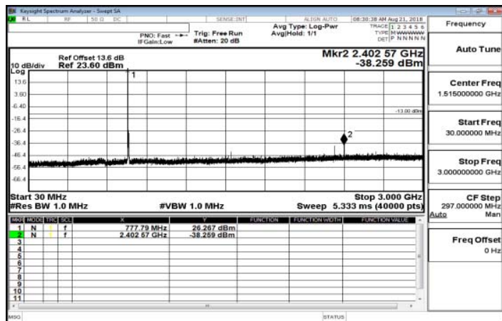
30MHz~3GHz_Band13_10MHz_QPSK_1_0_MidCH23230-782
