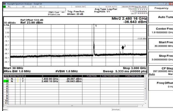
30MHz~3GHz_Band25_10MHz_QPSK_1_0_LowCH26090-1855
