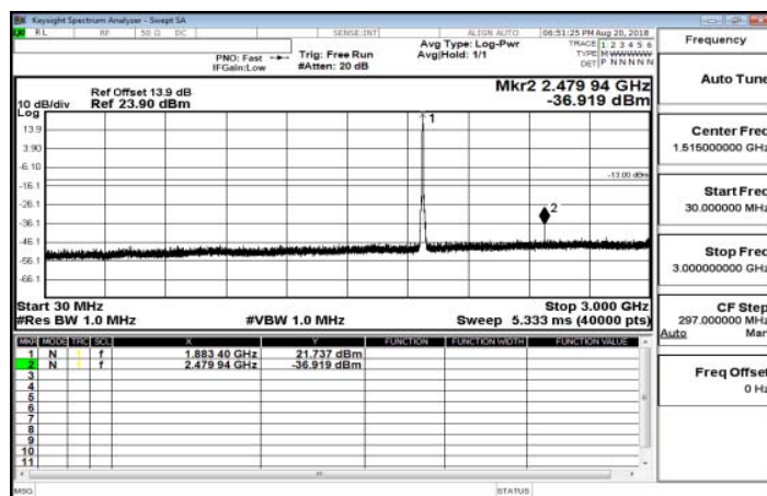
30MHz~3GHz_Band25_3MHz_QPSK_1_0_MidCH26365-1882.5
