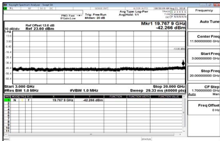
3GHz~20GHz_Band26_5MHz_QPSK_1_0_LowCH26815
