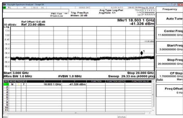
3GHz-20GHz_Band12_5MHz_QPSK_1_0_LowCH23035-701.5
