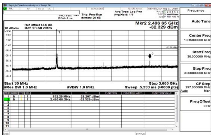
30MHz~3GHz_Band26_10MHz_QPSK_1_0_MidCH26915
