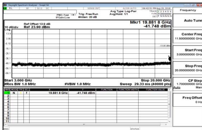
3GHz~20GHz_Band25_5MHz_QPSK_1_0_LowCH26065-1852.5
