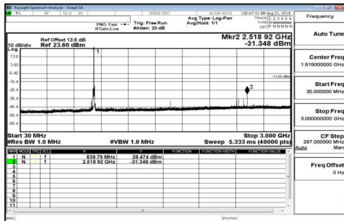
30MHz~3GHz_Band26_10MHz_QPSK_1_0_HighCH26990
