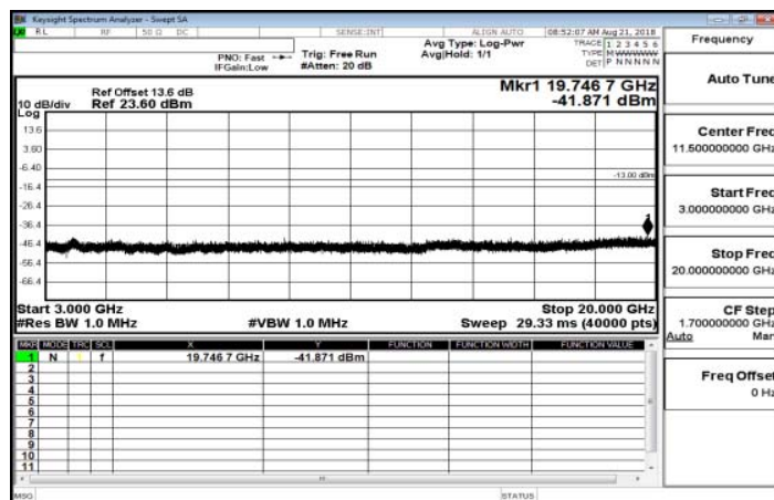
3GHz~20GHz_Band26_5MHz_QPSK_1_0_HighCH27015
