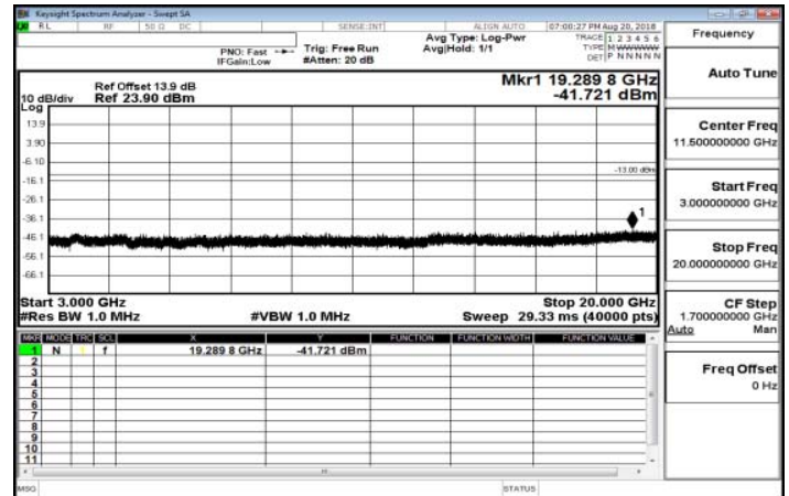
3GHz~20GHz_Band25_1_4MHz_QPSK_1_0_LowCH26047-1850.7
