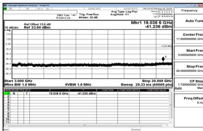
3GHz~20GHz_Band12_1_4MHz_QPSK_1_0_HighCH23173-715.3
