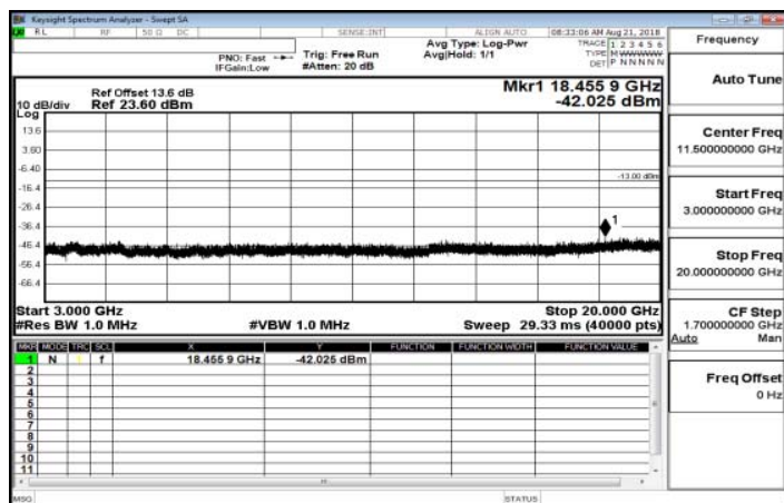
3GHz~20GHz_Band13_10MHz_QPSK_1_0_MidCH23230-782
