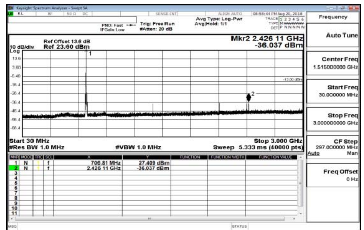
30MHz~3GHz_Band12_10MHz_QPSK_1_0_HighCH23130-711
