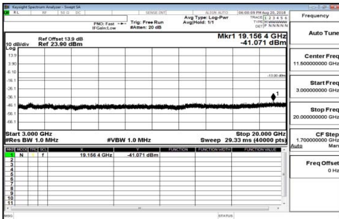
3GHz~20GHz_Band25_20MHz_QPSK_1_0_HighCH26590-1905
