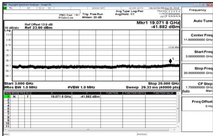
3GHz~20GHz_Band25_5MHz_QPSK_1_0_MidCH26365-1882.5
