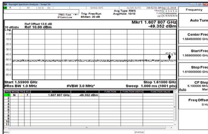
1559MHz~1610MHz_Band13_5MHz_QPSK_1_0_LowCH23205-779.5
