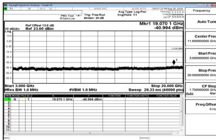
3GHz-20GHz_Band12_3MHz_QPSK_1_0_HighCH23165-714.5
