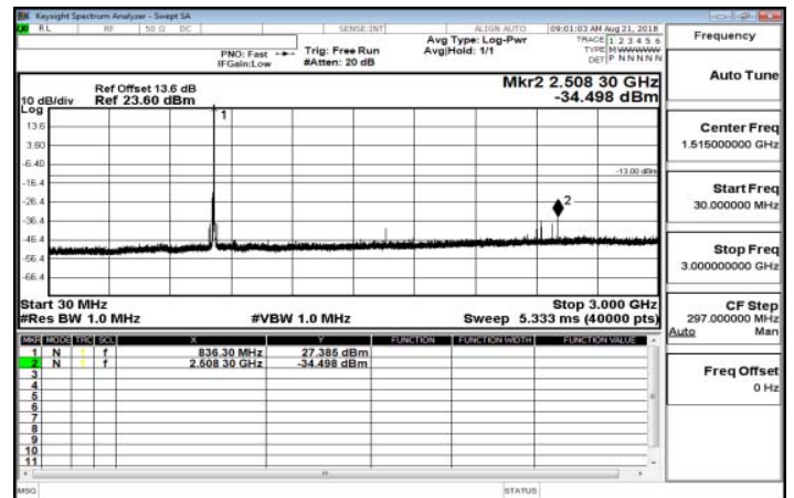
30MHz~3GHz_Band26_1_4MHz_QPSK_1_0_MidCH26915
