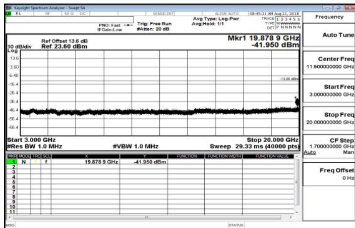
3GHz~20GHz_Band26_10MHz_QPSK_1_0_LowCH26840
