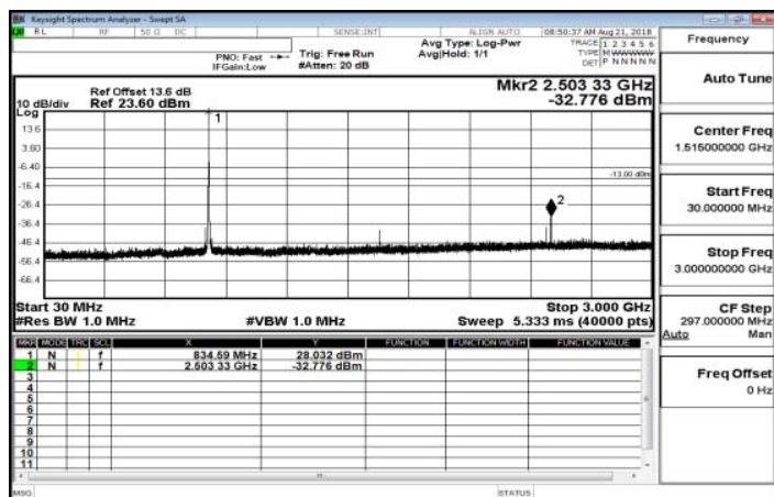
30MHz~3GHz_Band26_5MHz_QPSK_1_0_MidCH26915
