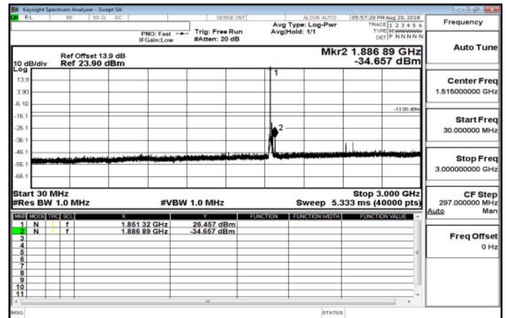
30MHz~3GHz_Band25_20MHz_QPSK_1_0_LowCH26140-1860
