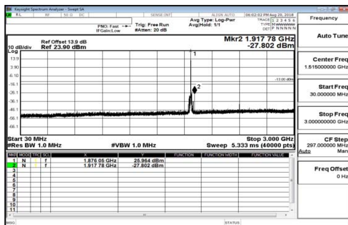
30MHz~3GHz_Band25_15MHz_QPSK_1_0_MidCH26365-1882.5
