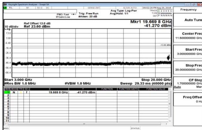
3GHz-20GHz_Band12_5MHz_QPSK_1_0_MidCH23095-707.5
