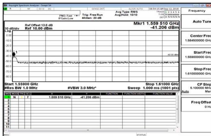
1559MHz~1610MHz_Band13_5MHz_QPSK_1_0_MidCH23230-782
