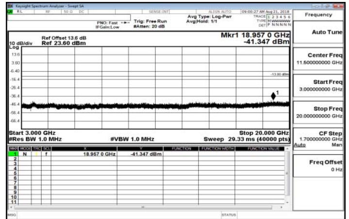
3GHz~20GHz_Band26_1_4MHz_QPSK_1_0_LowCH26797
