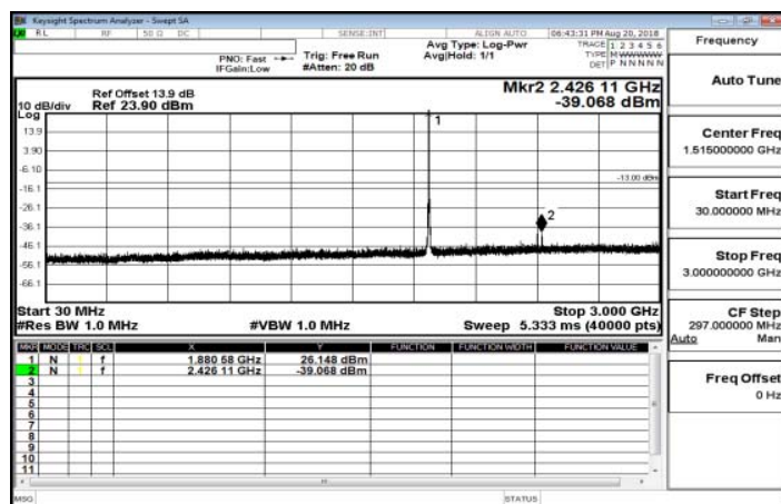
30MHz~3GHz_Band25_5MHz_QPSK_1_0_MidCH26365-1882.5
