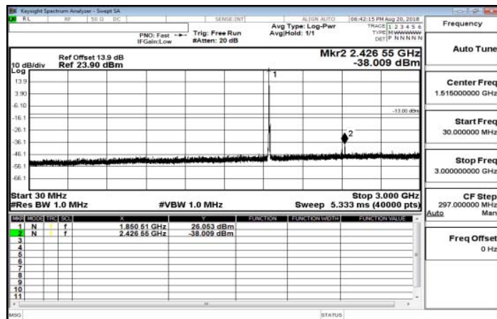
30MHz~3GHz_Band25_5MHz_QPSK_1_0_LowCH26065-1852.5
