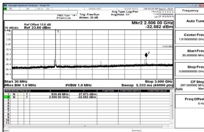
30MHz~3GHz_Band26_3MHz_QPSK_1_0_MidCH26915
