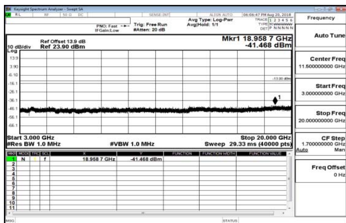
3GHz~20GHz_Band25_10MHz_QPSK_1_0_HighCH26640-1910
