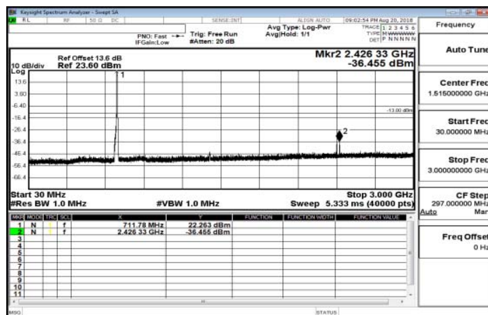
30MHz-3GHz_Band12_5MHz_QPSK_1_0_HighCH23155-713.5
