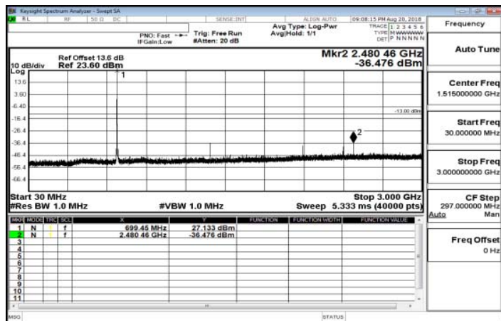
30MHz~3GHz_Band12_1_4MHz_QPSK_1_0_LowCH23017-699.7
