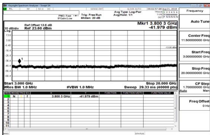
3GHz~20GHz_Band26_1_4MHz_QPSK_1_0_HighCH27033
