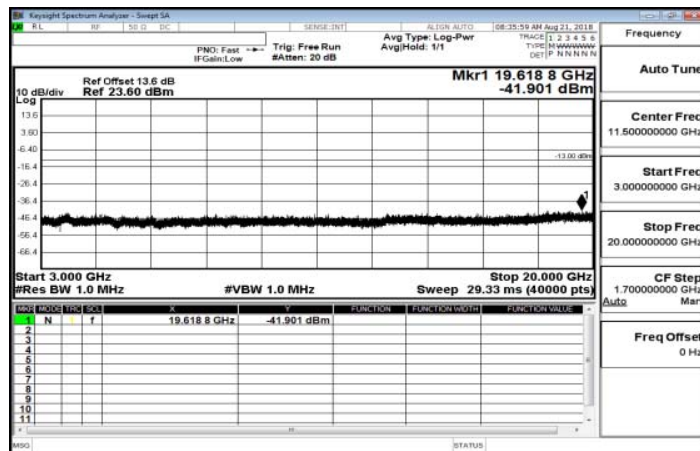
3GHz~20GHz_Band13_5MHz_QPSK_1_0_MidCH23230-782
