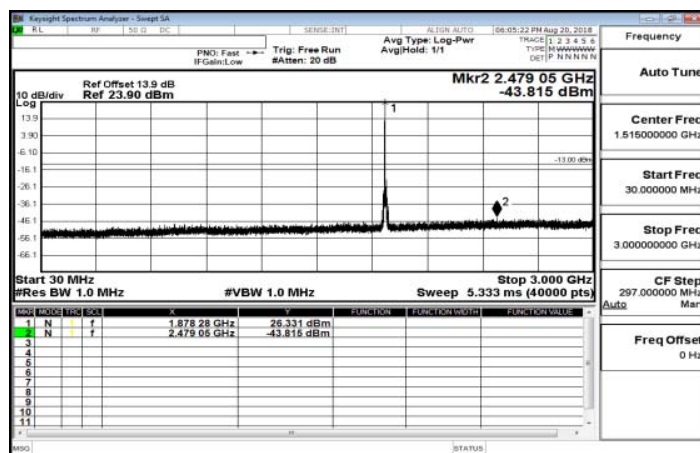
30MHz~3GHz_Band25_10MHz_QPSK_1_0_MidCH26365-1882.5
