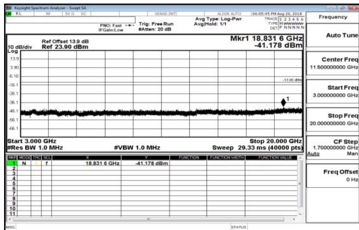
3GHz~20GHz_Band25_10MHz_QPSK_1_0_MidCH26365-1882.5
