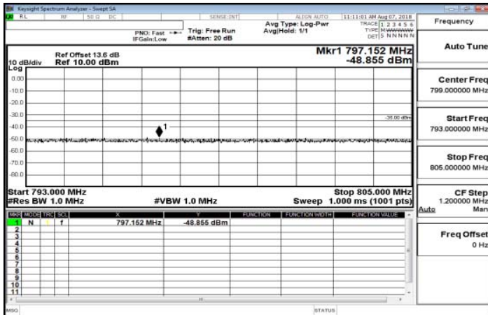
793MHz~806MHz_Band13_10MHz_QPSK_1_0_MidCH23230-782
