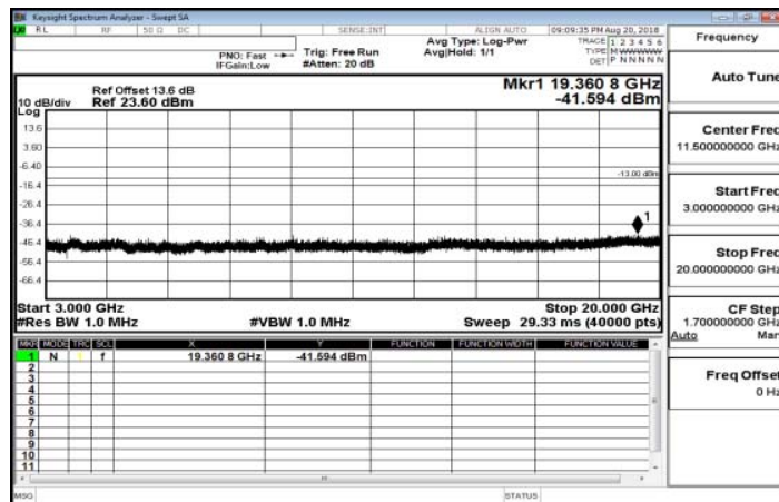
3GHz~20GHz_Band12_1_4MHz_QPSK_1_0_MidCH23095-707.5
