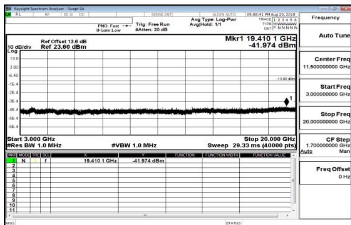
3GHz~20GHz_Band12_1_4MHz_QPSK_1_0_LowCH23017-699.7
