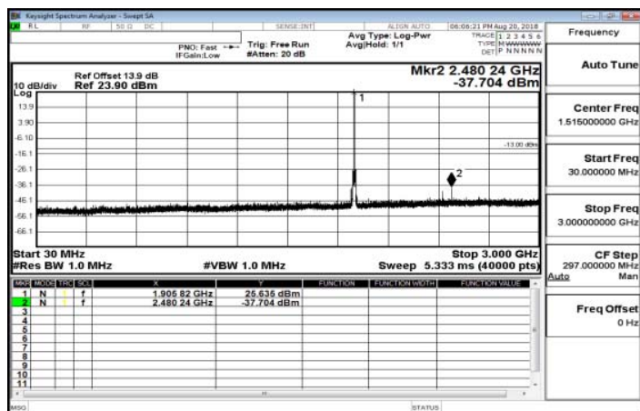
30MHz~3GHz_Band25_10MHz_QPSK_1_0_HighCH26640-1910
