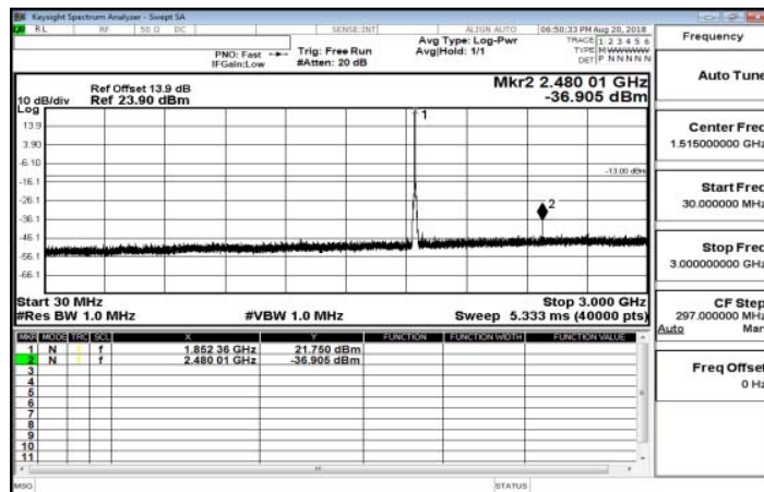
30MHz~3GHz_Band25_3MHz_QPSK_1_0_LowCH26055-1851.5
