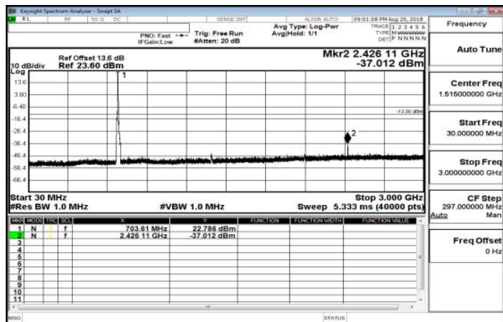
30MHz-3GHz_Band12_5MHz_QPSK_1_0_LowCH23035-701.5
