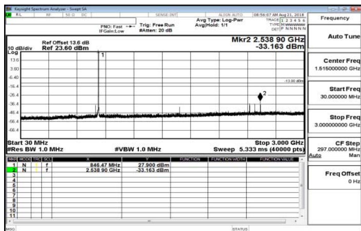
30MHz~3GHz_Band26_3MHz_QPSK_1_0_HighCH27025
