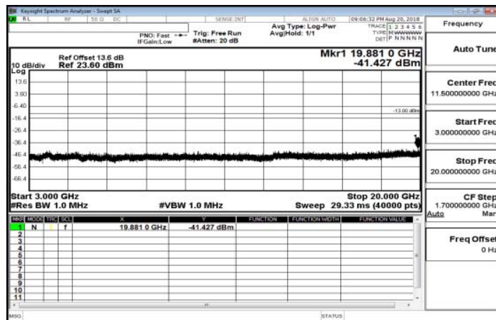
3GHz-20GHz_Band12_3MHz_QPSK_1_0_MidCH23095-707.5
