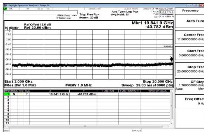
3GHz-20GHz_Band12_5MHz_QPSK_1_0_HighCH23155-713.5
