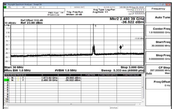
30MHz~3GHz_Band25_20MHz_QPSK_1_0_MidCH26365-1882.5
