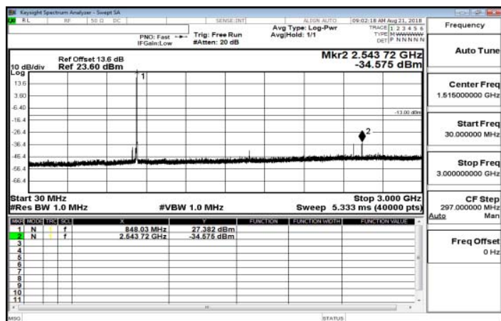
30MHz~3GHz_Band26_1_4MHz_QPSK_1_0_HighCH27033
