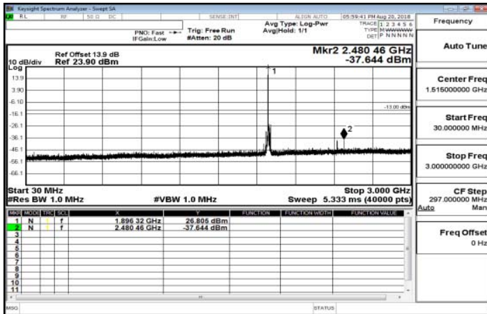
30MHz~3GHz_Band25_20MHz_QPSK_1_0_HighCH26590-1905
