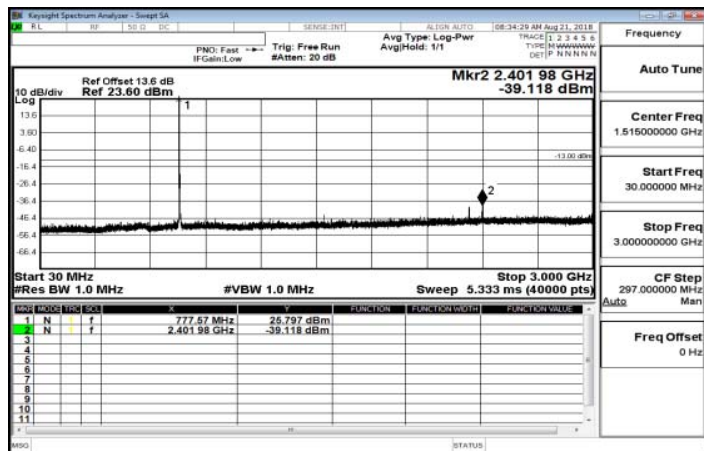
30MHz~3GHz_Band13_5MHz_QPSK_1_0_LowCH23205-779.5
