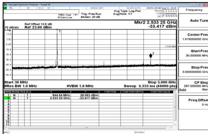
30MHz~3GHz_Band26_5MHz_QPSK_1_0_HighCH27015
