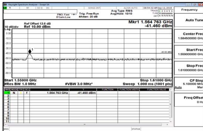
1559MHz~1610MHz_Band13_5MHz_QPSK_1_0_HighCH23255-784.5
