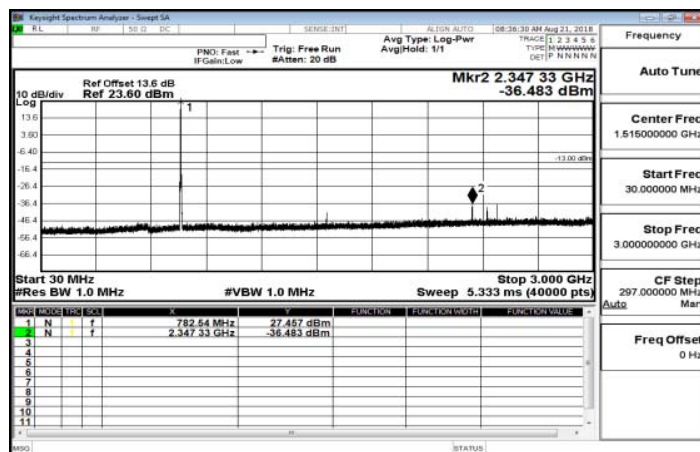
30MHz~3GHz_Band13_5MHz_QPSK_1_0_HighCH23255-784.5
