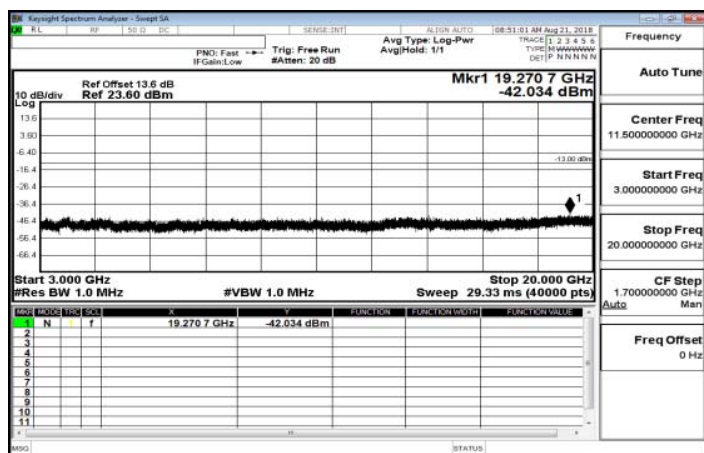
3GHz~20GHz_Band26_5MHz_QPSK_1_0_MidCH26915
