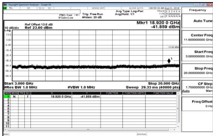
3GHz~20GHz_Band26_3MHz_QPSK_1_0_MidCH26915
