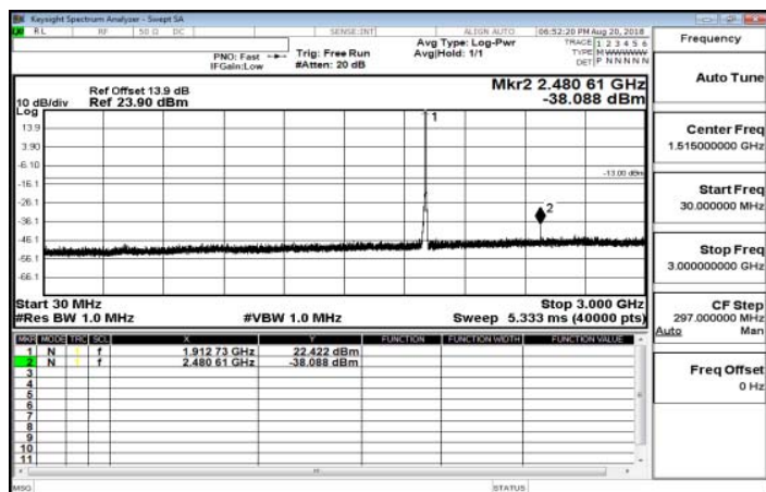
30MHz~3GHz_Band25_3MHz_QPSK_1_0_HighCH26675-1913.5
