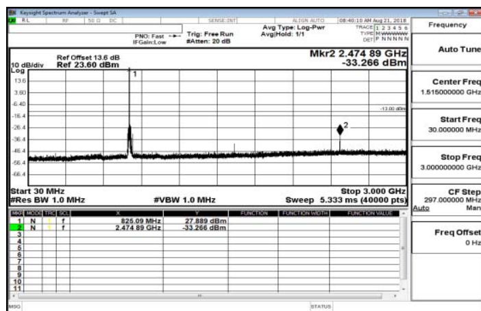
30MHz~3GHz_Band26_15MHz_QPSK_1_0_LowCH26865
