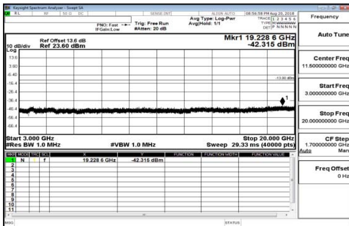
3GHz~20GHz_Band12_10MHz_QPSK_1_0_LowCH23060-704
