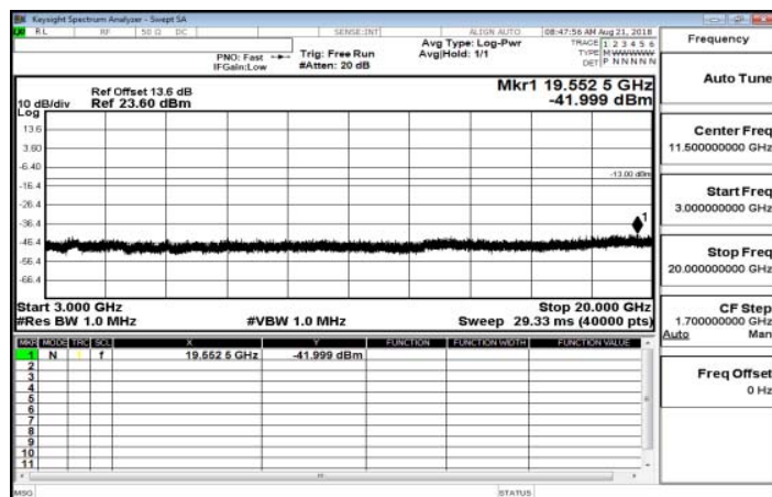
3GHz~20GHz_Band26_10MHz_QPSK_1_0_HighCH26990
