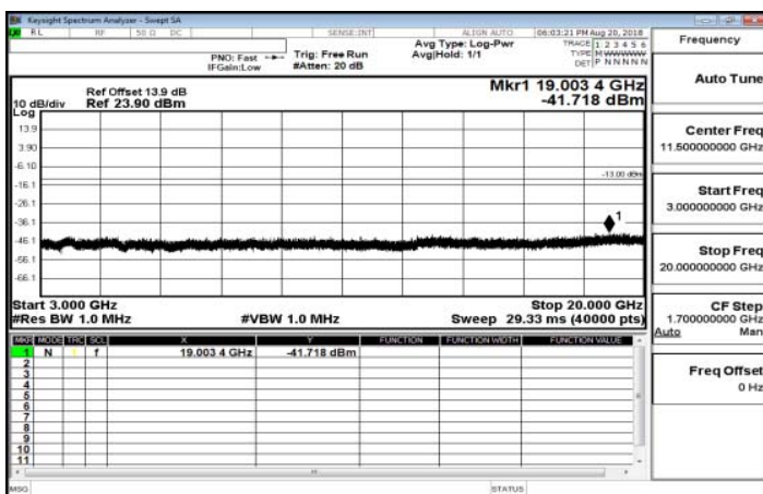
3GHz~20GHz_Band25_15MHz_QPSK_1_0_HighCH26615-1907.5
