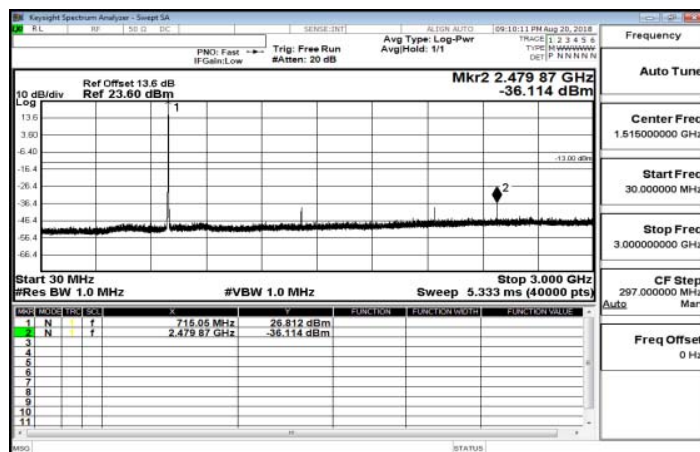
30MHz~3GHz_Band12_1_4MHz_QPSK_1_0_HighCH23173-715.3
