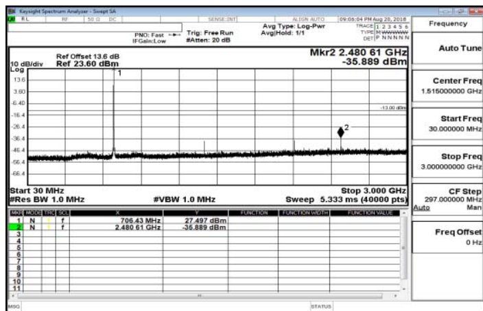
30MHz-3GHz_Band12_3MHz_QPSK_1_0_MidCH23095-707.5
