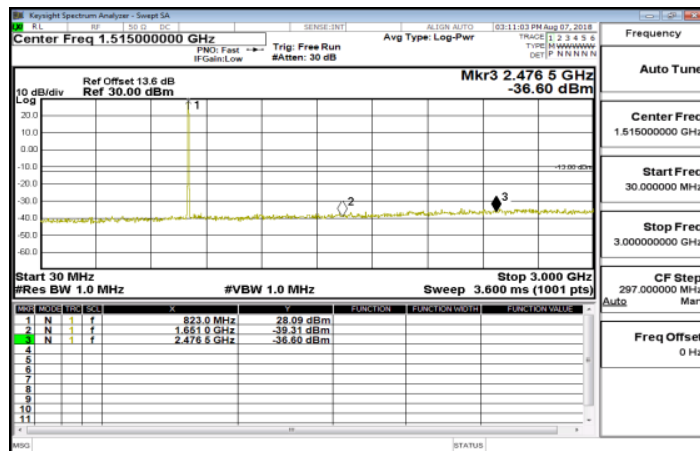
30MHz~3GHz_Band26_5MHz_QPSK_1_0_LowCH26805
