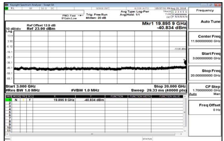
3GHz~20GHz_Band25_20MHz_QPSK_1_0_LowCH26140-1860
