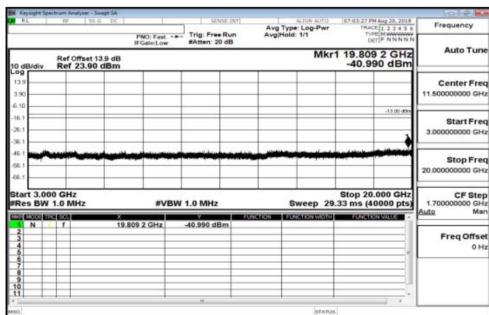
3GHz~20GHz_Band25_1_4MHz_QPSK_1_0_HighCH26683-1914.3
