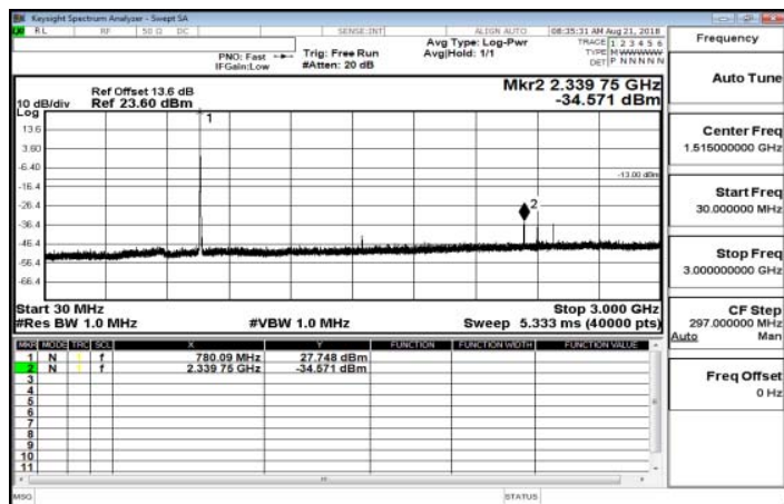
30MHz~3GHz_Band13_5MHz_QPSK_1_0_MidCH23230-782
