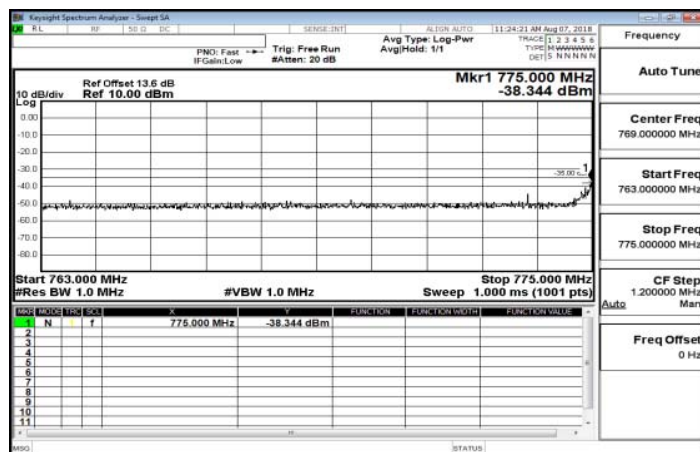
763.3MHz~775MHz_Band13_5MHz_QPSK_1_0_MidCH23230-782
