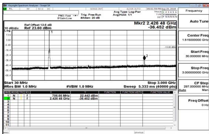
30MHz-3GHz_Band12_5MHz_QPSK_1_0_MidCH23095-707.5
