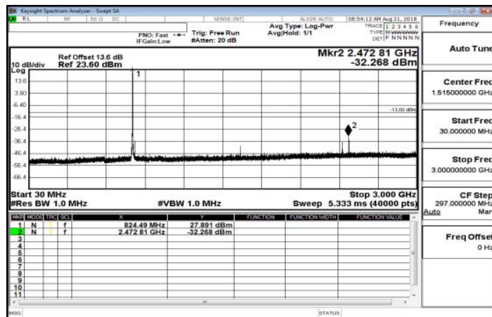
30MHz~3GHz_Band26_3MHz_QPSK_1_0_LowCH26805
