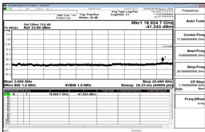
3GHz~20GHz_Band26_3MHz_QPSK_1_0_HighCH27025
