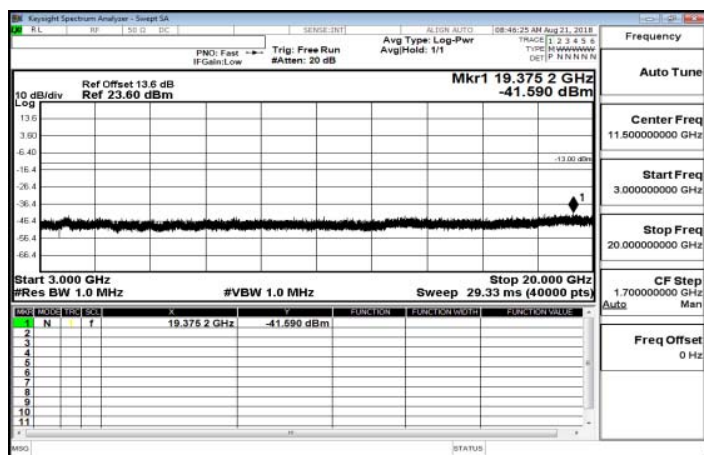
3GHz~20GHz_Band26_10MHz_QPSK_1_0_MidCH26915
