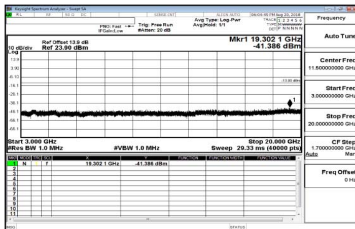
3GHz~20GHz_Band25_10MHz_QPSK_1_0_LowCH26090-1855
