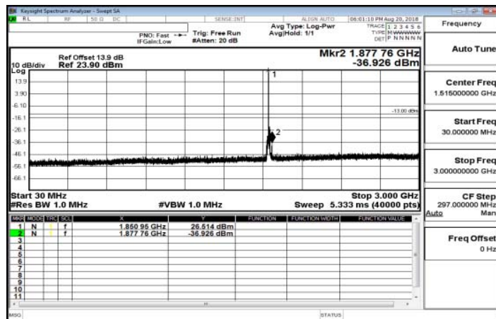
30MHz~3GHz_Band25_15MHz_QPSK_1_0_LowCH26115-1857.5
