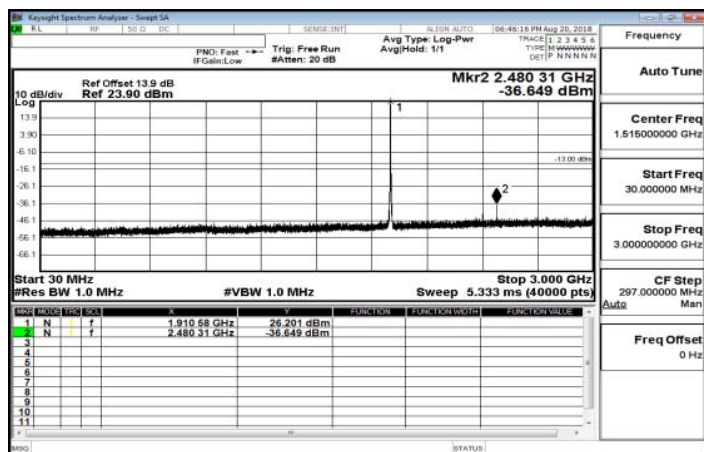
30MHz~3GHz_Band25_5MHz_QPSK_1_0_HighCH26665-1912.5
