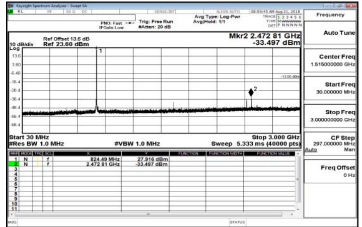
30MHz~3GHz_Band26_1_4MHz_QPSK_1_0_LowCH26797
