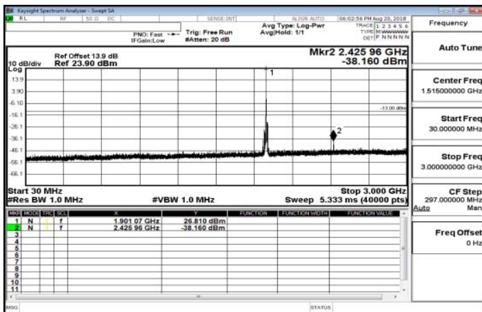
30MHz~3GHz_Band25_15MHz_QPSK_1_0_HighCH26615-1907.5
