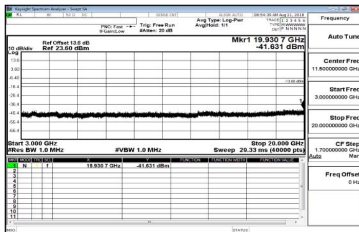
3GHz~20GHz_Band26_3MHz_QPSK_1_0_LowCH26805
