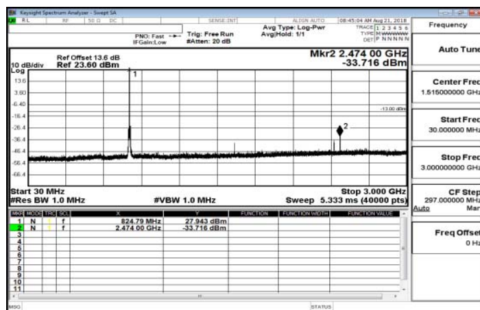
30MHz~3GHz_Band26_10MHz_QPSK_1_0_LowCH26840
