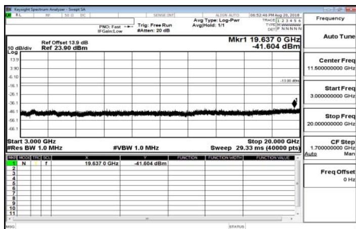
3GHz~20GHz_Band25_3MHz_QPSK_1_0_HighCH26675-1913.5
