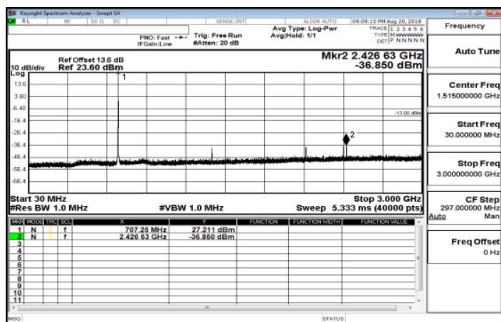
30MHz~3GHz_Band12_1_4MHz_QPSK_1_0_MidCH23095-707.5
