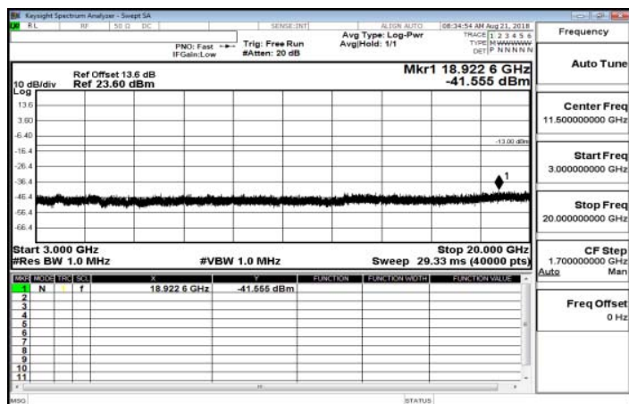
3GHz~20GHz_Band13_5MHz_QPSK_1_0_LowCH23205-779.5
