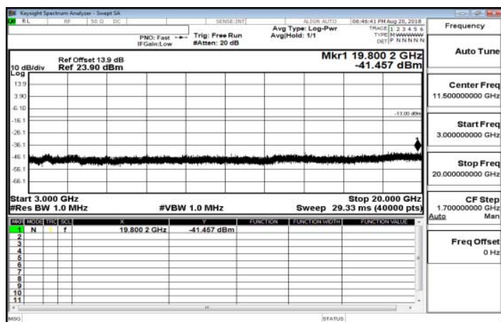
3GHz~20GHz_Band25_5MHz_QPSK_1_0_HighCH26665-1912.5
