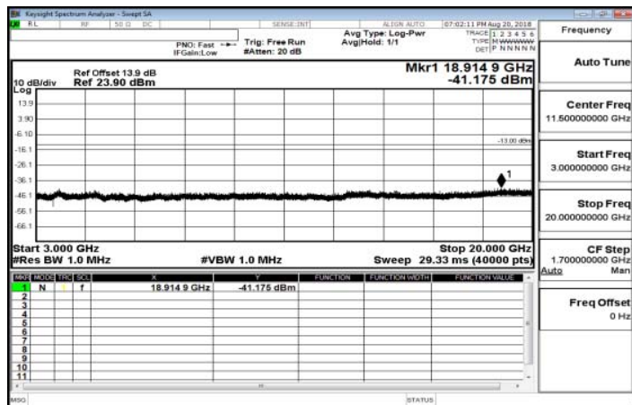
3GHz~20GHz_Band25_1_4MHz_QPSK_1_0_MidCH26365-1882.5
