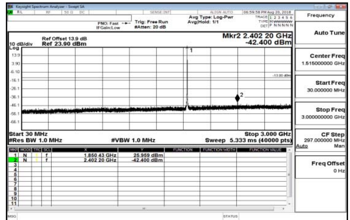
30MHz~3GHz_Band25_1_4MHz_QPSK_1_0_LowCH26047-1850.7
