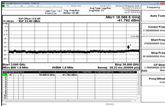
3GHz~20GHz_Band25_15MHz_QPSK_1_0_MidCH26365-1882.5
