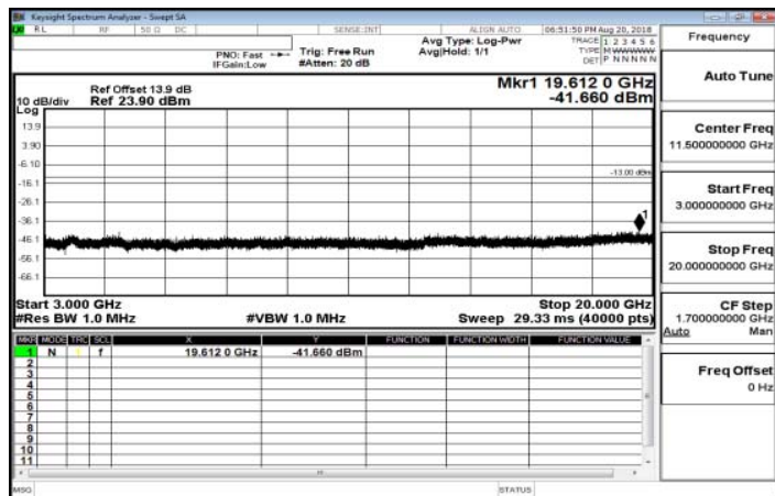
3GHz~20GHz_Band25_3MHz_QPSK_1_0_MidCH26365-1882.5
