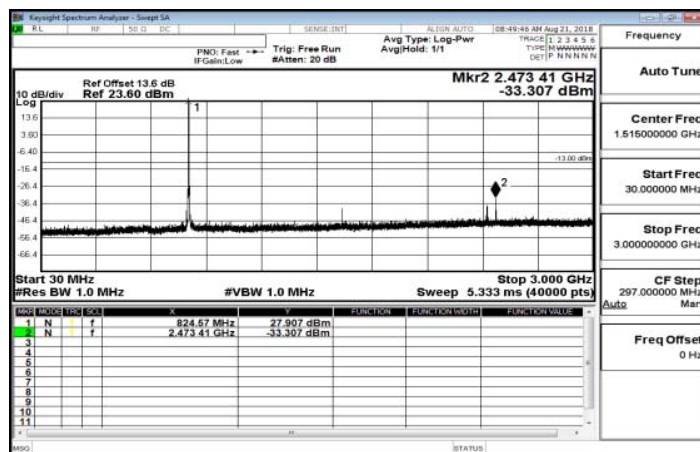
30MHz~3GHz_Band26_5MHz_QPSK_1_0_LowCH26815
