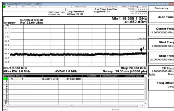
3GHz~20GHz_Band26_1_4MHz_QPSK_1_0_MidCH26915
