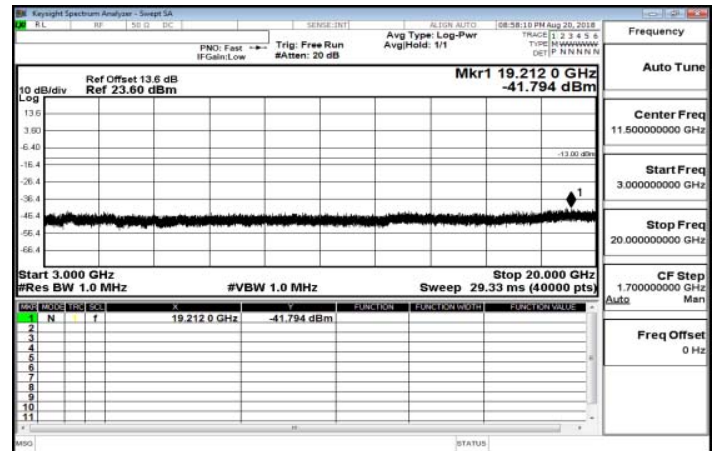
3GHz~20GHz_Band12_10MHz_QPSK_1_0_MidCH23095-707.5
