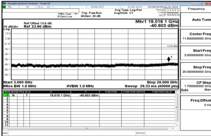
3GHz~20GHz_Band25_20MHz_QPSK_1_0_MidCH26365-1882.5
