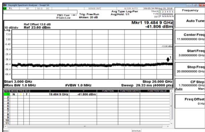
3GHz-20GHz_Band12_3MHz_QPSK_1_0_LowCH23025-700.5
