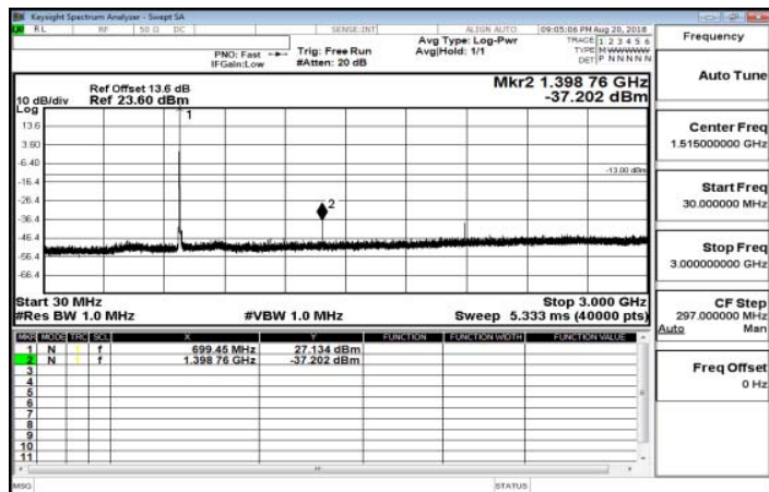
30MHz-3GHz_Band12_3MHz_QPSK_1_0_LowCH23025-700.5
