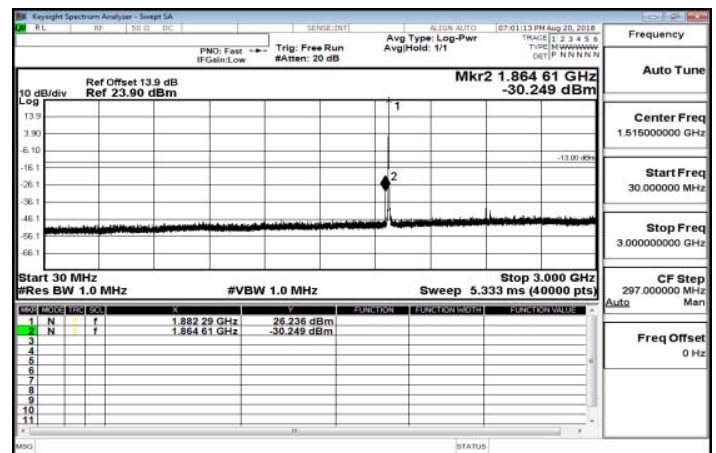
30MHz~3GHz_Band25_1_4MHz_QPSK_1_0_MidCH26365-1882.5
