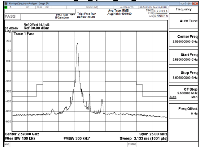
Band 41 5M QPSK MID RB1,24
