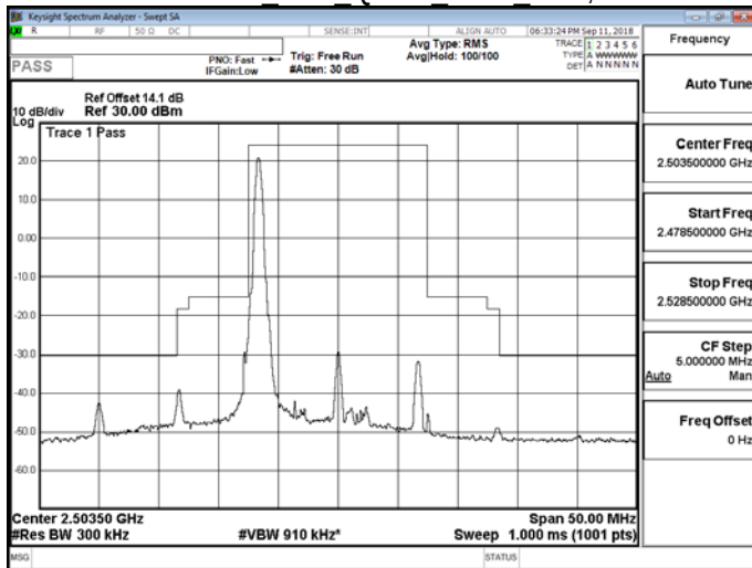
Band 41 15M QPSK LOW RB1,74
