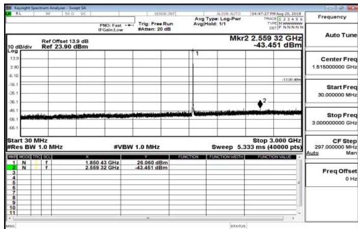
30MHz~3GHz_Band2_1_4MHz_QPSK_1_0_LowCH18607-1850.7
