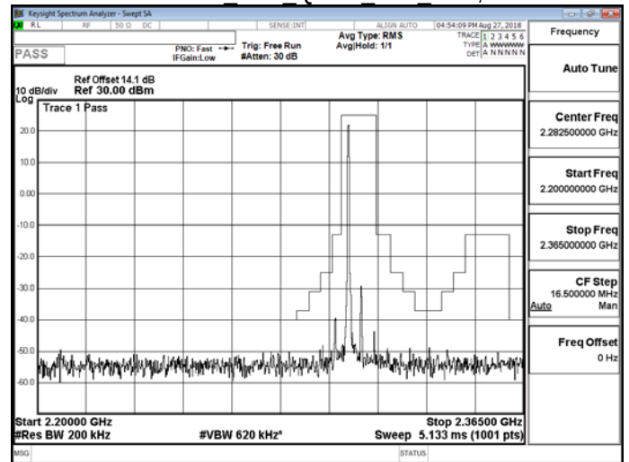
Band 30 10M QPSK MID RB1,49
