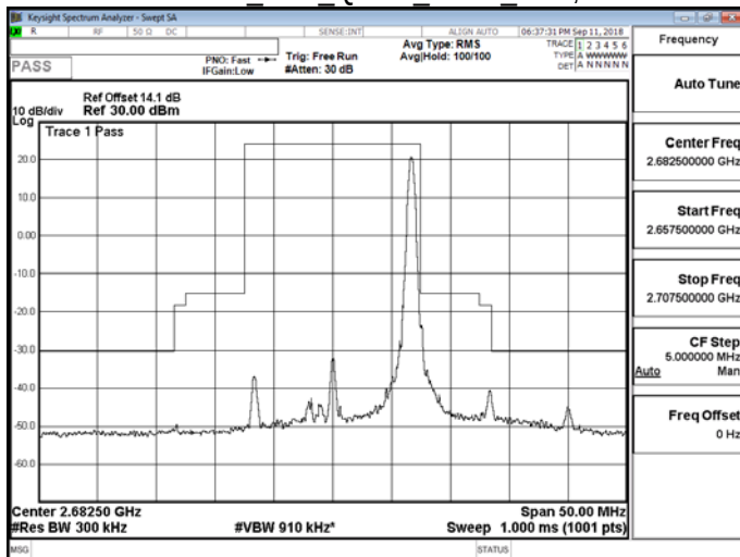
Band 41 15M QPSK HIGH RB75,0
