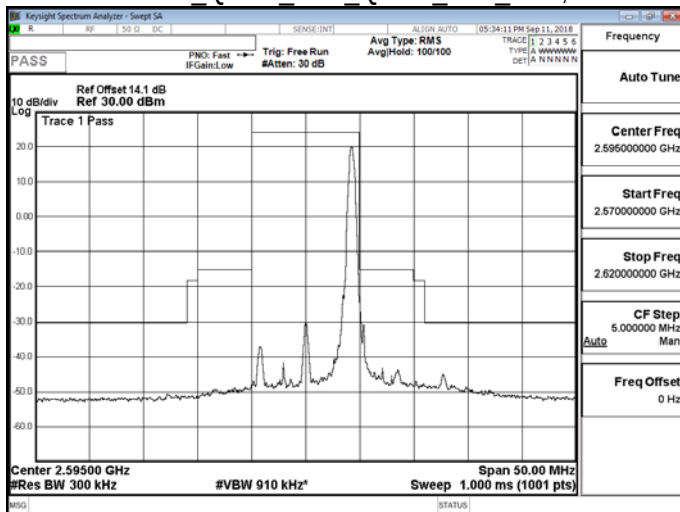
Band 38 QPSK 10M QPSK MID RB50,0
