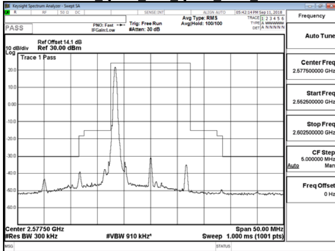
Band 38 QPSK 15M QPSK LOW RB1,74
