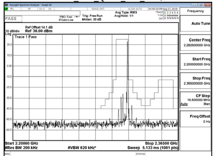
Band 30 10M QPSK MID RB50,0
