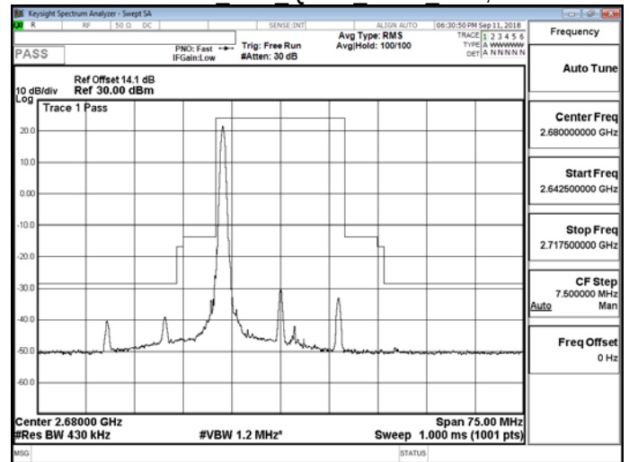
Band 41 20M QPSK HIGH RB1,99
