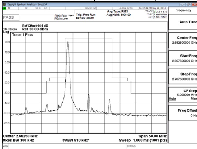
Band 41 15M QPSK HIGH RB1,74
