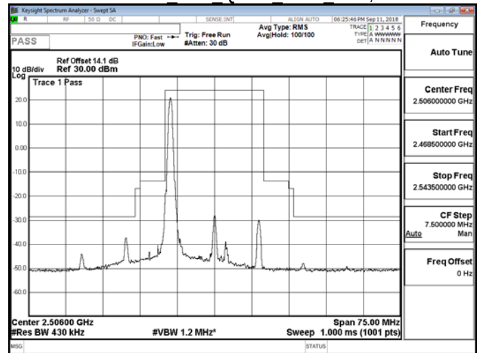
Band 41 20M QPSK LOW RB1,99
