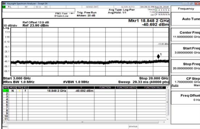
3GHz~20GHz_Band2_3MHz_QPSK_1_0_LowCH18615-1851.5
