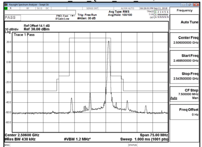
Band 41 20M QPSK LOW RB100,0
