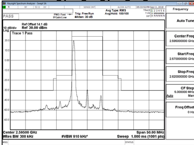
Band 38 QPSK 10M QPSK MID RB1,49
