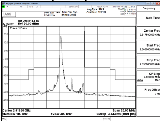
Band 38 QPSK 5M QPSK HIGH RB1,24
