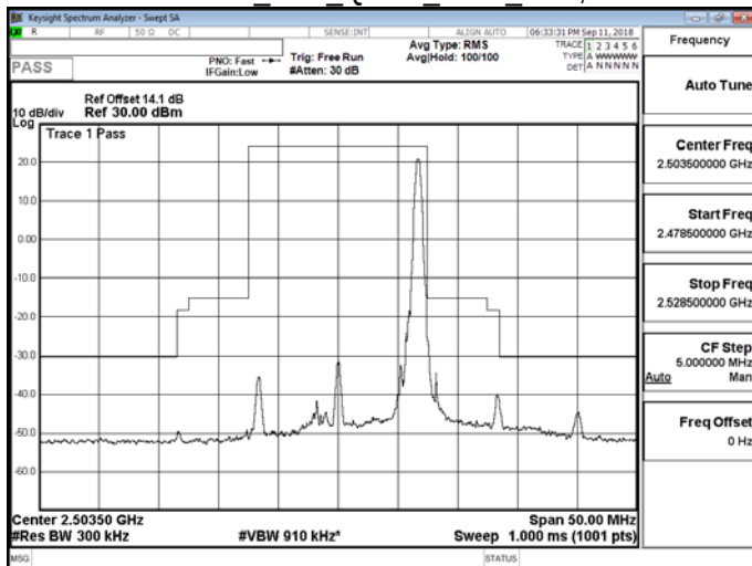
Band 41 15M QPSK LOW RB75,0
