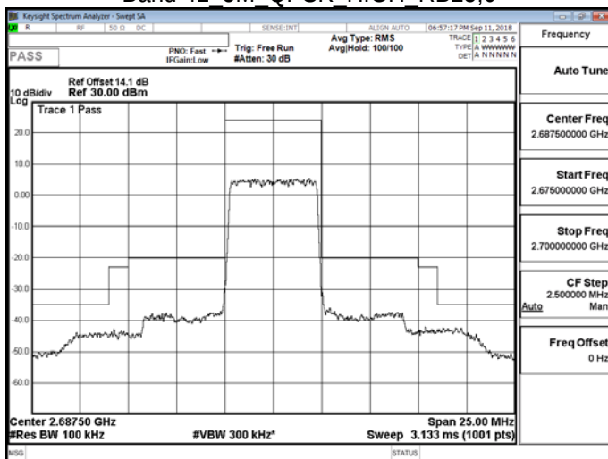
Band 41 5M QPSK HIGH RB25,0
