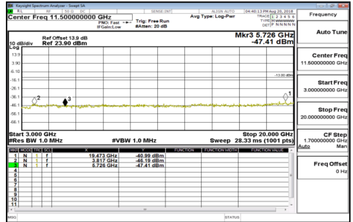
3GHz~20GHz_Band2_3MHz_QPSK_1_0_MidCH18900-1880
