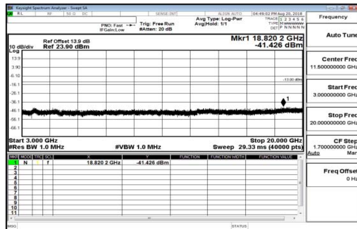
3GHz~20GHz_Band2_1_4MHz_QPSK_1_0_MidCH18900-1880
