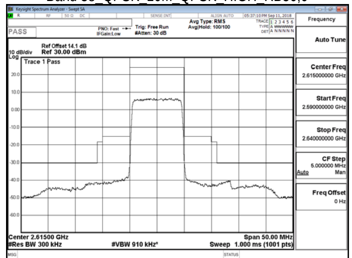
Band 38 QPSK 10M QPSK HIGH RB50,0
