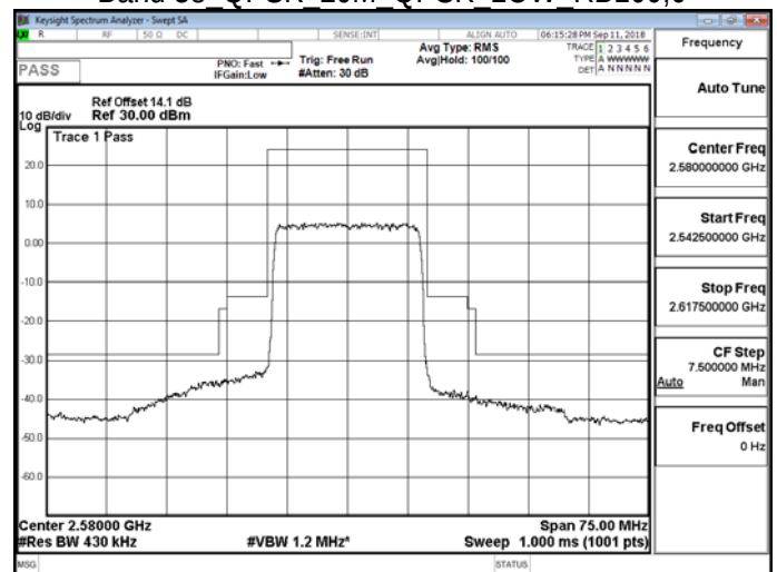
Band 38 QPSK 20M QPSK LOW RB100,0
