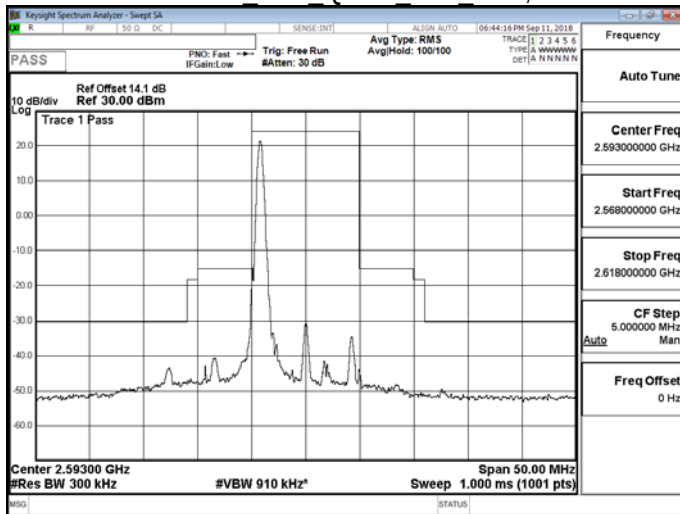
Band 41 10M QPSK MID RB1,49
