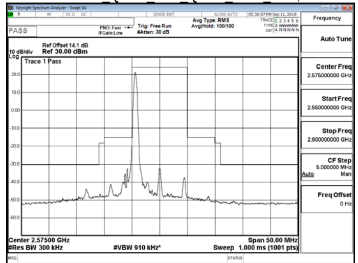
Band 38 QPSK 10M QPSK LOW RB1,49
