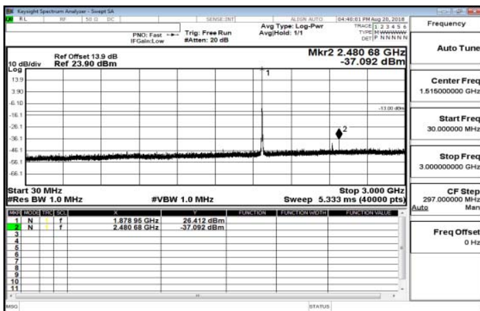
30MHz~3GHz_Band2_3MHz_QPSK_1_0_MidCH18900-1880
