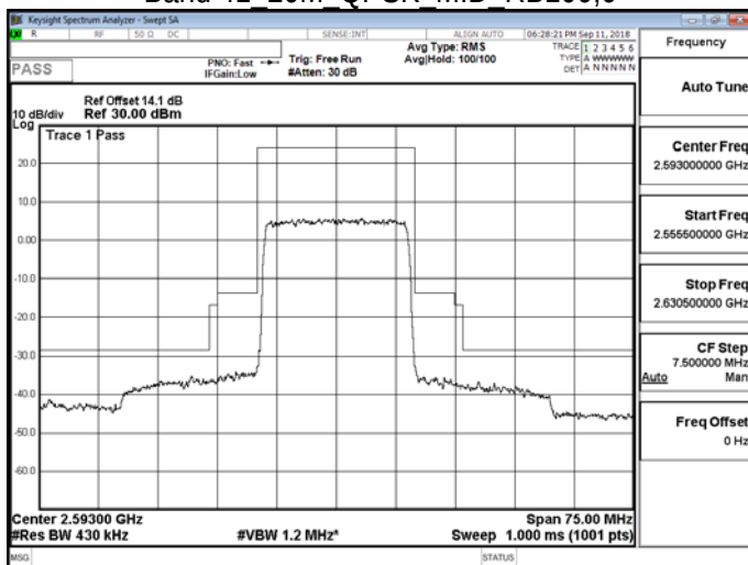
Band 41 20M QPSK MID RB100,0
