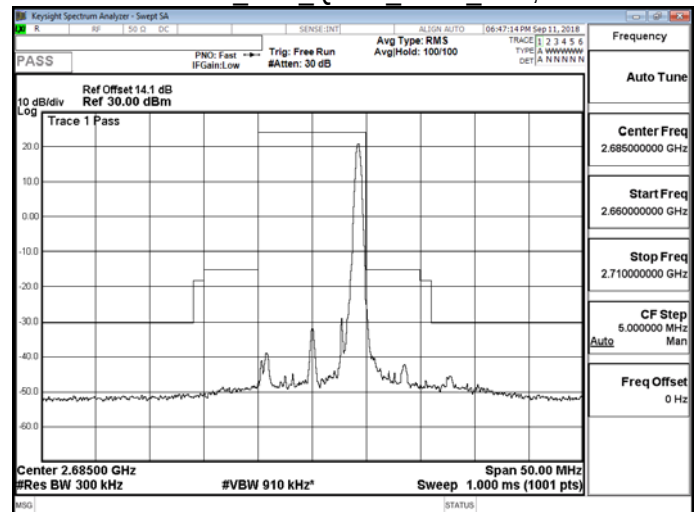
Band 41 10M QPSK HIGH RB50,0
