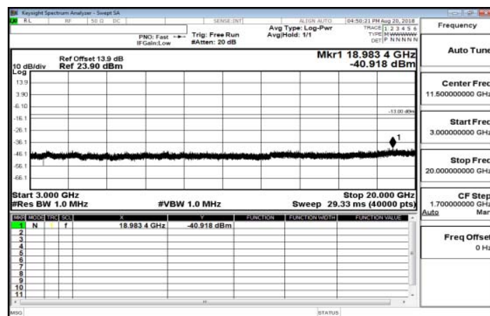
3GHz~20GHz_Band2_1_4MHz_QPSK_1_0_HighCH19193-1909.3
