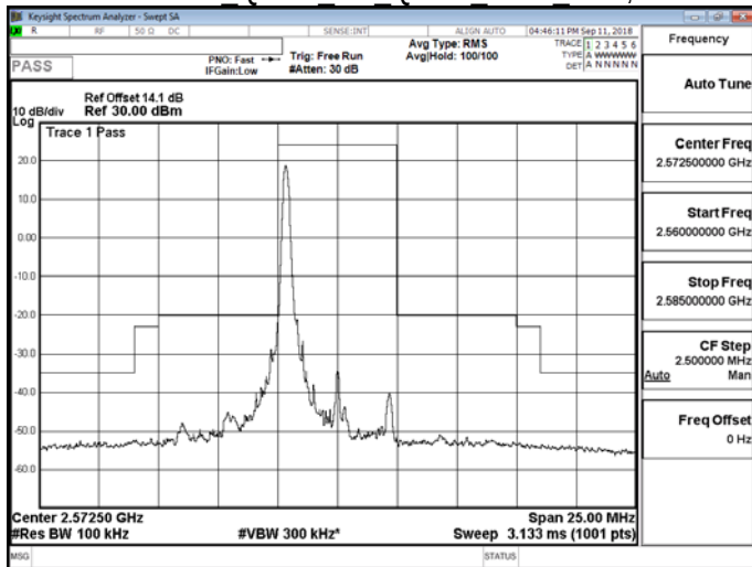
Band 38 QPSK 5M QPSK LOW RB1,24
