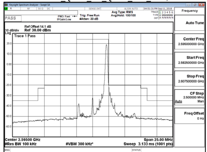
Band 38 QPSK 5M QPSK MID RB25,0
