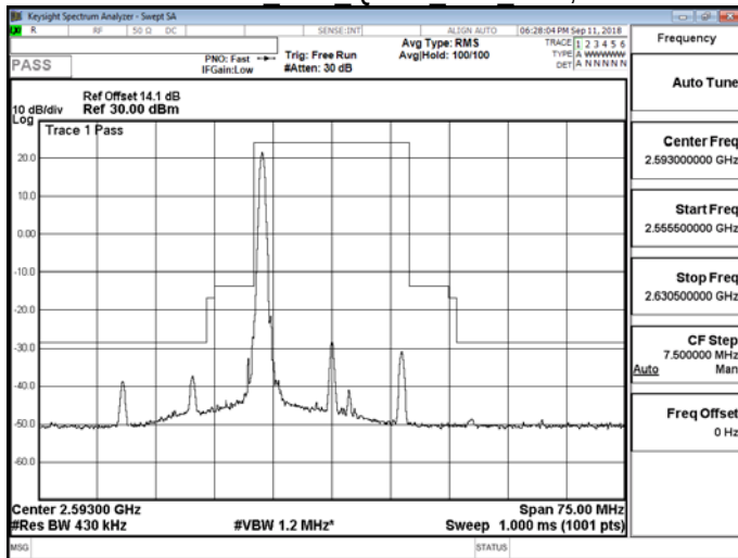
Band 41 20M QPSK MID RB1,99
