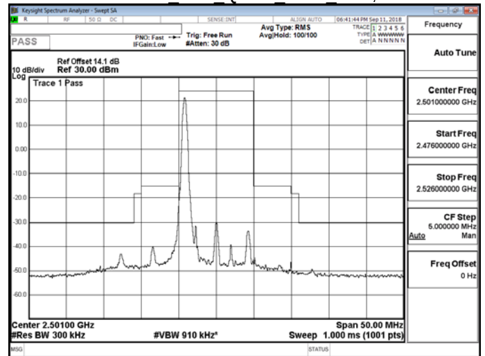
Band 41 10M QPSK LOW RB1,49
