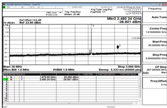
30MHz~3GHz_Band2_1_4MHz_QPSK_1_0_MidCH18900-1880
