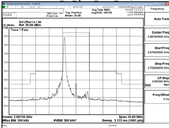
Band 41 5M QPSK HIGH RB1,24
