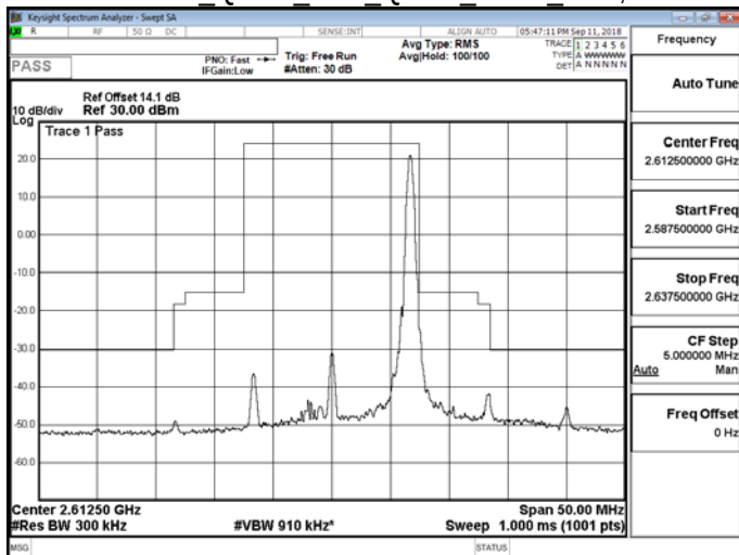
Band 38 QPSK 15M QPSK HIGH RB75,0
