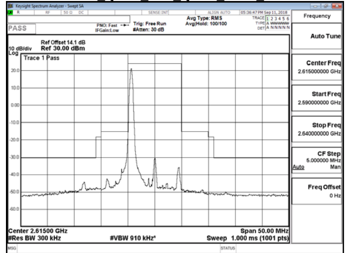
Band 38 QPSK 10M QPSK HIGH RB1,49
