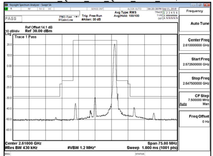
Band 38 QPSK 20M QPSK HIGH RB100,0
