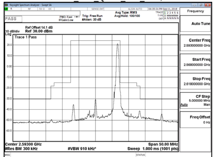
Band 41 15M QPSK MID RB75,0
