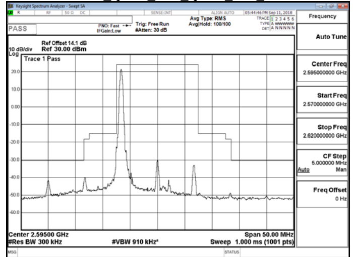
Band 38 QPSK 15M QPSK MID RB1,74
