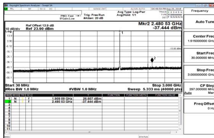
30MHz~3GHz_Band2_1_4MHz_QPSK_1_0_HighCH19193-1909.3
