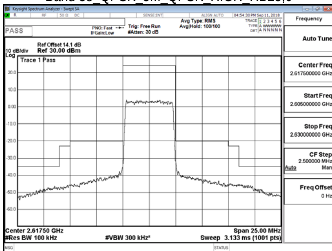
Band 38 QPSK 5M QPSK HIGH RB25,0
