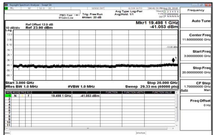
3GHz~20GHz_Band2_3MHz_QPSK_1_0_HighCH19185-1908.5
