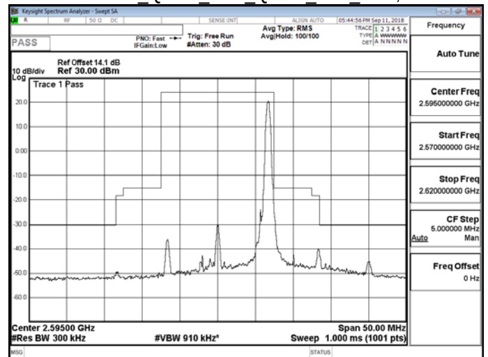
Band 38 QPSK 15M QPSK MID RB75,0
