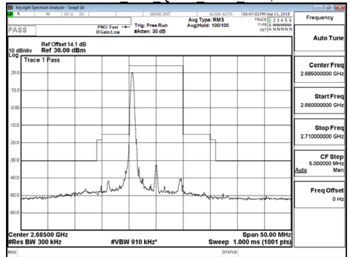
Band 41 10M QPSK HIGH RB1,49
