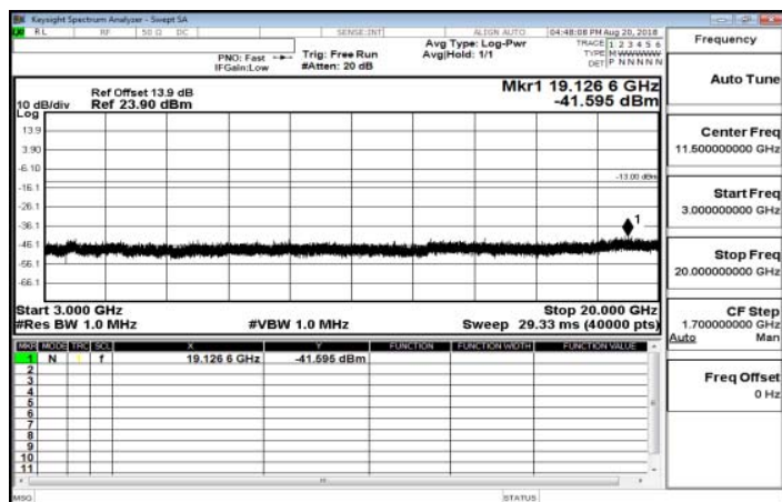
3GHz~20GHz_Band2_1_4MHz_QPSK_1_0_LowCH18607-1850.7
