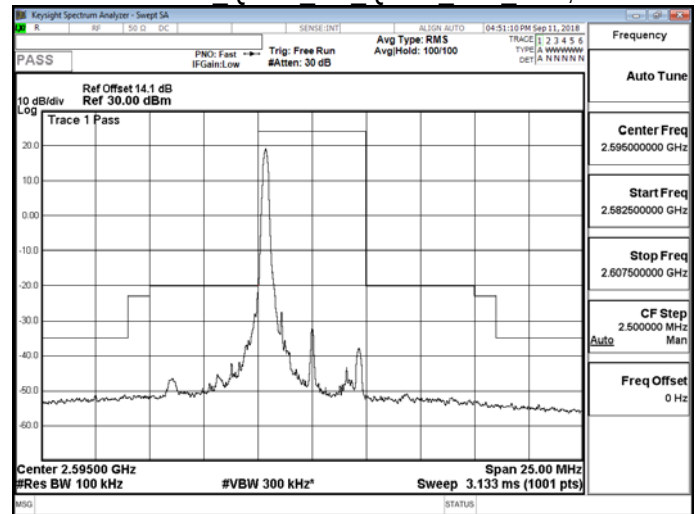
Band 38 QPSK 5M QPSK MID RB1,24
