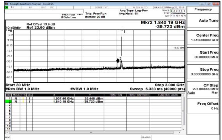
30MHz~3GHz_Band2_3MHz_QPSK_1_0_HighCH19185-1908.5
