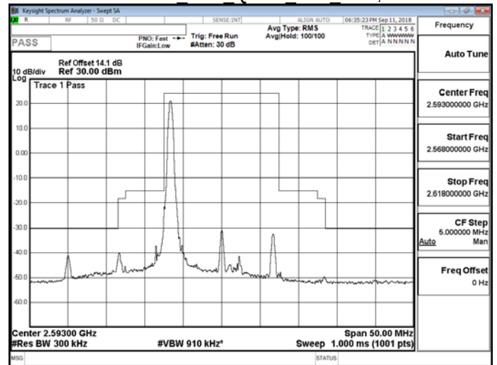
Band 41 15M QPSK MID RB1,74
