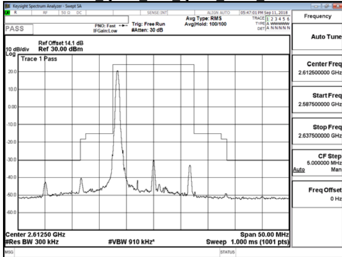
Band 38 QPSK 15M QPSK HIGH RB1,74
