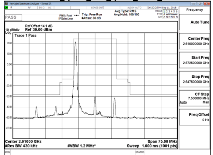
Band 38 QPSK 20M QPSK HIGH RB1,99
