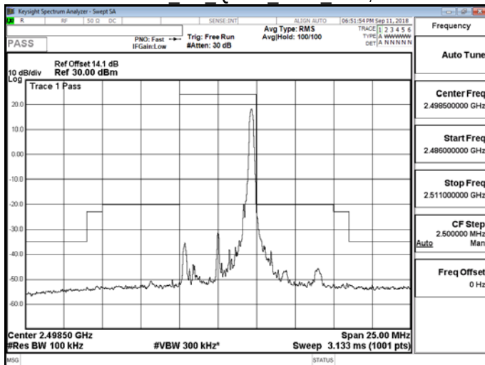
Band 41 5M QPSK LOW RB25,0
