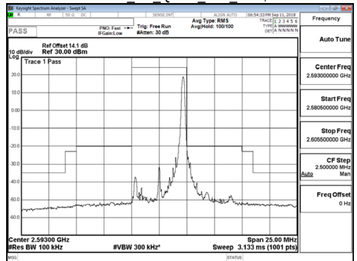
Band 41 5M QPSK MID RB25,0
