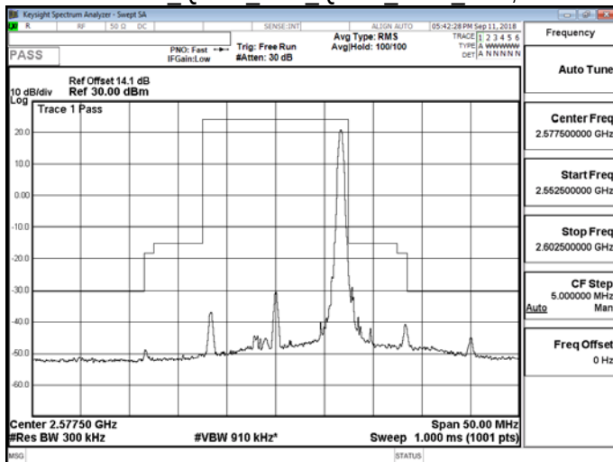
Band 38 QPSK 15M QPSK LOW RB75,0
