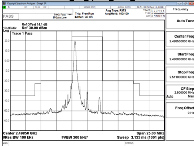
Band 41 5M QPSK LOW RB1,24
