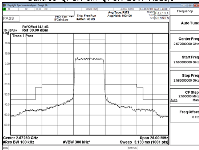
Band 38 QPSK 5M QPSK LOW RB25,0
