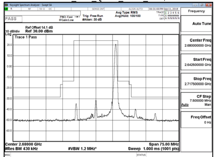
Band 41 20M QPSK HIGH RB100,0
