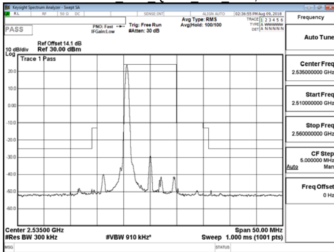
Band 7 10M QPSK MID RB1,49
