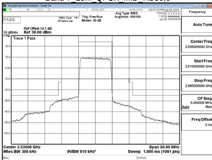
Band 7 10M QPSK MID RB50,0
