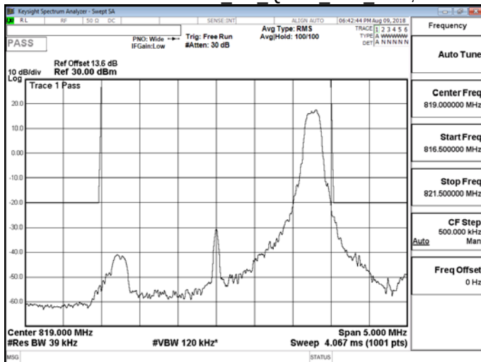
Band26 for Part 90S 3M QPSK MID RB15,0
