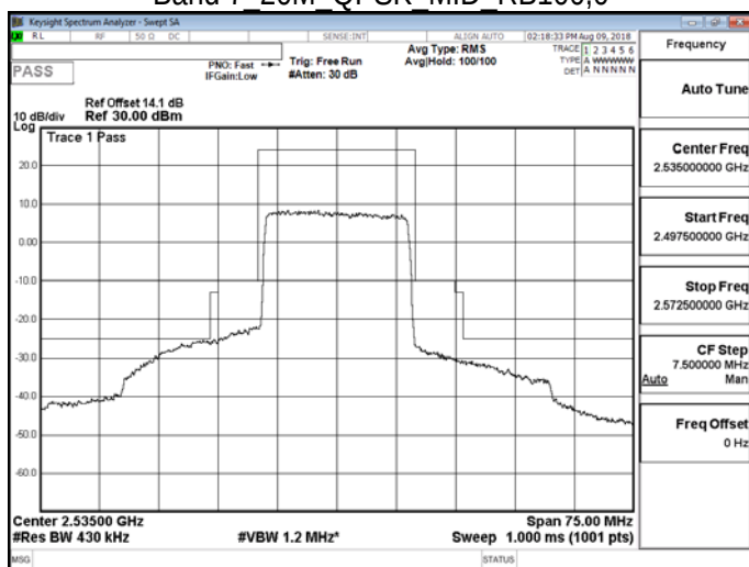
Band 7 20M QPSK MID RB100,0
