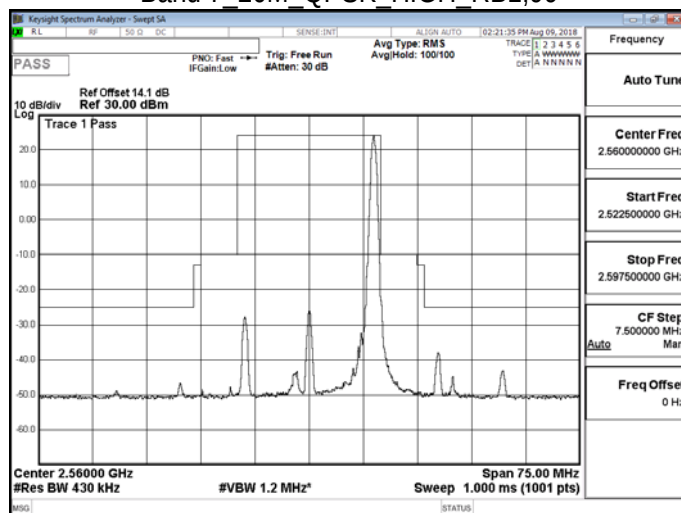
Band 7 20M QPSK HIGH RB100,0
