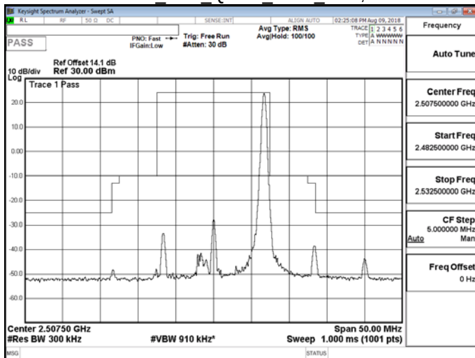
Band 7 15M QPSK LOW RB75,0
