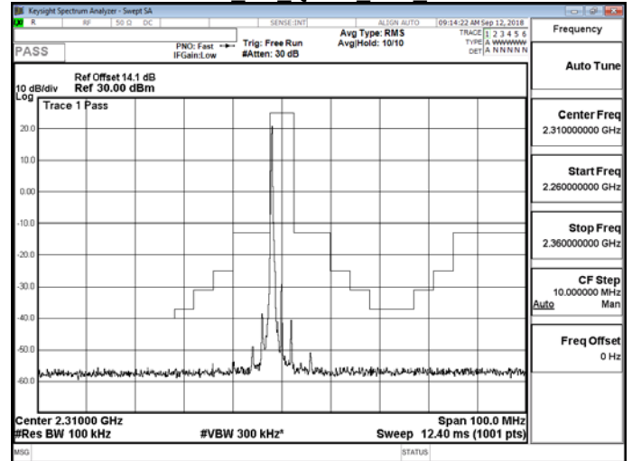
Band 30 5M QPSK MID RB1,24
