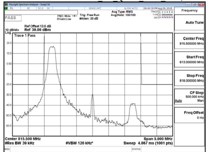
Band26 for Part 90S 3M QPSK LOW RB1,14
