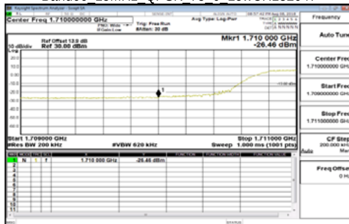
Band66 15MHz QPSK 75 0 LowCH132047
