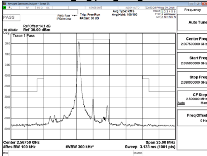
Band 7 5M QPSK HIGH RB1,24
