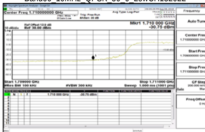
Band66 10MHz QPSK 50 0 LowCH132022
