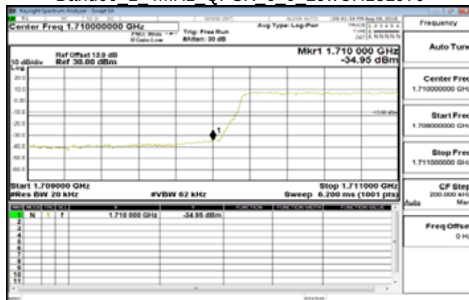
Band66 1 4MHz QPSK 6 0 LowCH131979
