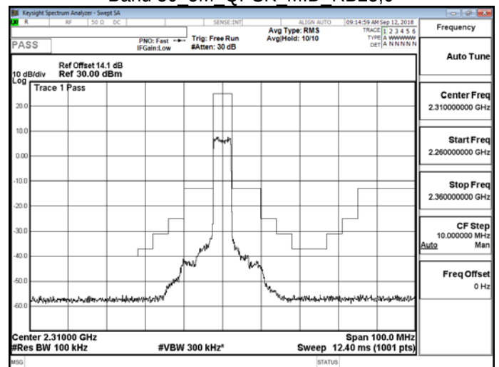
Band 30 5M QPSK MID RB25,0
