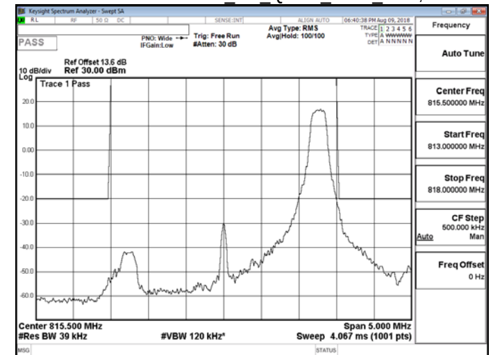
Band26 for Part 90S 3M QPSK LOW RB15,0
