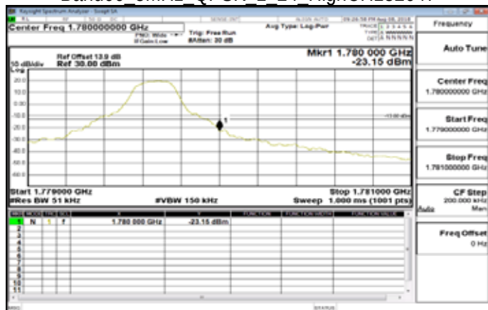
Band66 5MHz QPSK 1 24 HighCH132647
