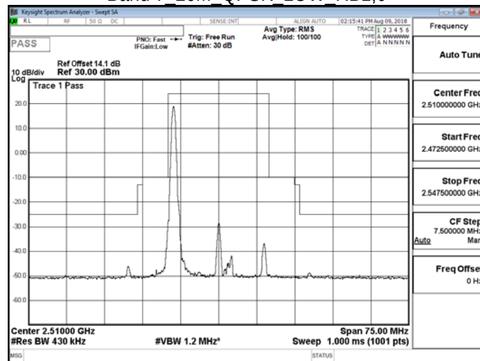
Band 7 20M QPSK LOW RB1,99
