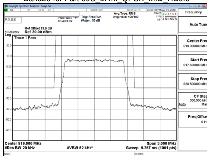
Band26 for Part 90S 1.4M QPSK MID RB6,0
