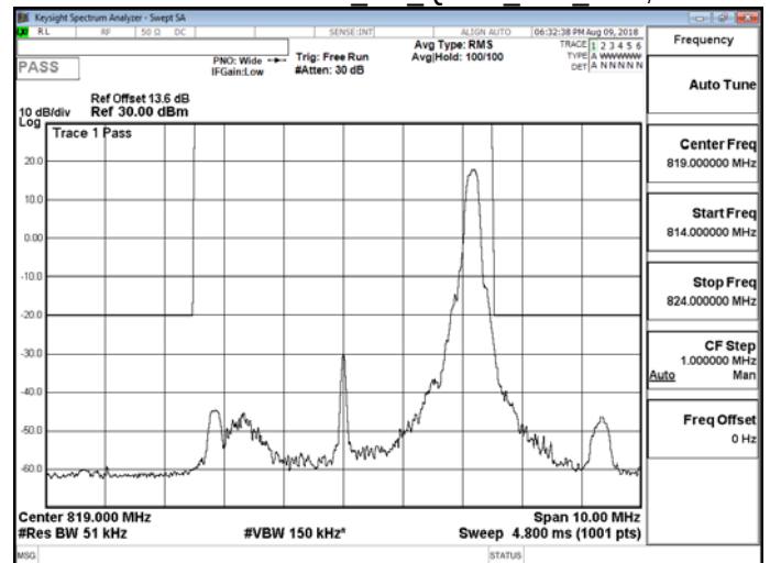
Band26 for Part 90S 5M QPSK MID RB25,0
