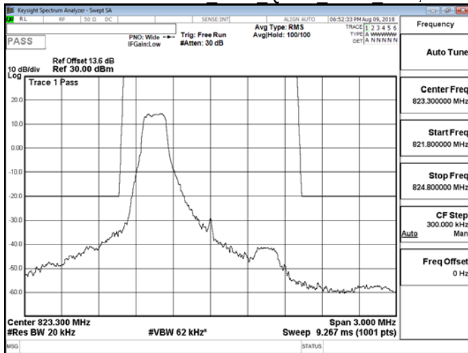
Band26 for Part 90S 1.4M QPSK HIGH RB1,5
