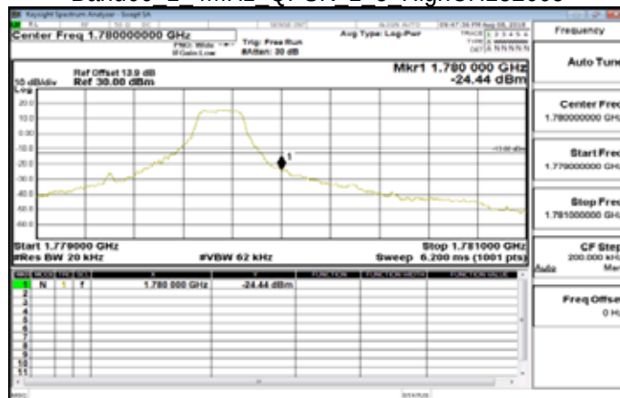
Band66 1 4MHz QPSK 1 5 HighCH132665
