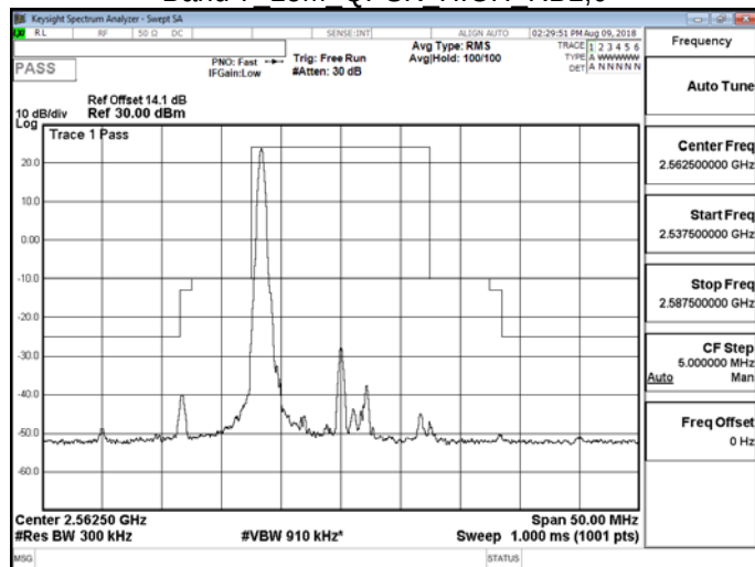
Band 7 15M QPSK HIGH RB1,74
