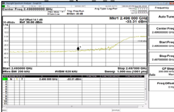
Band41 15MHz QPSK 75 0 LowCH39725
