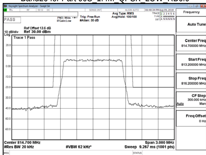
Band26 for Part 90S 1.4M QPSK LOW RB6,0
