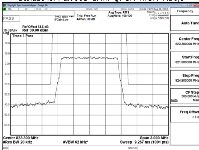
Band26 for Part 90S 1.4M QPSK HIGH RB6,0
