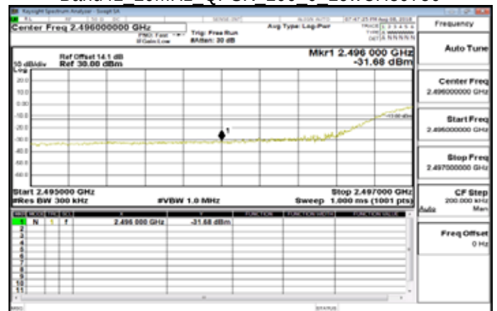
Band41 20MHz QPSK 100 0 LowCH39750
