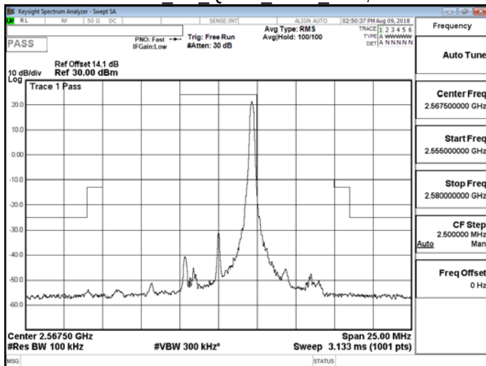
Band 7 5M QPSK HIGH RB25,0
