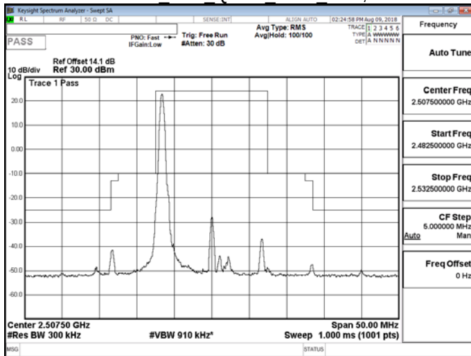
Band 7 15M QPSK LOW RB1,74
