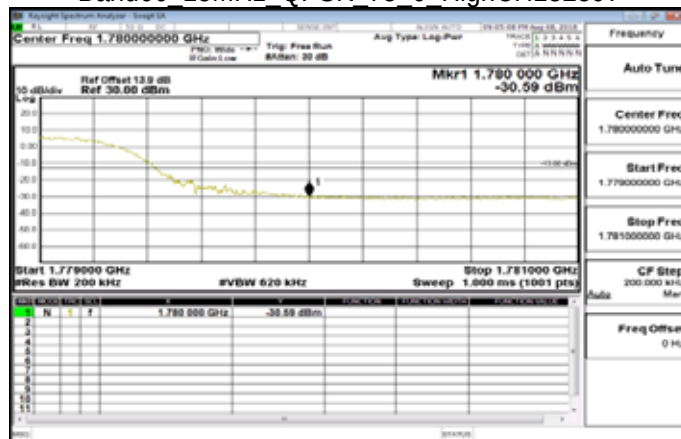
Band66 15MHz QPSK 75 0 HighCH132597
