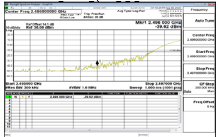
Band41 20MHz QPSK 1 0 LowCH39750
