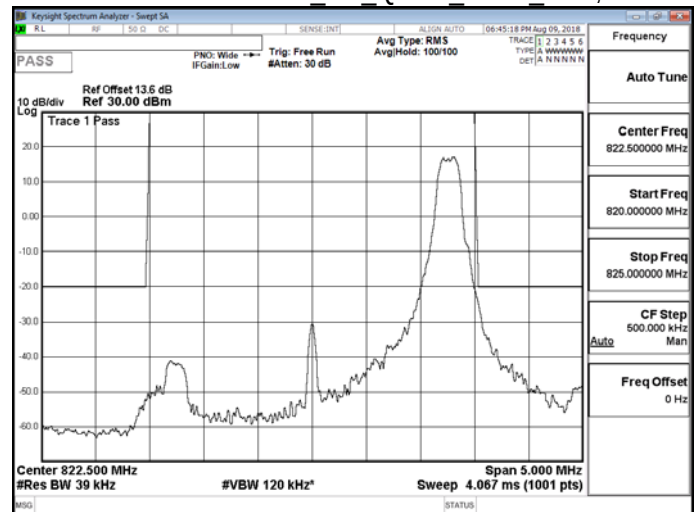
Band26 for Part 90S 3M QPSK HIGH RB15,0
