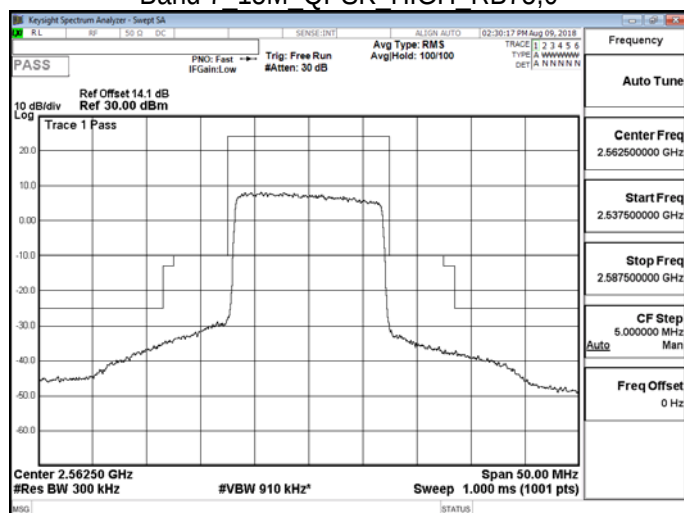
Band 7 15M QPSK HIGH RB75,0
