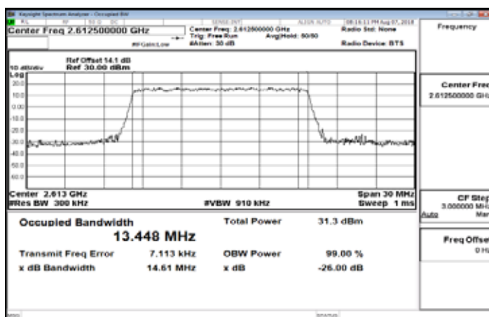
Band38_15MHz_QPSK_75_0_HighCH38175
