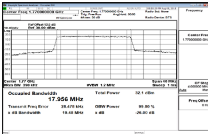
Band66_20MHz_QPSK_100_0_HighCH132572
