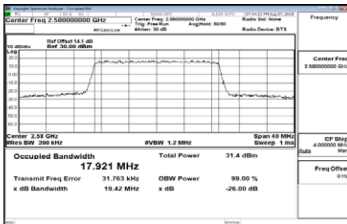
Band38_20MHz_QPSK_100_0_MidCH38000
