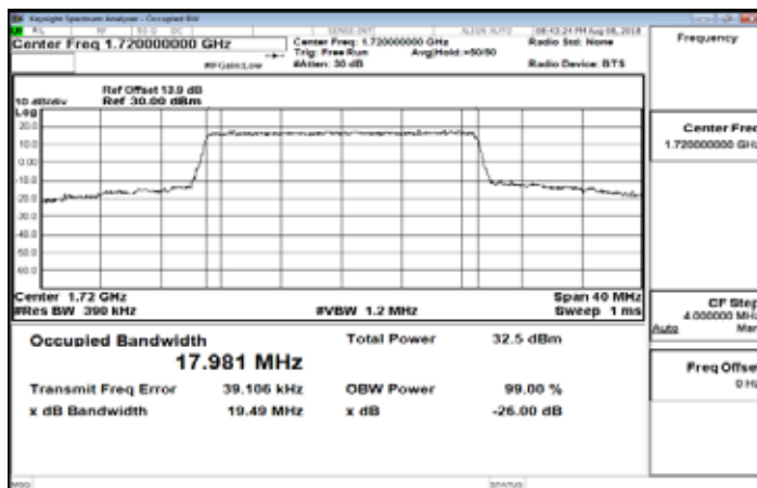
Band66_20MHz_QPSK_100_0_MidCH132322
