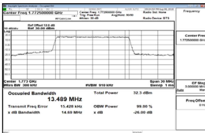
Band66_15MHz_QPSK_75_0_HighCH132597
