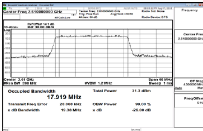
Band38_20MHz_QPSK_100_0_HighCH38150
