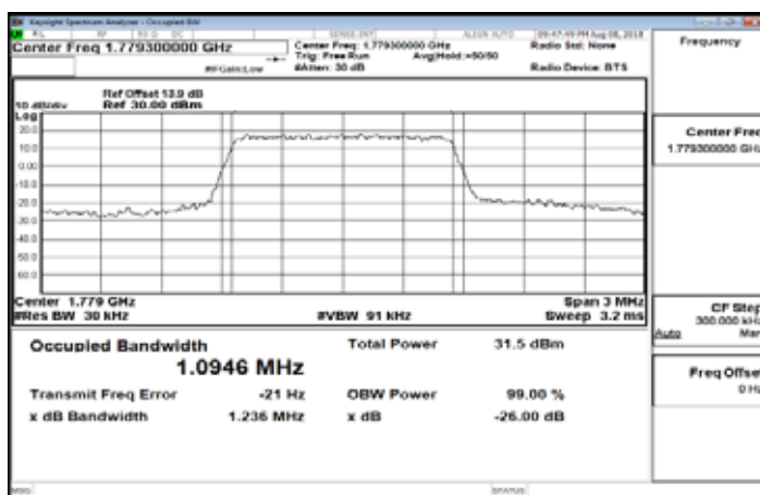
Band66_1_4MHz_QPSK_6_0_HighCH132665
