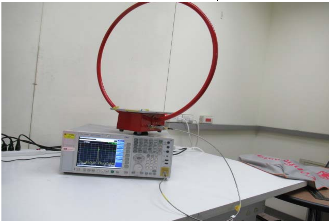
Frequency stability Setup Photo
