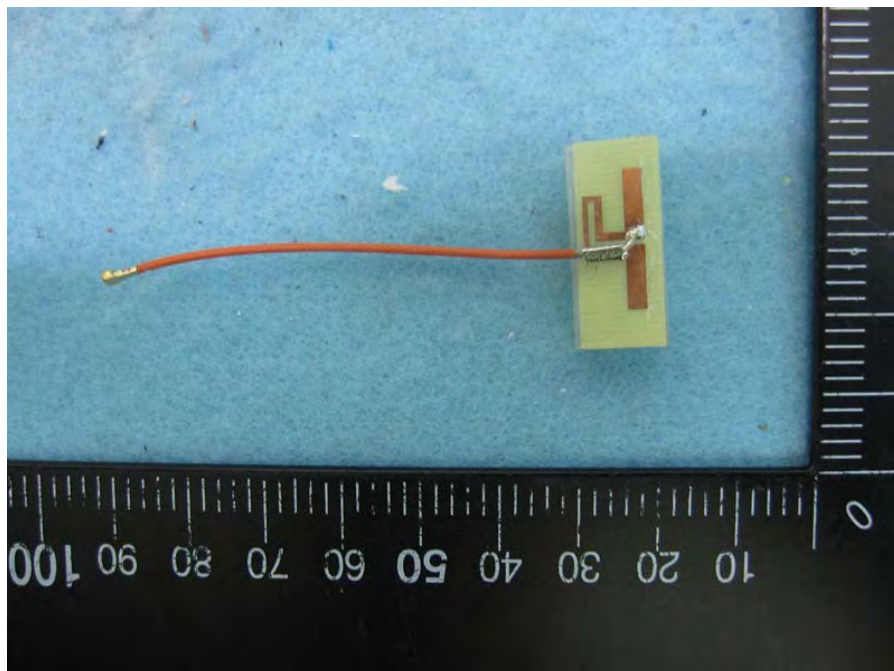
Dipole Antenna (for 5GHz)
