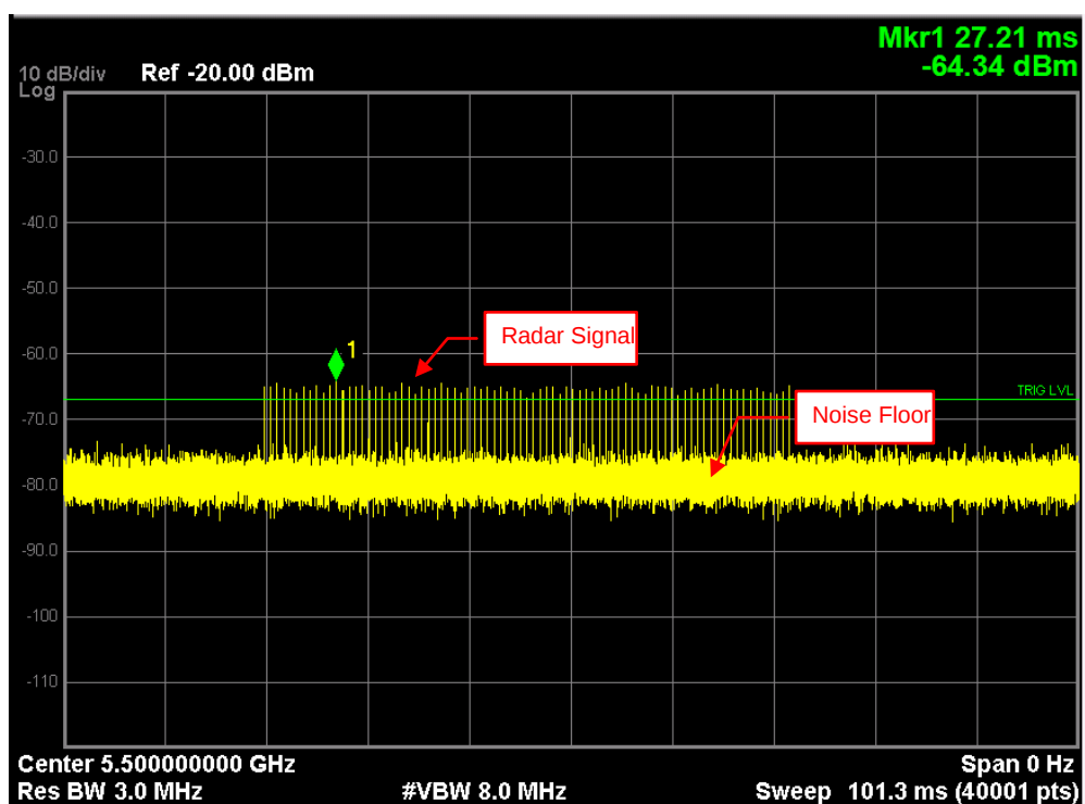
Radar Signal 1 (Test B)
